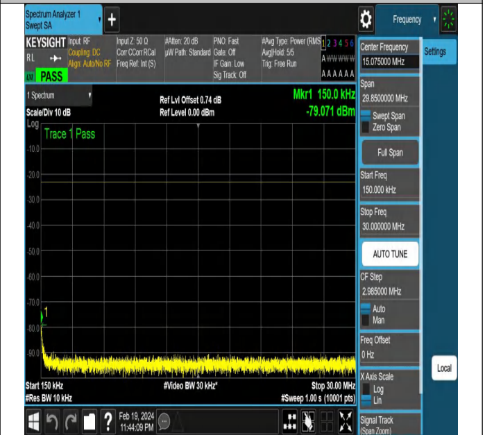
NTNV-N12-PC3-15-15-M-DFT-PI2BPSK-Edge_1RB_Right-An t1-PASS
