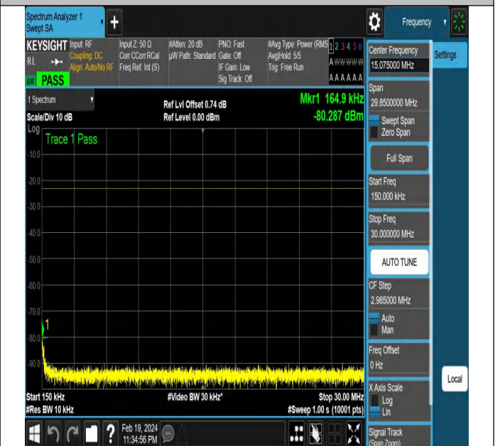
NTNV-N12-PC3-15-15-L-DFT-PI2BPSK-Edge_1RB_Right-Ant 1-PASS
