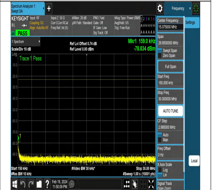
NTNV-N12-PC3-15-15-M-CP-QPSK-Edge_1RB_Right-Ant1-P ASS
