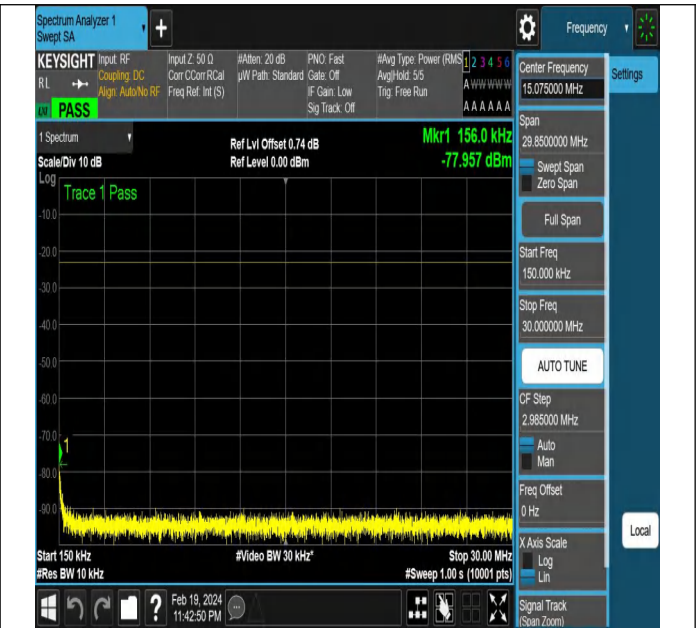
NTNV-N12-PC3-15-15-M-DFT-PI2BPSK-Edge_1RB_Left-Ant1
