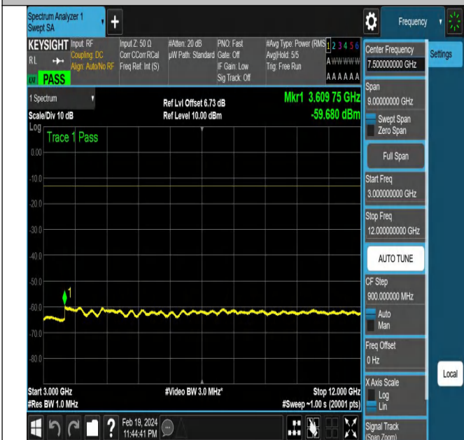
NTNV-N12-PC3-15-15-M-DFT-PI2BPSK-Edge_1RB_Right-An t1-PASS
