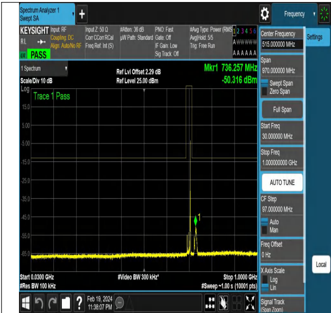
NTNV-N12-PC3-15-15-L-DFT-QPSK-Edge_1RB_Right-Ant1-P
