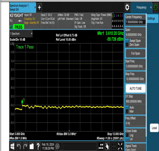
NTNV-N12-PC3-15-15-L-DFT-QPSK-Edge_1RB_Right-Ant1-P
