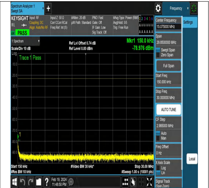
NTNV-N12-PC3-15-15-M-CP-QPSK-Edge_1RB_Left-Ant1-PA SS
