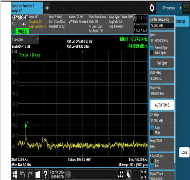
NTNV-N12-PC3-15-15-M-CP-QPSK-Edge_1RB_Right-Ant1-P ASS
