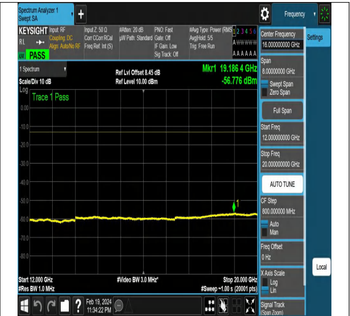
NTNV-N12-PC3-15-15-L-DFT-PI2BPSK-Edge_1RB_Left-Ant1- PASS
