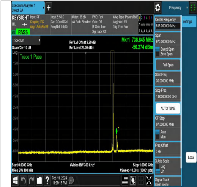
NTNV-N12-PC3-15-10-H-DFT-QPSK-Edge_1RB_Right-Ant1-
