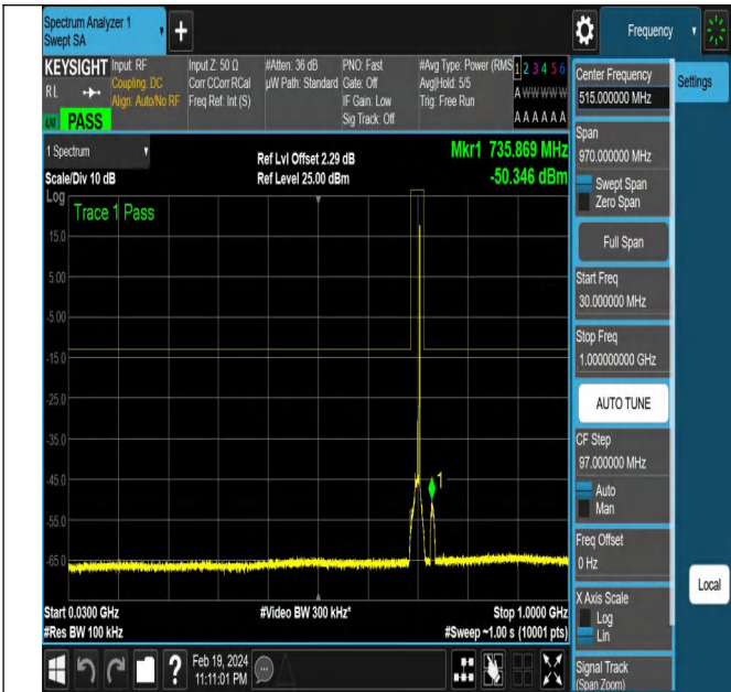
NTNV-N12-PC3-15-10-M-DFT-PI2BPSK-Edge_1RB_Right-An t1-PASS
