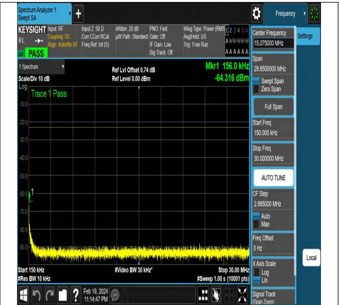
NTNV-N12-PC3-15-10-M-CP-QPSK-Edge_1RB_Left-Ant1-PA SS
