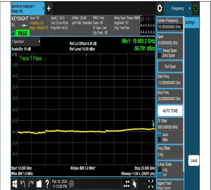
NTNV-N12-PC3-15-10-M-DFT-QPSK-Edge_1RB_Left-Ant1-P
