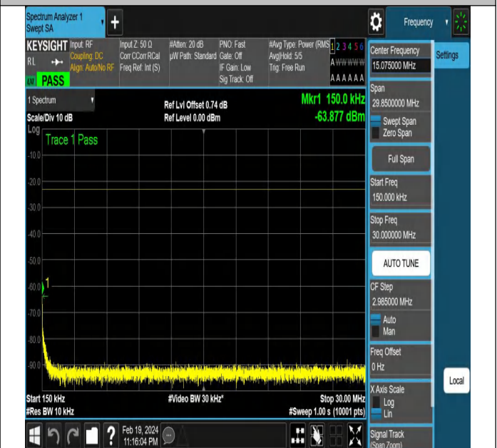
NTNV-N12-PC3-15-10-M-CP-QPSK-Edge_1RB_Right-Ant1-P ASS
