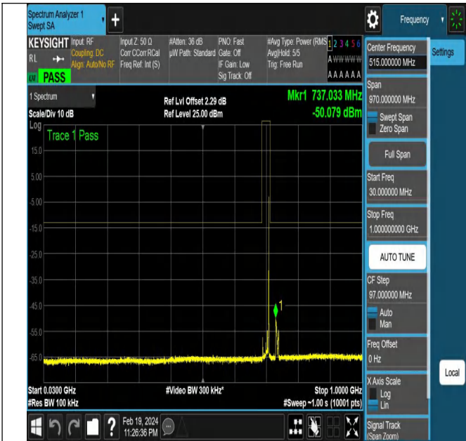
NTNV-N12-PC3-15-10-H-DFT-PI2BPSK-Edge_1RB_Right-Ant 1-PASS
