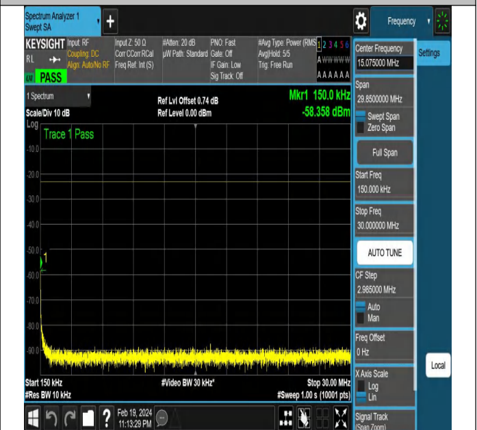
NTNV-N12-PC3-15-10-M-DFT-QPSK-Edge_1RB_Right-Ant1-
