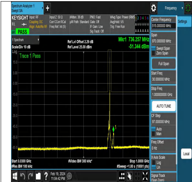
NTNV-N12-PC3-15-10-L-DFT-QPSK-Edge_1RB_Right-Ant1-P
