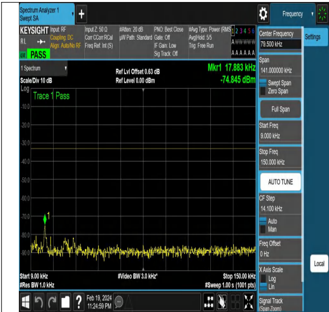
NTNV-N12-PC3-15-10-H-DFT-PI2BPSK-Edge_1RB_Left-Ant1
