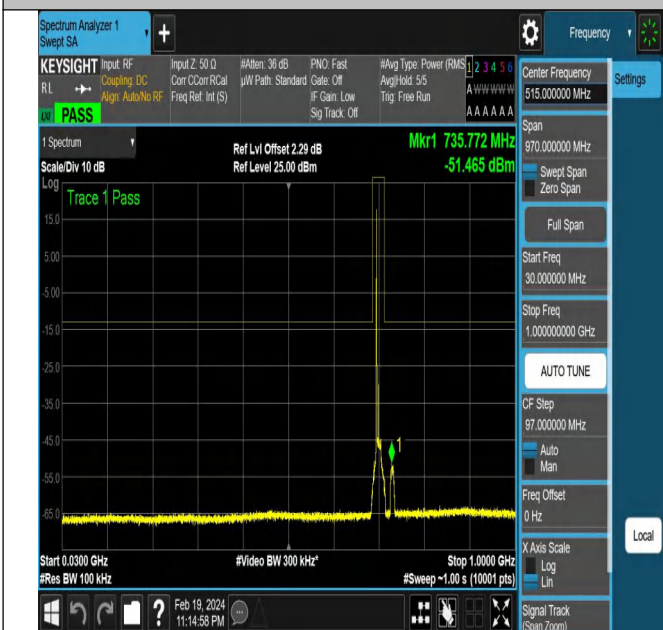
NTNV-N12-PC3-15-10-M-CP-QPSK-Edge_1RB_Left-Ant1-PA SS
