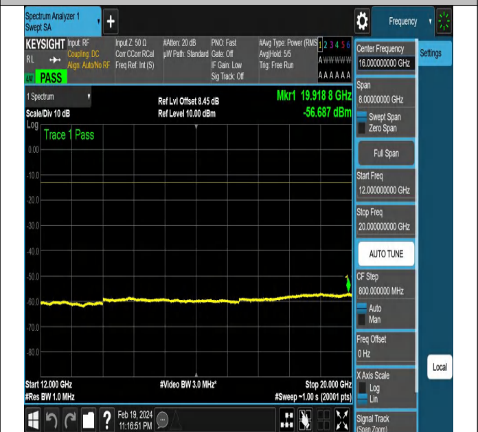
NTNV-N12-PC3-15-10-M-CP-QPSK-Edge_1RB_Right-Ant1-P
