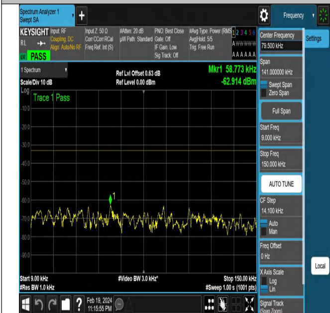
NTNV-N12-PC3-15-10-M-CP-QPSK-Edge_1RB_Right-Ant1-P ASS
