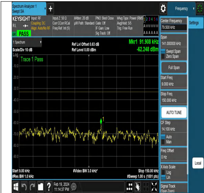
NTNV-N12-PC3-15-10-M-CP-QPSK-Edge_1RB_Left-Ant1-PA SS
