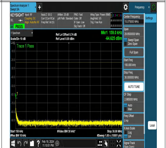
NTNV-N12-PC3-15-10-M-DFT-PI2BPSK-Edge_1RB_Right-An t1-PASS
