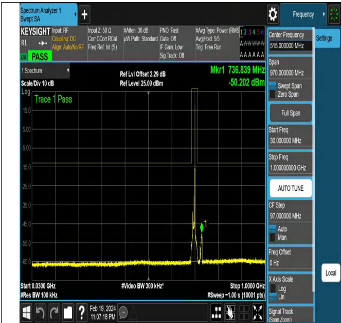
NTNV-N12-PC3-15-10-L-CP-QPSK-Edge_1RB_Right-Ant1-P
