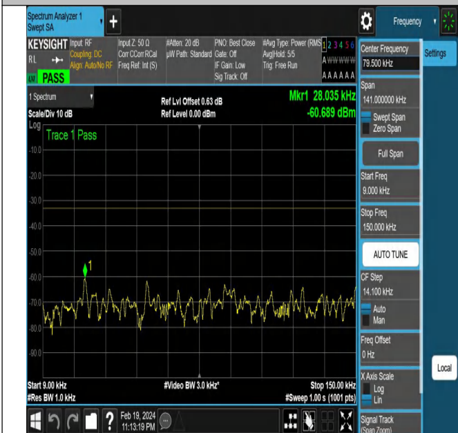
NTNV-N12-PC3-15-10-M-DFT-QPSK-Edge_1RB_Right-Ant1-
