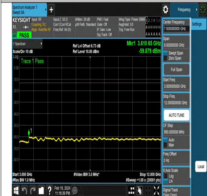
NTNV-N12-PC3-15-10-M-CP-QPSK-Edge_1RB_Right-Ant1-P
