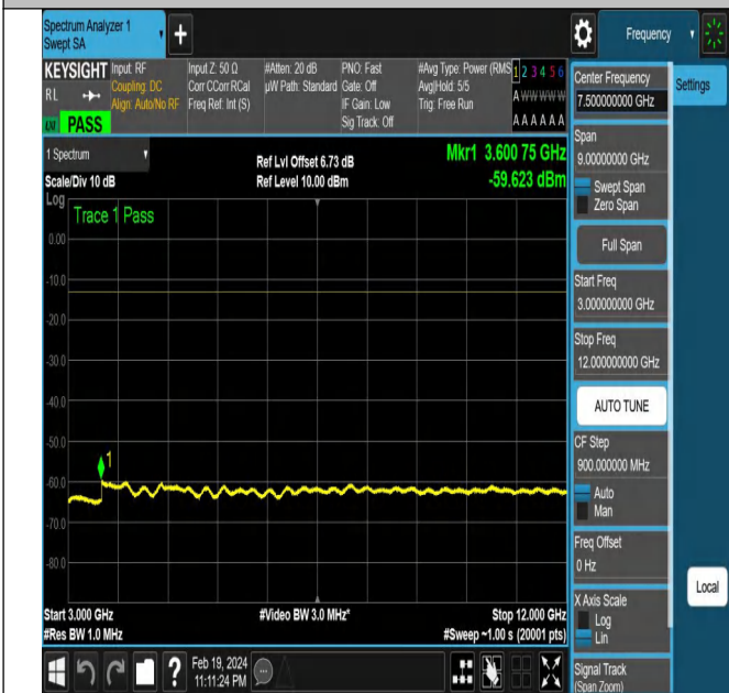
NTNV-N12-PC3-15-10-M-DFT-PI2BPSK-Edge_1RB_Right-An t1-PASS
