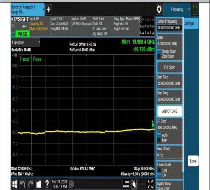
NTNV-N12-PC3-15-10-M-DFT-QPSK-Edge_1RB_Right-Ant1-
