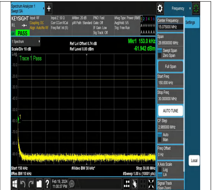
NTNV-N12-PC3-15-10-L-DFT-PI2BPSK-Edge_1RB_Left-Ant1-
