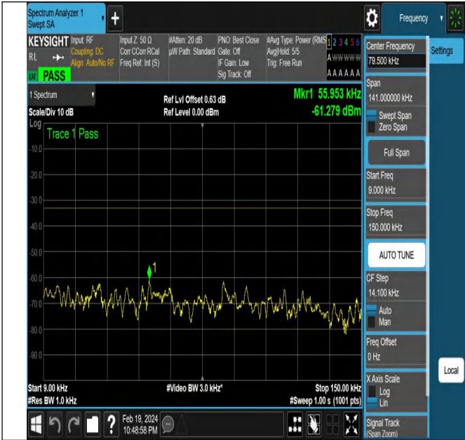
NTNV-N12-PC3-15-5-M-CP-QPSK-Edge_1RB_Left-Ant1-PAS
