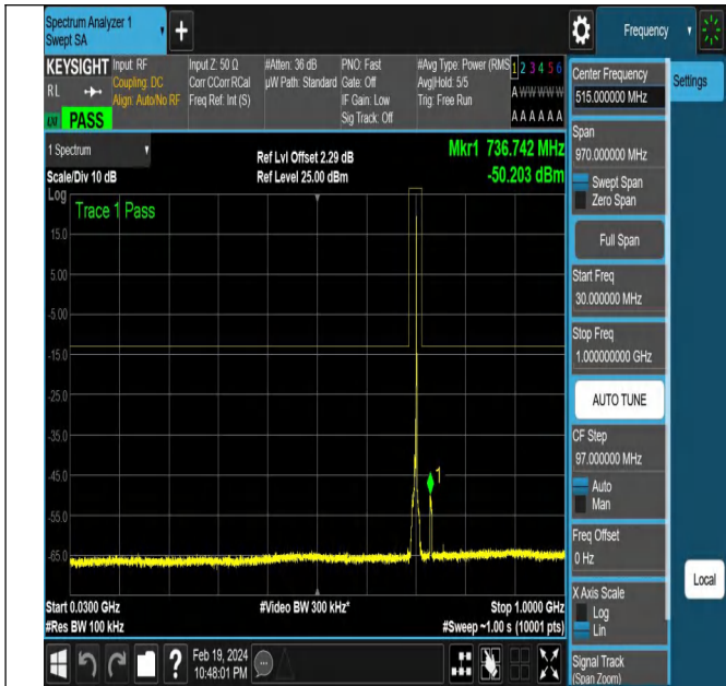
NTNV-N12-PC3-15-5-M-DFT-QPSK-Edge_1RB_Right-Ant1-P
