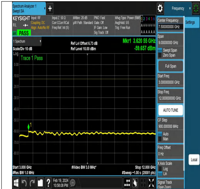
NTNV-N12-PC3-15-5-H-CP-QPSK-Edge_1RB_Left-Ant1-PAS S
