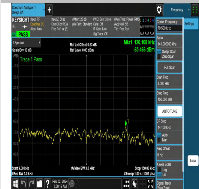
NTNV-N5-PC3-15-15-H-DFT-PI2BPSK-Edge_1RB_Right-Ant1
