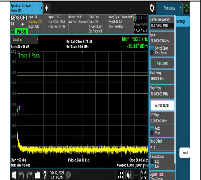
NTNV-N5-PC3-15-15-H-DFT-QPSK-Edge_1RB_Right-Ant1-P
