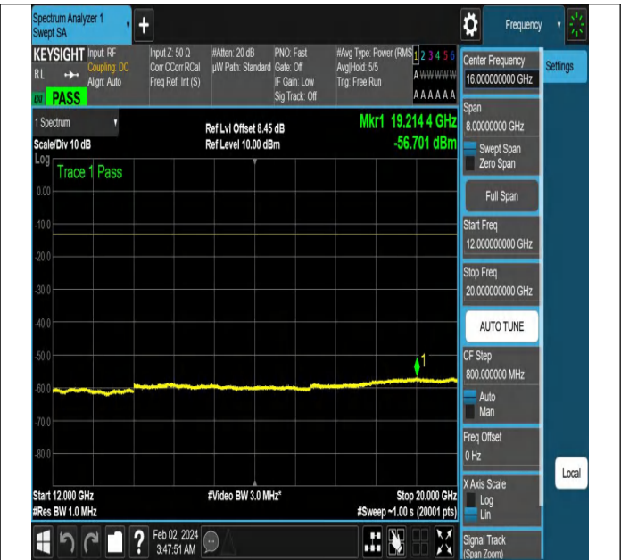
NTNV-N5-PC3-15-20-L-DFT-QPSK-Edge_1RB_Left-Ant1-PAS
