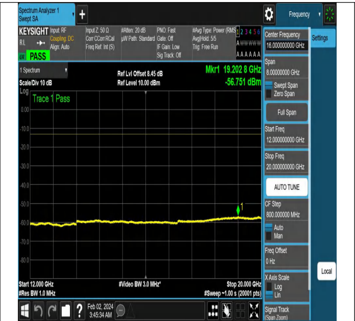
NTNV-N5-PC3-15-20-L-DFT-PI2BPSK-Edge_1RB_Left-Ant1-
