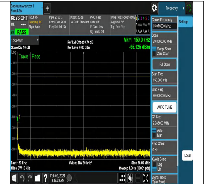
NTNV-N5-PC3-15-15-H-DFT-PI2BPSK-Edge_1RB_Left-Ant1- PASS
