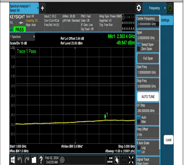
NTNV-N5-PC3-15-15-H-CP-QPSK-Edge_1RB_Left-Ant1-PAS
