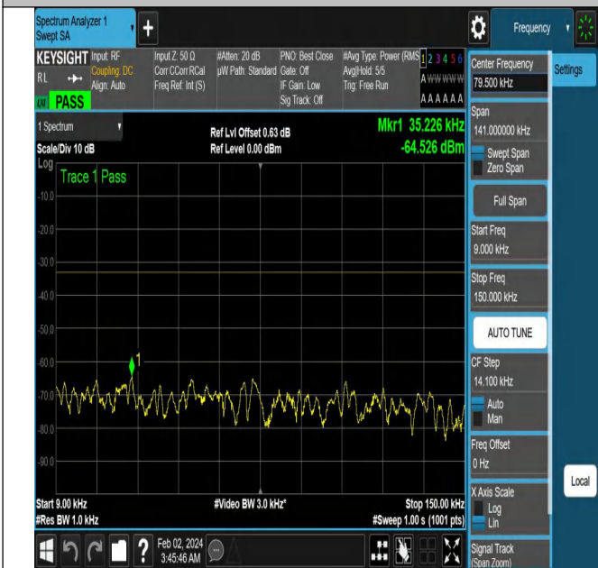
NTNV-N5-PC3-15-20-L-DFT-PI2BPSK-Edge_1RB_Right-Ant1
