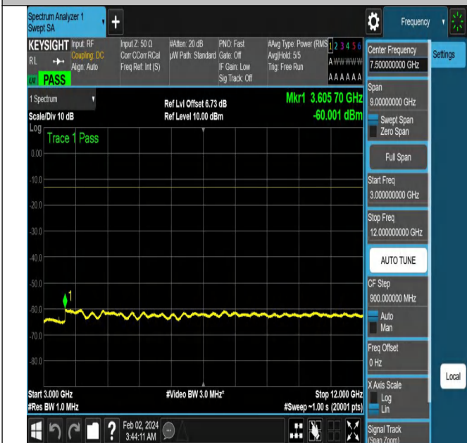
NTNV-N5-PC3-15-15-H-CP-QPSK-Edge_1RB_Right-Ant1-PA
