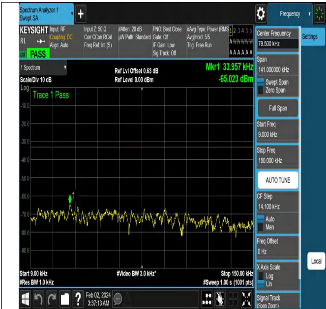
NTNV-N5-PC3-15-15-H-DFT-PI2BPSK-Edge_1RB_Left-Ant1- PASS
