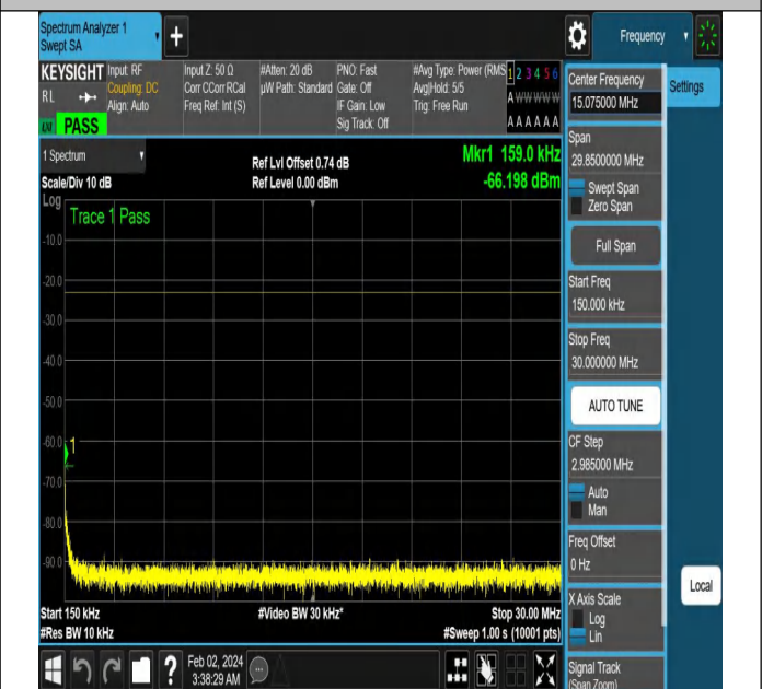
NTNV-N5-PC3-15-15-H-DFT-PI2BPSK-Edge_1RB_Right-Ant1
