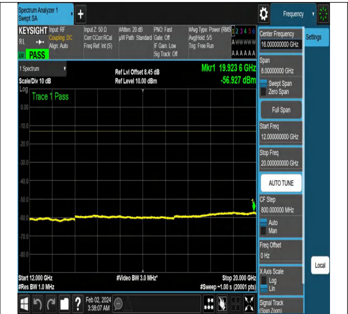
NTNV-N5-PC3-15-15-H-DFT-PI2BPSK-Edge_1RB_Left-Ant1-
