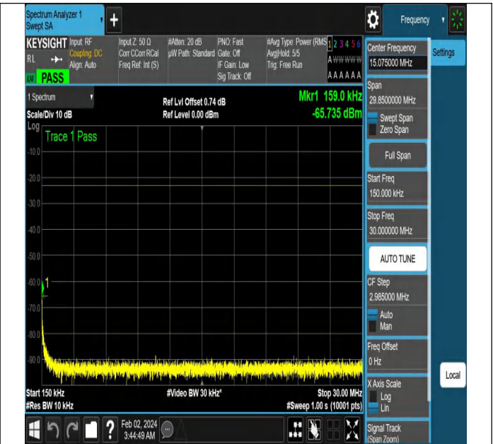
NTNV-N5-PC3-15-20-L-DFT-PI2BPSK-Edge_1RB_Left-Ant1- PASS
