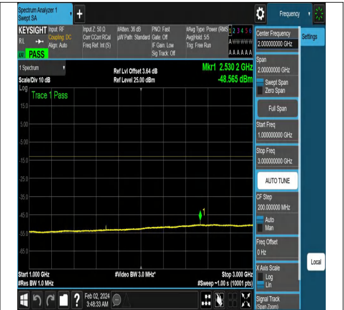
NTNV-N5-PC3-15-20-L-DFT-QPSK-Edge_1RB_Right-Ant1-PA
