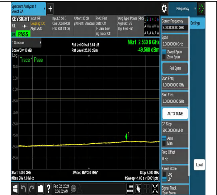
NTNV-N5-PC3-15-15-M-CP-QPSK-Edge_1RB_Right-Ant1-PA
