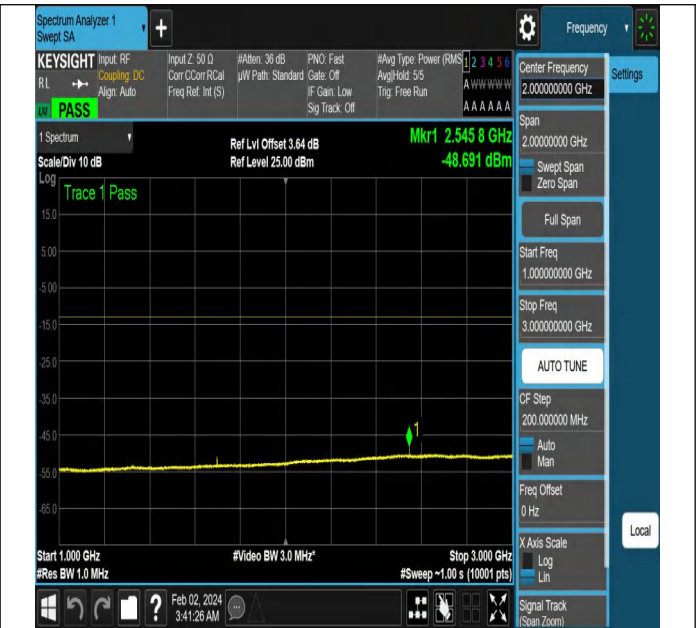
NTNV-N5-PC3-15-15-H-DFT-QPSK-Edge_1RB_Right-Ant1-P
