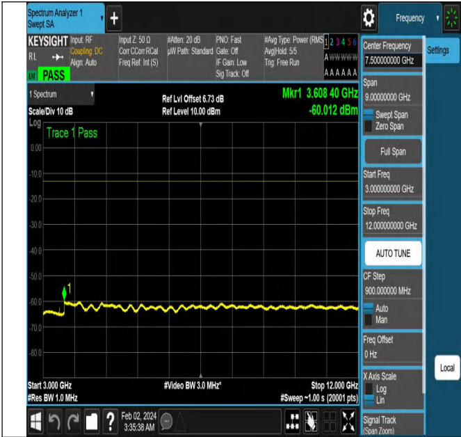
NTNV-N5-PC3-15-15-M-CP-QPSK-Edge_1RB_Left-Ant1-PAS
