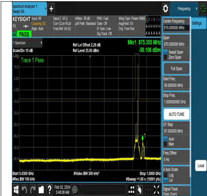
NTNV-N5-PC3-15-20-L-DFT-PI2BPSK-Edge_1RB_Right-Ant1
