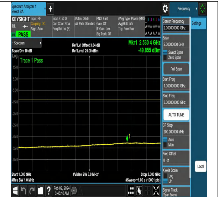
NTNV-N5-PC3-15-20-L-DFT-PI2BPSK-Edge_1RB_Right-Ant1
