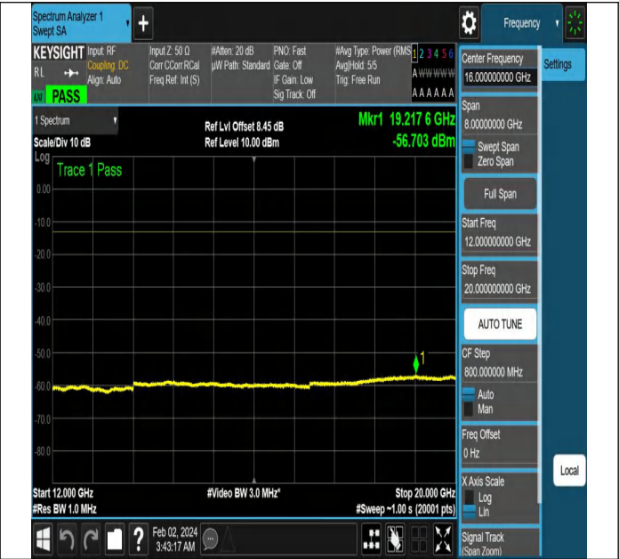
NTNV-N5-PC3-15-15-H-CP-QPSK-Edge_1RB_Left-Ant1-PAS
