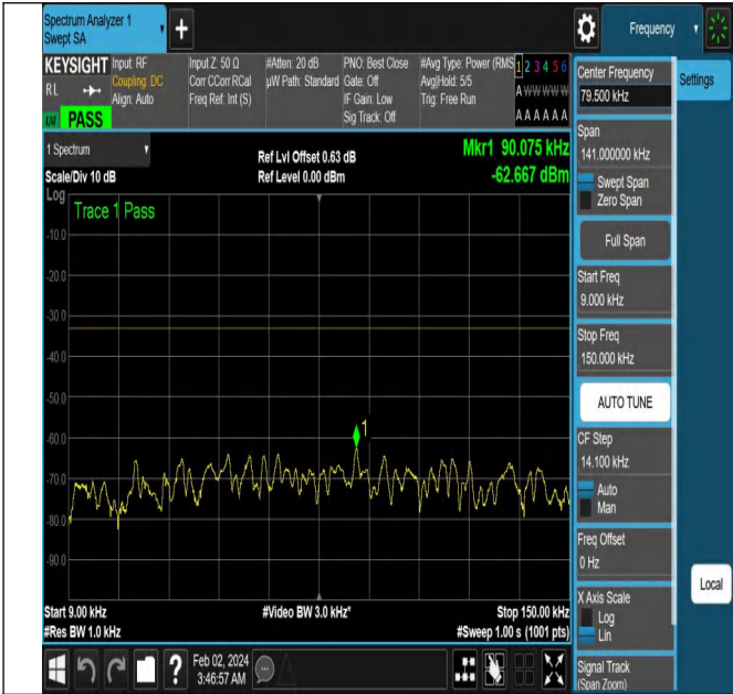
NTNV-N5-PC3-15-20-L-DFT-QPSK-Edge_1RB_Left-Ant1-PAS
