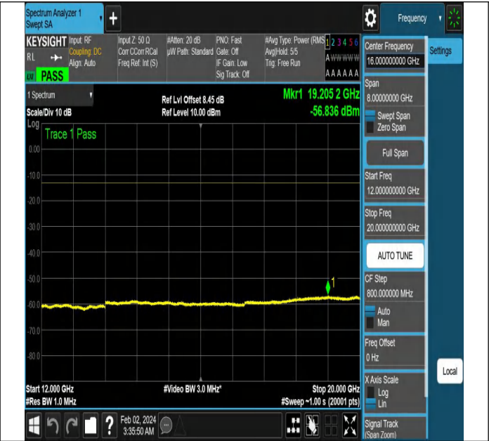
NTNV-N5-PC3-15-15-M-CP-QPSK-Edge_1RB_Left-Ant1-PAS
