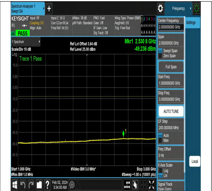
NTNV-N5-PC3-15-15-M-DFT-QPSK-Edge_1RB_Right-Ant1-P
