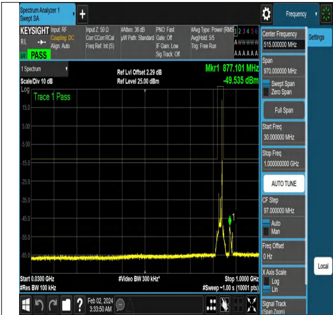
NTNV-N5-PC3-15-15-M-DFT-QPSK-Edge_1RB_Right-Ant1-P
