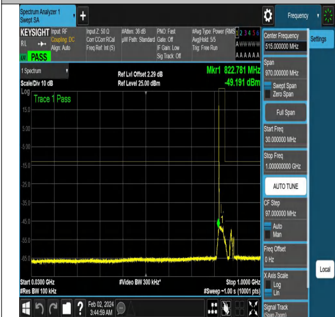
NTNV-N5-PC3-15-20-L-DFT-PI2BPSK-Edge_1RB_Left-Ant1- PASS
