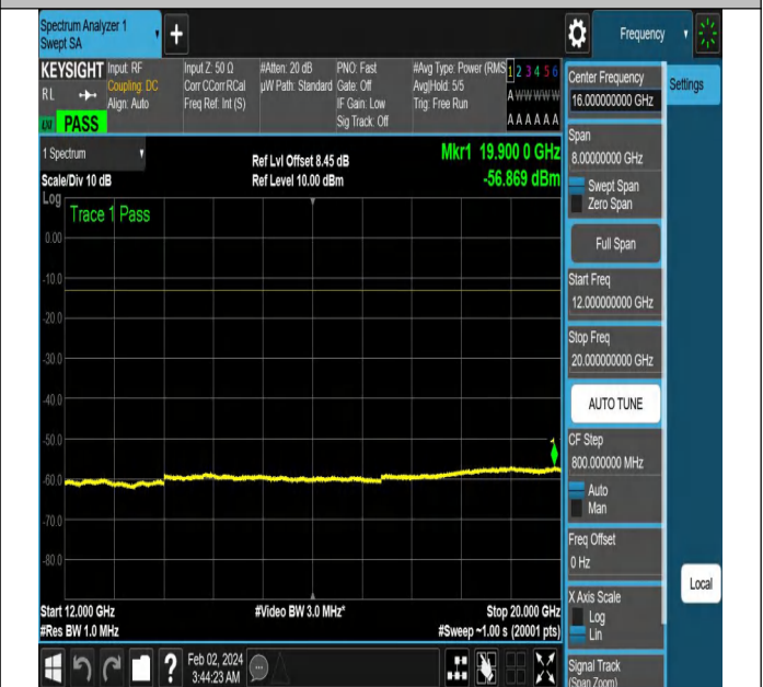
NTNV-N5-PC3-15-15-H-CP-QPSK-Edge_1RB_Right-Ant1-PA
