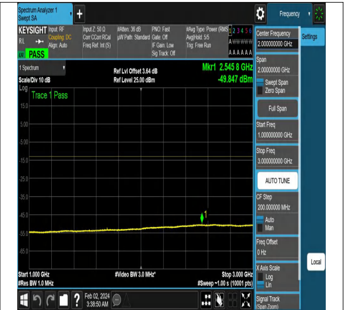
NTNV-N5-PC3-15-15-H-DFT-PI2BPSK-Edge_1RB_Right-Ant1 -PASS
