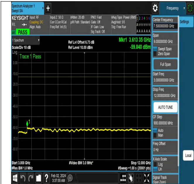
NTNV-N5-PC3-15-15-H-DFT-PI2BPSK-Edge_1RB_Left-Ant1-
