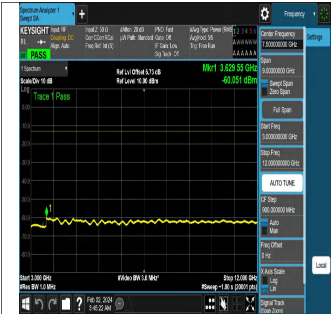
NTNV-N5-PC3-15-20-L-DFT-PI2BPSK-Edge_1RB_Left-Ant1-
