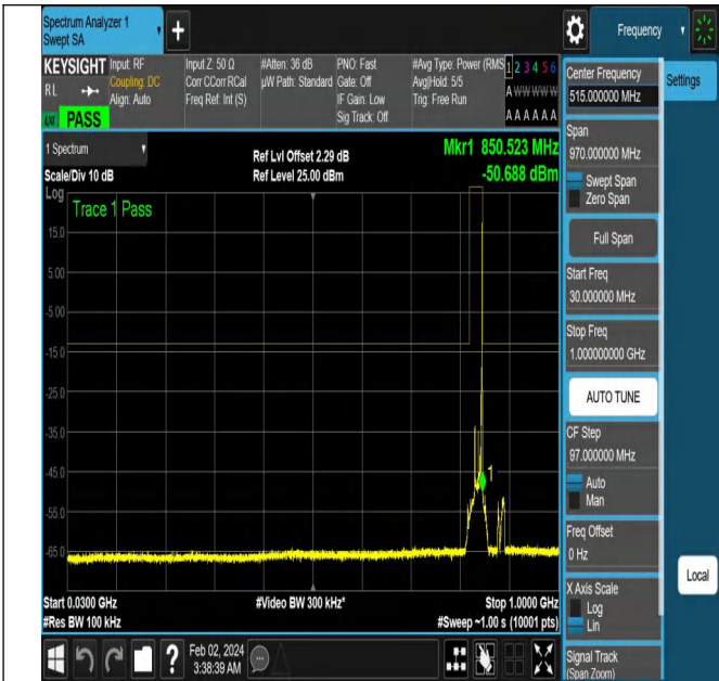
NTNV-N5-PC3-15-15-H-DFT-PI2BPSK-Edge_1RB_Right-Ant1 -PASS
