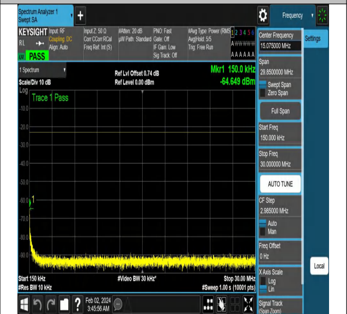
NTNV-N5-PC3-15-20-L-DFT-PI2BPSK-Edge_1RB_Right-Ant1
