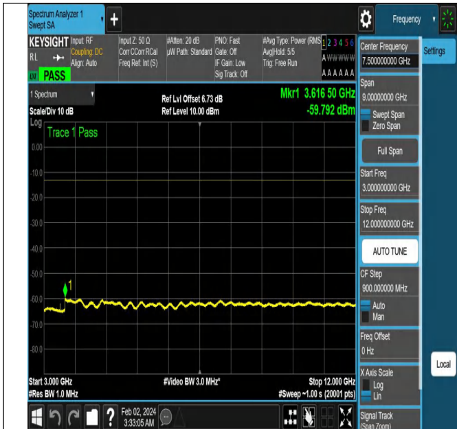
NTNV-N5-PC3-15-15-M-DFT-QPSK-Edge_1RB_Left-Ant1-PA
