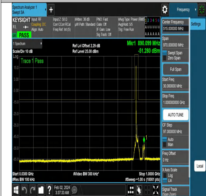
NTNV-N5-PC3-15-15-H-DFT-PI2BPSK-Edge_1RB_Left-Ant1- PASS
