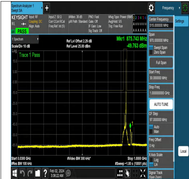
NTNV-N5-PC3-15-15-M-CP-QPSK-Edge_1RB_Right-Ant1-PA
