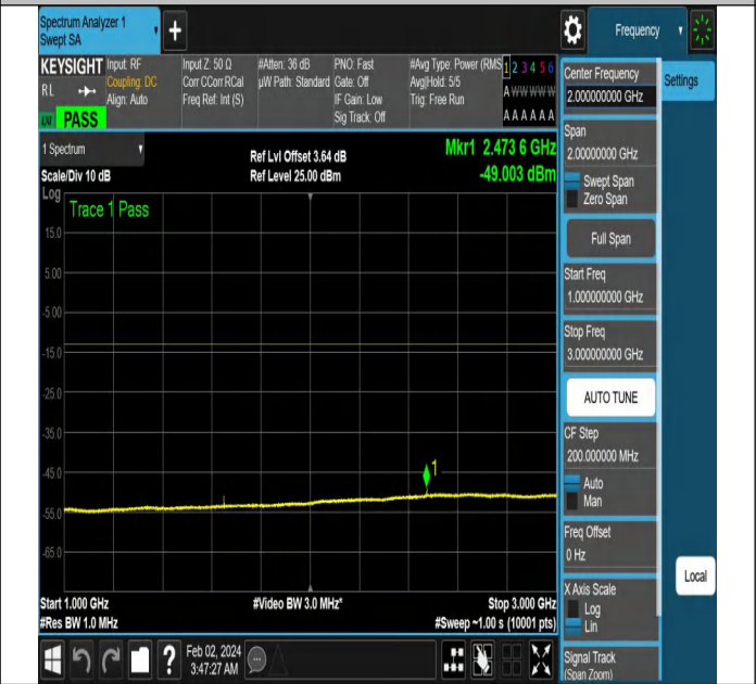
NTNV-N5-PC3-15-20-L-DFT-QPSK-Edge_1RB_Left-Ant1-PAS
