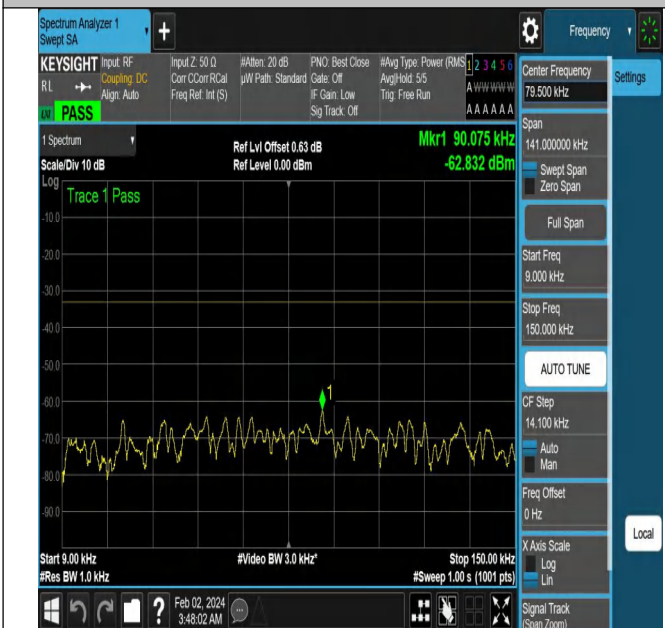
NTNV-N5-PC3-15-20-L-DFT-QPSK-Edge_1RB_Right-Ant1-PA
