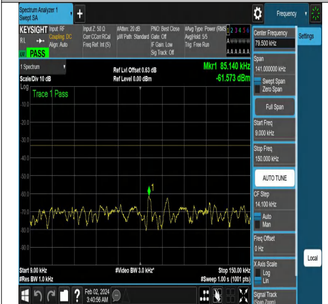
NTNV-N5-PC3-15-15-H-DFT-QPSK-Edge_1RB_Right-Ant1-P
