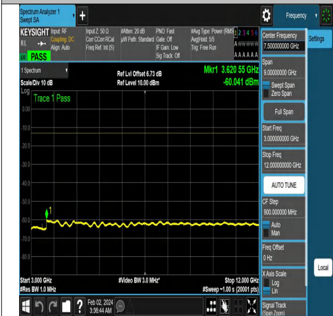
NTNV-N5-PC3-15-15-M-CP-QPSK-Edge_1RB_Right-Ant1-PA
