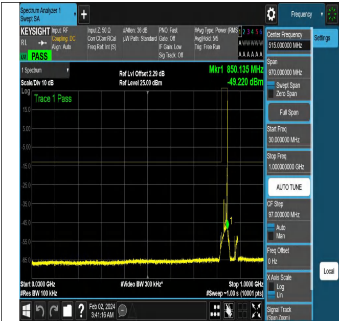
NTNV-N5-PC3-15-15-H-DFT-QPSK-Edge_1RB_Right-Ant1-P
