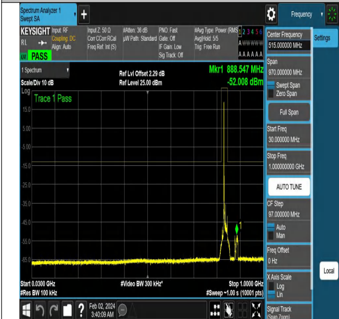
NTNV-N5-PC3-15-15-H-DFT-QPSK-Edge_1RB_Left-Ant1-PA
