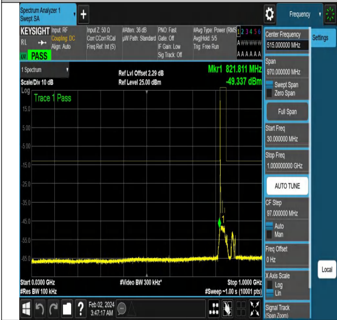
NTNV-N5-PC3-15-20-L-DFT-QPSK-Edge_1RB_Left-Ant1-PAS
