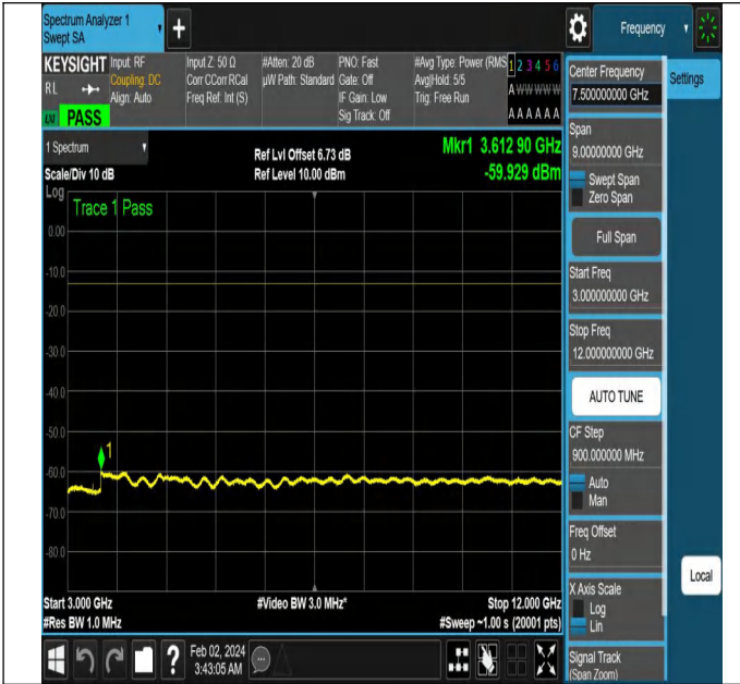
NTNV-N5-PC3-15-15-H-CP-QPSK-Edge_1RB_Left-Ant1-PAS
