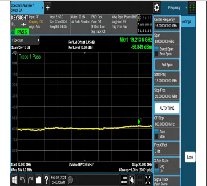
NTNV-N5-PC3-15-15-H-DFT-QPSK-Edge_1RB_Left-Ant1-PA
