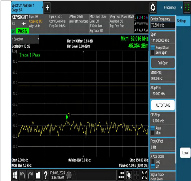
NTNV-N5-PC3-15-15-H-DFT-QPSK-Edge_1RB_Left-Ant1-PA
