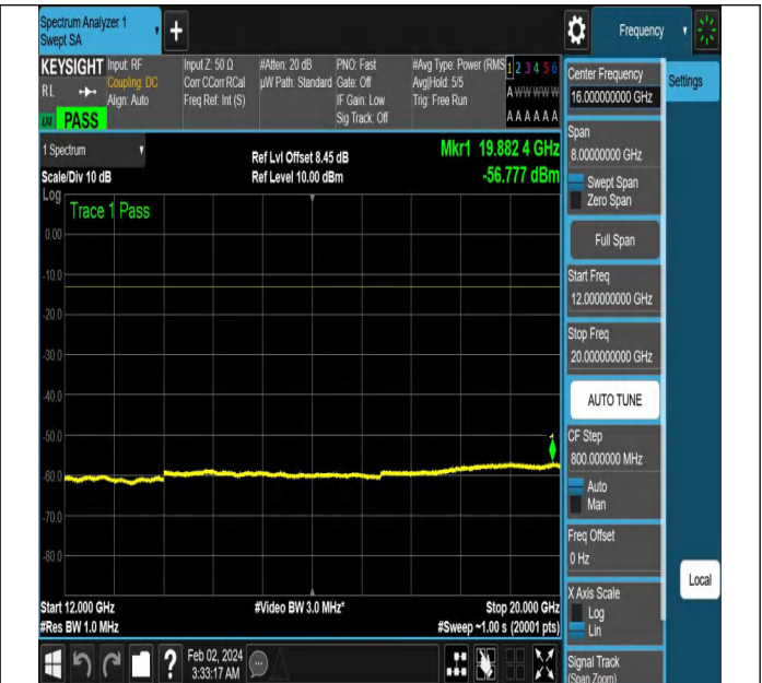
NTNV-N5-PC3-15-15-M-DFT-QPSK-Edge_1RB_Left-Ant1-PA
