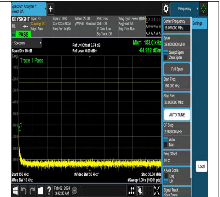
NTNV-N5-PC3-15-15-H-CP-QPSK-Edge_1RB_Left-Ant1-PAS
