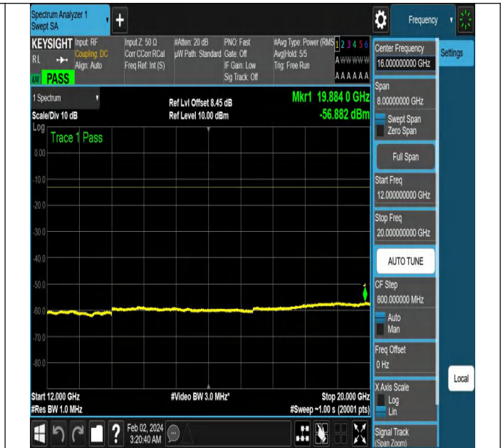
NTNV-N5-PC3-15-10-H-CP-QPSK-Edge_1RB_Left-Ant1-PAS
