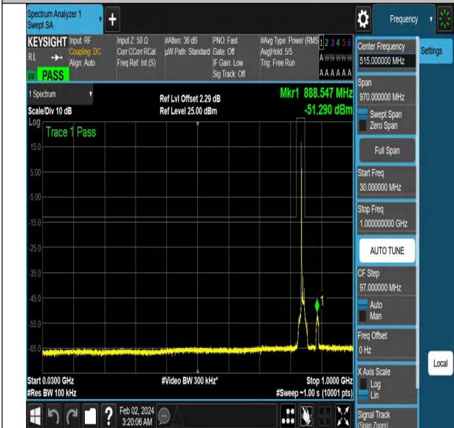
NTNV-N5-PC3-15-10-H-CP-QPSK-Edge_1RB_Left-Ant1-PAS
