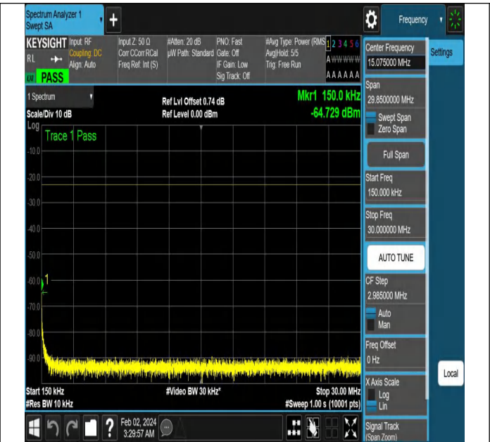
NTNV-N5-PC3-15-15-M-DFT-PI2BPSK-Edge_1RB_Left-Ant1-
