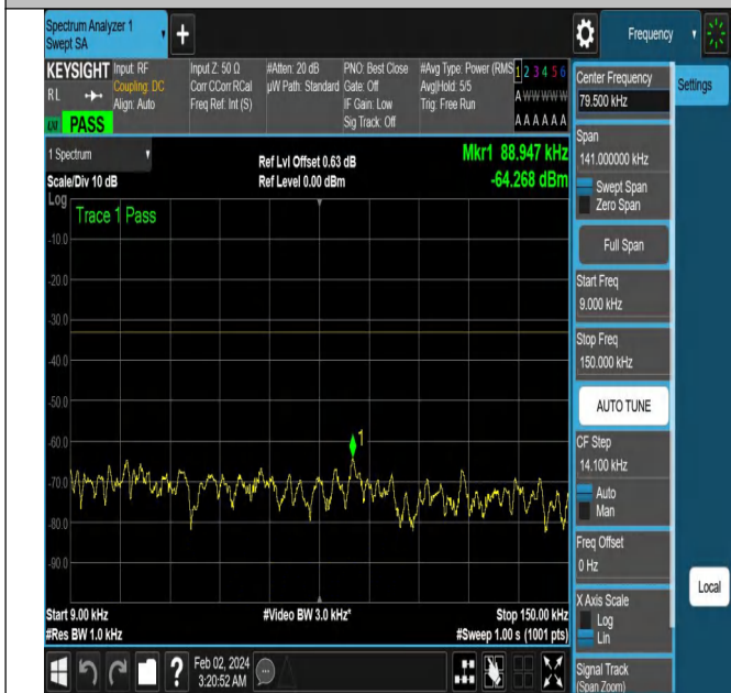
NTNV-N5-PC3-15-10-H-CP-QPSK-Edge_1RB_Right-Ant1-PA
