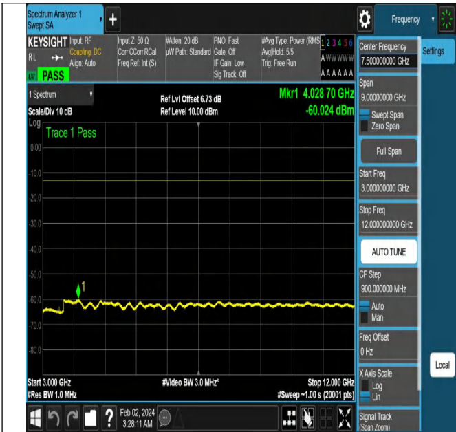
NTNV-N5-PC3-15-15-L-CP-QPSK-Edge_1RB_Left-Ant1-PAS
