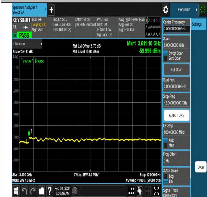
NTNV-N5-PC3-15-15-L-DFT-QPSK-Edge_1RB_Right-Ant1-PA
