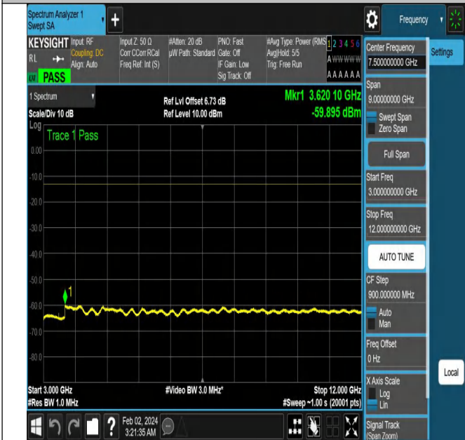
NTNV-N5-PC3-15-10-H-CP-QPSK-Edge_1RB_Right-Ant1-PA
