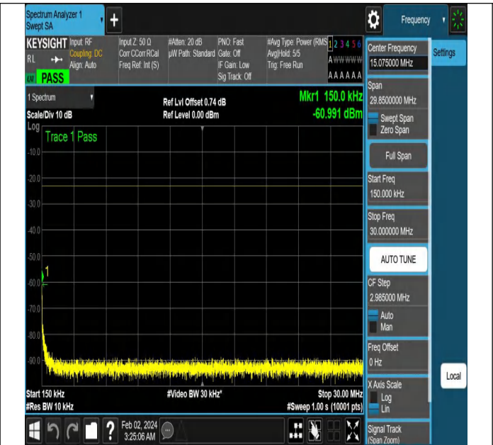
NTNV-N5-PC3-15-15-L-DFT-QPSK-Edge_1RB_Left-Ant1-PAS
