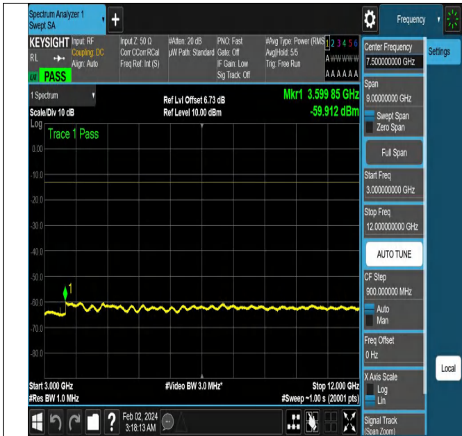
NTNV-N5-PC3-15-10-H-DFT-QPSK-Edge_1RB_Left-Ant1-PA
