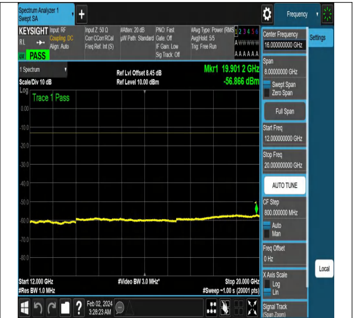
NTNV-N5-PC3-15-15-L-CP-QPSK-Edge_1RB_Left-Ant1-PAS
