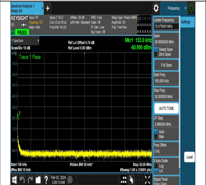
NTNV-N5-PC3-15-15-L-DFT-QPSK-Edge_1RB_Right-Ant1-PA
