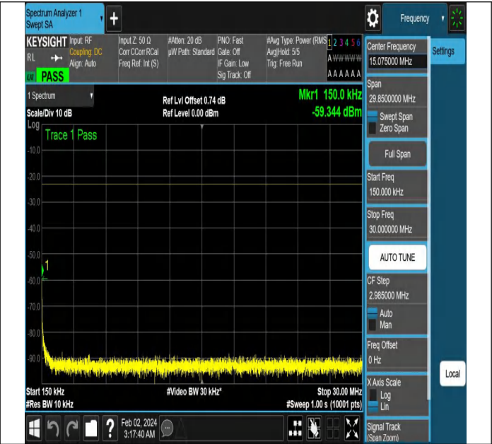
NTNV-N5-PC3-15-10-H-DFT-QPSK-Edge_1RB_Left-Ant1-PA
