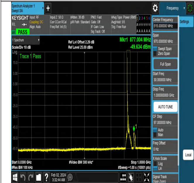
NTNV-N5-PC3-15-15-M-DFT-QPSK-Edge_1RB_Left-Ant1-PA
