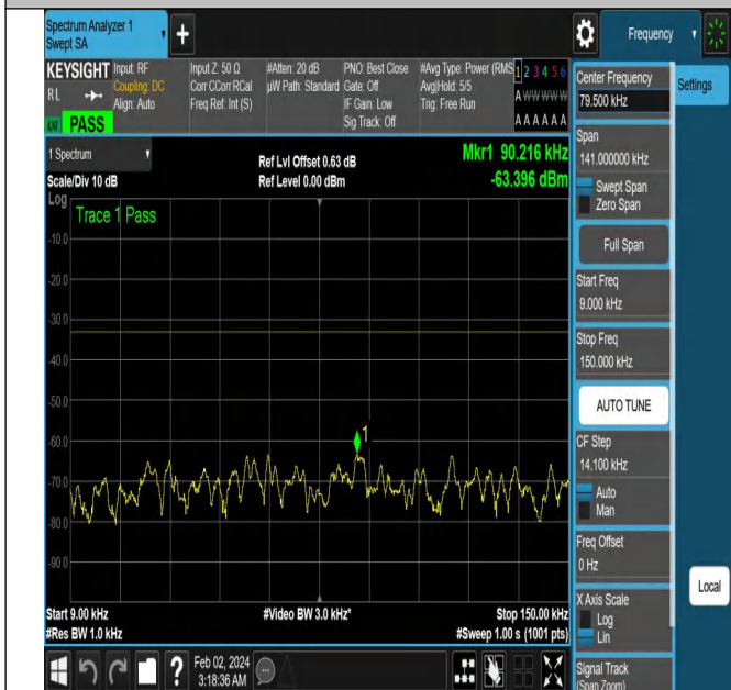
NTNV-N5-PC3-15-10-H-DFT-QPSK-Edge_1RB_Right-Ant1-P
