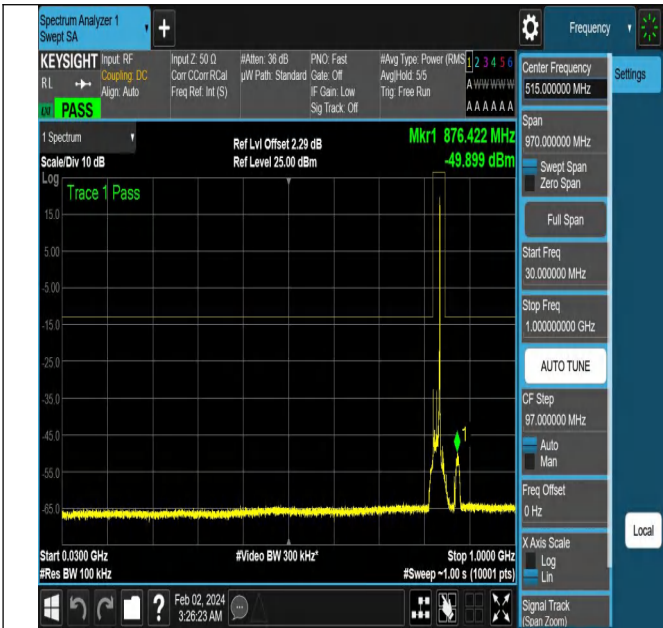
NTNV-N5-PC3-15-15-L-DFT-QPSK-Edge_1RB_Right-Ant1-PA
