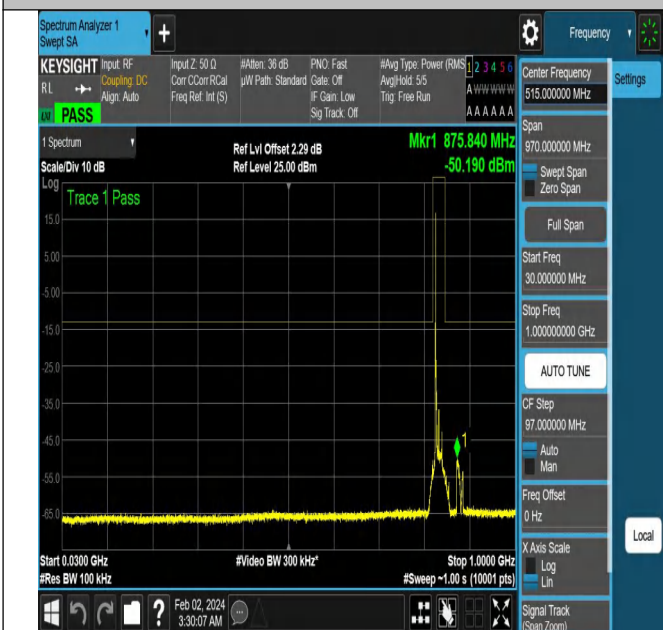
NTNV-N5-PC3-15-15-M-DFT-PI2BPSK-Edge_1RB_Left-Ant1-
