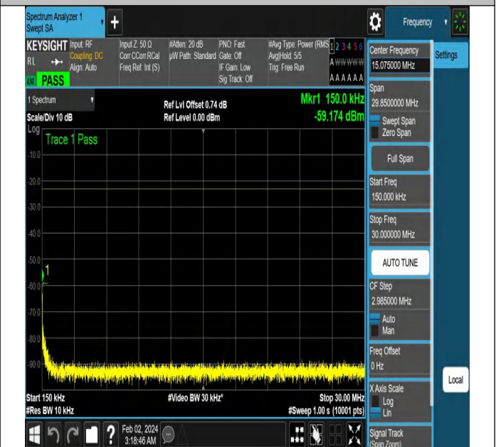
NTNV-N5-PC3-15-10-H-DFT-QPSK-Edge_1RB_Right-Ant1-P
