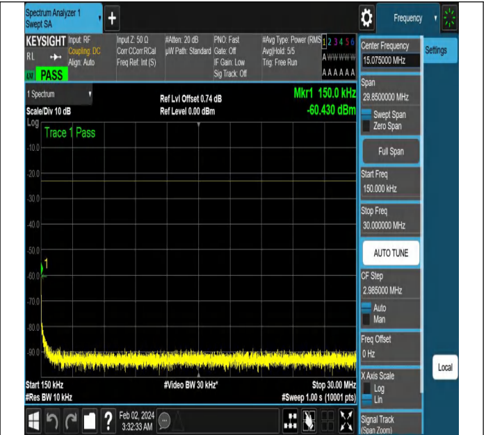
NTNV-N5-PC3-15-15-M-DFT-QPSK-Edge_1RB_Left-Ant1-PA
