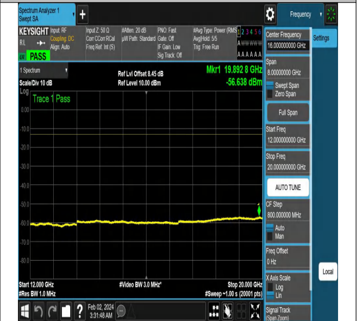
NTNV-N5-PC3-15-15-M-DFT-PI2BPSK-Edge_1RB_Right-Ant 1-PASS
