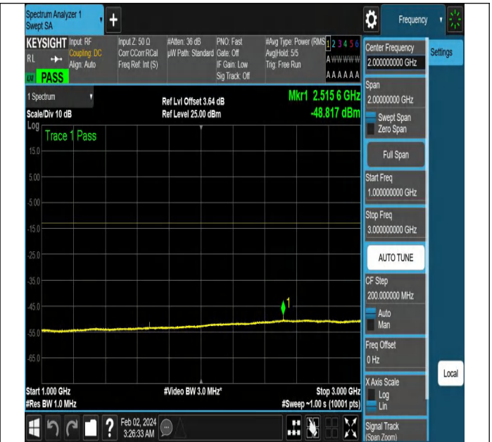
NTNV-N5-PC3-15-15-L-DFT-QPSK-Edge_1RB_Right-Ant1-PA
