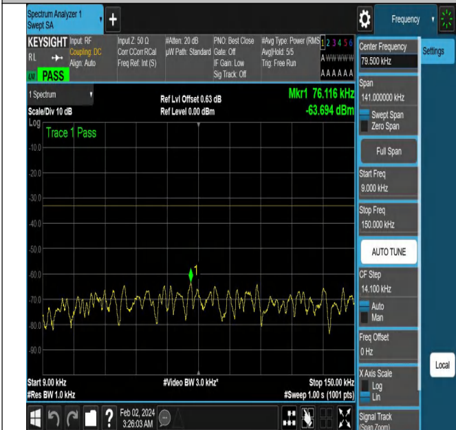
NTNV-N5-PC3-15-15-L-DFT-QPSK-Edge_1RB_Right-Ant1-PA
