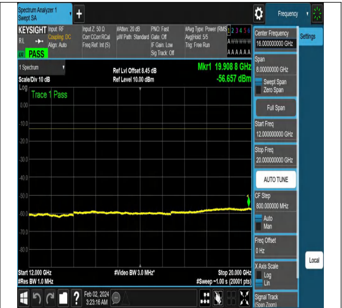
NTNV-N5-PC3-15-15-L-DFT-PI2BPSK-Edge_1RB_Left-Ant1- PASS
