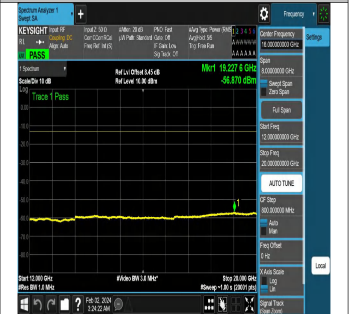
NTNV-N5-PC3-15-15-L-DFT-PI2BPSK-Edge_1RB_Right-Ant1 -PASS
