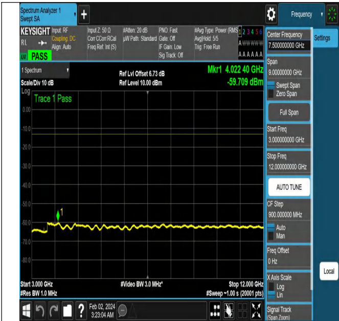
NTNV-N5-PC3-15-15-L-DFT-PI2BPSK-Edge_1RB_Left-Ant1- PASS
