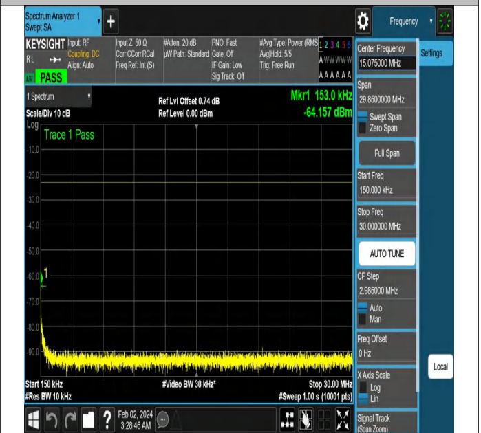
NTNV-N5-PC3-15-15-L-CP-QPSK-Edge_1RB_Right-Ant1-PA
