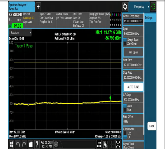
NTNV-N5-PC3-15-10-H-CP-QPSK-Edge_1RB_Right-Ant1-PA
