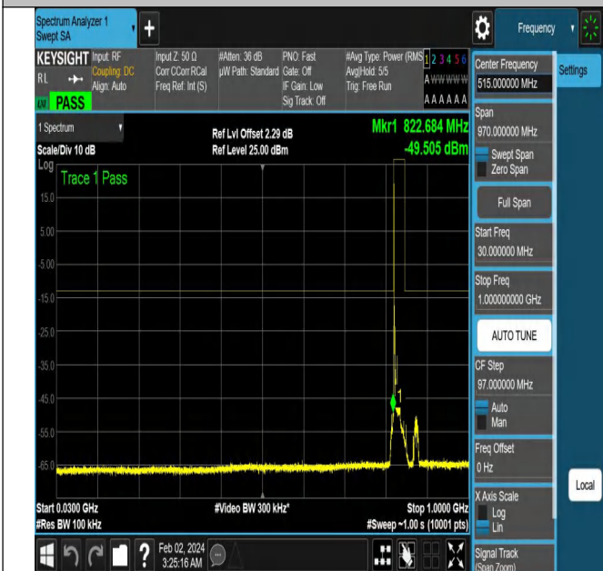
NTNV-N5-PC3-15-15-L-DFT-QPSK-Edge_1RB_Left-Ant1-PAS
