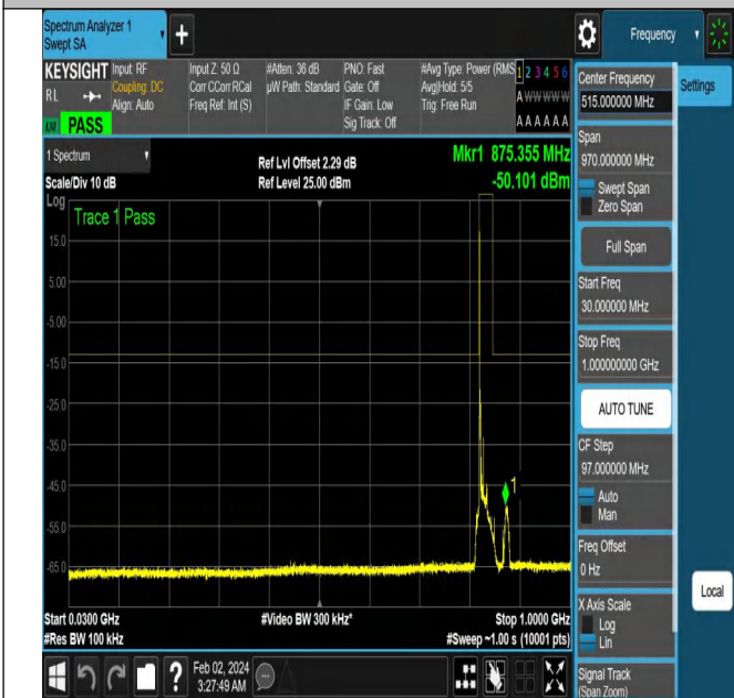
NTNV-N5-PC3-15-15-L-CP-QPSK-Edge_1RB_Left-Ant1-PAS
