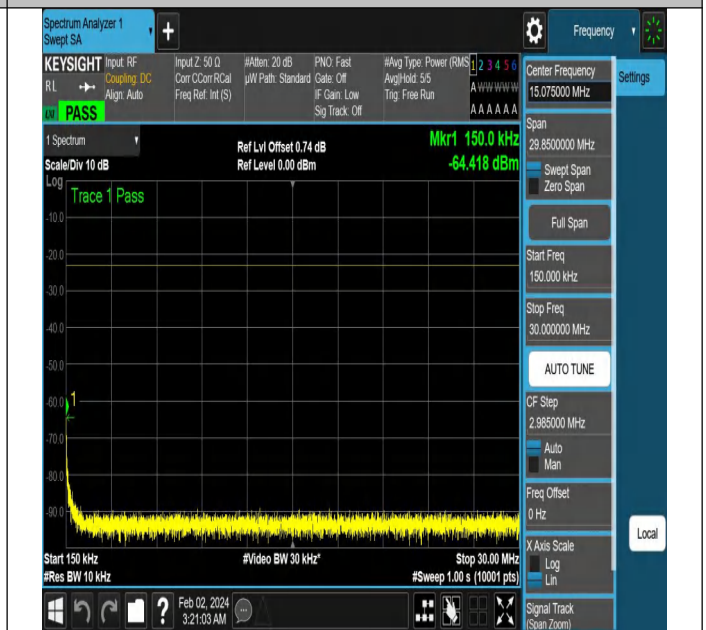
NTNV-N5-PC3-15-10-H-CP-QPSK-Edge_1RB_Right-Ant1-PA
