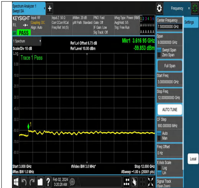
NTNV-N5-PC3-15-10-H-CP-QPSK-Edge_1RB_Left-Ant1-PAS
