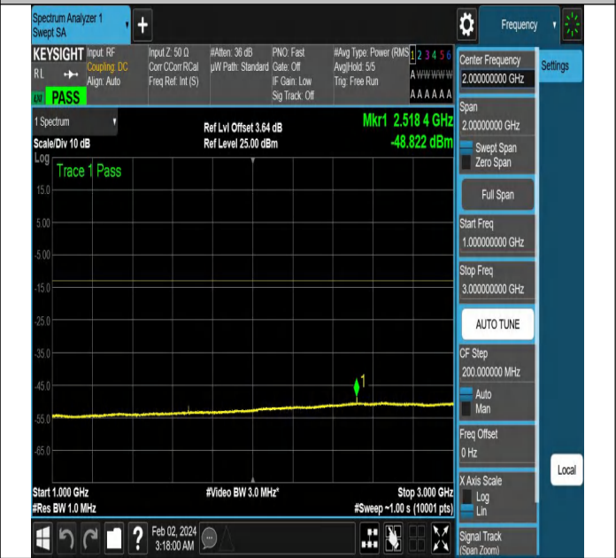
NTNV-N5-PC3-15-10-H-DFT-QPSK-Edge_1RB_Left-Ant1-PA
