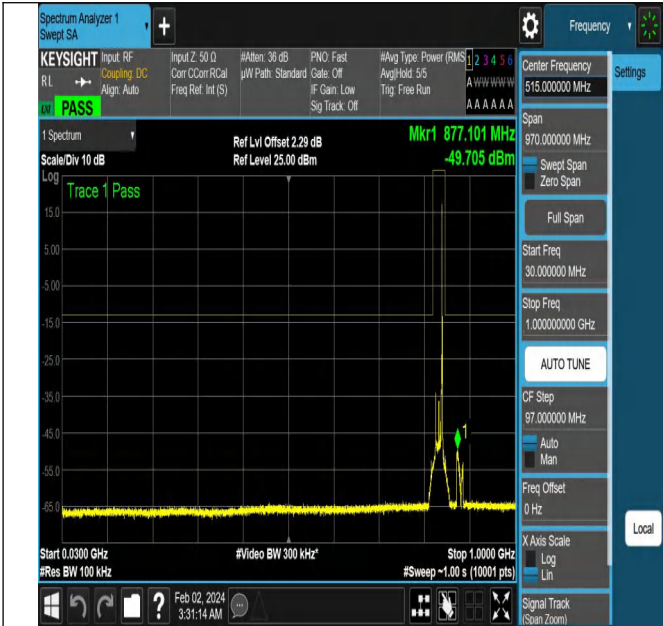
NTNV-N5-PC3-15-15-M-DFT-PI2BPSK-Edge_1RB_Right-Ant 1-PASS
