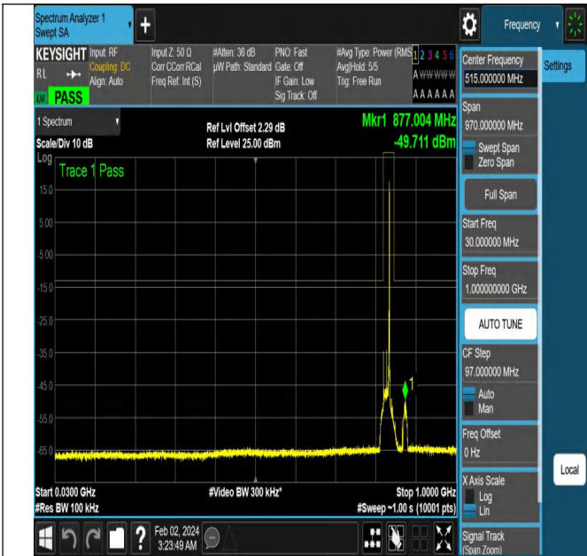
NTNV-N5-PC3-15-15-L-DFT-PI2BPSK-Edge_1RB_Right-Ant1 -PASS
