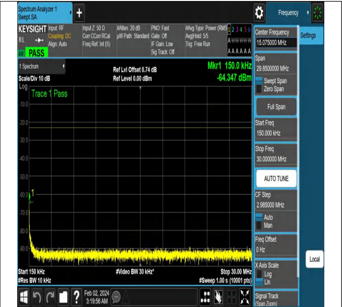
NTNV-N5-PC3-15-10-H-CP-QPSK-Edge_1RB_Left-Ant1-PAS
