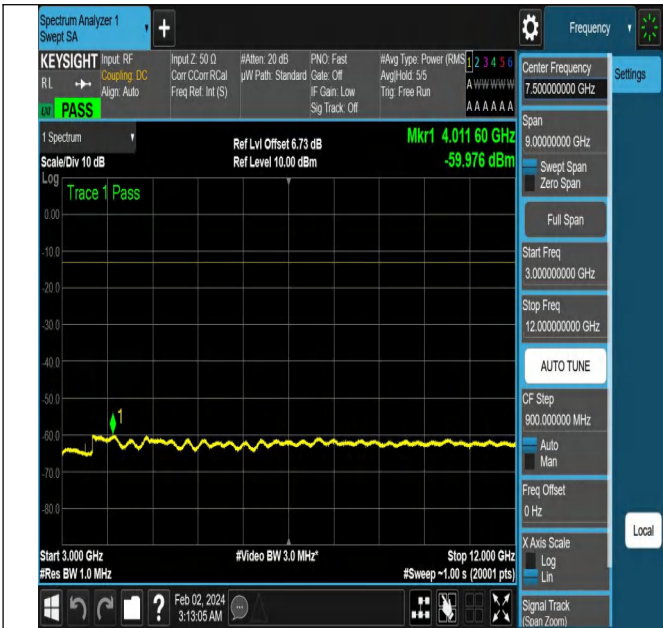
NTNV-N5-PC3-15-10-M-CP-QPSK-Edge_1RB_Left-Ant1-PAS
