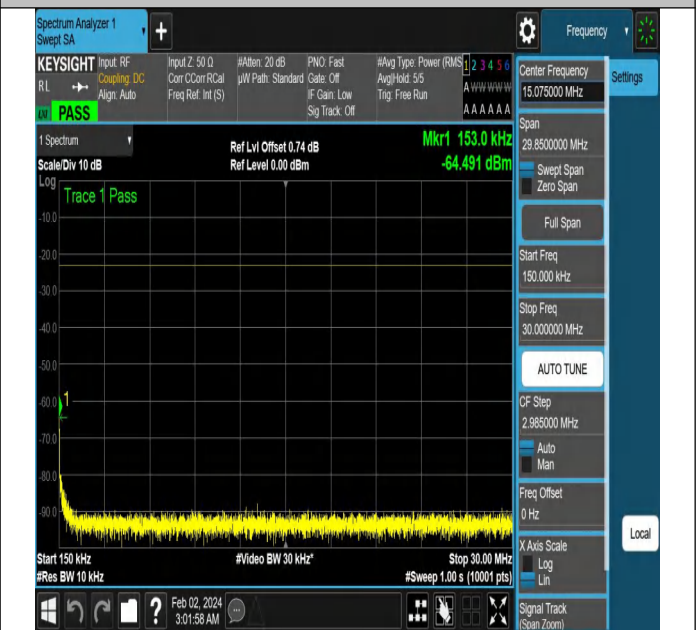
NTNV-N5-PC3-15-10-L-DFT-PI2BPSK-Edge_1RB_Right-Ant1 -PASS
