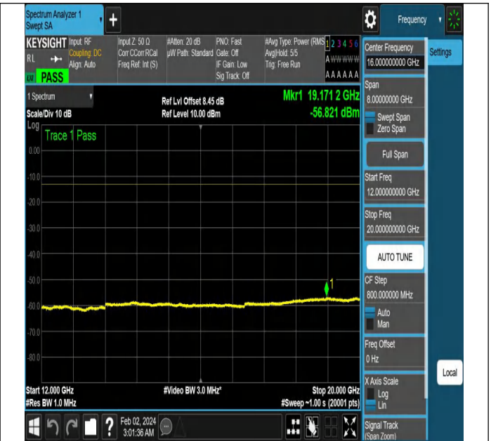
NTNV-N5-PC3-15-10-L-DFT-PI2BPSK-Edge_1RB_Left-Ant1- PASS
