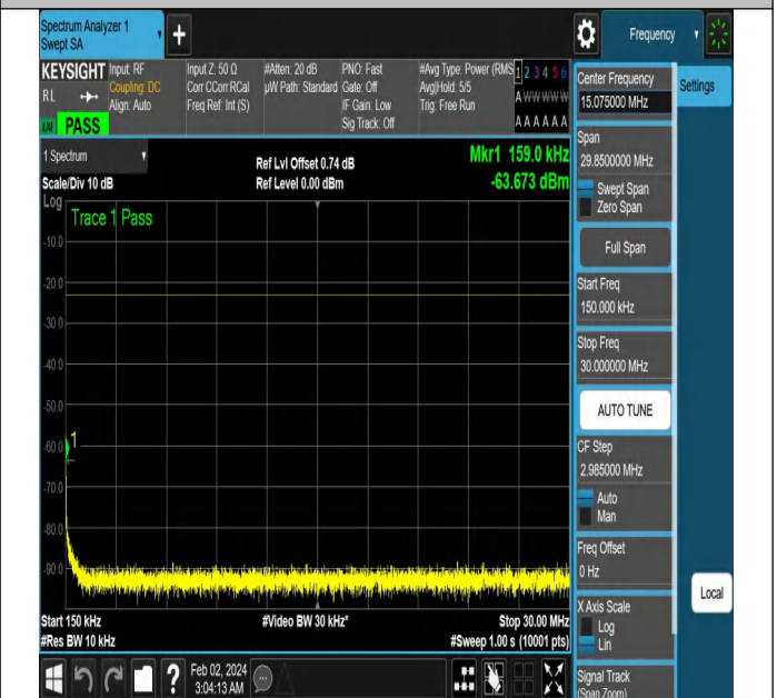
NTNV-N5-PC3-15-10-L-DFT-QPSK-Edge_1RB_Right-Ant1-PA
