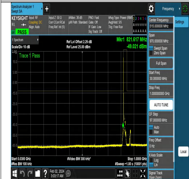
NTNV-N5-PC3-15-10-L-DFT-QPSK-Edge_1RB_Left-Ant1-PAS
