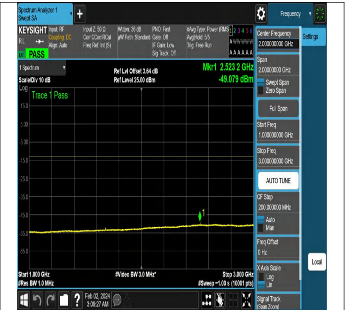
NTNV-N5-PC3-15-10-M-DFT-PI2BPSK-Edge_1RB_Right-Ant 1-PASS
