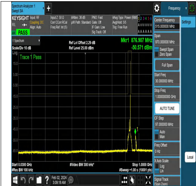
NTNV-N5-PC3-15-10-M-DFT-PI2BPSK-Edge_1RB_Right-Ant 1-PASS
