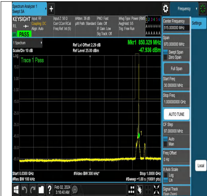
NTNV-N5-PC3-15-10-H-DFT-PI2BPSK-Edge_1RB_Right-Ant1
