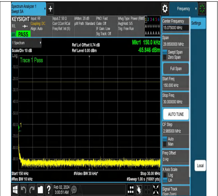
NTNV-N5-PC3-15-10-L-DFT-PI2BPSK-Edge_1RB_Left-Ant1-
