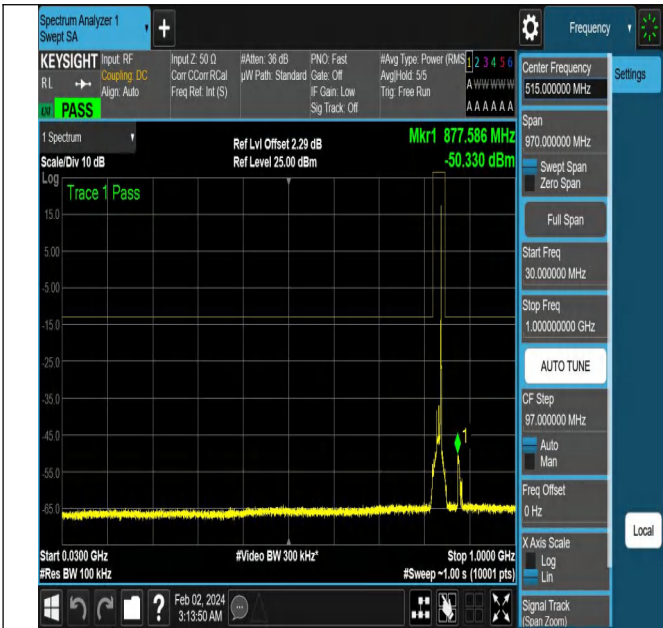
NTNV-N5-PC3-15-10-M-CP-QPSK-Edge_1RB_Right-Ant1-PA
