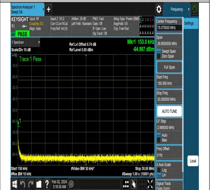
NTNV-N5-PC3-15-10-H-DFT-PI2BPSK-Edge_1RB_Right-Ant1 -PASS
