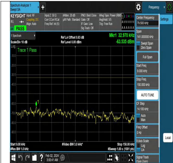
NTNV-N5-PC3-15-10-L-DFT-PI2BPSK-Edge_1RB_Left-Ant1-
