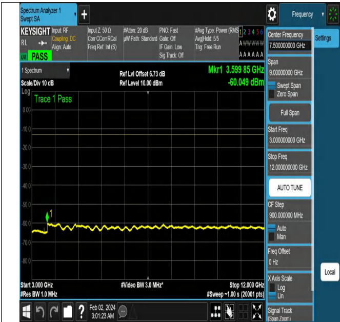
NTNV-N5-PC3-15-10-L-DFT-PI2BPSK-Edge_1RB_Left-Ant1- PASS
