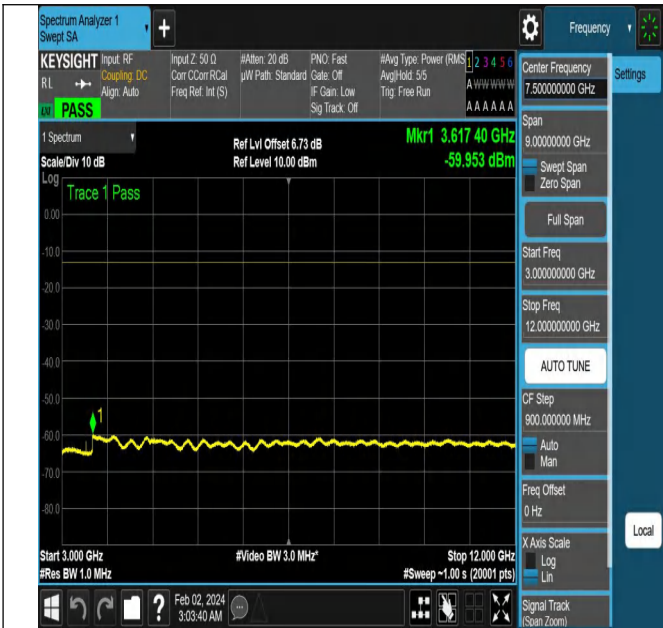
NTNV-N5-PC3-15-10-L-DFT-QPSK-Edge_1RB_Left-Ant1-PAS
