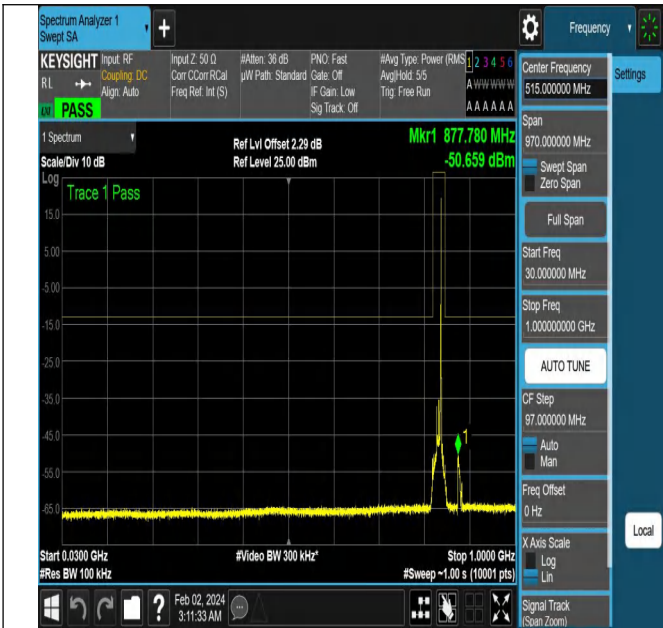
NTNV-N5-PC3-15-10-M-DFT-QPSK-Edge_1RB_Right-Ant1-P ASS
