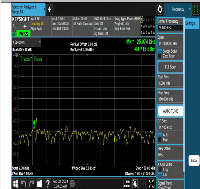
NTNV-N5-PC3-15-10-L-DFT-QPSK-Edge_1RB_Right-Ant1-PA
