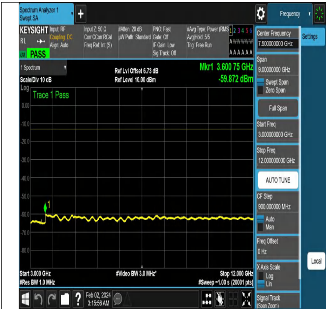
NTNV-N5-PC3-15-10-H-DFT-PI2BPSK-Edge_1RB_Left-Ant1- PASS
