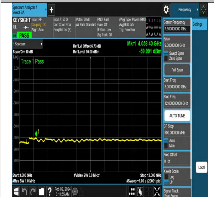
NTNV-N5-PC3-15-10-M-DFT-QPSK-Edge_1RB_Right-Ant1-P ASS
