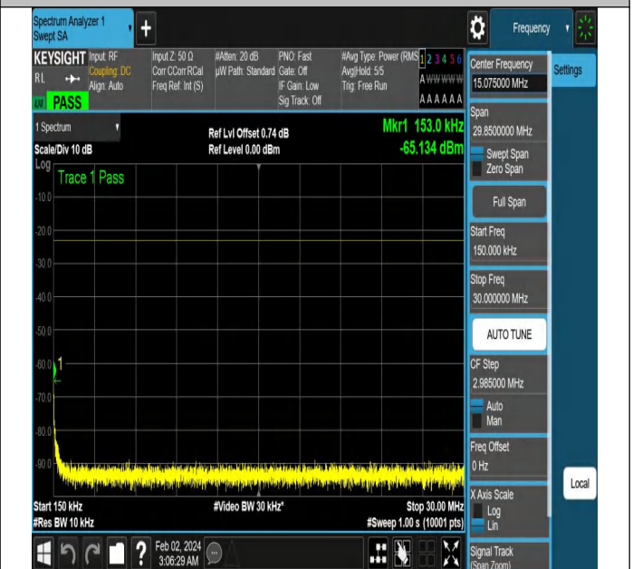
NTNV-N5-PC3-15-10-L-CP-QPSK-Edge_1RB_Right-Ant1-PA
