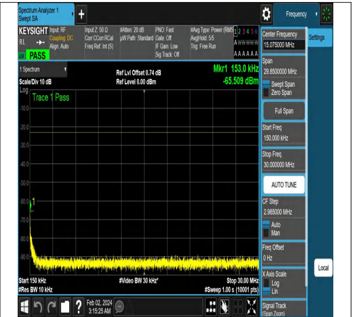
NTNV-N5-PC3-15-10-H-DFT-PI2BPSK-Edge_1RB_Left-Ant1- PASS
