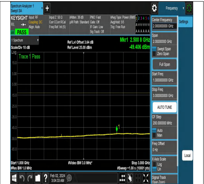
NTNV-N5-PC3-15-10-L-DFT-QPSK-Edge_1RB_Right-Ant1-PA
