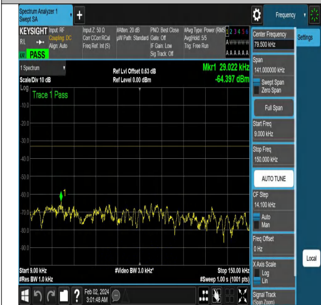
NTNV-N5-PC3-15-10-L-DFT-PI2BPSK-Edge_1RB_Right-Ant1 -PASS
