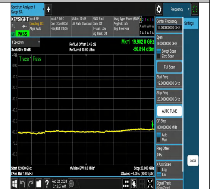
NTNV-N5-PC3-15-10-M-DFT-QPSK-Edge_1RB_Right-Ant1-P ASS
