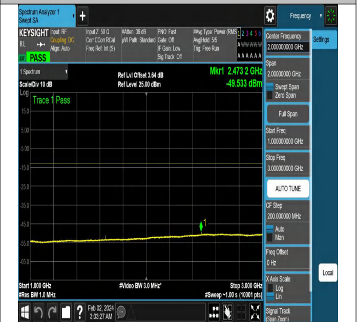
NTNV-N5-PC3-15-10-L-DFT-QPSK-Edge_1RB_Left-Ant1-PAS
