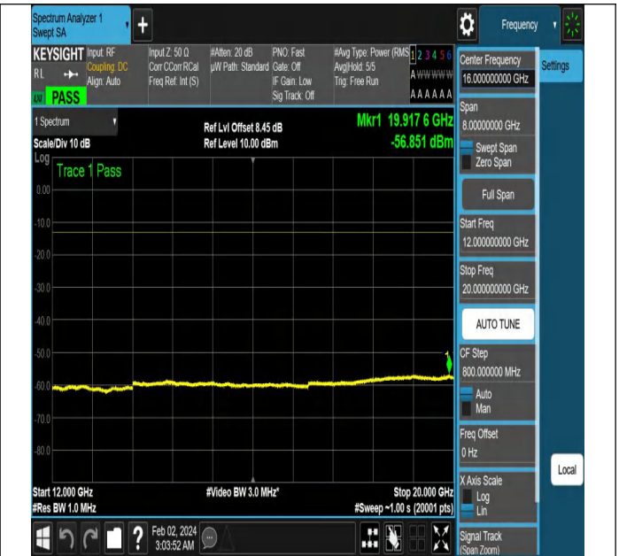
NTNV-N5-PC3-15-10-L-DFT-QPSK-Edge_1RB_Left-Ant1-PAS
