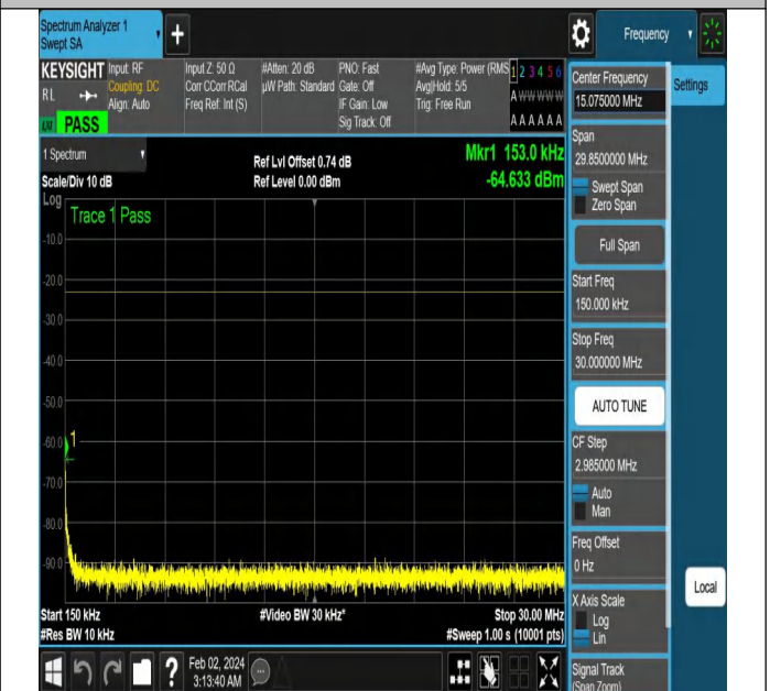
NTNV-N5-PC3-15-10-M-CP-QPSK-Edge_1RB_Right-Ant1-PA
