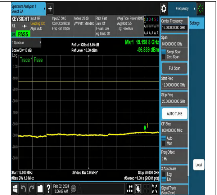
NTNV-N5-PC3-15-10-L-CP-QPSK-Edge_1RB_Left-Ant1-PAS
