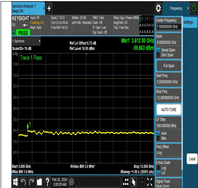
NTNV-N5-PC3-15-10-L-CP-QPSK-Edge_1RB_Left-Ant1-PAS
