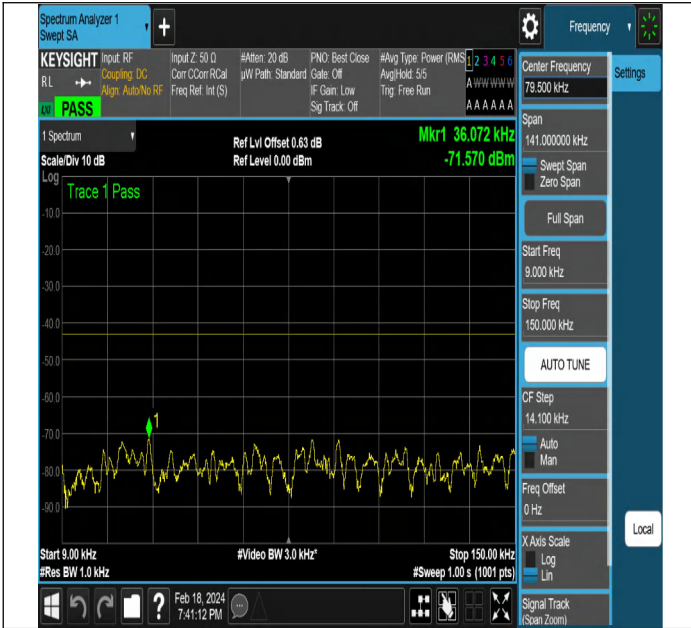
NTNV-DC_5A_n2A-PC3-15-5+20-M+M-QPSK-DFT-QPSK-Edge_1RB_Left-PASS
