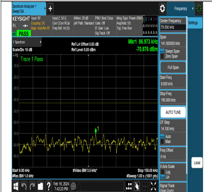
NTNV-DC_5A_n2A-PC3-15-5+20-M+M-QPSK-DFT-QPSK-Ed ge_1RB_Right-PASS
