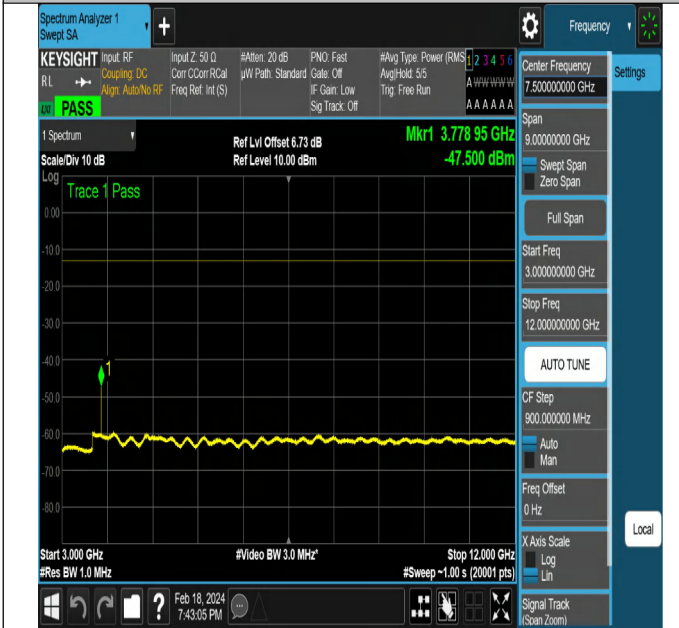
NTNV-DC_5A_n2A-PC3-15-5+20-M+M-QPSK-DFT-QPSK-Ed ge_1RB_Right-PASS
