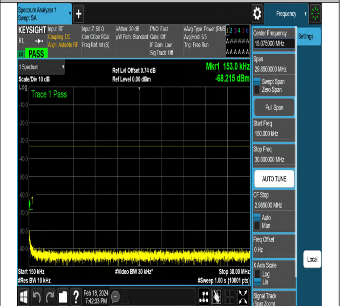
NTNV-DC_5A_n2A-PC3-15-5+20-M+M-QPSK-DFT-QPSK-Ed ge_1RB_Right-PASS
