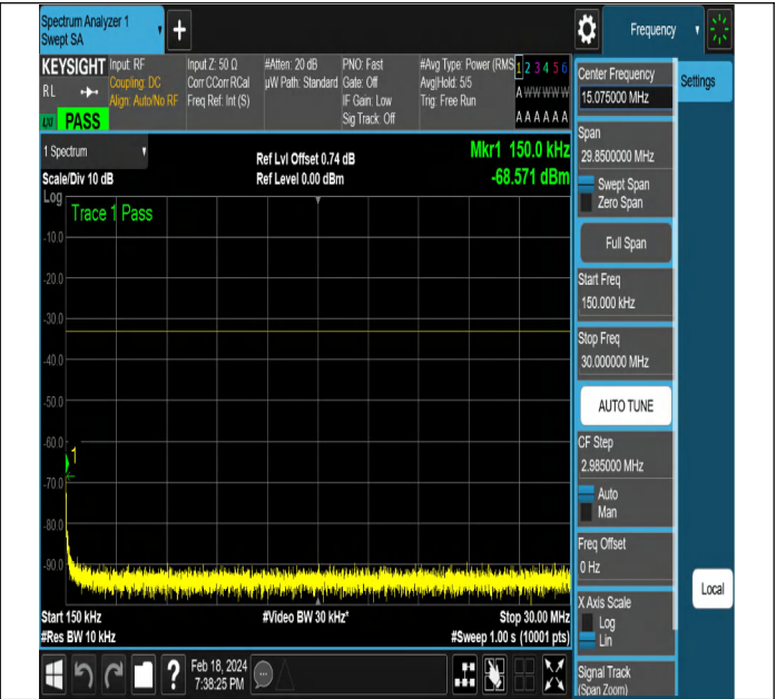
NTNV-DC_5A_n2A-PC3-15-5+20-M+M-QPSK-DFT-PI2BPSK-Edge_1RB_Left-PASS
