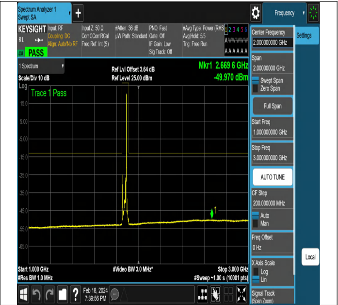
NTNV-DC_5A_n2A-PC3-15-5+20-M+M-QPSK-DFT-PI2BPSK-Edge_1RB_Right-PASS
