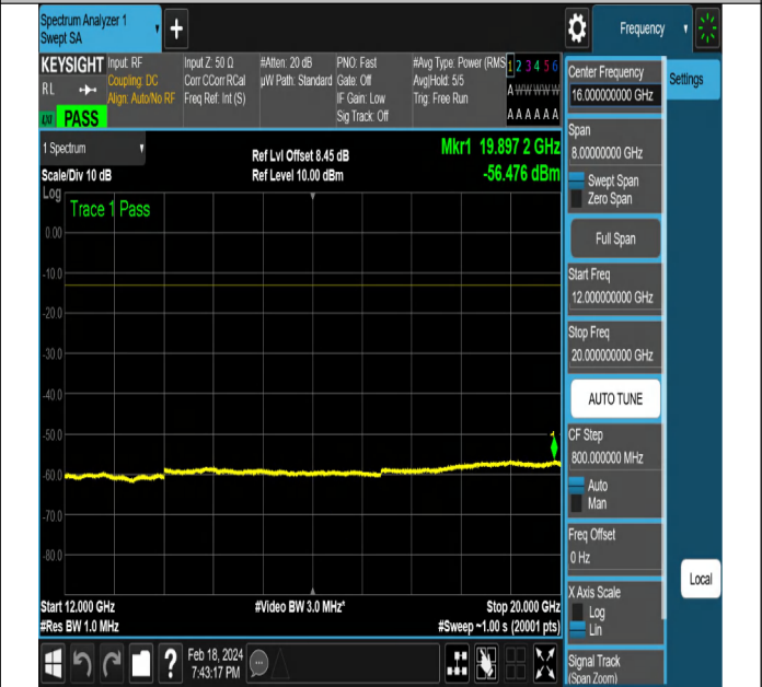
NTNV-DC_5A_n2A-PC3-15-5+20-M+M-QPSK-DFT-QPSK-Ed ge_1RB_Right-PASS
