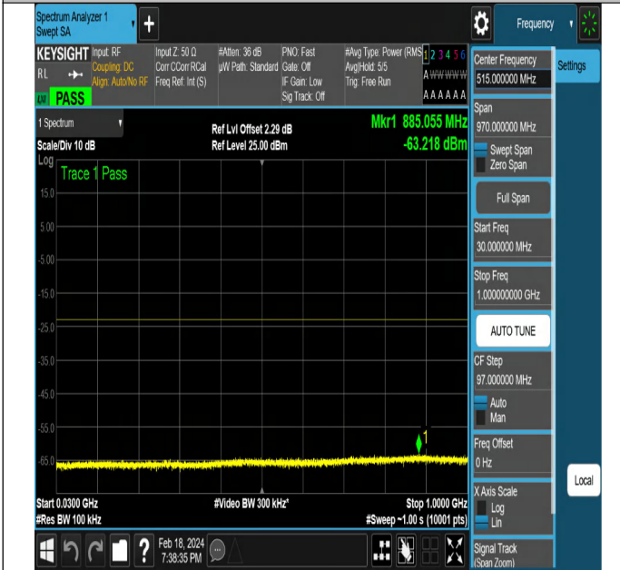
NTNV-DC_5A_n2A-PC3-15-5+20-M+M-QPSK-DFT-PI2BPSK-Edge_1RB_Left-PASS
