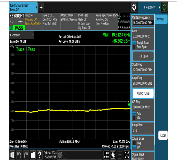
NTNV-DC_5A_n2A-PC3-15-5+20-M+M-QPSK-DFT-QPSK-Ed ge_1RB_Left-PASS
