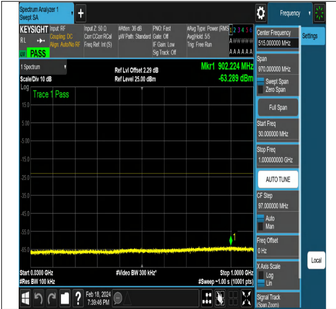
NTNV-DC_5A_n2A-PC3-15-5+20-M+M-QPSK-DFT-PI2BPSK-Edge_1RB_Right-PASS
