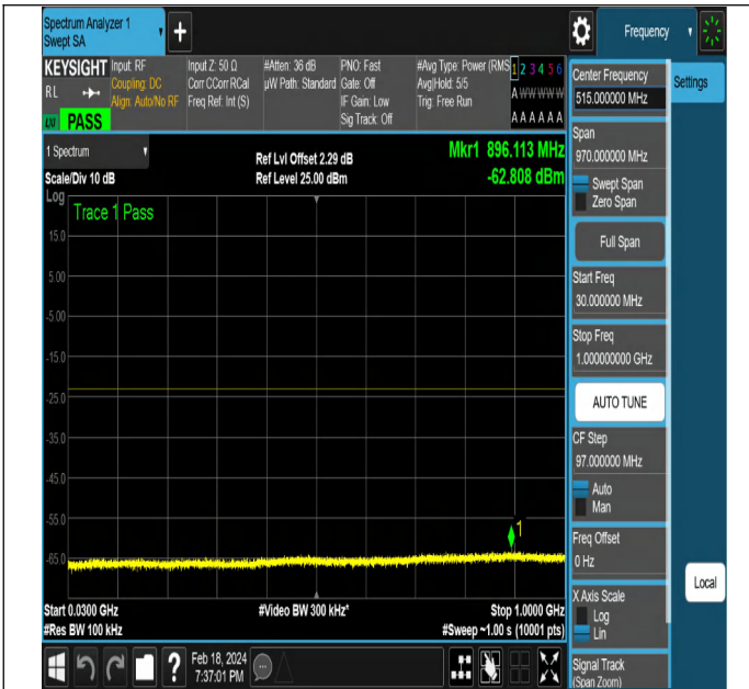
NTNV-DC_5A_n2A-PC3-15-5+20-M+L-QPSK-DFT-QPSK-Edge e_1RB_Right-PASS
