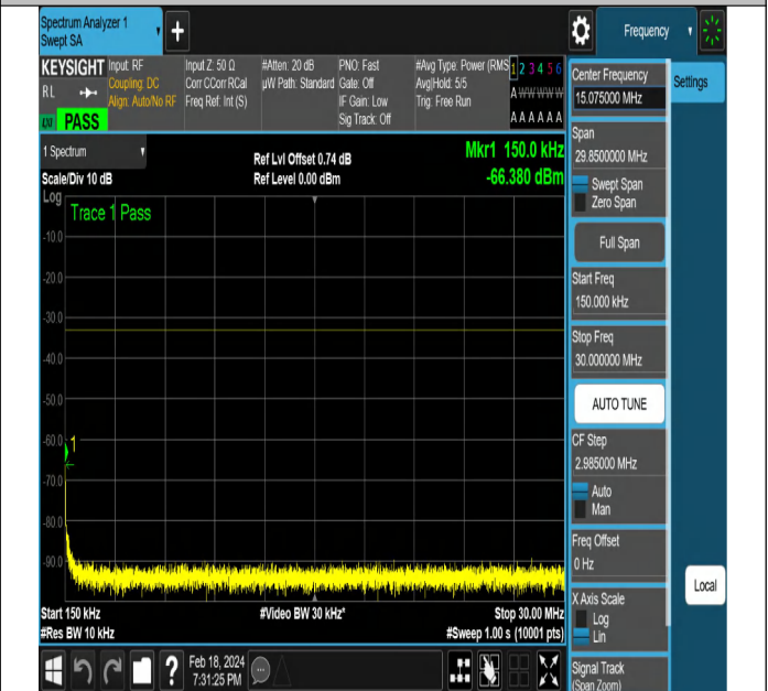
NTNV-DC_5A_n2A-PC3-15-5+15-M+H-QPSK-DFT-QPSK-Ed ge_1RB_Right-PASS
