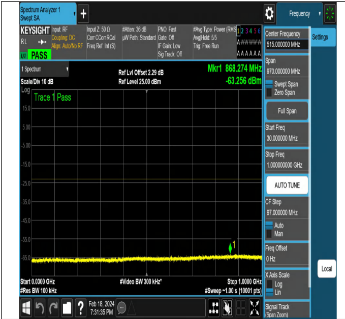
NTNV-DC_5A_n2A-PC3-15-5+15-M+H-QPSK-DFT-QPSK-Ed ge_1RB_Right-PASS
