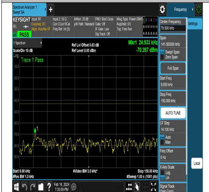
NTNV-DC_5A_n2A-PC3-15-5+20-M+L-QPSK-DFT-PI2BPSK- Edge_1RB_Right-PASS
