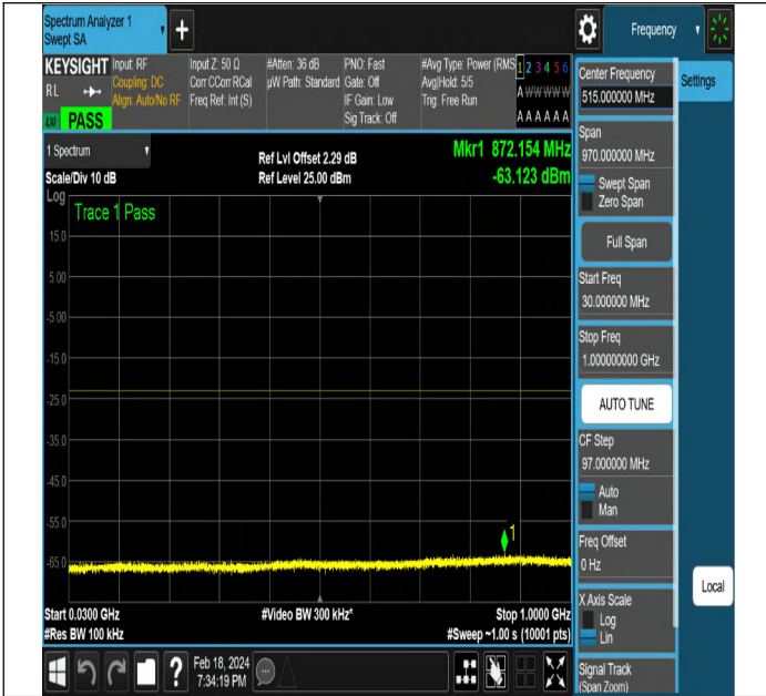
NTNV-DC_5A_n2A-PC3-15-5+20-M+L-QPSK-DFT-PI2BPSK-Edge_1RB_Right-PASS
