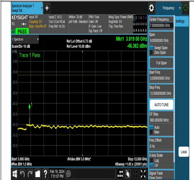
NTNV-DC_5A_n2A-PC3-15-5+15-M+H-QPSK-DFT-QPSK-Ed ge_1RB_Right-PASS
