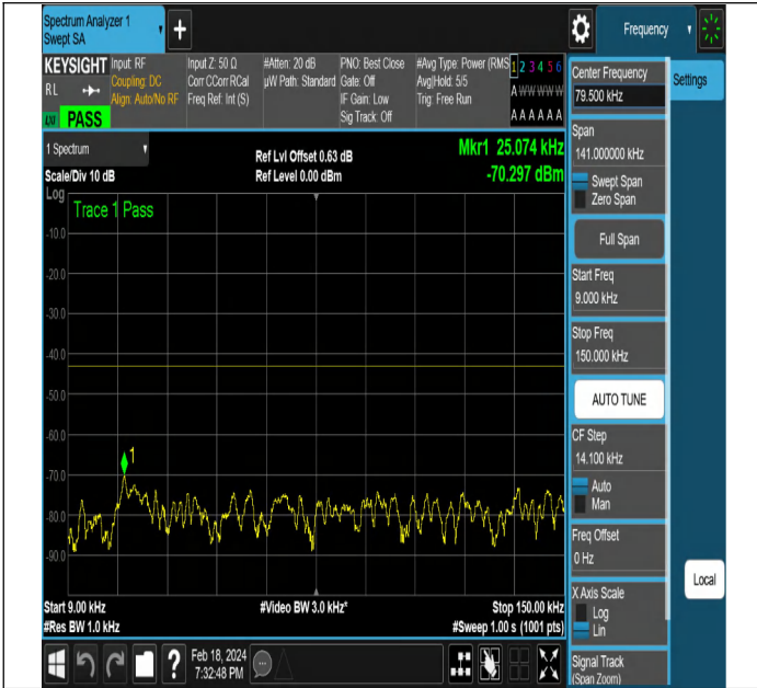
NTNV-DC_5A_n2A-PC3-15-5+20-M+L-QPSK-DFT-PI2BPSK- Edge_1RB_Left-PASS
