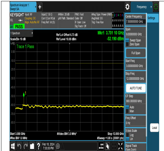
NTNV-DC_5A_n2A-PC3-15-5+20-M+L-QPSK-DFT-PI2BPSK- Edge_1RB_Left-PASS
