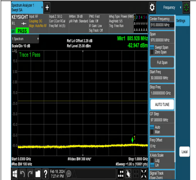
NTNV-DC_5A_n2A-PC3-15-5+15-M+H-QPSK-DFT-PI2BPSK- Edge_1RB_Left-PASS
