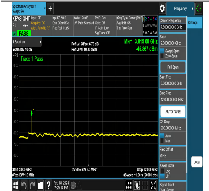
NTNV-DC_5A_n2A-PC3-15-5+15-M+H-QPSK-DFT-PI2BPSK-
