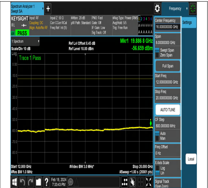
NTNV-DC_5A_n2A-PC3-15-5+20-M+L-QPSK-DFT-PI2BPSK- Edge_1RB_Left-PASS
