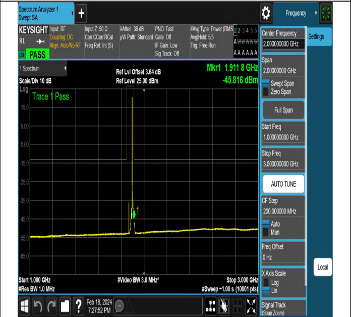
NTNV-DC_5A_n2A-PC3-15-5+15-M+H-QPSK-DFT-PI2BPSK- Edge_1RB_Left-PASS
