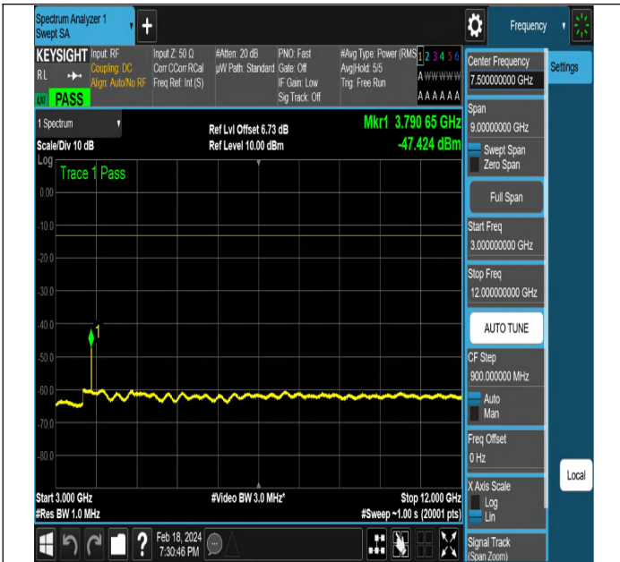
NTNV-DC_5A_n2A-PC3-15-5+15-M+H-QPSK-DFT-QPSK-Ed ge_1RB_Left-PASS
