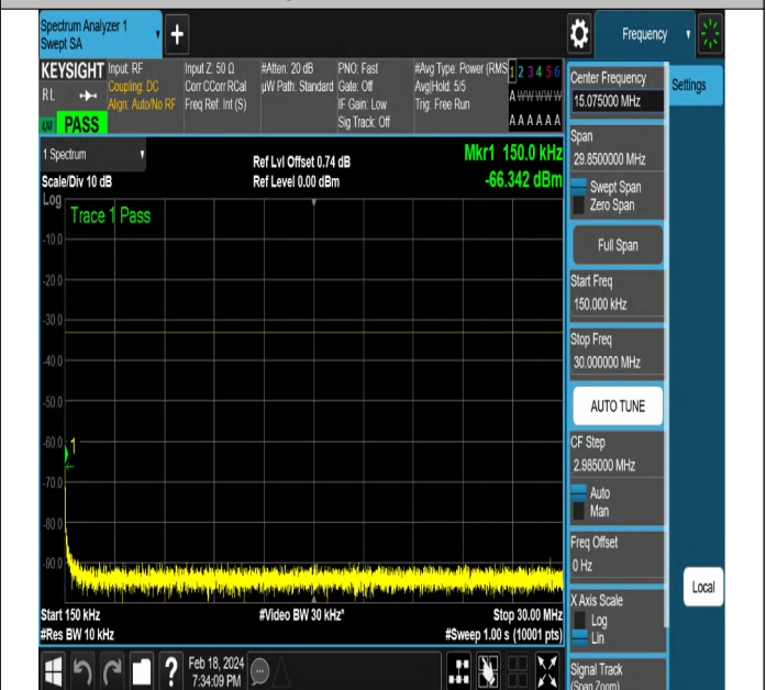
NTNV-DC_5A_n2A-PC3-15-5+20-M+L-QPSK-DFT-PI2BPSK- Edge_1RB_Right-PASS
