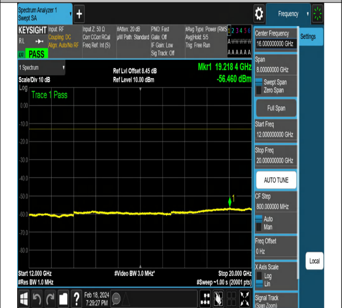
NTNV-DC_5A_n2A-PC3-15-5+15-M+H-QPSK-DFT-PI2BPSK-
