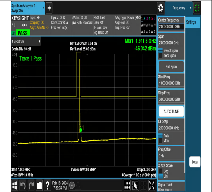
NTNV-DC_5A_n2A-PC3-15-5+15-M+H-QPSK-DFT-QPSK-Edge_1RB_Left-PASS
