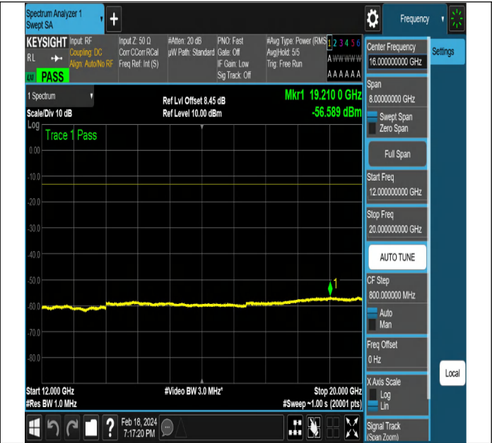
NTNV-DC_5A_n2A-PC3-15-5+15-M+L-QPSK-DFT-PI2BPSK- Edge_1RB_Left-PASS
