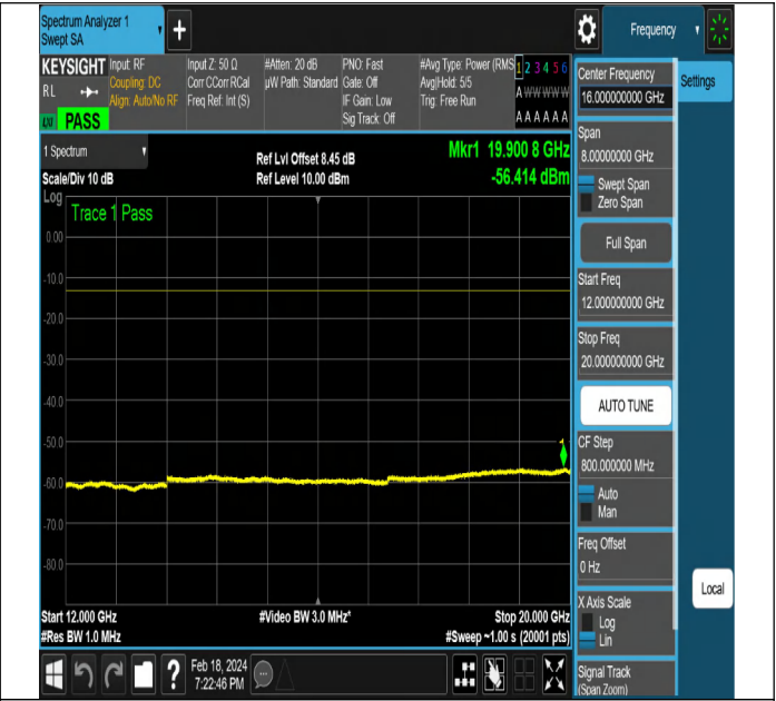
NTNV-DC_5A_n2A-PC3-15-5+15-M+M-QPSK-DFT-PI2BPSK-Edge_1RB_Left-PASS
