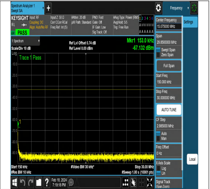
NTNV-DC_5A_n2A-PC3-15-5+15-M+L-QPSK-DFT-QPSK-Edg
