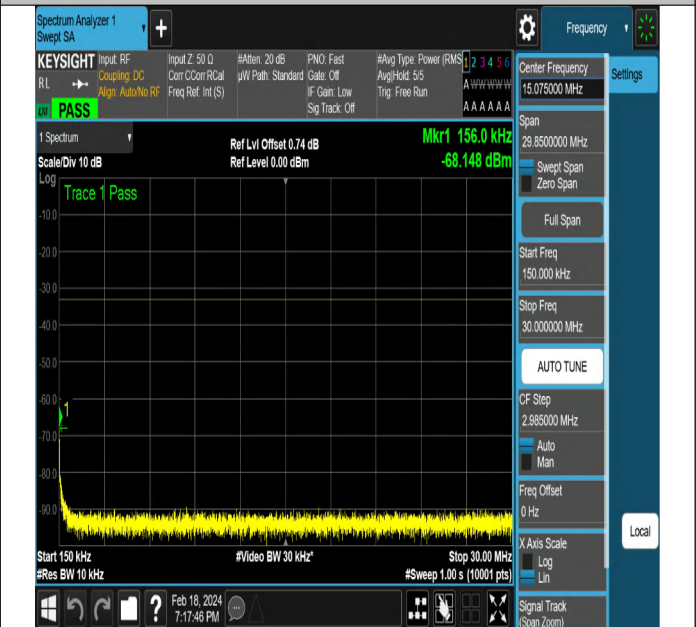
NTNV-DC_5A_n2A-PC3-15-5+15-M+L-QPSK-DFT-PI2BPSK- Edge_1RB_Right-PASS
