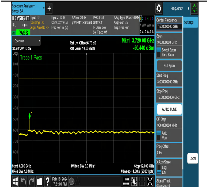
NTNV-DC_5A_n2A-PC3-15-5+15-M+L-QPSK-DFT-QPSK-Edg e_1RB_Right-PASS
