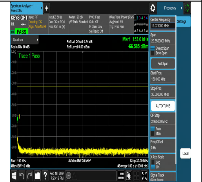
NTNV-DC_5A_n2A-PC3-15-5+15-M+M-QPSK-DFT-PI2BPSK-Edge_1RB_Right-PASS
