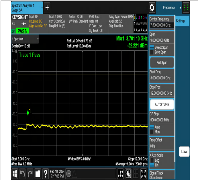
NTNV-DC_5A_n2A-PC3-15-5+15-M+L-QPSK-DFT-PI2BPSK- Edge_1RB_Left-PASS
