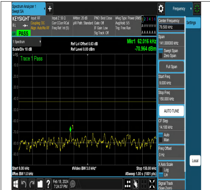
NTNV-DC_5A_n2A-PC3-15-5+15-M+M-QPSK-DFT-QPSK-Edge_1RB_Left-PASS
