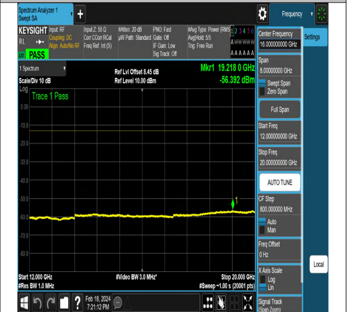
NTNV-DC_5A_n2A-PC3-15-5+15-M+L-QPSK-DFT-QPSK-Edg e_1RB_Right-PASS
