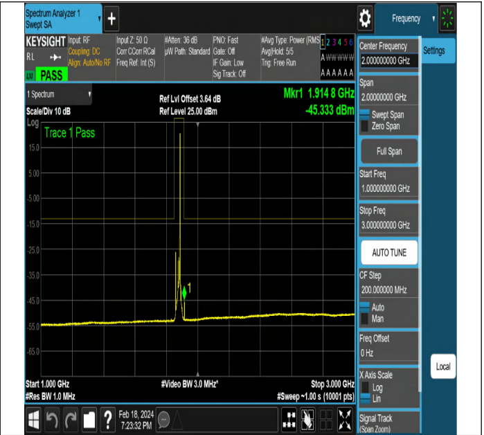
NTNV-DC_5A_n2A-PC3-15-5+15-M+M-QPSK-DFT-PI2BPSK-Edge_1RB_Right-PASS
