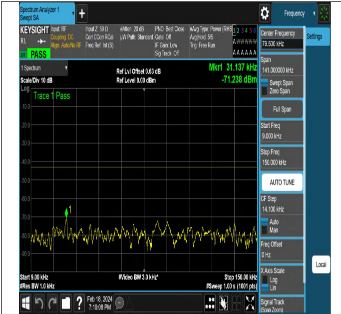
NTNV-DC_5A_n2A-PC3-15-5+15-M+L-QPSK-DFT-QPSK-Edg
