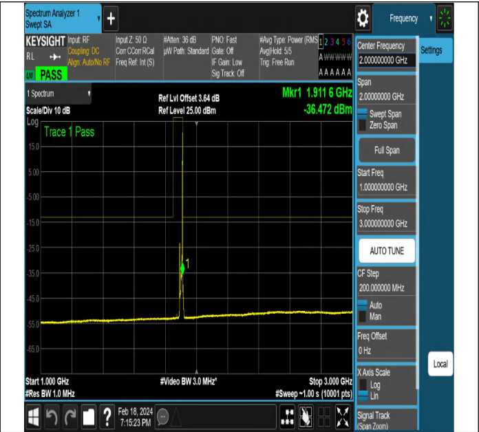
NTNV-DC_5A_n2A-PC3-15-5+10-M+H-QPSK-DFT-QPSK-Ed ge_1RB_Right-PASS
