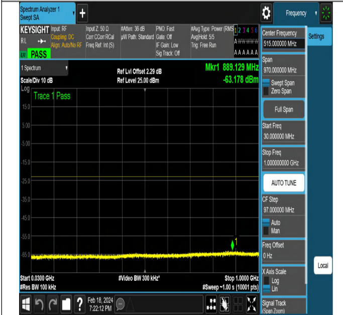
NTNV-DC_5A_n2A-PC3-15-5+15-M+M-QPSK-DFT-PI2BPSK-Edge_1RB_Left-PASS
