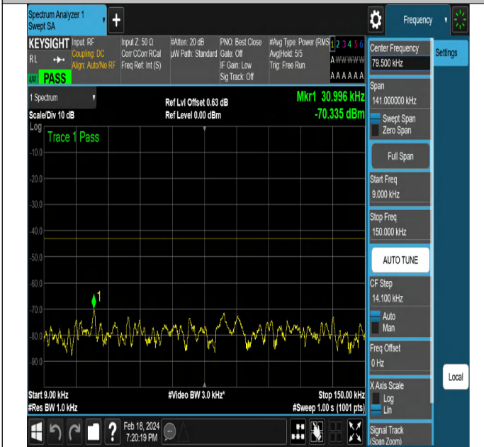
NTNV-DC_5A_n2A-PC3-15-5+15-M+L-QPSK-DFT-QPSK-Edge e_1RB_Right-PASS
