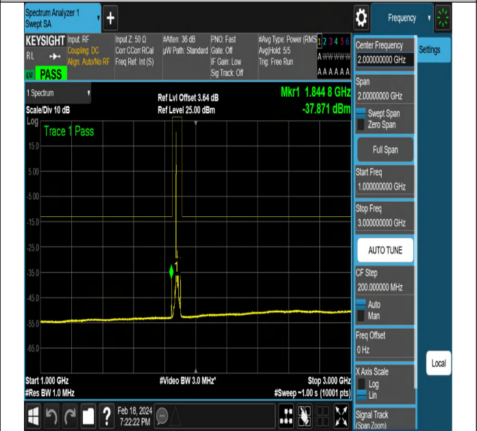
NTNV-DC_5A_n2A-PC3-15-5+15-M+M-QPSK-DFT-PI2BPSK-Edge_1RB_Left-PASS
