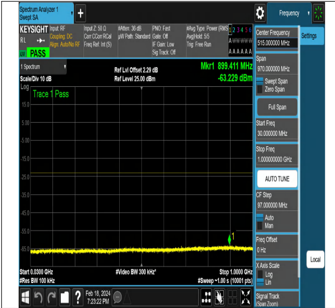
NTNV-DC_5A_n2A-PC3-15-5+15-M+M-QPSK-DFT-PI2BPSK-Edge_1RB_Right-PASS
