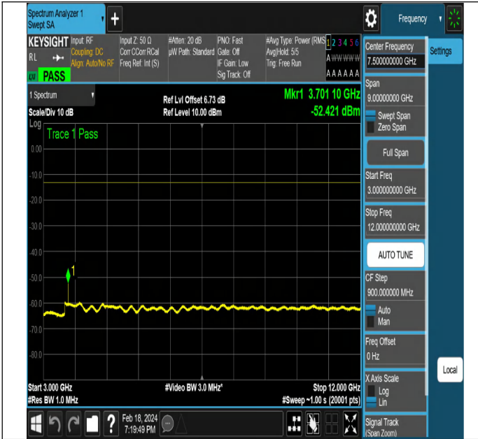
NTNV-DC_5A_n2A-PC3-15-5+15-M+L-QPSK-DFT-QPSK-Edge e_1RB_Left-PASS
