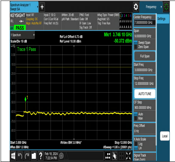
NTNV-DC_5A_n2A-PC3-15-5+15-M+M-QPSK-DFT-PI2BPSK-Edge_1RB_Left-PASS
