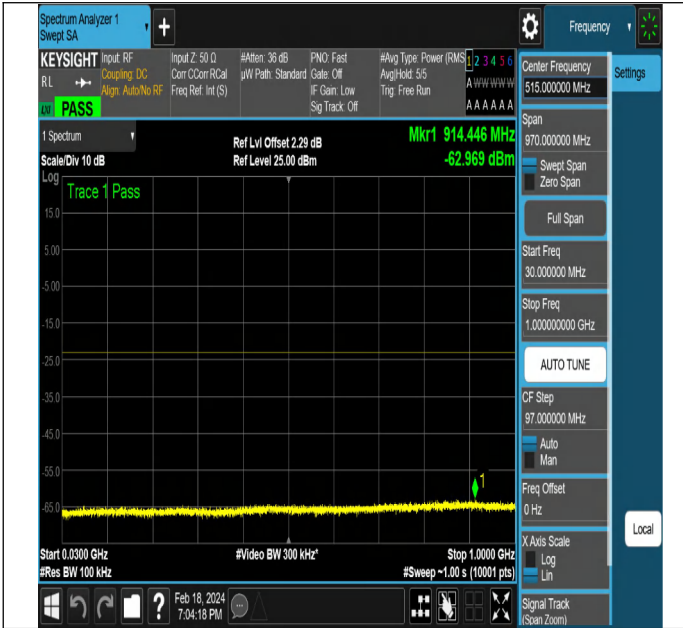
NTNV-DC_5A_n2A-PC3-15-5+10-M+L-QPSK-DFT-QPSK-Edge_e_1RB_Right-PASS
