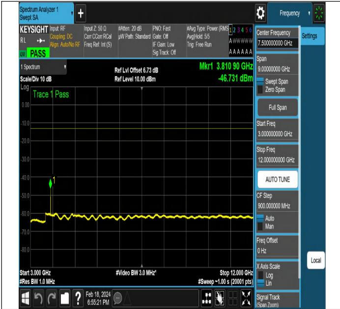
NTNV-DC_5A_n2A-PC3-15-5+5-M+H-QPSK-DFT-PI2BPSK-E dge_1RB_Left-PASS
