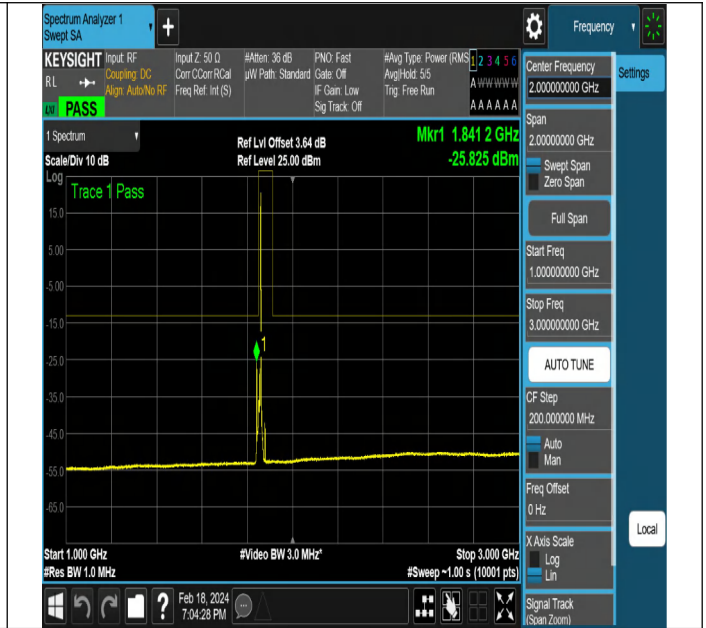
NTNV-DC_5A_n2A-PC3-15-5+10-M+L-QPSK-DFT-QPSK-Edge_e_1RB_Right-PASS
