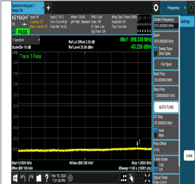
NTNV-DC_5A_n2A-PC3-15-5+10-M+L-QPSK-DFT-PI2BPSK-Edge_1RB_Right-PASS
