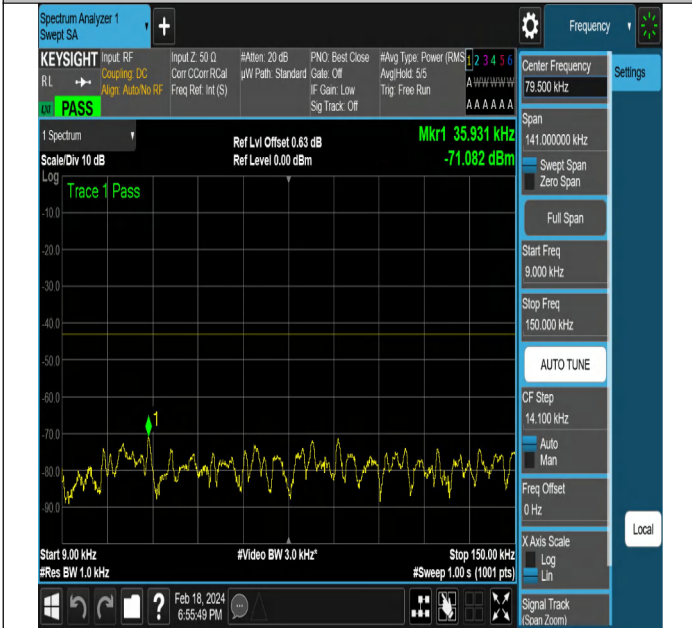
NTNV-DC_5A_n2A-PC3-15-5+5-M+H-QPSK-DFT-PI2BPSK-E dge_1RB_Right-PASS
