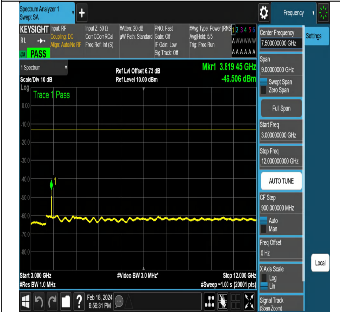
NTNV-DC_5A_n2A-PC3-15-5+5-M+H-QPSK-DFT-PI2BPSK-E dge_1RB_Right-PASS
