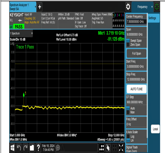
NTNV-DC_5A_n2A-PC3-15-5+10-M+L-QPSK-DFT-QPSK-Edge_e_1RB_Right-PASS
