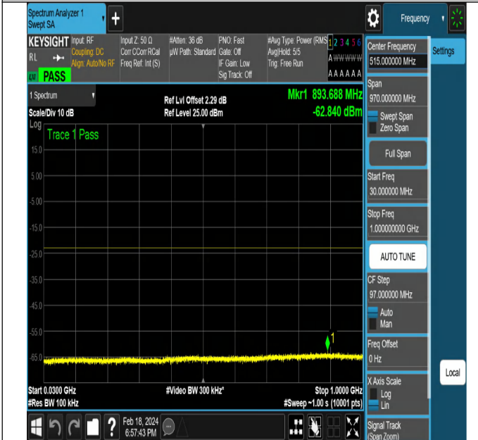
NTNV-DC_5A_n2A-PC3-15-5+5-M+H-QPSK-DFT-QPSK-Edge e_1RB_Left-PASS
