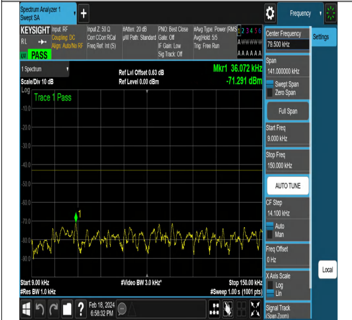
NTNV-DC_5A_n2A-PC3-15-5+5-M+H-QPSK-DFT-QPSK-Edge e_1RB_Right-PASS
