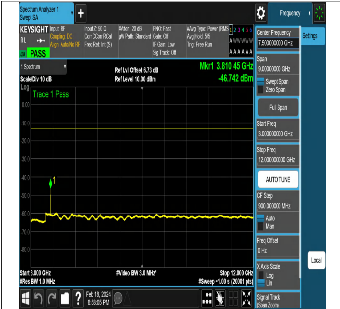
NTNV-DC_5A_n2A-PC3-15-5+5-M+H-QPSK-DFT-QPSK-Edge e_1RB_Left-PASS
