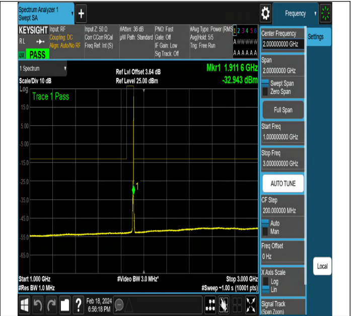
NTNV-DC_5A_n2A-PC3-15-5+5-M+H-QPSK-DFT-PI2BPSK-E dge_1RB_Right-PASS
