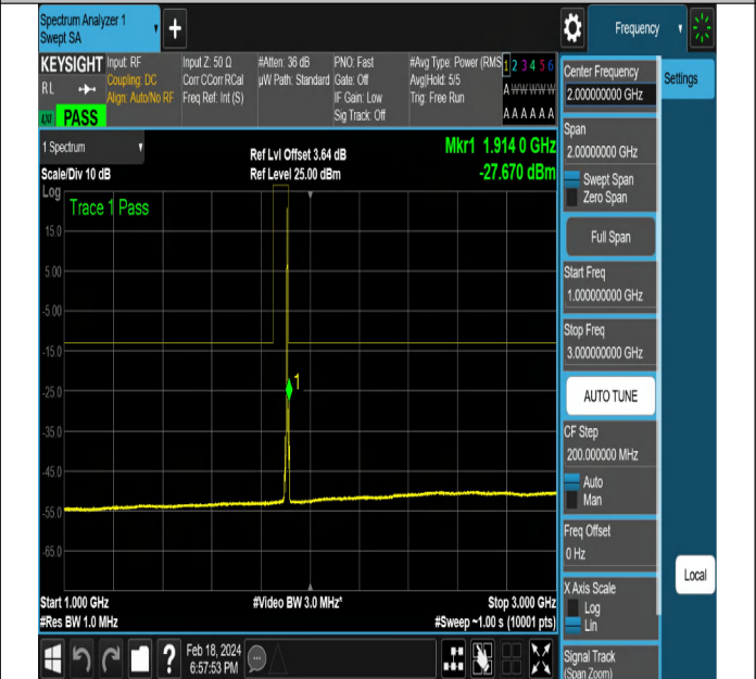
NTNV-DC_5A_n2A-PC3-15-5+5-M+H-QPSK-DFT-QPSK-Edge e_1RB_Left-PASS
