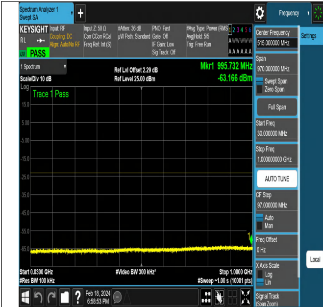
NTNV-DC_5A_n2A-PC3-15-5+5-M+H-QPSK-DFT-QPSK-Edg e_1RB_Right-PASS
