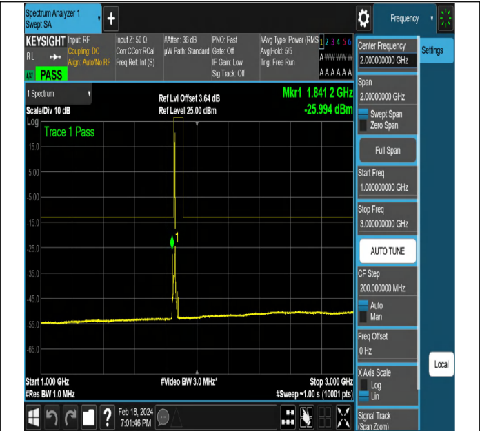
NTNV-DC_5A_n2A-PC3-15-5+10-M+L-QPSK-DFT-PI2BPSK-Edge_1RB_Right-PASS
