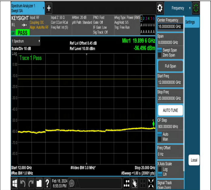
NTNV-DC_5A_n2A-PC3-15-5+5-M+H-QPSK-DFT-PI2BPSK-E dge_1RB_Left-PASS
