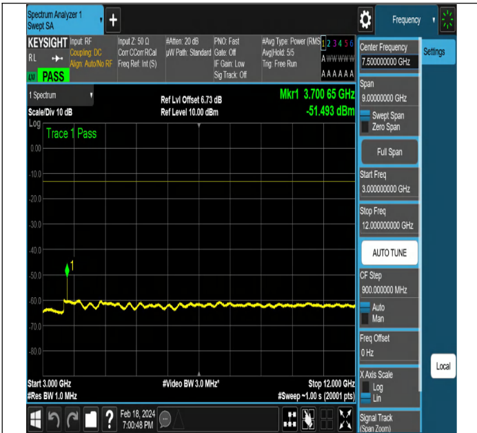
NTNV-DC_5A_n2A-PC3-15-5+10-M+L-QPSK-DFT-PI2BPSK- Edge_1RB_Left-PASS
