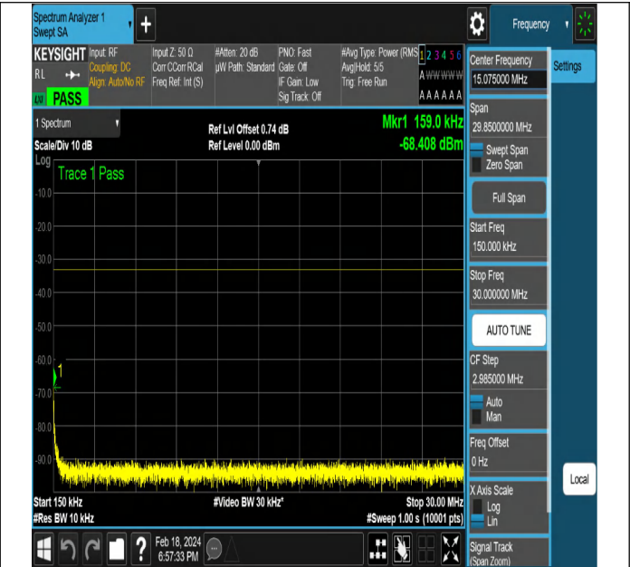
NTNV-DC_5A_n2A-PC3-15-5+5-M+H-QPSK-DFT-QPSK-Edge e_1RB_Left-PASS
