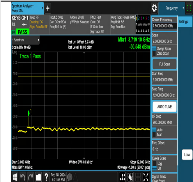
NTNV-DC_5A_n2A-PC3-15-5+10-M+L-QPSK-DFT-PI2BPSK-Edge_1RB_Right-PASS
