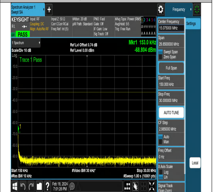
NTNV-DC_5A_n2A-PC3-15-5+10-M+L-QPSK-DFT-PI2BPSK- Edge_1RB_Right-PASS
