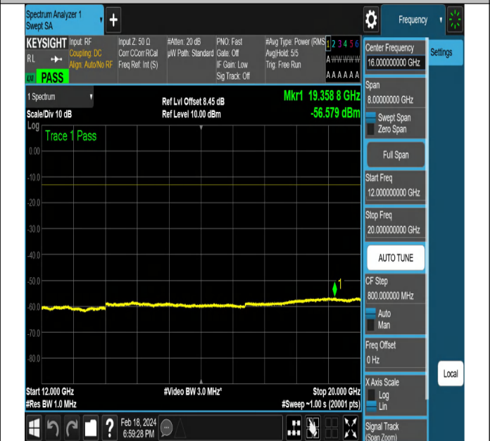
NTNV-DC_5A_n2A-PC3-15-5+5-M+H-QPSK-DFT-QPSK-Edg e_1RB_Right-PASS
