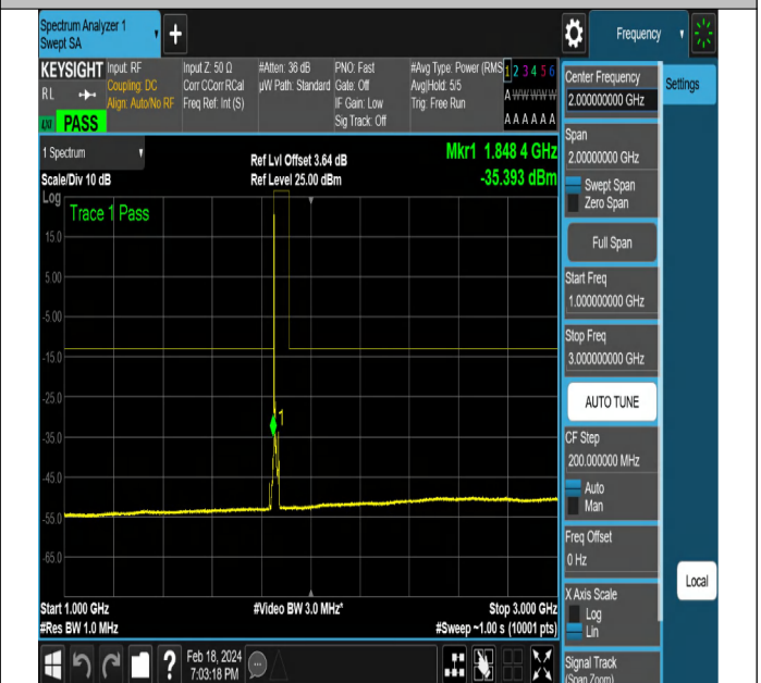
NTNV-DC_5A_n2A-PC3-15-5+10-M+L-QPSK-DFT-QPSK-Edge e_1RB_Left-PASS
