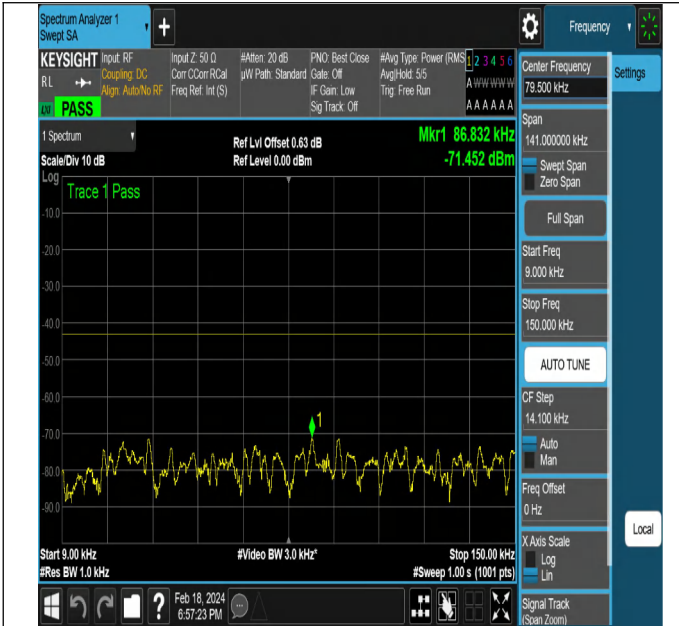
NTNV-DC_5A_n2A-PC3-15-5+5-M+H-QPSK-DFT-QPSK-Edge e_1RB_Left-PASS
