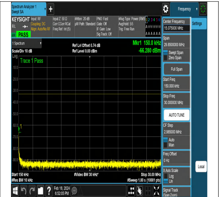
NTNV-DC_5A_n2A-PC3-15-5+5-M+M-QPSK-DFT-QPSK-Edge e_1RB_Left-PASS
