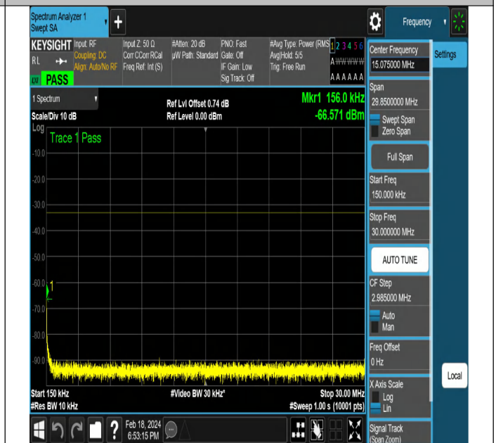
NTNV-DC_5A_n2A-PC3-15-5+5-M+M-QPSK-DFT-QPSK-Edge e_1RB_Right-PASS
