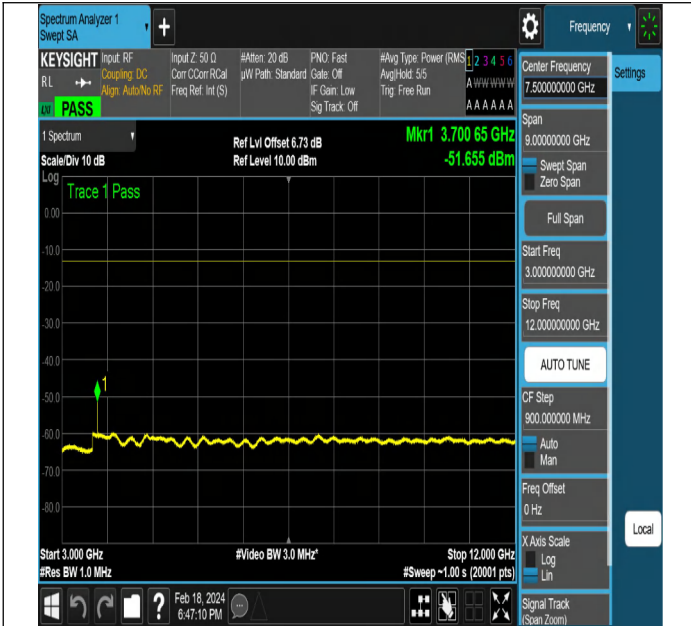
NTNV-DC_5A_n2A-PC3-15-5+5-M+L-QPSK-DFT-QPSK-Edge _1RB_Left-PASS
