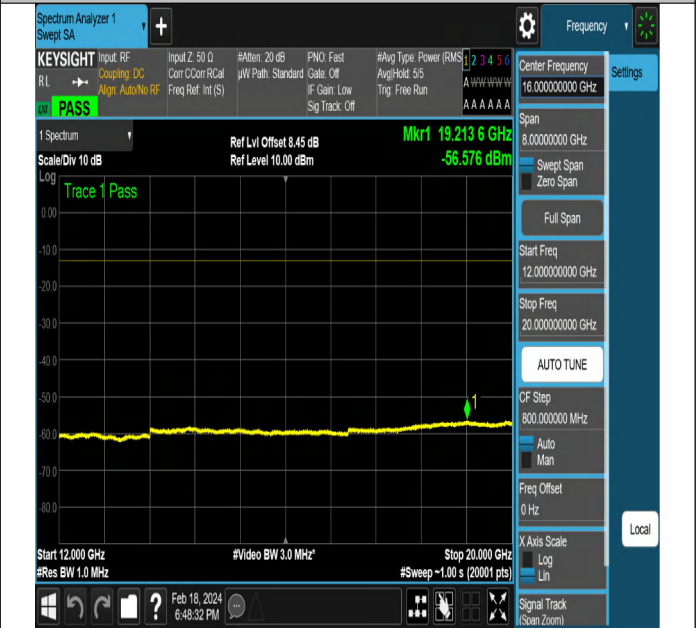
NTNV-DC_5A_n2A-PC3-15-5+5-M+L-QPSK-DFT-QPSK-Edge _1RB_Right-PASS
