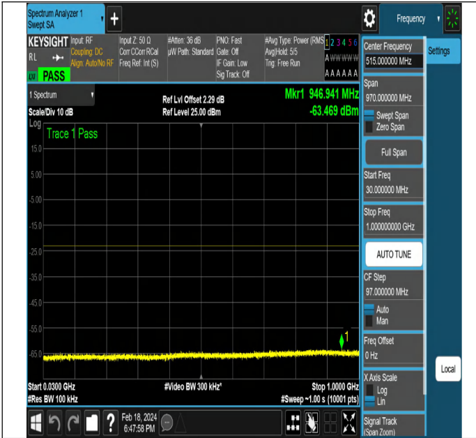
NTNV-DC_5A_n2A-PC3-15-5+5-M+L-QPSK-DFT-QPSK-Edge _1RB_Right-PASS
