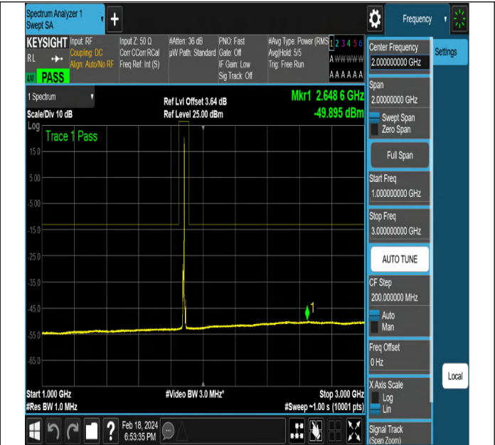
NTNV-DC_5A_n2A-PC3-15-5+5-M+M-QPSK-DFT-QPSK-Edge e_1RB_Right-PASS
