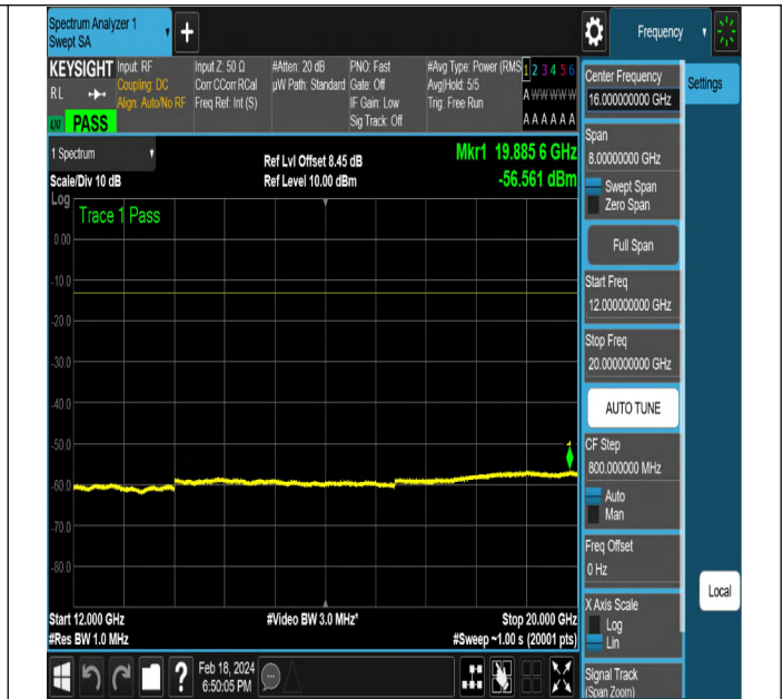
NTNV-DC_5A_n2A-PC3-15-5+5-M+M-QPSK-DFT-PI2BPSK-E
