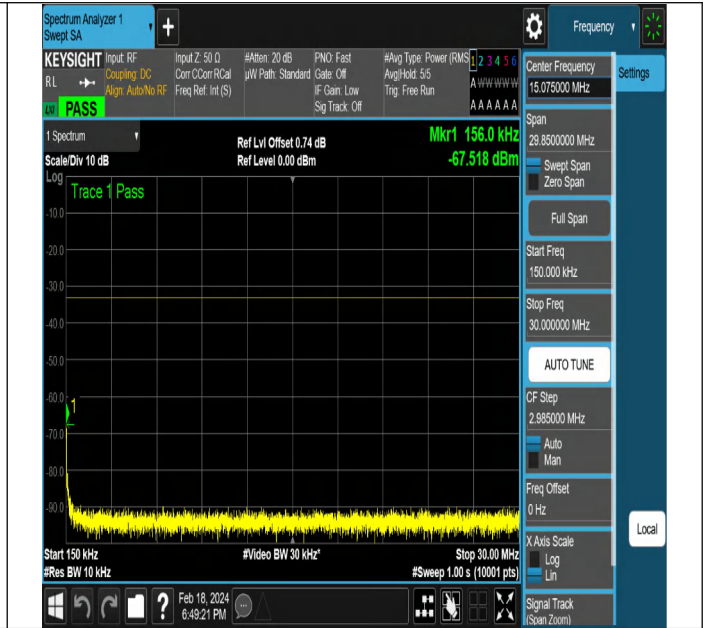
NTNV-DC_5A_n2A-PC3-15-5+5-M+M-QPSK-DFT-PI2BPSK-E dge_1RB_Left-PASS
