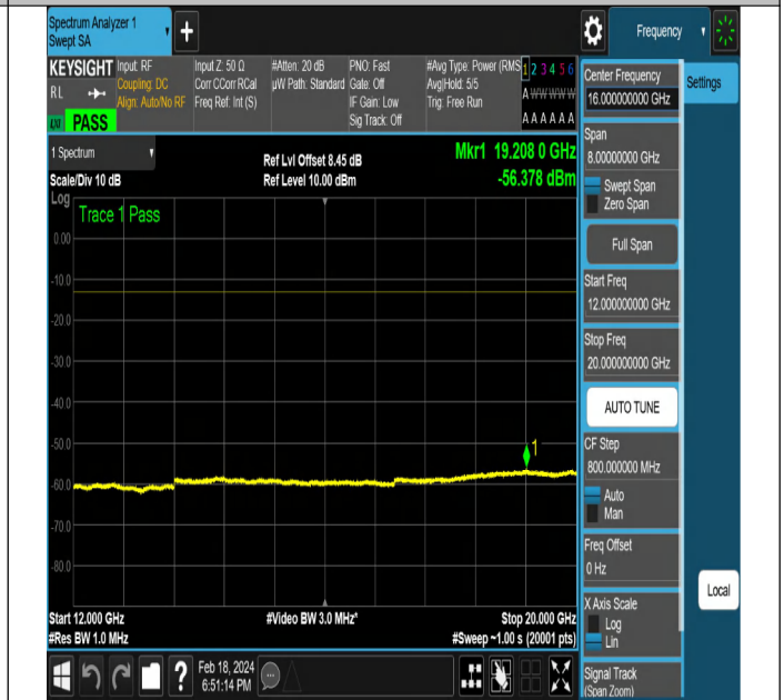
NTNV-DC_5A_n2A-PC3-15-5+5-M+M-QPSK-DFT-PI2BPSK-E dge_1RB_Right-PASS
