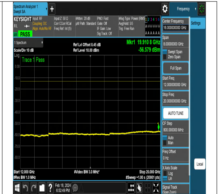
NTNV-DC_5A_n2A-PC3-15-5+5-M+M-QPSK-DFT-QPSK-Edge e_1RB_Left-PASS
