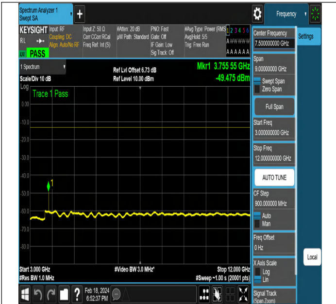
NTNV-DC_5A_n2A-PC3-15-5+5-M+M-QPSK-DFT-QPSK-Edge e_1RB_Left-PASS
