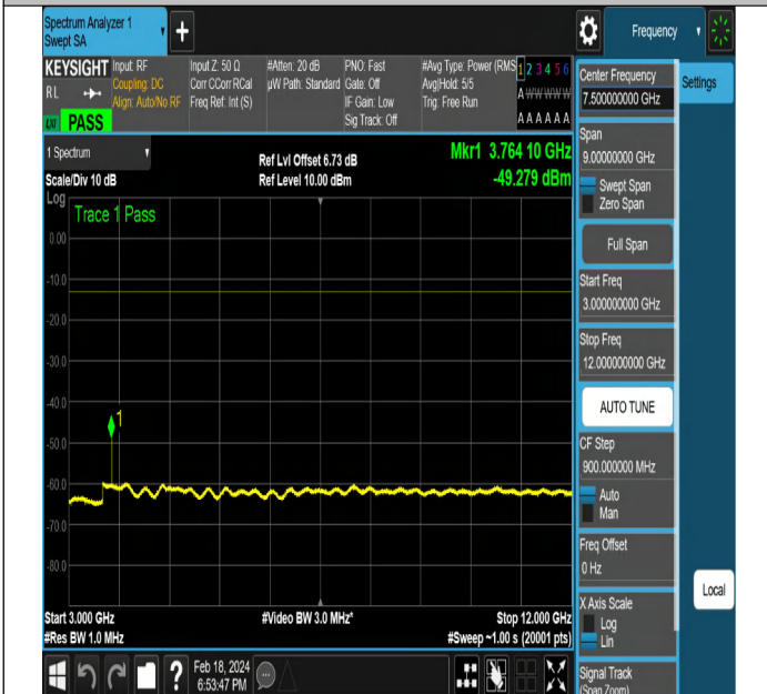
NTNV-DC_5A_n2A-PC3-15-5+5-M+M-QPSK-DFT-QPSK-Edge e_1RB_Right-PASS
