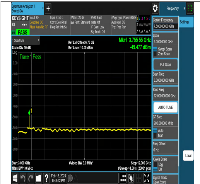
NTNV-DC_5A_n2A-PC3-15-5+5-M+M-QPSK-DFT-PI2BPSK-E
