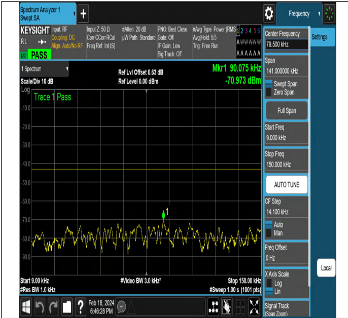
NTNV-DC_5A_n2A-PC3-15-5+5-M+L-QPSK-DFT-QPSK-Edge _1RB_Left-PASS
