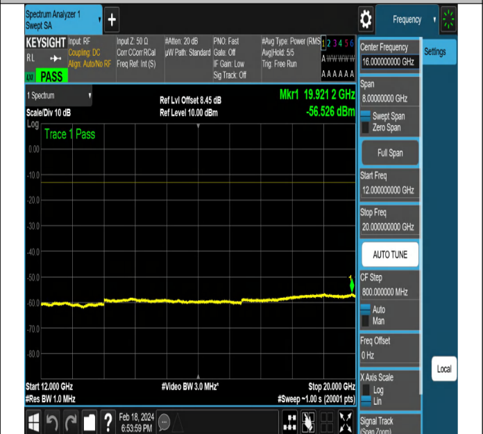
NTNV-DC_5A_n2A-PC3-15-5+5-M+M-QPSK-DFT-QPSK-Edge e_1RB_Right-PASS
