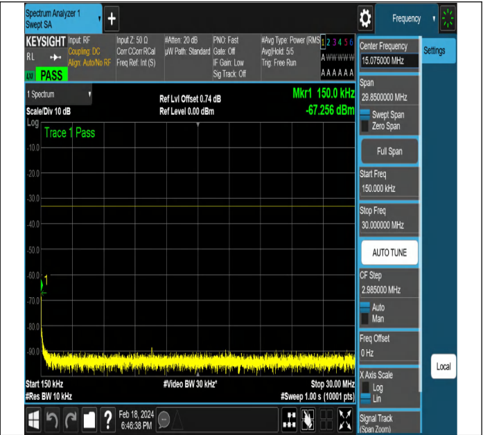
NTNV-DC_5A_n2A-PC3-15-5+5-M+L-QPSK-DFT-QPSK-Edge _1RB_Left-PASS
