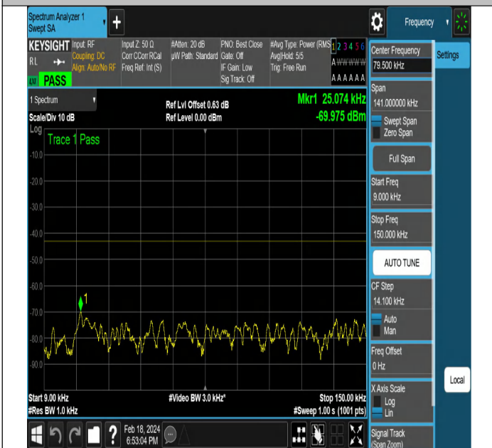
NTNV-DC_5A_n2A-PC3-15-5+5-M+M-QPSK-DFT-QPSK-Edge e_1RB_Right-PASS
