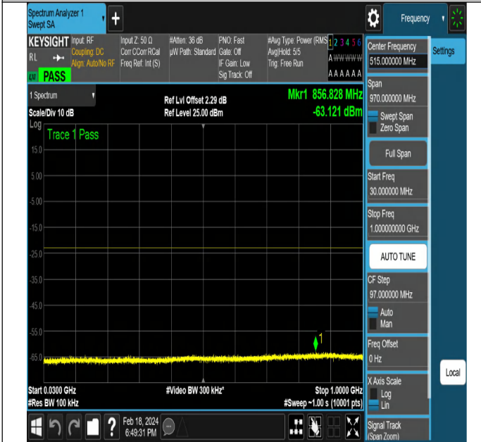
NTNV-DC_5A_n2A-PC3-15-5+5-M+M-QPSK-DFT-PI2BPSK-E dge_1RB_Left-PASS
