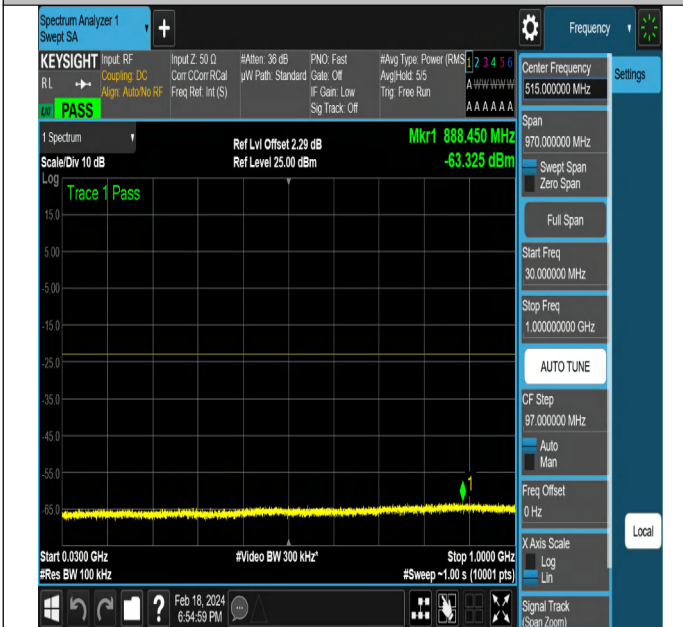
NTNV-DC_5A_n2A-PC3-15-5+5-M+H-QPSK-DFT-PI2BPSK-E dge_1RB_Left-PASS
