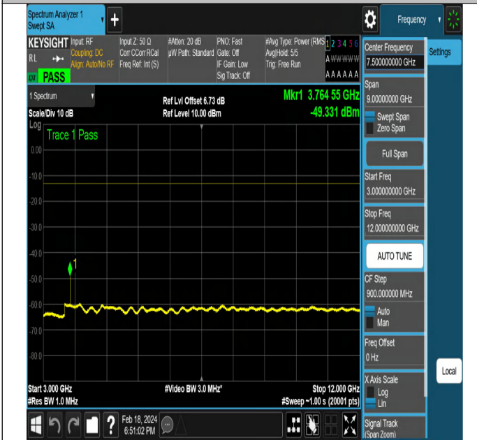
NTNV-DC_5A_n2A-PC3-15-5+5-M+M-QPSK-DFT-PI2BPSK-E dge_1RB_Right-PASS
