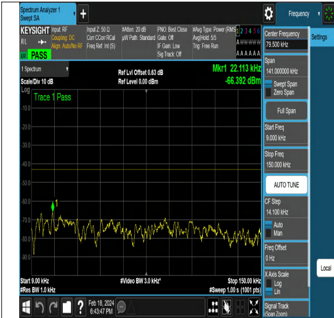
NTNV-DC_5A_n2A-PC3-15-5+5-M+L-QPSK-DFT-PI2BPSK-E dge_1RB_Left-PASS
