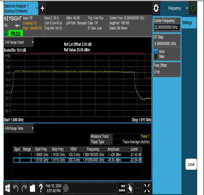
NTNV-DC_5A_n2A-PC3-15-5+20-M+H-QPSK-DFT-PI2BPSK-K-Outer_Full-PASS
