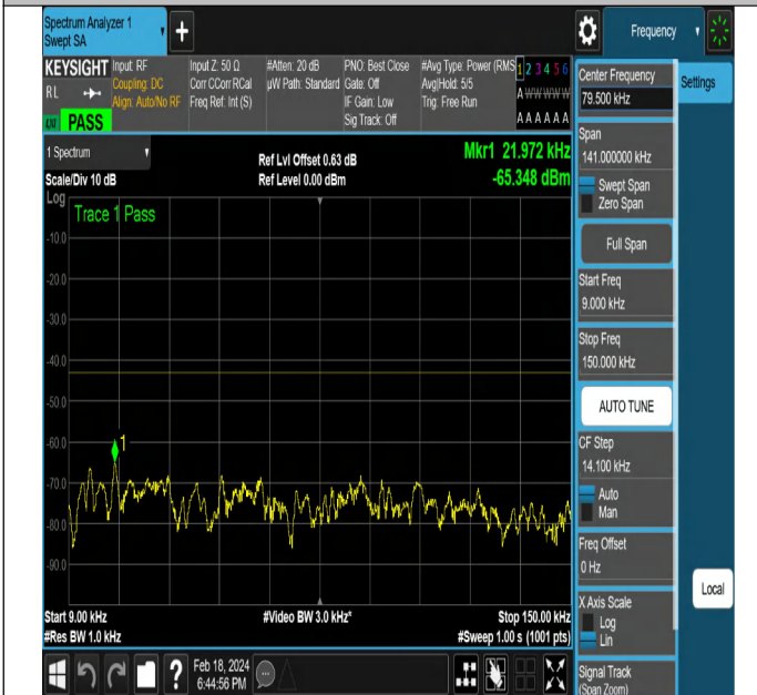
NTNV-DC_5A_n2A-PC3-15-5+5-M+L-QPSK-DFT-PI2BPSK-E dge_1RB_Right-PASS
