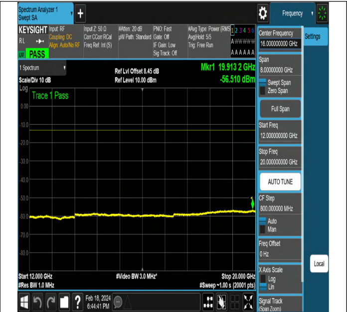
NTNV-DC_5A_n2A-PC3-15-5+5-M+L-QPSK-DFT-PI2BPSK-E dge_1RB_Left-PASS
