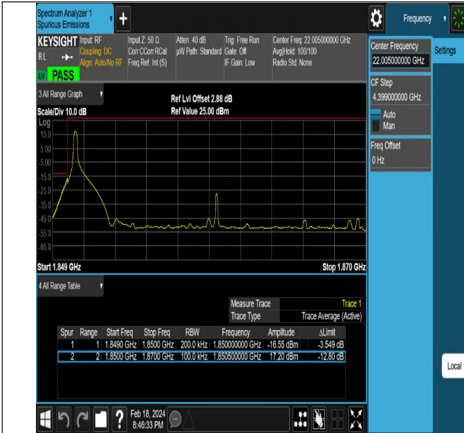
NTNV-DC_5A_n2A-PC3-15-5+20-M+L-QPSK-DFT-PI2BPSK-Ed ge_1RB_Left-PASS
