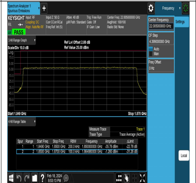
NTNV-DC_5A_n2A-PC3-15-5+20-M+L-QPSK-DFT-QPSK- Outer_Full-PASS
