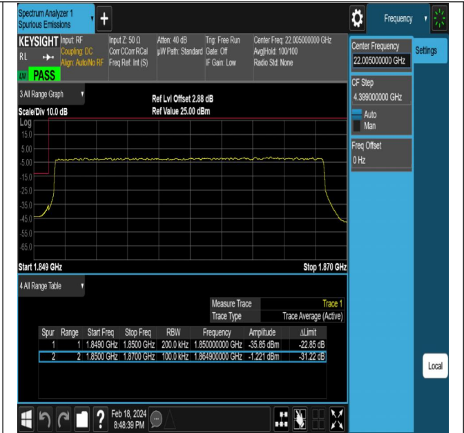
NTNV-DC_5A_n2A-PC3-15-5+20-M+L-QPSK-DFT-PI2BPS K-Outer_Full-PASS
