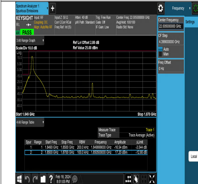
NTNV-DC_5A_n2A-PC3-15-5+20-M+L-QPSK-DFT-QPSK-Edge_ 1RB_Left-PASS
