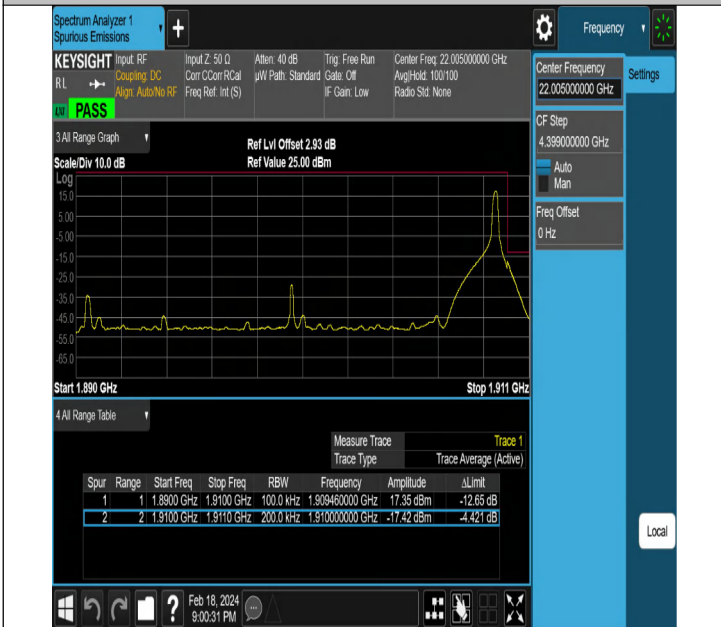
NTNV-DC_5A_n2A-PC3-15-5+20-M+H-QPSK-DFT-QPSK-Edge_1RB_Right-PASS
