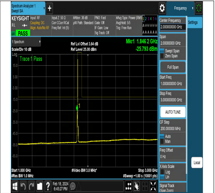
NTNV-DC_5A_n2A-PC3-15-5+5-M+L-QPSK-DFT-PI2BPSK-E dge_1RB_Right-PASS
