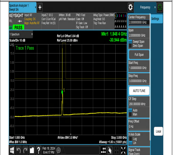
NTNV-DC_5A_n2A-PC3-15-5+5-M+L-QPSK-DFT-PI2BPSK-E dge_1RB_Left-PASS
