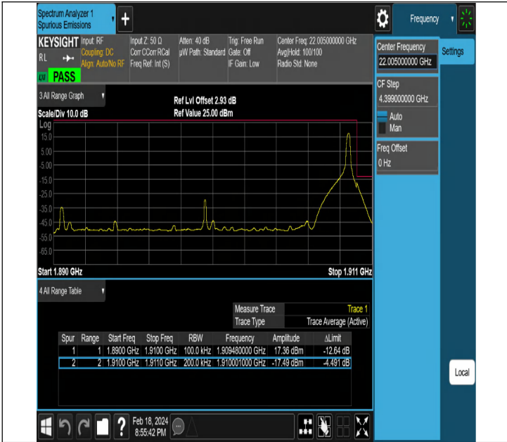
NTNV-DC_5A_n2A-PC3-15-5+20-M+H-QPSK-DFT-PI2BPSK-Edge_1RB_Right-PASS
