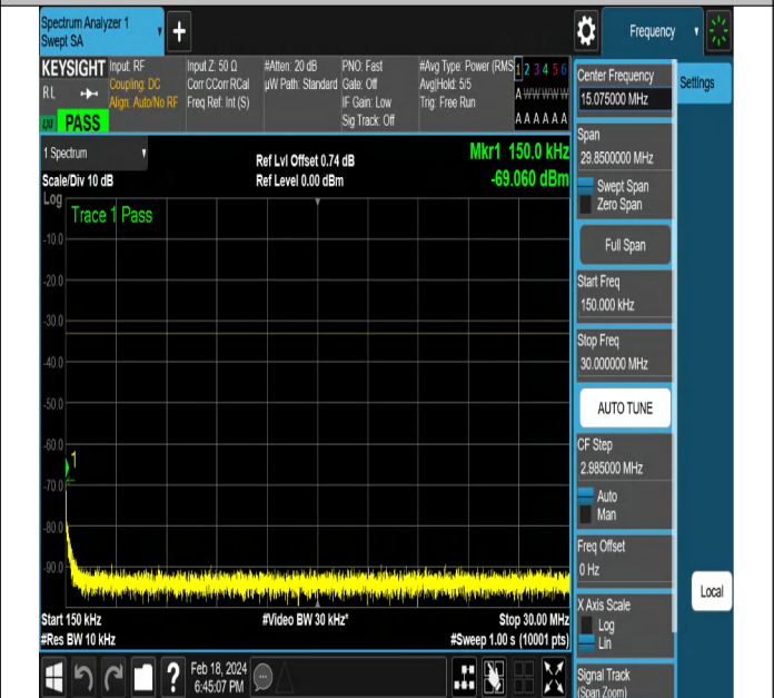
NTNV-DC_5A_n2A-PC3-15-5+5-M+L-QPSK-DFT-PI2BPSK-E dge_1RB_Right-PASS
