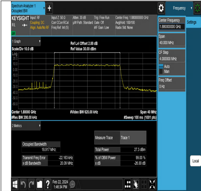
NTNV-DC_5A_n2A-PC3-15-5+20-M+M-N/A-N/A-CP-QPSK-Outer_Full-Ant1-PASS
