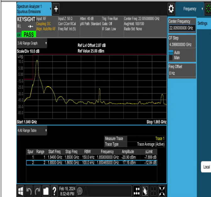
NTNV-DC_5A_n2A-PC3-15-5+15-M+L-QPSK-DFT-QPSK-Edge_ 1RB_Left-PASS
