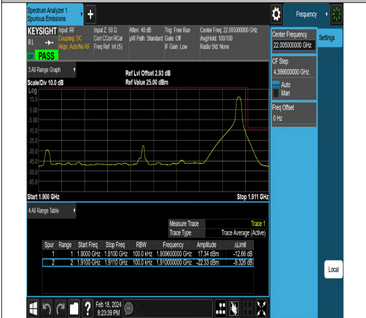
NTNV-DC_5A_n2A-PC3-15-5+10-M+H-QPSK-DFT-QPSK-Edge_1RB_Right-PASS
