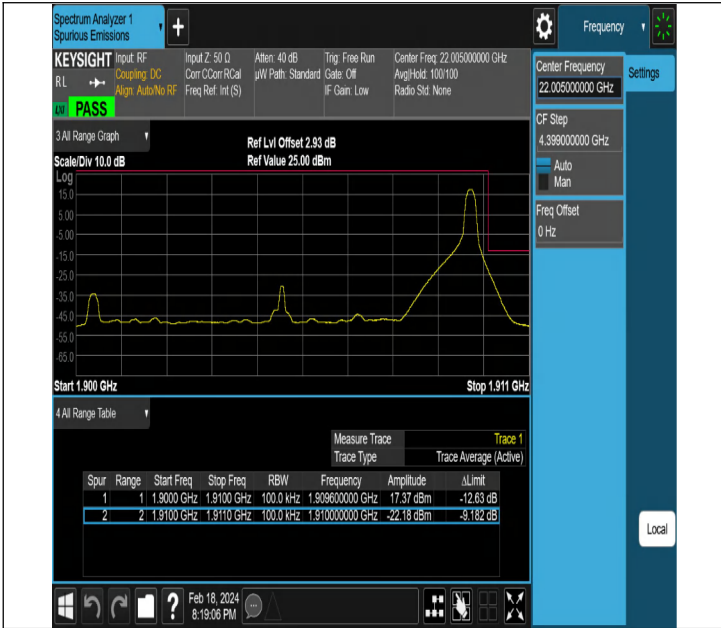
NTNV-DC_5A_n2A-PC3-15-5+10-M+H-QPSK-DFT-PI2BPSK-Edge_1RB_Right-PASS
