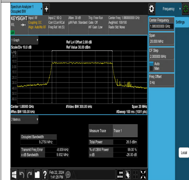
NTNV-DC_5A_n2A-PC3-15-5+10-M+M-N/A-N/A-CP-64QAM-Outer_Full-Ant1-PASS
