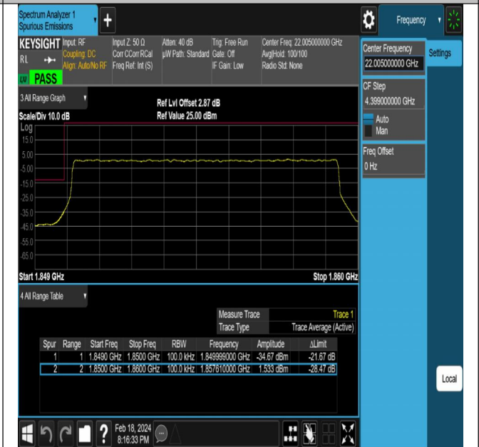
NTNV-DC_5A_n2A-PC3-15-5+10-M+L-QPSK-DFT-QPSK- Outer_Full-PASS
