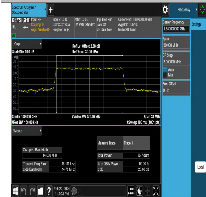
NTNV-DC_5A_n2A-PC3-15-5+15-M+M-N/A-N/A-CP-64QAM-Outer_Full-Ant1-PASS
