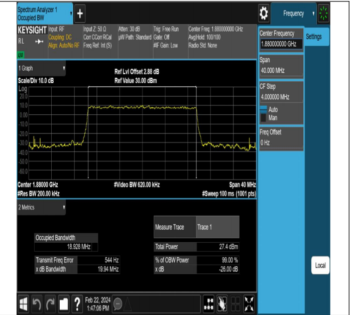
NTNV-DC_5A_n2A-PC3-15-5+20-M+M-N/A-N/A-CP-16QAM-Outer_Full-Ant1-PASS
