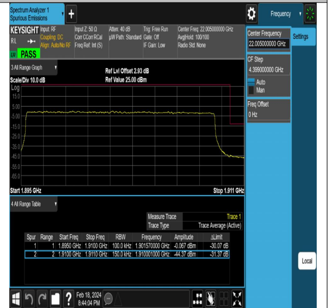
NTNV-DC_5A_n2A-PC3-15-5+15-M+H-QPSK-DFT-QPSK-Outer_Full-PASS
