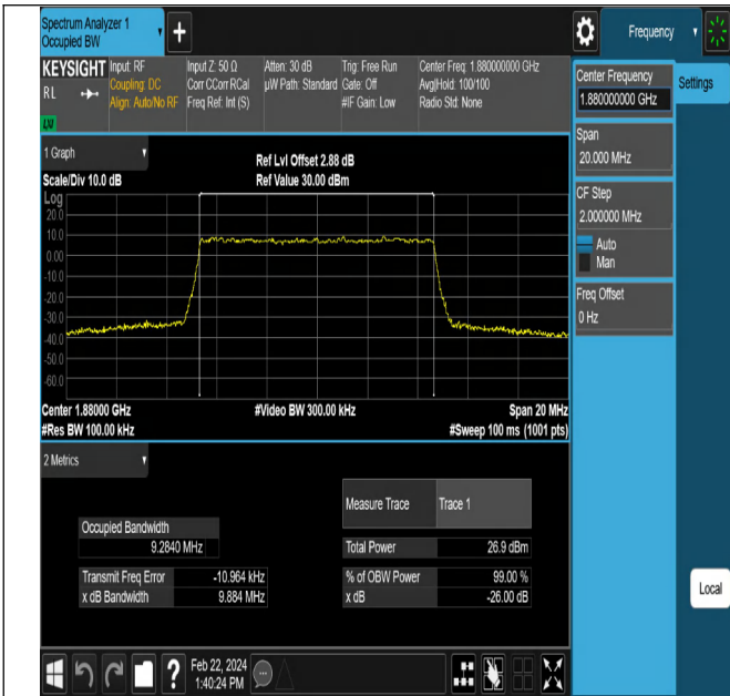
NTNV-DC_5A_n2A-PC3-15-5+10-M+M-N/A-N/A-CP-QPSK-Outer_Full-Ant1-PASS
