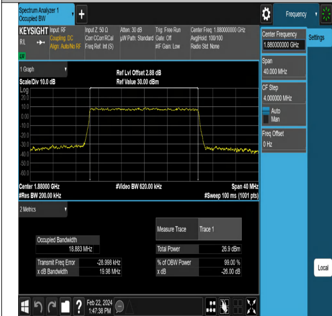
NTNV-DC_5A_n2A-PC3-15-5+20-M+M-N/A-N/A-CP-64QAM-Outer_Full-Ant1-PASS
