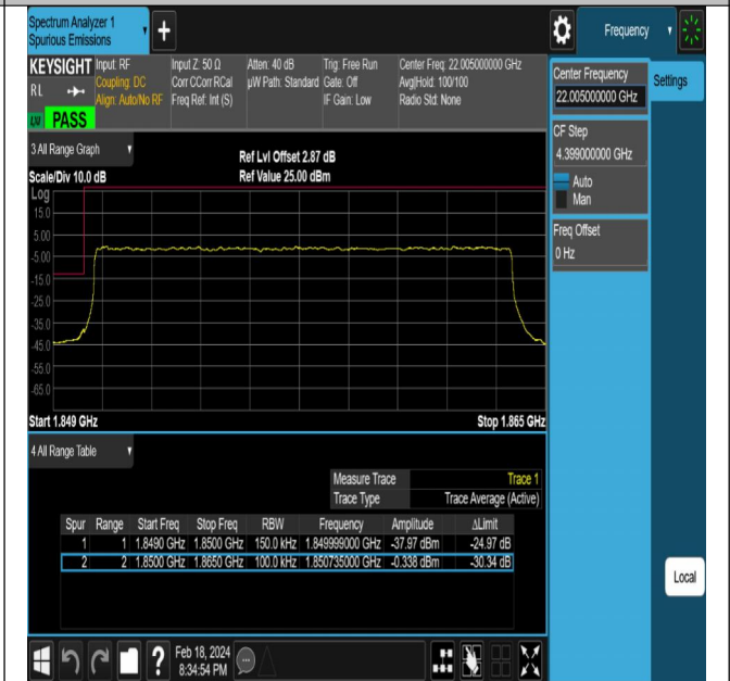
NTNV-DC_5A_n2A-PC3-15-5+15-M+L-QPSK-DFT-QPSK- Outer_Full-PASS
