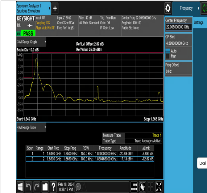
NTNV-DC_5A_n2A-PC3-15-5+15-M+L-QPSK-DFT-PI2BPSK-Ed ge_1RB_Left-PASS
