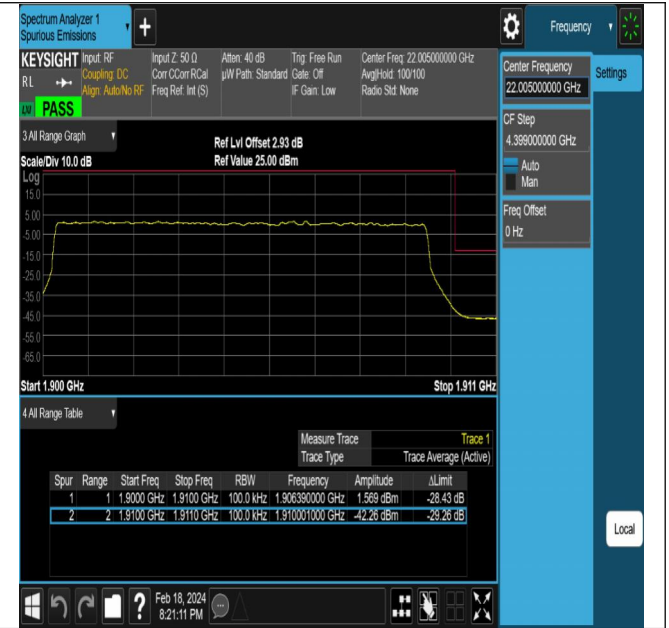
NTNV-DC_5A_n2A-PC3-15-5+10-M+H-QPSK-DFT-PI2BPSK-K-Outer_Full-PASS
