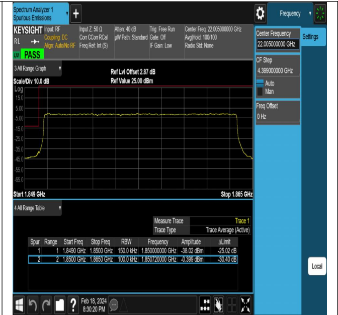
NTNV-DC_5A_n2A-PC3-15-5+15-M+L-QPSK-DFT-PI2BPS K-Outer_Full-PASS
