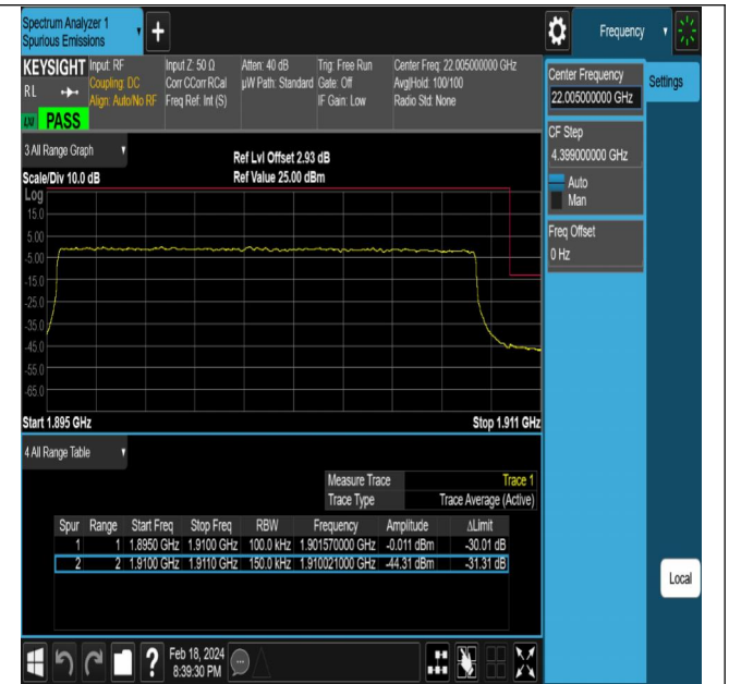
NTNV-DC_5A_n2A-PC3-15-5+15-M+H-QPSK-DFT-PI2BPSK-K-Outer_Full-PASS
