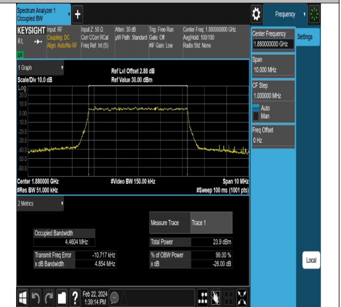
NTNV-DC_5A_n2A-PC3-15-5+5-M+M-N/A-N/A-CP-256QAM-Outer_Full-Ant1-PASS
