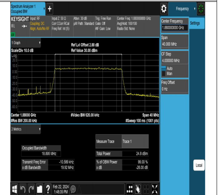
NTNV-DC_5A_n2A-PC3-15-5+20-M+M-N/A-N/A-CP-256QAM-Outer_Full-Ant1-PASS
