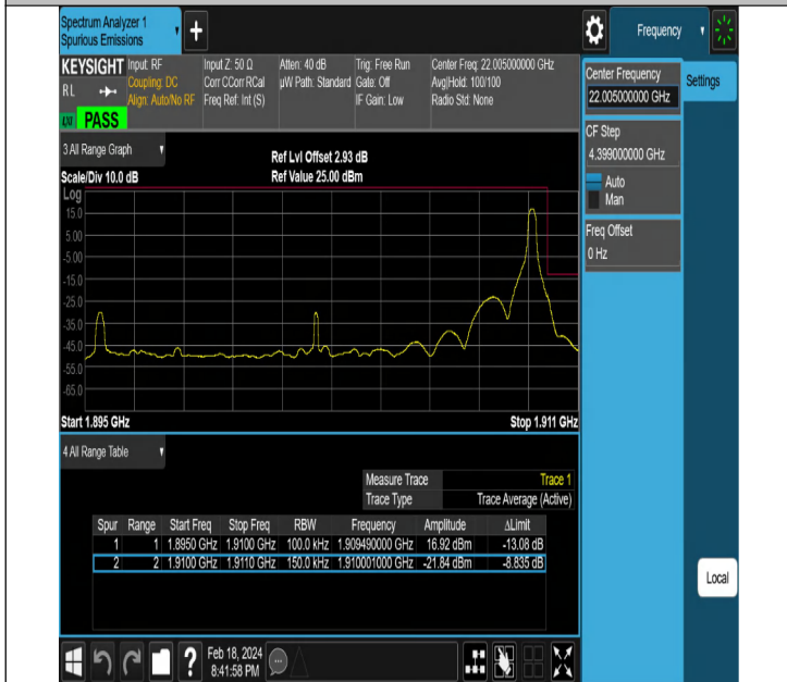
NTNV-DC_5A_n2A-PC3-15-5+15-M+H-QPSK-DFT-QPSK-Edge_1RB_Right-PASS
