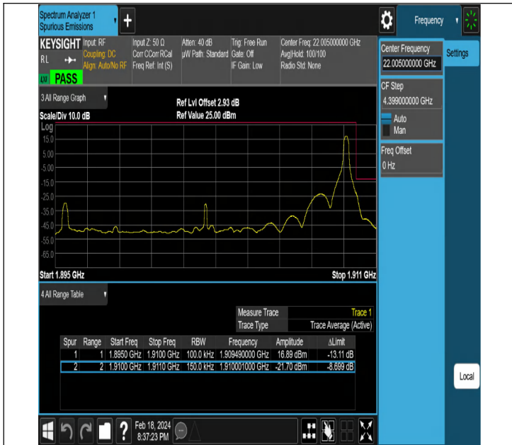
NTNV-DC_5A_n2A-PC3-15-5+15-M+H-QPSK-DFT-PI2BPSK-Edge_1RB_Right-PASS
