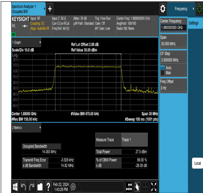
NTNV-DC_5A_n2A-PC3-15-5+15-M+M-N/A-N/A-CP-QPSK-Outer_Full-Ant1-PASS
