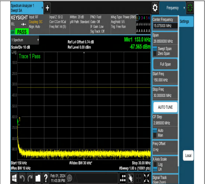
NTNV-N2-PC3-15-20-M-DFT-PI2BPSK-Edge_1RB_Left-Ant1- PASS
