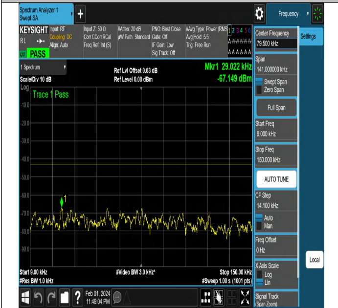
NTNV-N2-PC3-15-20-M-CP-QPSK-Edge_1RB_Right-Ant1-PA SS
