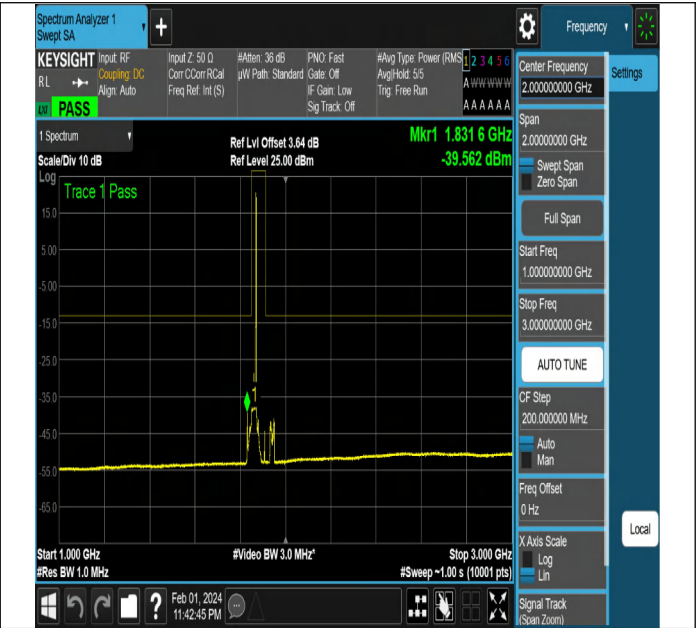
NTNV-N2-PC3-15-20-L-CP-QPSK-Edge_1RB_Right-Ant1-PA
