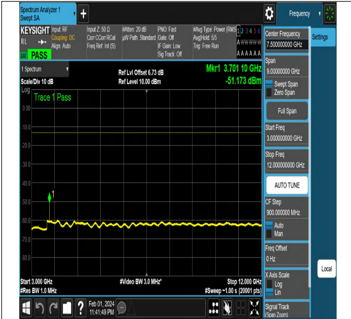
NTNV-N2-PC3-15-20-L-CP-QPSK-Edge_1RB_Left-Ant1-PAS
