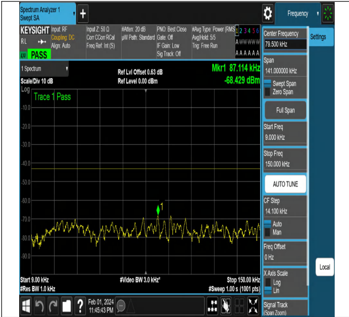
NTNV-N2-PC3-15-20-M-DFT-QPSK-Edge_1RB_Left-Ant1-PA SS
