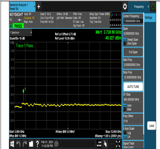
NTNV-N2-PC3-15-20-L-CP-QPSK-Edge_1RB_Right-Ant1-PA
