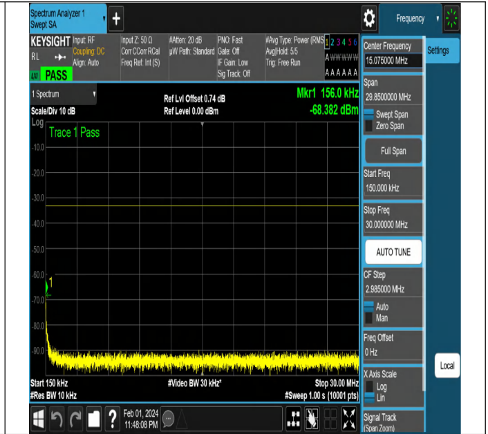
NTNV-N2-PC3-15-20-M-CP-QPSK-Edge_1RB_Left-Ant1-PAS S
