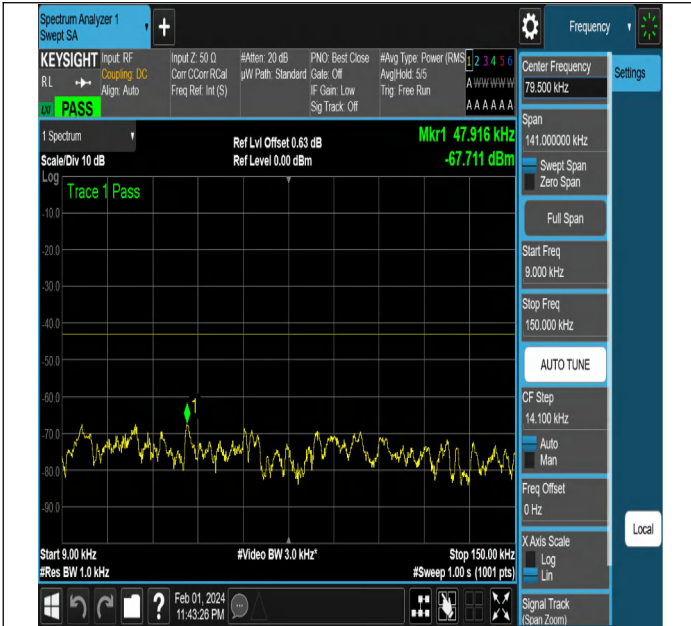
NTNV-N2-PC3-15-20-M-DFT-PI2BPSK-Edge_1RB_Left-Ant1- PASS
