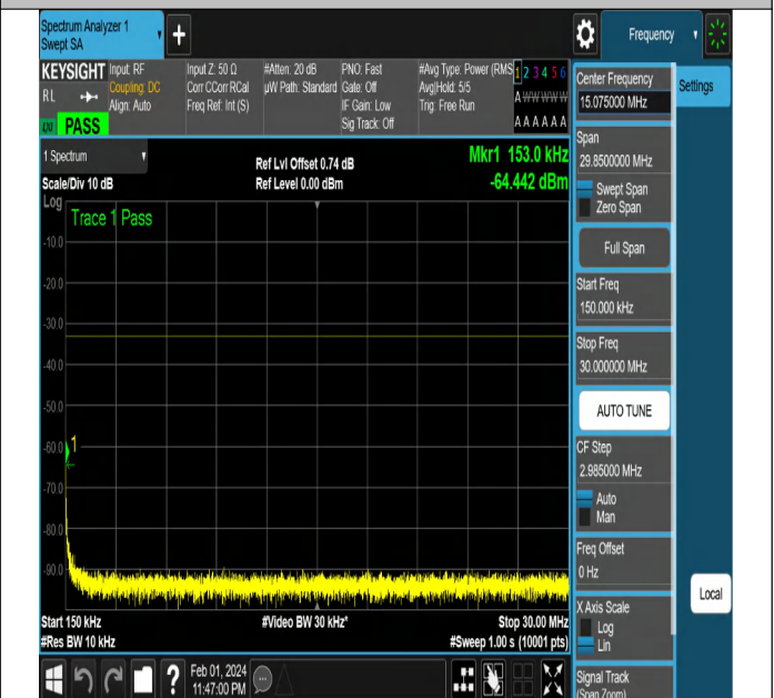
NTNV-N2-PC3-15-20-M-DFT-QPSK-Edge_1RB_Right-Ant1-P
