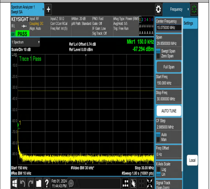
NTNV-N2-PC3-15-20-M-DFT-PI2BPSK-Edge_1RB_Right-Ant
