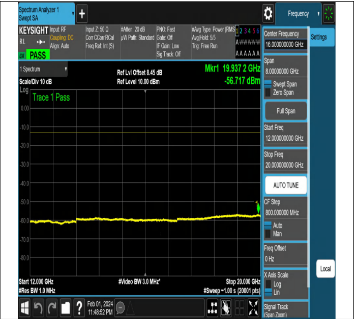
NTNV-N2-PC3-15-20-M-CP-QPSK-Edge_1RB_Left-Ant1-PAS S
