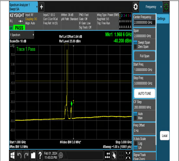
NTNV-N2-PC3-15-20-M-DFT-PI2BPSK-Edge_1RB_Right-Ant
