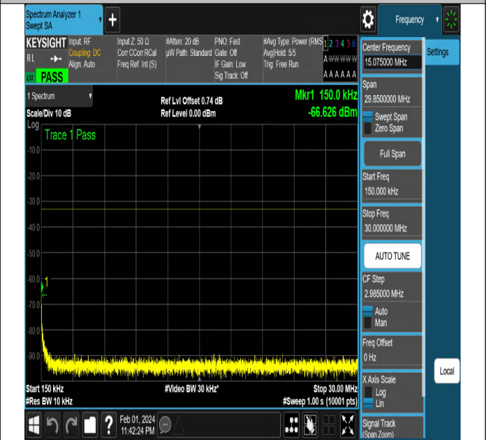
NTNV-N2-PC3-15-20-L-CP-QPSK-Edge_1RB_Right-Ant1-PA
