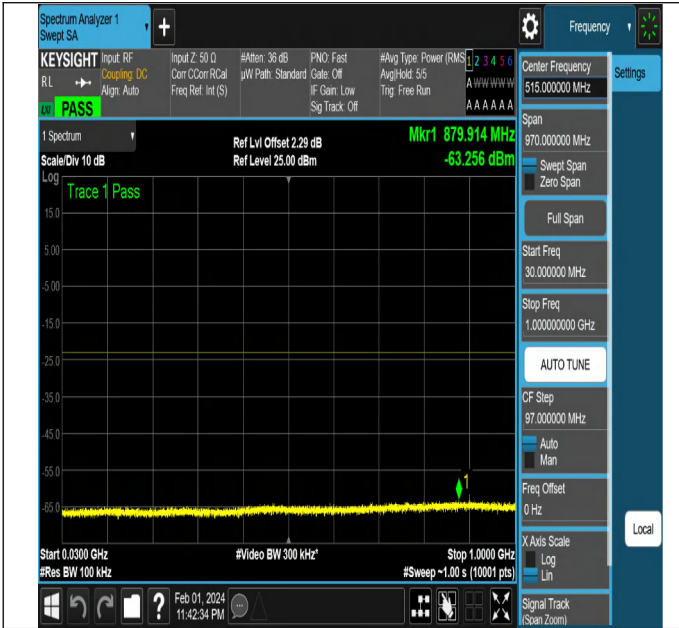
NTNV-N2-PC3-15-20-L-CP-QPSK-Edge_1RB_Right-Ant1-PA
