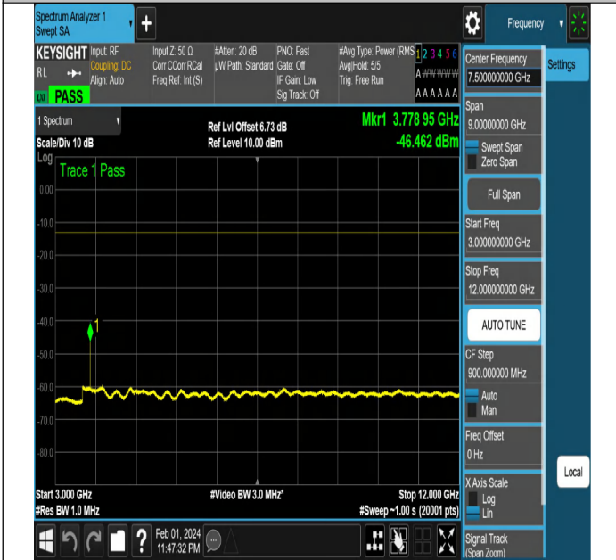
NTNV-N2-PC3-15-20-M-DFT-QPSK-Edge_1RB_Right-Ant1-P ASS
