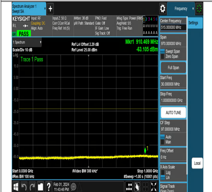
NTNV-N2-PC3-15-20-M-DFT-PI2BPSK-Edge_1RB_Left-Ant1- PASS
