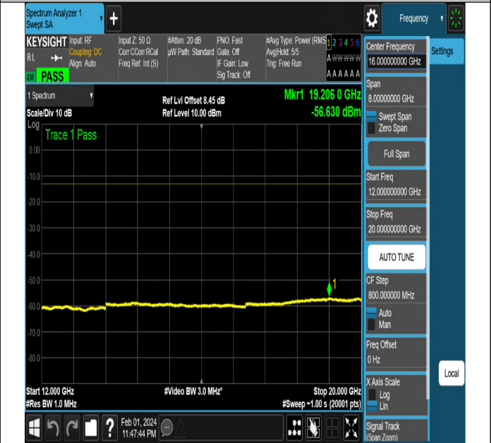
NTNV-N2-PC3-15-20-M-DFT-QPSK-Edge_1RB_Right-Ant1-P ASS
