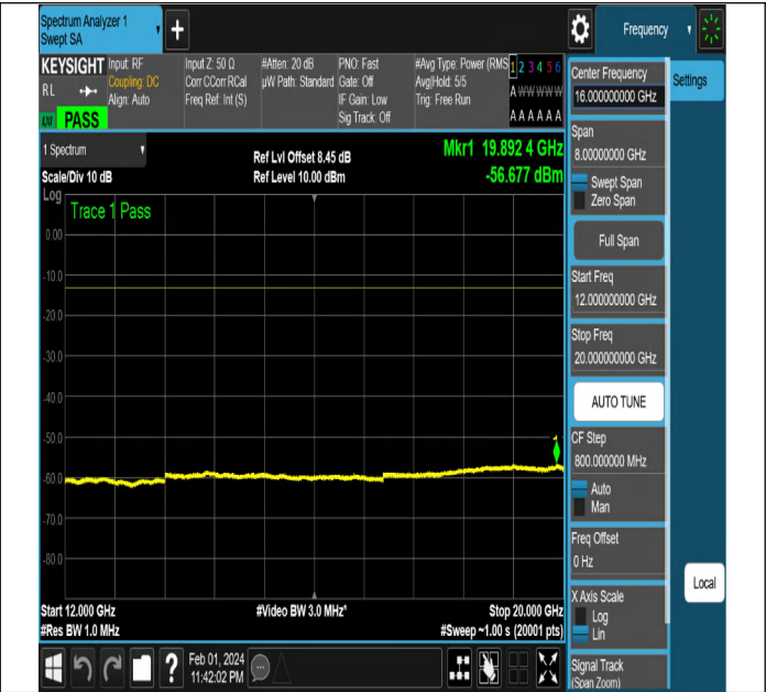
NTNV-N2-PC3-15-20-L-CP-QPSK-Edge_1RB_Left-Ant1-PAS
