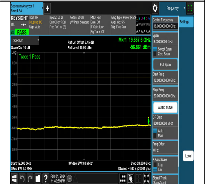
NTNV-N2-PC3-15-20-M-CP-QPSK-Edge_1RB_Right-Ant1-PA SS
