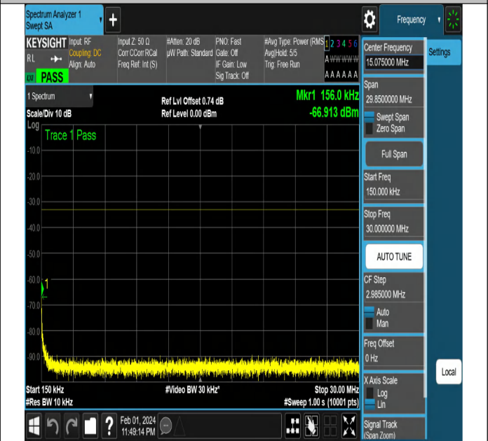
NTNV-N2-PC3-15-20-M-CP-QPSK-Edge_1RB_Right-Ant1-PA SS
