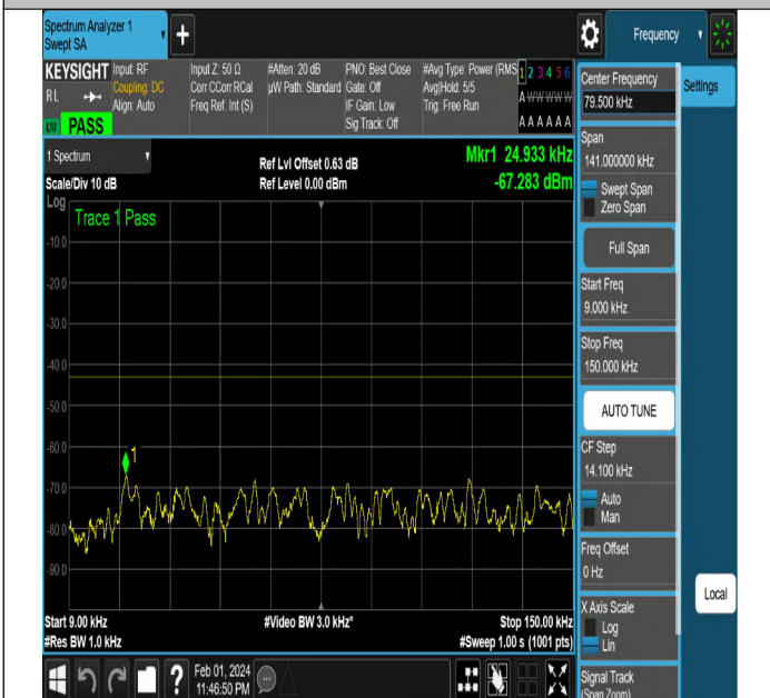
NTNV-N2-PC3-15-20-M-DFT-QPSK-Edge_1RB_Right-Ant1-P
