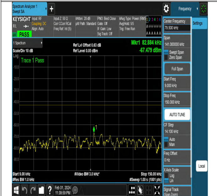
NTNV-N2-PC3-15-20-L-DFT-QPSK-Edge_1RB_Right-Ant1-PA SS
