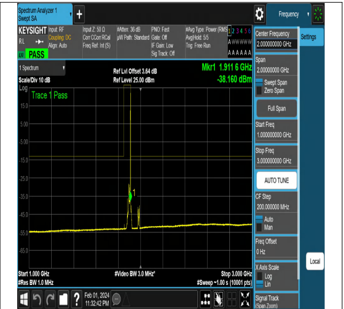
NTNV-N2-PC3-15-15-H-DFT-QPSK-Edge_1RB_Right-Ant1-P
