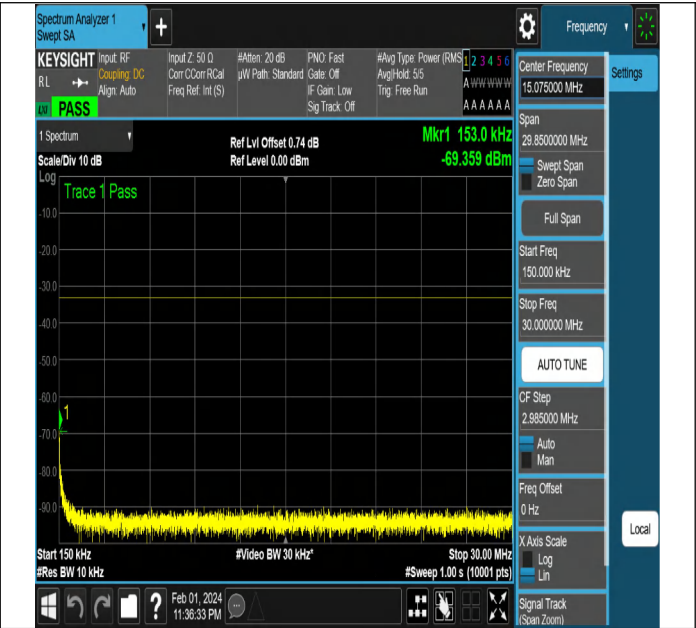
NTNV-N2-PC3-15-20-L-DFT-PI2BPSK-Edge_1RB_Left-Ant1-
