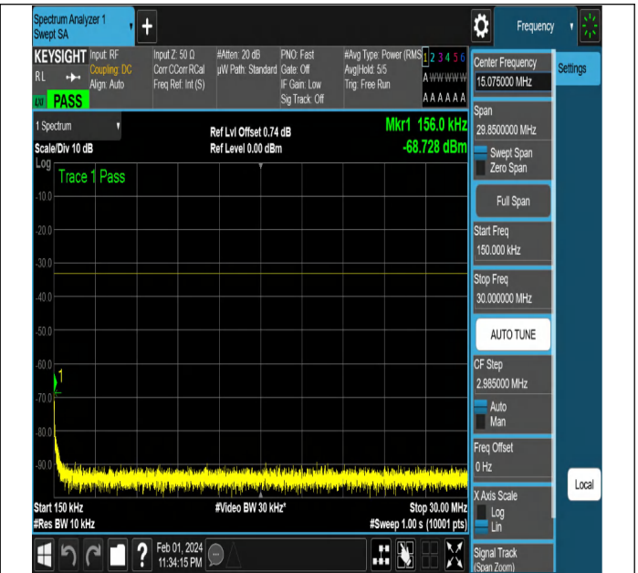
NTNV-N2-PC3-15-15-H-CP-QPSK-Edge_1RB_Left-Ant1-PAS
