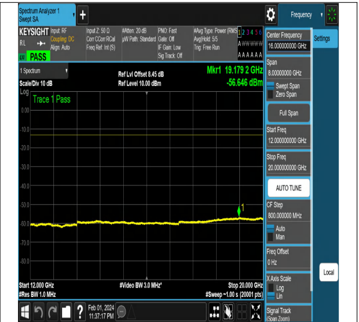
NTNV-N2-PC3-15-20-L-DFT-PI2BPSK-Edge_1RB_Left-Ant1-
