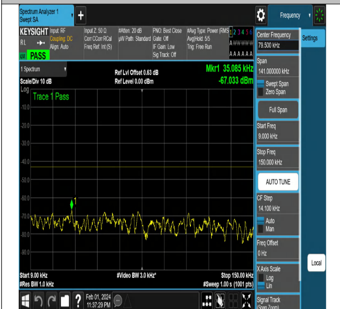
NTNV-N2-PC3-15-20-L-DFT-PI2BPSK-Edge_1RB_Right-Ant1
