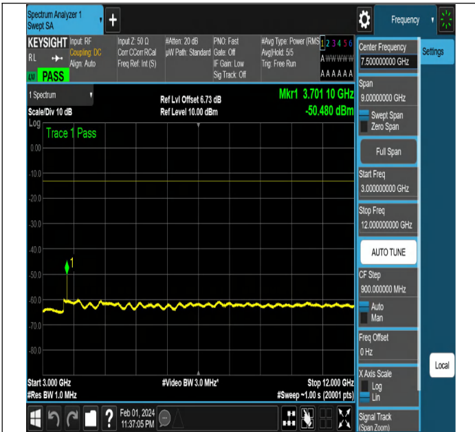
NTNV-N2-PC3-15-20-L-DFT-PI2BPSK-Edge_1RB_Left-Ant1-
