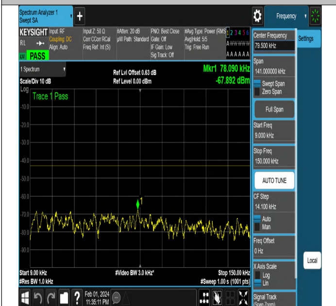
NTNV-N2-PC3-15-15-H-CP-QPSK-Edge_1RB_Right-Ant1-PA SS
