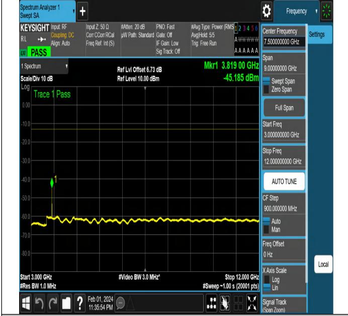
NTNV-N2-PC3-15-15-H-CP-QPSK-Edge_1RB_Right-Ant1-PA SS
