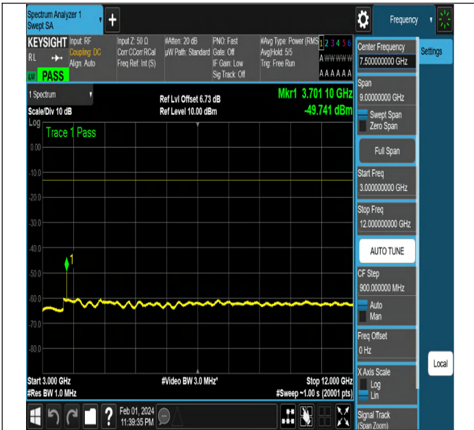
NTNV-N2-PC3-15-20-L-DFT-QPSK-Edge_1RB_Left-Ant1-PAS S
