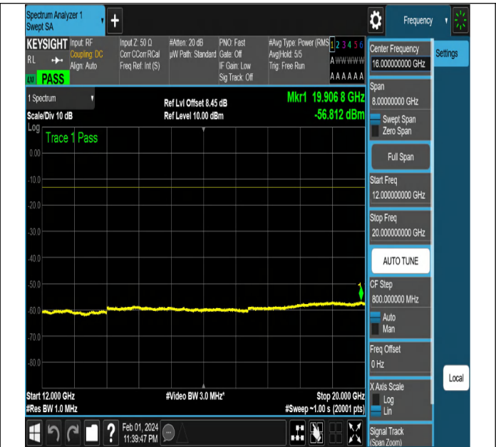
NTNV-N2-PC3-15-20-L-DFT-QPSK-Edge_1RB_Left-Ant1-PAS S
