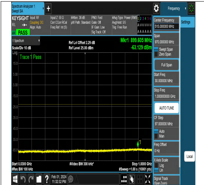
NTNV-N2-PC3-15-15-H-DFT-QPSK-Edge_1RB_Right-Ant1-P
