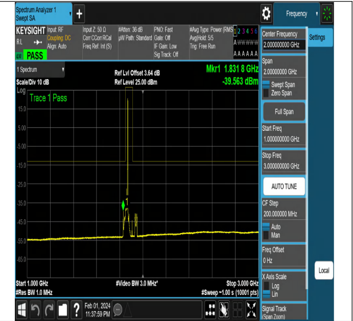
NTNV-N2-PC3-15-20-L-DFT-PI2BPSK-Edge_1RB_Right-Ant1 -PASS
