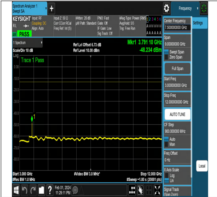
NTNV-N2-PC3-15-15-H-DFT-PI2BPSK-Edge_1RB_Left-Ant1-
