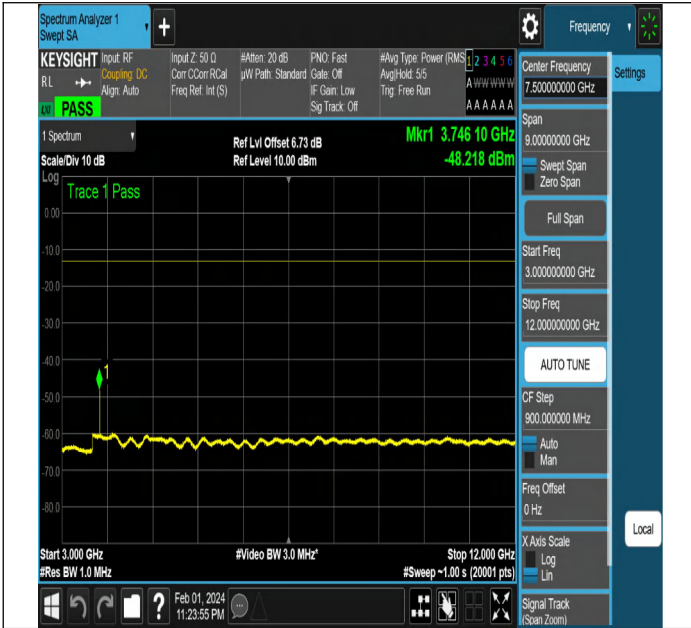
NTNV-N2-PC3-15-15-M-DFT-QPSK-Edge_1RB_Left-Ant1-PA
