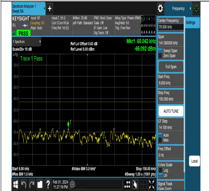
NTNV-N2-PC3-15-15-M-CP-QPSK-Edge_1RB_Right-Ant1-PA SS
