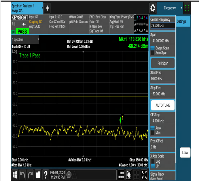
NTNV-N2-PC3-15-15-H-DFT-PI2BPSK-Edge_1RB_Right-Ant1
