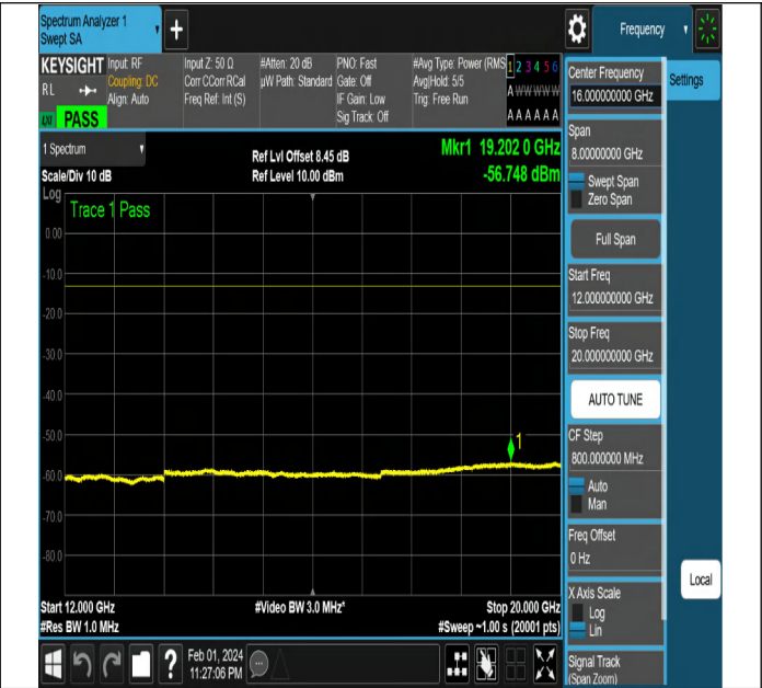
NTNV-N2-PC3-15-15-M-CP-QPSK-Edge_1RB_Left-Ant1-PAS S
