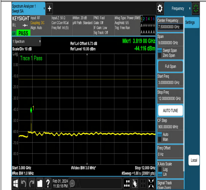
NTNV-N2-PC3-15-15-H-DFT-PI2BPSK-Edge_1RB_Right-Ant1 -PASS
