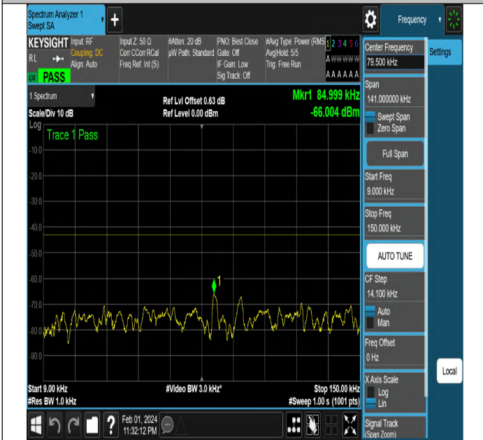
NTNV-N2-PC3-15-15-H-DFT-QPSK-Edge_1RB_Right-Ant1-P
