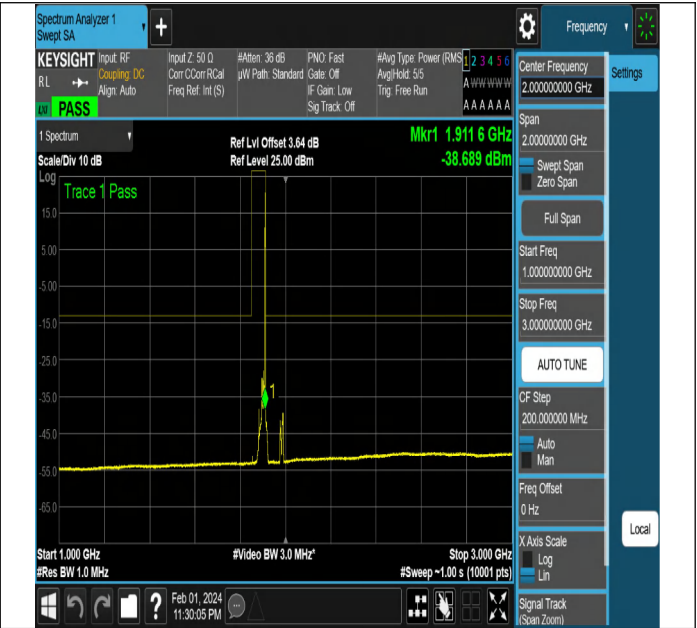
NTNV-N2-PC3-15-15-H-DFT-PI2BPSK-Edge_1RB_Right-Ant1 -PASS
