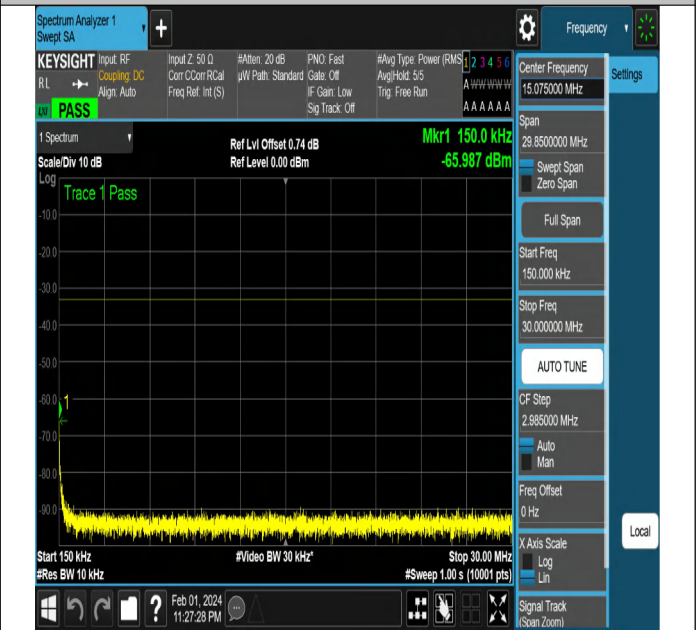
NTNV-N2-PC3-15-15-M-CP-QPSK-Edge_1RB_Right-Ant1-PA SS
