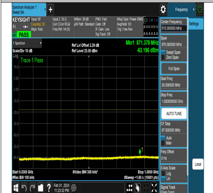
NTNV-N2-PC3-15-15-M-DFT-QPSK-Edge_1RB_Left-Ant1-PA SS
