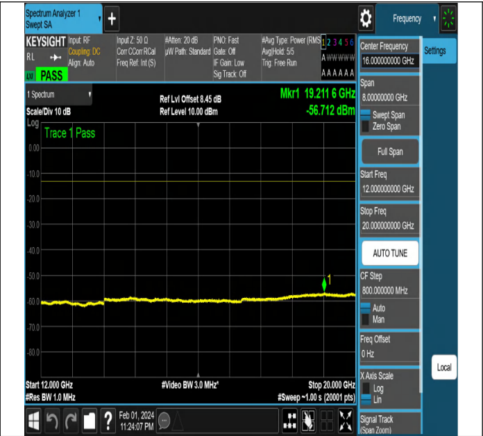
NTNV-N2-PC3-15-15-M-DFT-QPSK-Edge_1RB_Left-Ant1-PA
