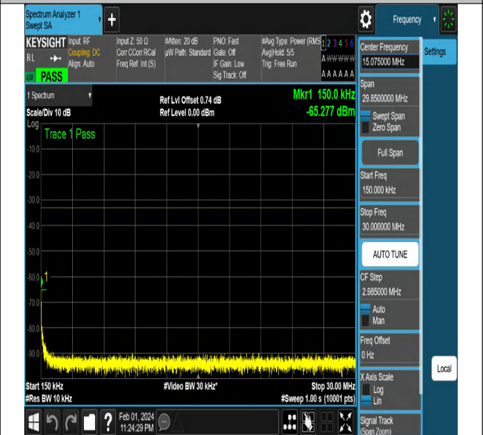
NTNV-N2-PC3-15-15-M-DFT-QPSK-Edge_1RB_Right-Ant1-P
