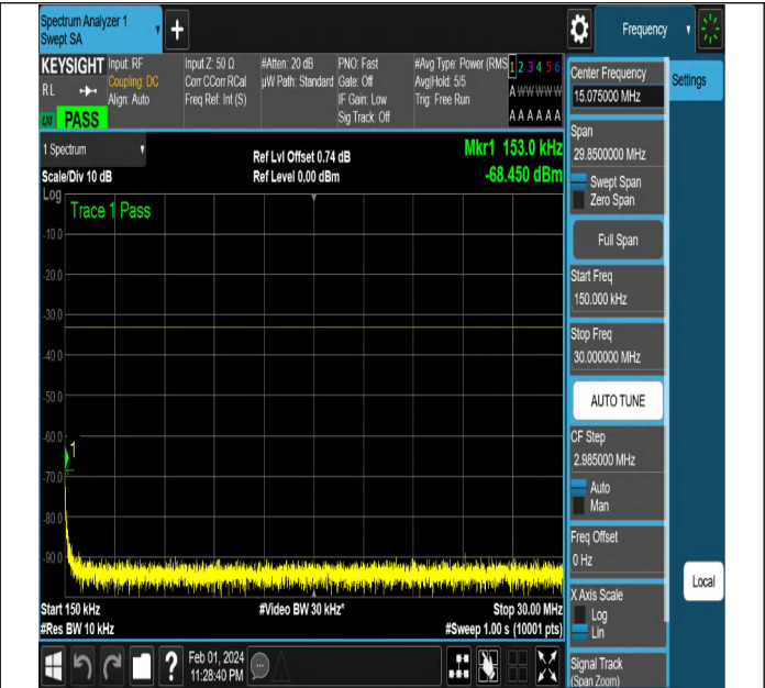
NTNV-N2-PC3-15-15-H-DFT-PI2BPSK-Edge_1RB_Left-Ant1- PASS
