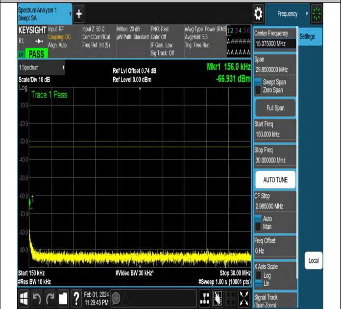
NTNV-N2-PC3-15-15-H-DFT-PI2BPSK-Edge_1RB_Right-Ant1
