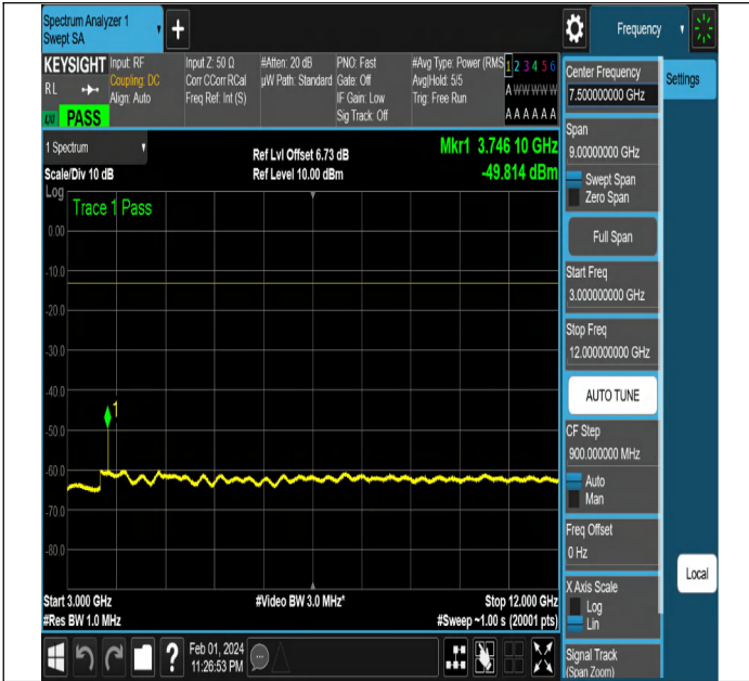
NTNV-N2-PC3-15-15-M-CP-QPSK-Edge_1RB_Left-Ant1-PAS S
