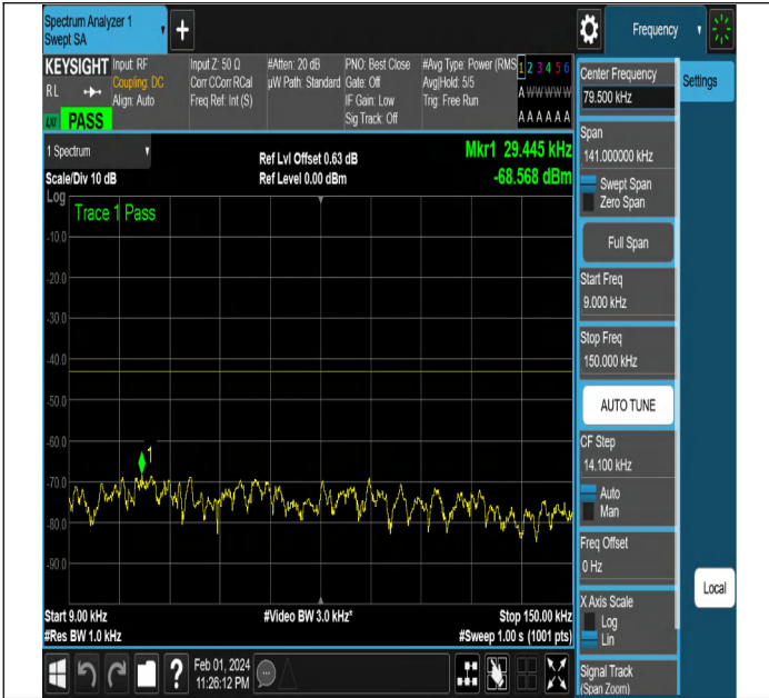
NTNV-N2-PC3-15-15-M-CP-QPSK-Edge_1RB_Left-Ant1-PAS
