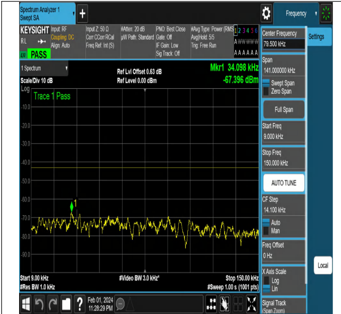
NTNV-N2-PC3-15-15-H-DFT-PI2BPSK-Edge_1RB_Left-Ant1- PASS
