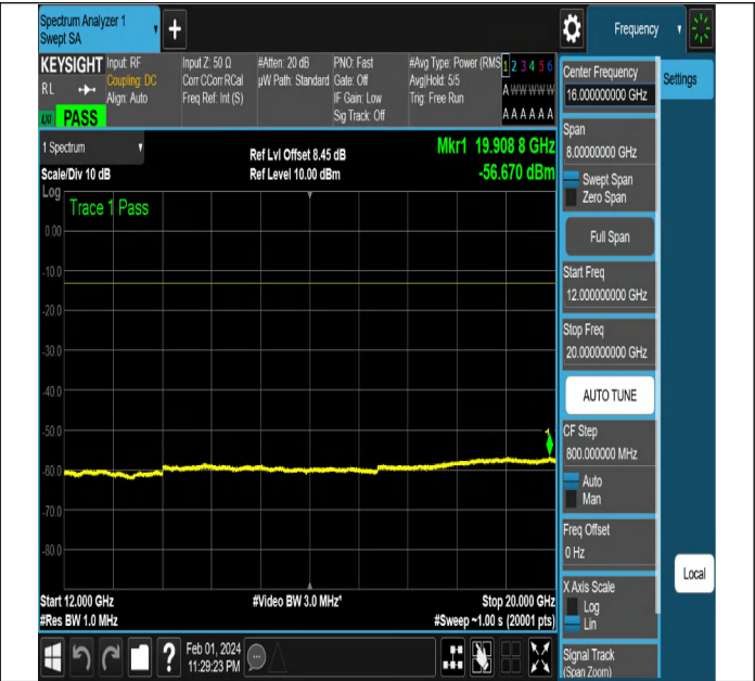
NTNV-N2-PC3-15-15-H-DFT-PI2BPSK-Edge_1RB_Left-Ant1-
