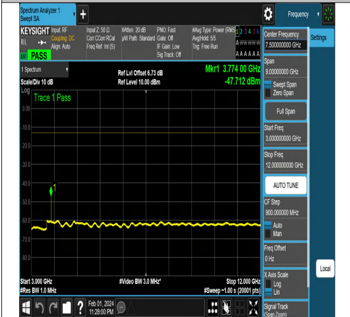
NTNV-N2-PC3-15-15-M-CP-QPSK-Edge_1RB_Right-Ant1-PA SS
