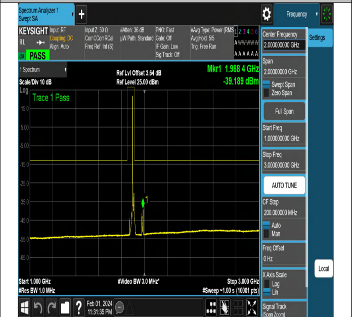
NTNV-N2-PC3-15-15-H-DFT-QPSK-Edge_1RB_Left-Ant1-PA
