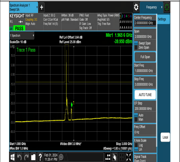
NTNV-N2-PC3-15-15-M-CP-QPSK-Edge_1RB_Left-Ant1-PAS
