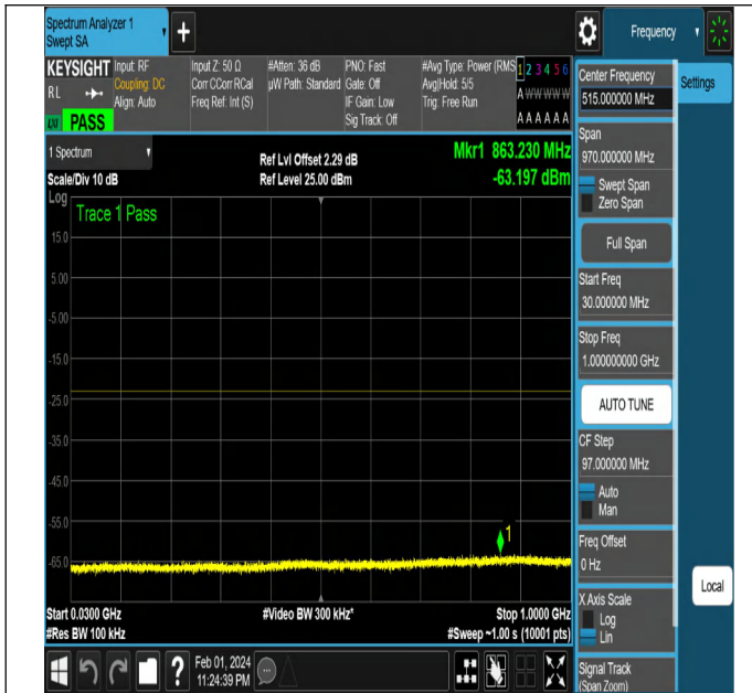
NTNV-N2-PC3-15-15-M-DFT-QPSK-Edge_1RB_Right-Ant1-P ASS
