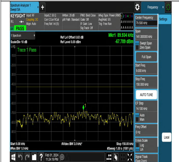
NTNV-N2-PC3-15-15-M-DFT-QPSK-Edge_1RB_Right-Ant1-P
