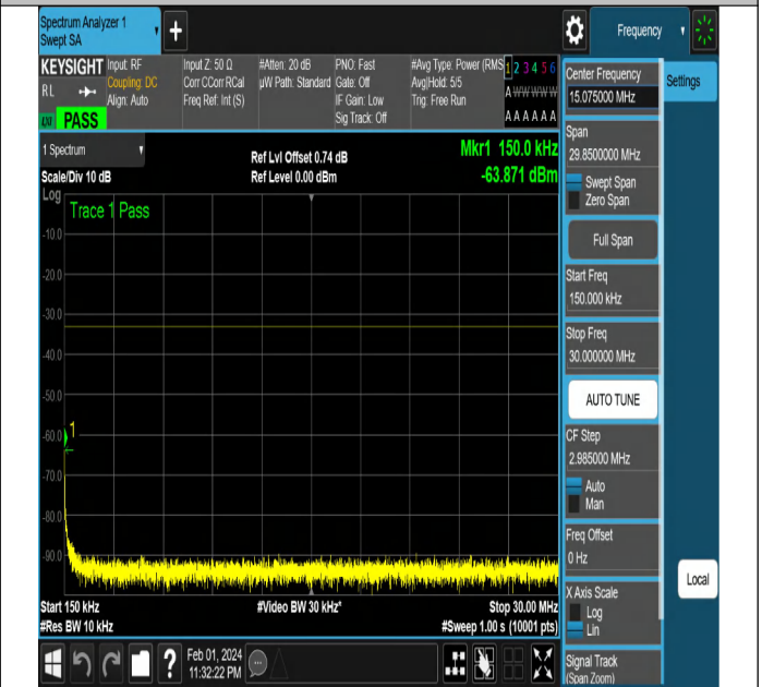
NTNV-N2-PC3-15-15-H-DFT-QPSK-Edge_1RB_Right-Ant1-P
