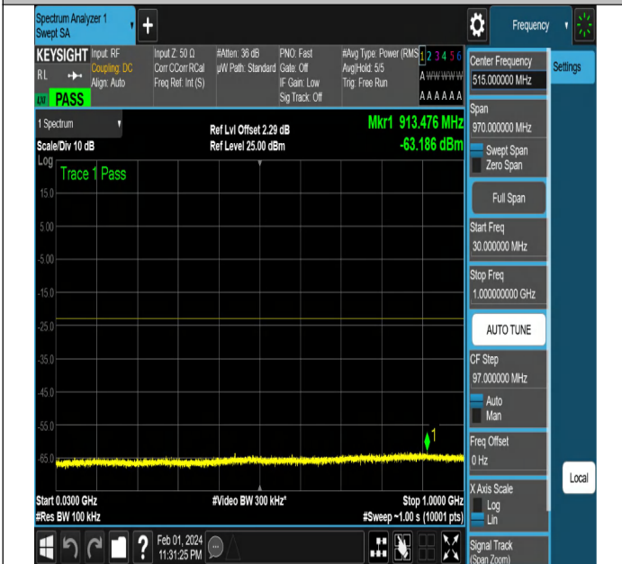
NTNV-N2-PC3-15-15-H-DFT-QPSK-Edge_1RB_Left-Ant1-PA
