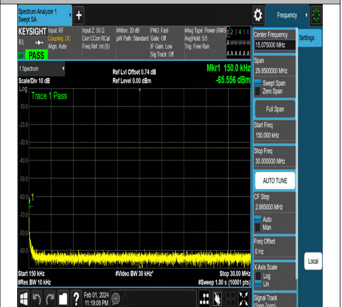
NTNV-N2-PC3-15-15-L-CP-QPSK-Edge_1RB_Right-Ant1-PA
