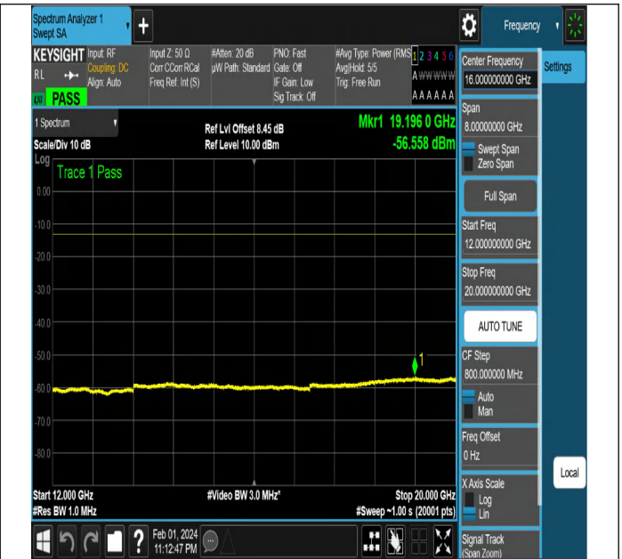
NTNV-N2-PC3-15-15-L-DFT-PI2BPSK-Edge_1RB_Left-Ant1- PASS
