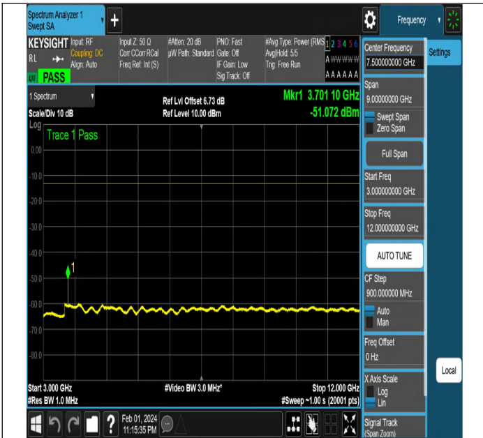
NTNV-N2-PC3-15-15-L-DFT-QPSK-Edge_1RB_Left-Ant1-PAS
