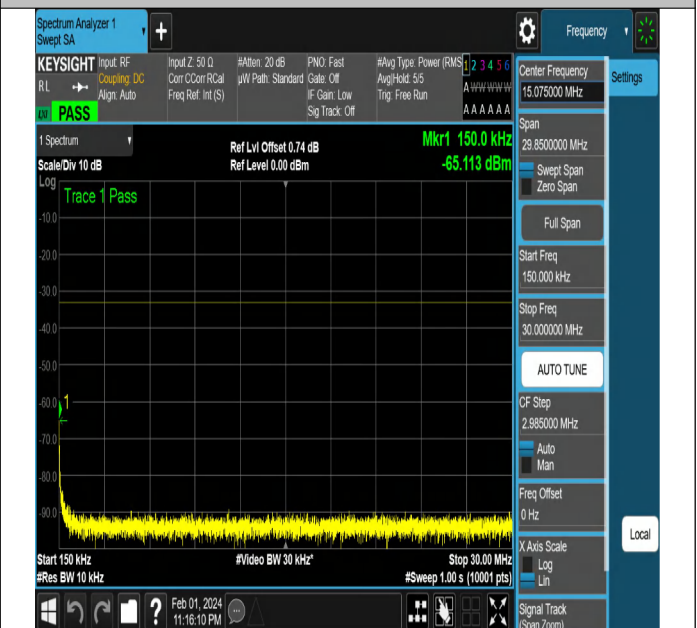
NTNV-N2-PC3-15-15-L-DFT-QPSK-Edge_1RB_Right-Ant1-PA
