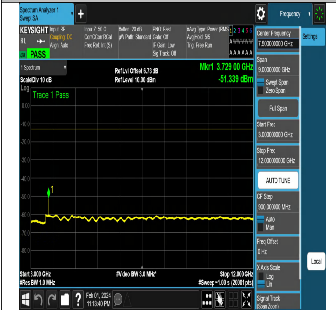
NTNV-N2-PC3-15-15-L-DFT-PI2BPSK-Edge_1RB_Right-Ant1
