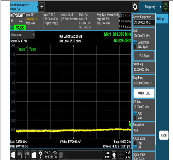
NTNV-N2-PC3-15-15-L-CP-QPSK-Edge_1RB_Right-Ant1-PA
