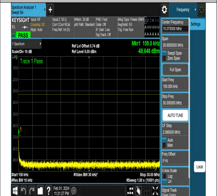
NTNV-N2-PC3-15-15-M-DFT-PI2BPSK-Edge_1RB_Right-Ant
