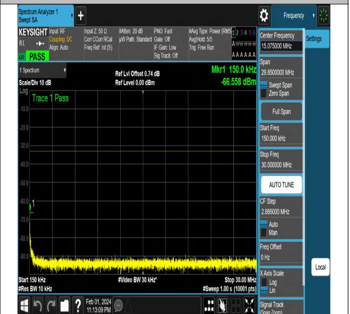
NTNV-N2-PC3-15-15-L-DFT-PI2BPSK-Edge_1RB_Right-Ant1 -PASS
