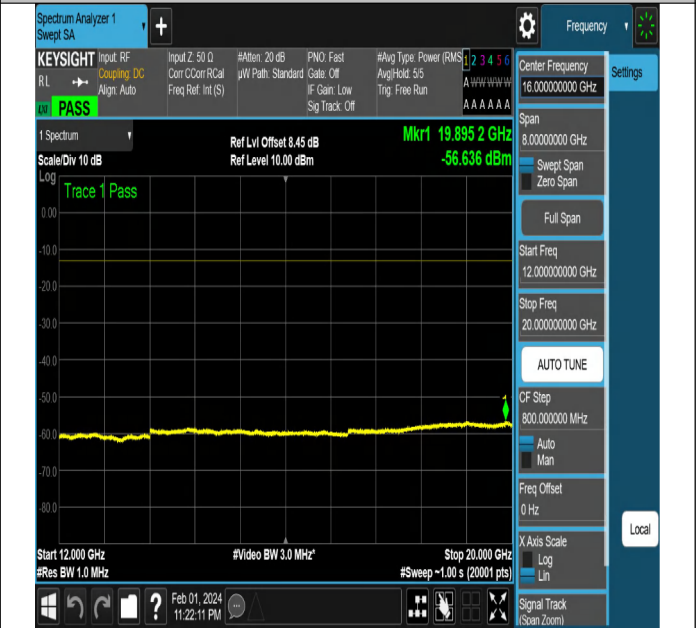
NTNV-N2-PC3-15-15-M-DFT-PI2BPSK-Edge_1RB_Right-Ant 1-PASS
