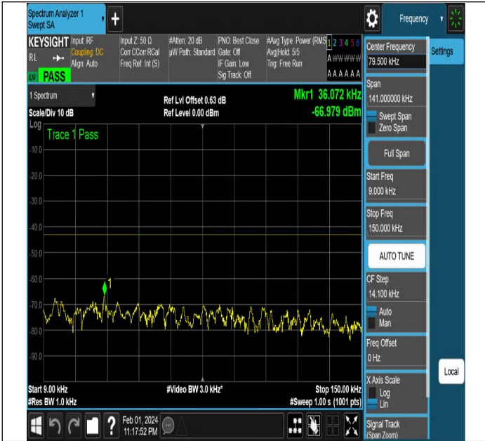
NTNV-N2-PC3-15-15-L-CP-QPSK-Edge_1RB_Left-Ant1-PAS
