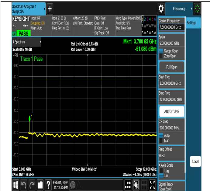
NTNV-N2-PC3-15-15-L-DFT-PI2BPSK-Edge_1RB_Left-Ant1- PASS
