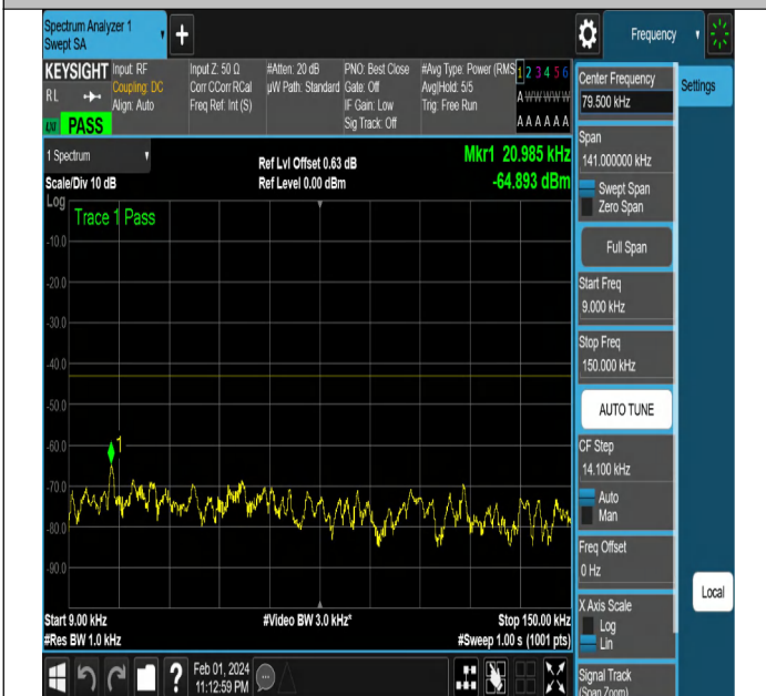
NTNV-N2-PC3-15-15-L-DFT-PI2BPSK-Edge_1RB_Right-Ant1 -PASS
