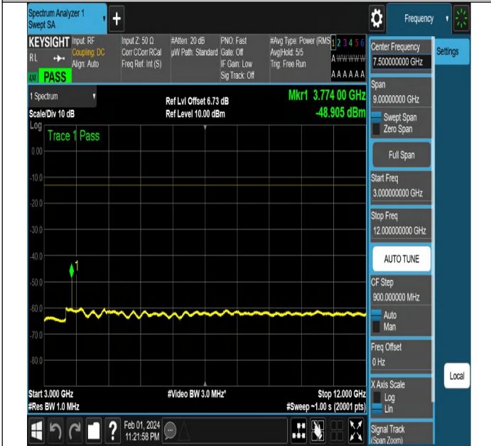
NTNV-N2-PC3-15-15-M-DFT-PI2BPSK-Edge_1RB_Right-Ant 1-PASS
