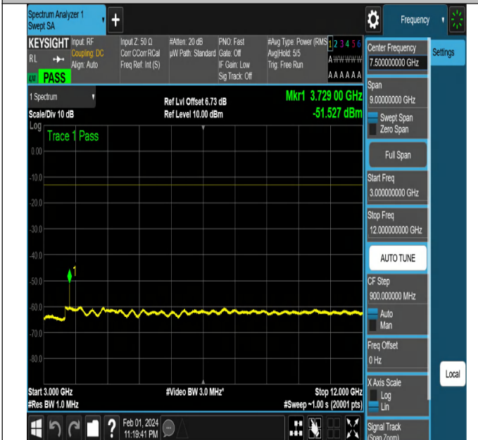
NTNV-N2-PC3-15-15-L-CP-QPSK-Edge_1RB_Right-Ant1-PA
