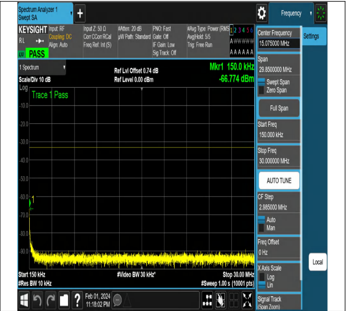
NTNV-N2-PC3-15-15-L-CP-QPSK-Edge_1RB_Left-Ant1-PAS
