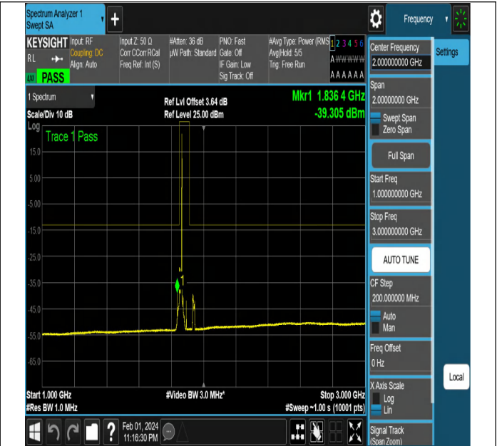
NTNV-N2-PC3-15-15-L-DFT-QPSK-Edge_1RB_Right-Ant1-PA SS
