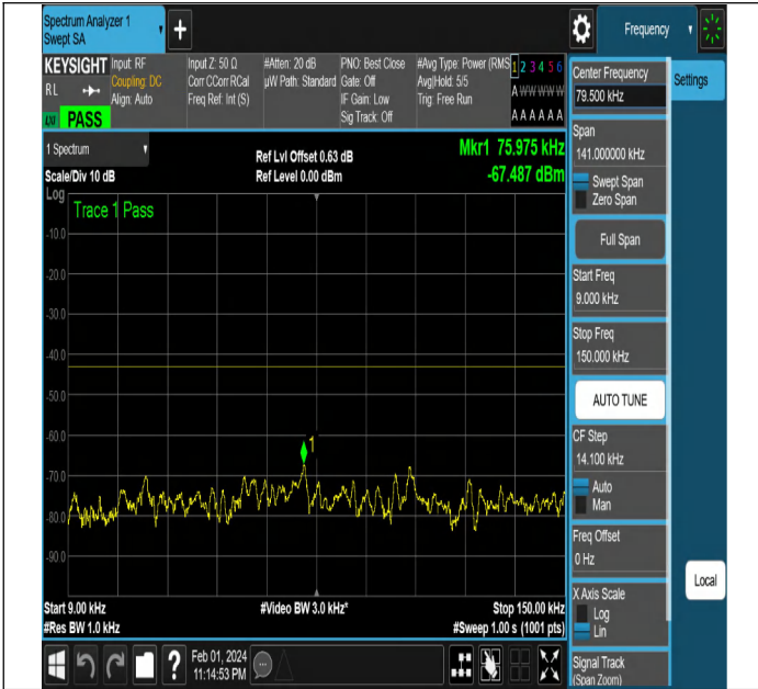
NTNV-N2-PC3-15-15-L-DFT-QPSK-Edge_1RB_Left-Ant1-PAS S
