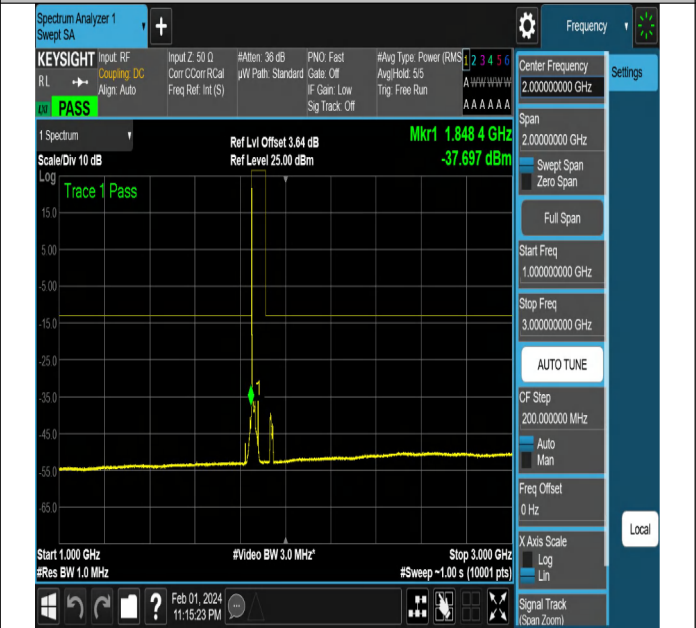
NTNV-N2-PC3-15-15-L-DFT-QPSK-Edge_1RB_Left-Ant1-PAS S
