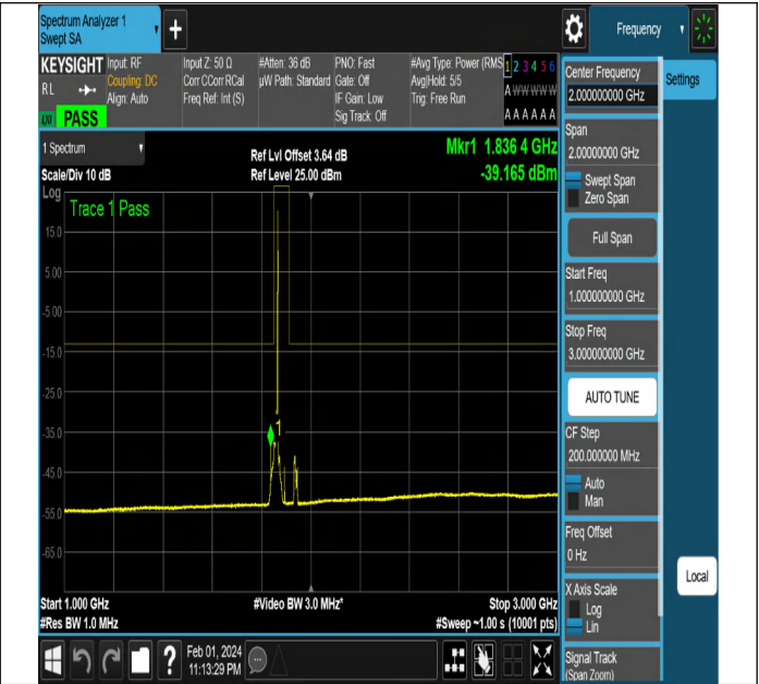
NTNV-N2-PC3-15-15-L-DFT-PI2BPSK-Edge_1RB_Right-Ant1
