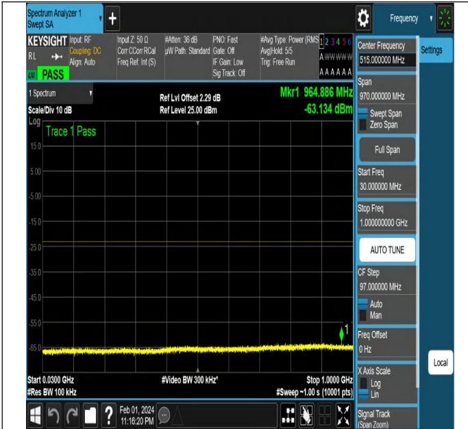
NTNV-N2-PC3-15-15-L-DFT-QPSK-Edge_1RB_Right-Ant1-PA SS
