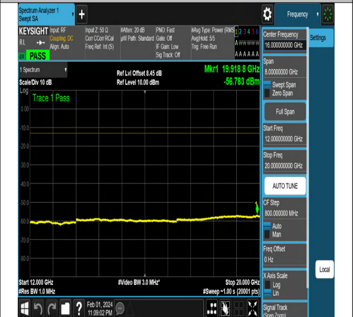
NTNV-N2-PC3-15-10-H-DFT-QPSK-Edge_1RB_Right-Ant1-P
