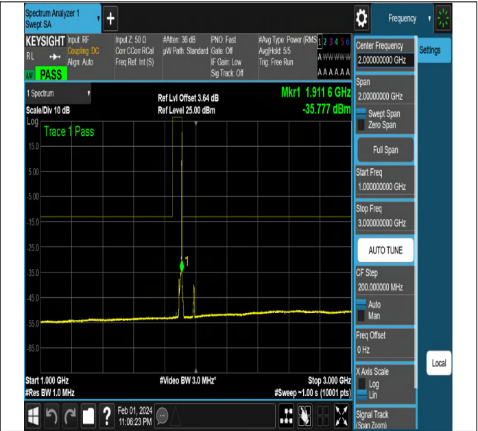
NTNV-N2-PC3-15-10-H-DFT-PI2BPSK-Edge_1RB_Right-Ant1 -PASS
