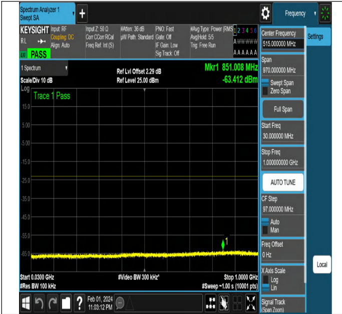
NTNV-N2-PC3-15-10-M-CP-QPSK-Edge_1RB_Right-Ant1-PA
