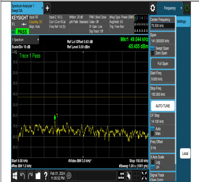
NTNV-N2-PC3-15-10-H-DFT-PI2BPSK-Edge_1RB_Right-Ant1
