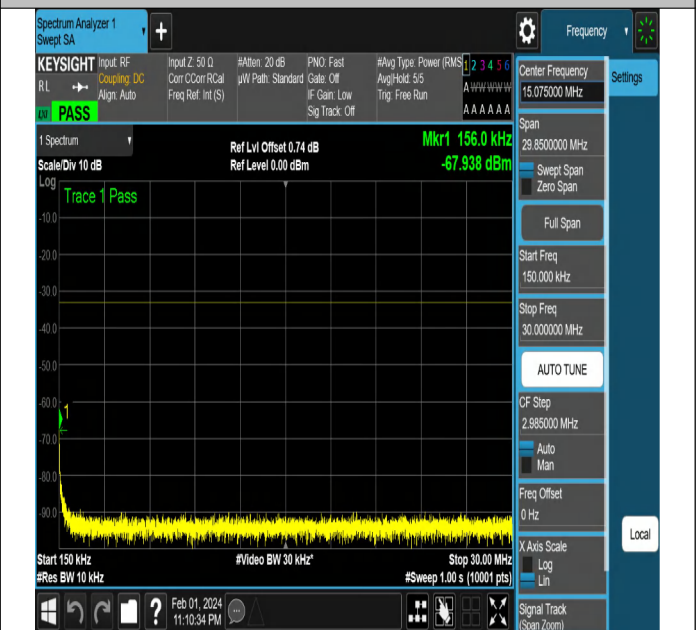
NTNV-N2-PC3-15-10-H-CP-QPSK-Edge_1RB_Right-Ant1-PA
