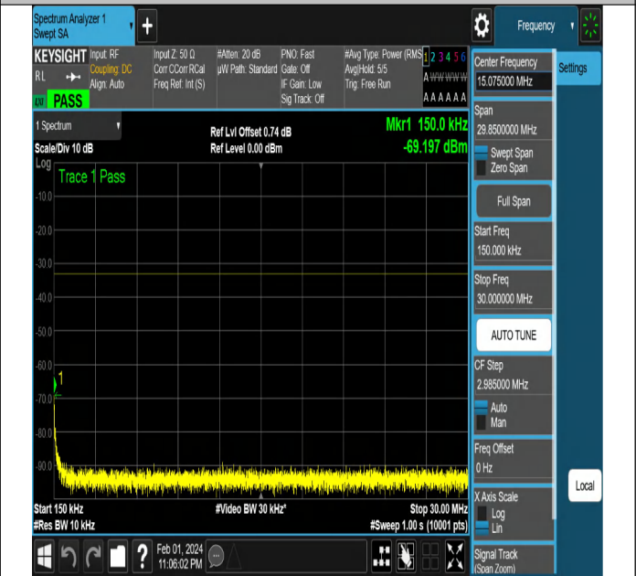
NTNV-N2-PC3-15-10-H-DFT-PI2BPSK-Edge_1RB_Right-Ant1
