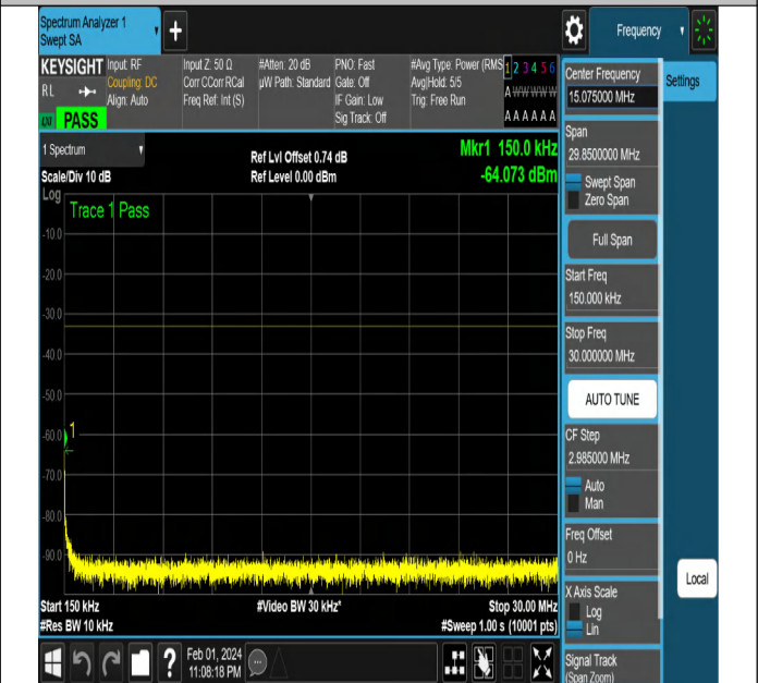
NTNV-N2-PC3-15-10-H-DFT-QPSK-Edge_1RB_Right-Ant1-P
