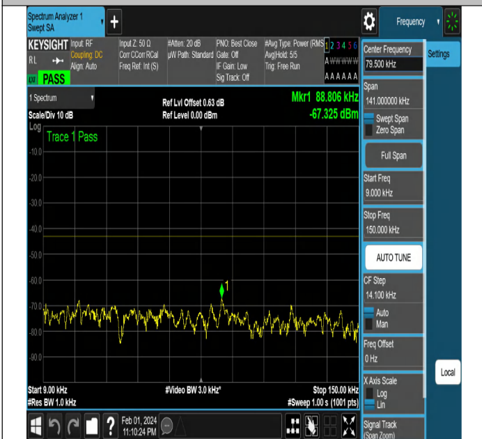
NTNV-N2-PC3-15-10-H-CP-QPSK-Edge_1RB_Right-Ant1-PA
