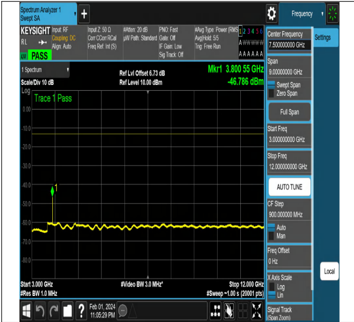
NTNV-N2-PC3-15-10-H-DFT-PI2BPSK-Edge_1RB_Left-Ant1-
