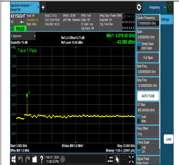
NTNV-N2-PC3-15-10-H-DFT-PI2BPSK-Edge_1RB_Right-Ant1 -PASS
