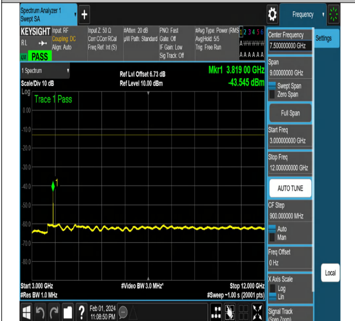
NTNV-N2-PC3-15-10-H-DFT-QPSK-Edge_1RB_Right-Ant1-P
