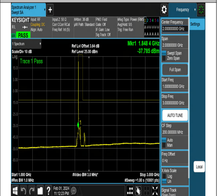
NTNV-N2-PC3-15-15-L-DFT-PI2BPSK-Edge_1RB_Left-Ant1-
