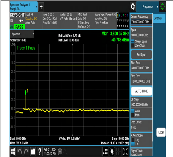
NTNV-N2-PC3-15-10-H-DFT-QPSK-Edge_1RB_Left-Ant1-PA
