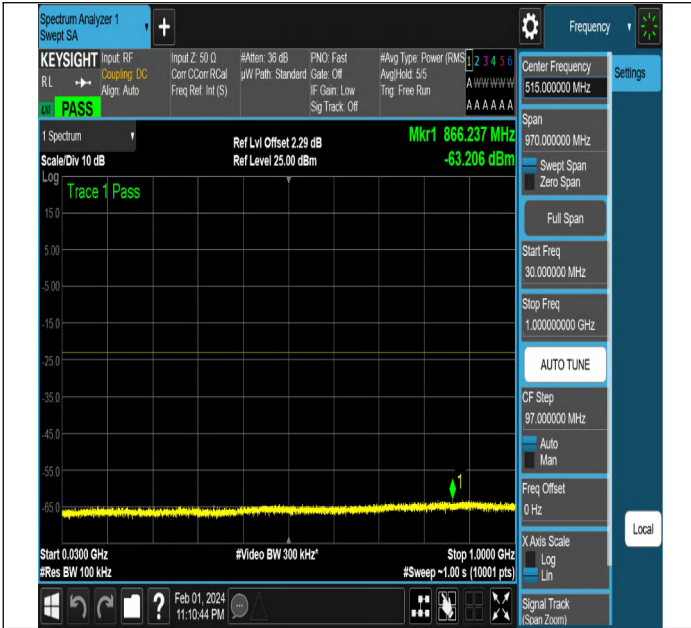
NTNV-N2-PC3-15-10-H-CP-QPSK-Edge_1RB_Right-Ant1-PA SS
