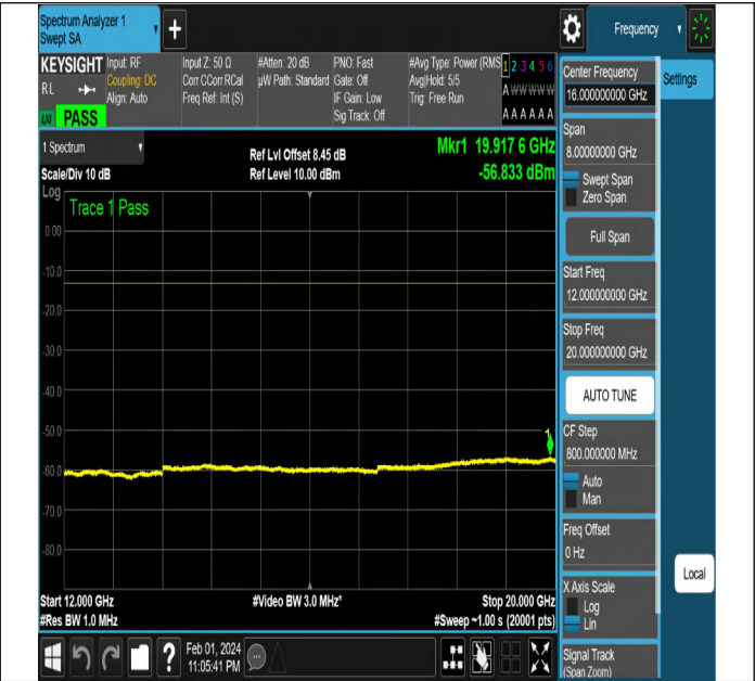
NTNV-N2-PC3-15-10-H-DFT-PI2BPSK-Edge_1RB_Left-Ant1-
