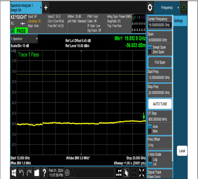
NTNV-N2-PC3-15-10-H-DFT-QPSK-Edge_1RB_Left-Ant1-PA
