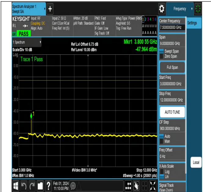
NTNV-N2-PC3-15-10-H-CP-QPSK-Edge_1RB_Left-Ant1-PAS
