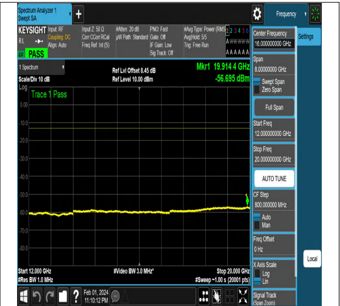
NTNV-N2-PC3-15-10-H-CP-QPSK-Edge_1RB_Left-Ant1-PAS
