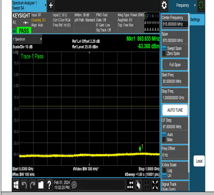
NTNV-N2-PC3-15-10-L-DFT-QPSK-Edge_1RB_Left-Ant1-PAS S
