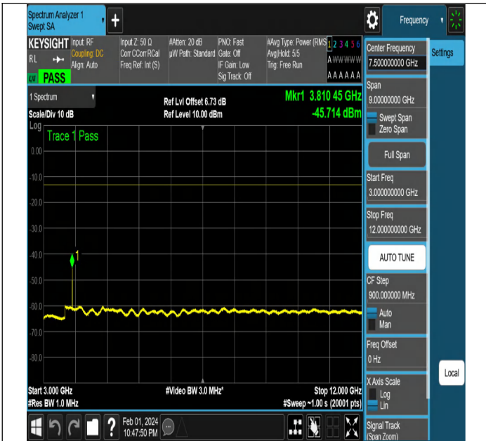
NTNV-N2-PC3-15-5-H-CP-QPSK-Edge_1RB_Left-Ant1-PASS
