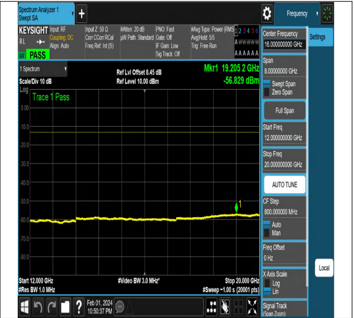
NTNV-N2-PC3-15-10-L-DFT-PI2BPSK-Edge_1RB_Left-Ant1-
