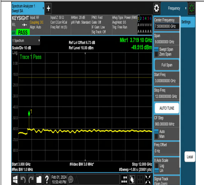
NTNV-N2-PC3-15-10-L-DFT-QPSK-Edge_1RB_Right-Ant1-PA
