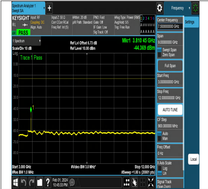
NTNV-N2-PC3-15-5-H-DFT-QPSK-Edge_1RB_Left-Ant1-PAS
