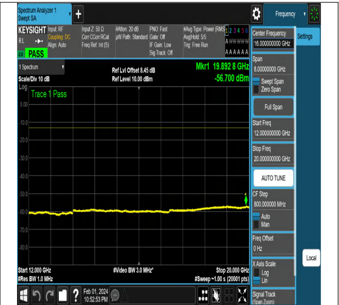
NTNV-N2-PC3-15-10-L-DFT-QPSK-Edge_1RB_Left-Ant1-PAS
