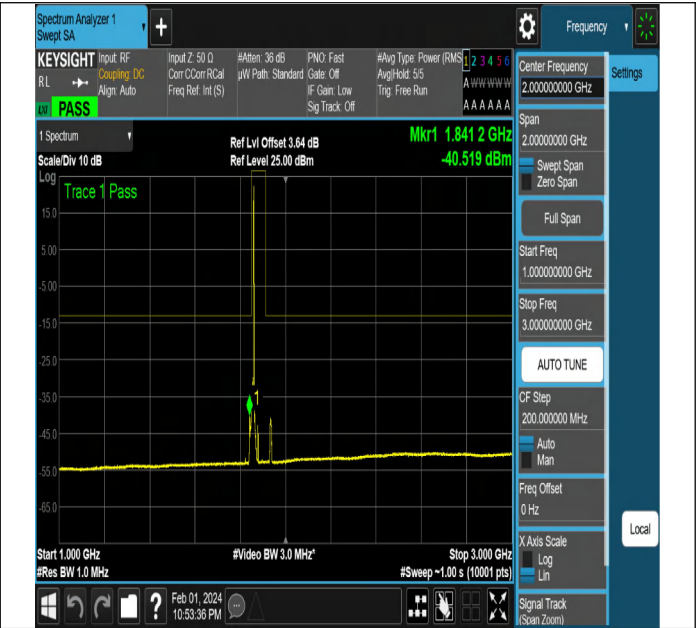
NTNV-N2-PC3-15-10-L-DFT-QPSK-Edge_1RB_Right-Ant1-PA
