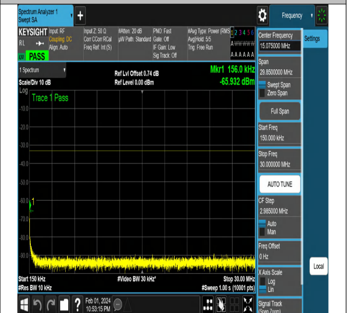
NTNV-N2-PC3-15-10-L-DFT-QPSK-Edge_1RB_Right-Ant1-PA
