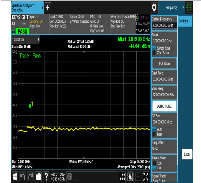
NTNV-N2-PC3-15-5-H-DFT-QPSK-Edge_1RB_Right-Ant1-PA SS
