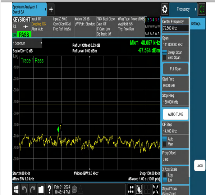
NTNV-N2-PC3-15-5-H-CP-QPSK-Edge_1RB_Right-Ant1-PAS
