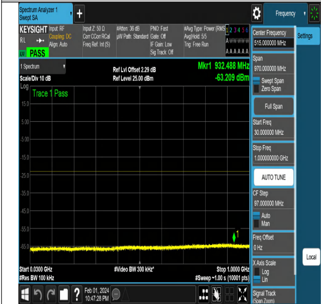
NTNV-N2-PC3-15-5-H-CP-QPSK-Edge_1RB_Left-Ant1-PASS
