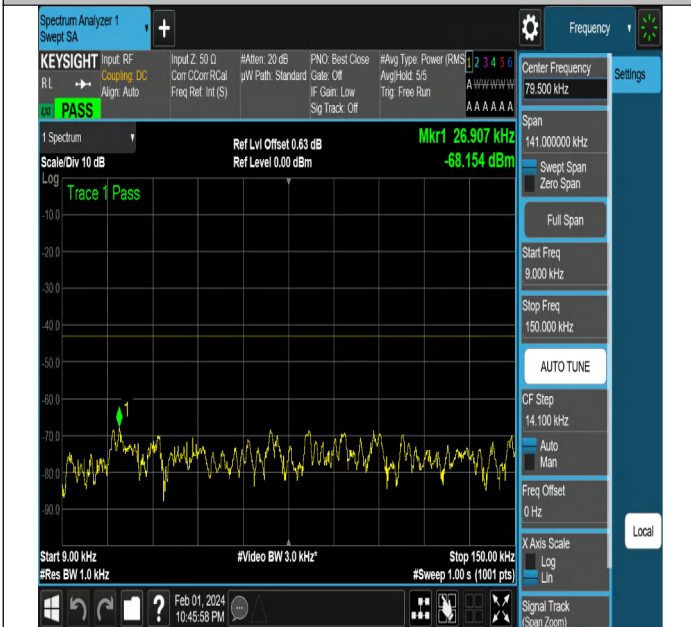
NTNV-N2-PC3-15-5-H-DFT-QPSK-Edge_1RB_Right-Ant1-PA
