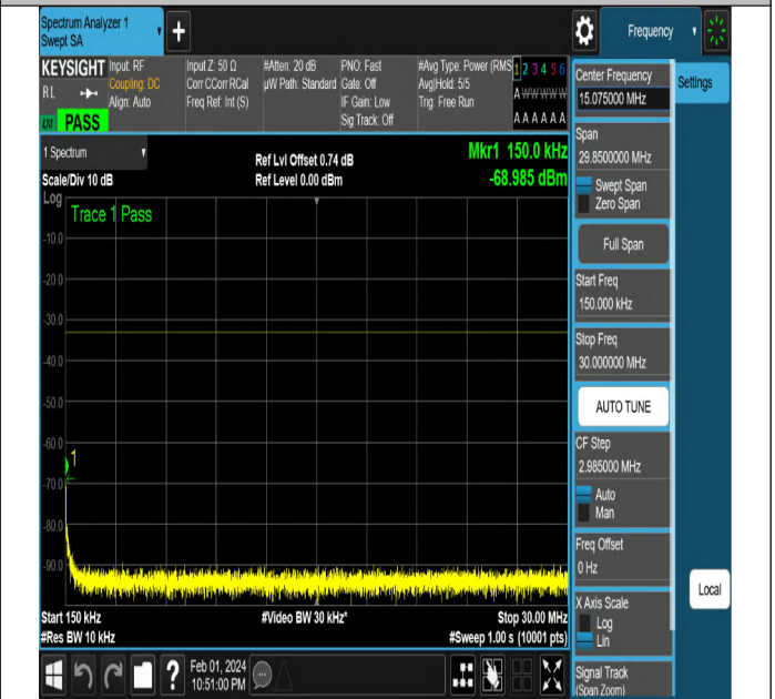
NTNV-N2-PC3-15-10-L-DFT-PI2BPSK-Edge_1RB_Right-Ant1
