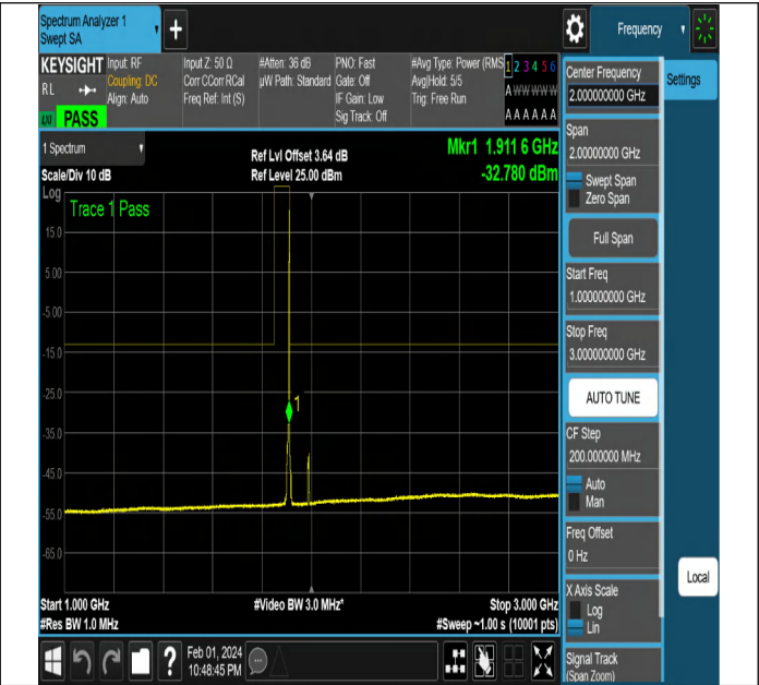
NTNV-N2-PC3-15-5-H-CP-QPSK-Edge_1RB_Right-Ant1-PAS S
