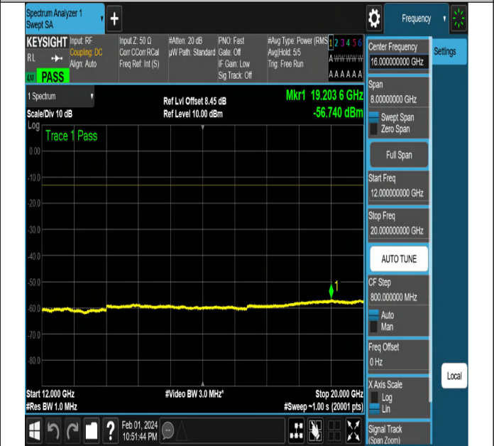
NTNV-N2-PC3-15-10-L-DFT-PI2BPSK-Edge_1RB_Right-Ant1 -PASS
