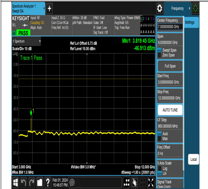
NTNV-N2-PC3-15-5-H-CP-QPSK-Edge_1RB_Right-Ant1-PAS S
