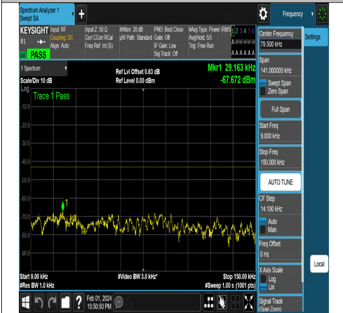
NTNV-N2-PC3-15-10-L-DFT-PI2BPSK-Edge_1RB_Right-Ant1
