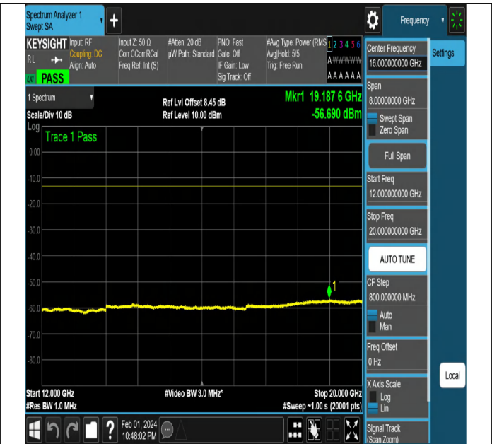
NTNV-N2-PC3-15-5-H-CP-QPSK-Edge_1RB_Left-Ant1-PASS
