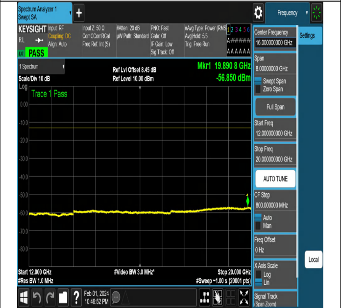
NTNV-N2-PC3-15-5-H-DFT-QPSK-Edge_1RB_Right-Ant1-PA SS
