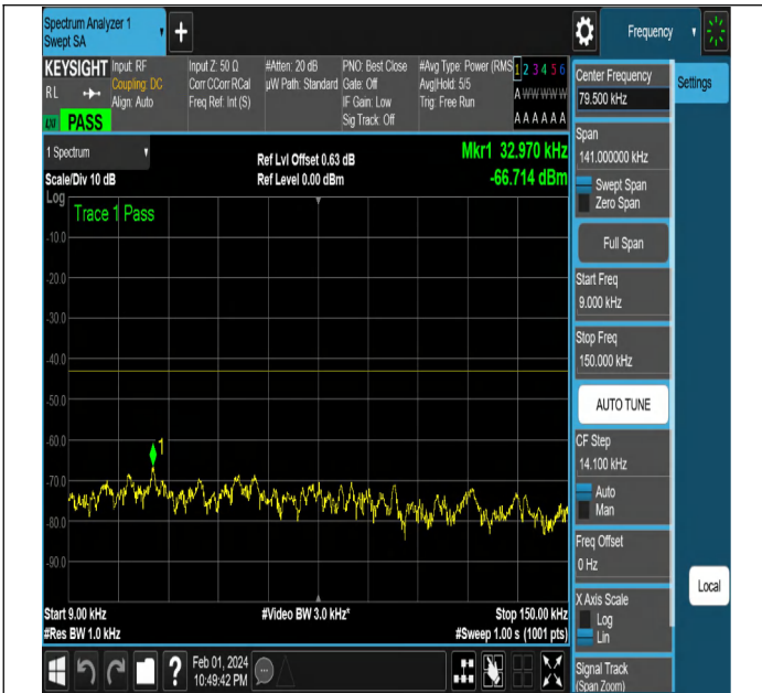
NTNV-N2-PC3-15-10-L-DFT-PI2BPSK-Edge_1RB_Left-Ant1- PASS
