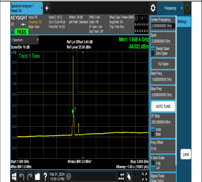
NTNV-N2-PC3-15-10-L-DFT-PI2BPSK-Edge_1RB_Left-Ant1- PASS
