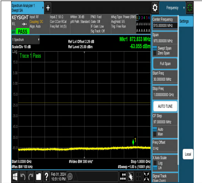
NTNV-N2-PC3-15-10-L-DFT-PI2BPSK-Edge_1RB_Right-Ant1 -PASS
