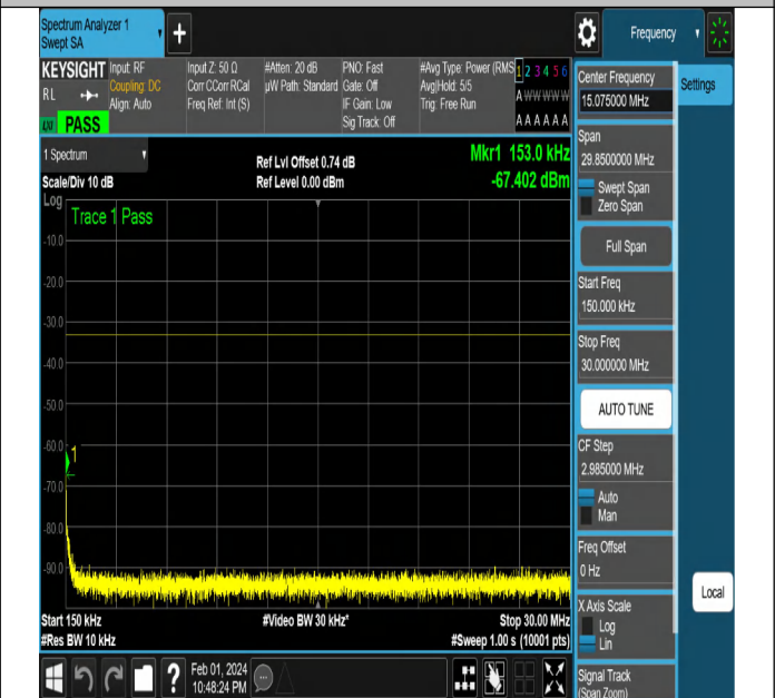
NTNV-N2-PC3-15-5-H-CP-QPSK-Edge_1RB_Right-Ant1-PAS
