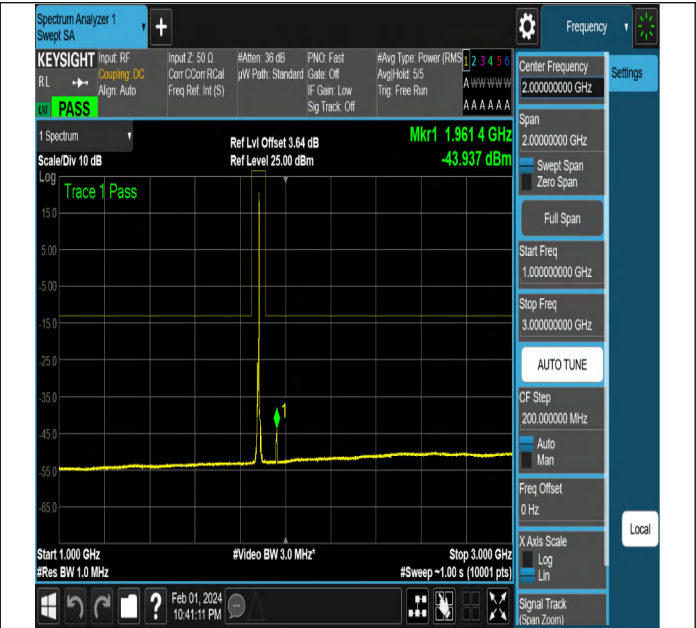
NTNV-N2-PC3-15-5-M-CP-QPSK-Edge_1RB_Right-Ant1-PAS S
