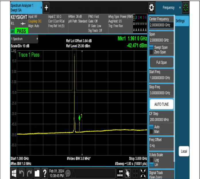
NTNV-N2-PC3-15-5-M-DFT-QPSK-Edge_1RB_Right-Ant1-PA SS
