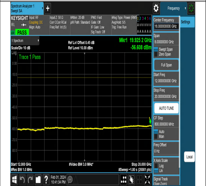
NTNV-N2-PC3-15-5-M-CP-QPSK-Edge_1RB_Right-Ant1-PAS S
