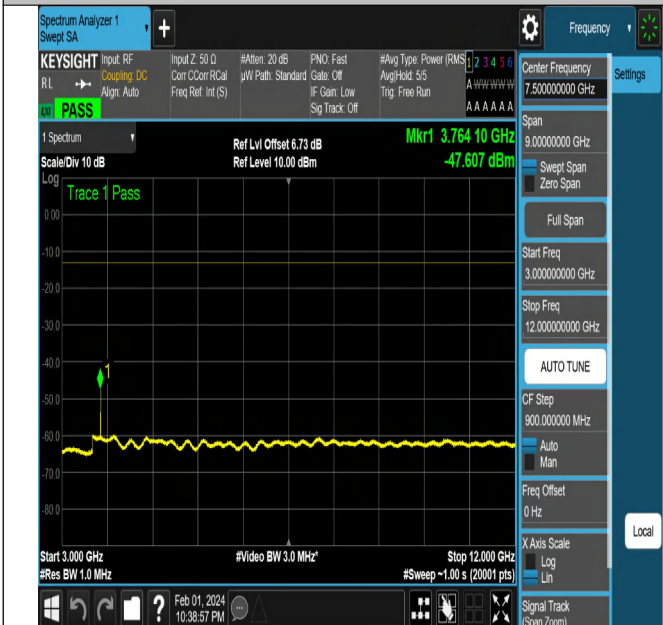
NTNV-N2-PC3-15-5-M-DFT-QPSK-Edge_1RB_Right-Ant1-PA SS
