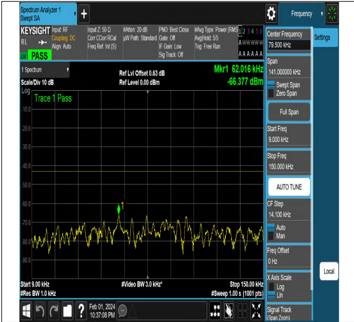
NTNV-N2-PC3-15-5-M-DFT-QPSK-Edge_1RB_Left-Ant1-PAS S
