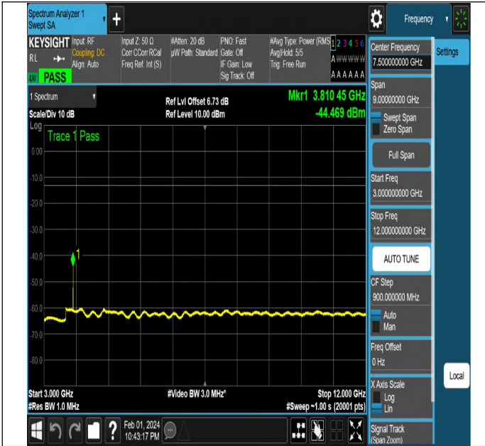
NTNV-N2-PC3-15-5-H-DFT-PI2BPSK-Edge_1RB_Left-Ant1-P ASS
