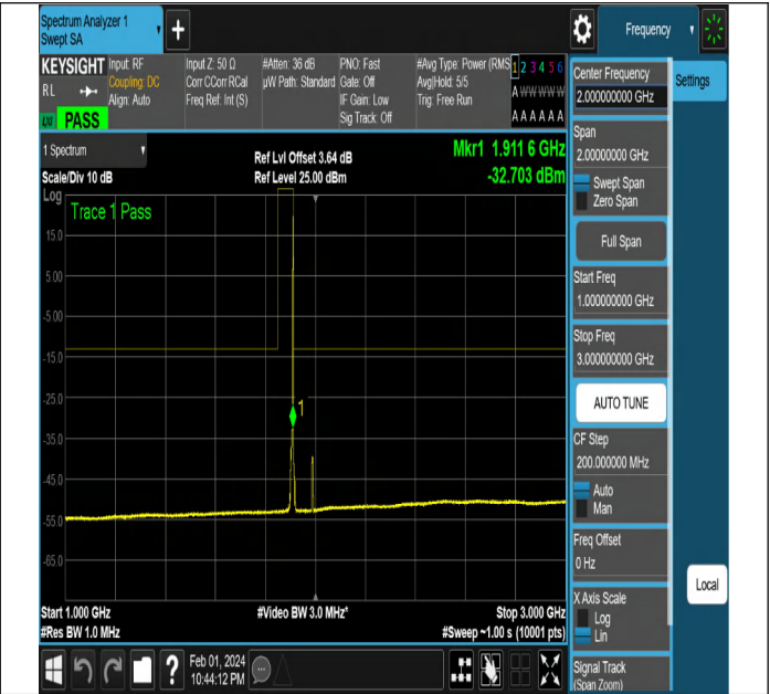
NTNV-N2-PC3-15-5-H-DFT-PI2BPSK-Edge_1RB_Right-Ant1- PASS
