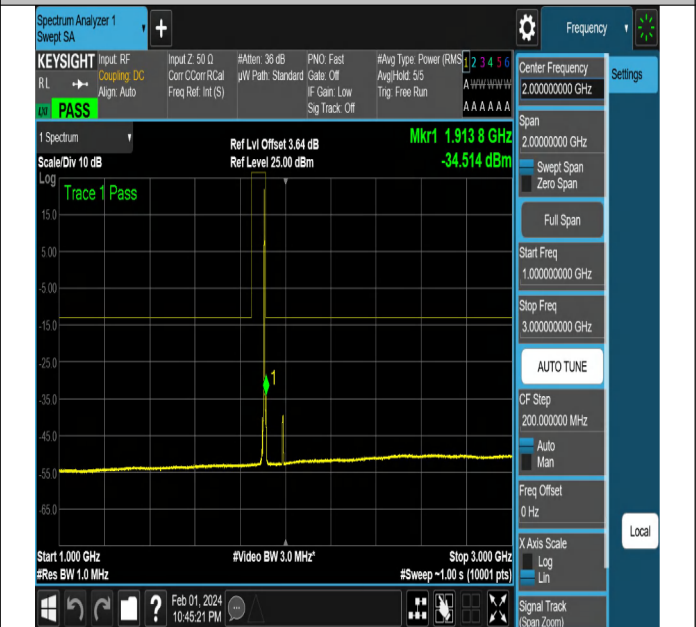
NTNV-N2-PC3-15-5-H-DFT-QPSK-Edge_1RB_Left-Ant1-PAS
