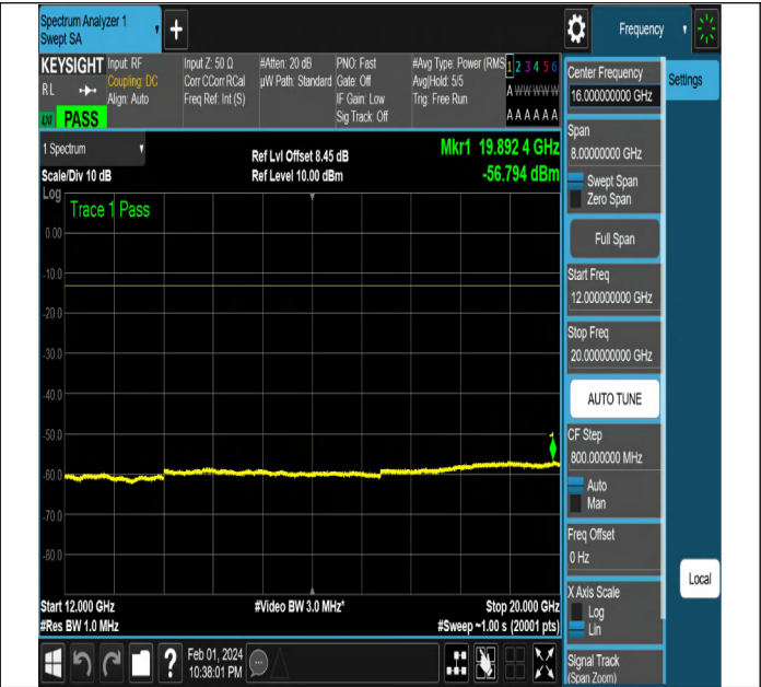
NTNV-N2-PC3-15-5-M-DFT-QPSK-Edge_1RB_Left-Ant1-PAS S
