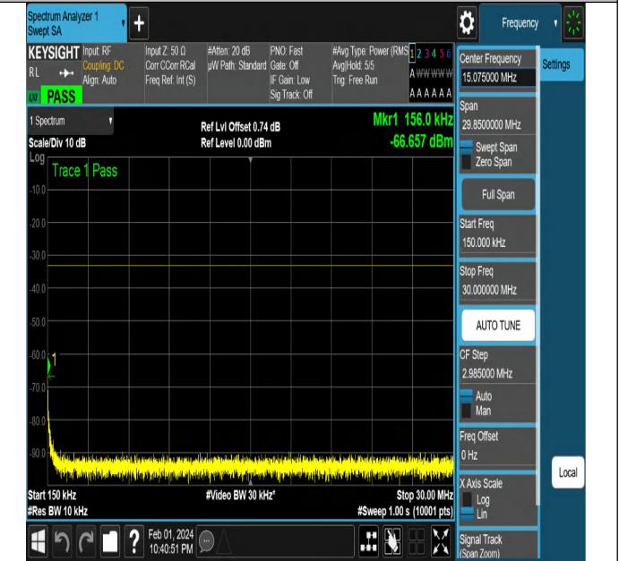
NTNV-N2-PC3-15-5-M-CP-QPSK-Edge_1RB_Right-Ant1-PAS
