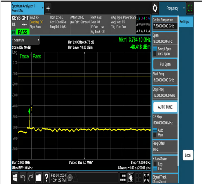
NTNV-N2-PC3-15-5-M-CP-QPSK-Edge_1RB_Right-Ant1-PAS S
