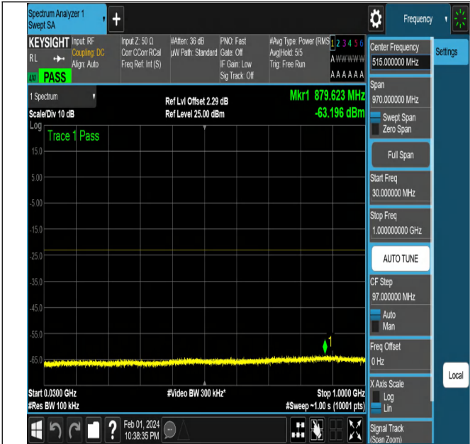
NTNV-N2-PC3-15-5-M-DFT-QPSK-Edge_1RB_Right-Ant1-PA SS
