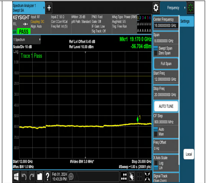
NTNV-N2-PC3-15-5-H-DFT-PI2BPSK-Edge_1RB_Left-Ant1-P ASS
