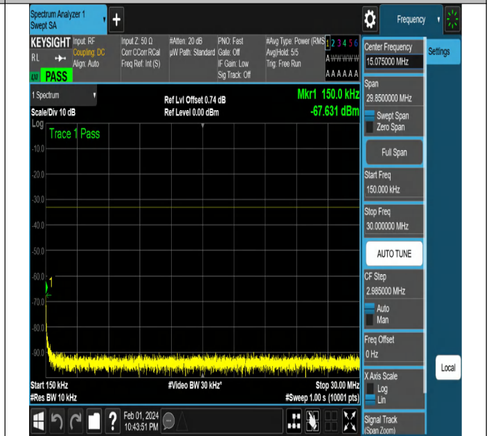
NTNV-N2-PC3-15-5-H-DFT-PI2BPSK-Edge_1RB_Right-Ant1-P PASS
