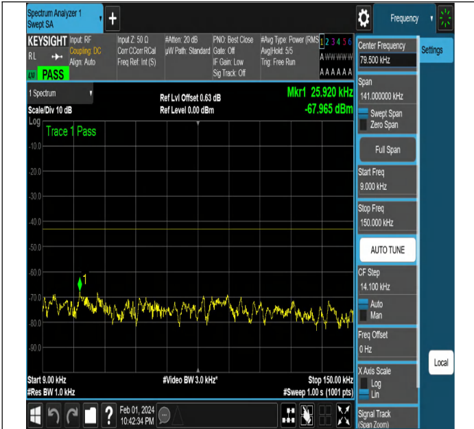
NTNV-N2-PC3-15-5-H-DFT-PI2BPSK-Edge_1RB_Left-Ant1-P ASS
