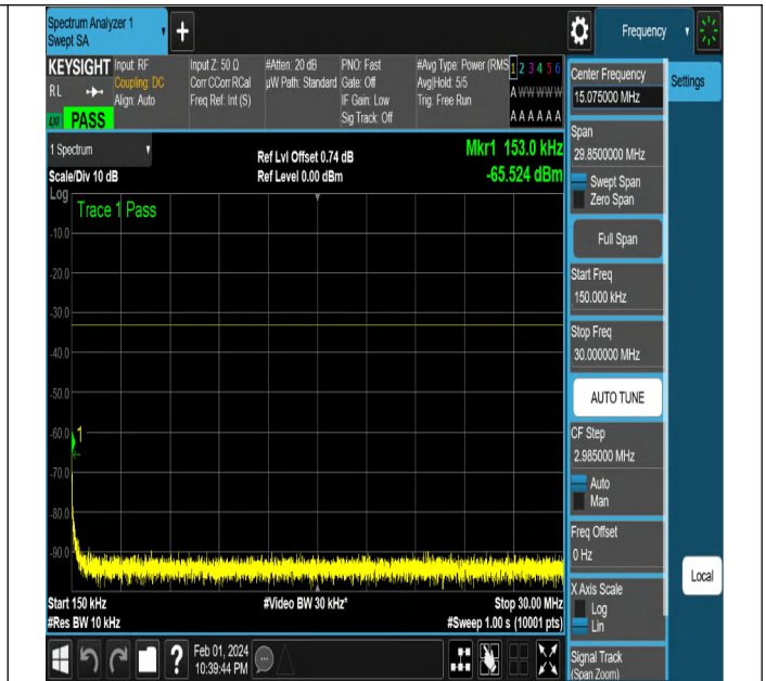
NTNV-N2-PC3-15-5-M-CP-QPSK-Edge_1RB_Left-Ant1-PASS
