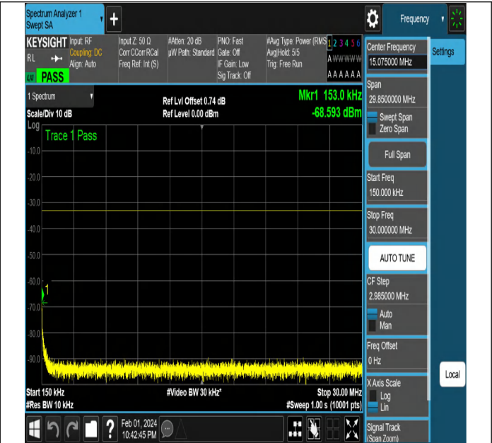
NTNV-N2-PC3-15-5-H-DFT-PI2BPSK-Edge_1RB_Left-Ant1-P ASS
