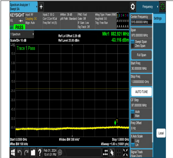
NTNV-N2-PC3-15-5-M-CP-QPSK-Edge_1RB_Right-Ant1-PAS S
