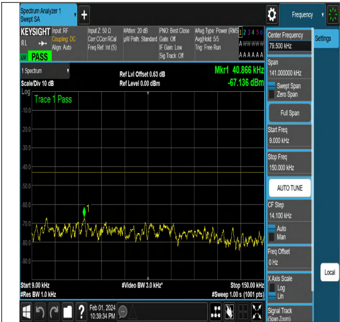
NTNV-N2-PC3-15-5-M-CP-QPSK-Edge_1RB_Left-Ant1-PASS
