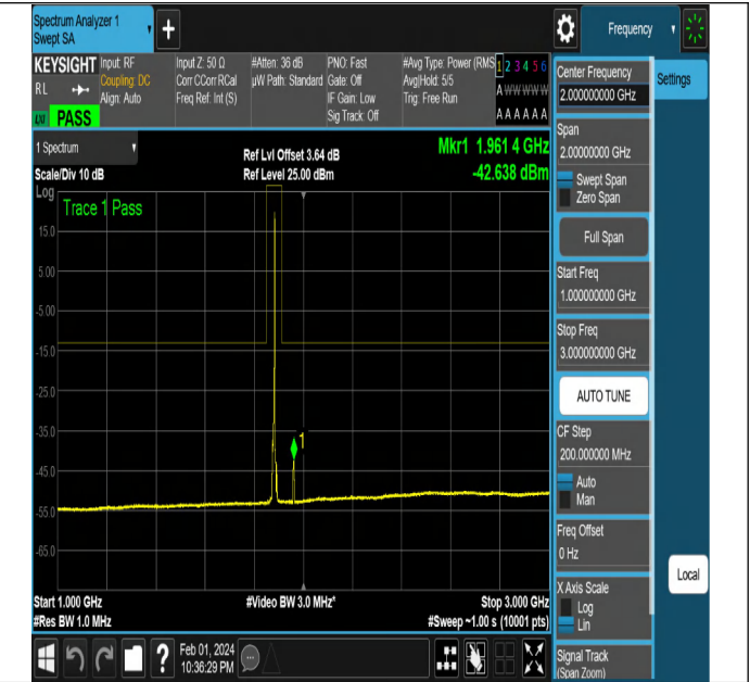
NTNV-N2-PC3-15-5-M-DFT-PI2BPSK-Edge_1RB_Right-Ant1- PASS
