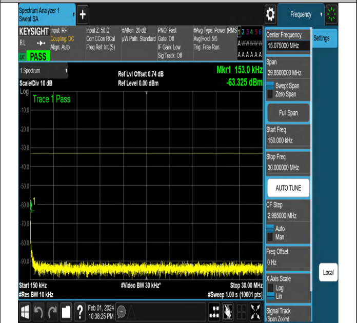
NTNV-N2-PC3-15-5-M-DFT-QPSK-Edge_1RB_Right-Ant1-PA SS
