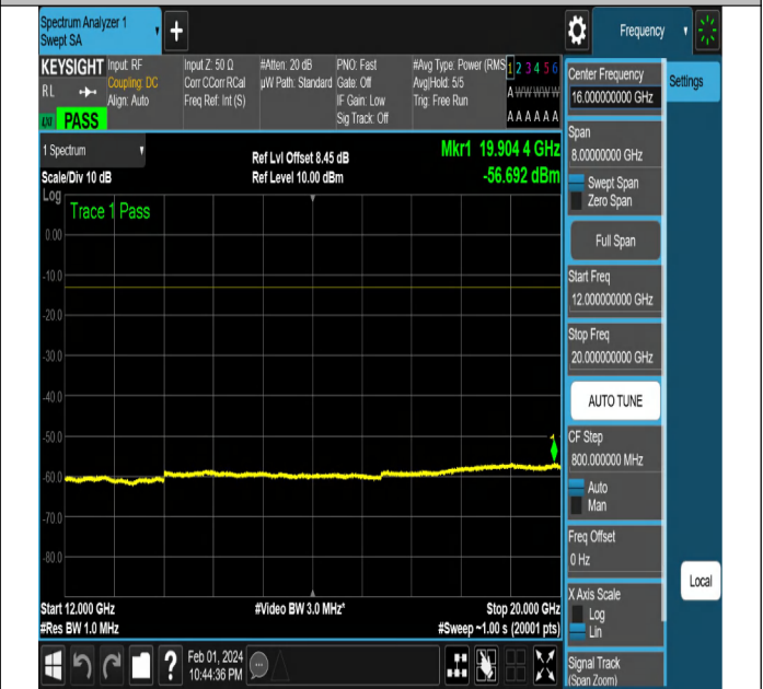
NTNV-N2-PC3-15-5-H-DFT-PI2BPSK-Edge_1RB_Right-Ant1- PASS
