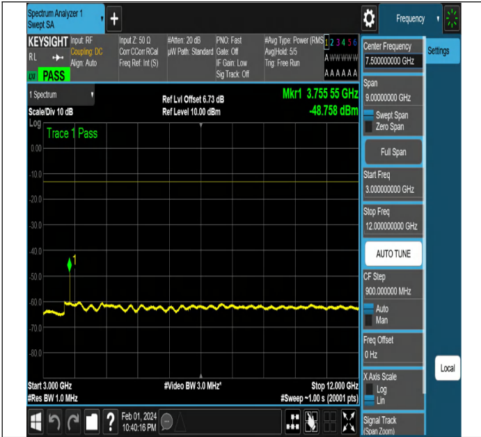
NTNV-N2-PC3-15-5-M-CP-QPSK-Edge_1RB_Left-Ant1-PASS
