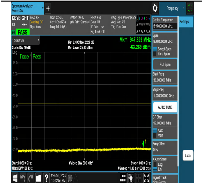
NTNV-N2-PC3-15-5-H-DFT-PI2BPSK-Edge_1RB_Left-Ant1-P ASS
