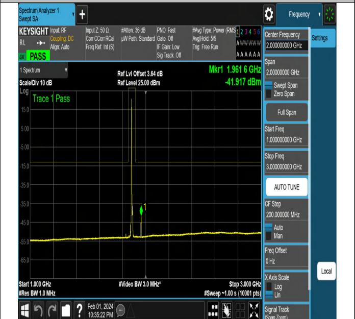
NTNV-N2-PC3-15-5-M-DFT-PI2BPSK-Edge_1RB_Left-Ant1-P
