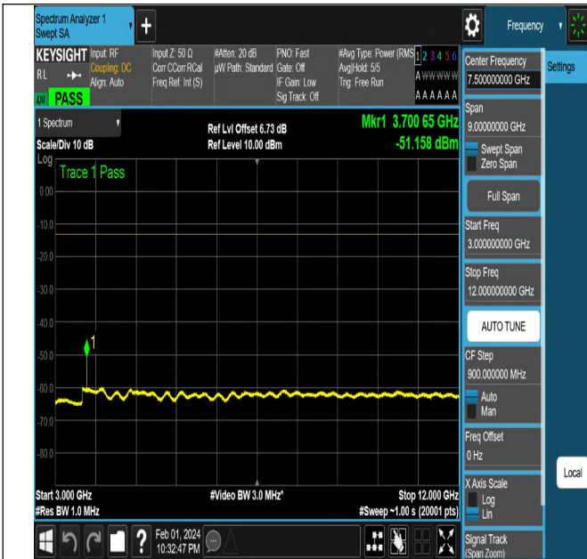
NTNV-N2-PC3-15-5-L-CP-QPSK-Edge_1RB_Left-Ant1-PASS
