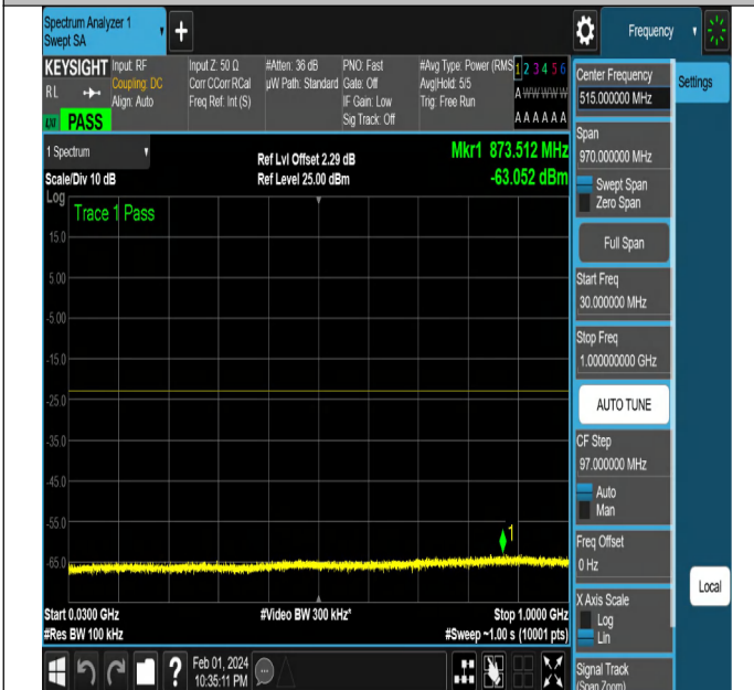
NTNV-N2-PC3-15-5-M-DFT-PI2BPSK-Edge_1RB_Left-Ant1-P
