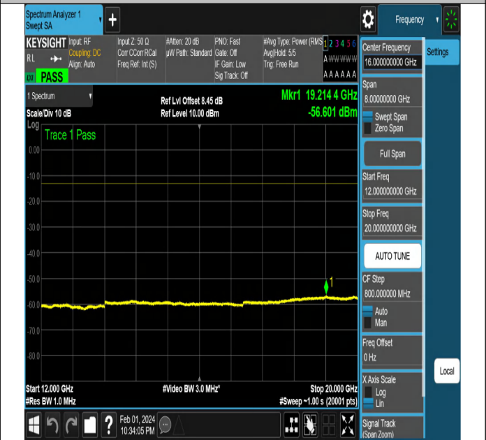
NTNV-N2-PC3-15-5-L-CP-QPSK-Edge_1RB_Right-Ant1-PAS
