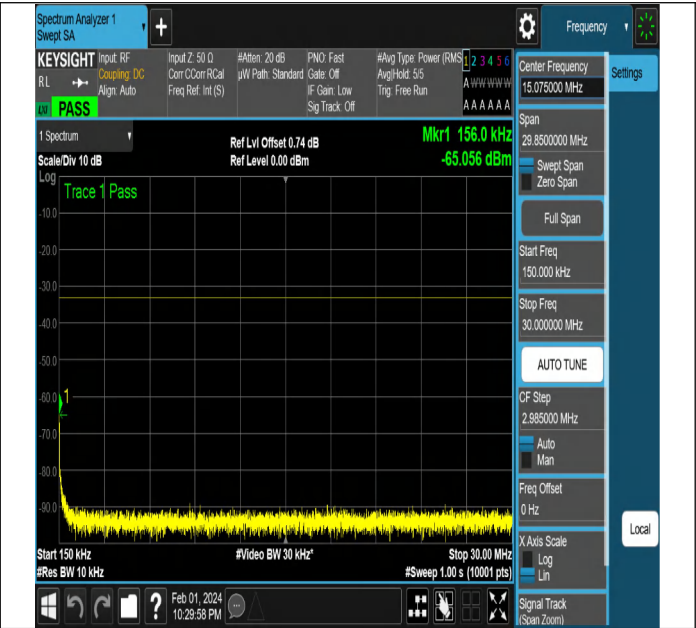
NTNV-N2-PC3-15-5-L-DFT-QPSK-Edge_1RB_Left-Ant1-PAS
