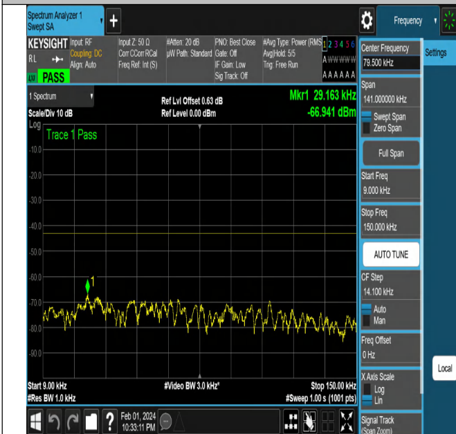
NTNV-N2-PC3-15-5-L-CP-QPSK-Edge_1RB_Right-Ant1-PAS
