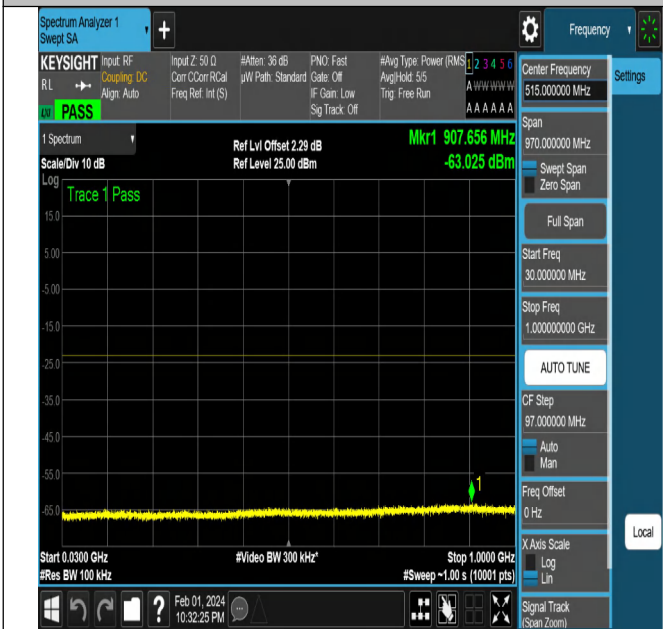
NTNV-N2-PC3-15-5-L-CP-QPSK-Edge_1RB_Left-Ant1-PASS
