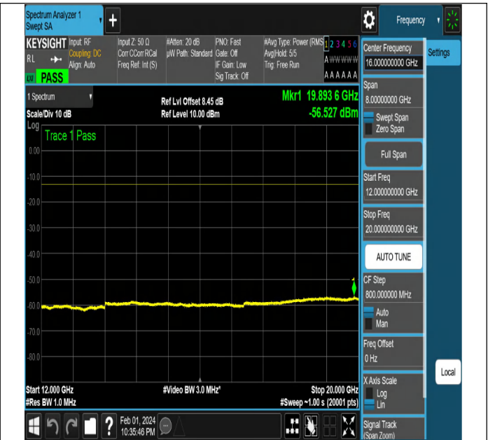
NTNV-N2-PC3-15-5-M-DFT-PI2BPSK-Edge_1RB_Left-Ant1-P
