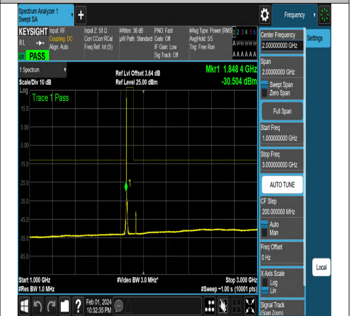
NTNV-N2-PC3-15-5-L-CP-QPSK-Edge_1RB_Left-Ant1-PASS
