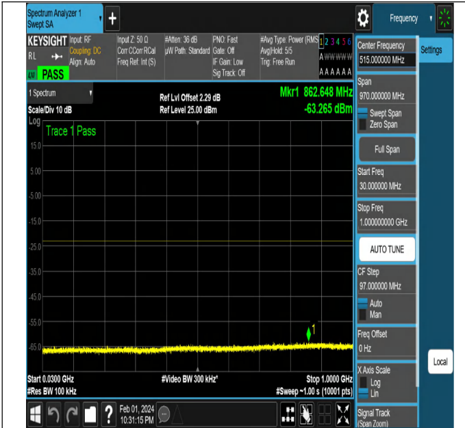
NTNV-N2-PC3-15-5-L-DFT-QPSK-Edge_1RB_Right-Ant1-PA
