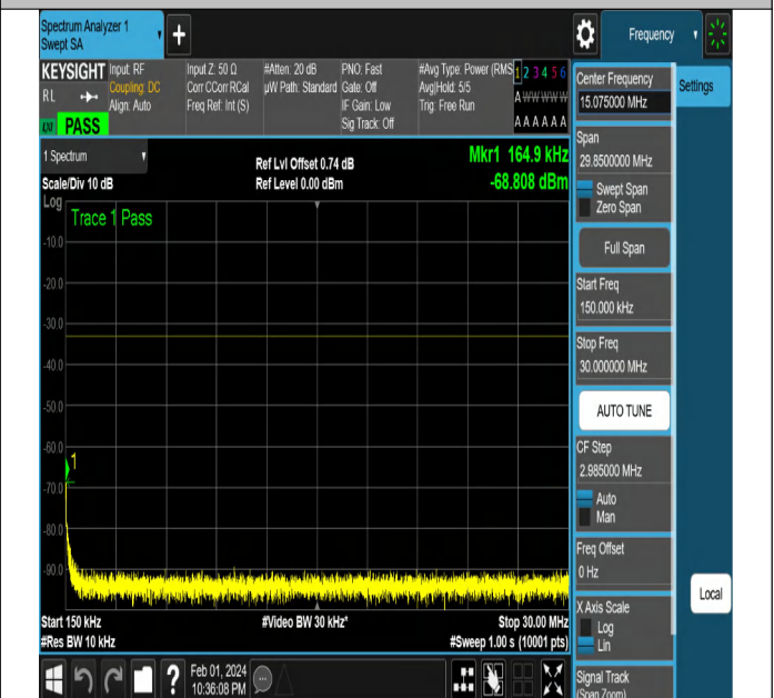
NTNV-N2-PC3-15-5-M-DFT-PI2BPSK-Edge_1RB_Right-Ant1-P
