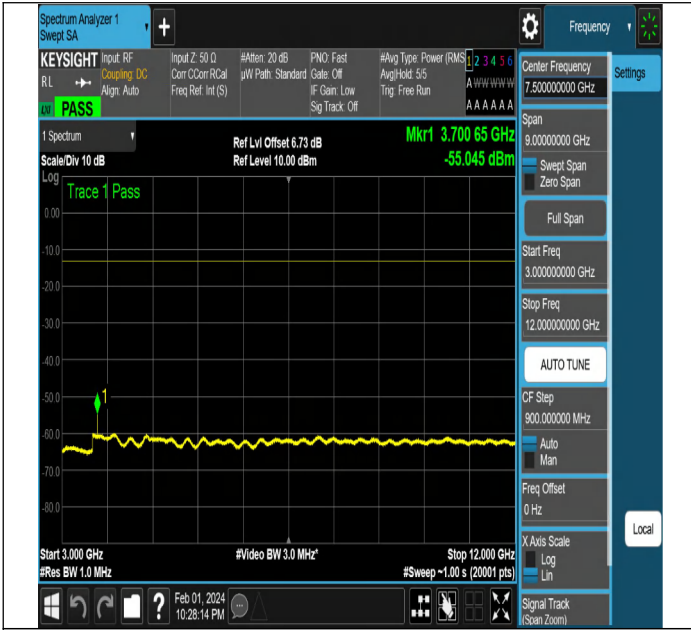
NTNV-N2-PC3-15-5-L-DFT-PI2BPSK-Edge_1RB_Left-Ant1-P
