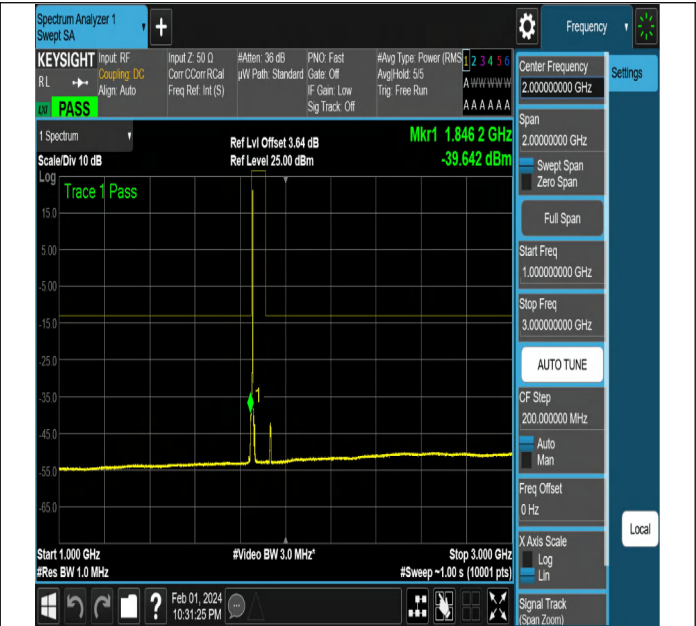
NTNV-N2-PC3-15-5-L-DFT-QPSK-Edge_1RB_Right-Ant1-PA
