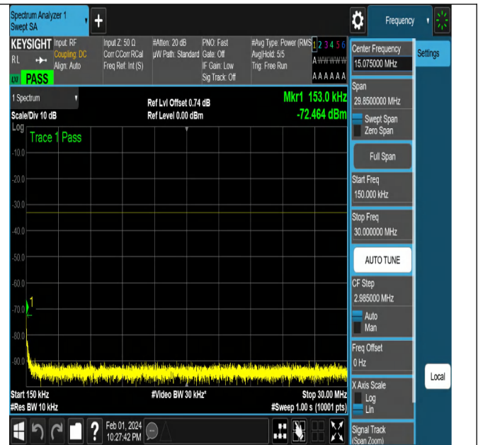
NTNV-N2-PC3-15-5-L-DFT-PI2BPSK-Edge_1RB_Left-Ant1-P ASS
