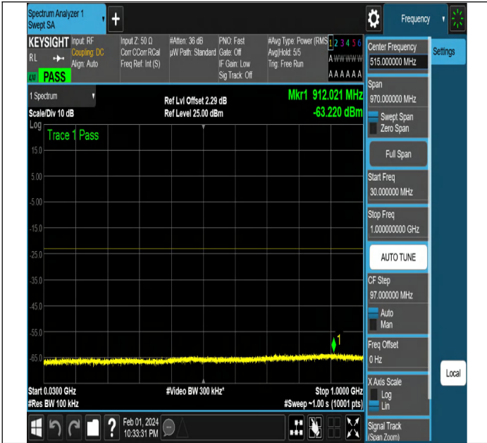
NTNV-N2-PC3-15-5-L-CP-QPSK-Edge_1RB_Right-Ant1-PAS
