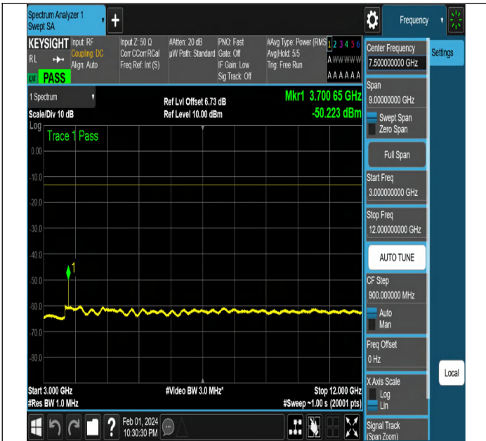
NTNV-N2-PC3-15-5-L-DFT-QPSK-Edge_1RB_Left-Ant1-PAS
