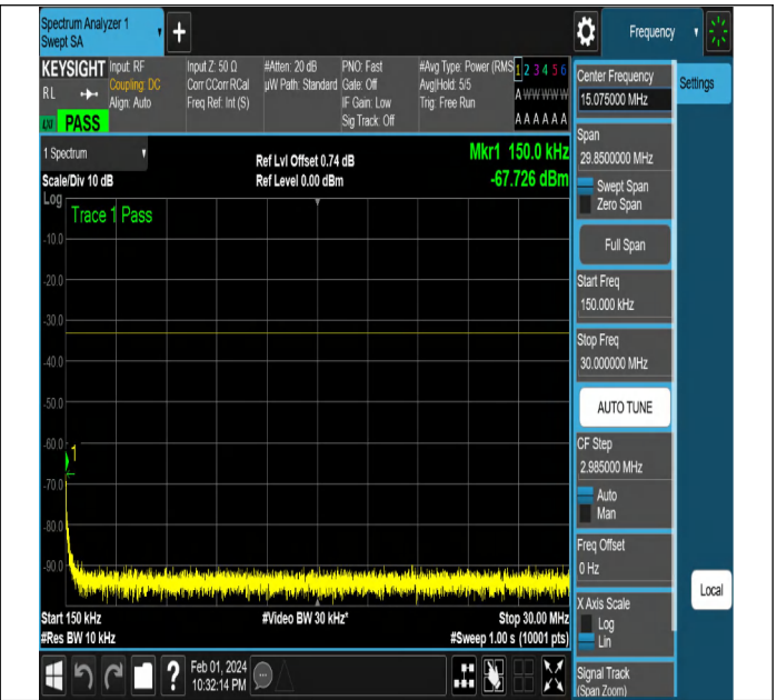
NTNV-N2-PC3-15-5-L-CP-QPSK-Edge_1RB_Left-Ant1-PASS
