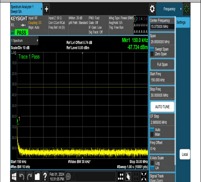
NTNV-N2-PC3-15-5-L-DFT-QPSK-Edge_1RB_Right-Ant1-PA
