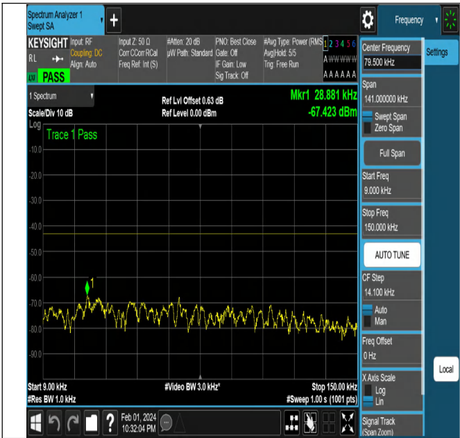
NTNV-N2-PC3-15-5-L-CP-QPSK-Edge_1RB_Left-Ant1-PASS
