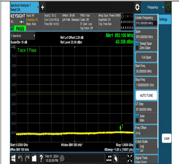
NTNV-N2-PC3-15-5-L-DFT-QPSK-Edge_1RB_Left-Ant1-PAS
