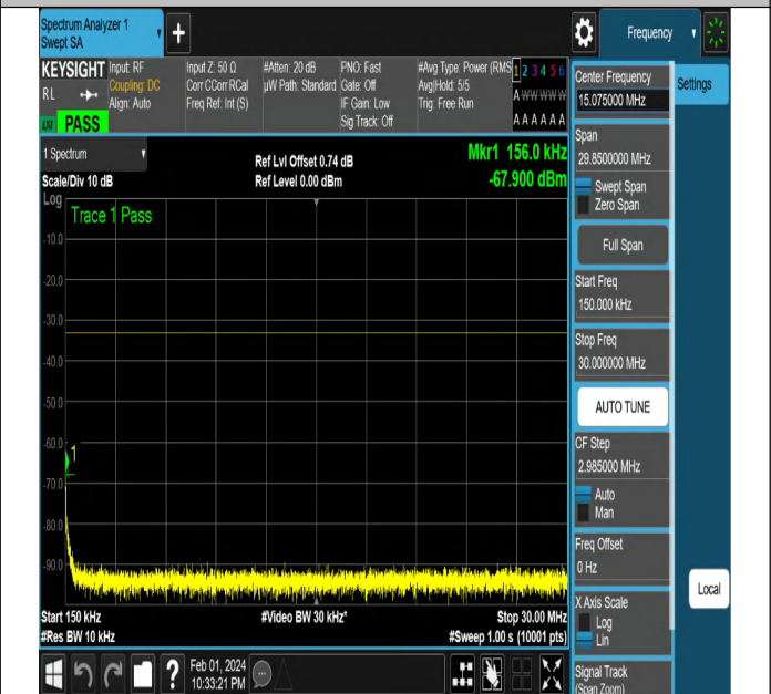
NTNV-N2-PC3-15-5-L-CP-QPSK-Edge_1RB_Right-Ant1-PAS
