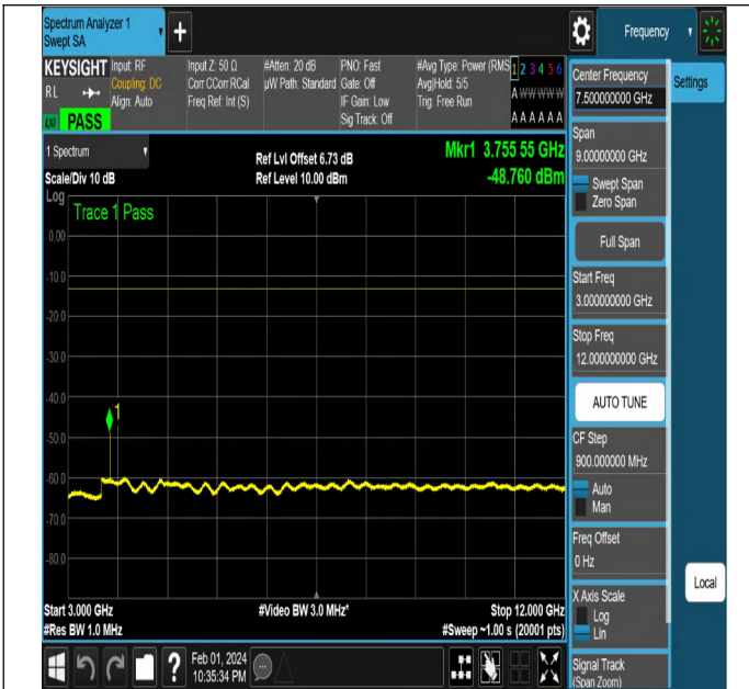
NTNV-N2-PC3-15-5-M-DFT-PI2BPSK-Edge_1RB_Left-Ant1-P
