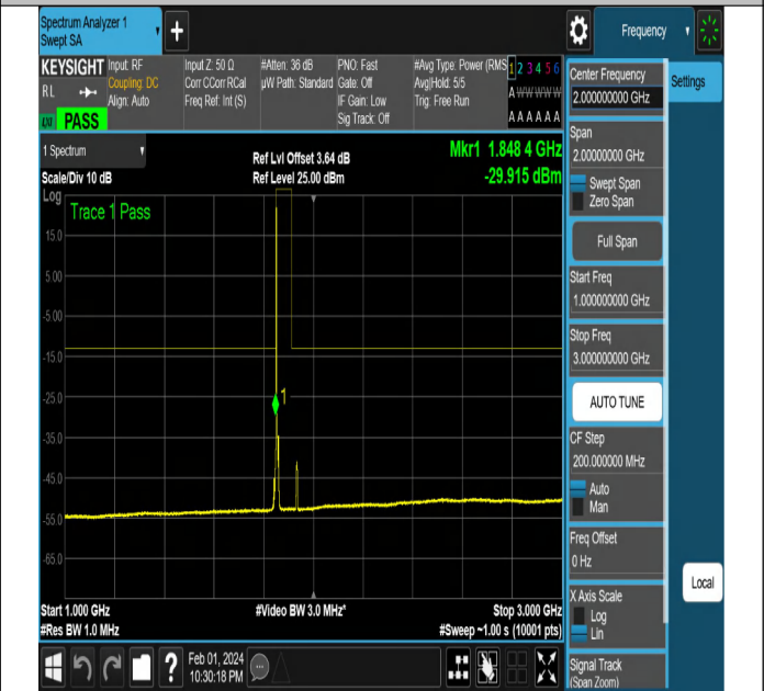
NTNV-N2-PC3-15-5-L-DFT-QPSK-Edge_1RB_Left-Ant1-PAS
