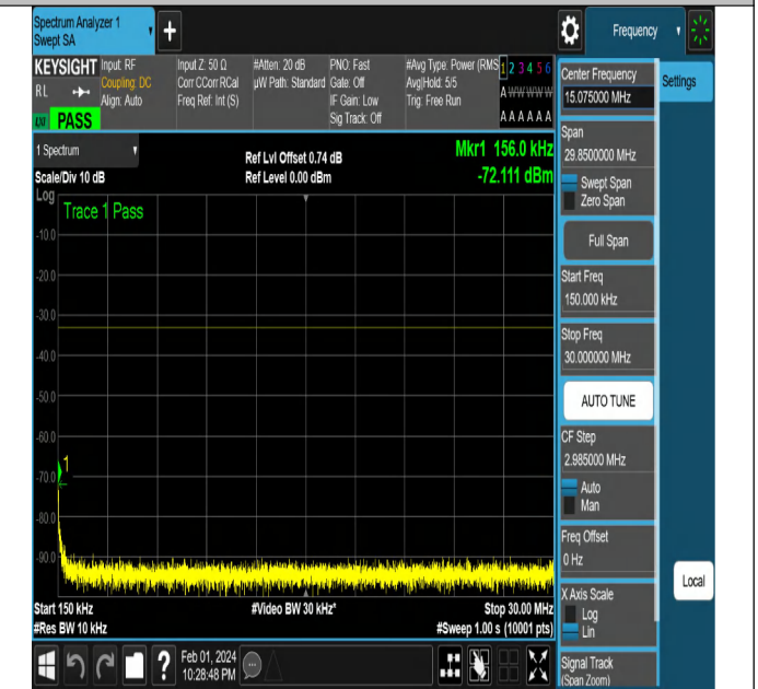
NTNV-N2-PC3-15-5-L-DFT-PI2BPSK-Edge_1RB_Right-Ant1-P
