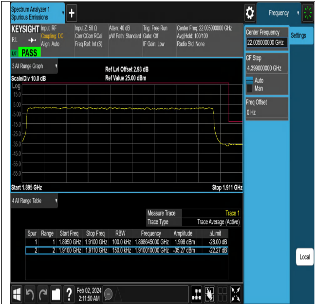
NTNV-N2-PC3-15-15-H-DFT-PI2BPSK-Outter_Full-Ant1-PA
