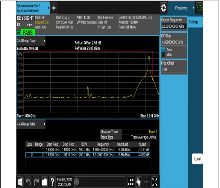
NTNV-N2-PC3-15-20-H-DFT-PI2BPSK-Edge_1RB_Right-Ant1-P ASS
