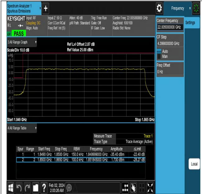
NTNV-N2-PC3-15-15-L-DFT-PI2BPSK-Outter_Full-Ant1-PA
