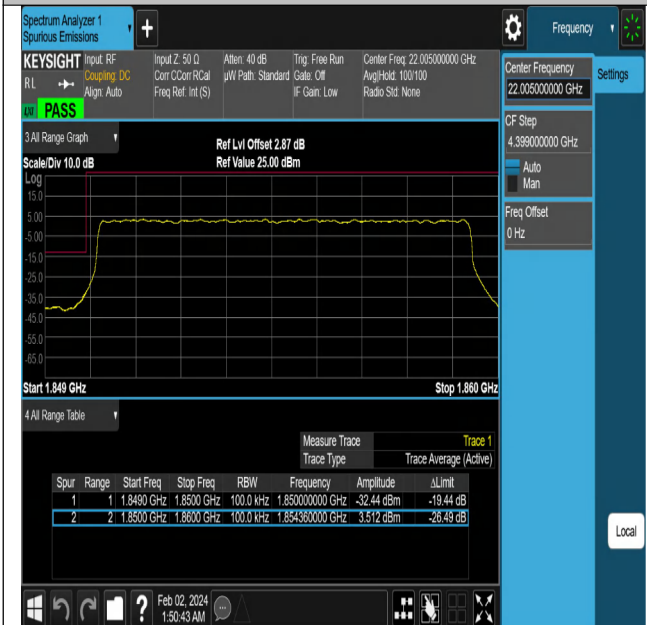
NTNV-N2-PC3-15-10-L-DFT-QPSK-Outter_Full-Ant1-PASS
