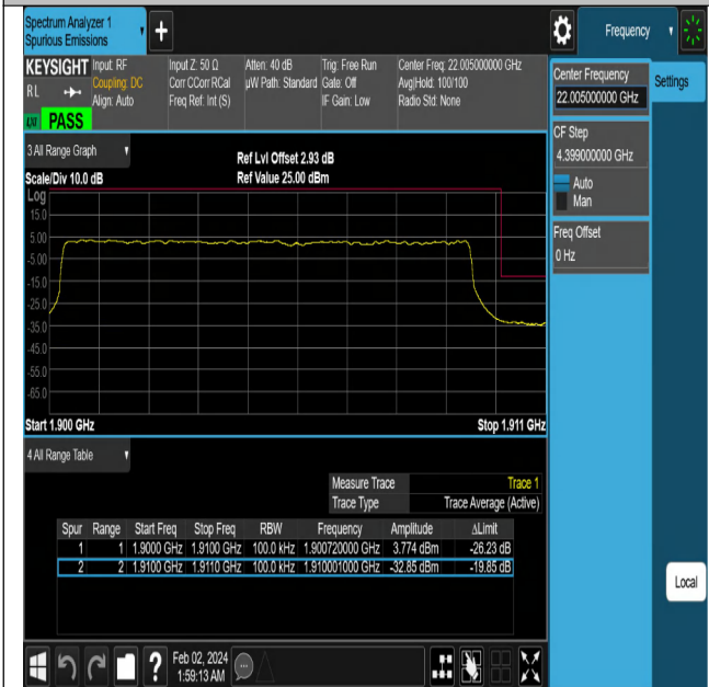
NTNV-N2-PC3-15-10-H-DFT-QPSK-Outter_Full-Ant1-PASS
