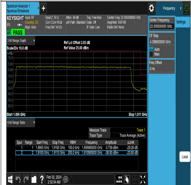
NTNV-N2-PC3-15-20-H-DFT-QPSK-Outter_Full-Ant1-PASS
