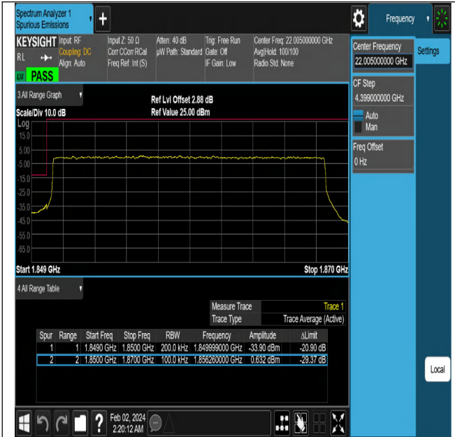
NTNV-N2-PC3-15-20-L-DFT-PI2BPSK-Outter_Full-Ant1-PA
