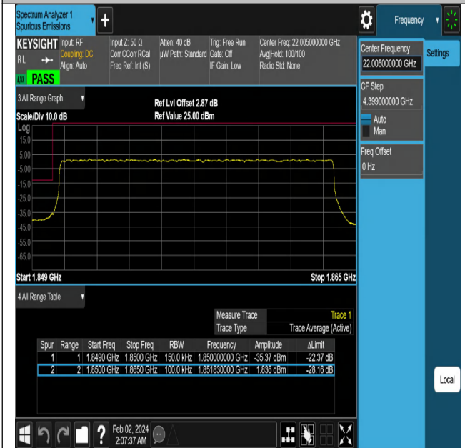
NTNV-N2-PC3-15-15-L-DFT-QPSK-Outter_Full-Ant1-PASS
