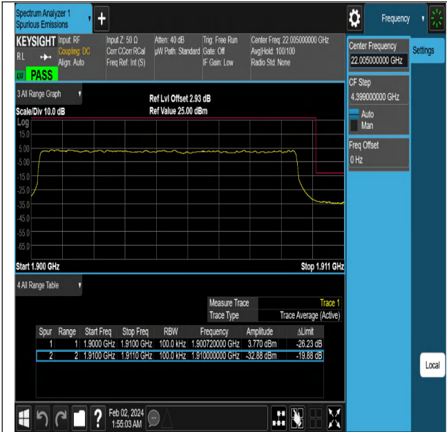
NTNV-N2-PC3-15-10-H-DFT-PI2BPSK-Outter_Full-Ant1-PA SS
