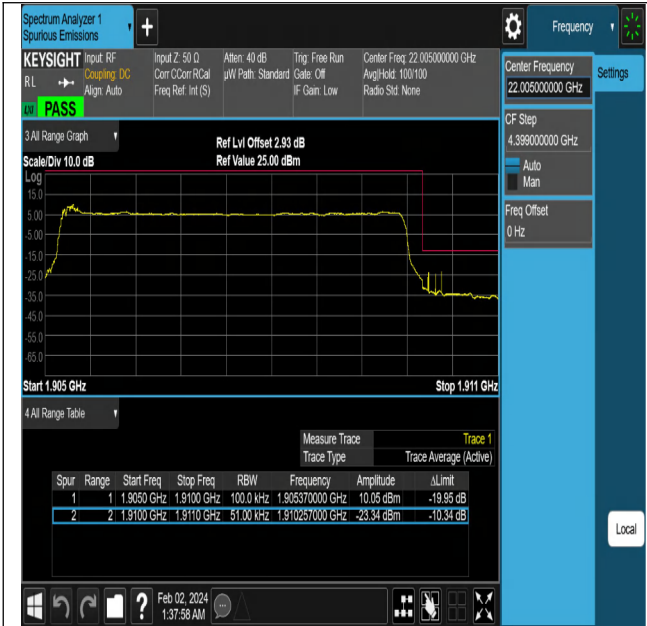
NTNV-N2-PC3-15-5-H-DFT-PI2BPSK-Outer_Full-Ant1-PA
