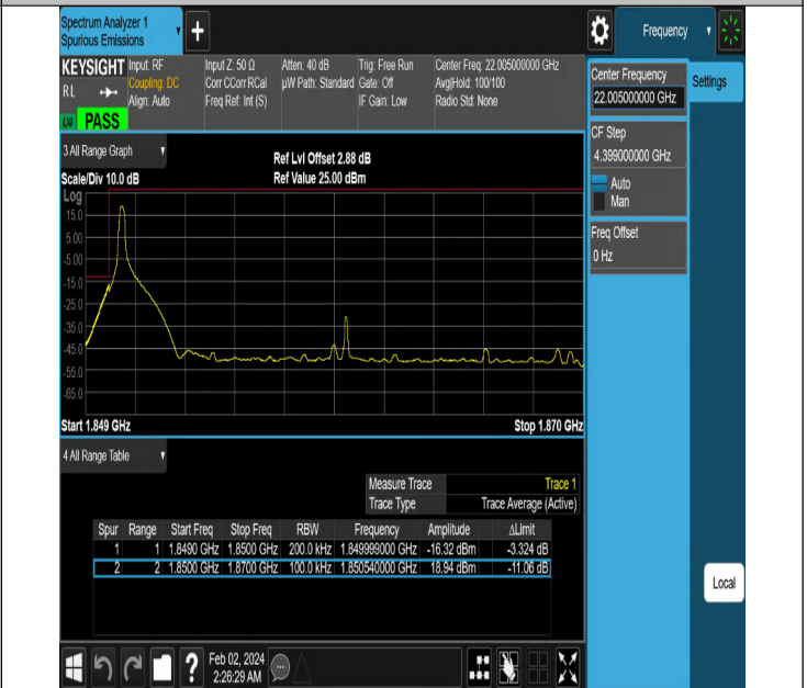
NTNV-N2-PC3-15-20-L-DFT-QPSK-Edge_1RB_Left-Ant1-PASS
