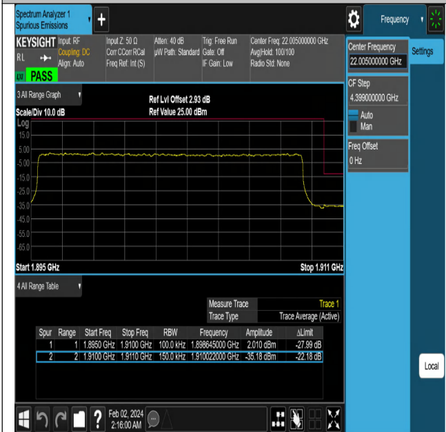
NTNV-N2-PC3-15-15-H-DFT-QPSK-Outter_Full-Ant1-PASS
