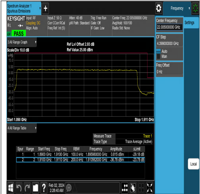
NTNV-N2-PC3-15-20-H-DFT-PI2BPSK-Outter_Full-Ant1-PA SS
