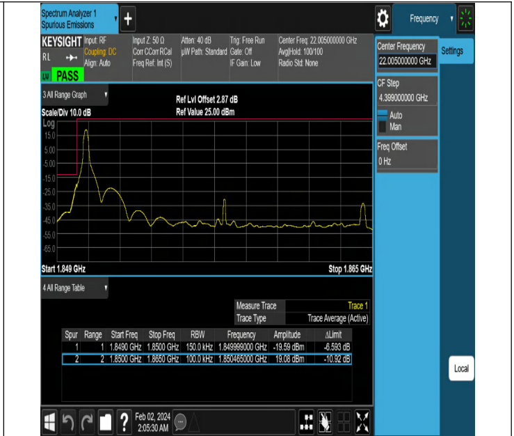
NTNV-N2-PC3-15-15-L-DFT-PI2BPSK-Edge_1RB_Left-Ant1-PAS
