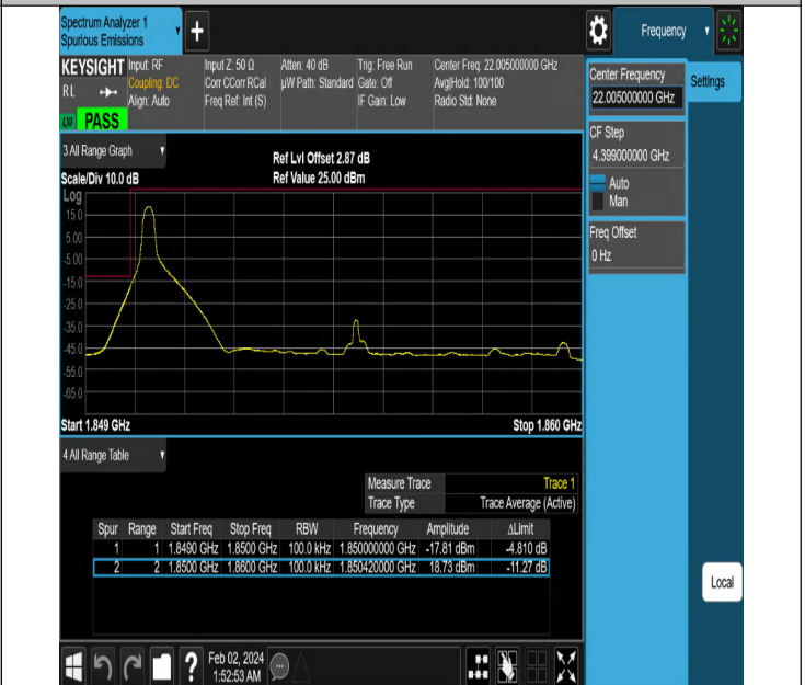
NTNV-N2-PC3-15-10-L-DFT-QPSK-Edge_1RB_Left-Ant1-PASS
