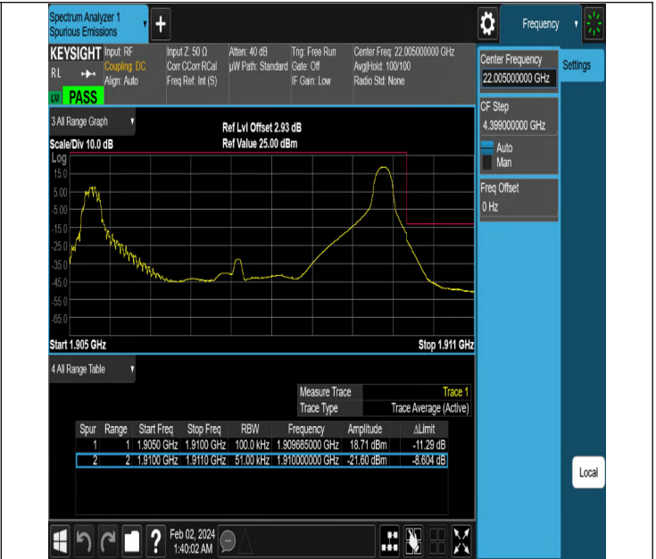
NTNV-N2-PC3-15-5-H-DFT-PI2BPSK-Edge_1RB_Right-Ant1-PA
