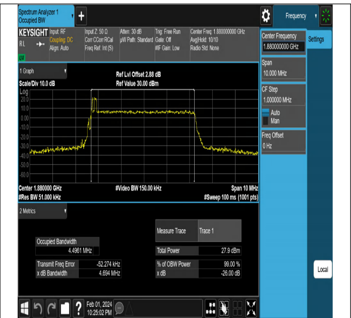
NTNV-N2-PC3-15-5-M-CP-16QAM-Outer_Full-Ant1-PASS
