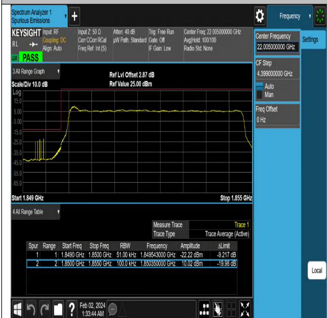
NTNV-N2-PC3-15-5-L-DFT-QPSK-Outter_Full-Ant1-PASS
