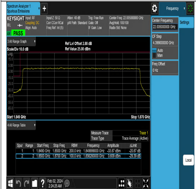
NTNV-N2-PC3-15-20-L-DFT-QPSK-Outter_Full-Ant1-PASS
