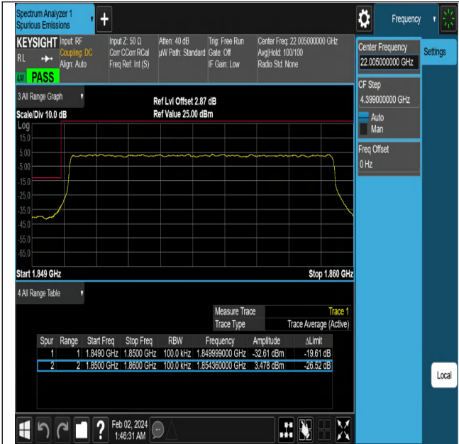
NTNV-N2-PC3-15-10-L-DFT-PI2BPSK-Outter_Full-Ant1-PA
