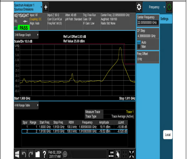
NTNV-N2-PC3-15-10-H-DFT-QPSK-Edge_1RB_Right-Ant1-PAS S
