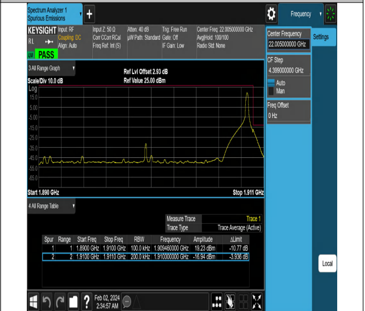
NTNV-N2-PC3-15-20-H-DFT-QPSK-Edge_1RB_Right-Ant1-PAS S
