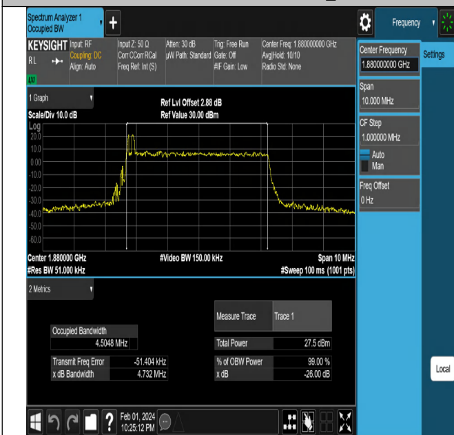
NTNV-N2-PC3-15-5-M-CP-64QAM-Outer_Full-Ant1-PASS
