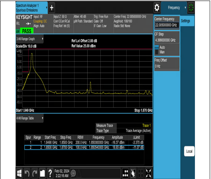
NTNV-N2-PC3-15-20-L-DFT-PI2BPSK-Edge_1RB_Left-Ant1-PAS
