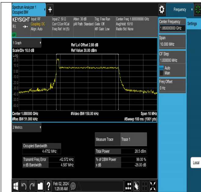
NTNV-N2-PC3-15-5-M-CP-QPSK-Outer_Full-Ant1-PASS
