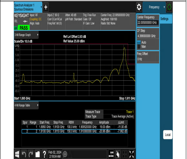
NTNV-N2-PC3-15-15-H-DFT-QPSK-Edge_1RB_Right-Ant1-PAS
