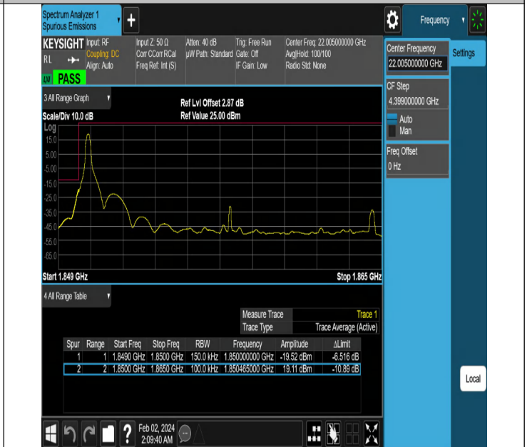
NTNV-N2-PC3-15-15-L-DFT-QPSK-Edge_1RB_Left-Ant1-PASS
