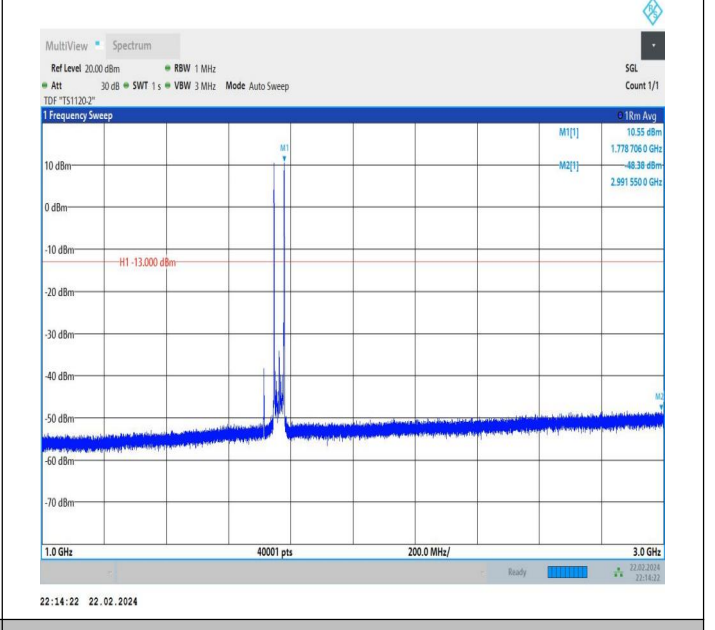
66-66-20MHz-15MHz-QPSK-QPSK-132423-132594-1RB#0-1 RB#74-1000~3000MHz-PASS
