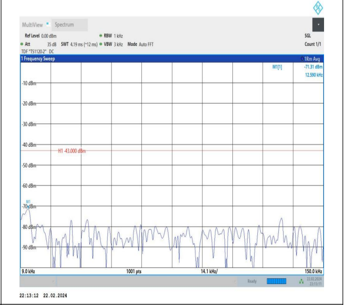
66-66-20MHz-15MHz-QPSK-QPSK-132423-132594-1RB#99-0 RB#0-0.009~0.15MHz-PASS
