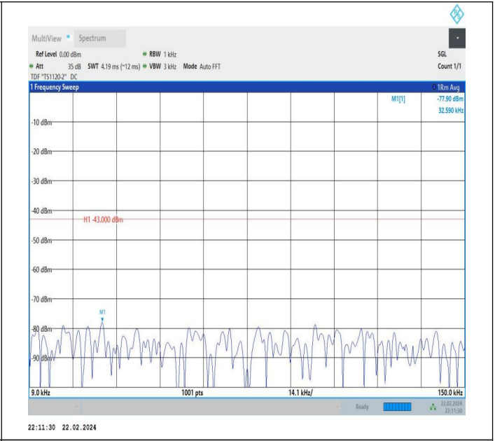
66-66-20MHz-15MHz-QPSK-QPSK-132348-132519-1RB#0-1 RB#74-0.009~0.15MHz-PASS
