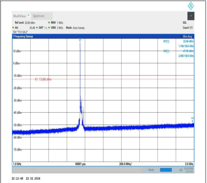
66-66-20MHz-15MHz-QPSK-QPSK-132423-132594-1RB#0-0 RB#0-1000~3000MHz-PASS
