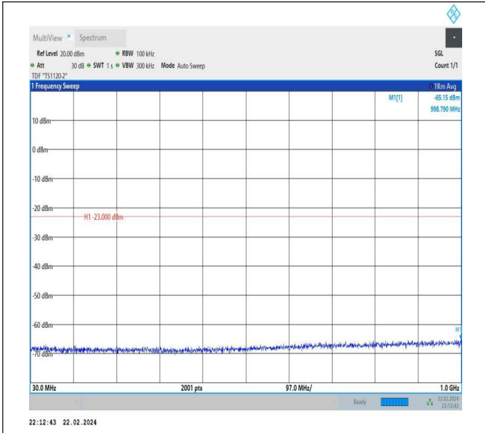
66-66-20MHz-15MHz-QPSK-QPSK-132423-132594-1RB#0-0 RB#0-30~1000MHz-PASS
