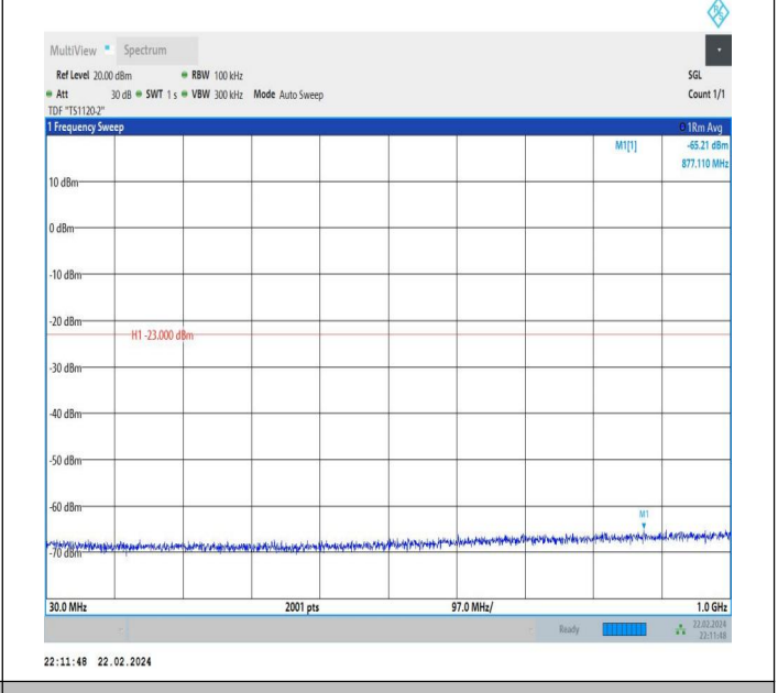
66-66-20MHz-15MHz-QPSK-QPSK-132348-132519-1RB#0-1 RB#74-30~1000MHz-PASS
