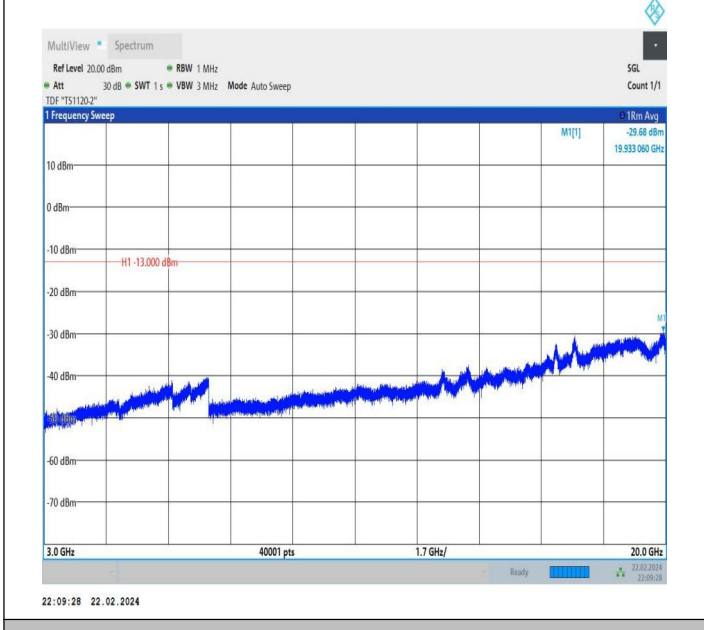
66-66-20MHz-15MHz-QPSK-QPSK-132072-132243-1RB#0-1 RB#74-3000~20000MHz-PASS
