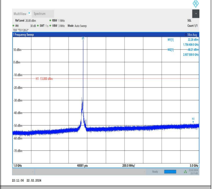
66-66-20MHz-15MHz-QPSK-QPSK-132348-132519-1RB#99-0 RB#0-1000~3000MHz-PASS
