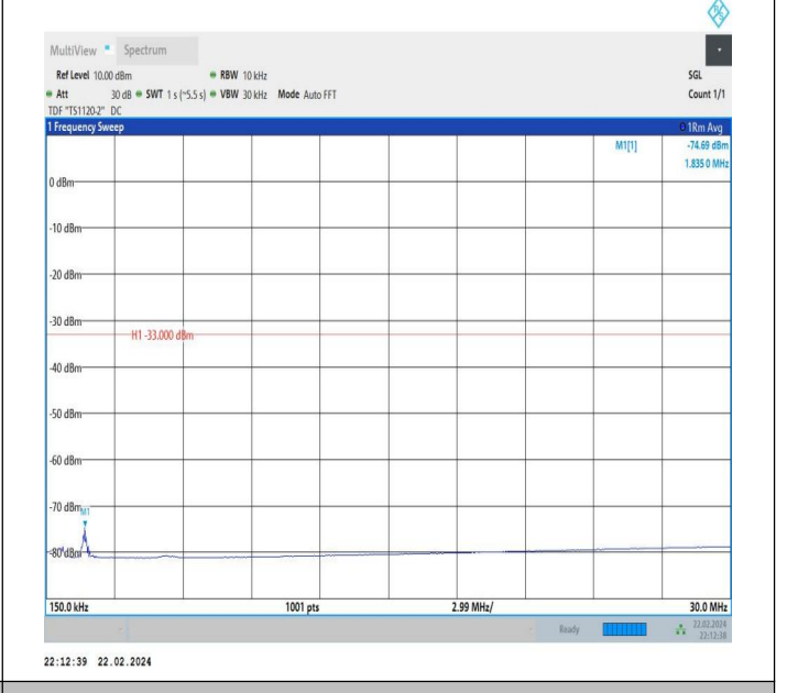
66-66-20MHz-15MHz-QPSK-QPSK-132423-132594-1RB#0-0 RB#0-0.15~30MHz-PASS
