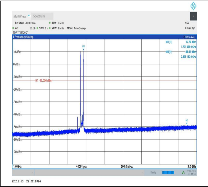
66-66-20MHz-15MHz-QPSK-QPSK-132348-132519-1RB#0-1 RB#74-1000~3000MHz-PASS
