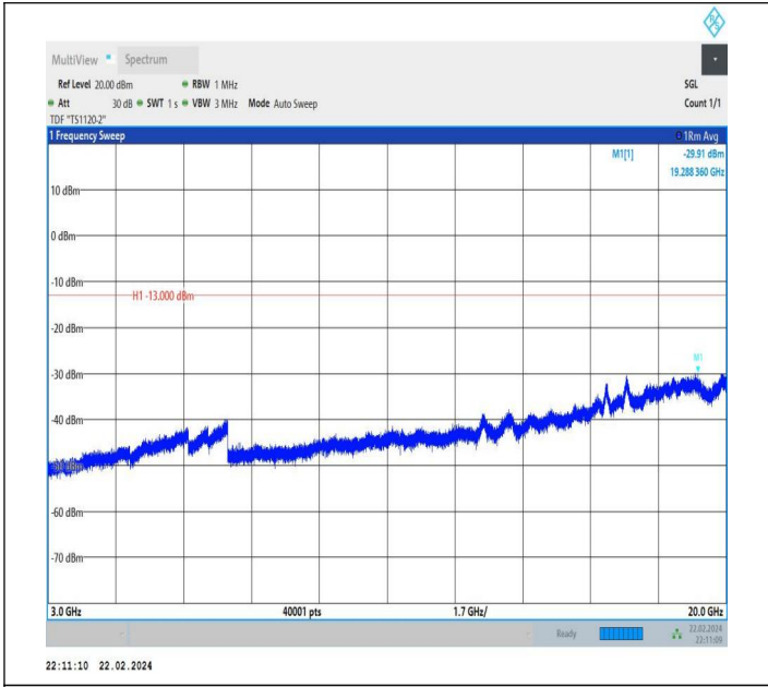
66-66-20MHz-15MHz-QPSK-QPSK-132348-132519-1RB#99-0 RB#0-3000~20000MHz-PASS
