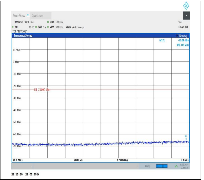
66-66-20MHz-15MHz-QPSK-QPSK-132423-132594-1RB#99-0 RB#0-30~1000MHz-PASS
