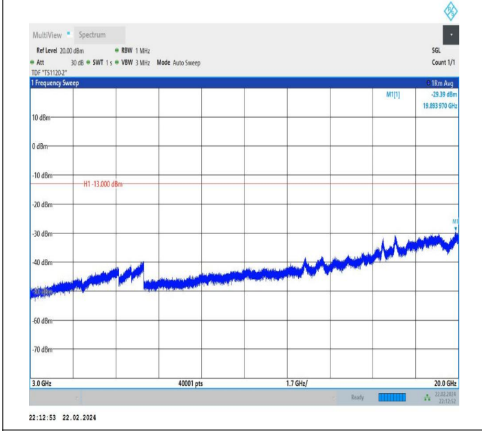
66-66-20MHz-15MHz-QPSK-QPSK-132423-132594-1RB#0-0 RB#0-3000~20000MHz-PASS
