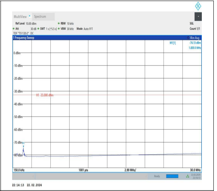
66-66-20MHz-15MHz-QPSK-QPSK-132423-132594-1RB#0-1 RB#74-0.15~30MHz-PASS
