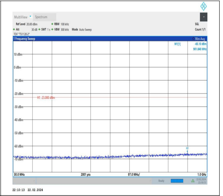
66-66-20MHz-15MHz-QPSK-QPSK-132348-132519-1RB#0-0 RB#0-30~1000MHz-PASS
