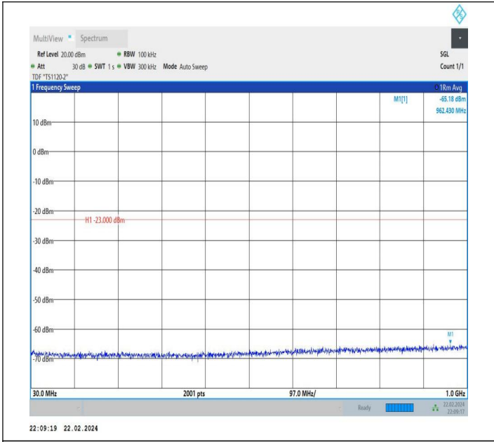
66-66-20MHz-15MHz-QPSK-QPSK-132072-132243-1RB#0-1 RB#74-30~1000MHz-PASS
