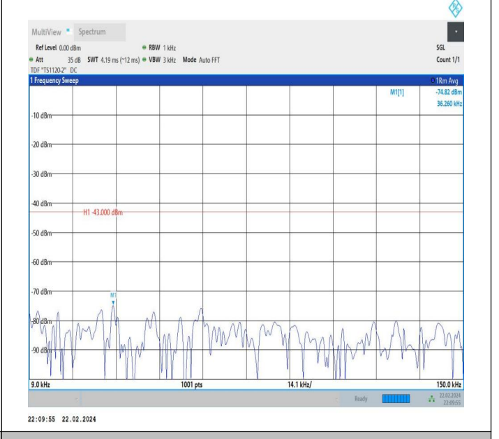
66-66-20MHz-15MHz-QPSK-QPSK-132348-132519-1RB#0-0 RB#0-0.009~0.15MHz-PASS
