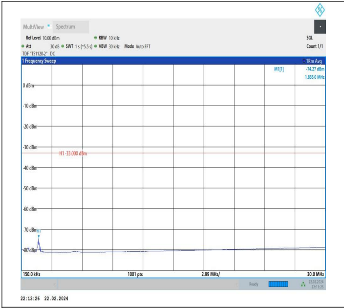
66-66-20MHz-15MHz-QPSK-QPSK-132423-132594-1RB#99-0 RB#0-0.15~30MHz-PASS
