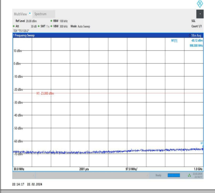
66-66-20MHz-15MHz-QPSK-QPSK-132423-132594-1RB#0-1 RB#74-30~1000MHz-PASS
