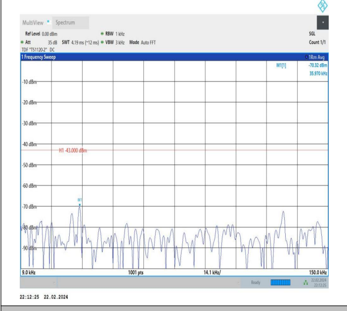
66-66-20MHz-15MHz-QPSK-QPSK-132423-132594-1RB#0-0 RB#0-0.009~0.15MHz-PASS
