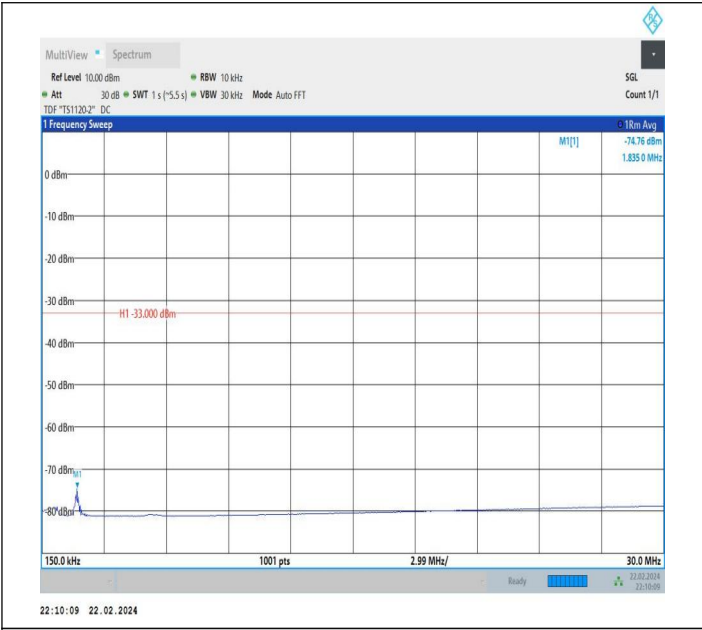
66-66-20MHz-15MHz-QPSK-QPSK-132348-132519-1RB#0-0 RB#0-0.15~30MHz-PASS
