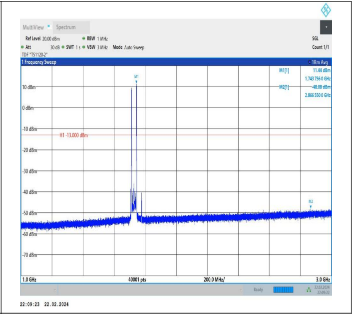
66-66-20MHz-15MHz-QPSK-QPSK-132072-132243-1RB#0-1 RB#74-1000~3000MHz-PASS
