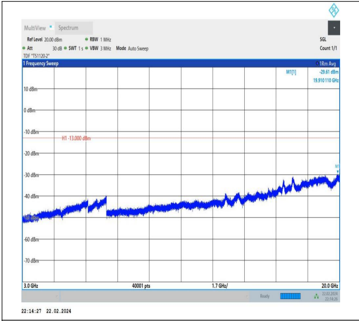
66-66-20MHz-15MHz-QPSK-QPSK-132423-132594-1RB#0-1 RB#74-3000~20000MHz-PASS
