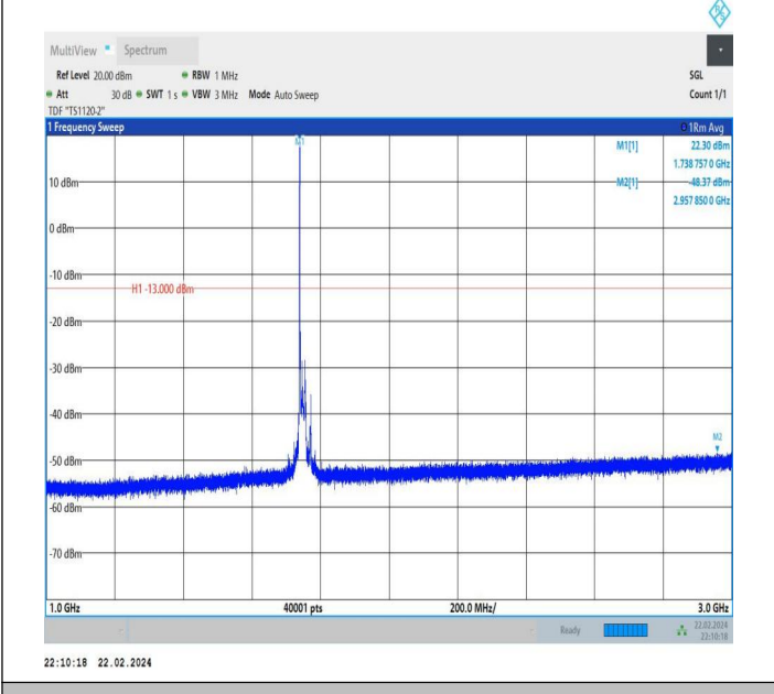
66-66-20MHz-15MHz-QPSK-QPSK-132348-132519-1RB#0-0 RB#0-1000~3000MHz-PASS
