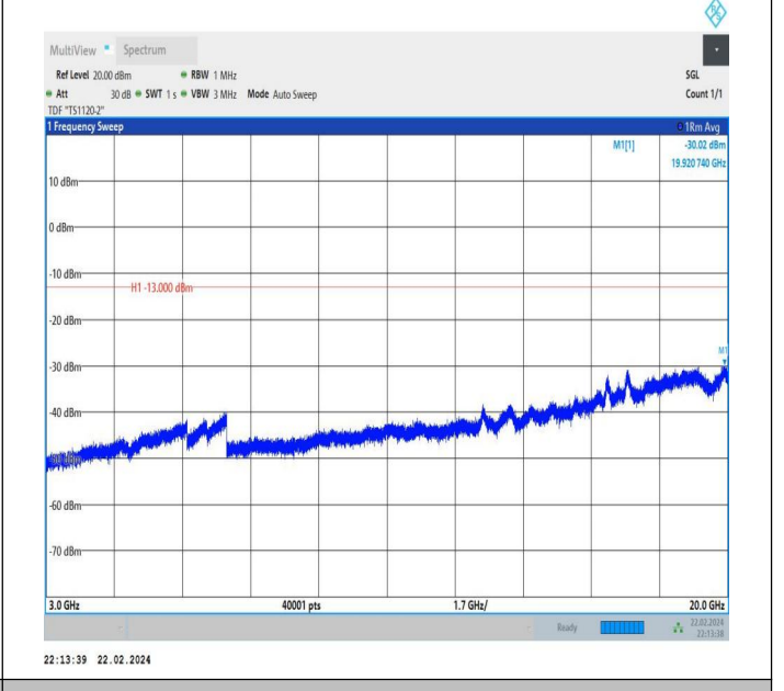
66-66-20MHz-15MHz-QPSK-QPSK-132423-132594-1RB#99-0 RB#0-3000~20000MHz-PASS
