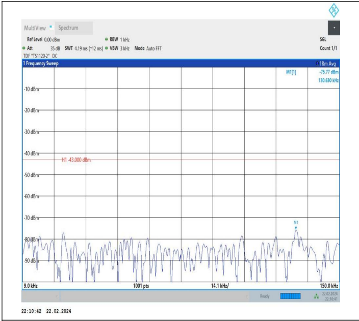
66-66-20MHz-15MHz-QPSK-QPSK-132348-132519-1RB#99-0 RB#0-0.009~0.15MHz-PASS
