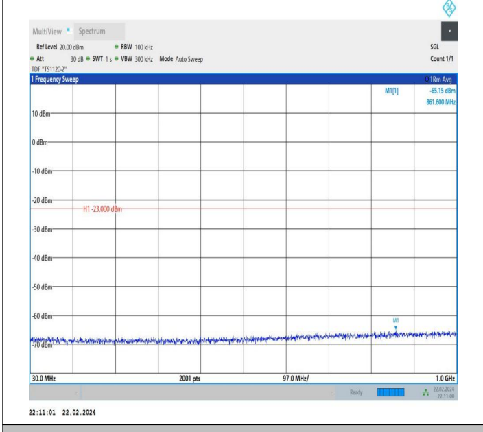
66-66-20MHz-15MHz-QPSK-QPSK-132348-132519-1RB#99-0 RB#0-30~1000MHz-PASS
