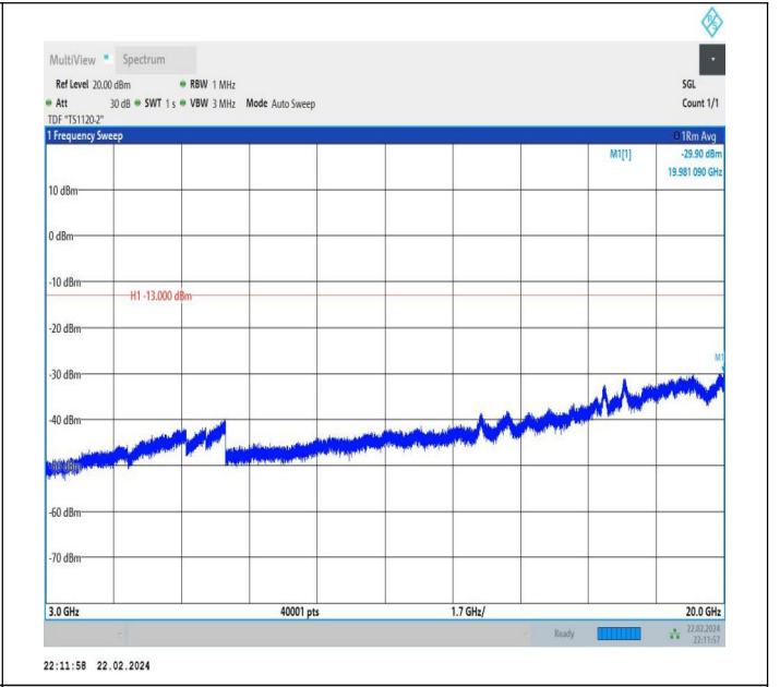
66-66-20MHz-15MHz-QPSK-QPSK-132348-132519-1RB#0-1 RB#74-3000~20000MHz-PASS
