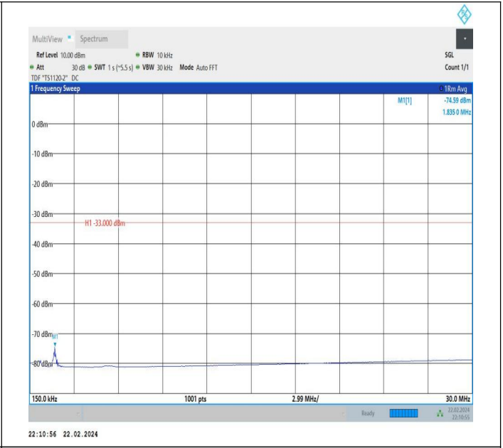
66-66-20MHz-15MHz-QPSK-QPSK-132348-132519-1RB#99-0 RB#0-0.15~30MHz-PASS
