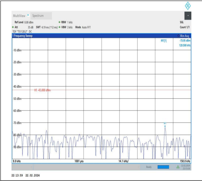
66-66-20MHz-15MHz-QPSK-QPSK-132423-132594-1RB#0-1 RB#74-0.009~0.15MHz-PASS
