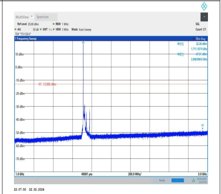
66-66-20MHz-15MHz-QPSK-QPSK-132072-132243-1RB#0-0 RB#0-1000~3000MHz-PASS
