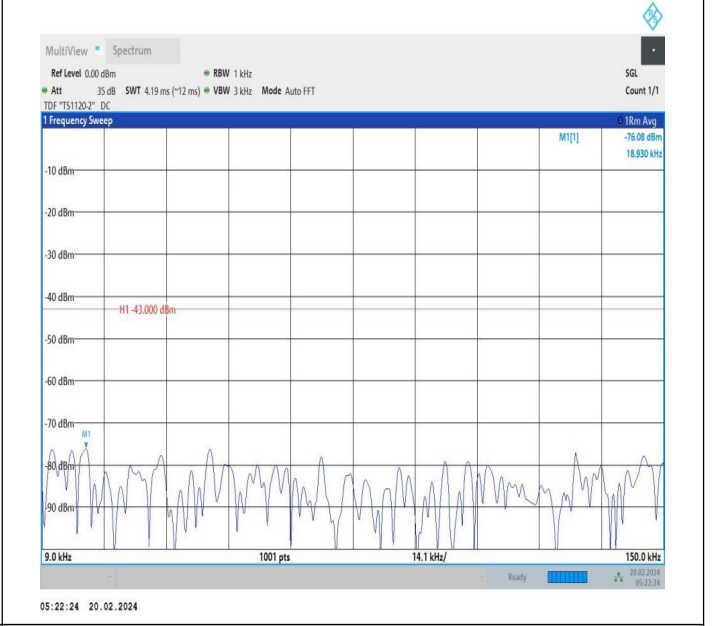
66-66-15MHz-20MHz-QPSK-QPSK-132401-132572-1RB#0-0 RB#0-0.009~0.15MHz-PASS
