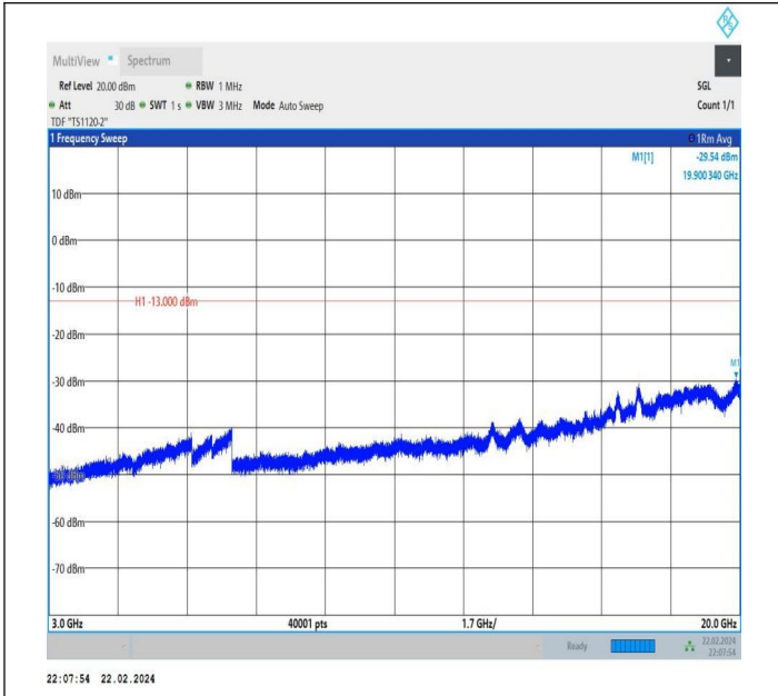
66-66-20MHz-15MHz-QPSK-QPSK-132072-132243-1RB#0-0 RB#0-3000~20000MHz-PASS
