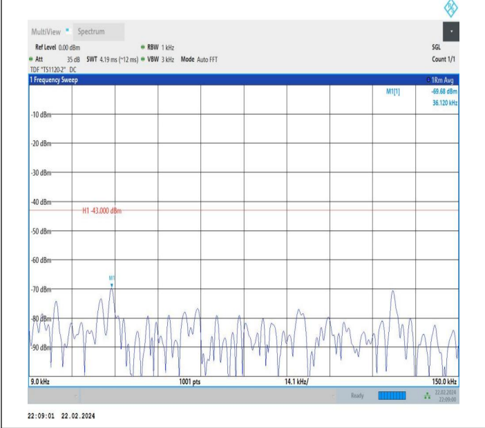
66-66-20MHz-15MHz-QPSK-QPSK-132072-132243-1RB#0-1 RB#74-0.009~0.15MHz-PASS
