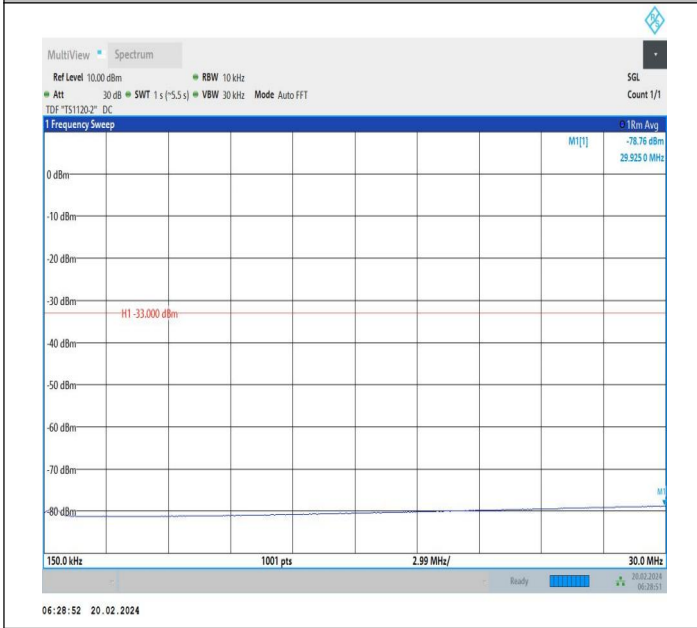
66-66-20MHz-5MHz-QPSK-QPSK-132522-132639-1RB#99-0 RB#0-0.15~30MHz-PASS
