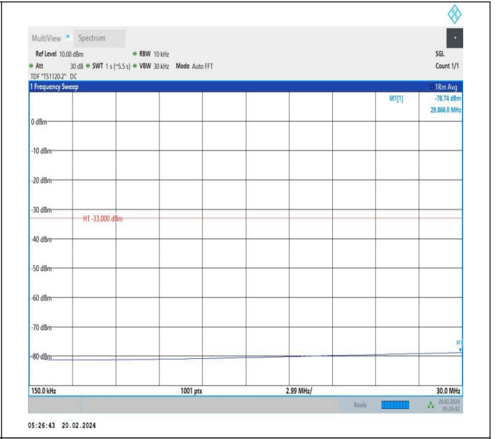
66-66-15MHz-20MHz-QPSK-QPSK-132401-132572-1RB#74-0 RB#0-0.15~30MHz-PASS
