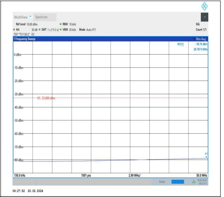
66-66-20MHz-5MHz-QPSK-QPSK-132522-132639-1RB#0-0R B#0-0.15~30MHz-PASS
