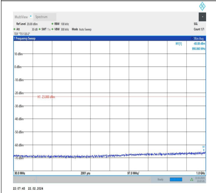
66-66-20MHz-15MHz-QPSK-QPSK-132072-132243-1RB#0-0 RB#0-30~1000MHz-PASS
