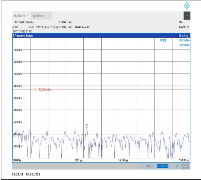
66-66-15MHz-20MHz-QPSK-QPSK-132401-132572-1RB#74-0 RB#0-0.009~0.15MHz-PASS
