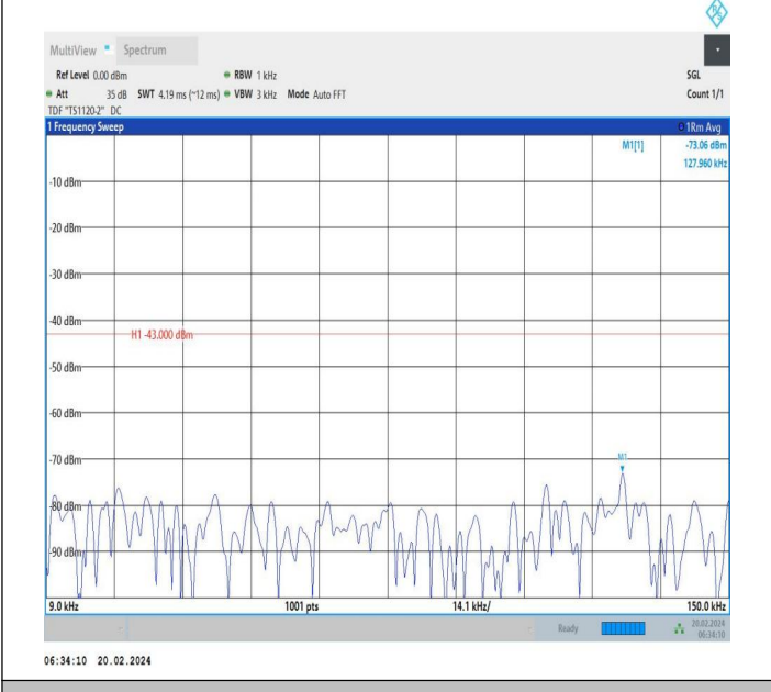
66-66-20MHz-5MHz-QPSK-QPSK-132522-132639-1RB#0-1R B#24-0.009~0.15MHz-PASS
