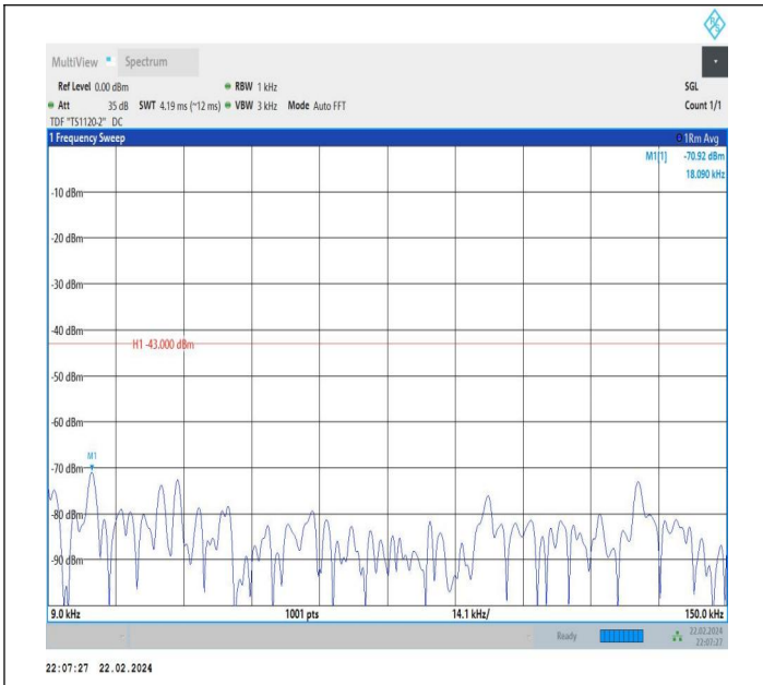
66-66-20MHz-15MHz-QPSK-QPSK-132072-132243-1RB#0-0 RB#0-0.009~0.15MHz-PASS
