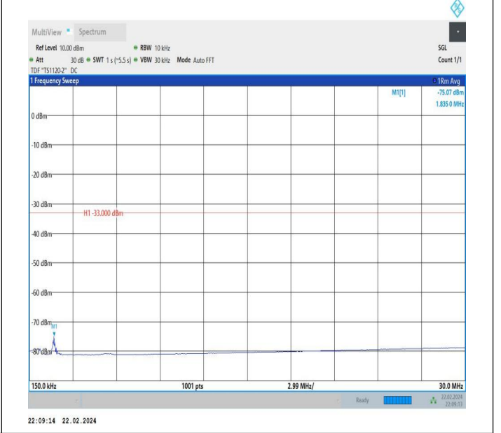
66-66-20MHz-15MHz-QPSK-QPSK-132072-132243-1RB#0-1 RB#74-0.15~30MHz-PASS
