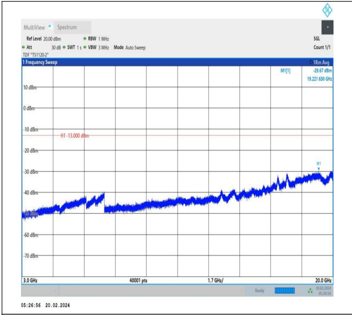
66-66-15MHz-20MHz-QPSK-QPSK-132401-132572-1RB#74-0 RB#0-3000~20000MHz-PASS
