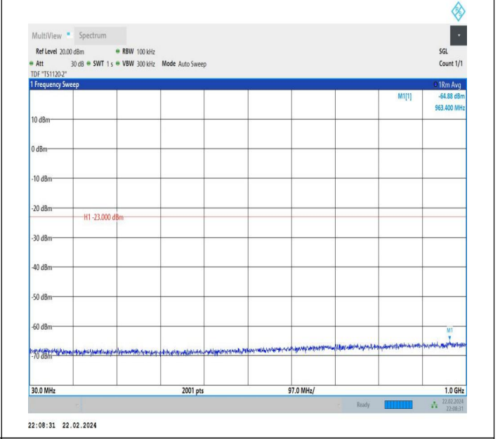
66-66-20MHz-15MHz-QPSK-QPSK-132072-132243-1RB#99-0 RB#0-30~1000MHz-PASS
