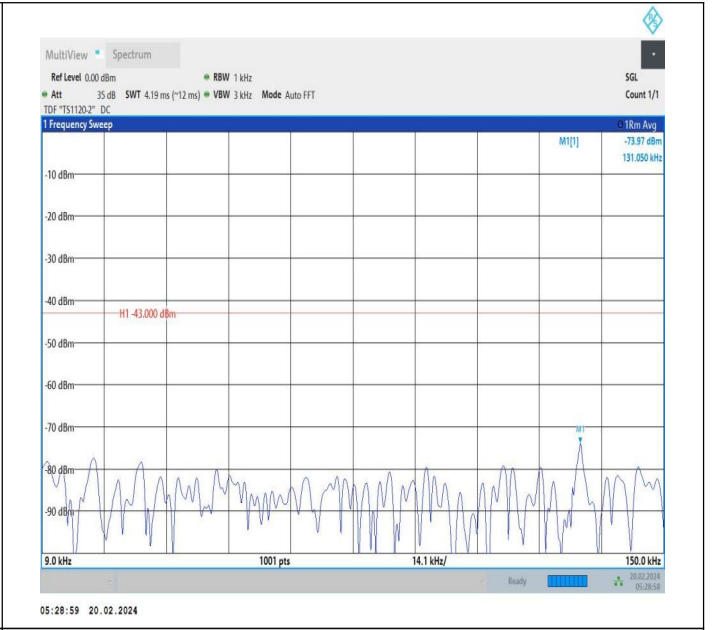
66-66-15MHz-20MHz-QPSK-QPSK-132401-132572-1RB#0-1 RB#99-0.009~0.15MHz-PASS
