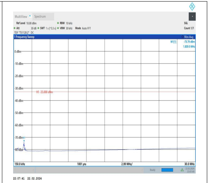
66-66-20MHz-15MHz-QPSK-QPSK-132072-132243-1RB#0-0 RB#0-0.15~30MHz-PASS
