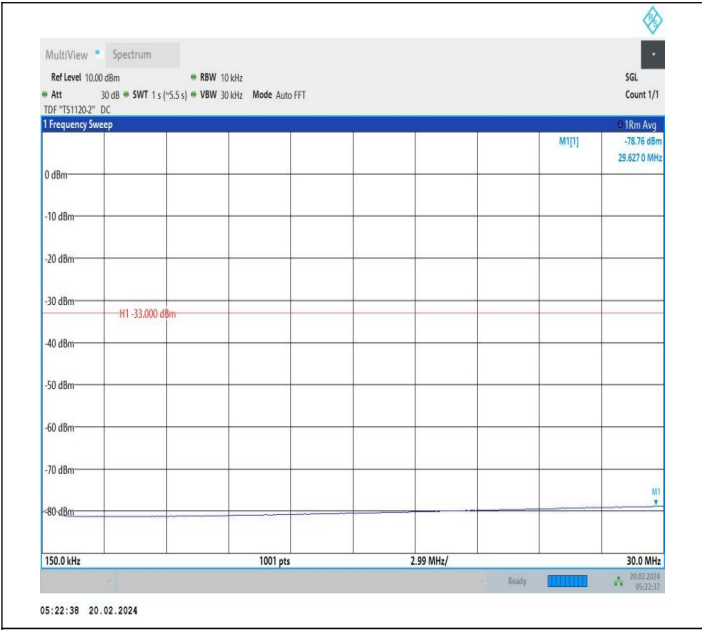
66-66-15MHz-20MHz-QPSK-QPSK-132401-132572-1RB#0-0 RB#0-0.15~30MHz-PASS
