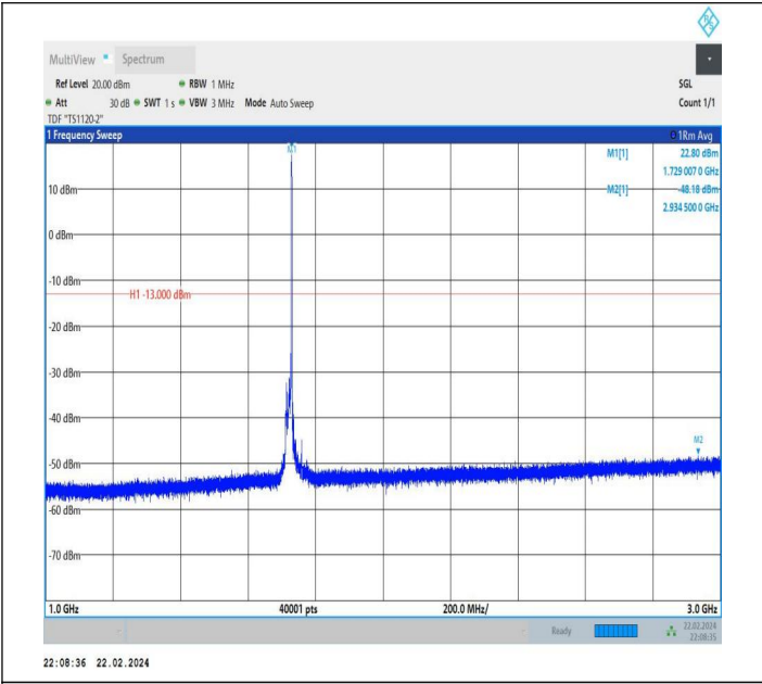
66-66-20MHz-15MHz-QPSK-QPSK-132072-132243-1RB#99-0 RB#0-1000~3000MHz-PASS
