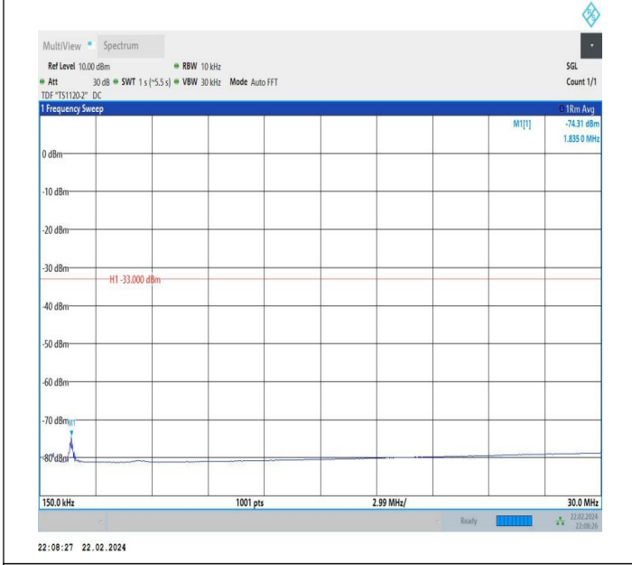
66-66-20MHz-15MHz-QPSK-QPSK-132072-132243-1RB#99-0 RB#0-0.15~30MHz-PASS
