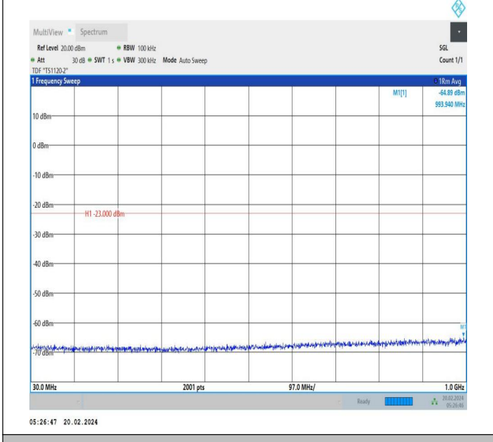
66-66-15MHz-20MHz-QPSK-QPSK-132401-132572-1RB#74-0 RB#0-30~1000MHz-PASS
