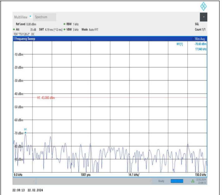
66-66-20MHz-15MHz-QPSK-QPSK-132072-132243-1RB#99-0 RB#0-0.009~0.15MHz-PASS
