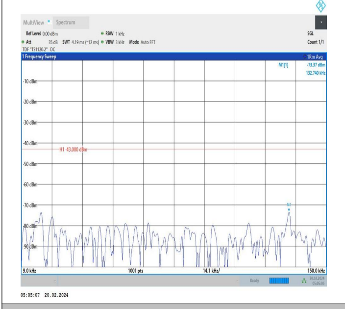
66-66-15MHz-20MHz-QPSK-QPSK-132050-132221-1RB#74-0 RB#0-0.009~0.15MHz-PASS
