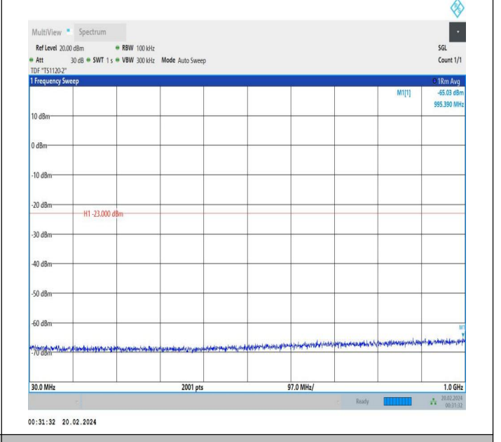
66-66-15MHz-10MHz-QPSK-QPSK-132047-132167-1RB#0-1 RB#49-30~1000MHz-PASS
