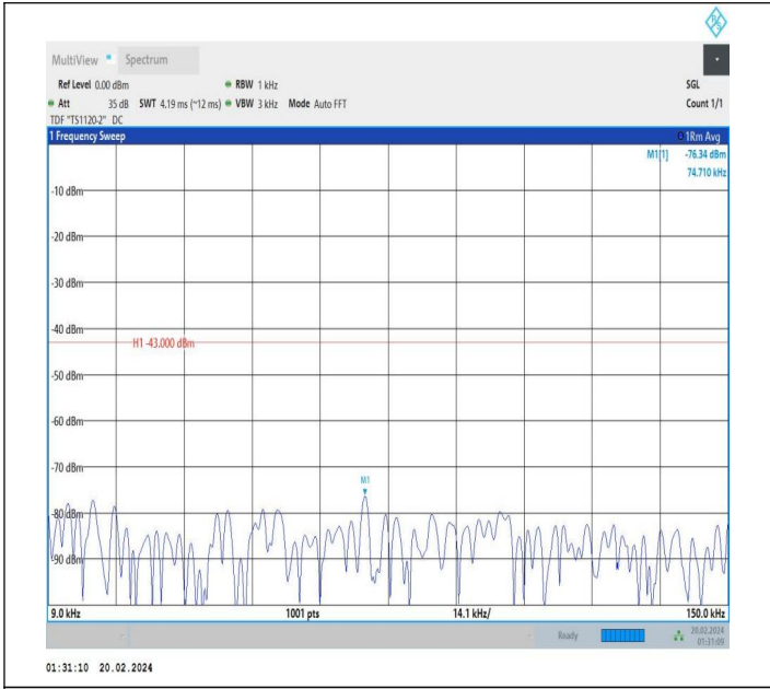
66-66-15MHz-15MHz-QPSK-QPSK-132047-132197-1RB#0-0 RB#0-0.009~0.15MHz-PASS
