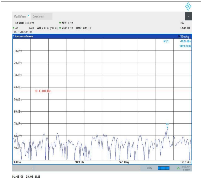
66-66-15MHz-15MHz-QPSK-QPSK-132347-132497-1RB#74-0 RB#0-0.009~0.15MHz-PASS
