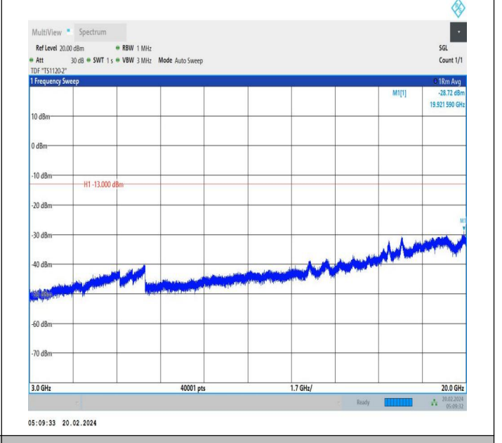
66-66-15MHz-20MHz-QPSK-QPSK-132050-132221-1RB#0-1 RB#99-3000~20000MHz-PASS
