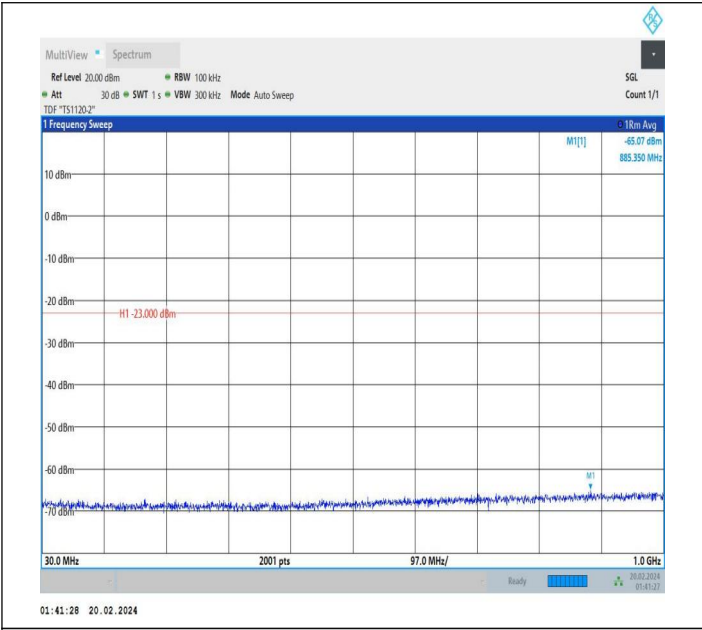
66-66-15MHz-15MHz-QPSK-QPSK-132047-132197-1RB#0-1 RB#74-30~1000MHz-PASS
