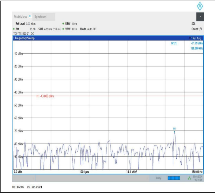
66-66-15MHz-20MHz-QPSK-QPSK-132325-132496-1RB#0-0 RB#0-0.009~0.15MHz-PASS
