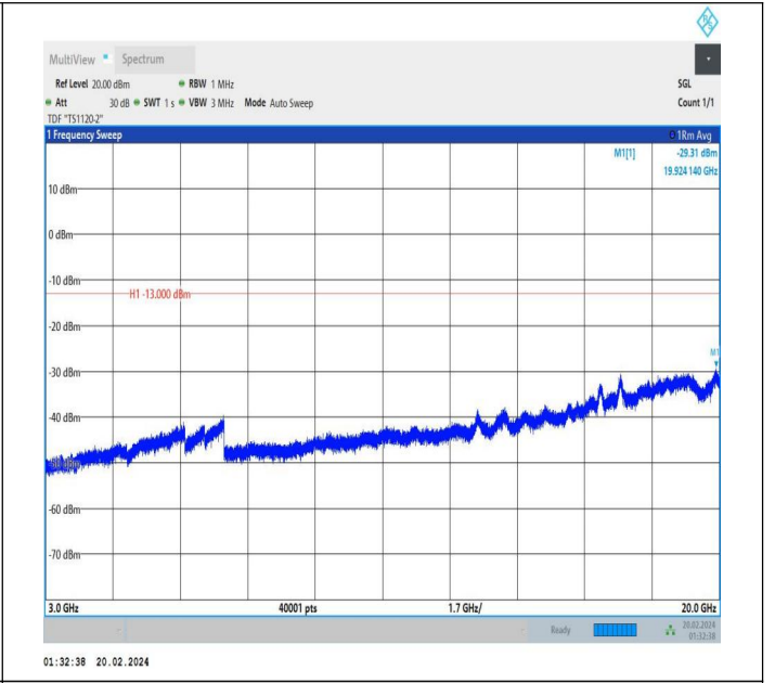
66-66-15MHz-15MHz-QPSK-QPSK-132047-132197-1RB#74-0 RB#0-3000~20000MHz-PASS
