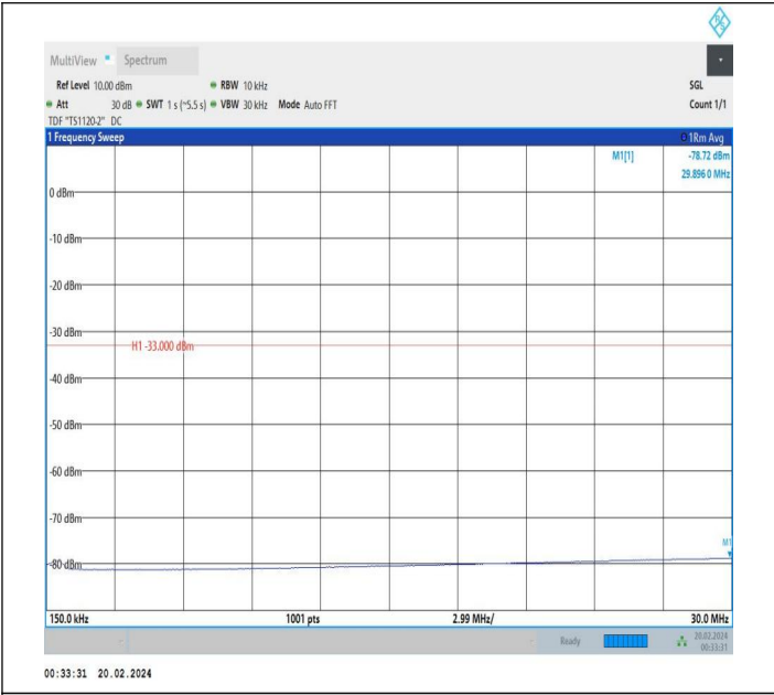
66-66-15MHz-10MHz-QPSK-QPSK-132373-132493-1RB#74-0 RB#0-0.15~30MHz-PASS
