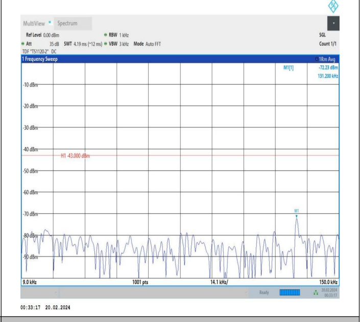
66-66-15MHz-10MHz-QPSK-QPSK-132373-132493-1RB#74-0 RB#0-0.009~0.15MHz-PASS
