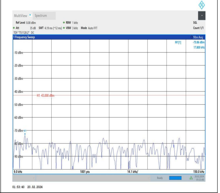
66-66-15MHz-15MHz-QPSK-QPSK-132447-132597-1RB#74-0 RB#0-0.009~0.15MHz-PASS
