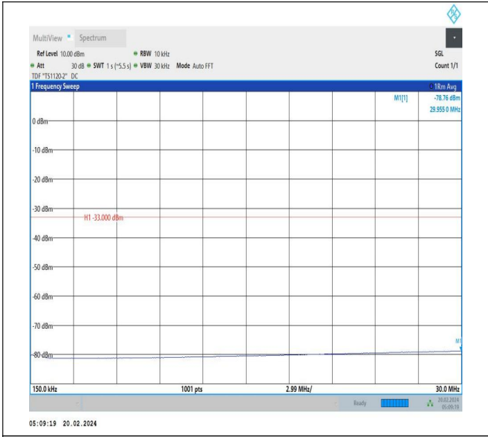
66-66-15MHz-20MHz-QPSK-QPSK-132050-132221-1RB#0-1 RB#99-0.15~30MHz-PASS
