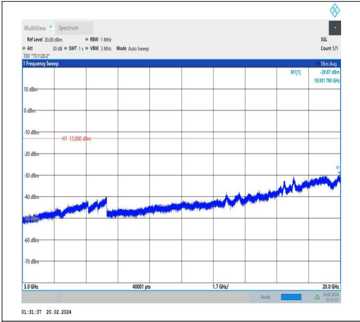
66-66-15MHz-15MHz-QPSK-QPSK-132047-132197-1RB#0-0 RB#0-3000~20000MHz-PASS
