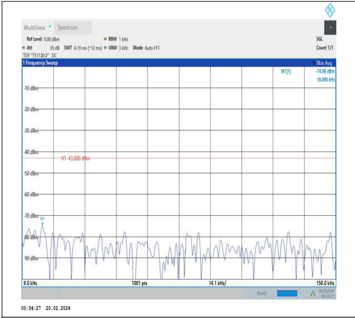
66-66-15MHz-10MHz-QPSK-QPSK-132373-132493-1RB#0-1 RB#49-0.009~0.15MHz-PASS
