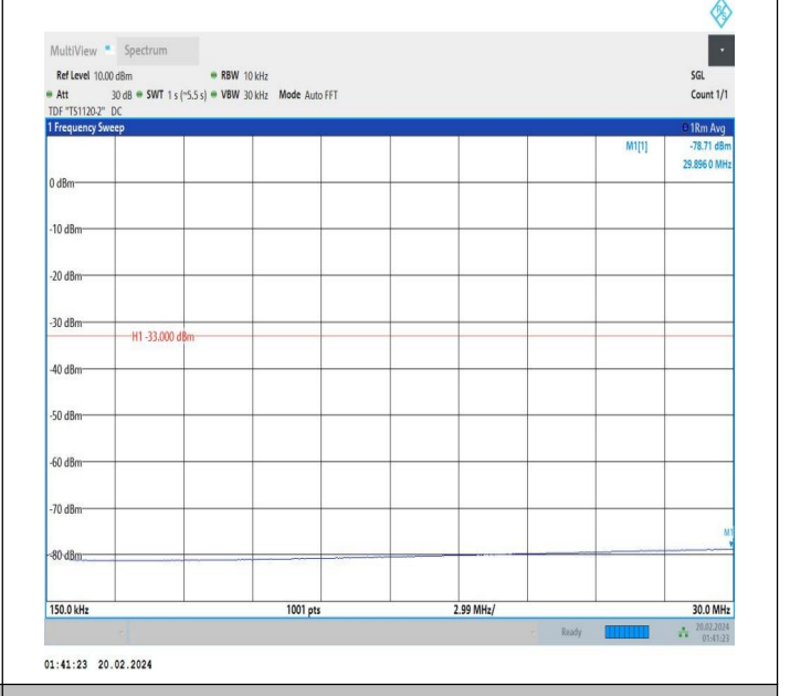
66-66-15MHz-15MHz-QPSK-QPSK-132047-132197-1RB#0-1 RB#74-0.15~30MHz-PASS
