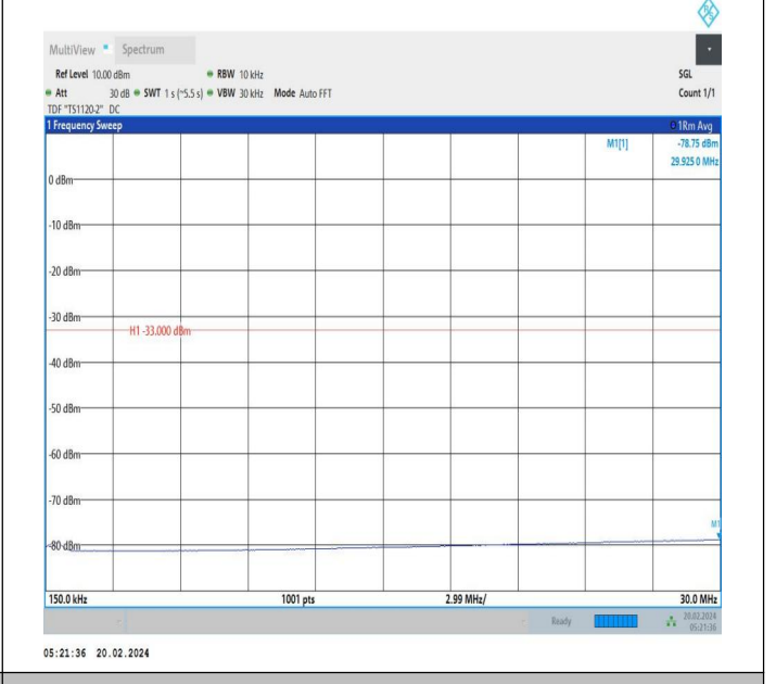
66-66-15MHz-20MHz-QPSK-QPSK-132325-132496-1RB#0-1 RB#99-0.15~30MHz-PASS
