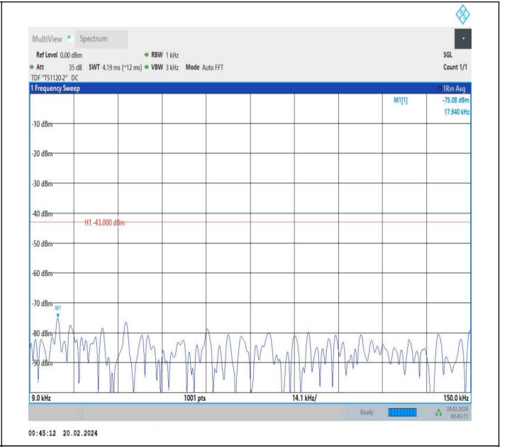
66-66-15MHz-10MHz-QPSK-QPSK-132499-132619-1RB#0-0 RB#0-0.009~0.15MHz-PASS
