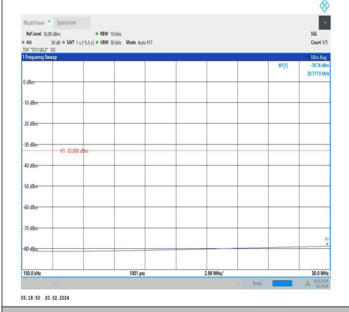
66-66-15MHz-20MHz-QPSK-QPSK-132325-132496-1RB#74-0 RB#0-0.15~30MHz-PASS
