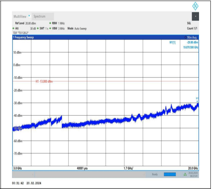
66-66-15MHz-10MHz-QPSK-QPSK-132047-132167-1RB#0-1 RB#49-3000~20000MHz-PASS
