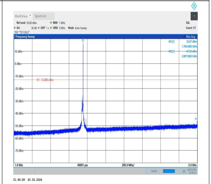
66-66-15MHz-15MHz-QPSK-QPSK-132347-132497-1RB#74-0 RB#0-1000~3000MHz-PASS
