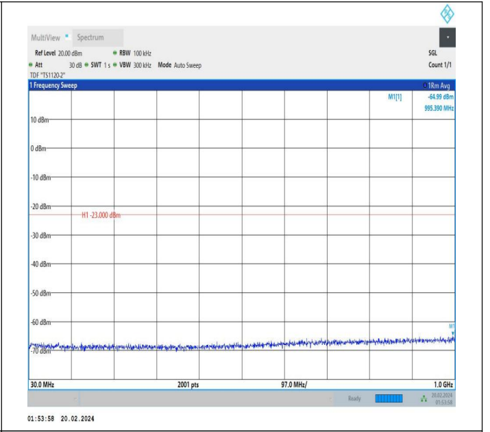
66-66-15MHz-15MHz-QPSK-QPSK-132447-132597-1RB#74-0 RB#0-30~1000MHz-PASS
