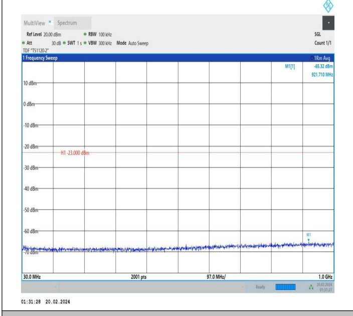
66-66-15MHz-15MHz-QPSK-QPSK-132047-132197-1RB#0-0 RB#0-30~1000MHz-PASS
