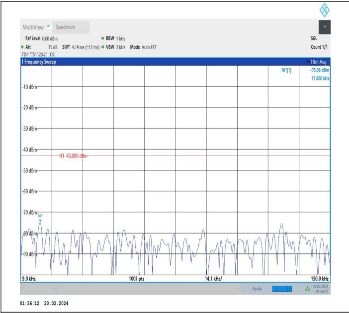
66-66-15MHz-15MHz-QPSK-QPSK-132447-132597-1RB#0-1 RB#74-0.009~0.15MHz-PASS
