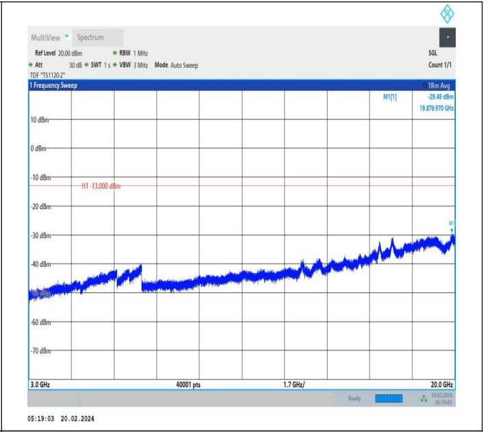
66-66-15MHz-20MHz-QPSK-QPSK-132325-132496-1RB#74-0 RB#0-3000~20000MHz-PASS
