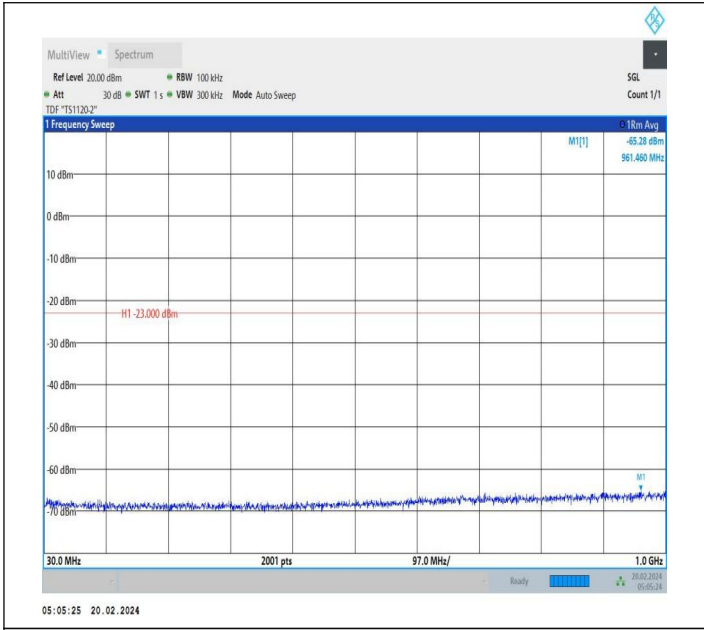
66-66-15MHz-20MHz-QPSK-QPSK-132050-132221-1RB#74-0 RB#0-30~1000MHz-PASS
