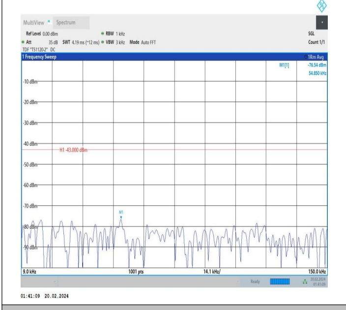
66-66-15MHz-15MHz-QPSK-QPSK-132047-132197-1RB#0-1 RB#74-0.009~0.15MHz-PASS
