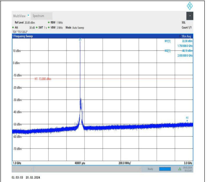
66-66-15MHz-15MHz-QPSK-QPSK-132447-132597-1RB#0-0 RB#0-1000~3000MHz-PASS
