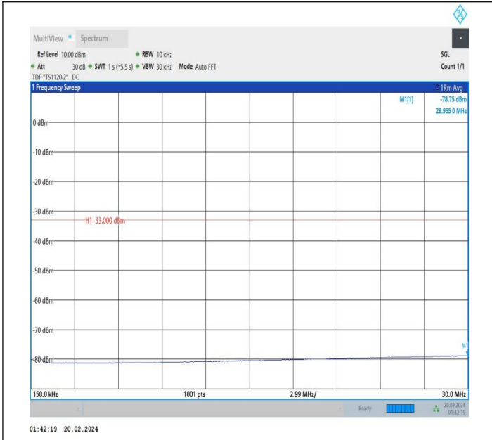
66-66-15MHz-15MHz-QPSK-QPSK-132347-132497-1RB#0-0 RB#0-0.15~30MHz-PASS
