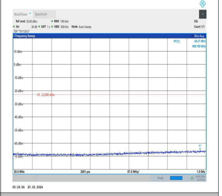
66-66-15MHz-20MHz-QPSK-QPSK-132325-132496-1RB#74-0 RB#0-30~1000MHz-PASS
