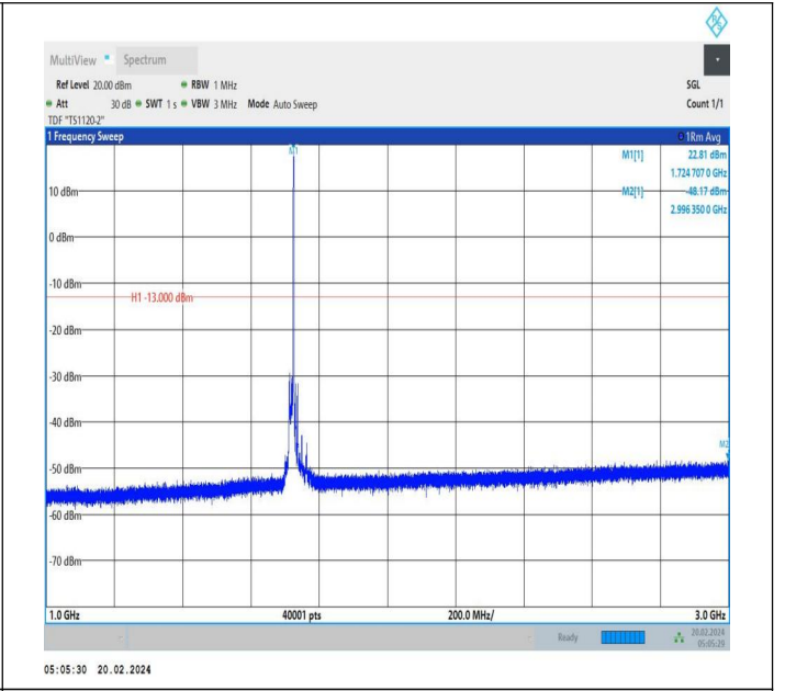
66-66-15MHz-20MHz-QPSK-QPSK-132050-132221-1RB#74-0 RB#0-1000~3000MHz-PASS
