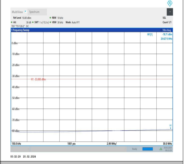
66-66-15MHz-10MHz-QPSK-QPSK-132373-132493-1RB#0-0 RB#0-0.15~30MHz-PASS
