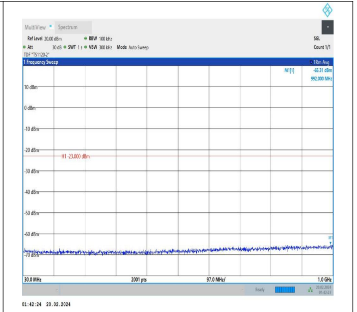
66-66-15MHz-15MHz-QPSK-QPSK-132347-132497-1RB#0-0 RB#0-30~1000MHz-PASS
