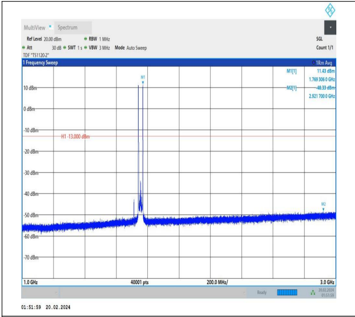
66-66-15MHz-15MHz-QPSK-QPSK-132347-132497-1RB#0-1 RB#74-1000~3000MHz-PASS
