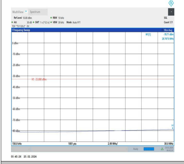
66-66-15MHz-10MHz-QPSK-QPSK-132499-132619-1RB#0-0 RB#0-0.15~30MHz-PASS
