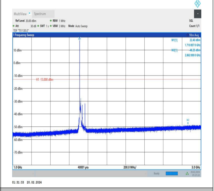
66-66-15MHz-15MHz-QPSK-QPSK-132047-132197-1RB#0-0 RB#0-1000~3000MHz-PASS
