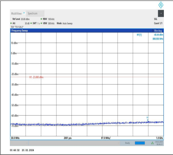
66-66-15MHz-10MHz-QPSK-QPSK-132499-132619-1RB#74-0 RB#0-30~1000MHz-PASS
