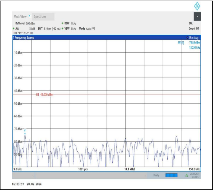
66-66-15MHz-20MHz-QPSK-QPSK-132050-132221-1RB#0-0 RB#0-0.009~0.15MHz-PASS
