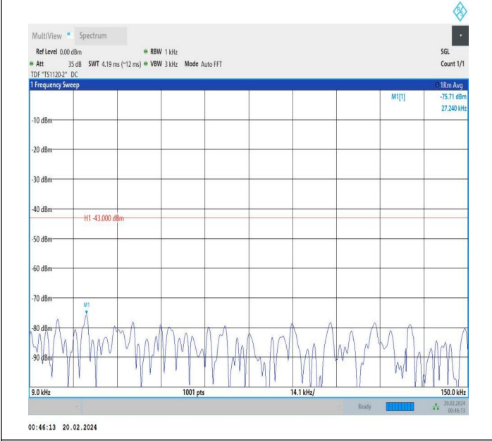
66-66-15MHz-10MHz-QPSK-QPSK-132499-132619-1RB#74-0 RB#0-0.009~0.15MHz-PASS
