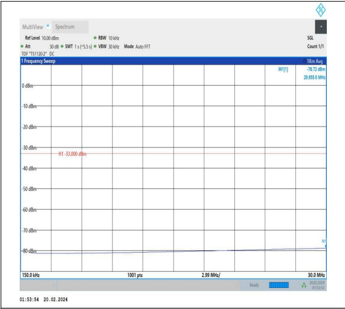
66-66-15MHz-15MHz-QPSK-QPSK-132447-132597-1RB#74-0 RB#0-0.15~30MHz-PASS
