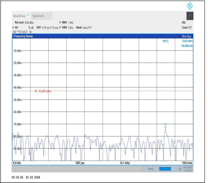
66-66-15MHz-20MHz-QPSK-QPSK-132325-132496-1RB#74-0 RB#0-0.009~0.15MHz-PASS
