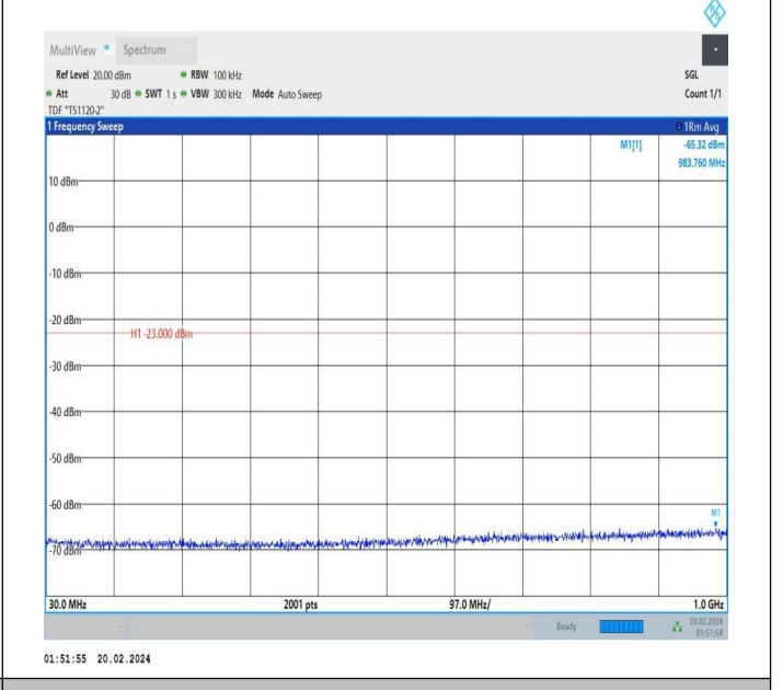
66-66-15MHz-15MHz-QPSK-QPSK-132347-132497-1RB#0-1 RB#74-30~1000MHz-PASS
