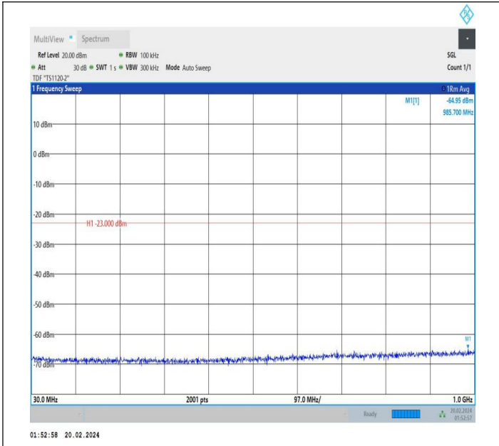
66-66-15MHz-15MHz-QPSK-QPSK-132447-132597-1RB#0-0 RB#0-30~1000MHz-PASS
