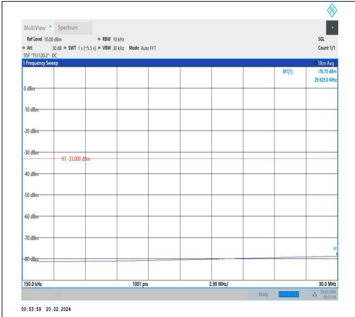
66-66-15MHz-10MHz-QPSK-QPSK-132499-132619-1RB#0-1 RB#49-0.15~30MHz-PASS
