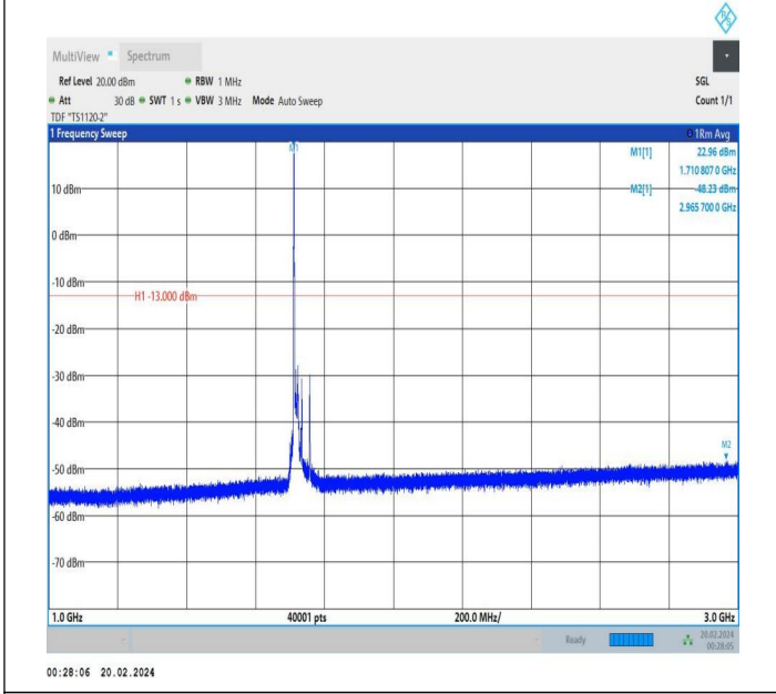
66-66-15MHz-10MHz-QPSK-QPSK-132047-132167-1RB#0-0 RB#0-1000~3000MHz-PASS
