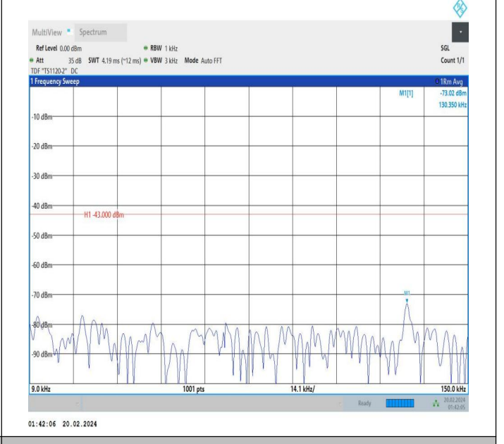
66-66-15MHz-15MHz-QPSK-QPSK-132347-132497-1RB#0-0 RB#0-0.009~0.15MHz-PASS
