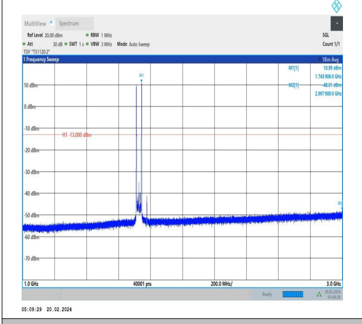
66-66-15MHz-20MHz-QPSK-QPSK-132050-132221-1RB#0-1 RB#99-1000~3000MHz-PASS
