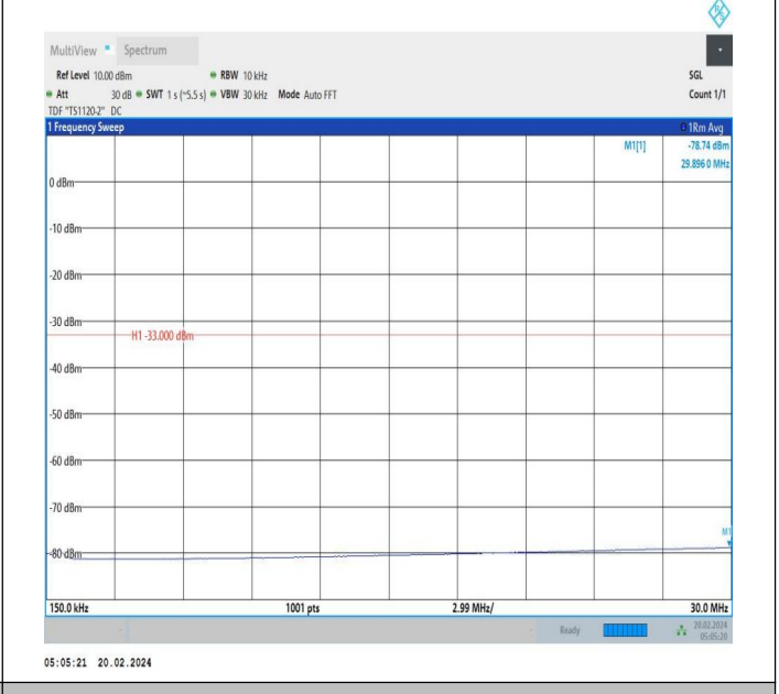
66-66-15MHz-20MHz-QPSK-QPSK-132050-132221-1RB#74-0 RB#0-0.15~30MHz-PASS
