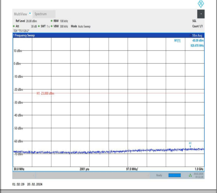
66-66-15MHz-15MHz-QPSK-QPSK-132047-132197-1RB#74-0 RB#0-30~1000MHz-PASS
