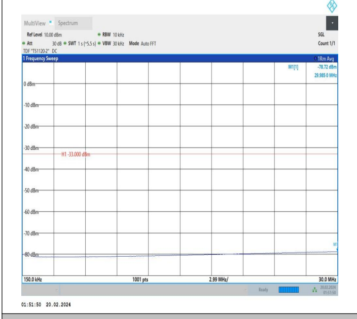
66-66-15MHz-15MHz-QPSK-QPSK-132347-132497-1RB#0-1 RB#74-0.15~30MHz-PASS
