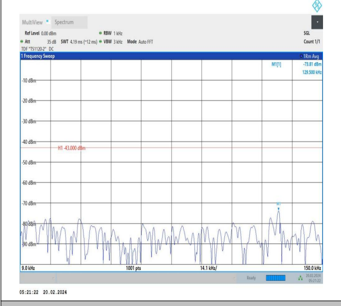
66-66-15MHz-20MHz-QPSK-QPSK-132325-132496-1RB#0-1 RB#99-0.009~0.15MHz-PASS
