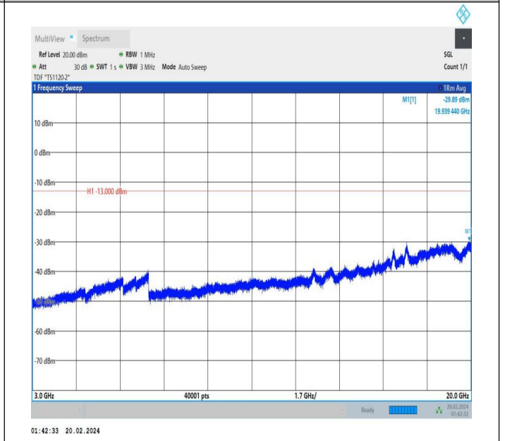
66-66-15MHz-15MHz-QPSK-QPSK-132347-132497-1RB#0-0 RB#0-3000~20000MHz-PASS
