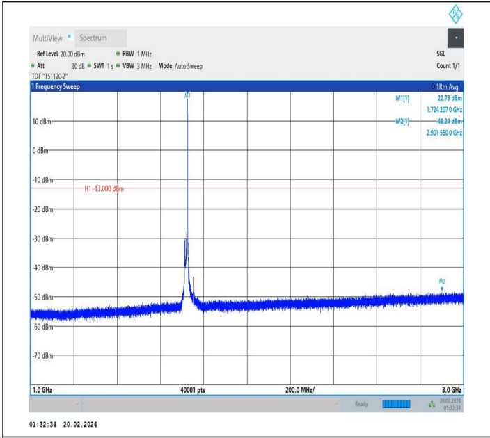
66-66-15MHz-15MHz-QPSK-QPSK-132047-132197-1RB#74-0 RB#0-1000~3000MHz-PASS
