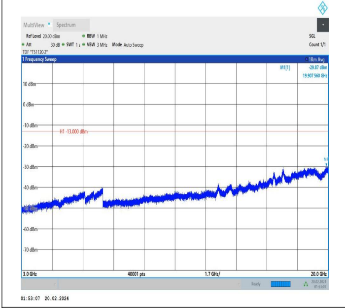
66-66-15MHz-15MHz-QPSK-QPSK-132447-132597-1RB#0-0 RB#0-3000~20000MHz-PASS
