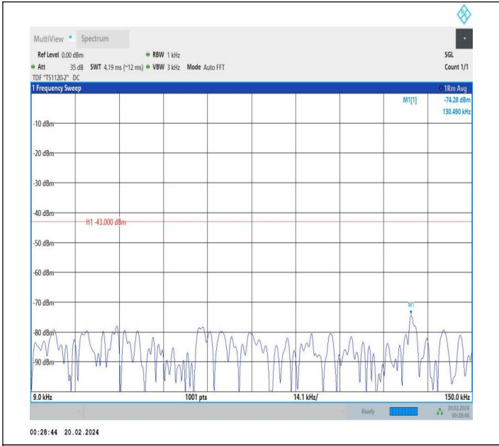
66-66-15MHz-10MHz-QPSK-QPSK-132047-132167-1RB#74-0 RB#0-0.009~0.15MHz-PASS
