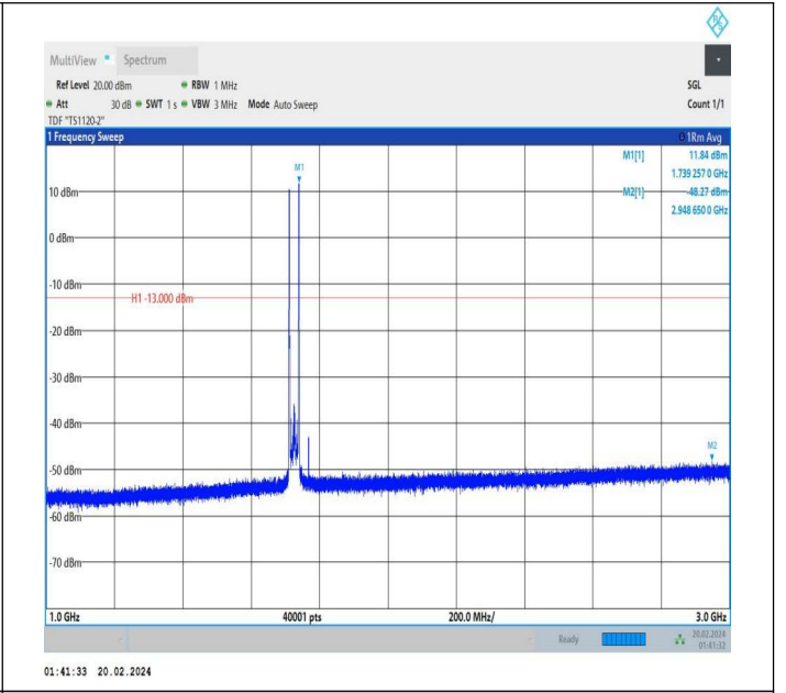
66-66-15MHz-15MHz-QPSK-QPSK-132047-132197-1RB#0-1 RB#74-1000~3000MHz-PASS
