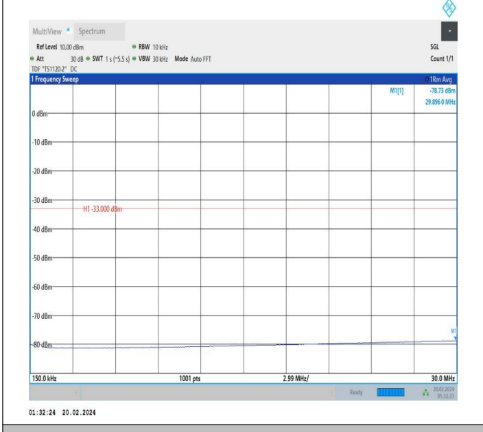
66-66-15MHz-15MHz-QPSK-QPSK-132047-132197-1RB#74-0 RB#0-0.15~30MHz-PASS
