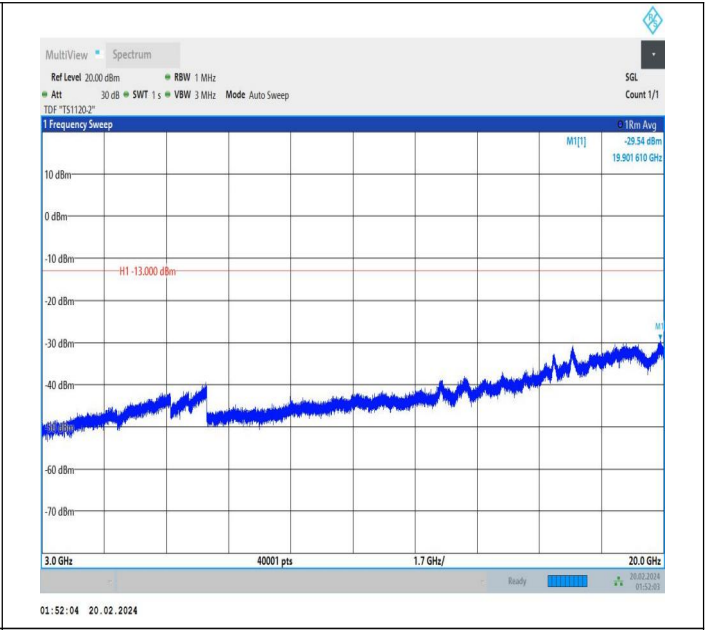
66-66-15MHz-15MHz-QPSK-QPSK-132347-132497-1RB#0-1 RB#74-3000~20000MHz-PASS
