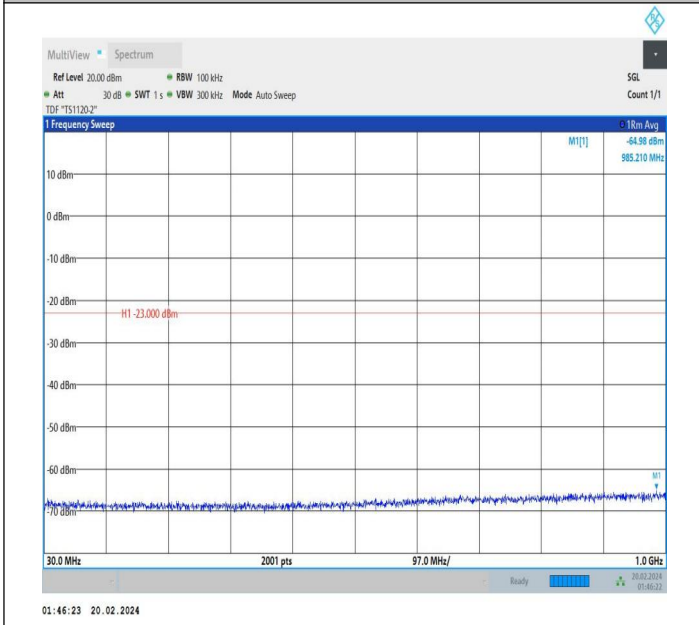
66-66-15MHz-15MHz-QPSK-QPSK-132347-132497-1RB#74-0 RB#0-30~1000MHz-PASS
