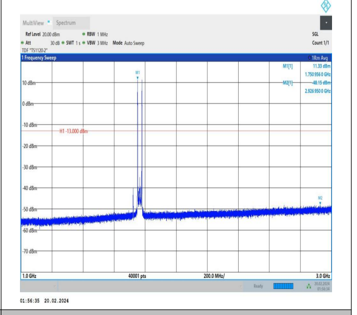
66-66-15MHz-15MHz-QPSK-QPSK-132447-132597-1RB#0-1 RB#74-1000~3000MHz-PASS
