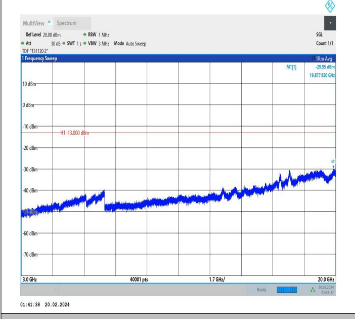
66-66-15MHz-15MHz-QPSK-QPSK-132047-132197-1RB#0-1 RB#74-3000~20000MHz-PASS
