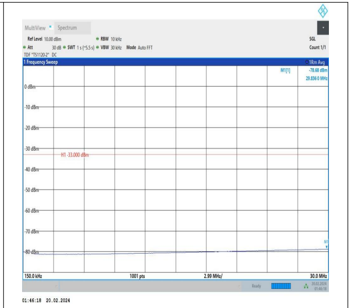
66-66-15MHz-15MHz-QPSK-QPSK-132347-132497-1RB#74-0 RB#0-0.15~30MHz-PASS
