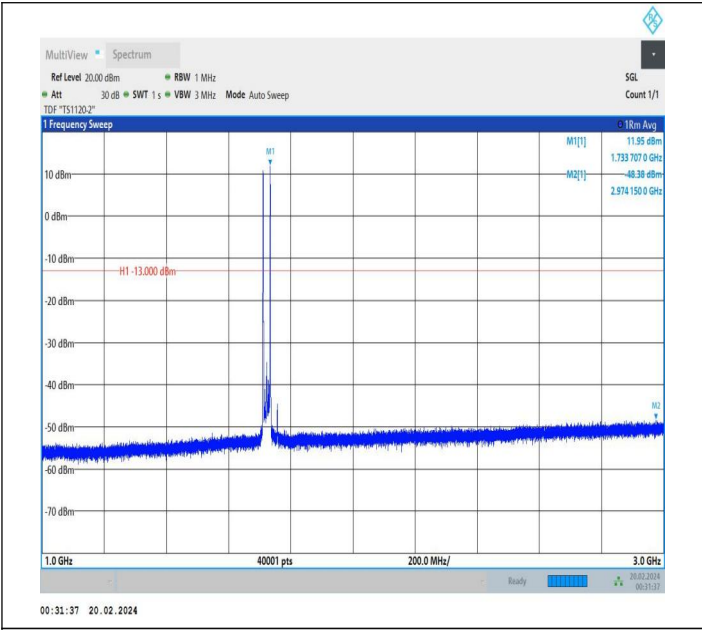
66-66-15MHz-10MHz-QPSK-QPSK-132047-132167-1RB#0-1 RB#49-1000~3000MHz-PASS
