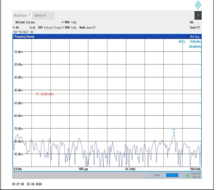
66-66-15MHz-10MHz-QPSK-QPSK-132047-132167-1RB#0-0 RB#0-0.009~0.15MHz-PASS
