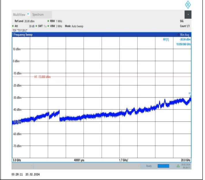
66-66-15MHz-10MHz-QPSK-QPSK-132047-132167-1RB#0-0 RB#0-3000~20000MHz-PASS
