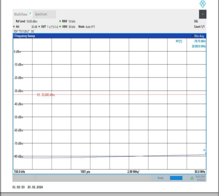
66-66-15MHz-15MHz-QPSK-QPSK-132447-132597-1RB#0-0 RB#0-0.15~30MHz-PASS
