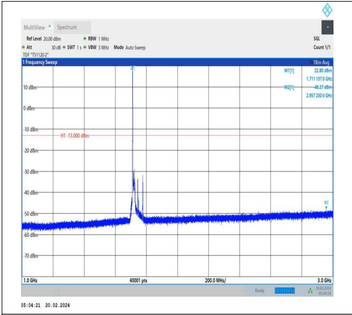
66-66-15MHz-20MHz-QPSK-QPSK-132050-132221-1RB#0-0 RB#0-1000~3000MHz-PASS
