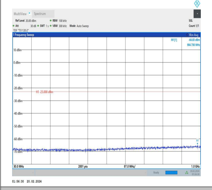
66-66-15MHz-15MHz-QPSK-QPSK-132447-132597-1RB#0-1 RB#74-30~1000MHz-PASS
