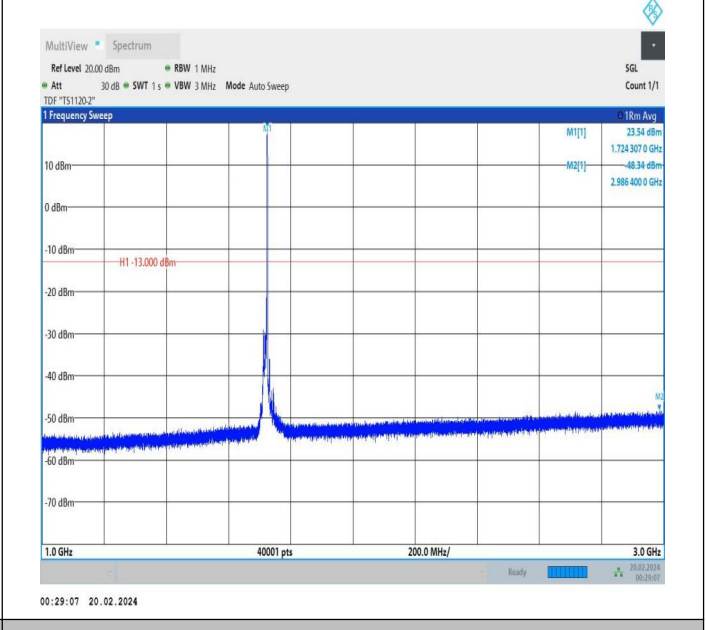
66-66-15MHz-10MHz-QPSK-QPSK-132047-132167-1RB#74-0 RB#0-1000~3000MHz-PASS
