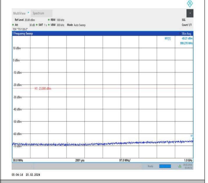
66-66-15MHz-20MHz-QPSK-QPSK-132050-132221-1RB#0-0 RB#0-30~1000MHz-PASS
