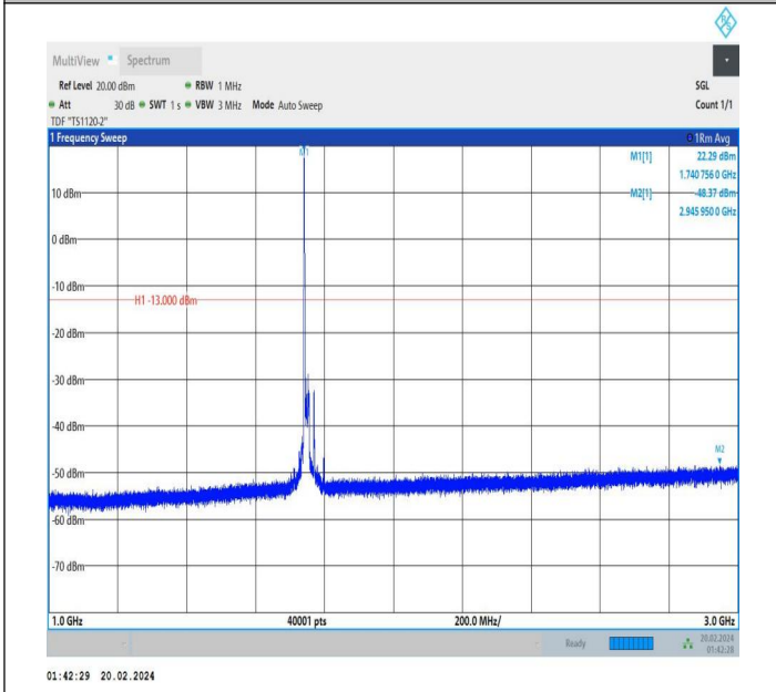
66-66-15MHz-15MHz-QPSK-QPSK-132347-132497-1RB#0-0 RB#0-1000~3000MHz-PASS
