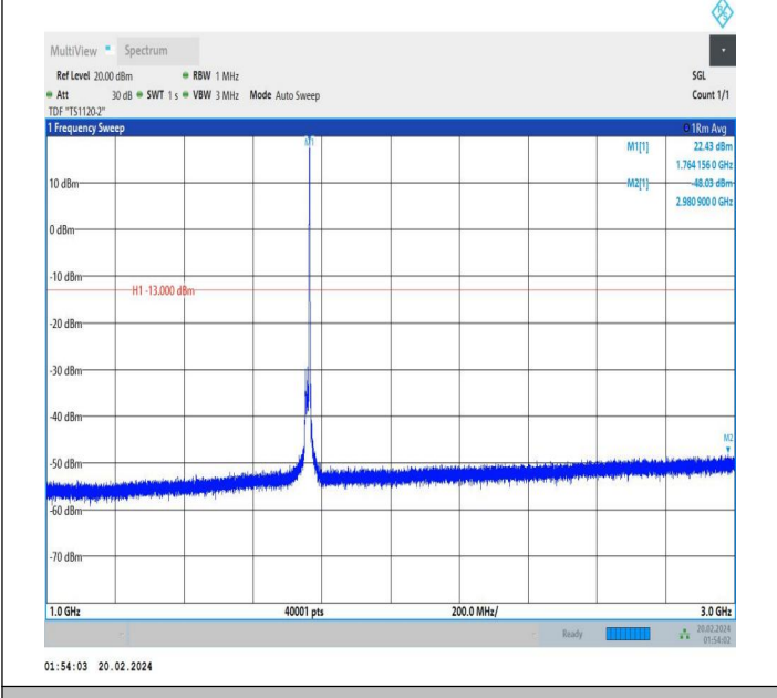
66-66-15MHz-15MHz-QPSK-QPSK-132447-132597-1RB#74-0 RB#0-1000~3000MHz-PASS
