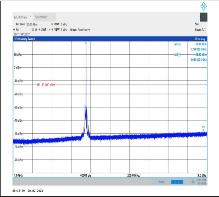
66-66-15MHz-20MHz-QPSK-QPSK-132325-132496-1RB#74-0 RB#0-1000~3000MHz-PASS
