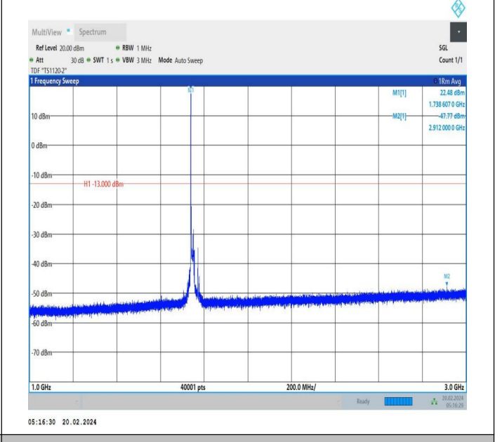
66-66-15MHz-20MHz-QPSK-QPSK-132325-132496-1RB#0-0 RB#0-1000~3000MHz-PASS
