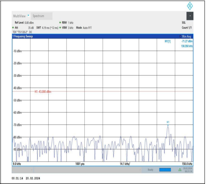
66-66-15MHz-10MHz-QPSK-QPSK-132047-132167-1RB#0-1 RB#49-0.009~0.15MHz-PASS
