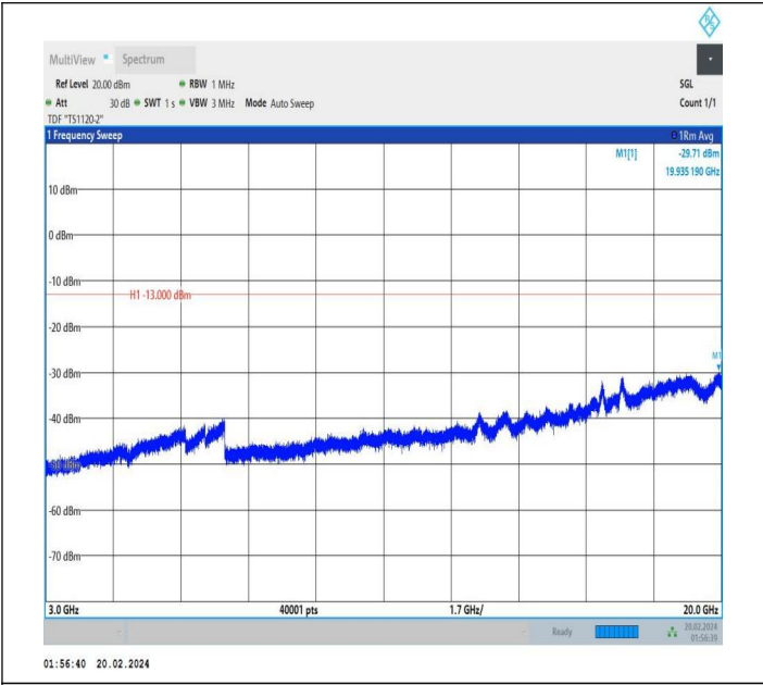
66-66-15MHz-15MHz-QPSK-QPSK-132447-132597-1RB#0-1 RB#74-3000~20000MHz-PASS
