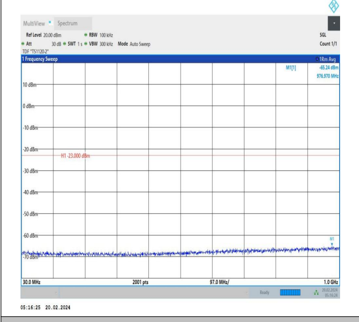
66-66-15MHz-20MHz-QPSK-QPSK-132325-132496-1RB#0-0 RB#0-30~1000MHz-PASS
