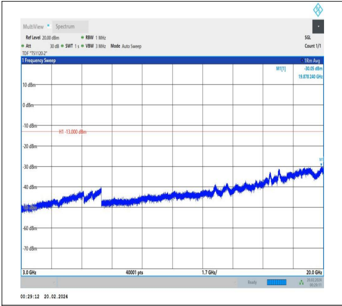
66-66-15MHz-10MHz-QPSK-QPSK-132047-132167-1RB#74-0 RB#0-3000~20000MHz-PASS
