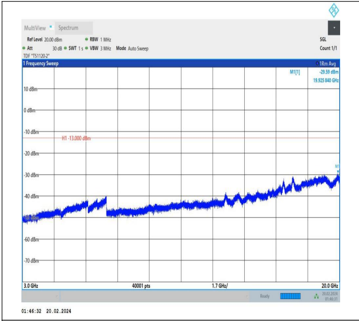
66-66-15MHz-15MHz-QPSK-QPSK-132347-132497-1RB#74-0 RB#0-3000~20000MHz-PASS
