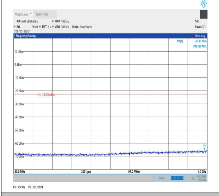
66-66-15MHz-10MHz-QPSK-QPSK-132047-132167-1RB#74-0 RB#0-30~1000MHz-PASS
