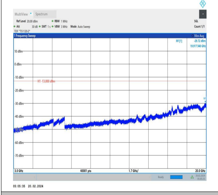
66-66-15MHz-20MHz-QPSK-QPSK-132050-132221-1RB#74-0 RB#0-3000~20000MHz-PASS
