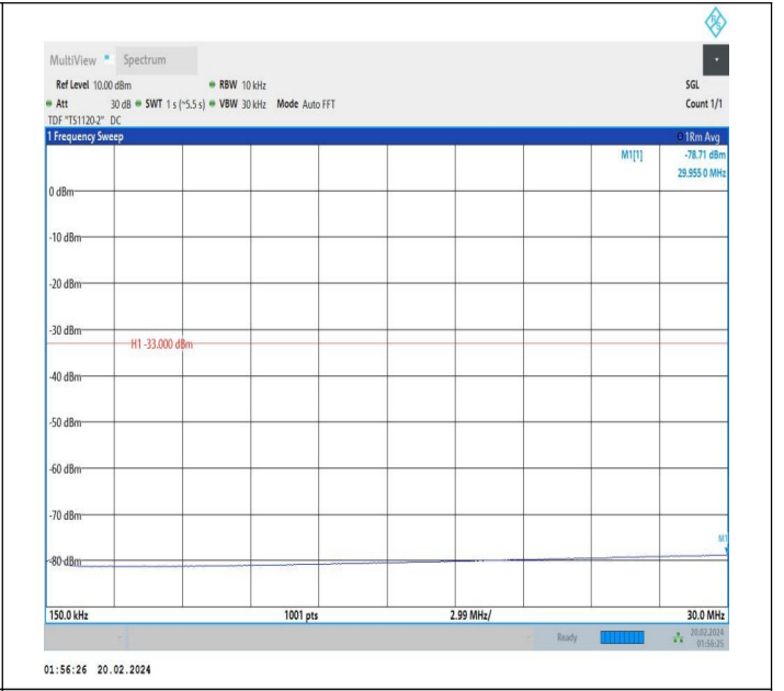
66-66-15MHz-15MHz-QPSK-QPSK-132447-132597-1RB#0-1 RB#74-0.15~30MHz-PASS
