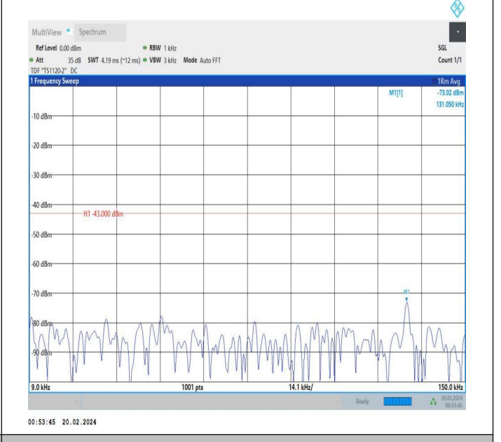
66-66-15MHz-10MHz-QPSK-QPSK-132499-132619-1RB#0-1 RB#49-0.009~0.15MHz-PASS
