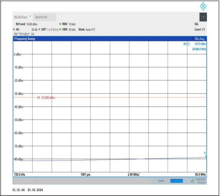
66-66-15MHz-15MHz-QPSK-QPSK-132047-132197-1RB#0-0 RB#0-0.15~30MHz-PASS
