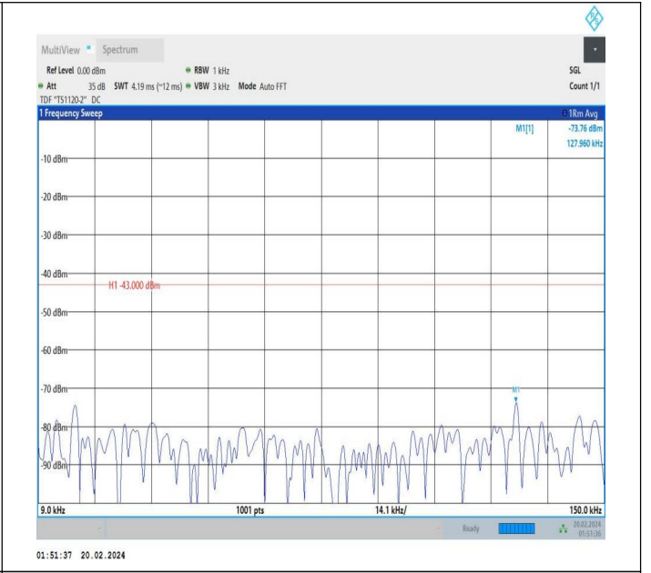
66-66-15MHz-15MHz-QPSK-QPSK-132347-132497-1RB#0-1 RB#74-0.009~0.15MHz-PASS
