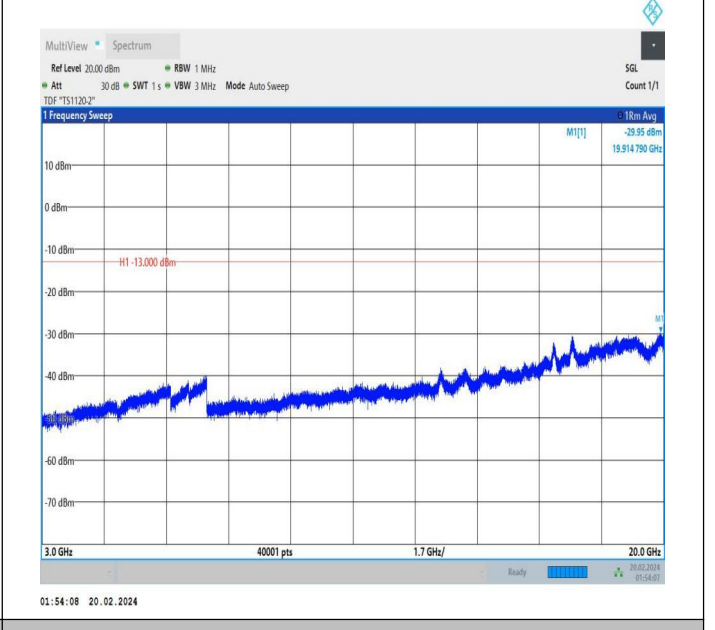
66-66-15MHz-15MHz-QPSK-QPSK-132447-132597-1RB#74-0 RB#0-3000~20000MHz-PASS
