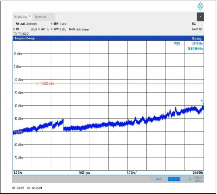
66-66-15MHz-20MHz-QPSK-QPSK-132050-132221-1RB#0-0 RB#0-3000~20000MHz-PASS
