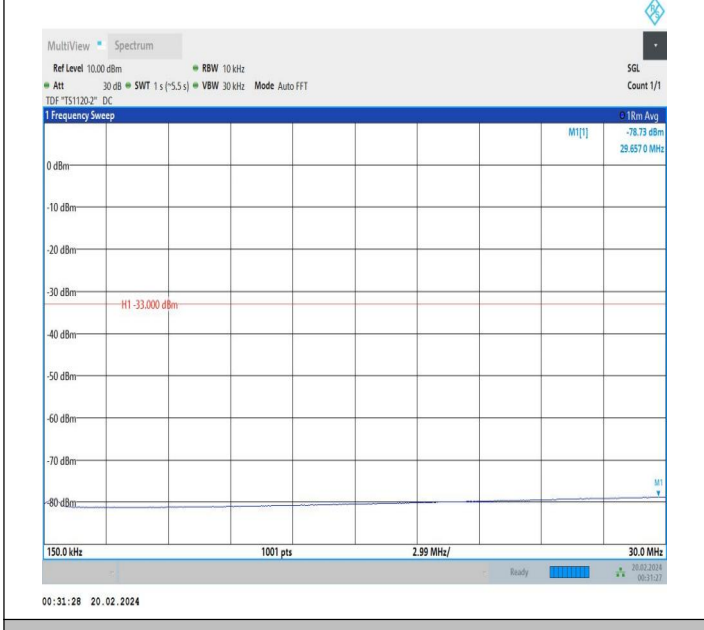
66-66-15MHz-10MHz-QPSK-QPSK-132047-132167-1RB#0-1 RB#49-0.15~30MHz-PASS
