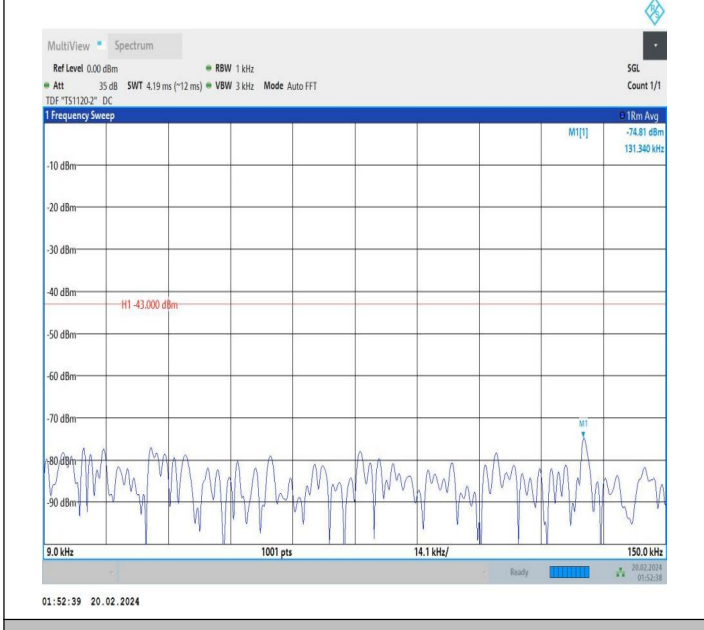
66-66-15MHz-15MHz-QPSK-QPSK-132447-132597-1RB#0-0 RB#0-0.009~0.15MHz-PASS
