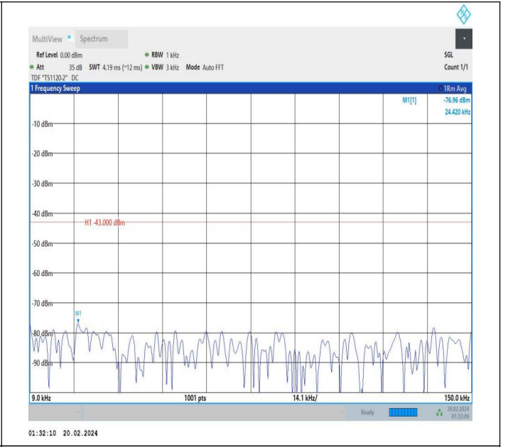
66-66-15MHz-15MHz-QPSK-QPSK-132047-132197-1RB#74-0 RB#0-0.009~0.15MHz-PASS
