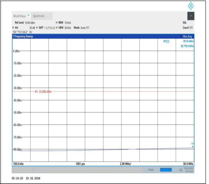
66-66-15MHz-20MHz-QPSK-QPSK-132325-132496-1RB#0-0 RB#0-0.15~30MHz-PASS
