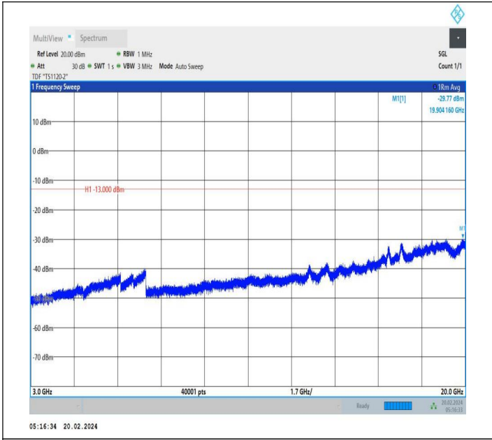
66-66-15MHz-20MHz-QPSK-QPSK-132325-132496-1RB#0-0 RB#0-3000~20000MHz-PASS
