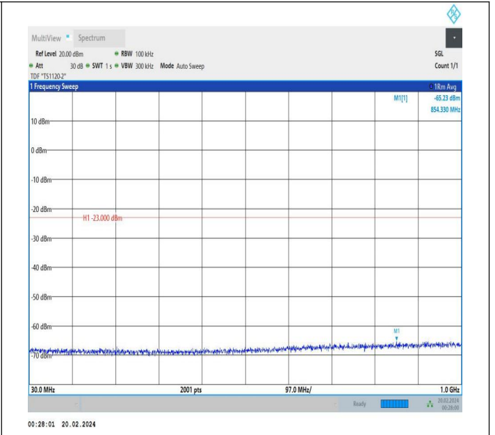
66-66-15MHz-10MHz-QPSK-QPSK-132047-132167-1RB#0-0 RB#0-30~1000MHz-PASS
