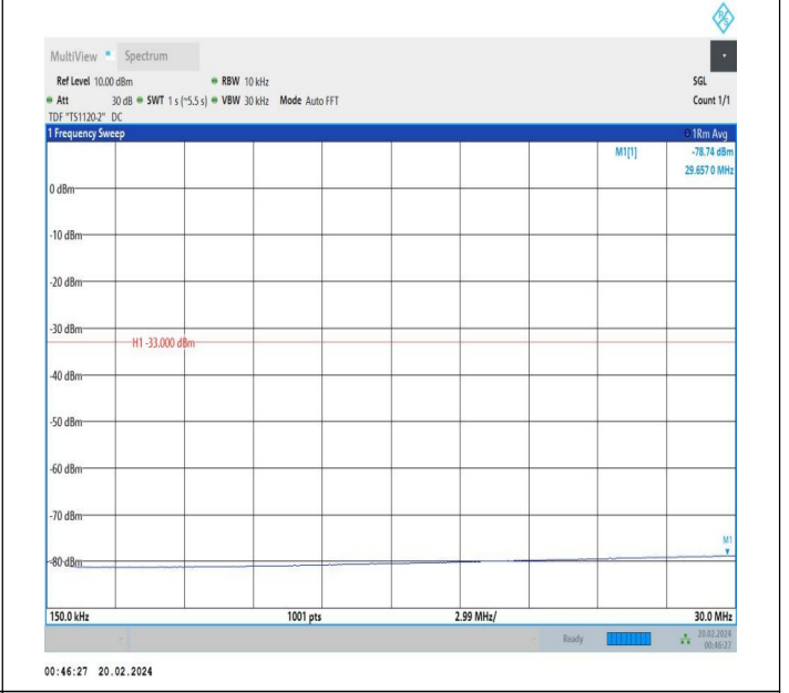
66-66-15MHz-10MHz-QPSK-QPSK-132499-132619-1RB#74-0 RB#0-0.15~30MHz-PASS
