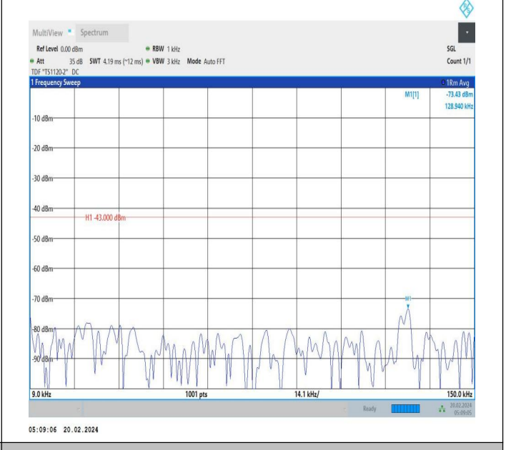
66-66-15MHz-20MHz-QPSK-QPSK-132050-132221-1RB#0-1 RB#99-0.009~0.15MHz-PASS
