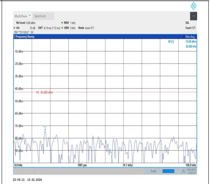
66-66-10MHz-20MHz-QPSK-QPSK-132027-132171-1RB#49-0 RB#0-0.009~0.15MHz-PASS
