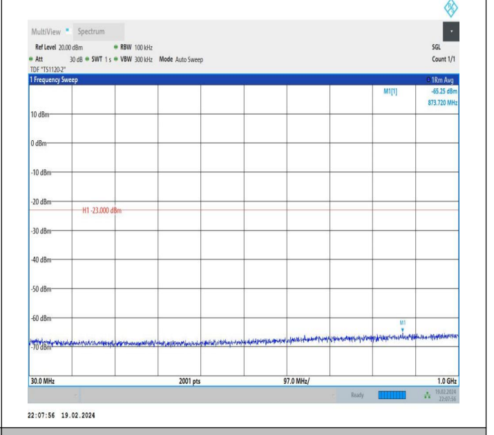
66-66-10MHz-15MHz-QPSK-QPSK-132351-132471-1RB#49-0 RB#0-30~1000MHz-PASS
