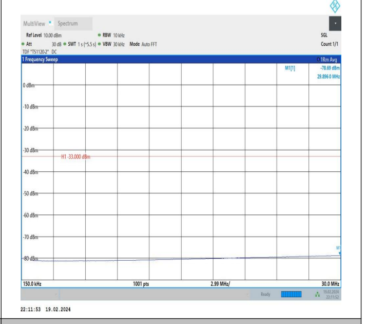
66-66-10MHz-15MHz-QPSK-QPSK-132351-132471-1RB#0-1 RB#74-0.15~30MHz-PASS
