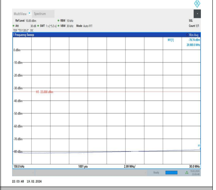
66-66-10MHz-15MHz-QPSK-QPSK-132025-132145-1RB#49-0 RB#0-0.15~30MHz-PASS
