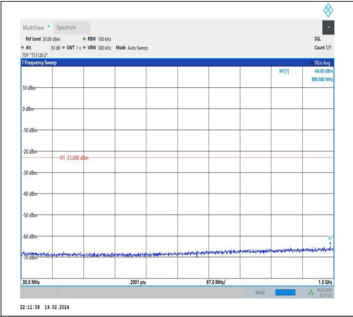
66-66-10MHz-15MHz-QPSK-QPSK-132351-132471-1RB#0-1 RB#74-30~1000MHz-PASS
