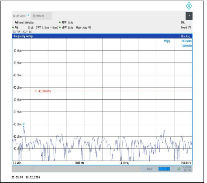
66-66-10MHz-20MHz-QPSK-QPSK-132428-132572-1RB#49-0 RB#0-0.009~0.15MHz-PASS
