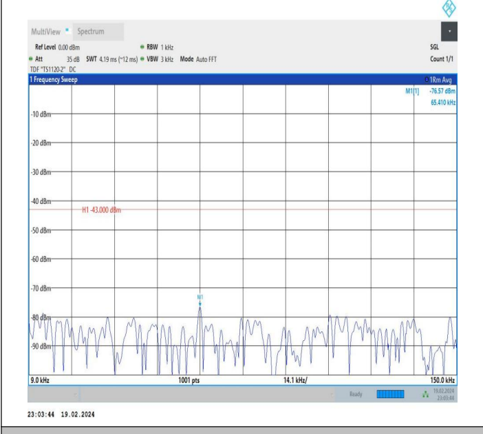
66-66-10MHz-20MHz-QPSK-QPSK-132027-132171-1RB#0-0 RB#0-0.009~0.15MHz-PASS
