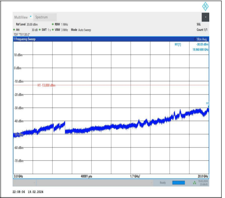
66-66-10MHz-15MHz-QPSK-QPSK-132351-132471-1RB#49-0 RB#0-3000~20000MHz-PASS
