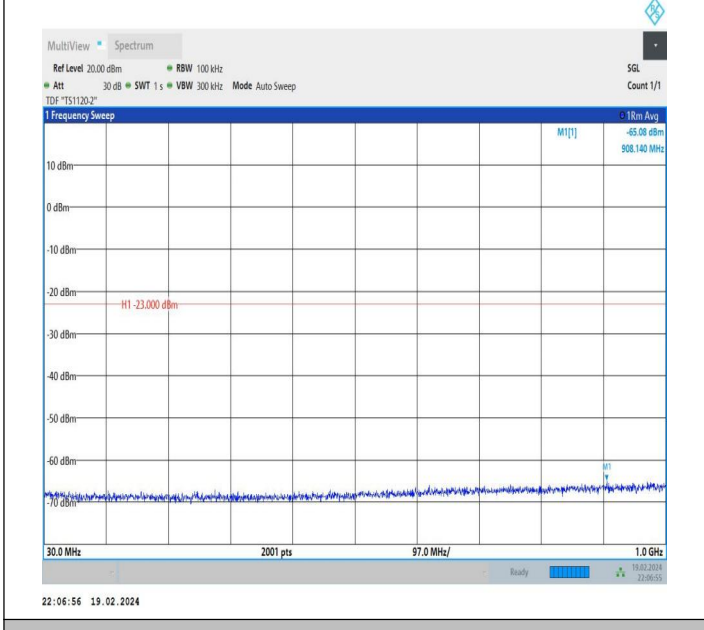
66-66-10MHz-15MHz-QPSK-QPSK-132351-132471-1RB#0-0 RB#0-30~1000MHz-PASS
