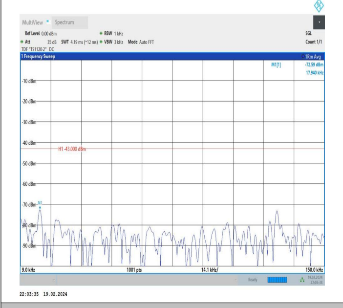
66-66-10MHz-15MHz-QPSK-QPSK-132025-132145-1RB#49-0 RB#0-0.009~0.15MHz-PASS
