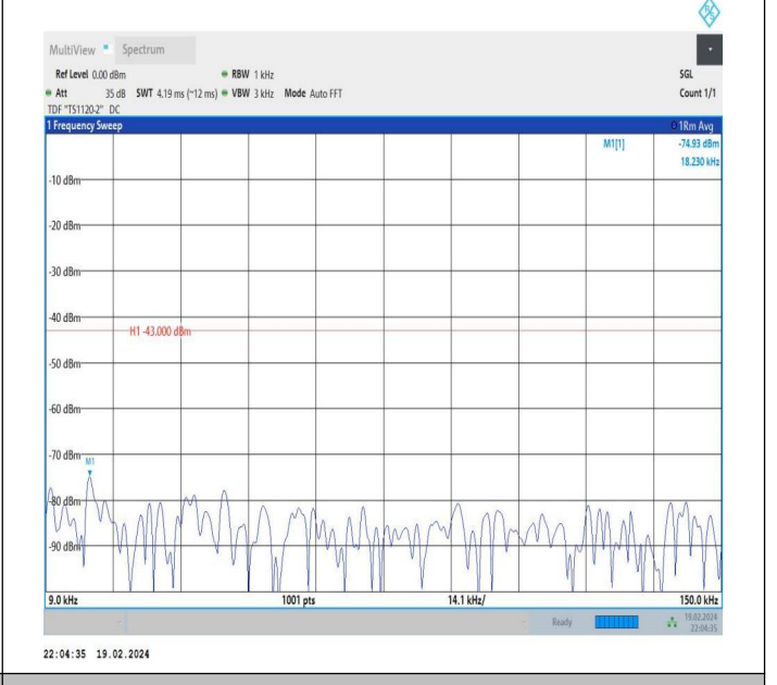
66-66-10MHz-15MHz-QPSK-QPSK-132025-132145-1RB#0-1 RB#74-0.009~0.15MHz-PASS
