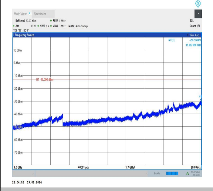
66-66-10MHz-15MHz-QPSK-QPSK-132025-132145-1RB#49-0 RB#0-3000~20000MHz-PASS
