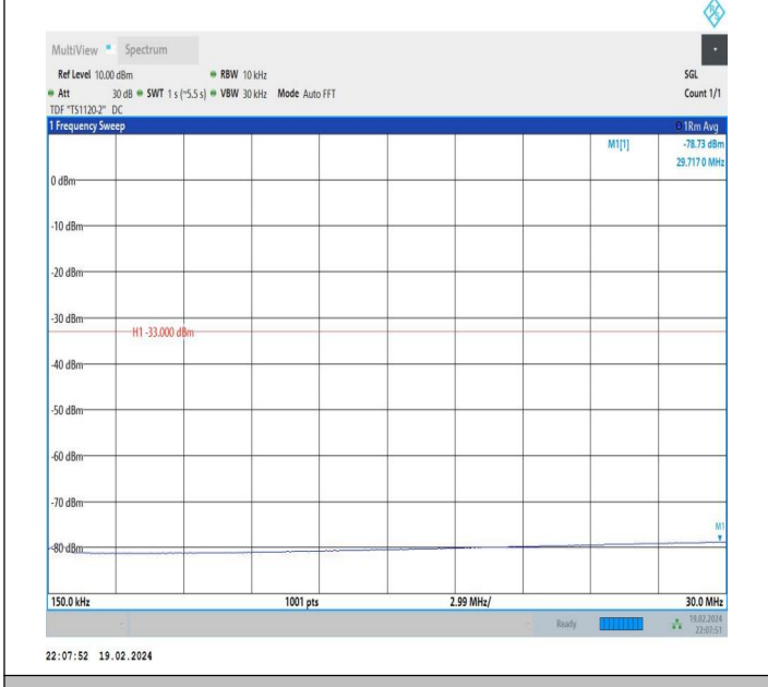
66-66-10MHz-15MHz-QPSK-QPSK-132351-132471-1RB#49-0 RB#0-0.15~30MHz-PASS
