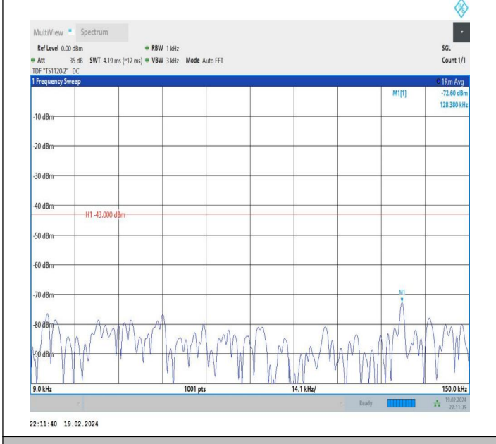
66-66-10MHz-15MHz-QPSK-QPSK-132351-132471-1RB#0-1 RB#74-0.009~0.15MHz-PASS
