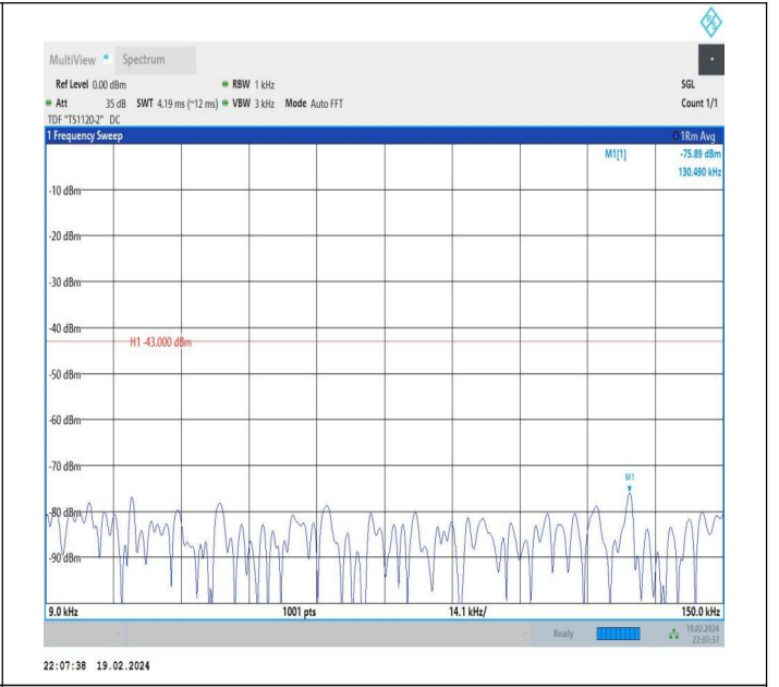
66-66-10MHz-15MHz-QPSK-QPSK-132351-132471-1RB#49-0 RB#0-0.009~0.15MHz-PASS
