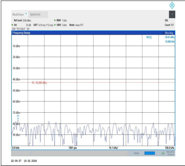
66-66-10MHz-15MHz-QPSK-QPSK-132351-132471-1RB#0-0 RB#0-0.009~0.15MHz-PASS
