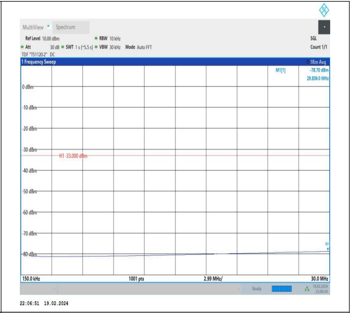
66-66-10MHz-15MHz-QPSK-QPSK-132351-132471-1RB#0-0 RB#0-0.15~30MHz-PASS
