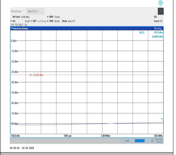
66-66-10MHz-20MHz-QPSK-QPSK-132328-132472-1RB#49-0 RB#0-0.15~30MHz-PASS
