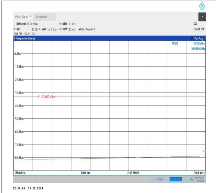
66-66-10MHz-15MHz-QPSK-QPSK-132025-132145-1RB#0-1 RB#74-0.15~30MHz-PASS
