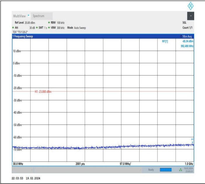
66-66-10MHz-15MHz-QPSK-QPSK-132025-132145-1RB#49-0 RB#0-30~1000MHz-PASS
