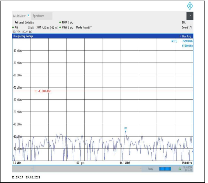
66-66-10MHz-15MHz-QPSK-QPSK-132025-132145-1RB#0-0 RB#0-0.009~0.15MHz-PASS
