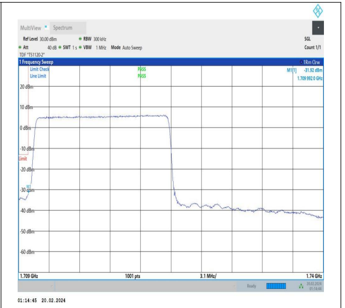
15MHz-15MHz_QPSK@QPSK-QPSK@QPSK_132047-132197 97_75RB#0@75RB#0-75RB#0@75RB#0
