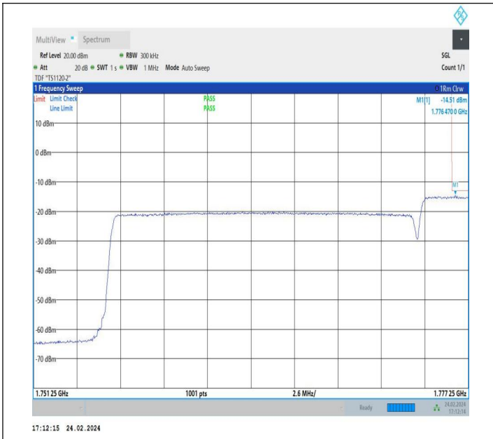
20MHz-5MHz_QPSK@QPSK-QPSK@QPSK_132522-132572_100RB#0@100RB#0-25RB#0@25RB#0
