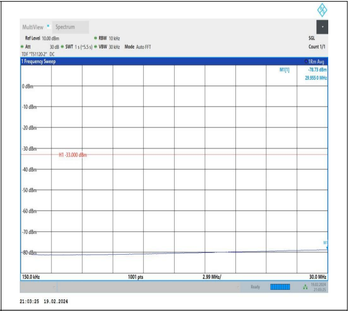
66-66-5MHz-20MHz-QPSK-QPSK-132328-132472-1RB#24-0 RB#0-0.15~30MHz-PASS
