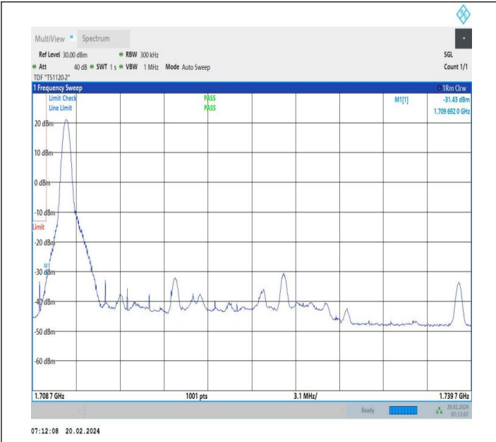
20MHz-10MHz_QPSK@QPSK-QPSK@QPSK_132072-132216_1RB#0@100RB#0-0RB#0@50RB#0
