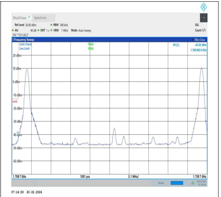
20MHz-10MHz_QPSK@QPSK-QPSK@QPSK_132072-132216_16_1RB#0@100RB#0-1RB#49@50RB#0
