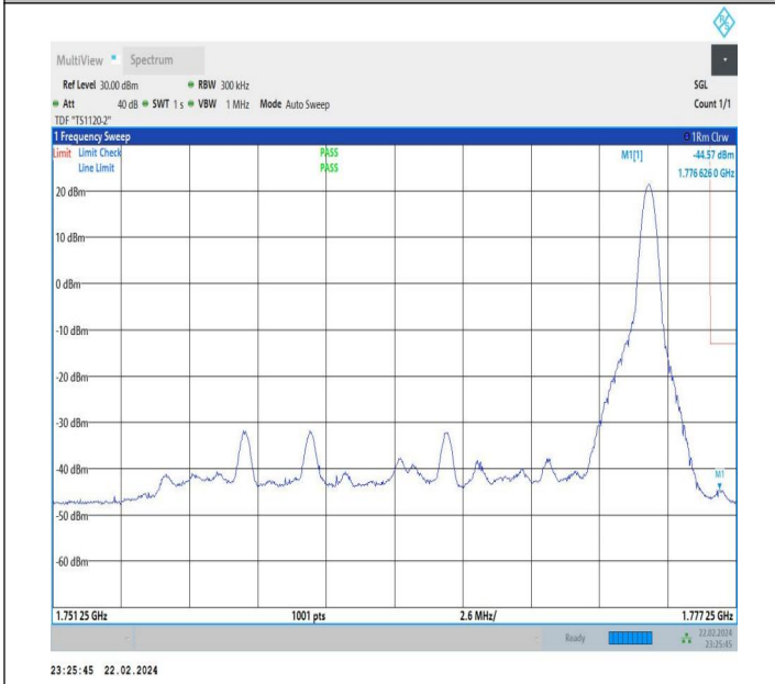
20MHz-5MHz_QPSK@QPSK-QPSK@QPSK_132522-132572_1RB#99@100RB#0-0RB#0@25RB#0
