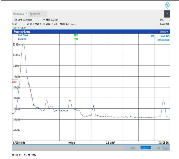
10MHz-15MHz_QPSK@QPSK-QPSK@QPSK_132025-132145_1RB#0@50RB#0-0RB#0@75RB#0
