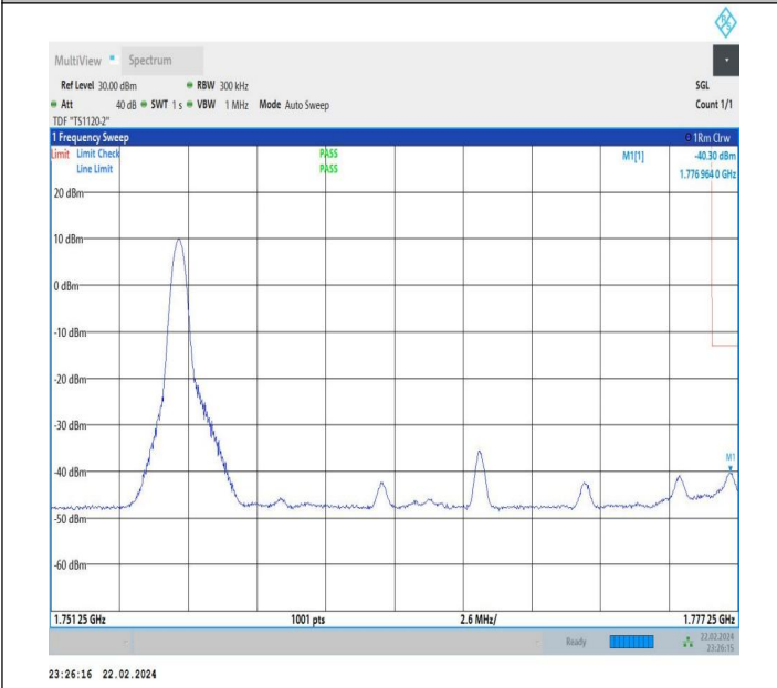
20MHz-5MHz_QPSK@QPSK-QPSK@QPSK_132522-132572_1RB#0@100RB#0-1RB#24@25RB#0
