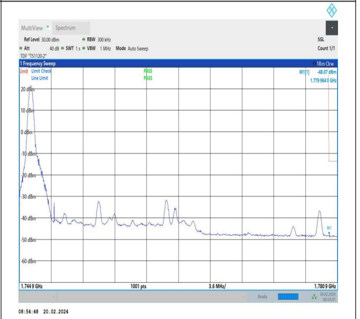
20MHz-15MHz_QPSK@QPSK-QPSK@QPSK_132423-132594_94_1RB#0@100RB#0-0RB#0@75RB#0
