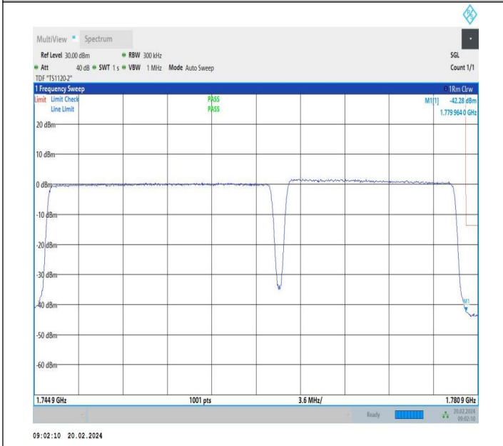
20MHz-15MHz_QPSK@QPSK-QPSK@QPSK_132423-132594_100RB#0@100RB#0-75RB#0@75RB#0
