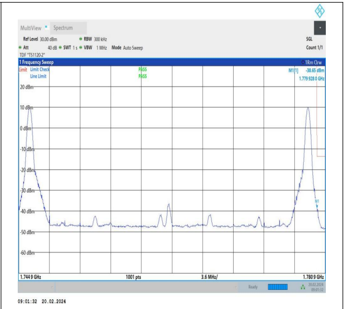
20MHz-15MHz_QPSK@QPSK-QPSK@QPSK_132423-132594_94_1RB#0@100RB#0-1RB#74@75RB#0
