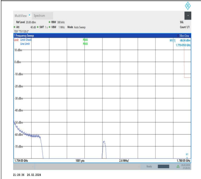
5MHz-20MHz_QPSK@QPSK-QPSK@QPSK_132428-132572_1RB#0@25RB#0-0RB#0@100RB#0
