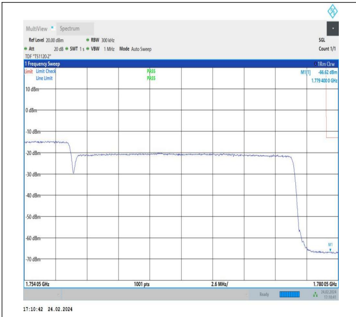
5MHz-20MHz_QPSK@QPSK-QPSK@QPSK_132428-132572_25RB#0@25RB#0-100RB#0@100RB#0
