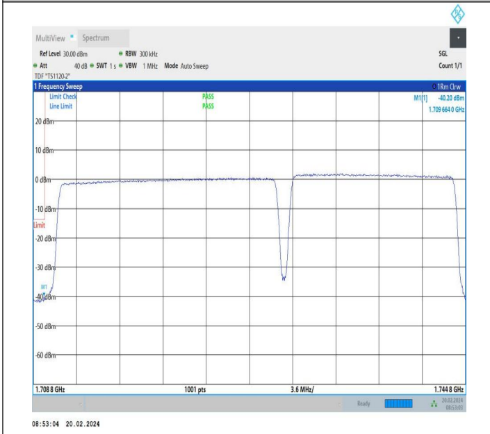
20MHz-15MHz_QPSK@QPSK-QPSK@QPSK_132072-132243_100RB#0@100RB#0-75RB#0@75RB#0
