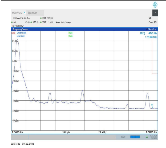
15MHz-10MHz_QPSK@QPSK-QPSK@QPSK_132499-132619 _1RB#0@75RB#0-0RB#0@50RB#0
