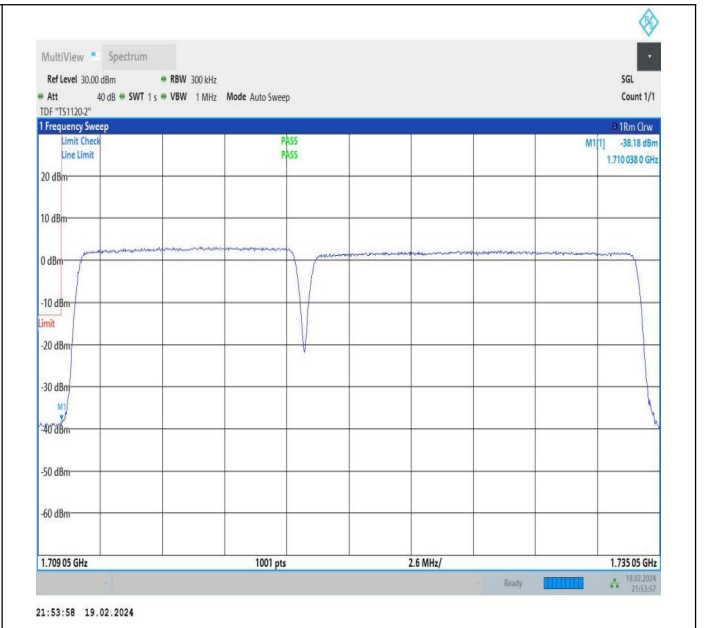
10MHz-15MHz_QPSK@QPSK-QPSK@QPSK_132025-132145 45_50RB#0@50RB#0-75RB#0@75RB#0
