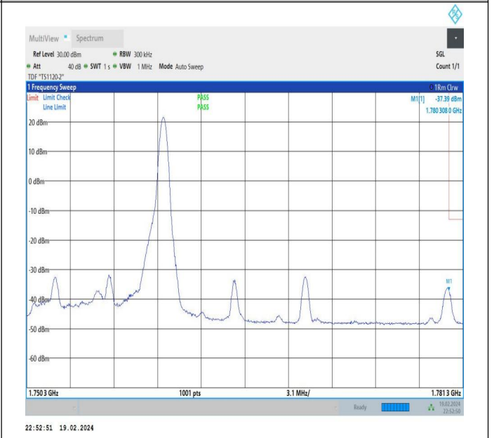
10MHz-20MHz_QPSK@QPSK-QPSK@QPSK_132428-132572_72_1RB#49@50RB#0-0RB#0@100RB#0
