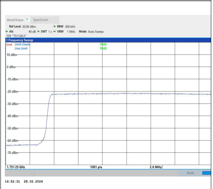
20MHz-5MHz_QPSK@QPSK-QPSK@QPSK_132522-132572_2_100RB#0@100RB#0-25RB#0@25RB#0
