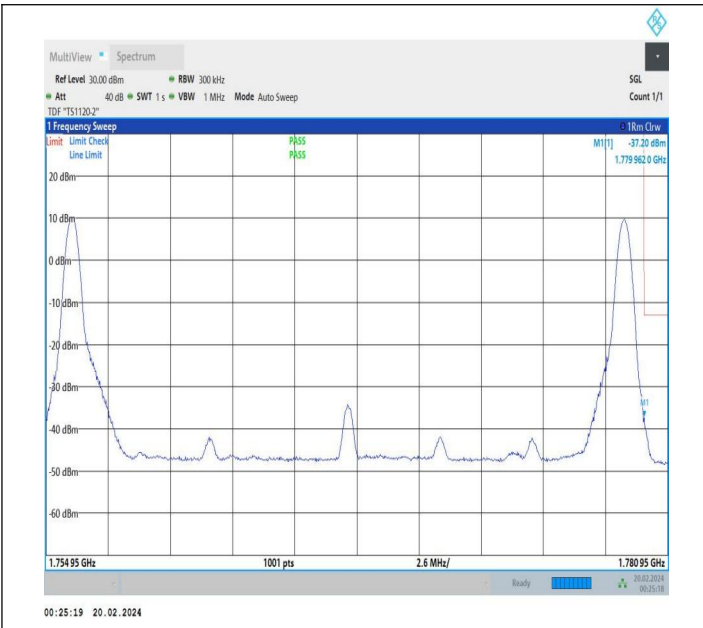
15MHz-10MHz_QPSK@QPSK-QPSK@QPSK_132499-132619_1RB#0@75RB#0-1RB#49@50RB#0
