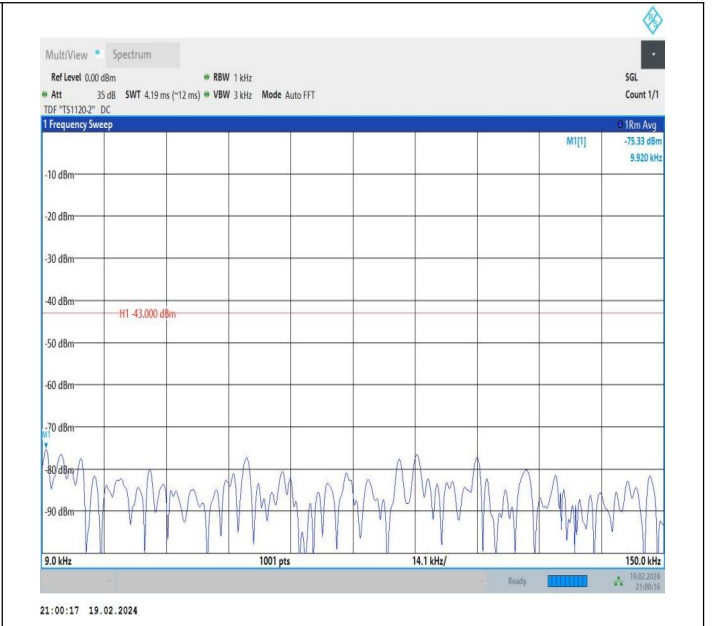
66-66-5MHz-20MHz-QPSK-QPSK-132027-132171-1RB#24-0 RB#0-0.009~0.15MHz-PASS
