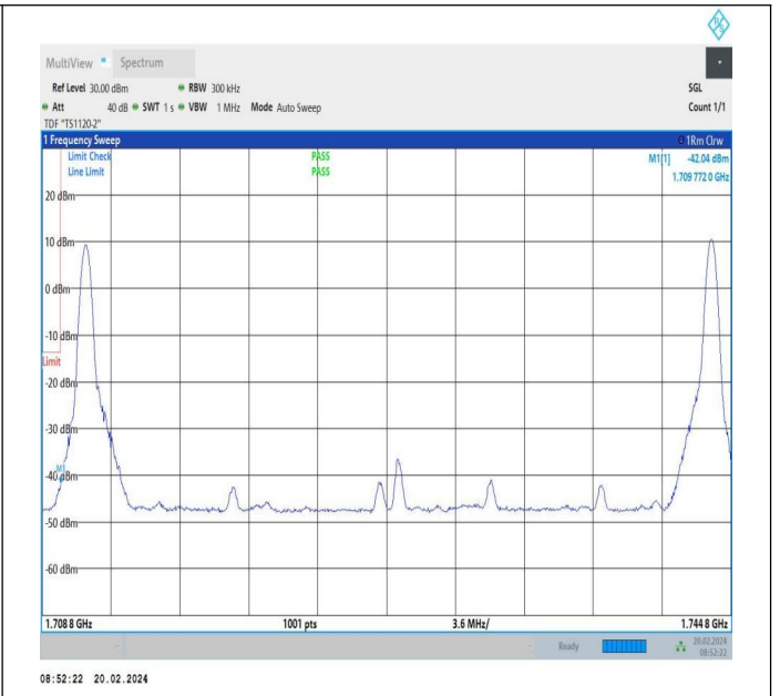
20MHz-15MHz_QPSK@QPSK-QPSK@QPSK_132072-132243_43_1RB#0@100RB#0-1RB#74@75RB#0
