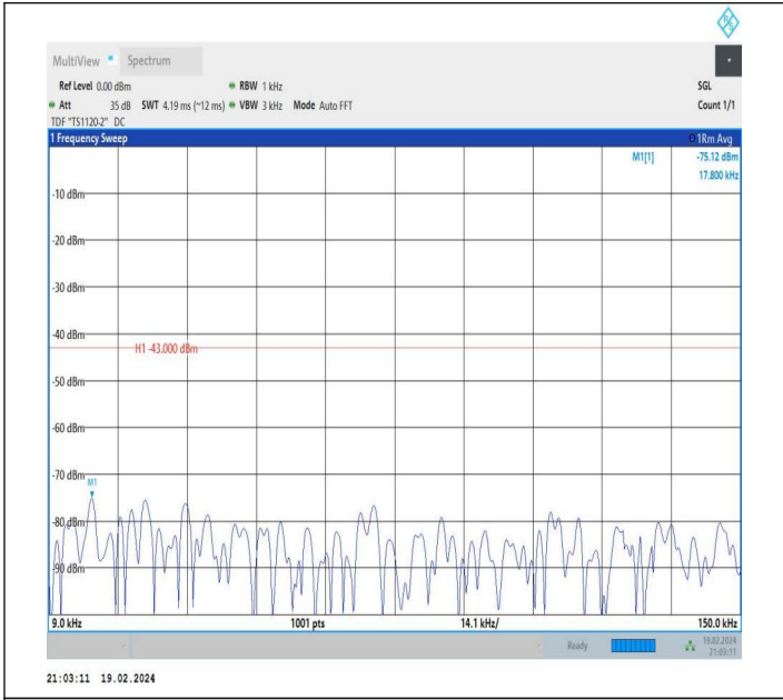
66-66-5MHz-20MHz-QPSK-QPSK-132328-132472-1RB#24-0 RB#0-0.009~0.15MHz-PASS
