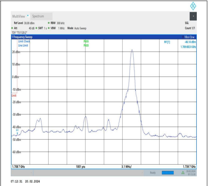
20MHz-10MHz_QPSK@QPSK-QPSK@QPSK_132072-132216_16_1RB#99@100RB#0-0RB#0@50RB#0
