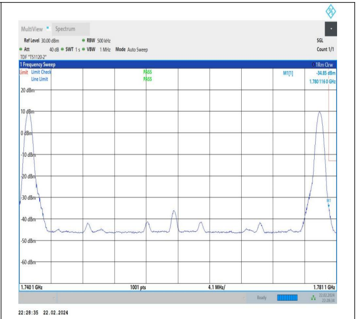
20MHz-20MHz_QPSK@QPSK-QPSK@QPSK_132374-1325 72_1RB#0@100RB#0-1RB#99@100RB#0
