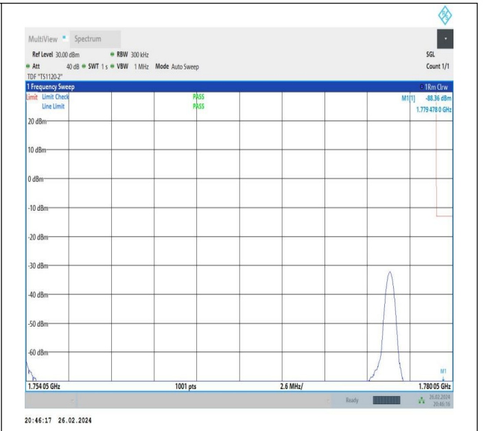
5MHz-20MHz_QPSK@QPSK-QPSK@QPSK_132428-132572_2_1RB#0@25RB#0-1RB#99@100RB#0
