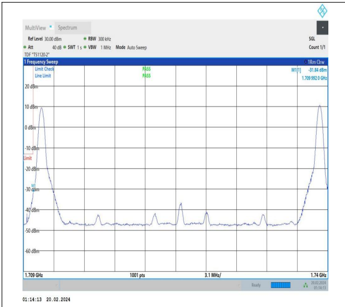
15MHz-15MHz_QPSK@QPSK-QPSK@QPSK_132047-132197 _1RB#0@75RB#0-1RB#74@75RB#0
