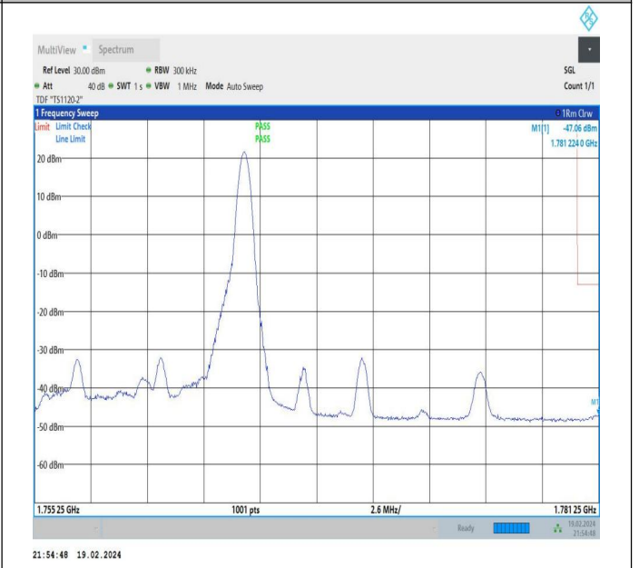
10MHz-15MHz_QPSK@QPSK-QPSK@QPSK_132477-132597 97_1RB#49@50RB#0-0RB#0@75RB#0
