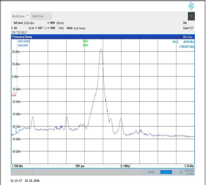
15MHz-15MHz_QPSK@QPSK-QPSK@QPSK_132047-132197_97_1RB#74@75RB#0-0RB#0@75RB#0
