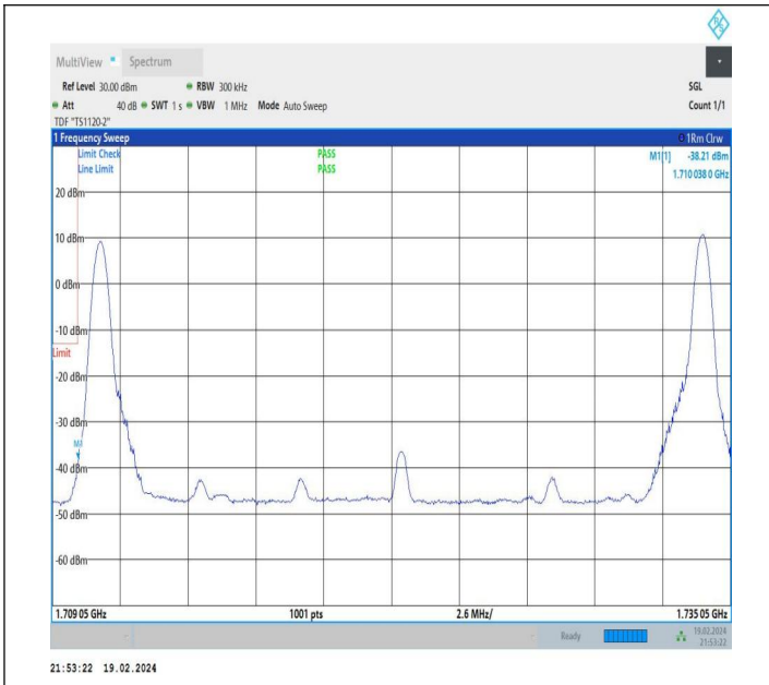
10MHz-15MHz_QPSK@QPSK-QPSK@QPSK_132025-132145 _1RB#0@50RB#0-1RB#74@75RB#0
