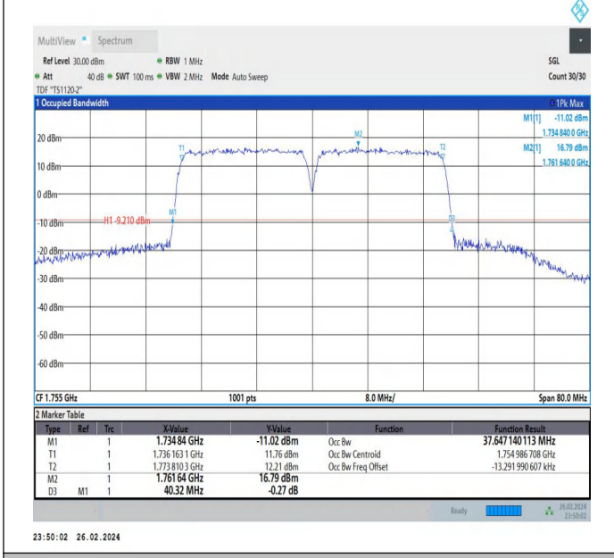
66-66-20MHz-20MHz-64QAM-64QAM-132323-132521-100RB#0-100RB#0-PASS
