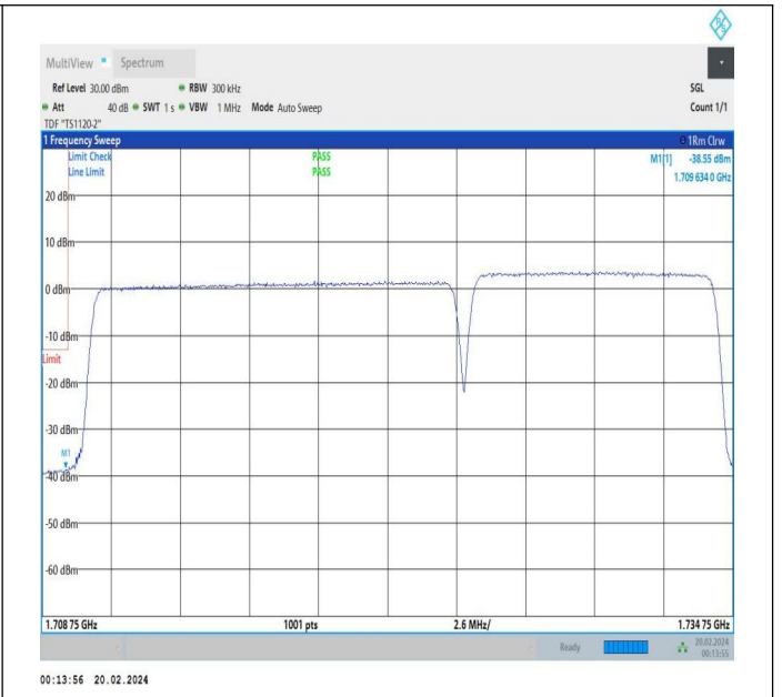
15MHz-10MHz_QPSK@QPSK-QPSK@QPSK_132047-132167 67_75RB#0@75RB#0-50RB#0@50RB#0
