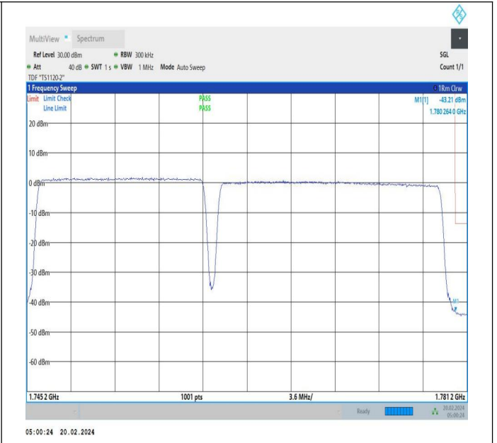
15MHz-20MHz_QPSK@QPSK-QPSK@QPSK_132401-132572_72_75RB#0@75RB#0-100RB#0@100RB#0
