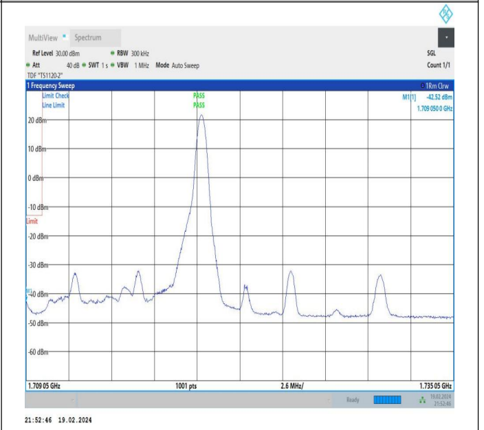
10MHz-15MHz_QPSK@QPSK-QPSK@QPSK_132025-132145_45_1RB#49@50RB#0-0RB#0@75RB#0
