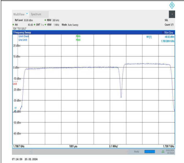
20MHz-10MHz_QPSK@QPSK-QPSK@QPSK_132072-132216_100RB#0@100RB#0-50RB#0@50RB#0
