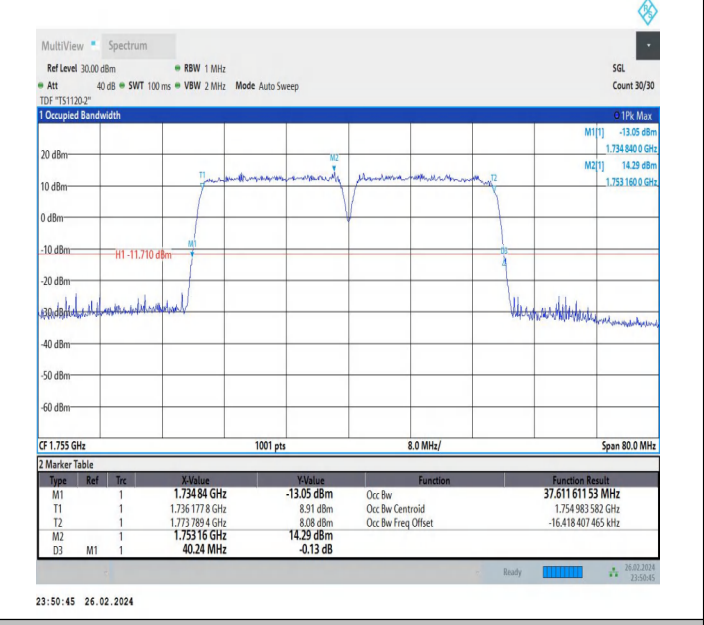
66-66-20MHz-20MHz-256QAM-256QAM-132323-132521-100RB#0-100RB#0-PASS
