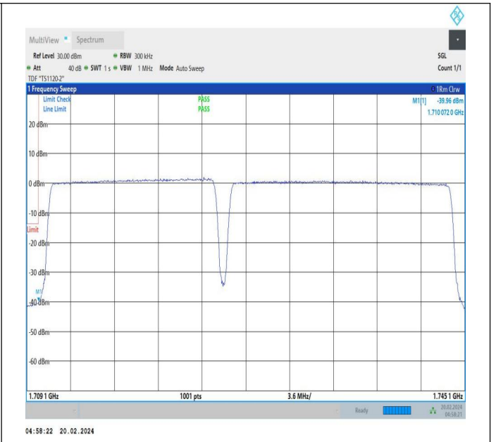
15MHz-20MHz_QPSK@QPSK-QPSK@QPSK_132050-132221_21_75RB#0@75RB#0-100RB#0@100RB#0
