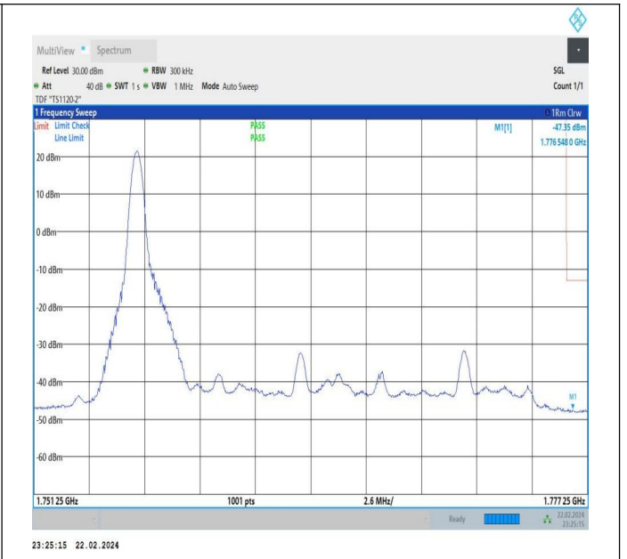
20MHz-5MHz_QPSK@QPSK-QPSK@QPSK_132522-132572_2_1RB#0@100RB#0-0RB#0@25RB#0
