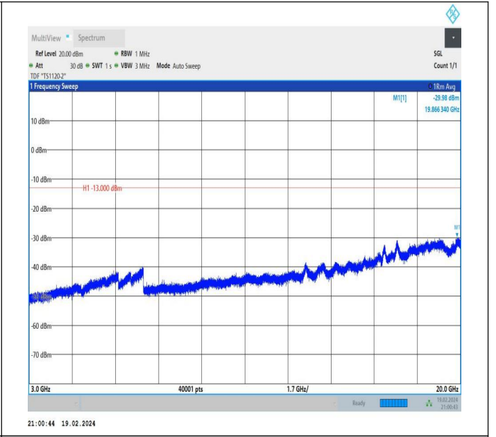
66-66-5MHz-20MHz-QPSK-QPSK-132027-132171-1RB#24-0 RB#0-3000~20000MHz-PASS
