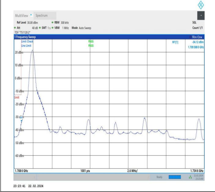
20MHz-5MHz_QPSK@QPSK-QPSK@QPSK_132072-132189_1RB#0@100RB#0-0RB#0@25RB#0
