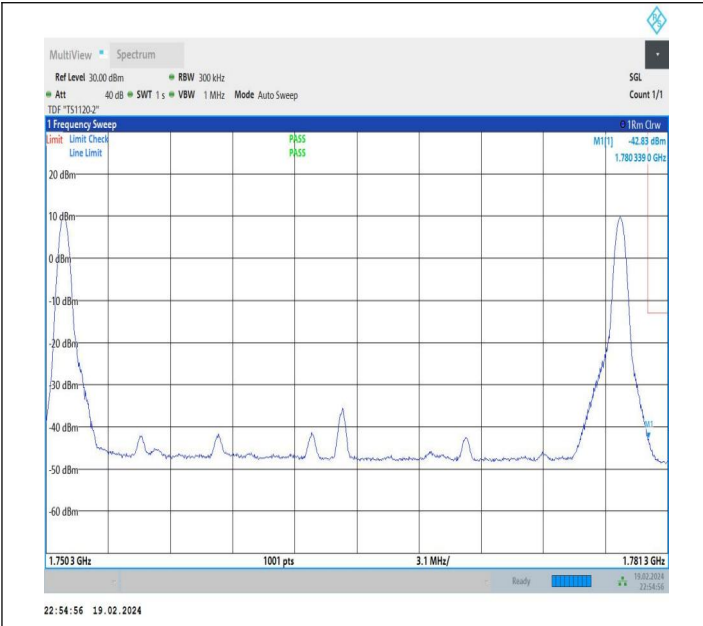
10MHz-20MHz_QPSK@QPSK-QPSK@QPSK_132428-132572 _1RB#0@50RB#0-1RB#99@100RB#0
