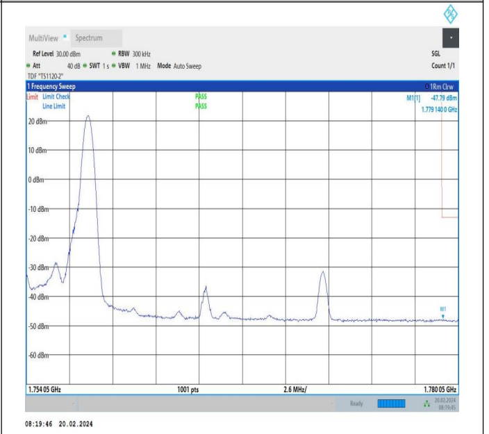
5MHz-20MHz_QPSK@QPSK-QPSK@QPSK_132428-132572_2_1RB#24@25RB#0-0RB#0@100RB#0
