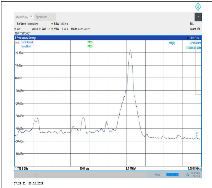
20MHz-10MHz_QPSK@QPSK-QPSK@QPSK_132473-132617_1RB#99@100RB#0-0RB#0@50RB#0
