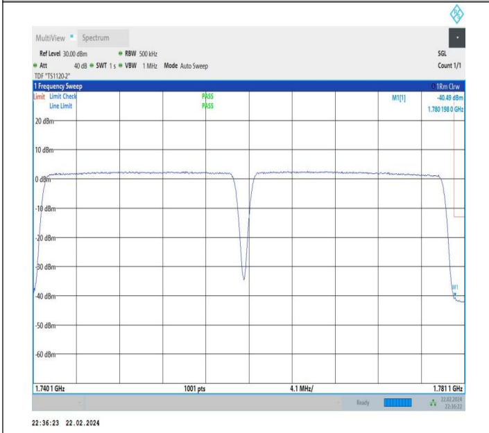
20MHz-20MHz_QPSK@QPSK-QPSK@QPSK_132374-132572 _100RB#0@100RB#0-100RB#0@100RB#0
