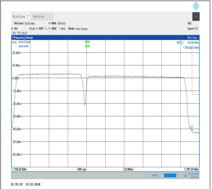
10MHz-15MHz_QPSK@QPSK-QPSK@QPSK_132477-132597_97_50RB#0@50RB#0-75RB#0@75RB#0
