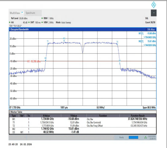
66-66-20MHz-20MHz-16QAM-16QAM-132323-132521-100RB# 0-100RB#0-PASS
