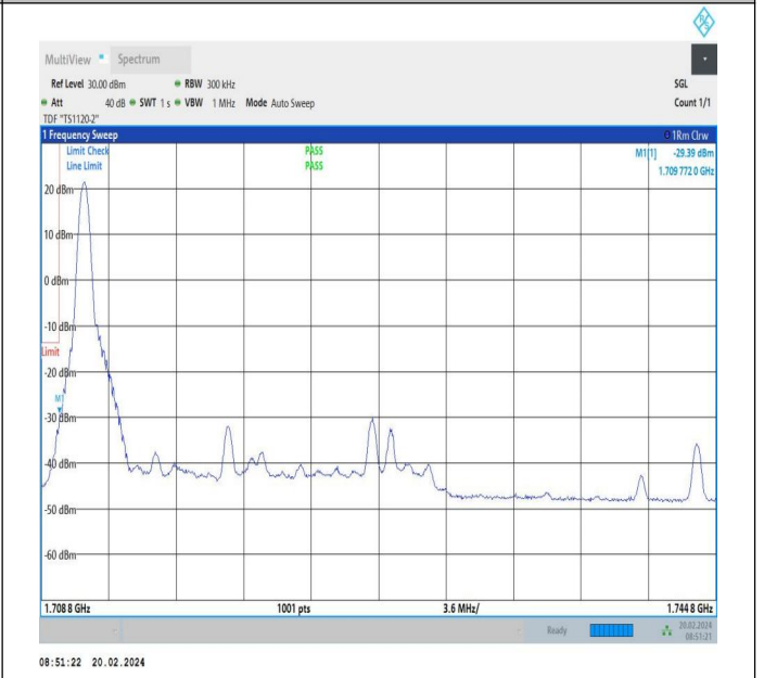
20MHz-15MHz_QPSK@QPSK-QPSK@QPSK_132072-132243_1RB#0@100RB#0-0RB#0@75RB#0
