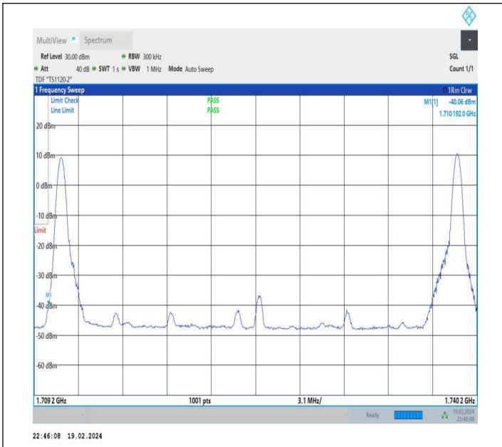
10MHz-20MHz_QPSK@QPSK-QPSK@QPSK_132027-132171_1RB#0@50RB#0-1RB#99@100RB#0
