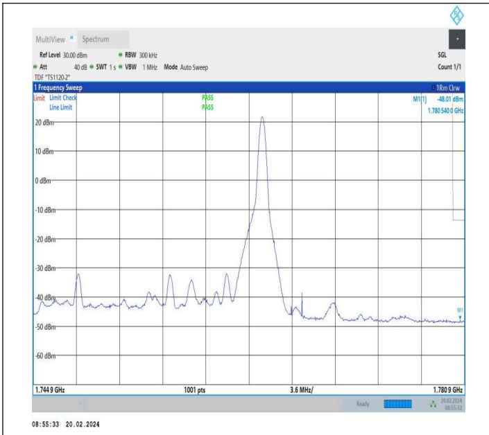
20MHz-15MHz_QPSK@QPSK-QPSK@QPSK_132423-132594_1RB#99@100RB#0-0RB#0@75RB#0
