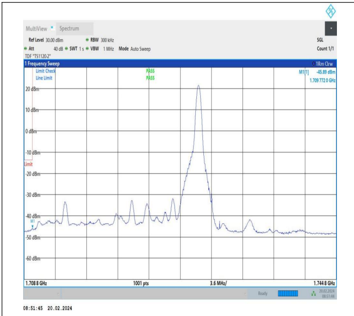
20MHz-15MHz_QPSK@QPSK-QPSK@QPSK_132072-132243_1RB#99@100RB#0-0RB#0@75RB#0
