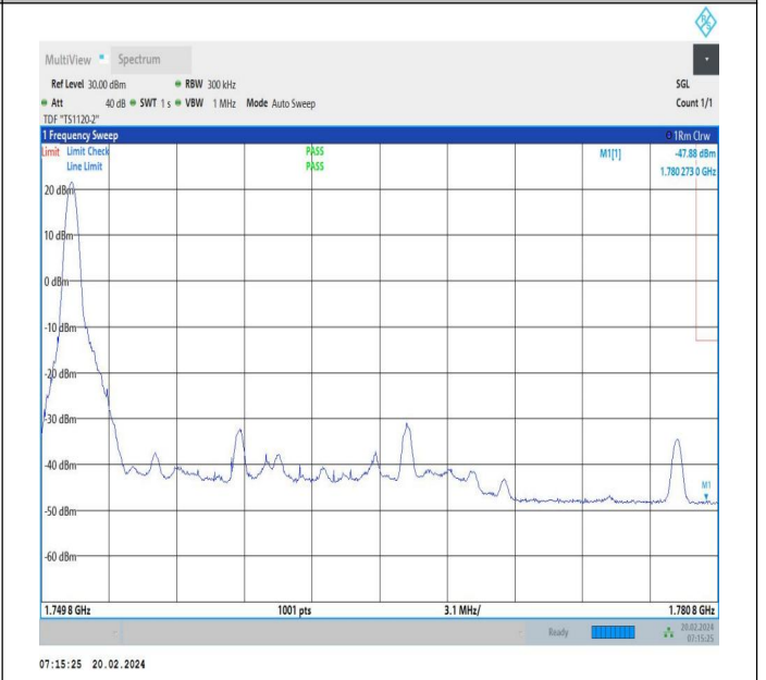
20MHz-10MHz_QPSK@QPSK-QPSK@QPSK_132473-132617_17_1RB#0@100RB#0-0RB#0@50RB#0
