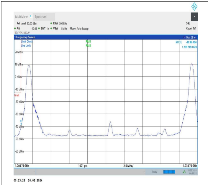
15MHz-10MHz_QPSK@QPSK-QPSK@QPSK_132047-132167 _1RB#0@75RB#0-1RB#49@50RB#0
