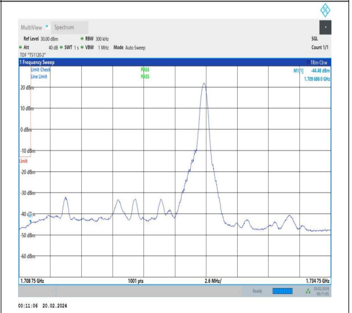
15MHz-10MHz_QPSK@QPSK-QPSK@QPSK_132047-132167 67_1RB#74@75RB#0-0RB#0@50RB#0
