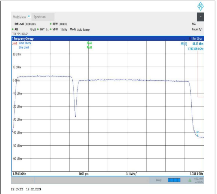
10MHz-20MHz_QPSK@QPSK-QPSK@QPSK_132428-132572 72_50RB#0@50RB#0-100RB#0@100RB#0
