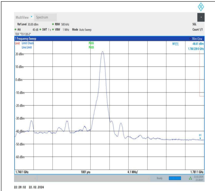
20MHz-20MHz_QPSK@QPSK-QPSK@QPSK_132374-132572 _1RB#99@100RB#0-0RB#0@100RB#0
