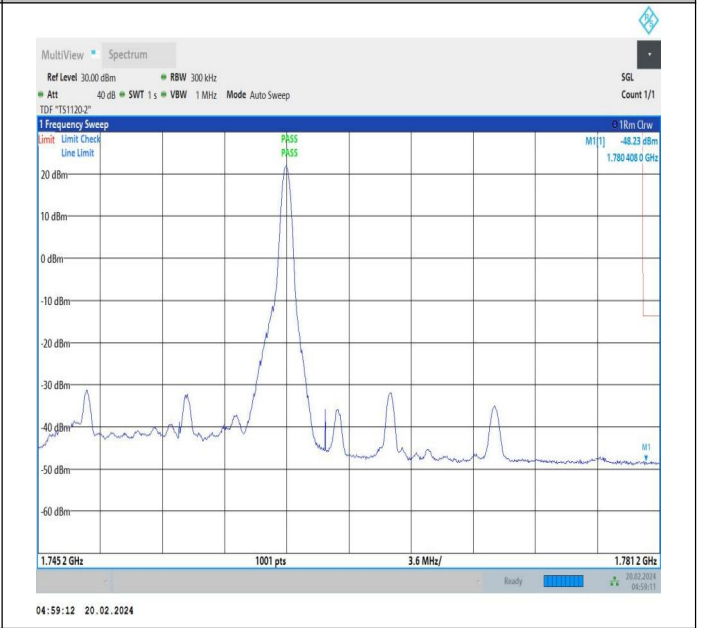
15MHz-20MHz_QPSK@QPSK-QPSK@QPSK_132401-132572_72_1RB#74@75RB#0-0RB#0@100RB#0
