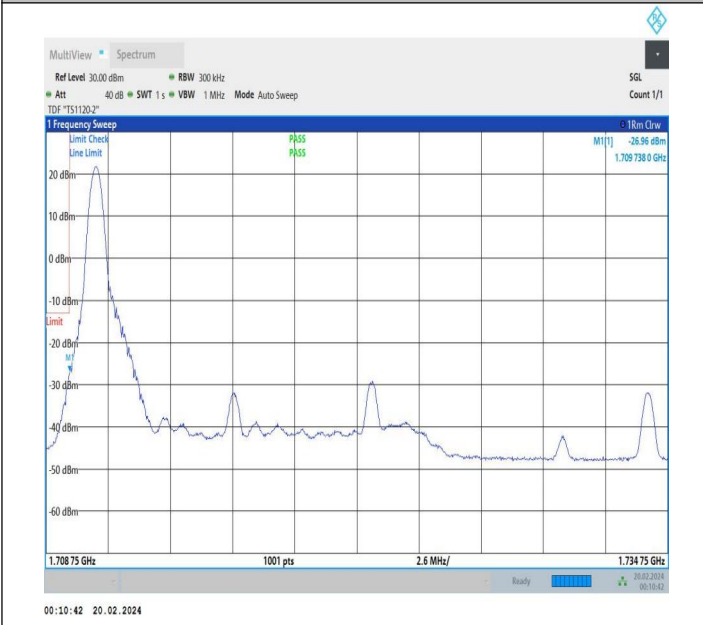
15MHz-10MHz_QPSK@QPSK-QPSK@QPSK_132047-132167 _1RB#0@75RB#0-0RB#0@50RB#0
