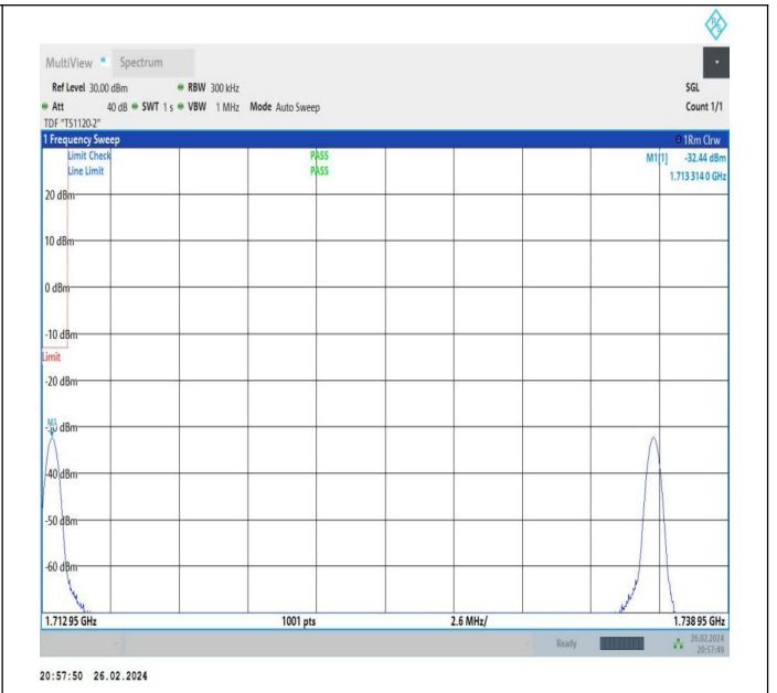
5MHz-20MHz_QPSK@QPSK-QPSK@QPSK_132027-132171_1_1RB#0@25RB#0-1RB#99@100RB#0
