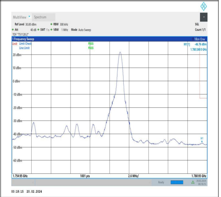
15MHz-10MHz_QPSK@QPSK-QPSK@QPSK_132499-132619 19_1RB#74@75RB#0-0RB#0@50RB#0
