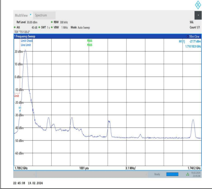
10MHz-20MHz_QPSK@QPSK-QPSK@QPSK_132027-132171_1RB#0@50RB#0-0RB#0@100RB#0
