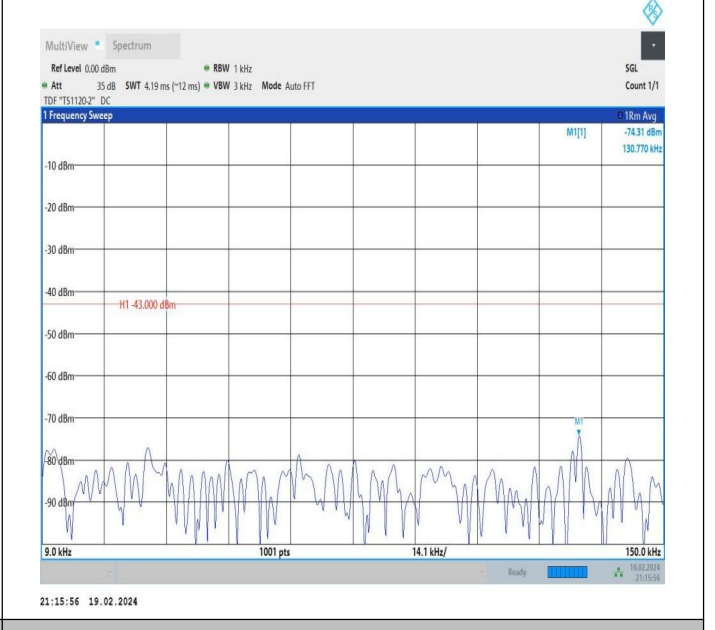
66-66-5MHz-20MHz-QPSK-QPSK-132428-132572-1RB#24-0 RB#0-0.009~0.15MHz-PASS
