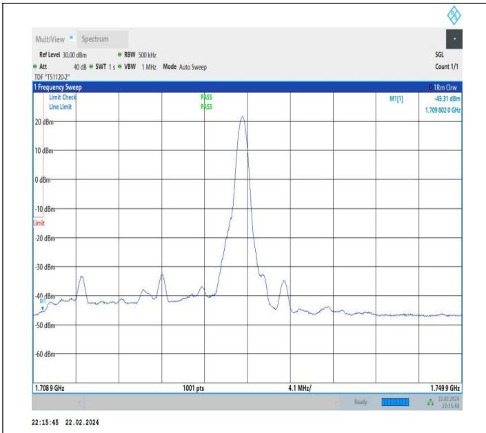
20MHz-20MHz_QPSK@QPSK-QPSK@QPSK_132072-132270 _1RB#99@100RB#0-0RB#0@100RB#0
