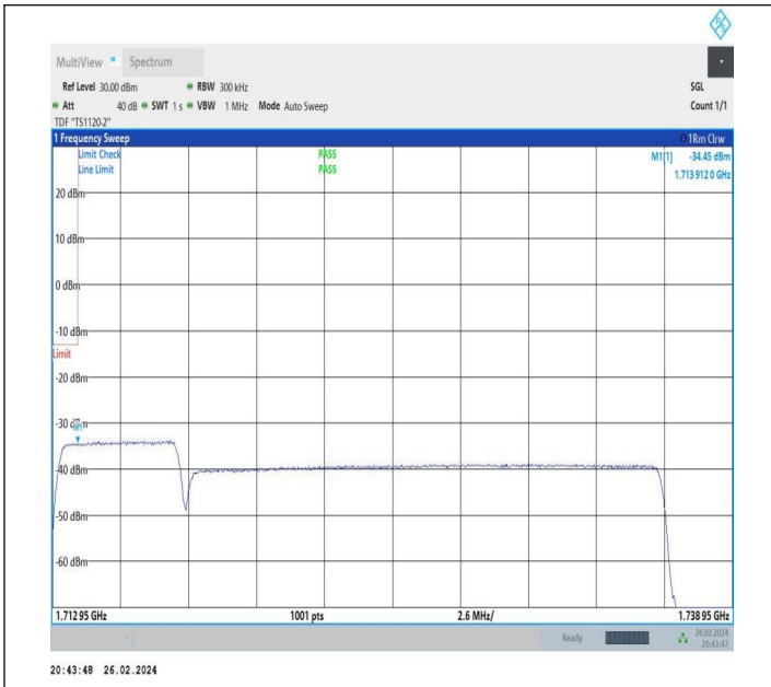
5MHz-20MHz_QPSK@QPSK-QPSK@QPSK_132027-132171_25RB#0@25RB#0-100RB#0@100RB#0
