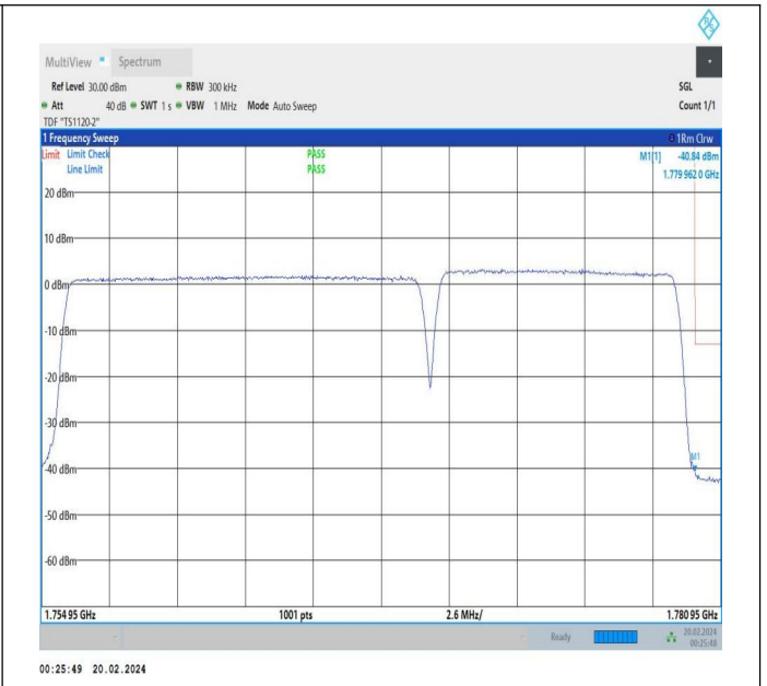
15MHz-10MHz_QPSK@QPSK-QPSK@QPSK_132499-132619_19_75RB#0@75RB#0-50RB#0@50RB#0
