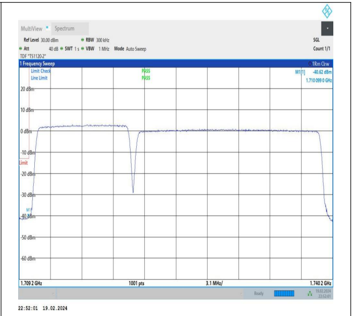
10MHz-20MHz_QPSK@QPSK-QPSK@QPSK_132027-132171_71_50RB#0@50RB#0-100RB#0@100RB#0
