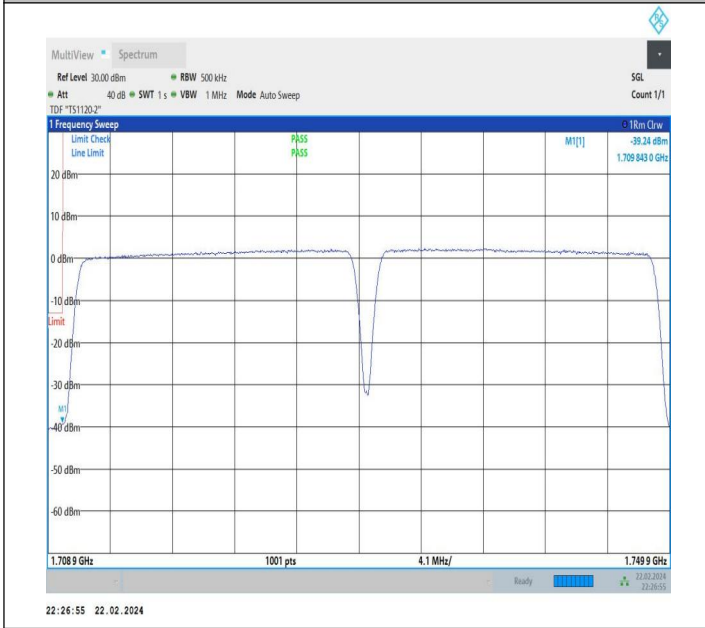
20MHz-20MHz_QPSK@QPSK-QPSK@QPSK_132072-132270 _100RB#0@100RB#0-100RB#0@100RB#0
