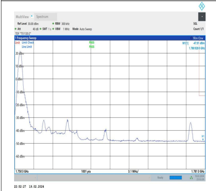
10MHz-20MHz_QPSK@QPSK-QPSK@QPSK_132428-132572_1RB#0@50RB#0-0RB#0@100RB#0
