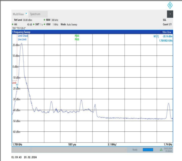
15MHz-15MHz_QPSK@QPSK-QPSK@QPSK_132047-132197_1RB#0@75RB#0-0RB#0@75RB#0
