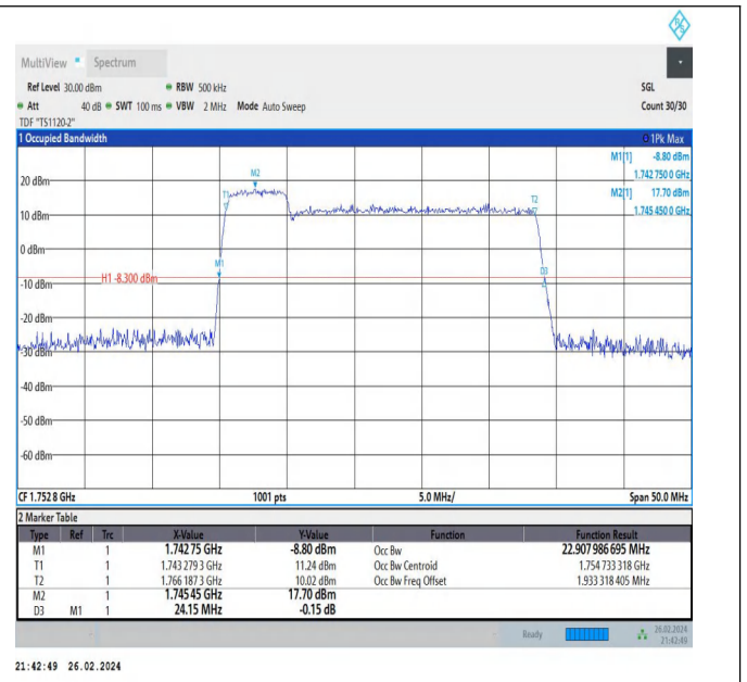
66-66-5MHz-20MHz-16QAM-16QAM-132328-132472-25RB#0-100RB#0-PASS
