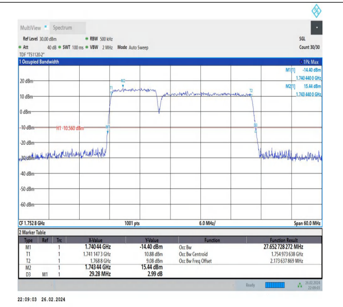
66-66-10MHz-20MHz-16QAM-16QAM-132328-132472-50RB#0-100RB#0-PASS
