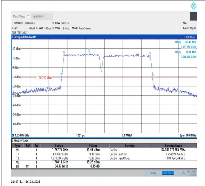
66-66-15MHz-20MHz-64QAM-64QAM-132325-132496-75RB#0-100RB#0-PASS
