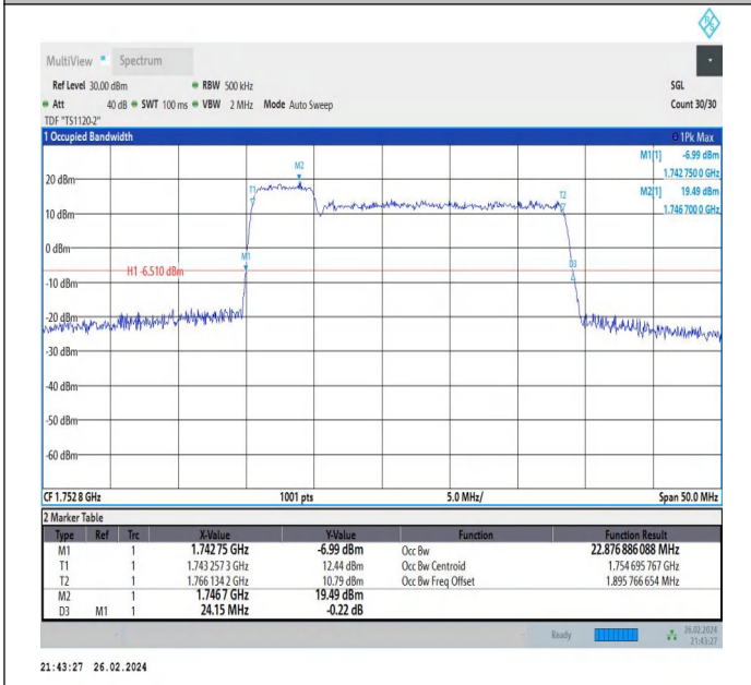
66-66-5MHz-20MHz-64QAM-64QAM-132328-132472-25RB#0-100RB#0-PASS
