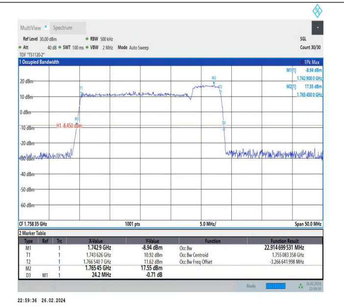
66-66-20MHz-5MHz-16QAM-16QAM-132397-132514-100RB#0-25RB#0-PASS
