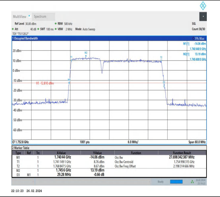
66-66-10MHz-20MHz-256QAM-256QAM-132328-132472-50RB#0-100RB#0-PASS
