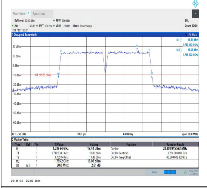
66-66-15MHz-15MHz-64QAM-64QAM-132347-132497-75RB#0-75RB#0-PASS
