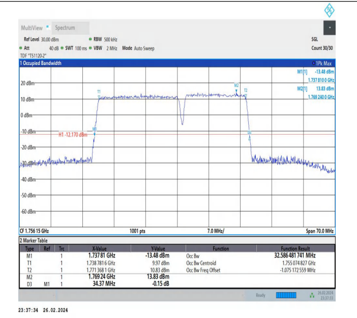
66-66-20MHz-15MHz-16QAM-16QAM-132348-132519-100RB# 0-75RB#0-PASS
