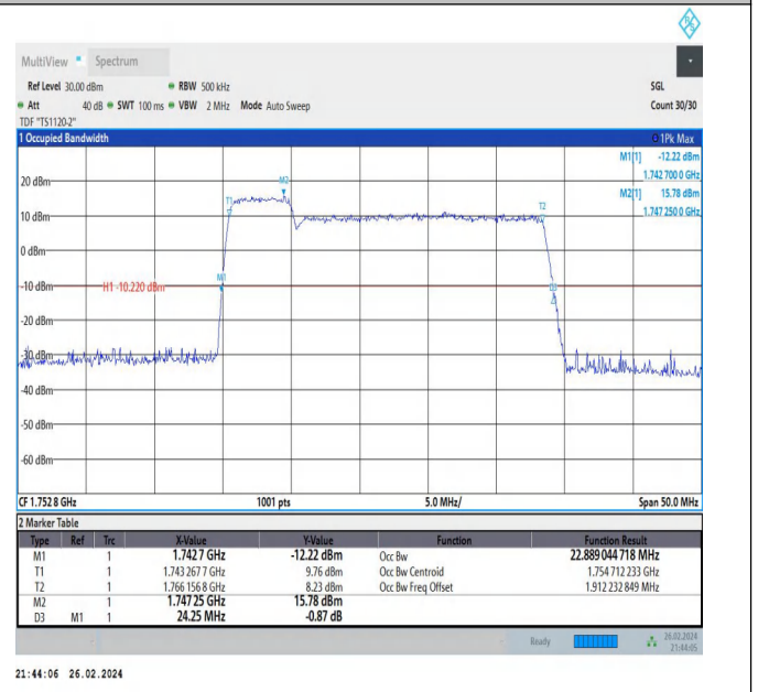
66-66-5MHz-20MHz-256QAM-256QAM-132328-132472-25RB#0-100RB#0-PASS
