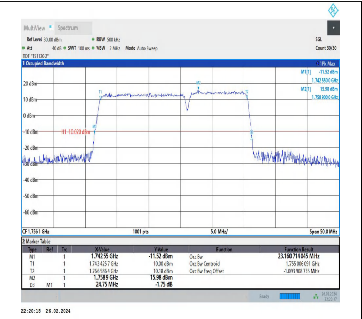
66-66-15MHz-10MHz-16QAM-16QAM-132373-132493-75RB#0-50RB#0-PASS
