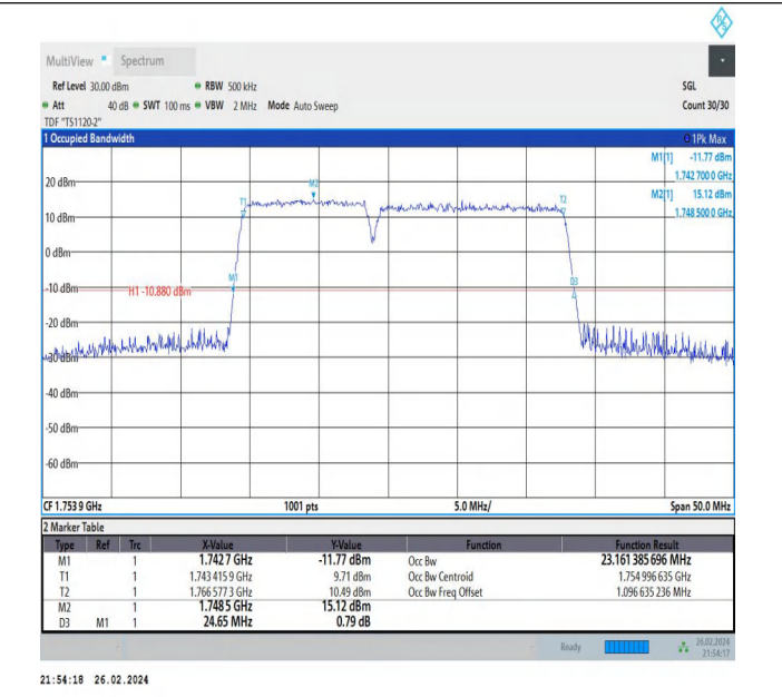
66-66-10MHz-15MHz-16QAM-16QAM-132351-132471-50RB#0-75RB#0-PASS
