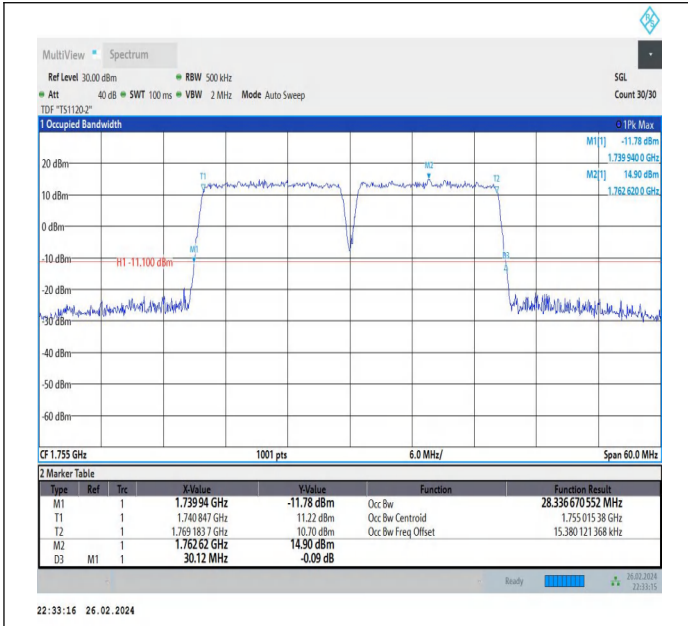
66-66-15MHz-15MHz-QPSK-QPSK-132347-132497-75RB#0-75RB#0-PASS
