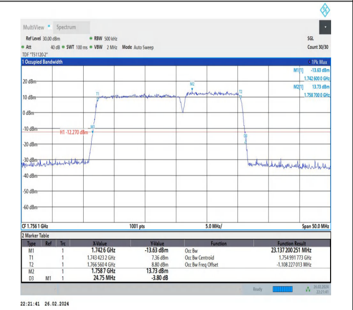
66-66-15MHz-10MHz-256QAM-256QAM-132373-132493-75RB#0-50RB#0-PASS
