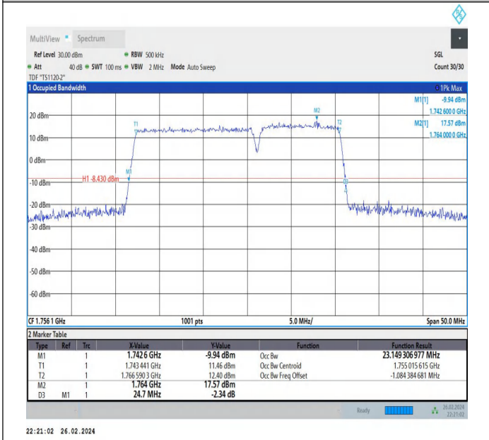
66-66-15MHz-10MHz-64QAM-64QAM-132373-132493-75RB#0-50RB#0-PASS
