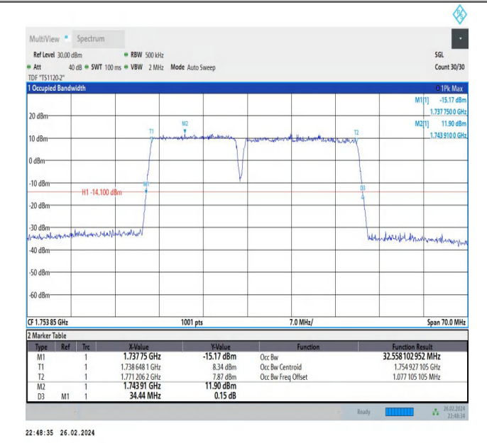
66-66-15MHz-20MHz-256QAM-256QAM-132325-132496-75RB#0-100RB#0-PASS
