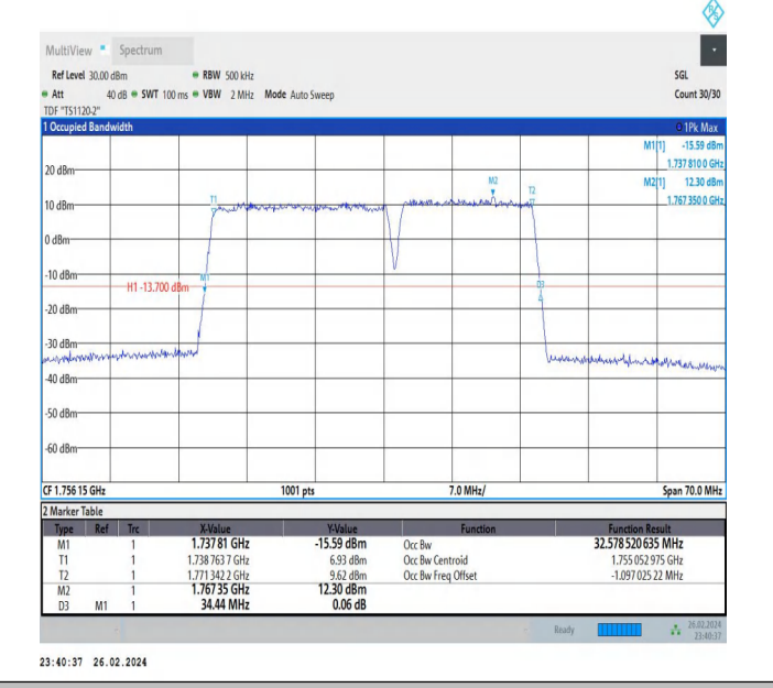
66-66-20MHz-15MHz-256QAM-256QAM-132348-132519-100RB#0-75RB#0-PASS
