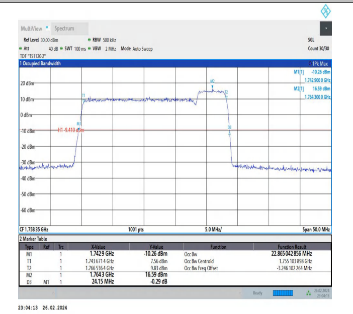
66-66-20MHz-5MHz-256QAM-256QAM-132397-132514-100RB#0-25RB#0-PASS
