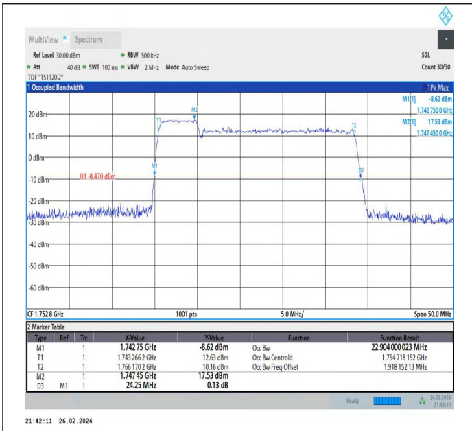
66-66-5MHz-20MHz-QPSK-QPSK-132328-132472-25RB#0-100RB#0-PASS
