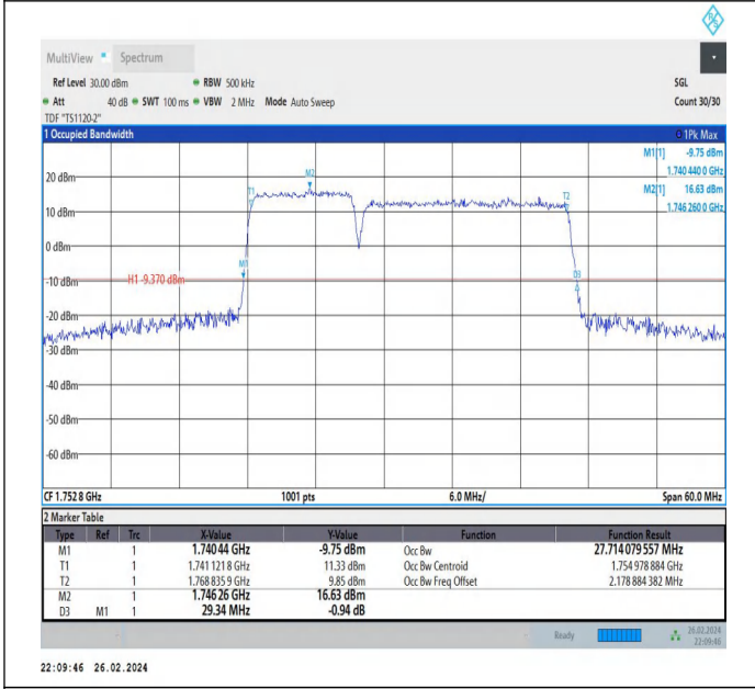
66-66-10MHz-20MHz-64QAM-64QAM-132328-132472-50RB#0-100RB#0-PASS
