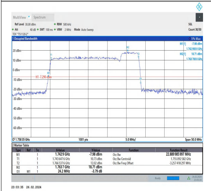
66-66-20MHz-5MHz-64QAM-64QAM-132397-132514-100RB#0-25RB#0-PASS
