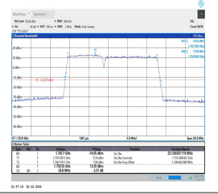
66-66-10MHz-15MHz-256QAM-256QAM-132351-132471-50RB#0-75RB#0-PASS
