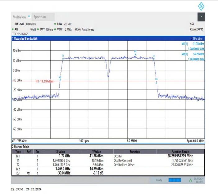
66-66-15MHz-15MHz-16QAM-16QAM-132347-132497-75RB#0-75RB#0-PASS
