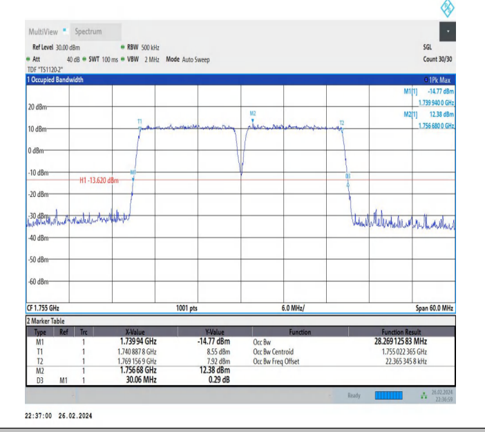
66-66-15MHz-15MHz-256QAM-256QAM-132347-132497-75RB#0-75RB#0-PASS
