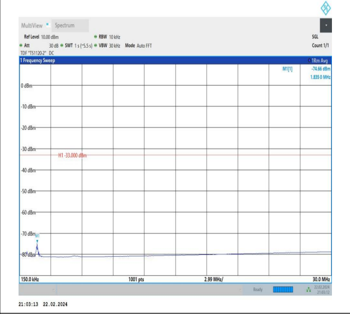
66-66-5MHz-15MHz-QPSK-QPSK-132504-132597-1RB#0-0R B#0-0.15~30MHz-PASS
