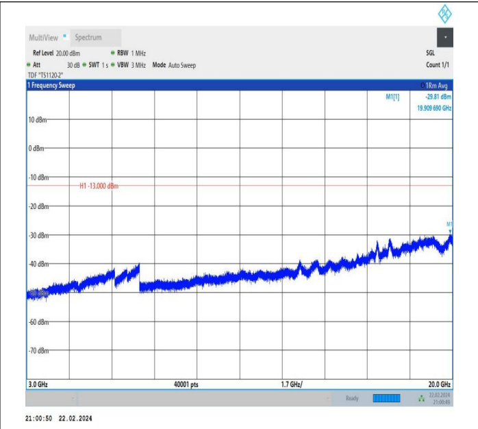
66-66-5MHz-15MHz-QPSK-QPSK-132353-132446-1RB#0-1R B#74-3000~20000MHz-PASS
