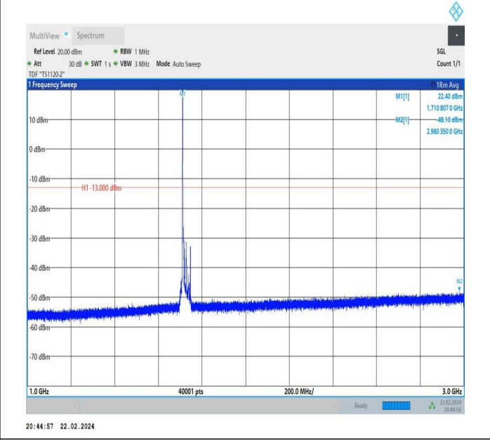
66-66-5MHz-15MHz-QPSK-QPSK-132002-132095-1RB#0-0R B#0-1000~3000MHz-PASS
