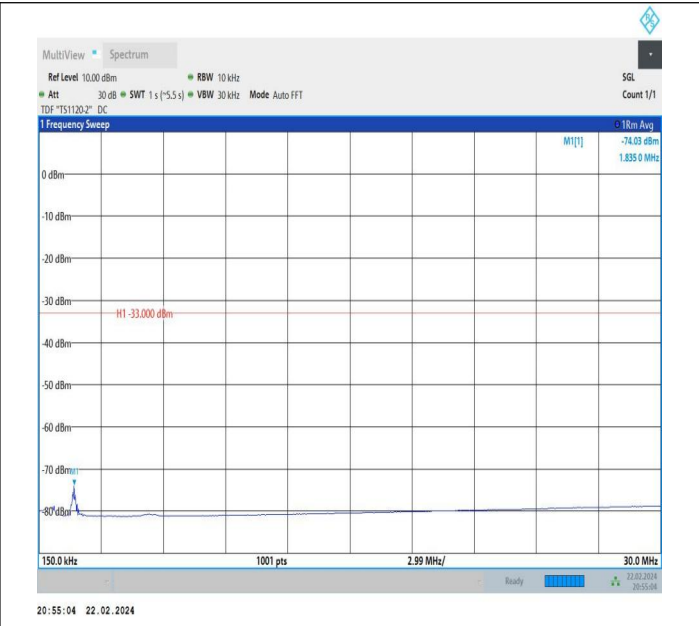
66-66-5MHz-15MHz-QPSK-QPSK-132353-132446-1RB#24-0 RB#0-0.15~30MHz-PASS
