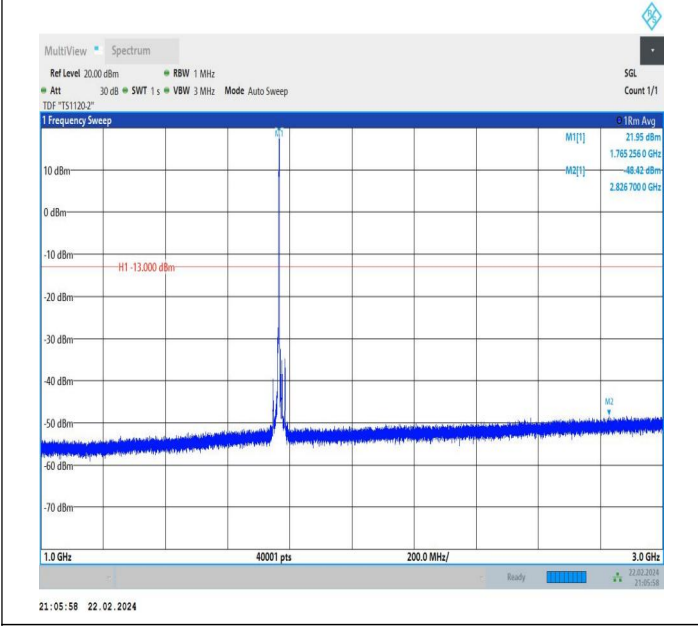
66-66-5MHz-15MHz-QPSK-QPSK-132504-132597-1RB#24-0 RB#0-1000~3000MHz-PASS
