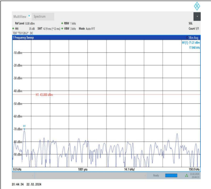
66-66-5MHz-15MHz-QPSK-QPSK-132002-132095-1RB#0-0R B#0-0.009~0.15MHz-PASS
