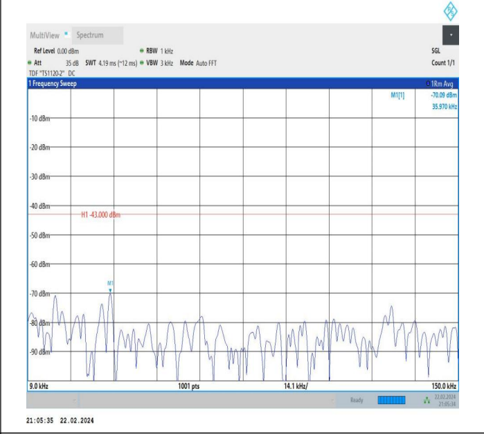
66-66-5MHz-15MHz-QPSK-QPSK-132504-132597-1RB#24-0 RB#0-0.009~0.15MHz-PASS
