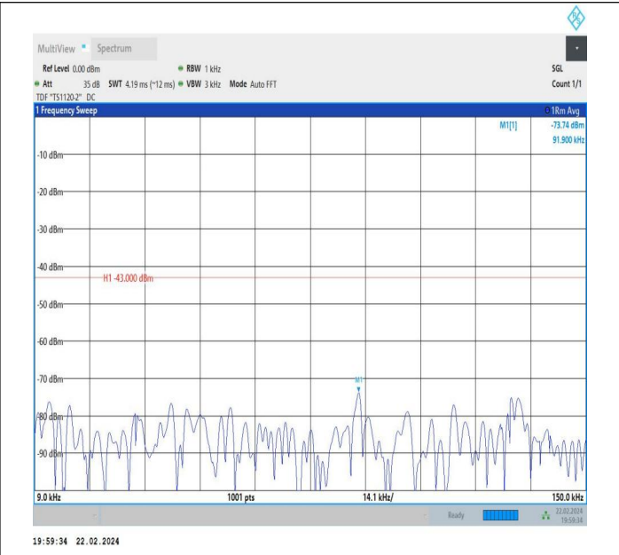
66-66-10MHz-5MHz-QPSK-QPSK-132572-132644-1RB#49-0 RB#0-0.009~0.15MHz-PASS
