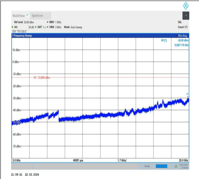
66-66-5MHz-15MHz-QPSK-QPSK-132504-132597-1RB#0-1R B#74-3000~20000MHz-PASS
