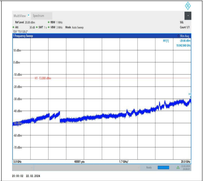
66-66-10MHz-5MHz-QPSK-QPSK-132572-132644-1RB#49-0 RB#0-3000~20000MHz-PASS
