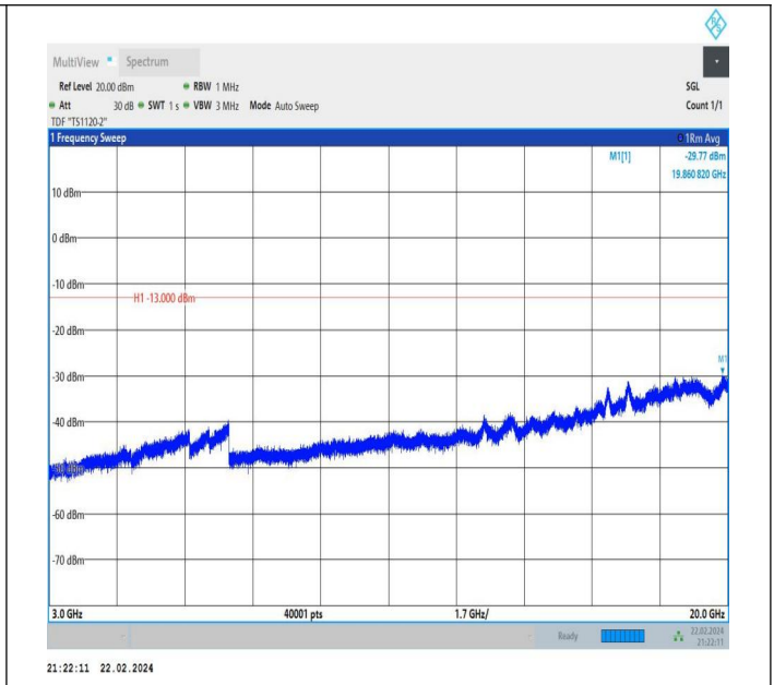
66-66-15MHz-5MHz-QPSK-QPSK-132047-132140-1RB#0-0R B#0-3000~20000MHz-PASS
