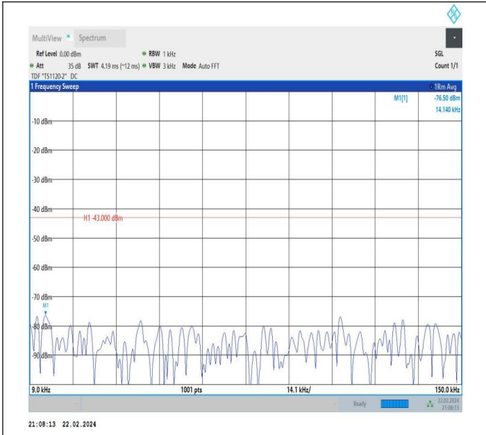
66-66-5MHz-15MHz-QPSK-QPSK-132504-132597-1RB#0-1R B#74-0.009~0.15MHz-PASS
