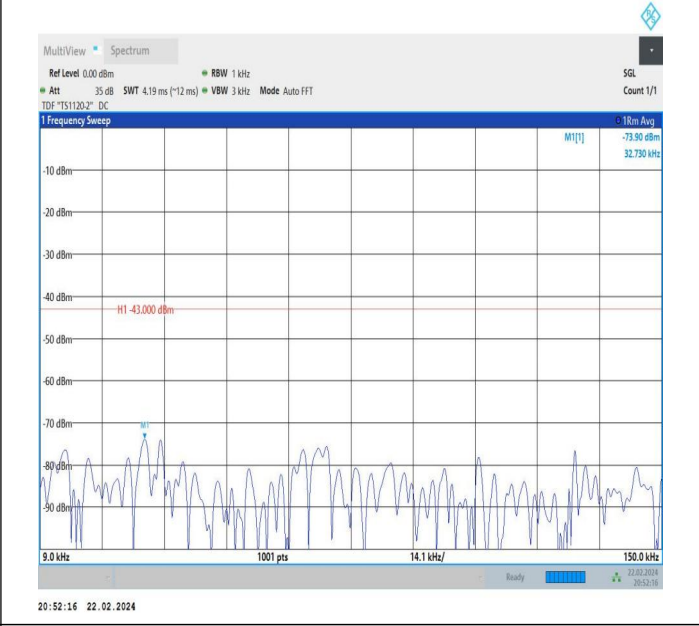
66-66-5MHz-15MHz-QPSK-QPSK-132353-132446-1RB#0-0R B#0-0.009~0.15MHz-PASS
