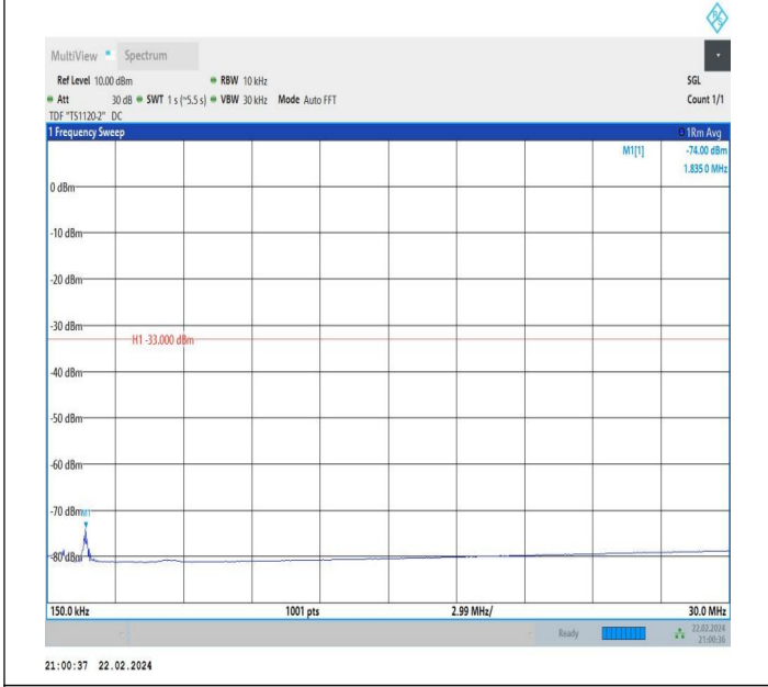
66-66-5MHz-15MHz-QPSK-QPSK-132353-132446-1RB#0-1R B#74-0.15~30MHz-PASS
