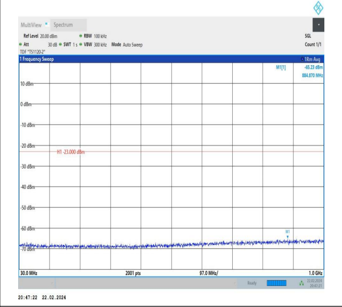
66-66-5MHz-15MHz-QPSK-QPSK-132002-132095-1RB#24-0 RB#0-30~1000MHz-PASS
