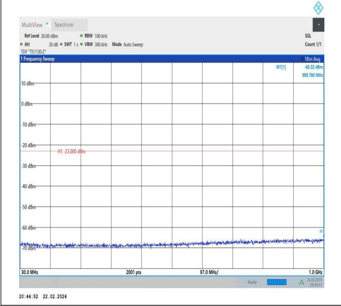
66-66-5MHz-15MHz-QPSK-QPSK-132002-132095-1RB#0-0R B#0-30~1000MHz-PASS
