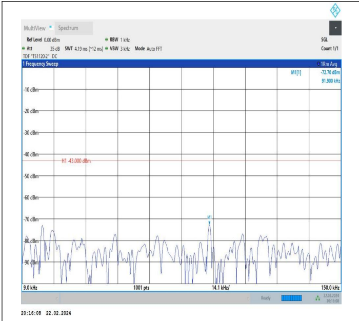
66-66-10MHz-10MHz-QPSK-QPSK-132022-132121-1RB#49-ORB#0-0.009~0.15MHz-PASS
