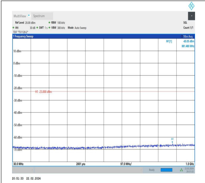
66-66-5MHz-15MHz-QPSK-QPSK-132002-132095-1RB#0-1R B#74-30~1000MHz-PASS
