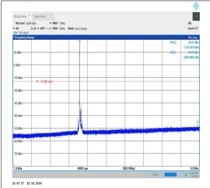
66-66-5MHz-15MHz-QPSK-QPSK-132002-132095-1RB#24-0 RB#0-1000~3000MHz-PASS
