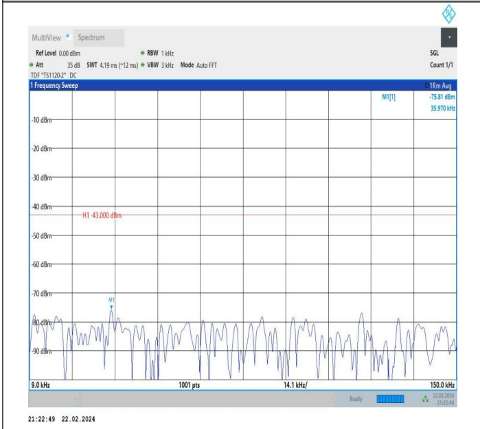
66-66-15MHz-5MHz-QPSK-QPSK-132047-132140-1RB#74-0 RB#0-0.009~0.15MHz-PASS
