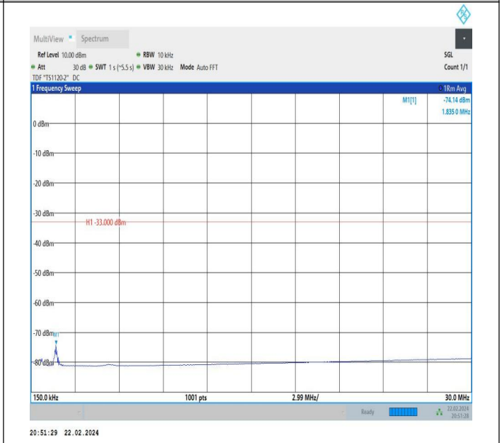
66-66-5MHz-15MHz-QPSK-QPSK-132002-132095-1RB#0-1R B#74-0.15~30MHz-PASS
