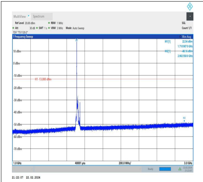
66-66-15MHz-5MHz-QPSK-QPSK-132047-132140-1RB#0-0R B#0-1000~3000MHz-PASS
