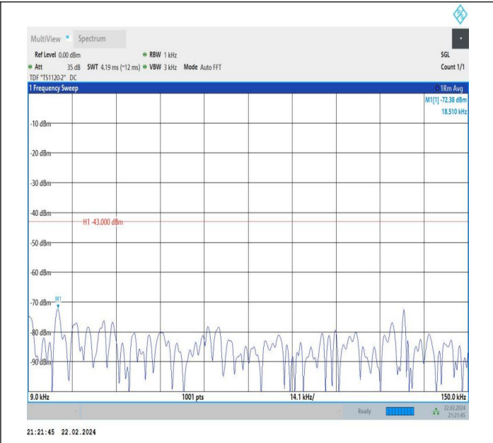
66-66-15MHz-5MHz-QPSK-QPSK-132047-132140-1RB#0-0R B#0-0.009~0.15MHz-PASS
