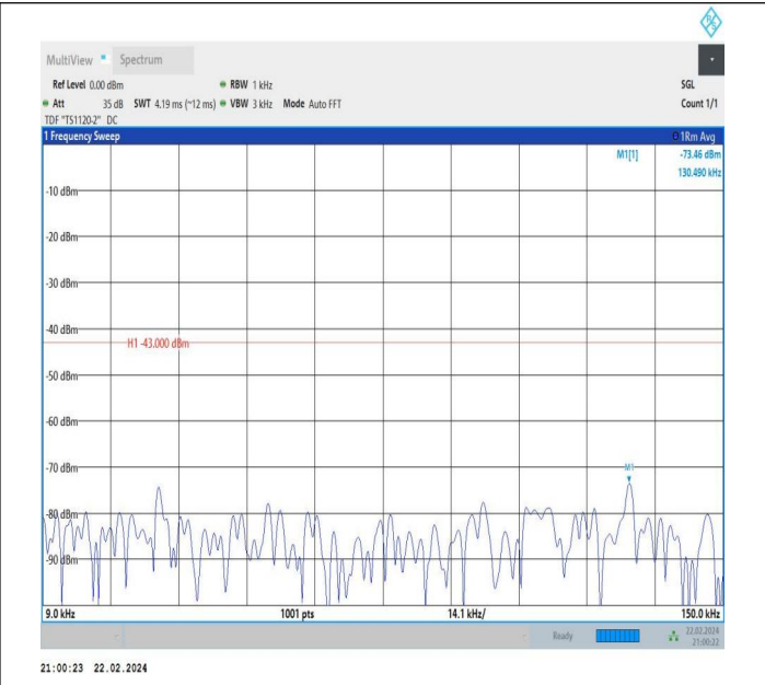
66-66-5MHz-15MHz-QPSK-QPSK-132353-132446-1RB#0-1R B#74-0.009~0.15MHz-PASS
