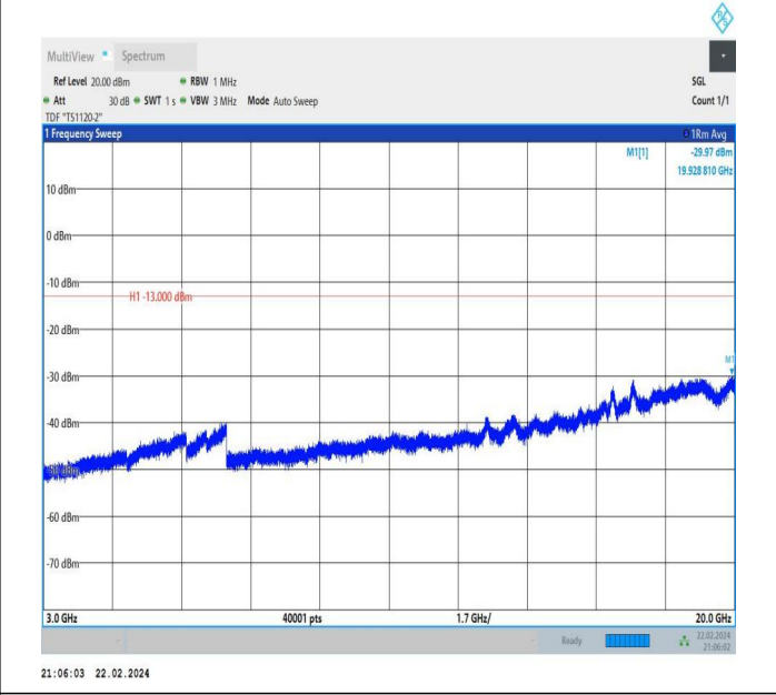
66-66-5MHz-15MHz-QPSK-QPSK-132504-132597-1RB#24-0 RB#0-3000~20000MHz-PASS
