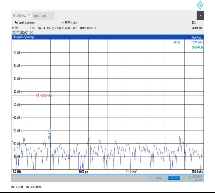
66-66-10MHz-10MHz-QPSK-QPSK-132523-132622-1RB#0-1RB#49-0.009~0.15MHz-PASS
