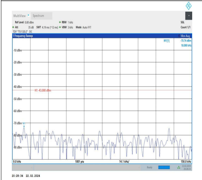
66-66-10MHz-10MHz-QPSK-QPSK-132523-132622-1RB#49- ORB#0-0.009~0.15MHz-PASS
