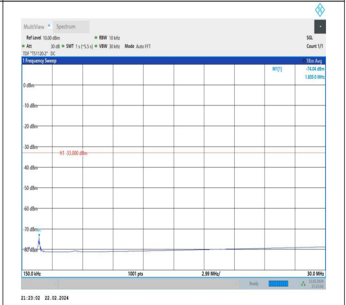
66-66-15MHz-5MHz-QPSK-QPSK-132047-132140-1RB#74-0 RB#0-0.15~30MHz-PASS
