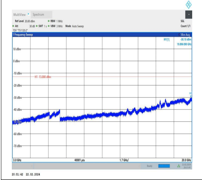
66-66-5MHz-15MHz-QPSK-QPSK-132002-132095-1RB#0-1R B#74-3000~20000MHz-PASS
