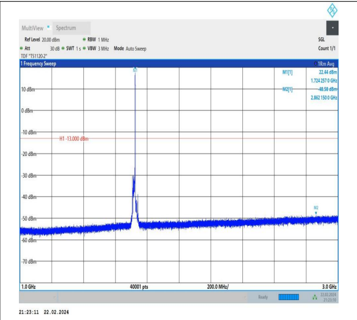
66-66-15MHz-5MHz-QPSK-QPSK-132047-132140-1RB#74-0 RB#0-1000~3000MHz-PASS
