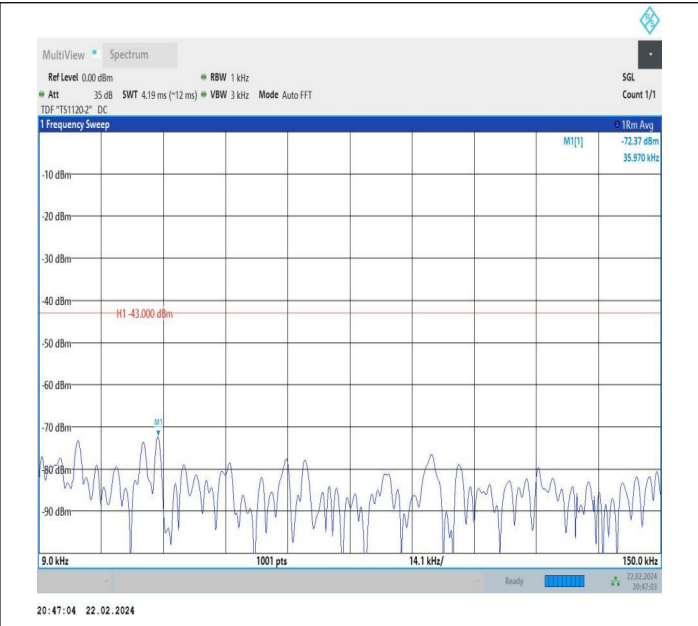
66-66-5MHz-15MHz-QPSK-QPSK-132002-132095-1RB#24-0 RB#0-0.009~0.15MHz-PASS
