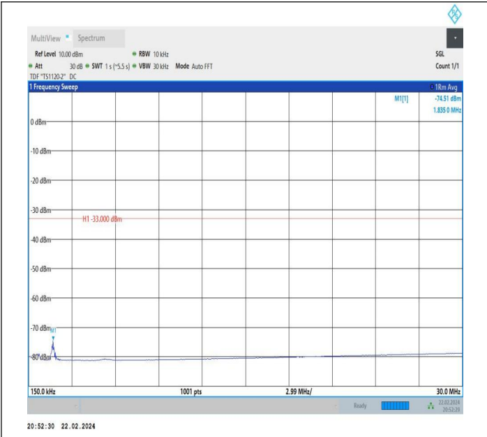
66-66-5MHz-15MHz-QPSK-QPSK-132353-132446-1RB#0-0R B#0-0.15~30MHz-PASS
