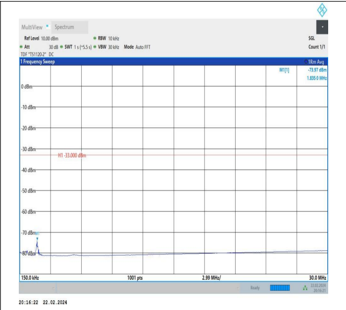
66-66-10MHz-10MHz-QPSK-QPSK-132022-132121-1RB#49-ORB#0-0.15~30MHz-PASS
