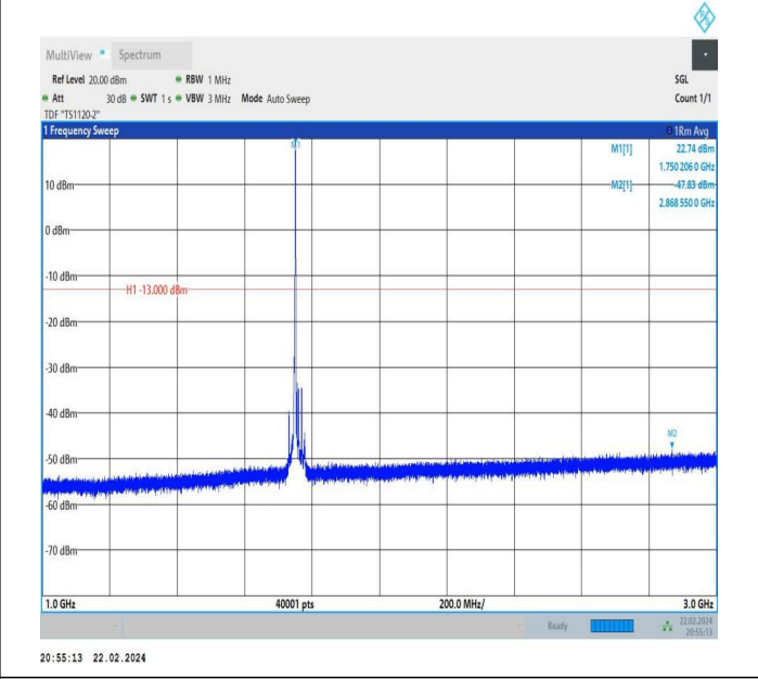
66-66-5MHz-15MHz-QPSK-QPSK-132353-132446-1RB#24-0 RB#0-1000~3000MHz-PASS
