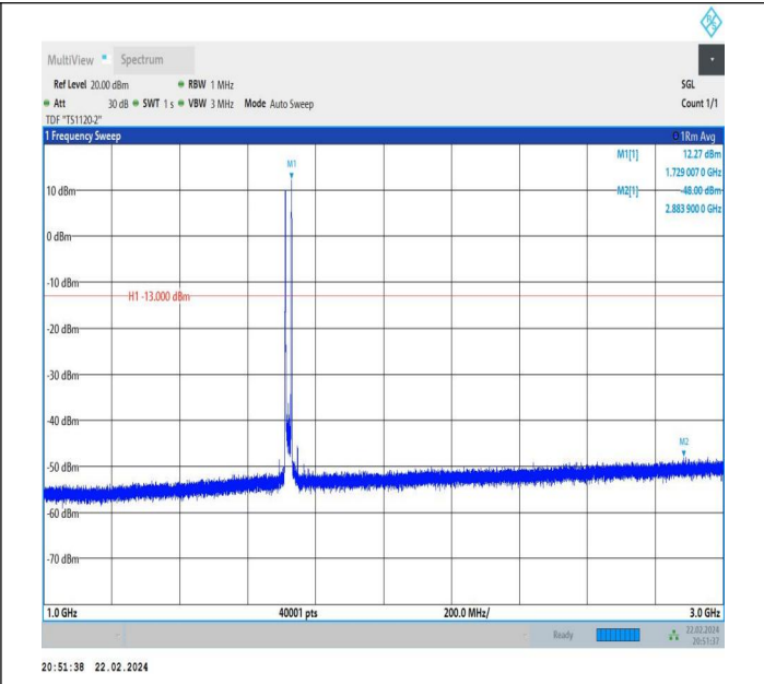
66-66-5MHz-15MHz-QPSK-QPSK-132002-132095-1RB#0-1R B#74-1000~3000MHz-PASS
