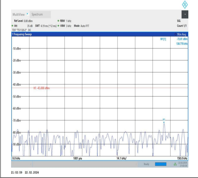
66-66-5MHz-15MHz-QPSK-QPSK-132504-132597-1RB#0-0R B#0-0.009~0.15MHz-PASS
