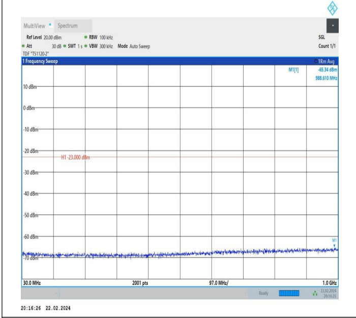
66-66-10MHz-10MHz-QPSK-QPSK-132022-132121-1RB#49-ORB#0-30~1000MHz-PASS
