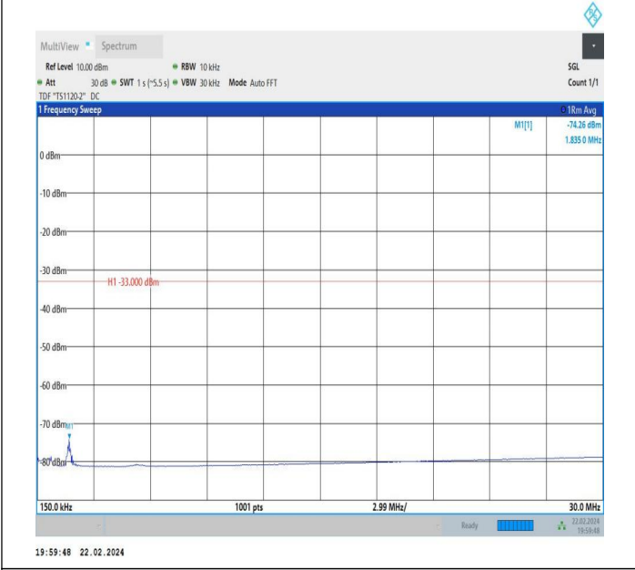
66-66-10MHz-5MHz-QPSK-QPSK-132572-132644-1RB#49-0 RB#0-0.15~30MHz-PASS
