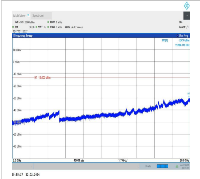
66-66-5MHz-15MHz-QPSK-QPSK-132353-132446-1RB#24-0 RB#0-3000~20000MHz-PASS
