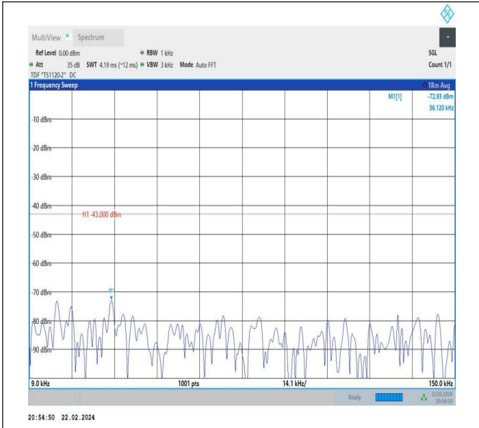
66-66-5MHz-15MHz-QPSK-QPSK-132353-132446-1RB#24-0 RB#0-0.009~0.15MHz-PASS
