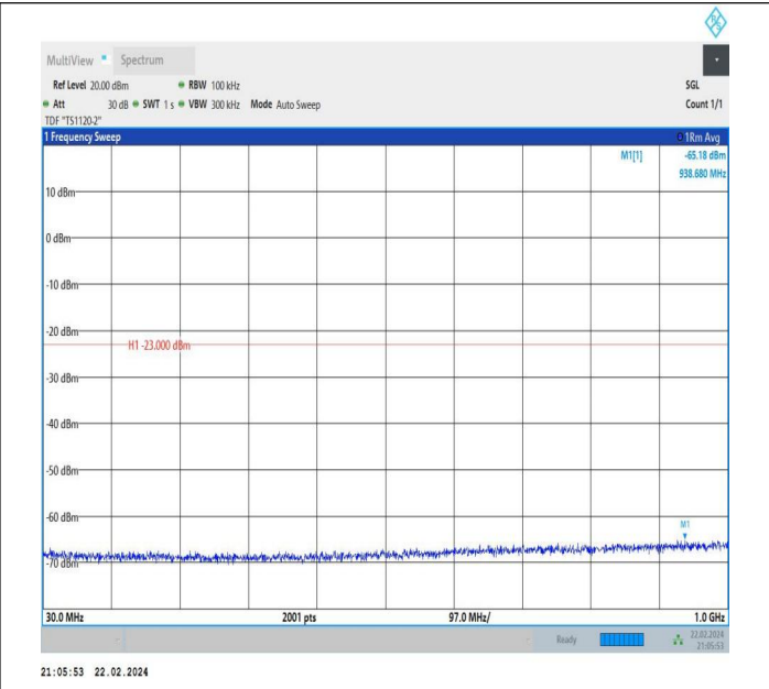
66-66-5MHz-15MHz-QPSK-QPSK-132504-132597-1RB#24-0 RB#0-30~1000MHz-PASS
