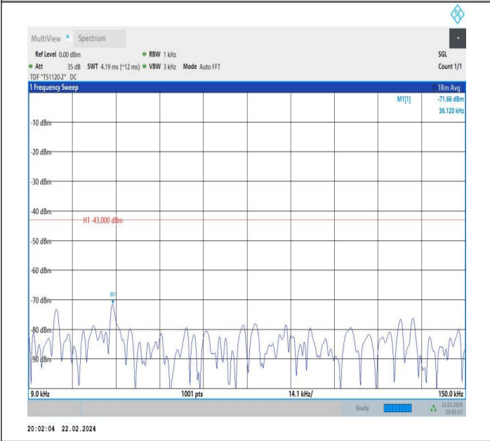
66-66-10MHz-5MHz-QPSK-QPSK-132572-132644-1RB#0-1R B#24-0.009~0.15MHz-PASS
