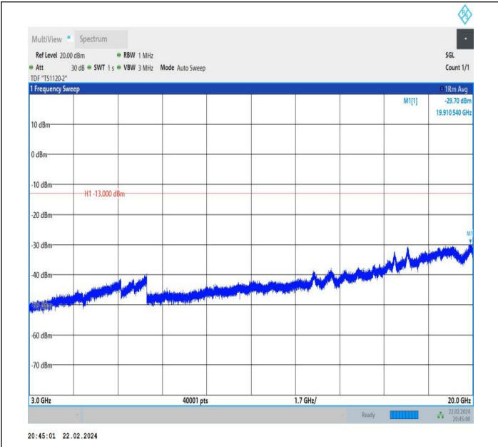
66-66-5MHz-15MHz-QPSK-QPSK-132002-132095-1RB#0-0R B#0-3000~20000MHz-PASS
