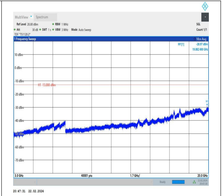
66-66-5MHz-15MHz-QPSK-QPSK-132002-132095-1RB#24-0 RB#0-3000~20000MHz-PASS
