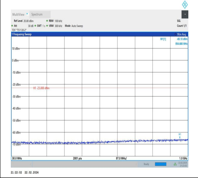
66-66-15MHz-5MHz-QPSK-QPSK-132047-132140-1RB#0-0R B#0-30~1000MHz-PASS
