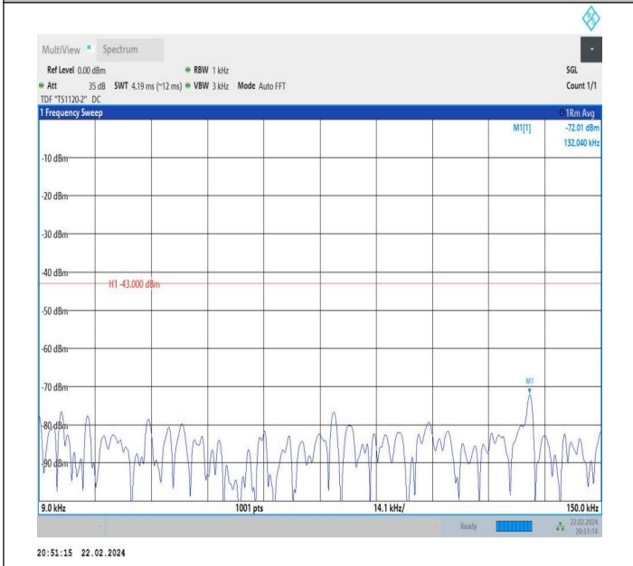
66-66-5MHz-15MHz-QPSK-QPSK-132002-132095-1RB#0-1R B#74-0.009~0.15MHz-PASS
