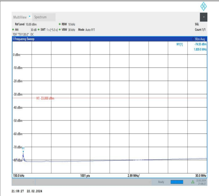
66-66-5MHz-15MHz-QPSK-QPSK-132504-132597-1RB#0-1R B#74-0.15~30MHz-PASS
