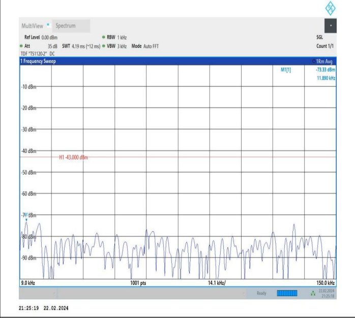
66-66-15MHz-5MHz-QPSK-QPSK-132047-132140-1RB#0-1R B#24-0.009~0.15MHz-PASS
