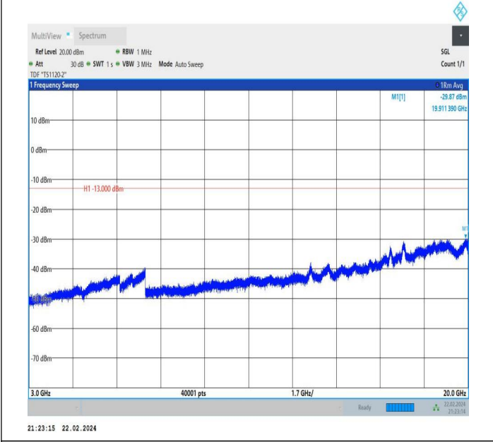
66-66-15MHz-5MHz-QPSK-QPSK-132047-132140-1RB#74-0 RB#0-3000~20000MHz-PASS
