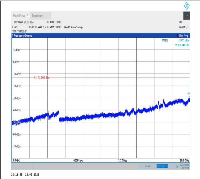
66-66-10MHz-10MHz-QPSK-QPSK-132022-132121-1RB#49-ORB#0-3000~20000MHz-PASS
