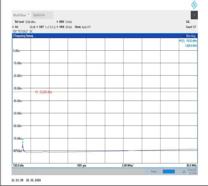
66-66-15MHz-5MHz-QPSK-QPSK-132047-132140-1RB#0-0R B#0-0.15~30MHz-PASS
