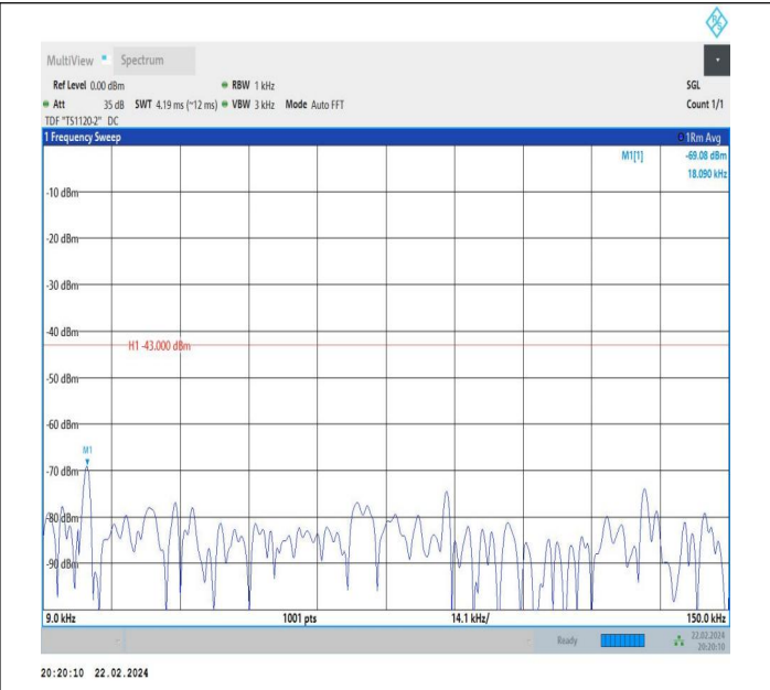
66-66-10MHz-10MHz-QPSK-QPSK-132022-132121-1RB#0-1RB#49-0.009~0.15MHz-PASS
