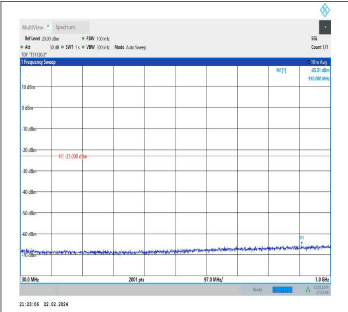
66-66-15MHz-5MHz-QPSK-QPSK-132047-132140-1RB#74-0 RB#0-30~1000MHz-PASS
