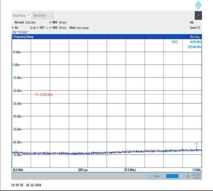
66-66-10MHz-5MHz-QPSK-QPSK-132572-132644-1RB#49-0 RB#0-30~1000MHz-PASS
