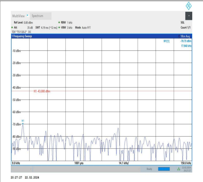
66-66-10MHz-10MHz-QPSK-QPSK-132523-132622-1RB#0-0 RB#0-0.009~0.15MHz-PASS
