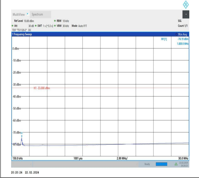
66-66-10MHz-10MHz-QPSK-QPSK-132022-132121-1RB#0-1RB#49-0.15~30MHz-PASS
