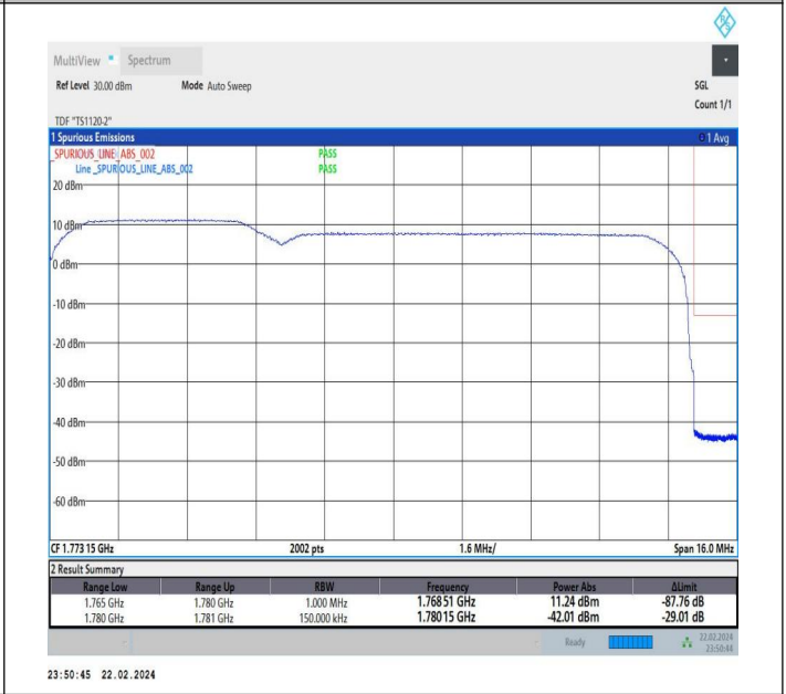
5MHz-10MHz_QPSK@QPSK-QPSK@QPSK_132550-132622_25RB#0@25RB#0-50RB#0@50RB#0
