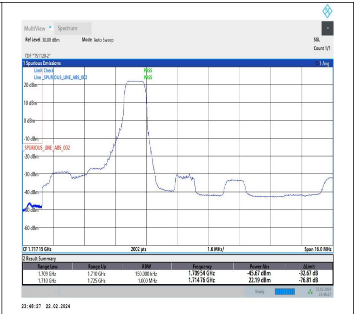
5MHz-10MHz_QPSK@QPSK-QPSK@QPSK_132000-132072_1RB#24@25RB#0-0RB#0@50RB#0
