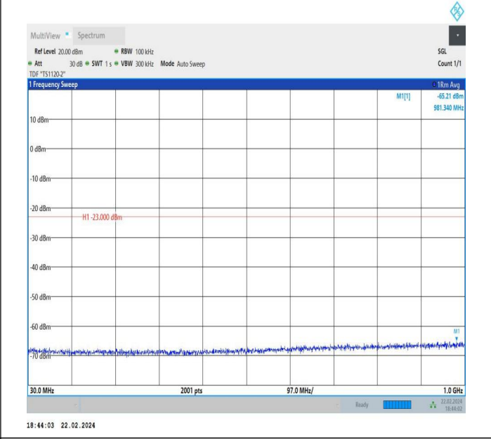
66-66-5MHz-5MHz-QPSK-QPSK-132398-132446-1RB#0-1RB #15-30~1000MHz-PASS
