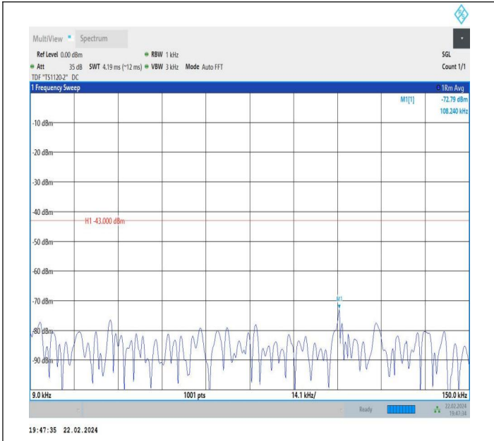
66-66-10MHz-5MHz-QPSK-QPSK-132022-132094-1RB#0-1R B#24-0.009~0.15MHz-PASS
