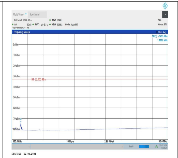
66-66-5MHz-5MHz-QPSK-QPSK-131997-132045-1RB#0-0RB #0-0.15~30MHz-PASS
