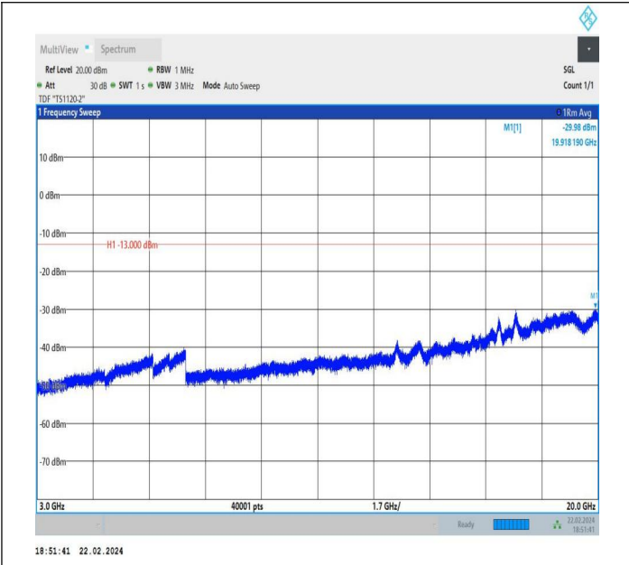
66-66-5MHz-5MHz-QPSK-QPSK-132599-132647-1RB#0-1RB #15-3000~20000MHz-PASS
