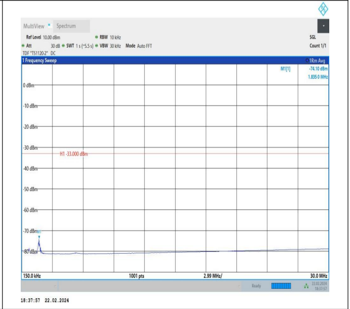
66-66-5MHz-5MHz-QPSK-QPSK-131997-132045-1RB#0-1RB #15-0.15~30MHz-PASS
