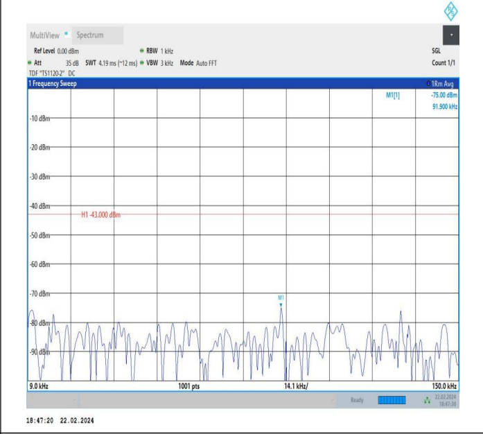
66-66-5MHz-5MHz-QPSK-QPSK-132599-132647-1RB#24-ORB#0-0.009~0.15MHz-PASS
