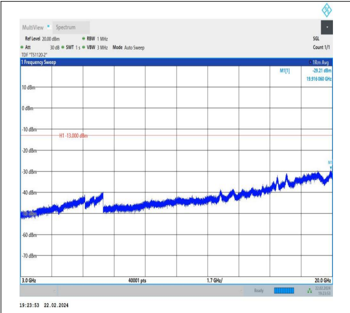
66-66-5MHz-10MHz-QPSK-QPSK-132550-132622-1RB#24-0 RB#0-3000~20000MHz-PASS
