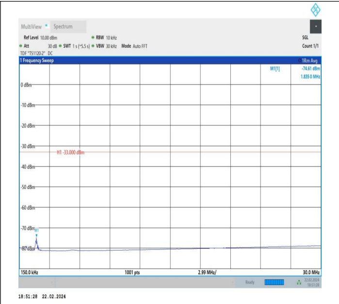
66-66-5MHz-5MHz-QPSK-QPSK-132599-132647-1RB#0-1RB #15-0.15~30MHz-PASS
