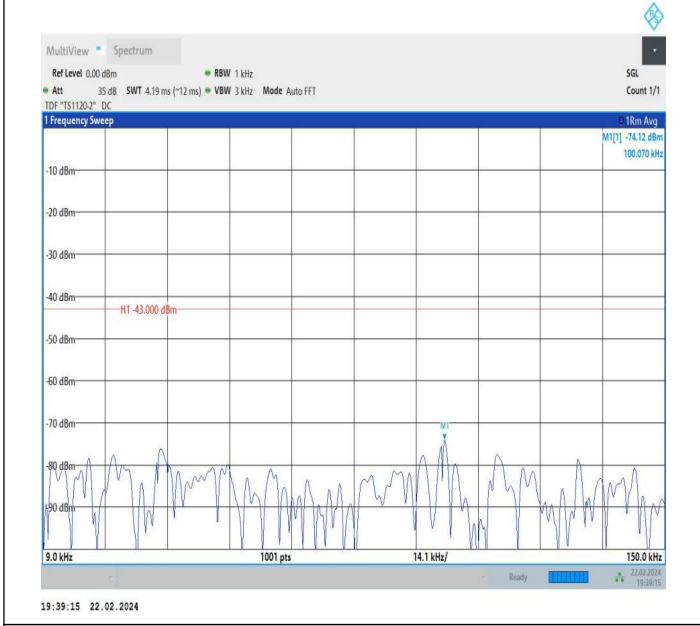
66-66-10MHz-5MHz-QPSK-QPSK-132022-132094-1RB#0-0R B#0-0.009~0.15MHz-PASS
