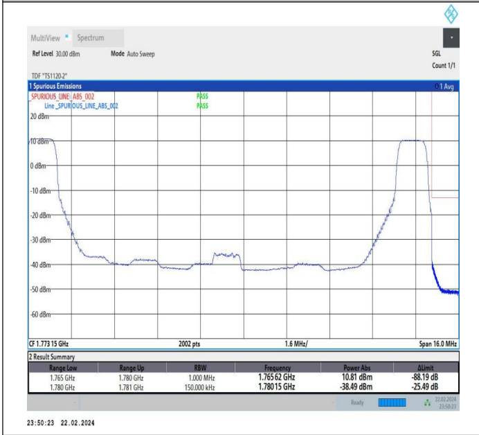
5MHz-10MHz_QPSK@QPSK-QPSK@QPSK_132550-132622_1RB#0@25RB#0-1RB#49@50RB#0
