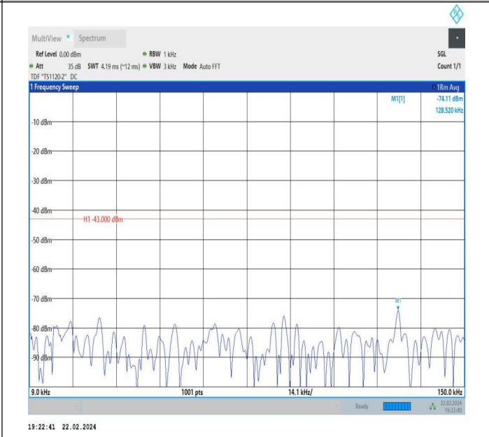
66-66-5MHz-10MHz-QPSK-QPSK-132550-132622-1RB#0-0R B#0-0.009~0.15MHz-PASS
