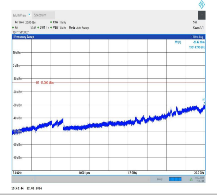
66-66-10MHz-5MHz-QPSK-QPSK-132022-132094-1RB#49-0 RB#0-3000~20000MHz-PASS
