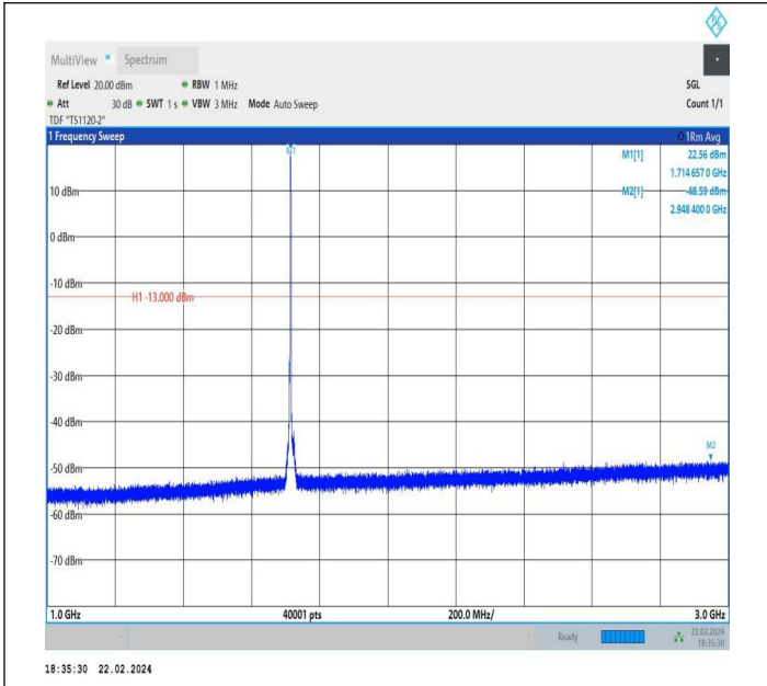
66-66-5MHz-5MHz-QPSK-QPSK-131997-132045-1RB#24-0R B#0-1000~3000MHz-PASS
