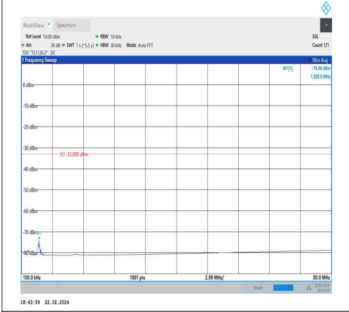
66-66-5MHz-5MHz-QPSK-QPSK-132398-132446-1RB#0-1RB #15-0.15~30MHz-PASS
