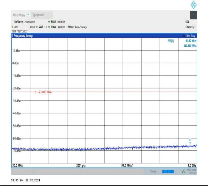
66-66-5MHz-5MHz-QPSK-QPSK-131997-132045-1RB#24-0R B#0-30~1000MHz-PASS
