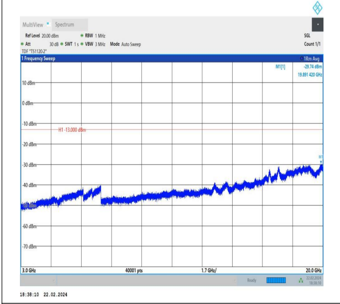
66-66-5MHz-5MHz-QPSK-QPSK-131997-132045-1RB#0-1RB #15-3000~20000MHz-PASS
