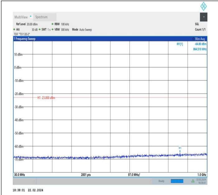
66-66-5MHz-5MHz-QPSK-QPSK-131997-132045-1RB#0-1RB #15-30~1000MHz-PASS
