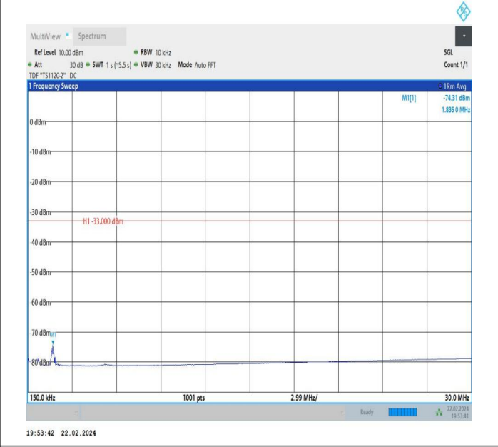
66-66-10MHz-5MHz-QPSK-QPSK-132397-132469-1RB#49-0 RB#0-0.15~30MHz-PASS
