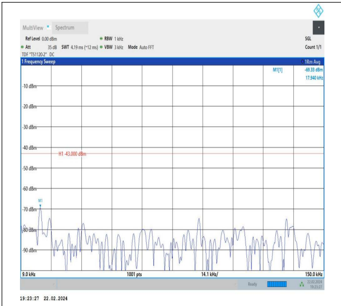
66-66-5MHz-10MHz-QPSK-QPSK-132550-132622-1RB#24-0 RB#0-0.009~0.15MHz-PASS
