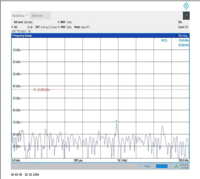
66-66-5MHz-5MHz-QPSK-QPSK-132398-132446-1RB#0-1RB #15-0.009~0.15MHz-PASS
