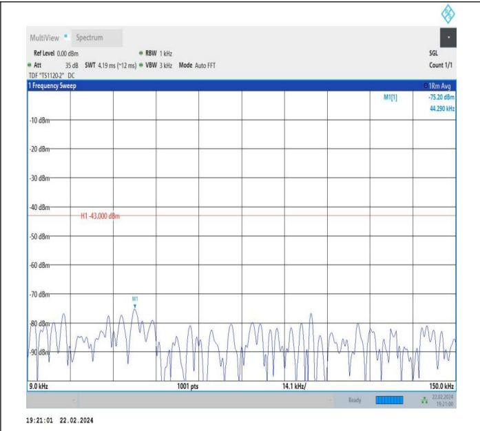
66-66-5MHz-10MHz-QPSK-QPSK-132375-132447-1RB#24-0 RB#0-0.009~0.15MHz-PASS
