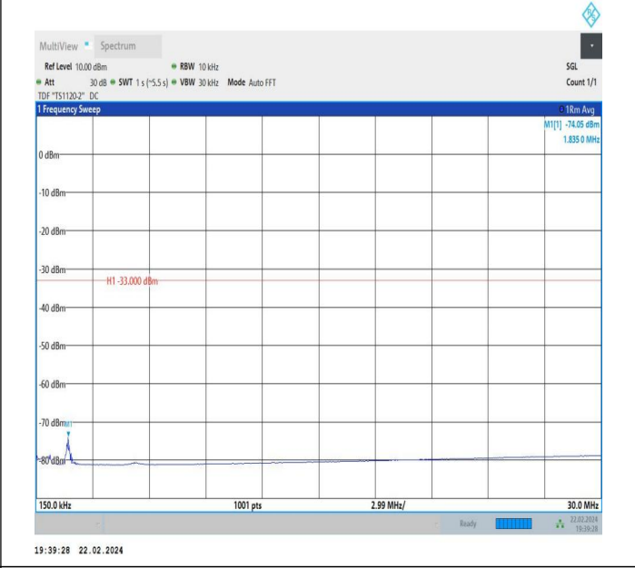
66-66-10MHz-5MHz-QPSK-QPSK-132022-132094-1RB#0-0R B#0-0.15~30MHz-PASS
