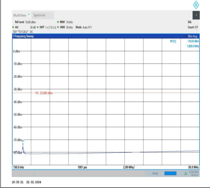
66-66-5MHz-5MHz-QPSK-QPSK-131997-132045-1RB#24-0R B#0-0.15~30MHz-PASS
