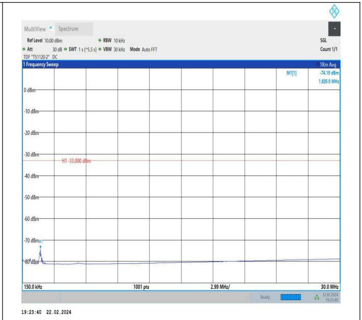
66-66-5MHz-10MHz-QPSK-QPSK-132550-132622-1RB#24-0 RB#0-0.15~30MHz-PASS
