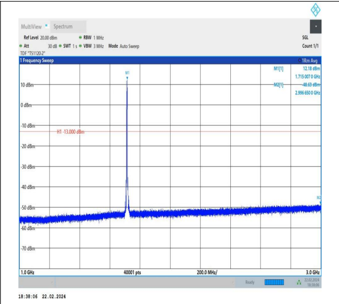
66-66-5MHz-5MHz-QPSK-QPSK-131997-132045-1RB#0-1RB #15-1000~3000MHz-PASS
