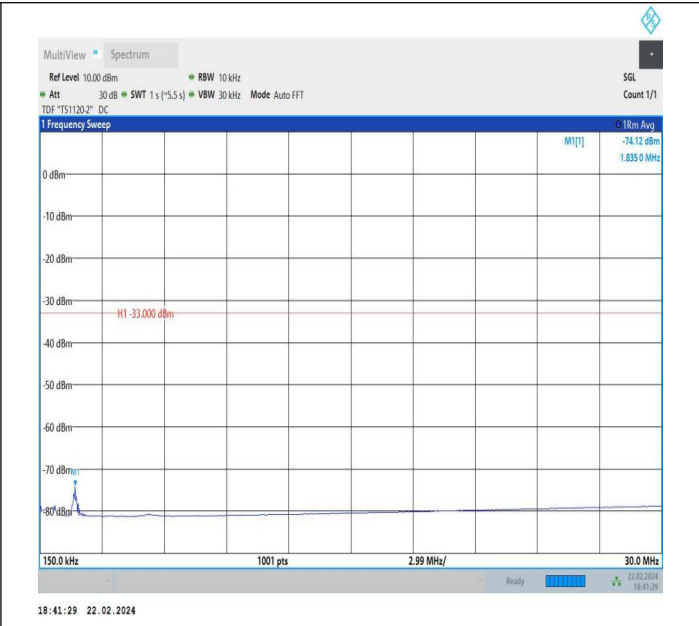
66-66-5MHz-5MHz-QPSK-QPSK-132398-132446-1RB#24-0R B#0-0.15~30MHz-PASS
