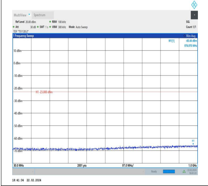
66-66-5MHz-5MHz-QPSK-QPSK-132398-132446-1RB#24-0R B#0-30~1000MHz-PASS
