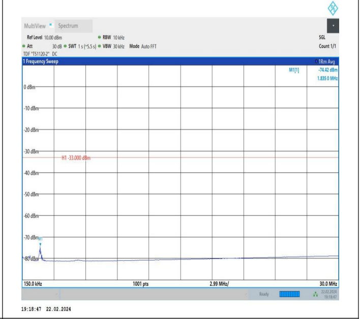
66-66-5MHz-10MHz-QPSK-QPSK-132000-132072-1RB#24-0 RB#0-0.15~30MHz-PASS
