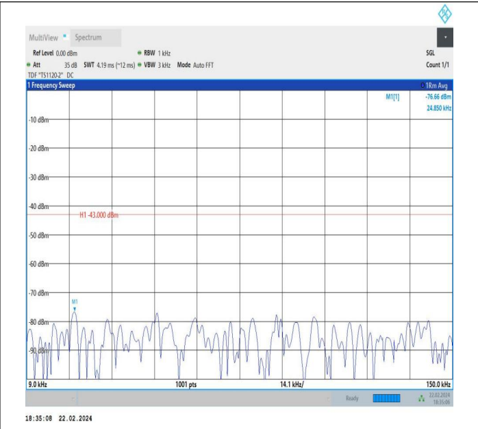
66-66-5MHz-5MHz-QPSK-QPSK-131997-132045-1RB#24-0R B#0-0.009~0.15MHz-PASS
