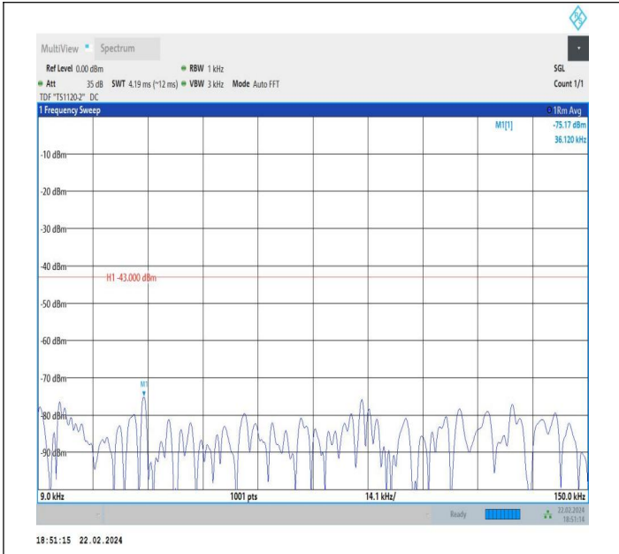
66-66-5MHz-5MHz-QPSK-QPSK-132599-132647-1RB#0-1RB #15-0.009~0.15MHz-PASS
