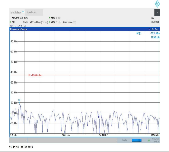
66-66-10MHz-5MHz-QPSK-QPSK-132022-132094-1RB#49-0 RB#0-0.009~0.15MHz-PASS
