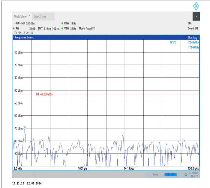
66-66-5MHz-5MHz-QPSK-QPSK-132398-132446-1RB#24-0R B#0-0.009~0.15MHz-PASS
