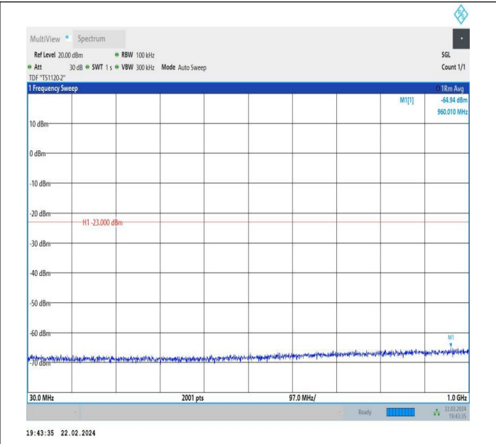
66-66-10MHz-5MHz-QPSK-QPSK-132022-132094-1RB#49-0 RB#0-30~1000MHz-PASS
