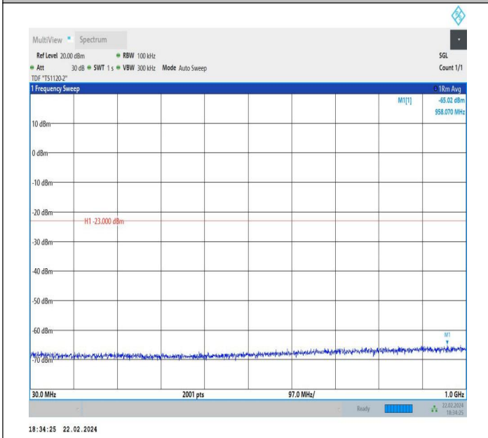
66-66-5MHz-5MHz-QPSK-QPSK-131997-132045-1RB#0-0RB #0-30~1000MHz-PASS
