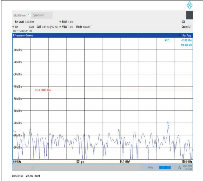
66-66-5MHz-5MHz-QPSK-QPSK-131997-132045-1RB#0-1RB #15-0.009~0.15MHz-PASS
