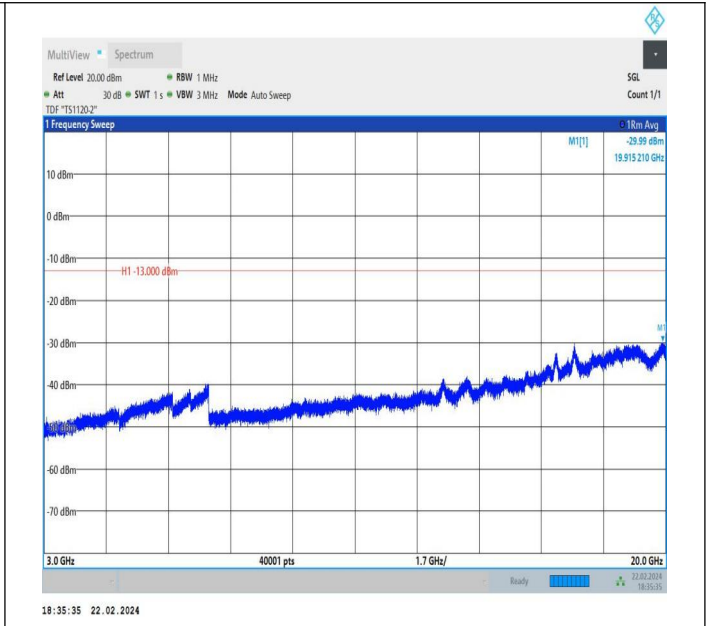
66-66-5MHz-5MHz-QPSK-QPSK-131997-132045-1RB#24-0R B#0-3000~20000MHz-PASS
