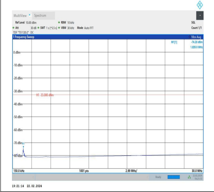
66-66-5MHz-10MHz-QPSK-QPSK-132375-132447-1RB#24-0 RB#0-0.15~30MHz-PASS
