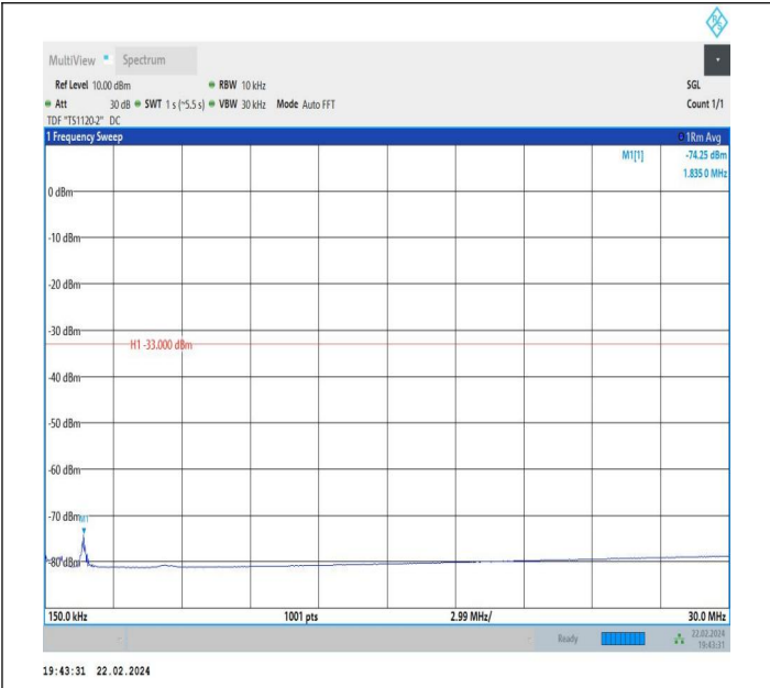
66-66-10MHz-5MHz-QPSK-QPSK-132022-132094-1RB#49-0 RB#0-0.15~30MHz-PASS
