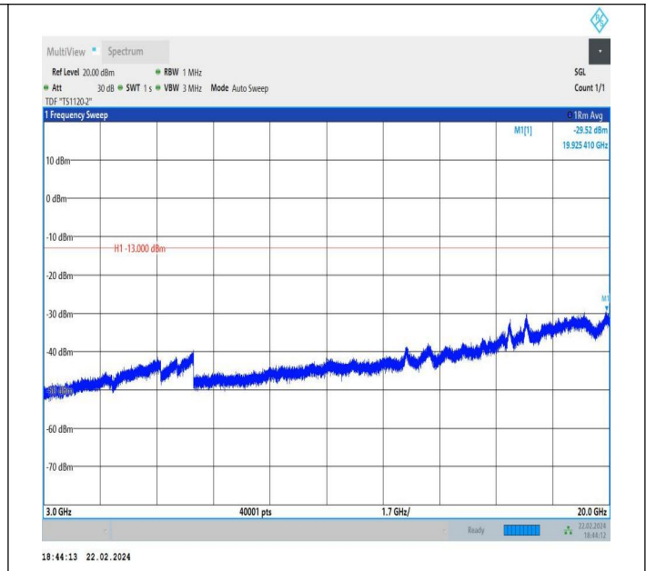
66-66-5MHz-5MHz-QPSK-QPSK-132398-132446-1RB#0-1RB #15-3000~20000MHz-PASS
