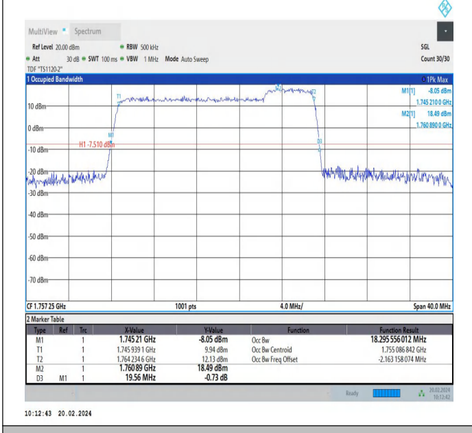
66-66-15MHz-5MHz-64QAM-64QAM-132398-132491-75RB#0-25RB#0-PASS
