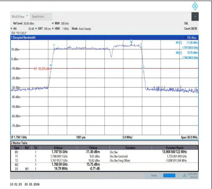
66-66-10MHz-5MHz-16QAM-16QAM-132397-132469-50RB#0-25RB#0-PASS
