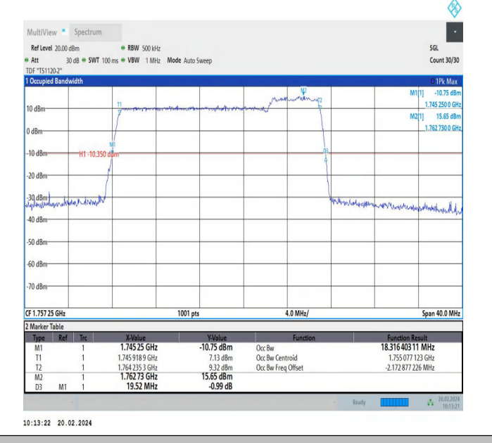
66-66-15MHz-5MHz-256QAM-256QAM-132398-132491-75RB#0-25RB#0-PASS
