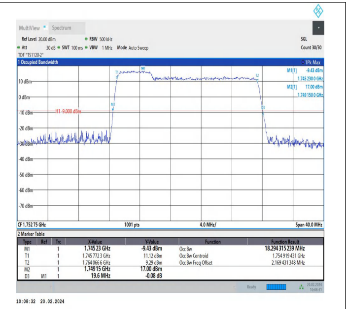
66-66-5MHz-15MHz-16QAM-16QAM-132353-132446-25RB#0-75RB#0-PASS
