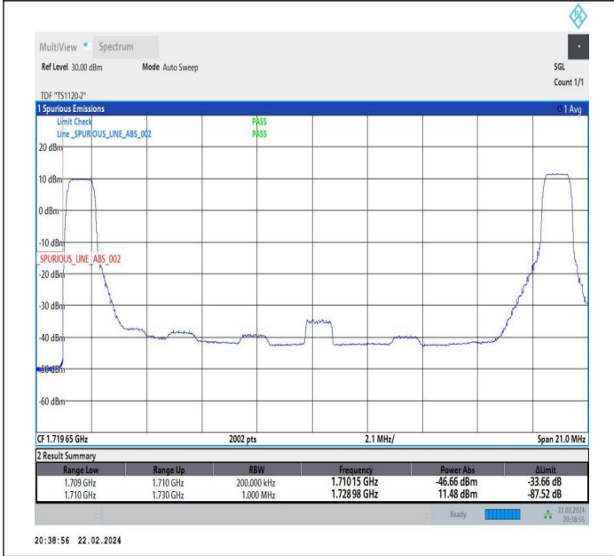
5MHz-15MHz_QPSK@QPSK-QPSK@QPSK_132002-132095_1RB#0@25RB#0-1RB#74@75RB#0
