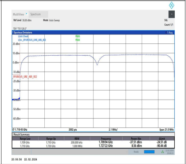
10MHz-10MHz_QPSK@QPSK-QPSK@QPSK_132022-13212 1_50RB#0@50RB#0-50RB#0@50RB#0
