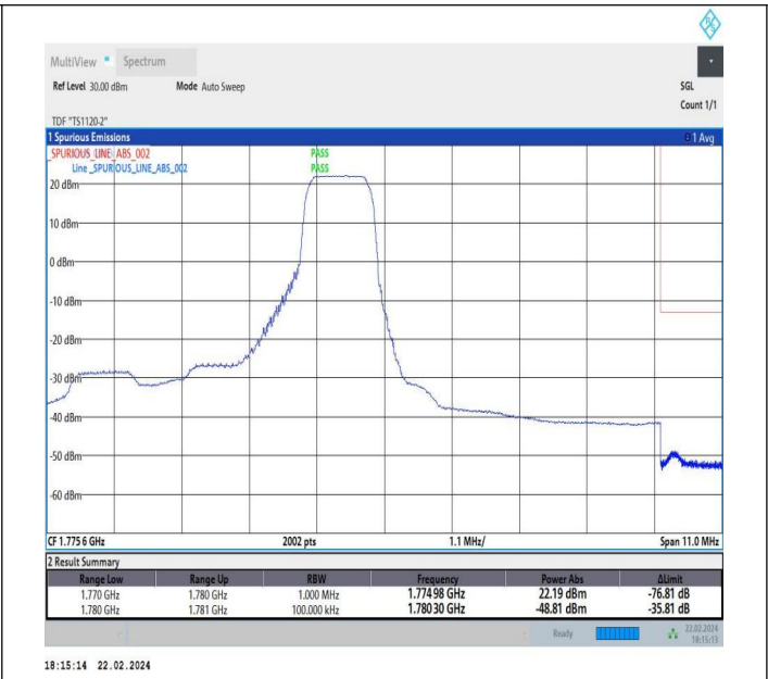
5MHz-5MHz_QPSK@QPSK-QPSK@QPSK_132599-132647_1RB#24@25RB#0-0RB#0@25RB#0
