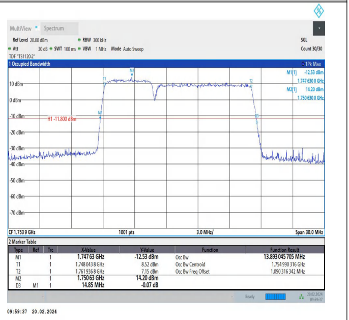
66-66-5MHz-10MHz-256QAM-256QAM-132375-132447-25RB#0-50RB#0-PASS
