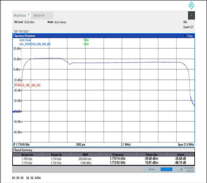
5MHz-15MHz_QPSK@QPSK-QPSK@QPSK_132002-132095_25RB#0@25RB#0-75RB#0@75RB#0
