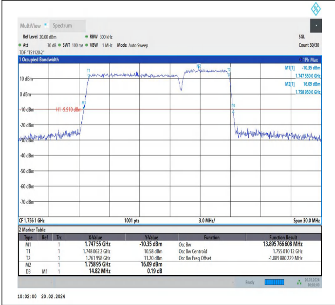
66-66-10MHz-5MHz-64QAM-64QAM-132397-132469-50RB#0-25RB#0-PASS
