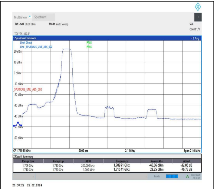
5MHz-15MHz_QPSK@QPSK-QPSK@QPSK_132002-132095_1RB#24@25RB#0-0RB#0@75RB#0
