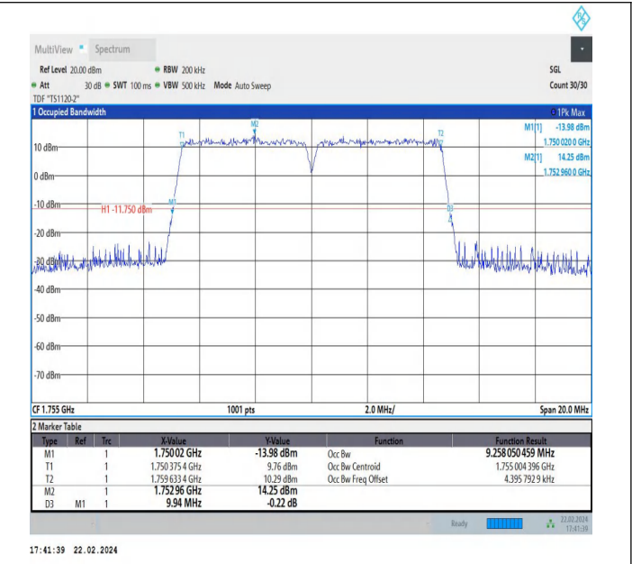
66-66-5MHz-5MHz-16QAM-16QAM-132398-132446-25RB#0-2 5RB#0-PASS
