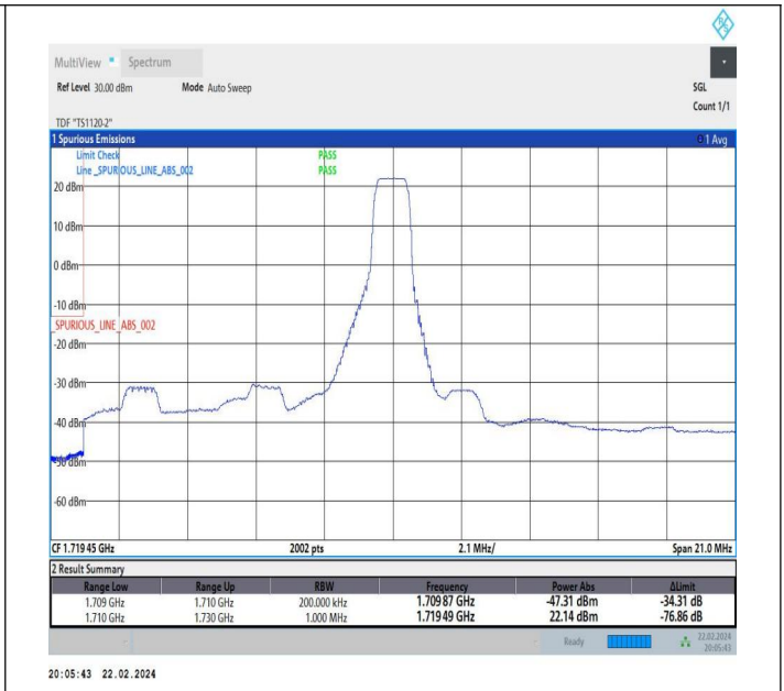
10MHz-10MHz_QPSK@QPSK-QPSK@QPSK_132022-13212 1_1RB#49@50RB#0-0RB#0@50RB#0
