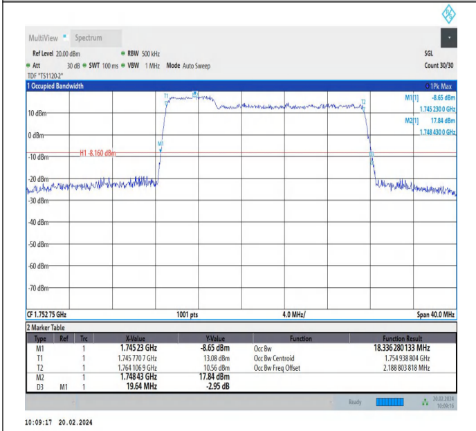
66-66-5MHz-15MHz-64QAM-64QAM-132353-132446-25RB#0-75RB#0-PASS
