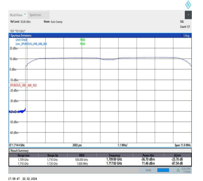
5MHz-5MHz_QPSK@QPSK-QPSK@QPSK_131997-132045_25RB#0@25RB#0-25RB#0@25RB#0
