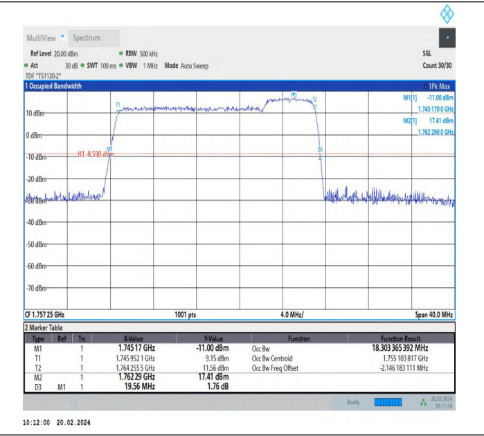
66-66-15MHz-5MHz-16QAM-16QAM-132398-132491-75RB#0-25RB#0-PASS
