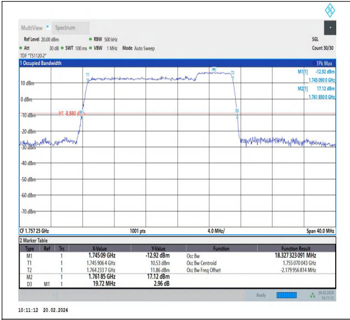
66-66-15MHz-5MHz-QPSK-QPSK-132398-132491-75RB#0-2 5RB#0-PASS
