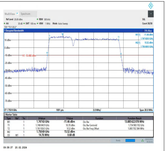
66-66-5MHz-10MHz-16QAM-16QAM-132375-132447-25RB#0-50RB#0-PASS
