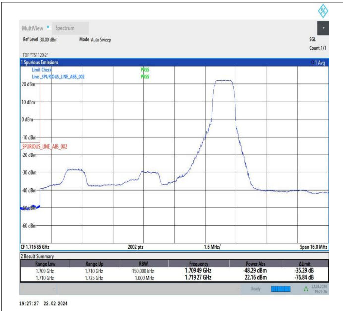
10MHz-5MHz_QPSK@QPSK-QPSK@QPSK_132022-132094 _1RB#49@50RB#0-0RB#0@25RB#0
