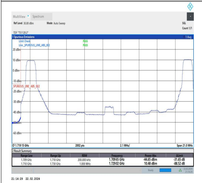
15MHz-5MHz_QPSK@QPSK-QPSK@QPSK_132047-132140_1RB#0@75RB#0-1RB#24@25RB#0
