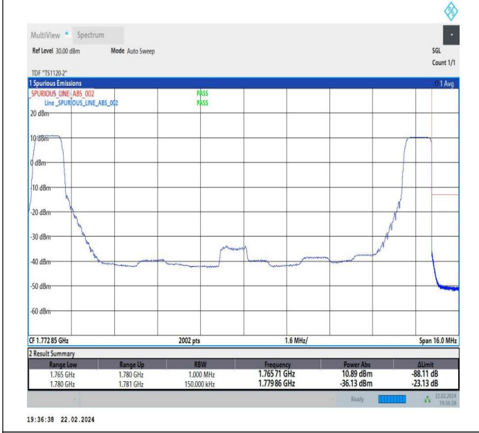
10MHz-5MHz_QPSK@QPSK-QPSK@QPSK_132572-132644_1RB#0@50RB#0-1RB#24@25RB#0
