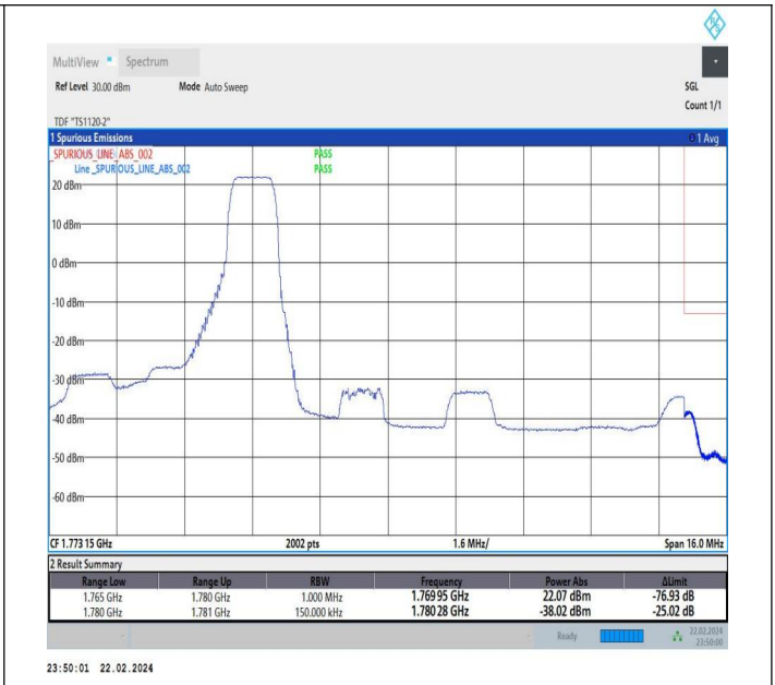
5MHz-10MHz_QPSK@QPSK-QPSK@QPSK_132550-132622 _1RB#24@25RB#0-0RB#0@50RB#0
