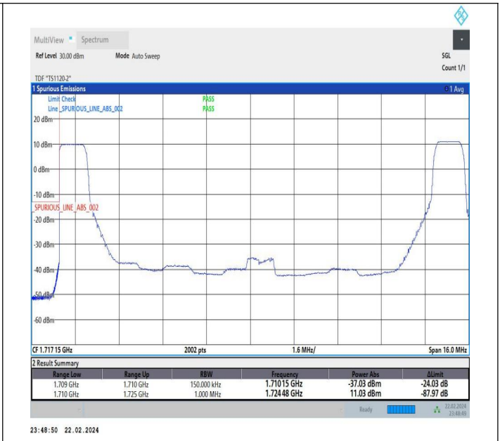
5MHz-10MHz_QPSK@QPSK-QPSK@QPSK_132000-132072_1RB#0@25RB#0-1RB#49@50RB#0
