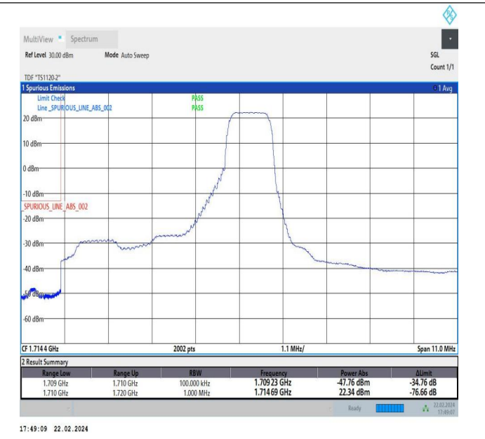
5MHz-5MHz_QPSK@QPSK-QPSK@QPSK_131997-132045_1RB#24@25RB#0-0RB#0@25RB#0
