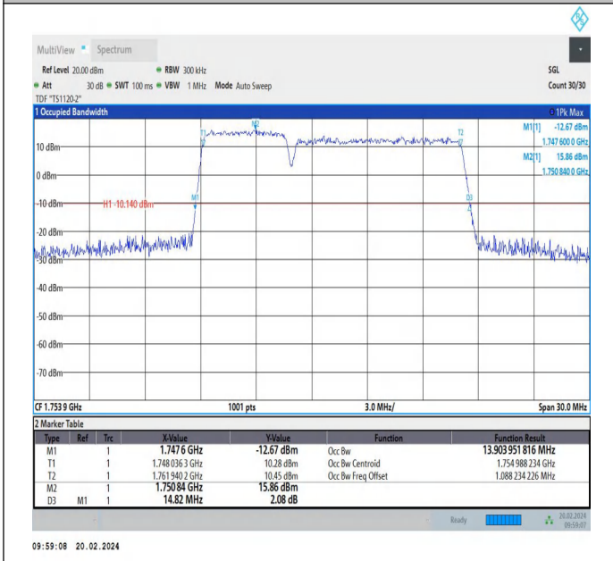
66-66-5MHz-10MHz-64QAM-64QAM-132375-132447-25RB#0-50RB#0-PASS
