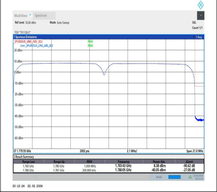
10MHz-10MHz_QPSK@QPSK-QPSK@QPSK_132523-13262 2_50RB#0@50RB#0-50RB#0@50RB#0
