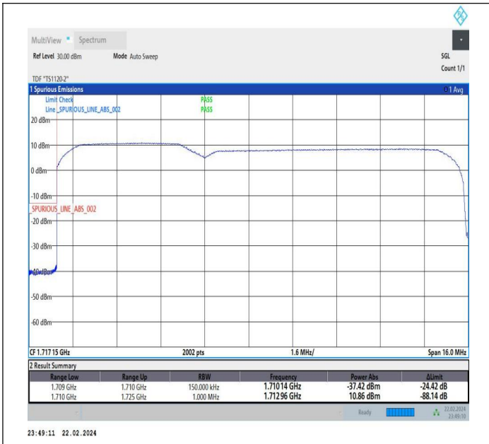
5MHz-10MHz_QPSK@QPSK-QPSK@QPSK_132000-132072_25RB#0@25RB#0-50RB#0@50RB#0
