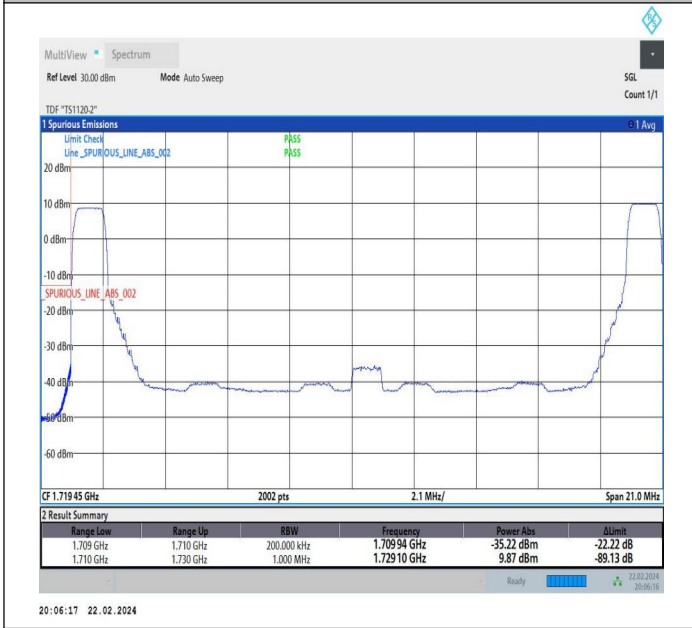
10MHz-10MHz_QPSK@QPSK-QPSK@QPSK_132022-13212 1_1RB#0@50RB#0-1RB#49@50RB#0
