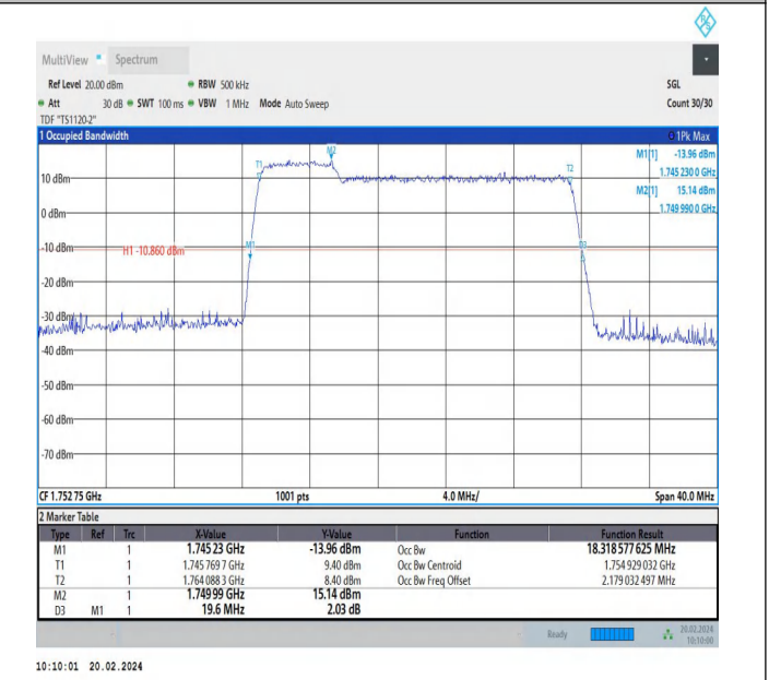
66-66-5MHz-15MHz-256QAM-256QAM-132353-132446-25RB#0-75RB#0-PASS
