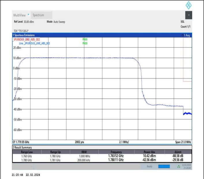
15MHz-5MHz_QPSK@QPSK-QPSK@QPSK_132549-132642_75RB#0@75RB#0-25RB#0@25RB#0
