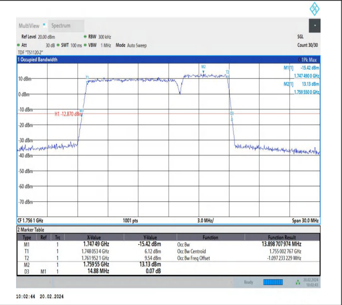
66-66-10MHz-5MHz-256QAM-256QAM-132397-132469-50RB#0-25RB#0-PASS
