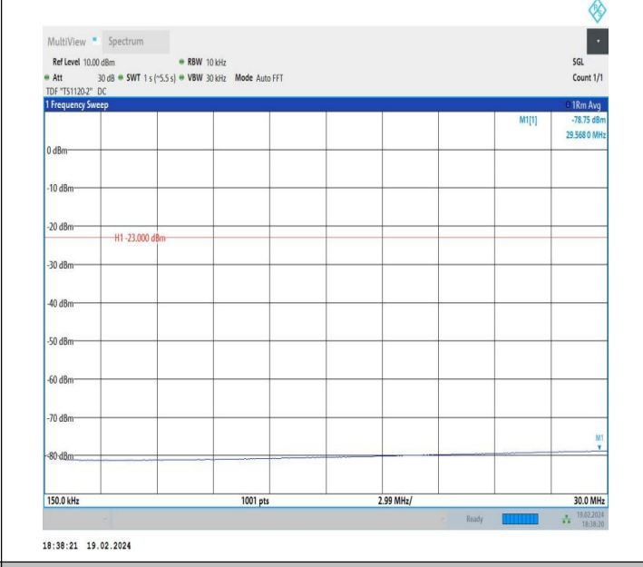
5-5-10MHz-5MHz-QPSK-QPSK-20550-20622-1RB#49-0RB#0-0 0.15~30MHz-PASS
