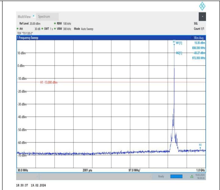
5-5-10MHz-5MHz-QPSK-QPSK-20500-20572-1RB#49-0RB#0- 30~1000MHz-PASS
