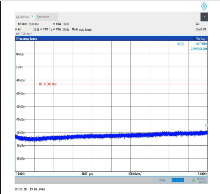
5-5-10MHz-10MHz-QPSK-QPSK-20501-20600-1RB#0-0RB#0-1000~3000MHz-PASS
