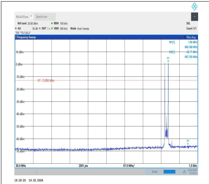
5-5-10MHz-10MHz-QPSK-QPSK-20450-20549-1RB#0-1RB#49 -30~1000MHz-PASS
