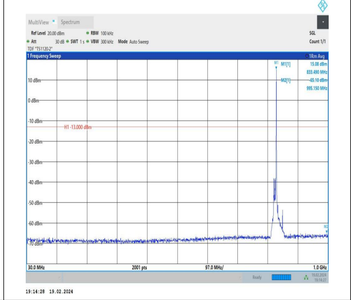
5-5-10MHz-10MHz-QPSK-QPSK-20450-20549-1RB#49-0RB#0-30~1000MHz-PASS
