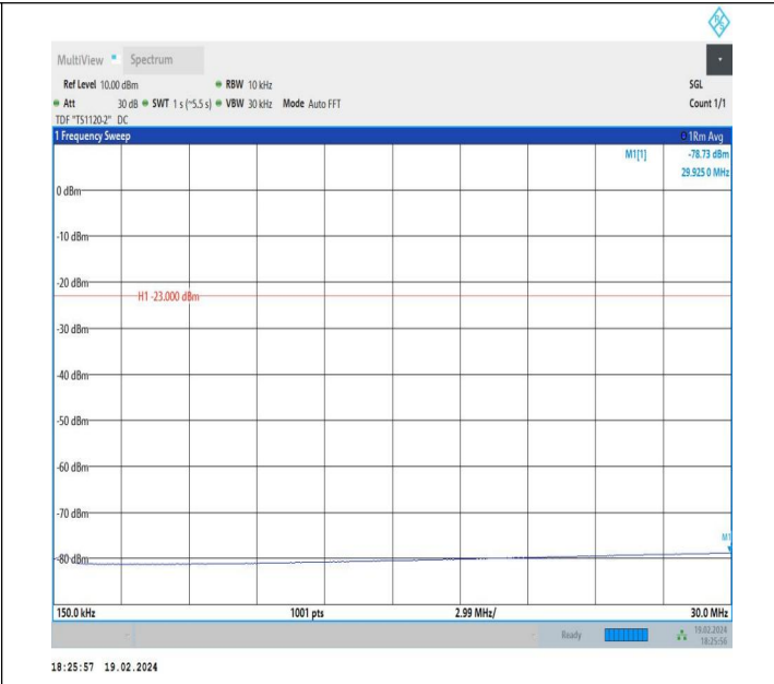
5-5-10MHz-5MHz-QPSK-QPSK-20450-20522-1RB#49-0RB#0-0.15~30MHz-PASS
