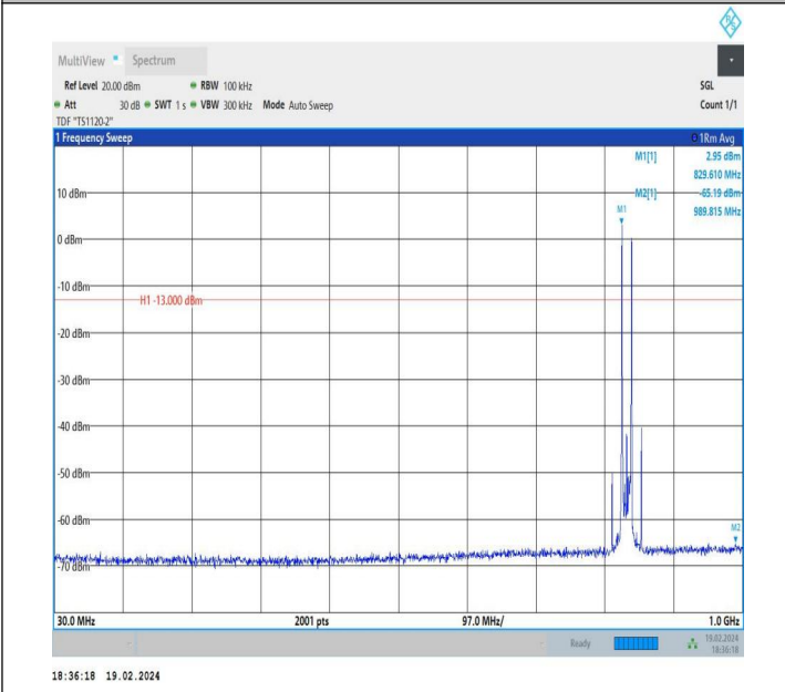
5-5-10MHz-5MHz-QPSK-QPSK-20500-20572-1RB#0-1RB#24-30~1000MHz-PASS
