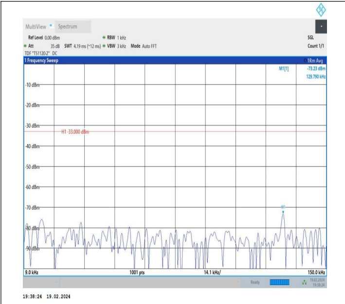
5-5-10MHz-10MHz-QPSK-QPSK-20501-20600-1RB#0-1RB#49 -0.009~0.15MHz-PASS
