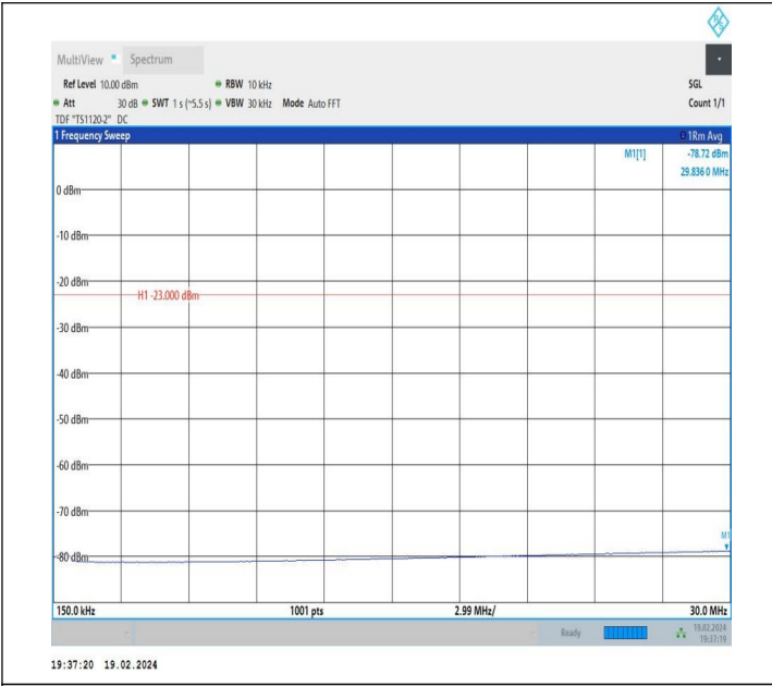
5-5-10MHz-10MHz-QPSK-QPSK-20501-20600-1RB#49-0RB#0 -0.15~30MHz-PASS
