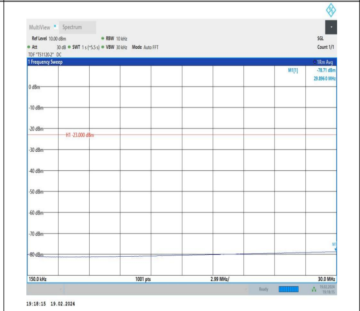
5-5-10MHz-10MHz-QPSK-QPSK-20450-20549-1RB#0-1RB#49 -0.15~30MHz-PASS
