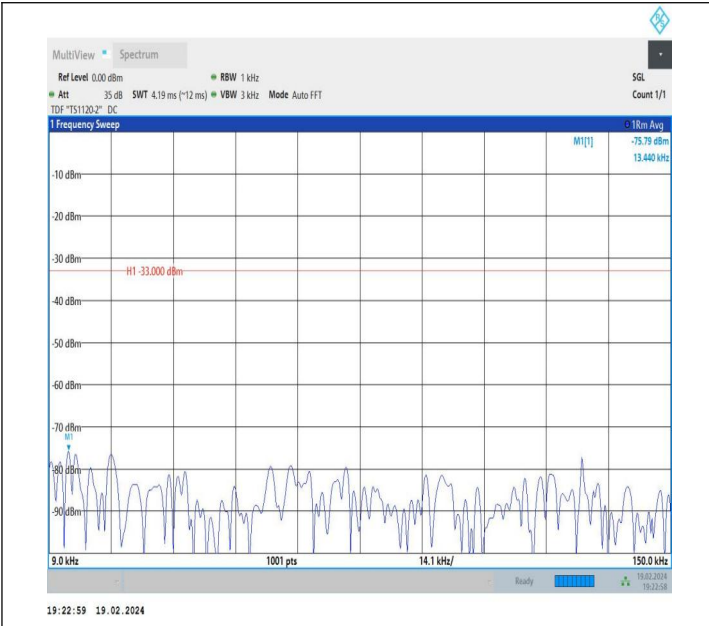
5-5-10MHz-10MHz-QPSK-QPSK-20476-20575-1RB#49-ORB#0 -0.009~0.15MHz-PASS
