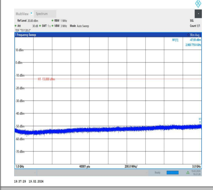
5-5-10MHz-10MHz-QPSK-QPSK-20501-20600-1RB#49-0RB#0 -1000~3000MHz-PASS
