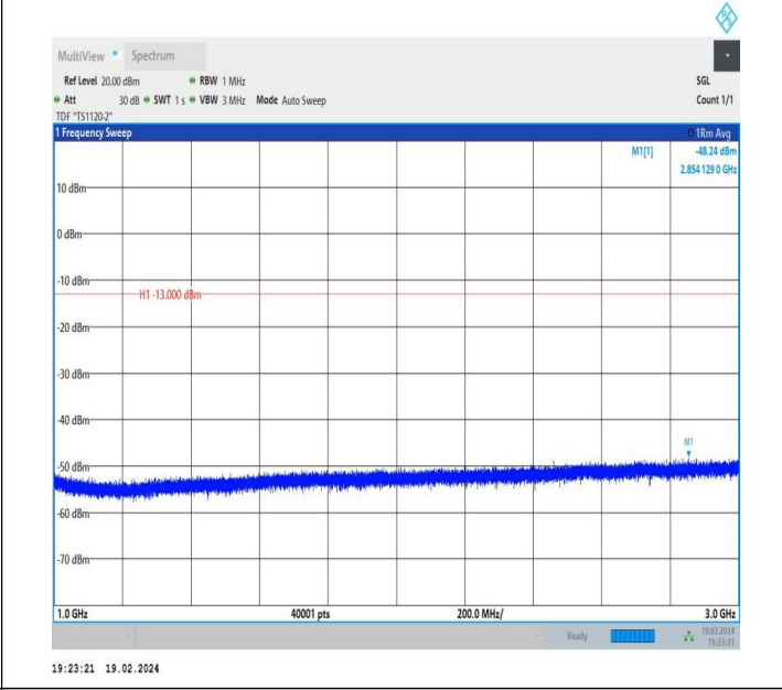
5-5-10MHz-10MHz-QPSK-QPSK-20476-20575-1RB#49-ORB#0 -1000~3000MHz-PASS
