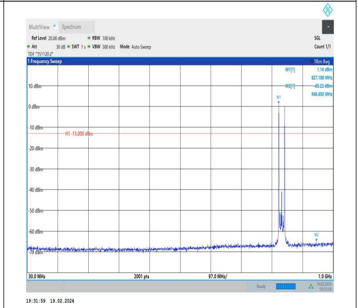
5-5-10MHz-10MHz-QPSK-QPSK-20476-20575-1RB#0-1RB#49 -30~1000MHz-PASS
