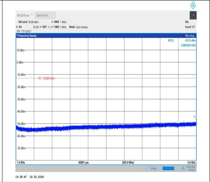
5-5-10MHz-10MHz-QPSK-QPSK-20501-20600-1RB#0-1RB#49 -1000~3000MHz-PASS
