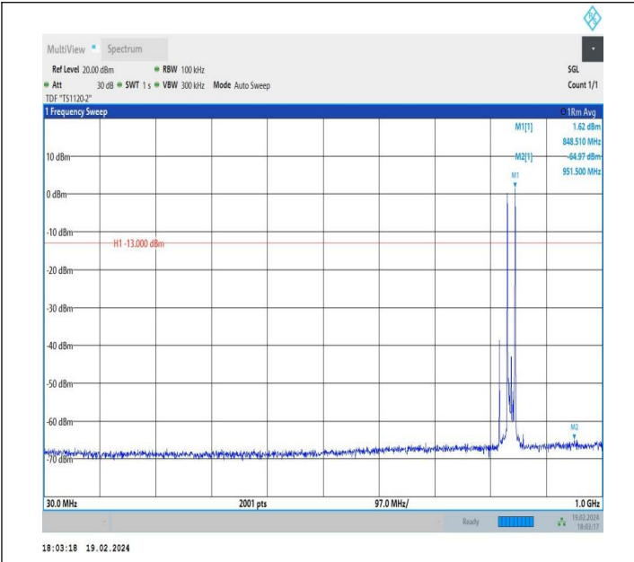
5-5-5MHz-10MHz-QPSK-QPSK-20528-20600-1RB#0-1RB#49-30~1000MHz-PASS
