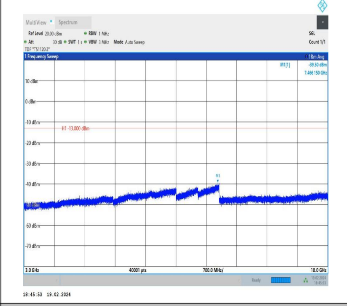
5-5-10MHz-5MHz-QPSK-QPSK-20550-20622-1RB#0-1RB#24- 3000~10000MHz-PASS
