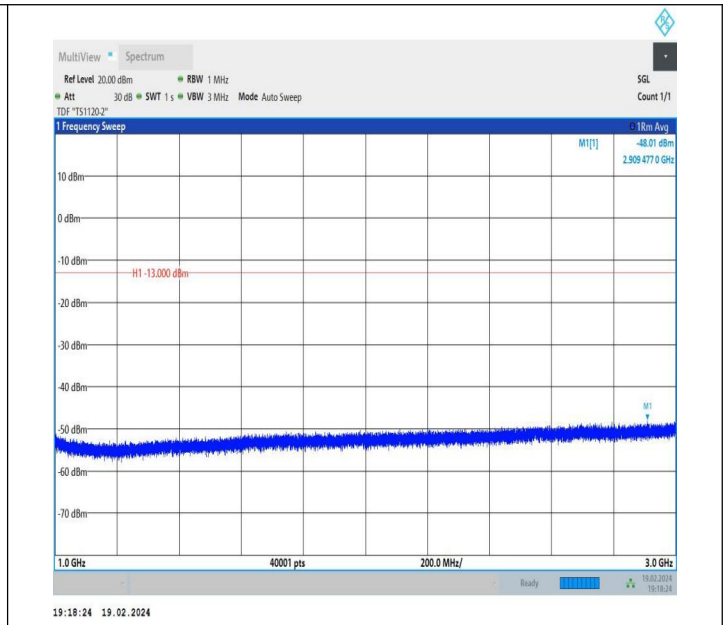
5-5-10MHz-10MHz-QPSK-QPSK-20450-20549-1RB#0-1RB#49 -1000~3000MHz-PASS
