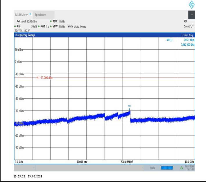
5-5-10MHz-10MHz-QPSK-QPSK-20501-20600-1RB#0-0RB#0-3000~10000MHz-PASS
