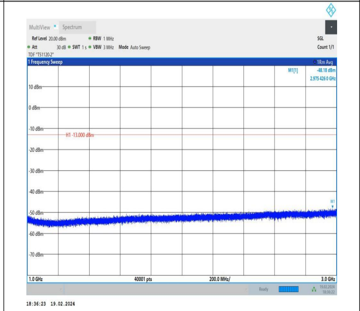
5-5-10MHz-5MHz-QPSK-QPSK-20500-20572-1RB#0-1RB#24-1000~3000MHz-PASS
