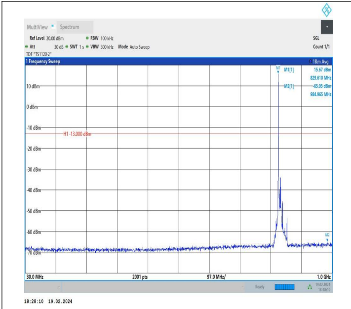
5-5-10MHz-5MHz-QPSK-QPSK-20500-20572-1RB#0-0RB#0-3 0~1000MHz-PASS
