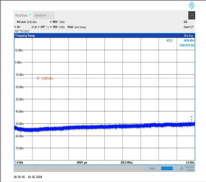
5-5-10MHz-5MHz-QPSK-QPSK-20500-20572-1RB#49-0RB#0- 1000~3000MHz-PASS
