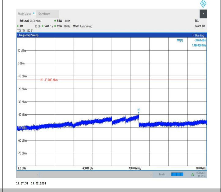
5-5-10MHz-10MHz-QPSK-QPSK-20501-20600-1RB#49-0RB#0 -3000~10000MHz-PASS
