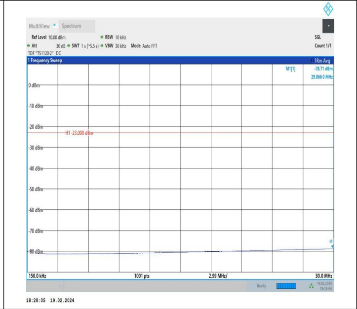
5-5-10MHz-5MHz-QPSK-QPSK-20500-20572-1RB#0-0RB#0-0. 15~30MHz-PASS
