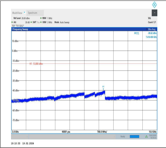
5-5-10MHz-10MHz-QPSK-QPSK-20450-20549-1RB#0-0RB#0-3000~10000MHz-PASS
