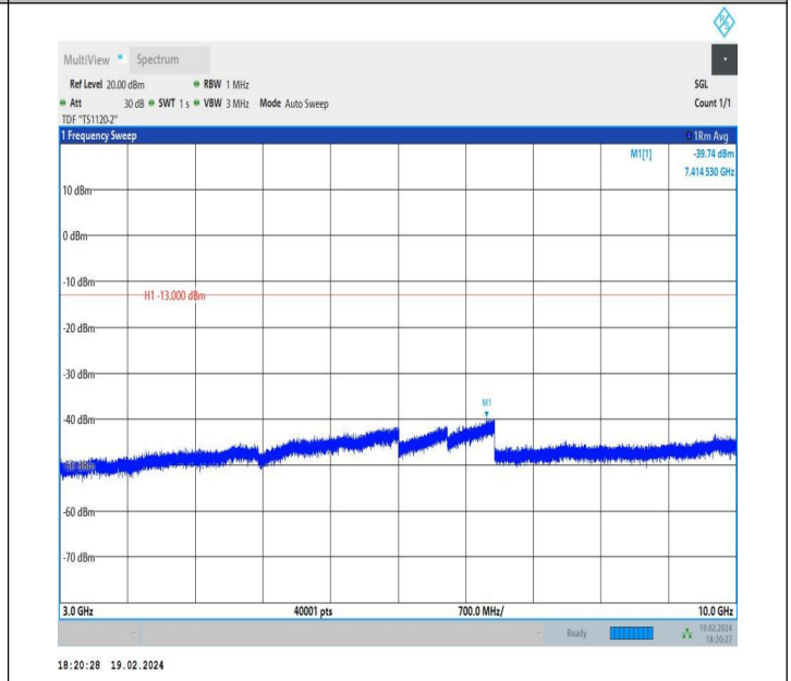
5-5-10MHz-5MHz-QPSK-QPSK-20450-20522-1RB#0-0RB#0-3 000~10000MHz-PASS
