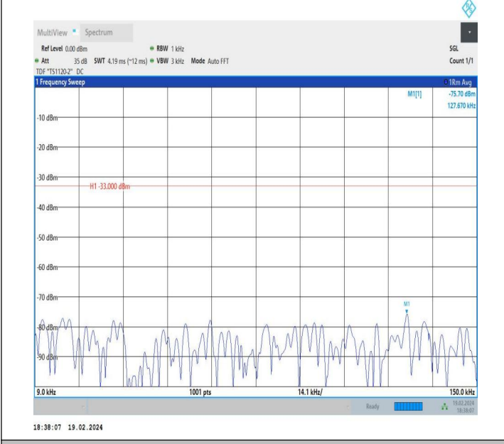
5-5-10MHz-5MHz-QPSK-QPSK-20550-20622-1RB#49-0RB#0-0 0.009~0.15MHz-PASS
