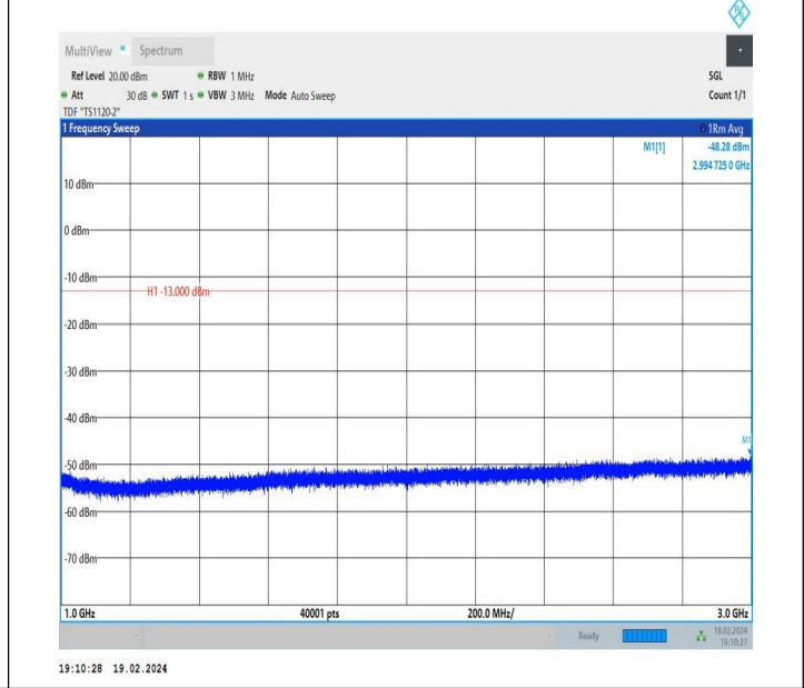
5-5-10MHz-10MHz-QPSK-QPSK-20450-20549-1RB#0-0RB#0-1000~3000MHz-PASS
