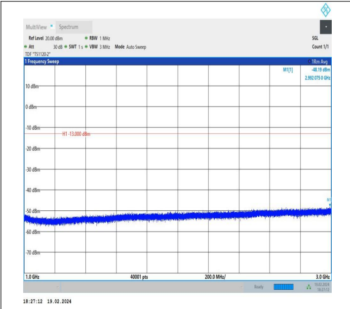
5-5-10MHz-5MHz-QPSK-QPSK-20450-20522-1RB#0-1RB#24- 1000~3000MHz-PASS
