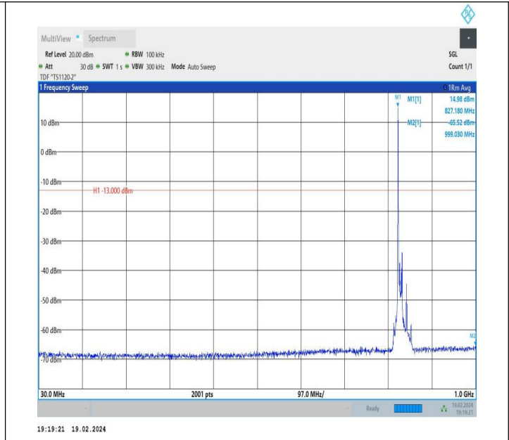
5-5-10MHz-10MHz-QPSK-QPSK-20476-20575-1RB#0-0RB#0-30~1000MHz-PASS
