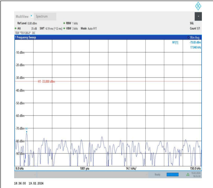
5-5-10MHz-5MHz-QPSK-QPSK-20500-20572-1RB#0-1RB#24-0.009~0.15MHz-PASS
