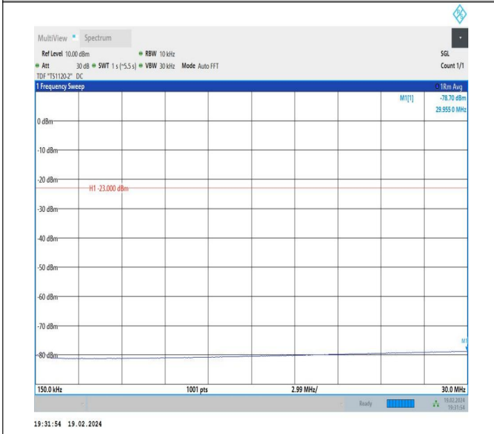
5-5-10MHz-10MHz-QPSK-QPSK-20476-20575-1RB#0-1RB#49 -0.15~30MHz-PASS
