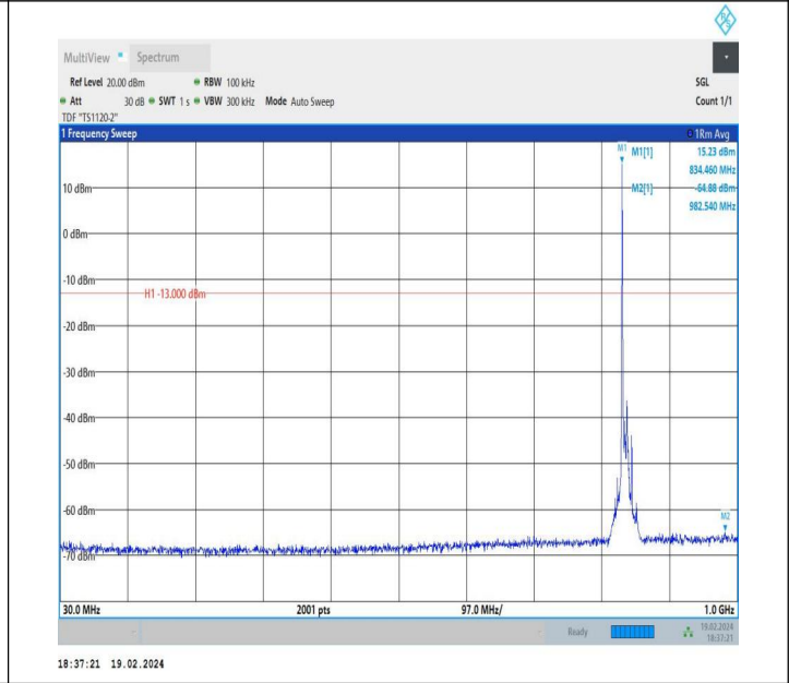
5-5-10MHz-5MHz-QPSK-QPSK-20550-20622-1RB#0-0RB#0-30~1000MHz-PASS
