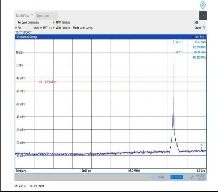
5-5-10MHz-10MHz-QPSK-QPSK-20476-20575-1RB#49-ORB#0 -30~1000MHz-PASS
