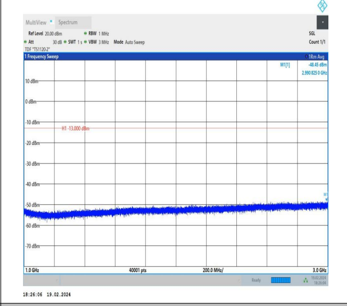
5-5-10MHz-5MHz-QPSK-QPSK-20450-20522-1RB#49-0RB#0-1000~3000MHz-PASS
