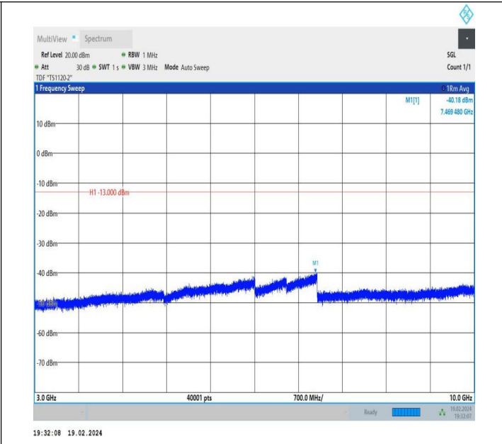
5-5-10MHz-10MHz-QPSK-QPSK-20476-20575-1RB#0-1RB#49 -3000~10000MHz-PASS
