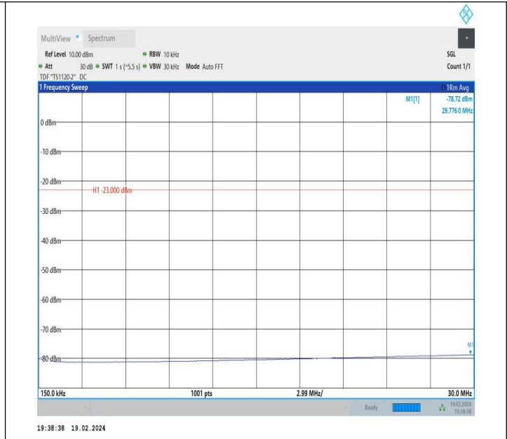
5-5-10MHz-10MHz-QPSK-QPSK-20501-20600-1RB#0-1RB#49 -0.15~30MHz-PASS
