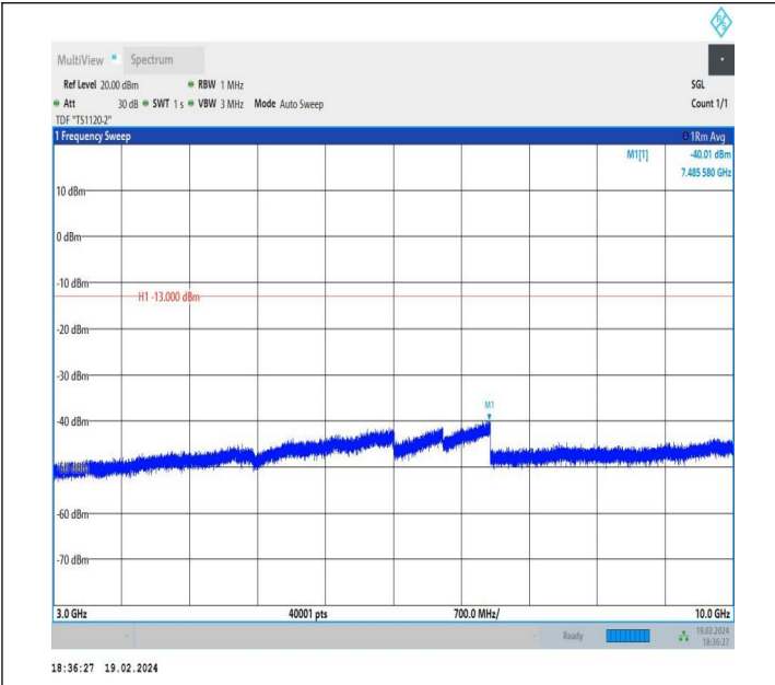
5-5-10MHz-5MHz-QPSK-QPSK-20500-20572-1RB#0-1RB#24-3000~10000MHz-PASS
