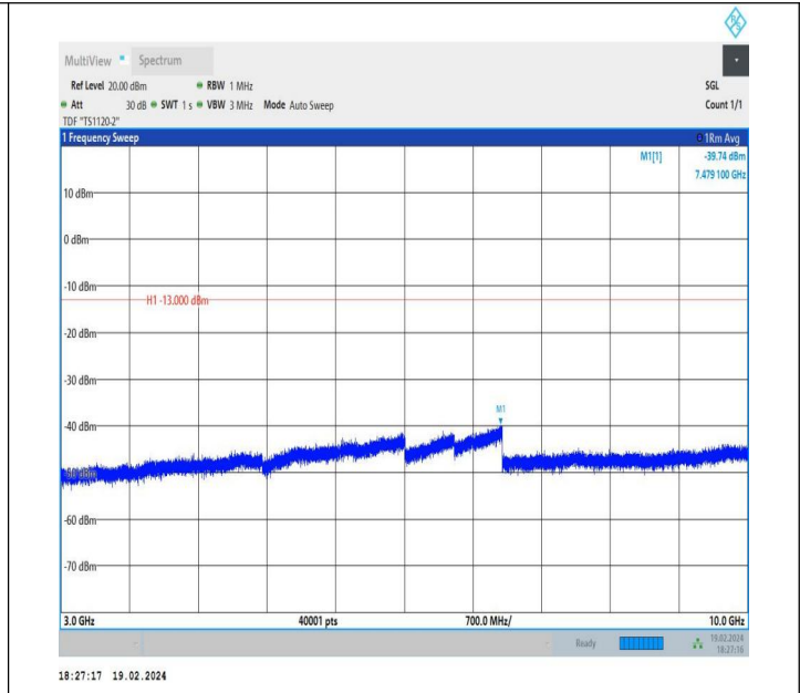
5-5-10MHz-5MHz-QPSK-QPSK-20450-20522-1RB#0-1RB#24- 3000~10000MHz-PASS
