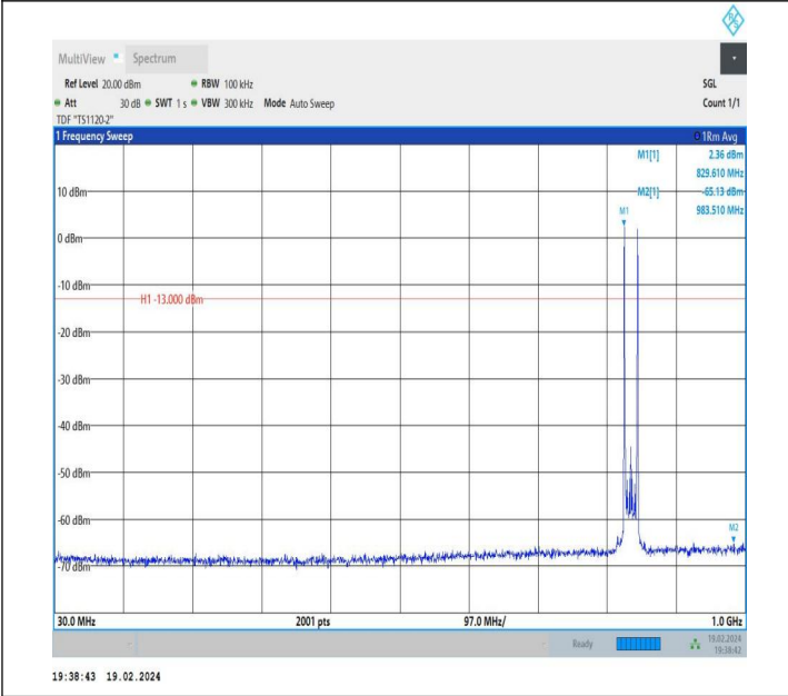
5-5-10MHz-10MHz-QPSK-QPSK-20501-20600-1RB#0-1RB#49 -30~1000MHz-PASS
