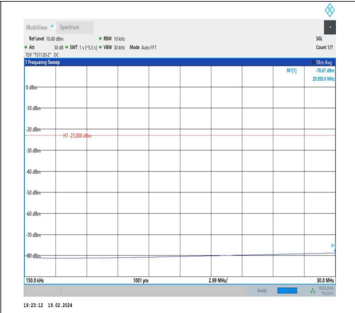
5-5-10MHz-10MHz-QPSK-QPSK-20476-20575-1RB#49-ORB#0 -0.15~30MHz-PASS
