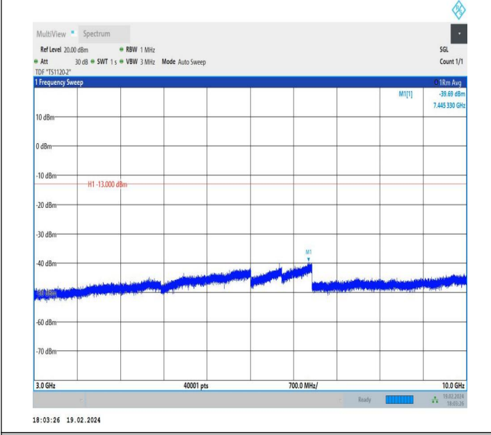
5-5-5MHz-10MHz-QPSK-QPSK-20528-20600-1RB#0-1RB#49-3000~10000MHz-PASS
