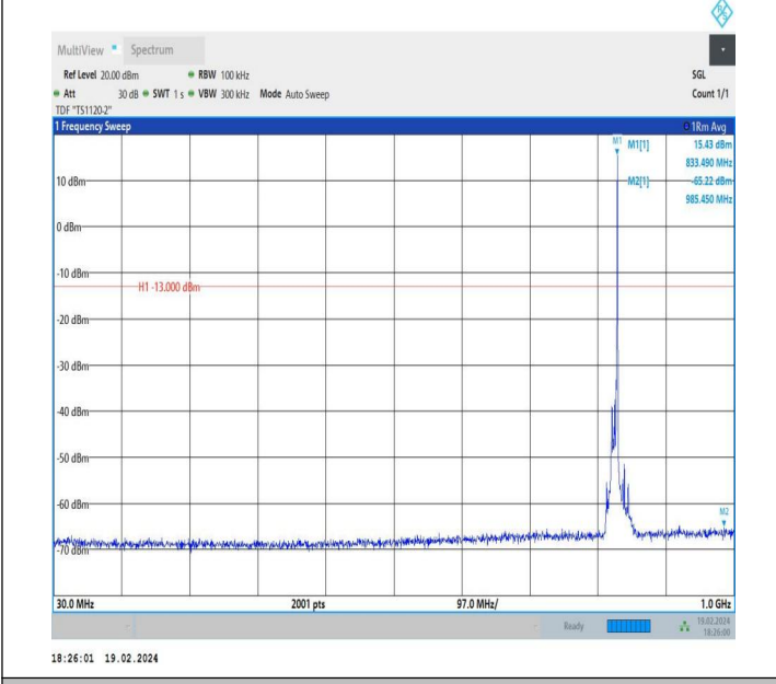
5-5-10MHz-5MHz-QPSK-QPSK-20450-20522-1RB#49-0RB#0-30~1000MHz-PASS
