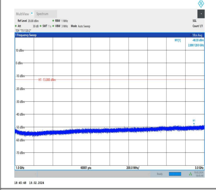
5-5-10MHz-5MHz-QPSK-QPSK-20550-20622-1RB#0-1RB#24- 1000~3000MHz-PASS
