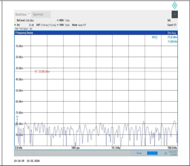
5-5-10MHz-10MHz-QPSK-QPSK-20450-20549-1RB#49-0RB#0-0.009~0.15MHz-PASS
