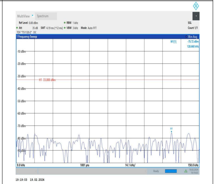
5-5-10MHz-10MHz-QPSK-QPSK-20476-20575-1RB#0-0RB#0- 0.009~0.15MHz-PASS
