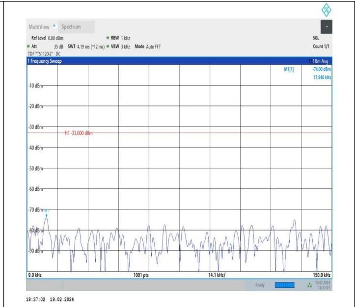
5-5-10MHz-5MHz-QPSK-QPSK-20550-20622-1RB#0-0RB#0-0.009~0.15MHz-PASS
