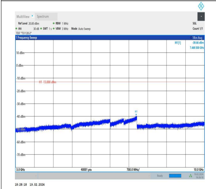
5-5-10MHz-5MHz-QPSK-QPSK-20500-20572-1RB#0-0RB#0-3 000~10000MHz-PASS
