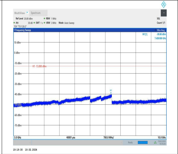
5-5-10MHz-10MHz-QPSK-QPSK-20476-20575-1RB#0-0RB#0-3000~10000MHz-PASS
