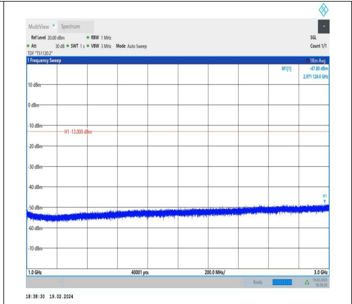
5-5-10MHz-5MHz-QPSK-QPSK-20550-20622-1RB#49-0RB#0-1000~3000MHz-PASS
