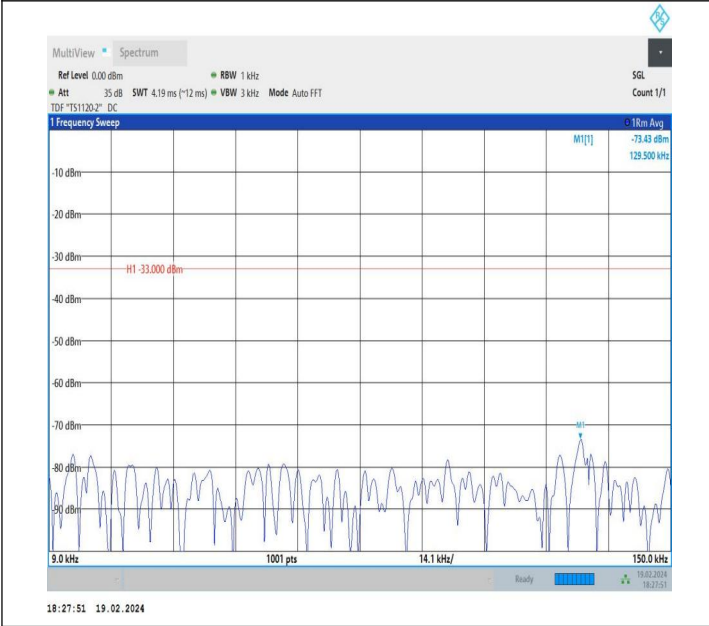
5-5-10MHz-5MHz-QPSK-QPSK-20500-20572-1RB#0-0RB#0-0. 009~0.15MHz-PASS
