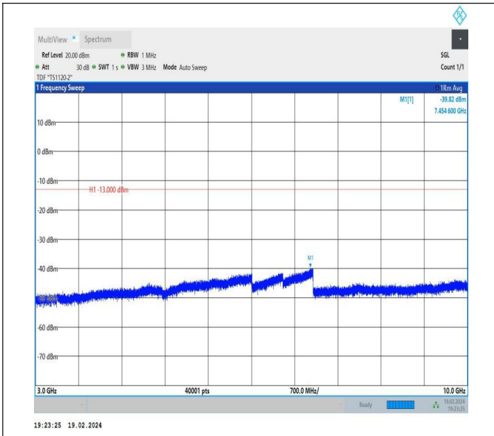
5-5-10MHz-10MHz-QPSK-QPSK-20476-20575-1RB#49-0RB#0 -3000~10000MHz-PASS
