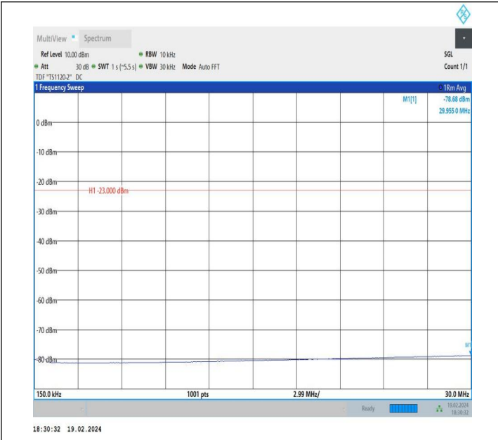
5-5-10MHz-5MHz-QPSK-QPSK-20500-20572-1RB#49-0RB#0- 0.15~30MHz-PASS
