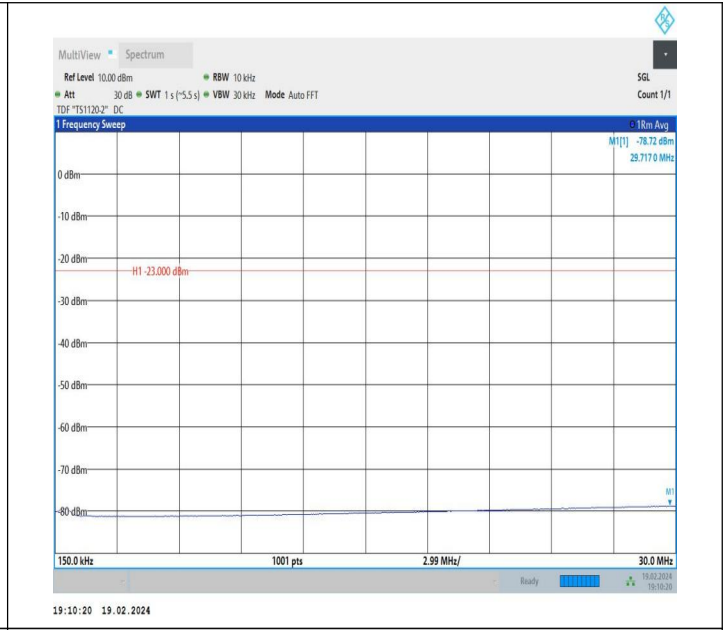
5-5-10MHz-10MHz-QPSK-QPSK-20450-20549-1RB#0-0RB#0-0.15~30MHz-PASS
