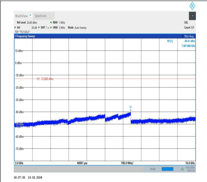
5-5-10MHz-5MHz-QPSK-QPSK-20550-20622-1RB#0-0RB#0-3 000~10000MHz-PASS
