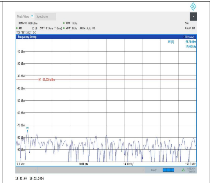
5-5-10MHz-10MHz-QPSK-QPSK-20476-20575-1RB#0-1RB#49 -0.009~0.15MHz-PASS
