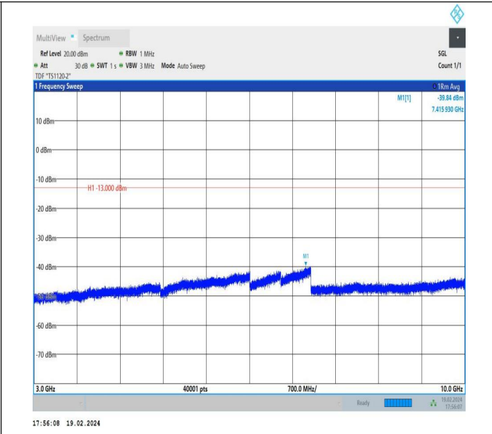
5-5-5MHz-10MHz-QPSK-QPSK-20528-20600-1RB#24-0RB#0-3000~10000MHz-PASS
