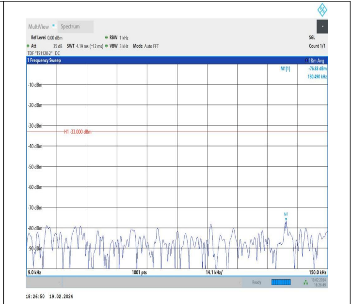
5-5-10MHz-5MHz-QPSK-QPSK-20450-20522-1RB#0-1RB#24-0.009~0.15MHz-PASS
