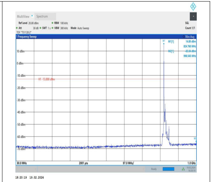
5-5-10MHz-5MHz-QPSK-QPSK-20450-20522-1RB#0-0RB#0-3 0~1000MHz-PASS
