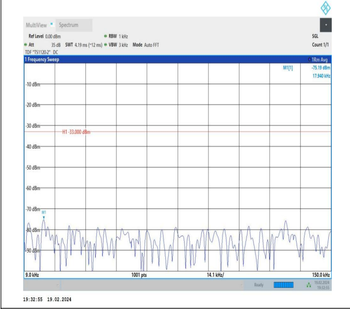
5-5-10MHz-10MHz-QPSK-QPSK-20501-20600-1RB#0-0RB#0- 0.009~0.15MHz-PASS
