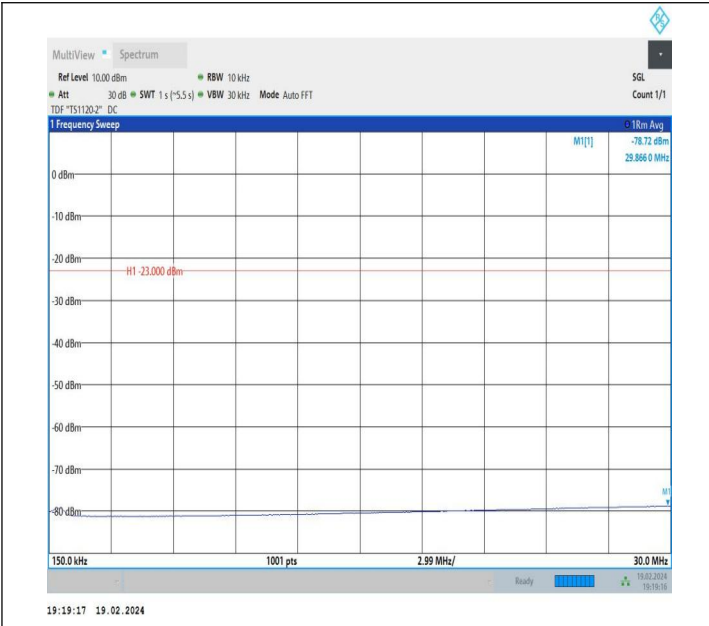
5-5-10MHz-10MHz-QPSK-QPSK-20476-20575-1RB#0-0RB#0-0.15~30MHz-PASS
