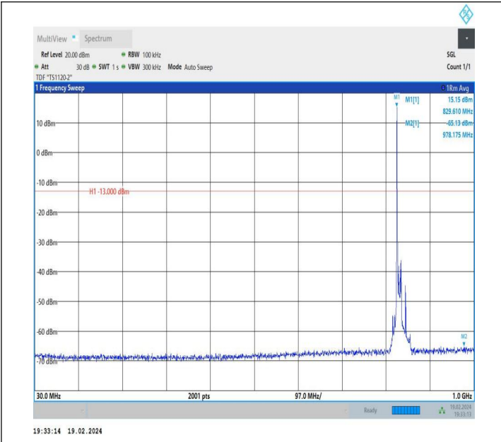
5-5-10MHz-10MHz-QPSK-QPSK-20501-20600-1RB#0-0RB#0-30~1000MHz-PASS
