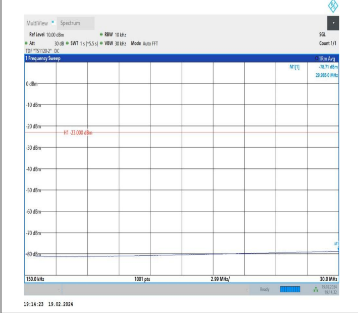
5-5-10MHz-10MHz-QPSK-QPSK-20450-20549-1RB#49-0RB#0-0.15~30MHz-PASS
