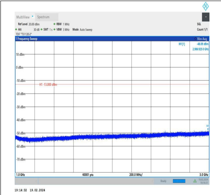
5-5-10MHz-10MHz-QPSK-QPSK-20450-20549-1RB#49-0RB#0 -1000~3000MHz-PASS
