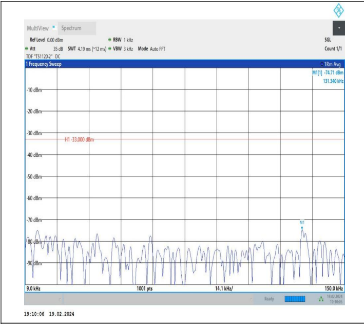
5-5-10MHz-10MHz-QPSK-QPSK-20450-20549-1RB#0-0RB#0-0.009~0.15MHz-PASS
