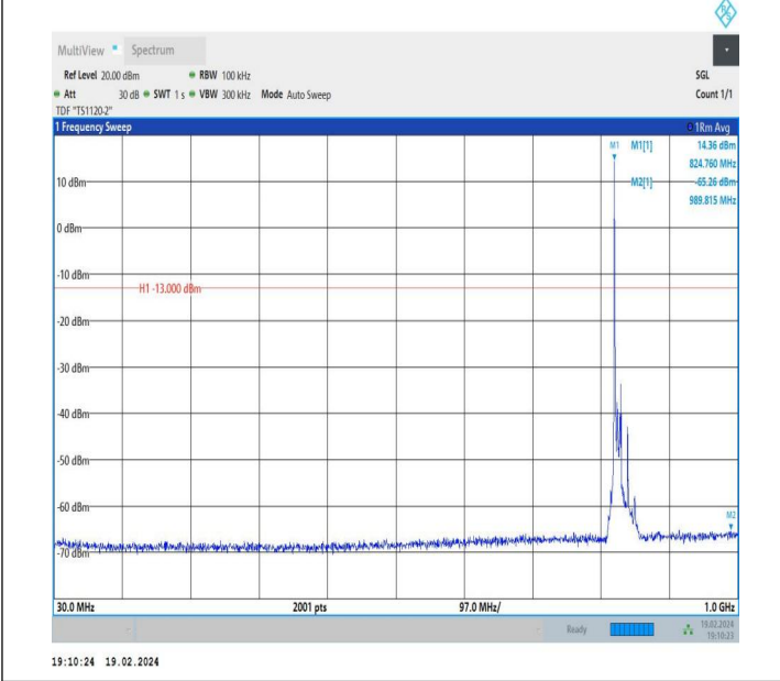
5-5-10MHz-10MHz-QPSK-QPSK-20450-20549-1RB#0-0RB#0-30~1000MHz-PASS
