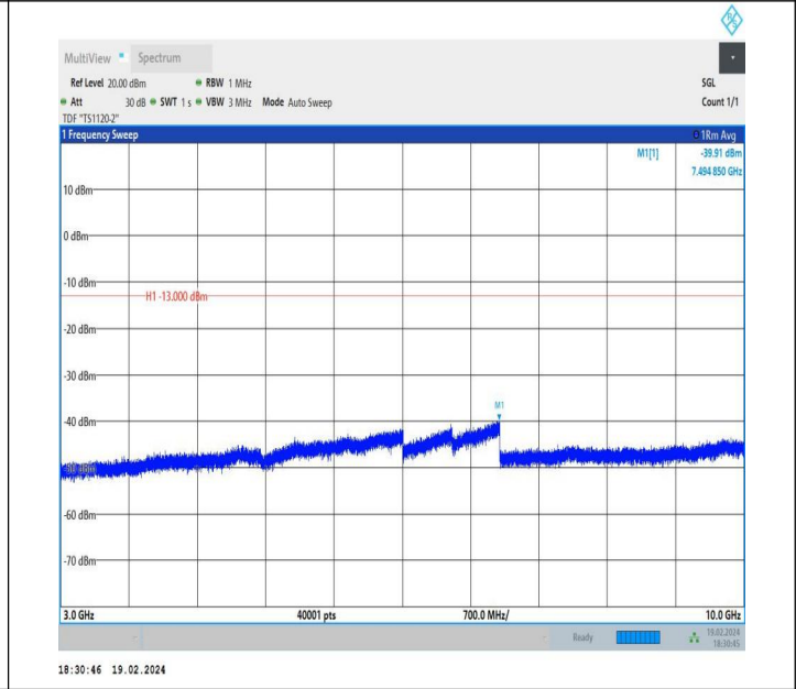
5-5-10MHz-5MHz-QPSK-QPSK-20500-20572-1RB#49-0RB#0- 3000~10000MHz-PASS
