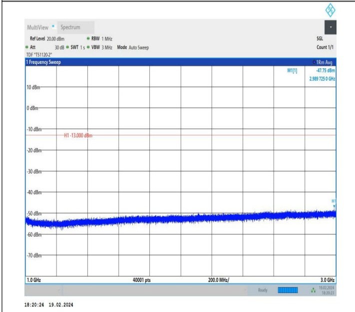
5-5-10MHz-5MHz-QPSK-QPSK-20450-20522-1RB#0-0RB#0-1 000~3000MHz-PASS
