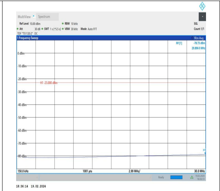
5-5-10MHz-5MHz-QPSK-QPSK-20500-20572-1RB#0-1RB#24-0.15~30MHz-PASS
