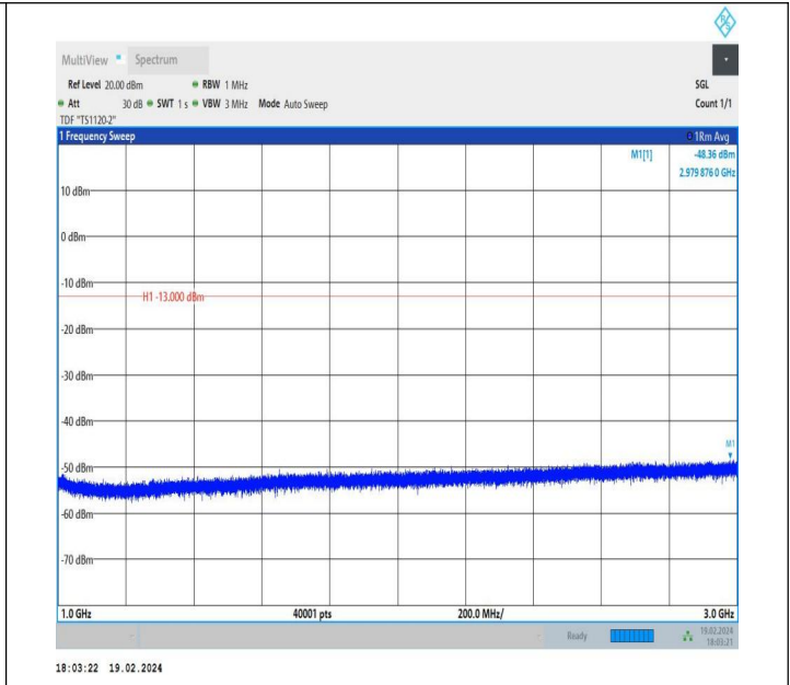
5-5-5MHz-10MHz-QPSK-QPSK-20528-20600-1RB#0-1RB#49-1000~3000MHz-PASS
