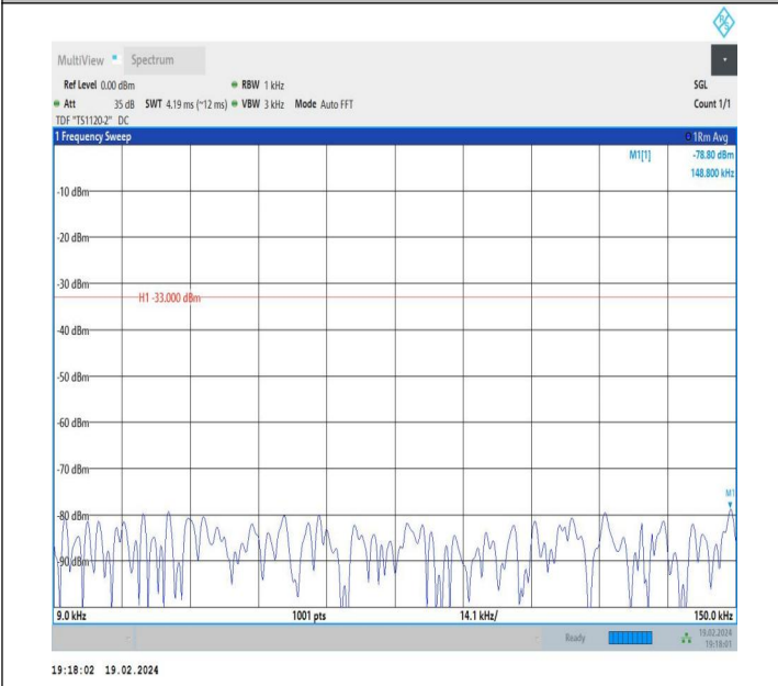
5-5-10MHz-10MHz-QPSK-QPSK-20450-20549-1RB#0-1RB#49 -0.009~0.15MHz-PASS
