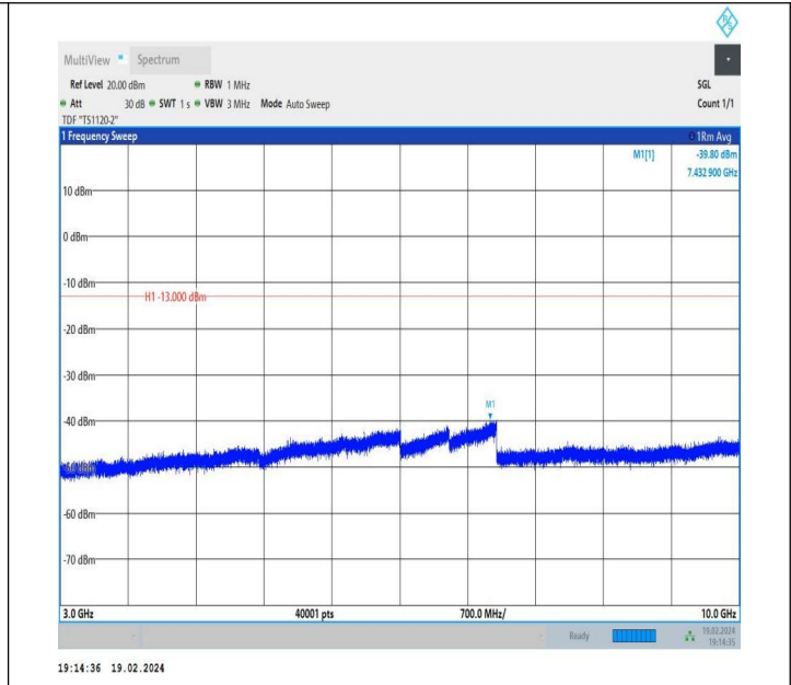
5-5-10MHz-10MHz-QPSK-QPSK-20450-20549-1RB#49-0RB#0 -3000~10000MHz-PASS
