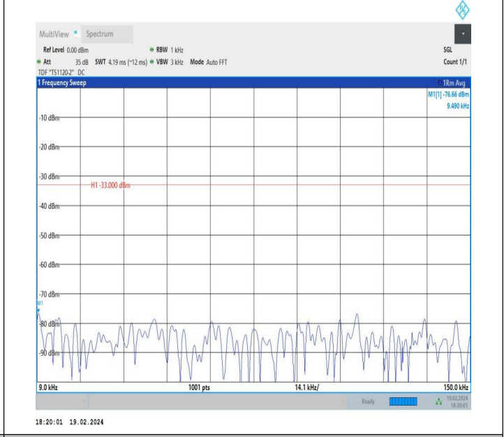
5-5-10MHz-5MHz-QPSK-QPSK-20450-20522-1RB#0-0RB#0-0.009~0.15MHz-PASS
