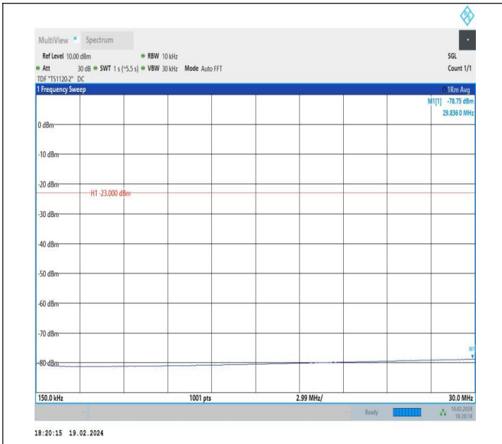
5-5-10MHz-5MHz-QPSK-QPSK-20450-20522-1RB#0-0RB#0-0. 15~30MHz-PASS
