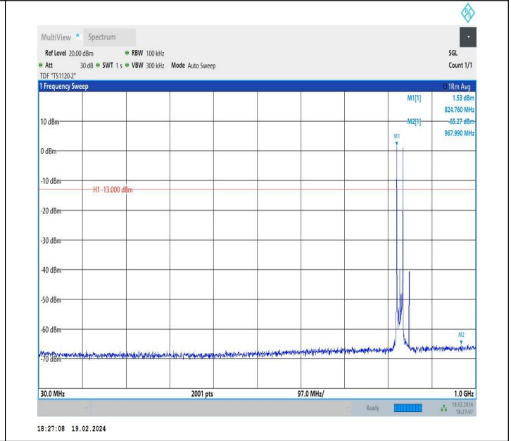
5-5-10MHz-5MHz-QPSK-QPSK-20450-20522-1RB#0-1RB#24-30~1000MHz-PASS
