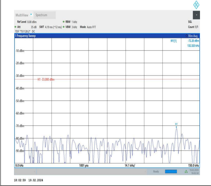
5-5-5MHz-10MHz-QPSK-QPSK-20528-20600-1RB#0-1RB#49-0.009~0.15MHz-PASS
