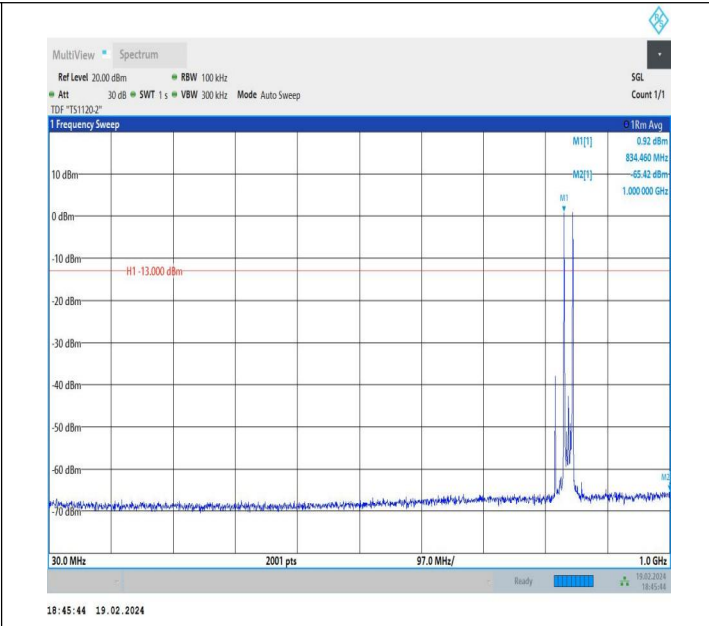
5-5-10MHz-5MHz-QPSK-QPSK-20550-20622-1RB#0-1RB#24- 30~1000MHz-PASS
