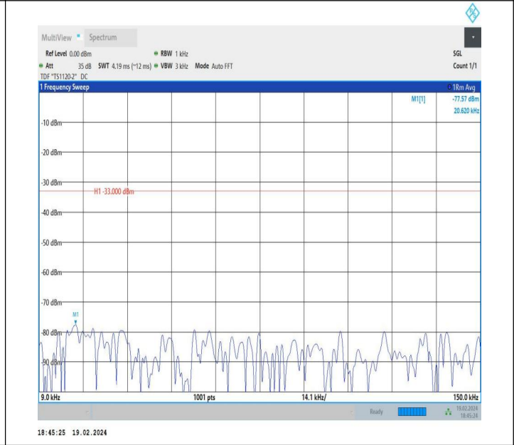
5-5-10MHz-5MHz-QPSK-QPSK-20550-20622-1RB#0-1RB#24-0.009~0.15MHz-PASS
