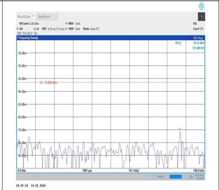
5-5-10MHz-5MHz-QPSK-QPSK-20500-20572-1RB#49-0RB#0-0 0.009~0.15MHz-PASS
