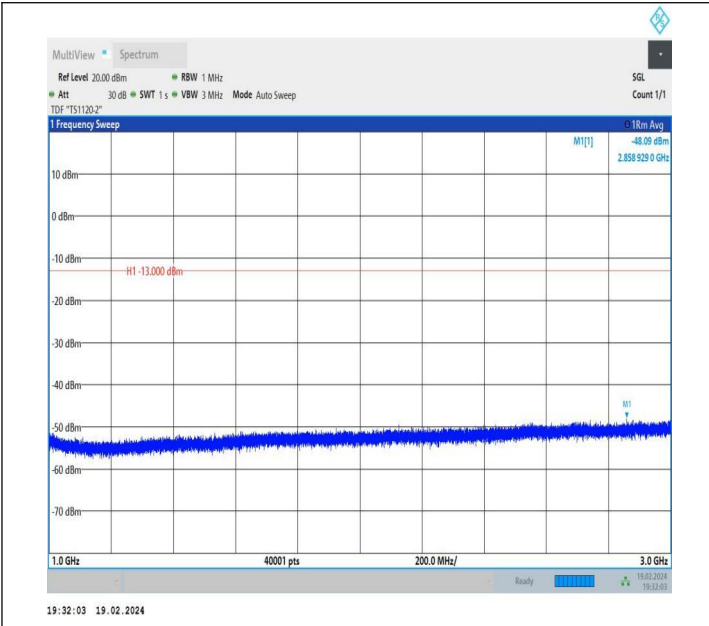
5-5-10MHz-10MHz-QPSK-QPSK-20476-20575-1RB#0-1RB#49 -1000~3000MHz-PASS
