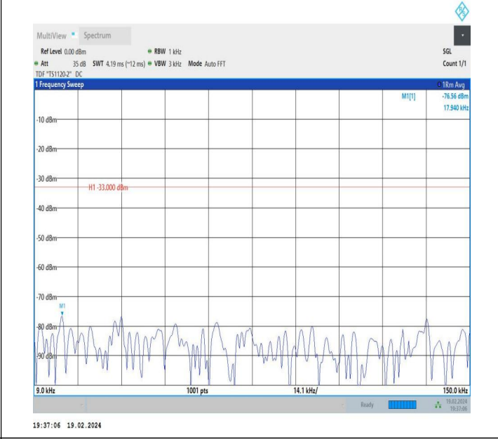
5-5-10MHz-10MHz-QPSK-QPSK-20501-20600-1RB#49-0RB#0-0.009~0.15MHz-PASS
