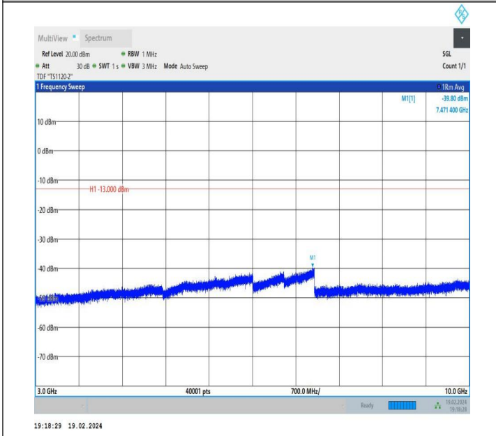
5-5-10MHz-10MHz-QPSK-QPSK-20450-20549-1RB#0-1RB#49 -3000~10000MHz-PASS
