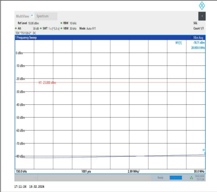
5-5-5MHz-3MHz-QPSK-QPSK-20425-20464-1RB#0-0RB#0-0.1 5~30MHz-PASS
