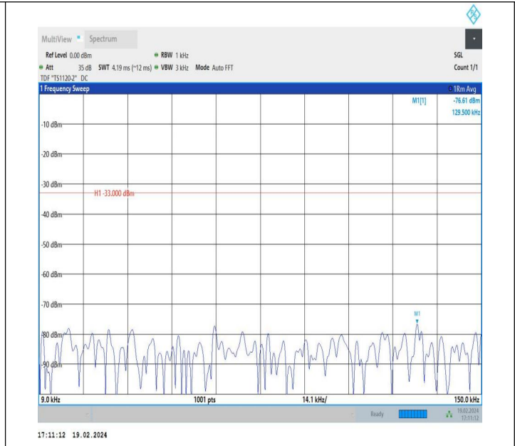
5-5-5MHz-3MHz-QPSK-QPSK-20425-20464-1RB#0-0RB#0-0.0 09~0.15MHz-PASS
