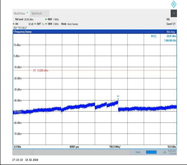
5-5-5MHz-3MHz-QPSK-QPSK-20425-20464-1RB#0-1RB#15-3 000~10000MHz-PASS
