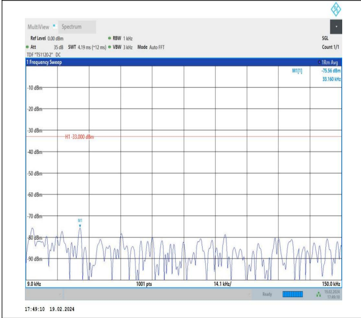
5-5-5MHz-10MHz-QPSK-QPSK-20478-20550-1RB#24-0RB#0-0 0.009~0.15MHz-PASS
