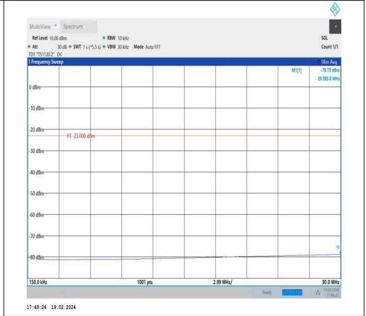
5-5-5MHz-10MHz-QPSK-QPSK-20478-20550-1RB#24-0RB#0-0 0.15~30MHz-PASS
