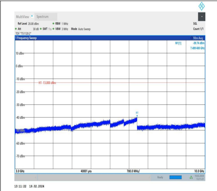
5-5-3MHz-5MHz-QPSK-QPSK-20501-20540-1RB#0-1RB#24-3 000~10000MHz-PASS
