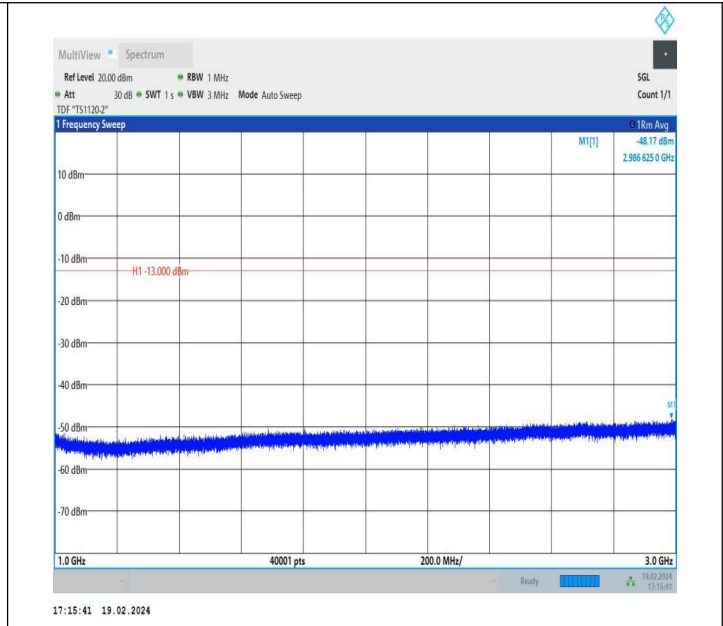
5-5-5MHz-3MHz-QPSK-QPSK-20510-20549-1RB#0-1RB#15-1 000~3000MHz-PASS
