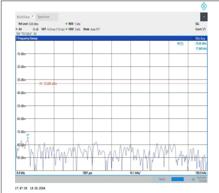
5-5-5MHz-10MHz-QPSK-QPSK-20428-20500-1RB#0-1RB#49- 0.009~0.15MHz-PASS
