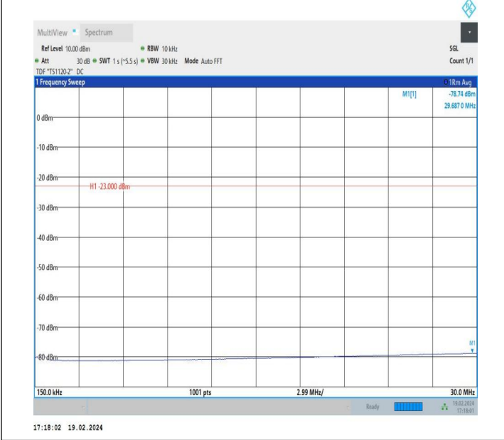
5-5-5MHz-3MHz-QPSK-QPSK-20595-20634-1RB#0-1RB#15-0. 15~30MHz-PASS
