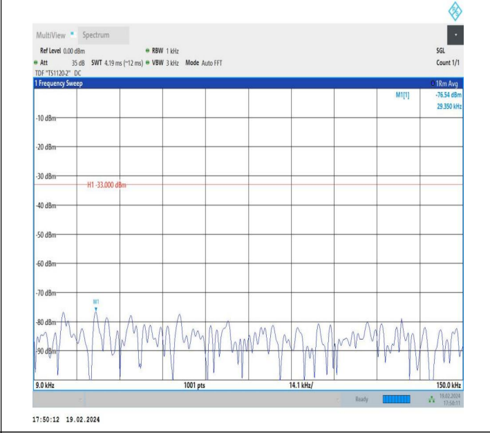
5-5-5MHz-10MHz-QPSK-QPSK-20478-20550-1RB#0-1RB#49-0.009~0.15MHz-PASS
