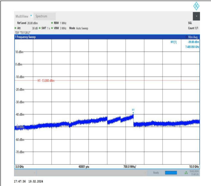
5-5-5MHz-10MHz-QPSK-QPSK-20428-20500-1RB#0-1RB#49-3000~10000MHz-PASS
