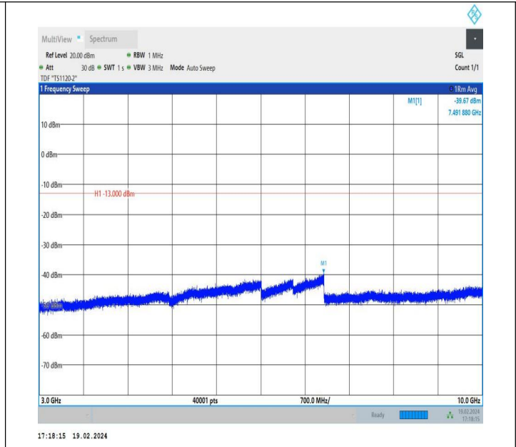
5-5-5MHz-3MHz-QPSK-QPSK-20595-20634-1RB#0-1RB#15-3 000~10000MHz-PASS
