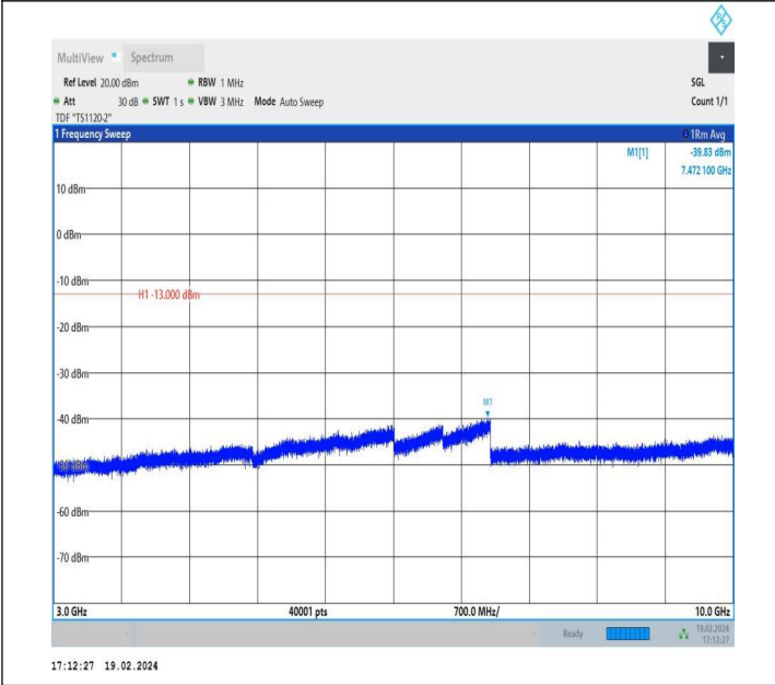
5-5-5MHz-3MHz-QPSK-QPSK-20425-20464-1RB#24-0RB#0-3 000~10000MHz-PASS
