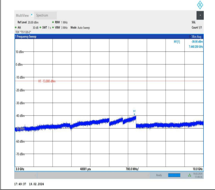
5-5-5MHz-10MHz-QPSK-QPSK-20478-20550-1RB#24-0RB#0-3000~10000MHz-PASS
