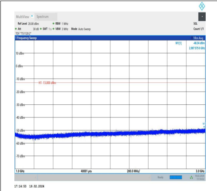
5-5-5MHz-3MHz-QPSK-QPSK-20510-20549-1RB#24-0RB#0-1 000~3000MHz-PASS
