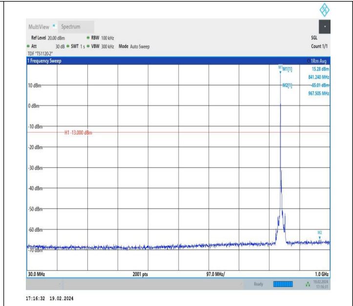
5-5-5MHz-3MHz-QPSK-QPSK-20595-20634-1RB#0-0RB#0-30 ~1000MHz-PASS
