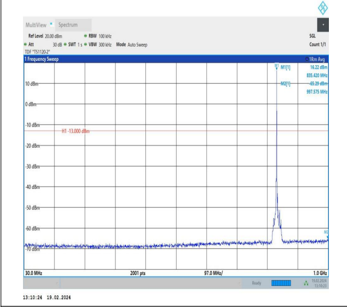
5-5-3MHz-5MHz-QPSK-QPSK-20501-20540-1RB#14-0RB#0-3 0~1000MHz-PASS
