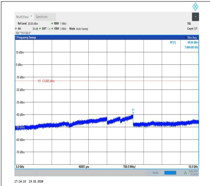
5-5-5MHz-3MHz-QPSK-QPSK-20510-20549-1RB#0-0RB#0-30 00~10000MHz-PASS
