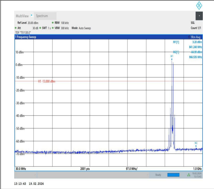
5-5-3MHz-5MHz-QPSK-QPSK-20586-20625-1RB#0-1RB#24-3 0~1000MHz-PASS
