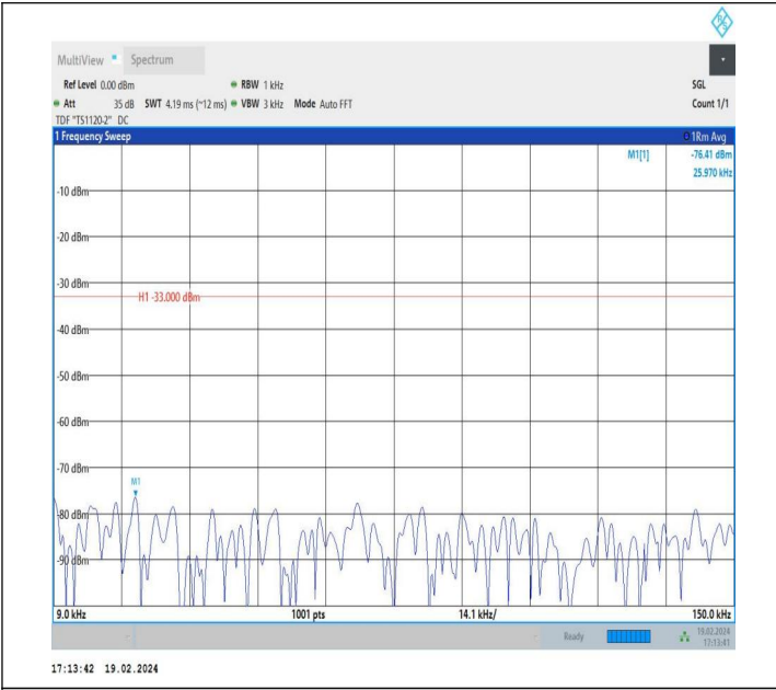
5-5-5MHz-3MHz-QPSK-QPSK-20510-20549-1RB#0-0RB#0-0.0 09~0.15MHz-PASS
