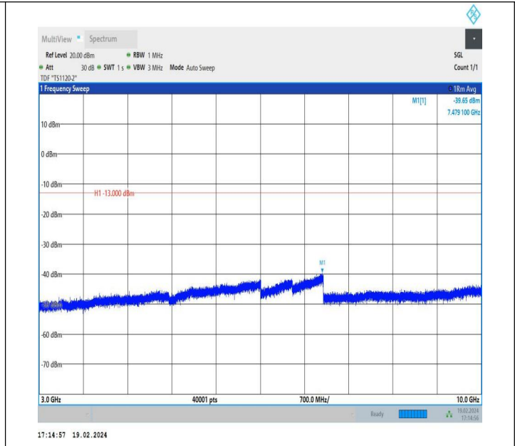
5-5-5MHz-3MHz-QPSK-QPSK-20510-20549-1RB#24-0RB#0-3 000~10000MHz-PASS
