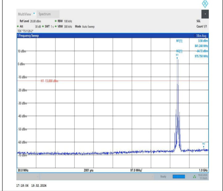
5-5-5MHz-3MHz-QPSK-QPSK-20595-20634-1RB#0-1RB#15-3 0~1000MHz-PASS
