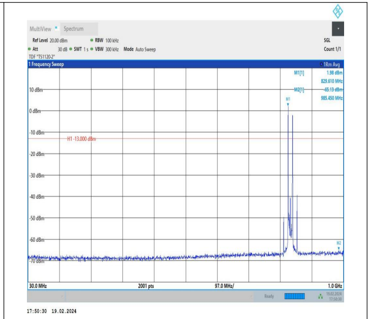
5-5-5MHz-10MHz-QPSK-QPSK-20478-20550-1RB#0-1RB#49- 30~1000MHz-PASS
