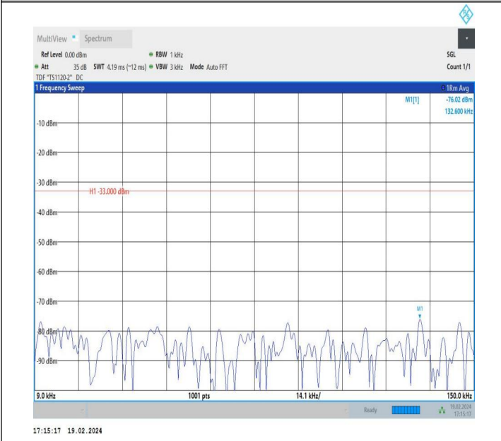
5-5-5MHz-3MHz-QPSK-QPSK-20510-20549-1RB#0-1RB#15-0. 009~0.15MHz-PASS
