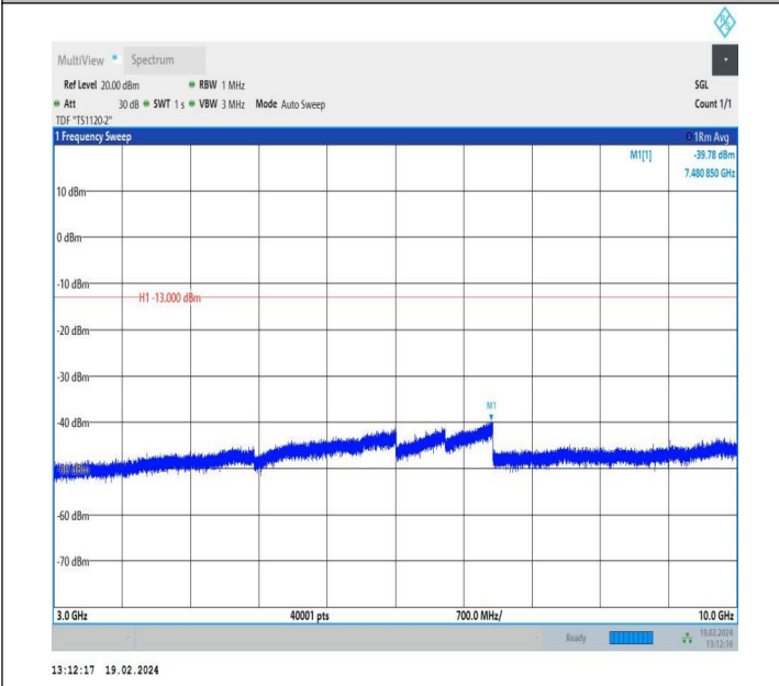
5-5-3MHz-5MHz-QPSK-QPSK-20586-20625-1RB#0-0RB#0-30 00~10000MHz-PASS
