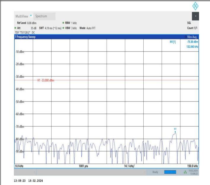
5-5-3MHz-5MHz-QPSK-QPSK-20416-20455-1RB#0-1RB#24-0. 009~0.15MHz-PASS
