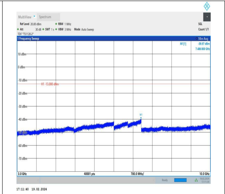
5-5-5MHz-3MHz-QPSK-QPSK-20425-20464-1RB#0-ORB#0-30 00~10000MHz-PASS
