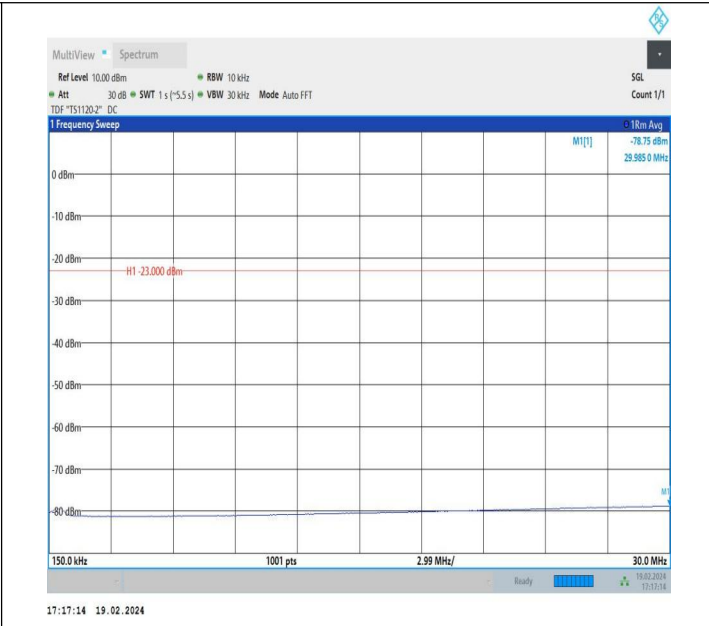
5-5-5MHz-3MHz-QPSK-QPSK-20595-20634-1RB#24-0RB#0-0. 15~30MHz-PASS
