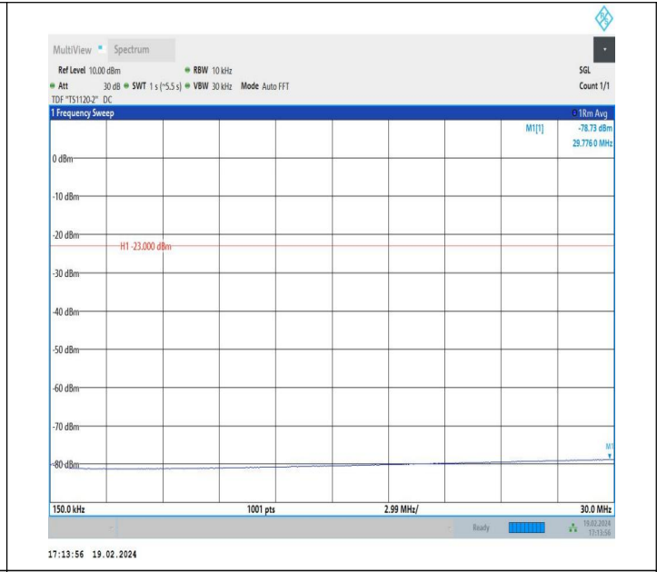
5-5-5MHz-3MHz-QPSK-QPSK-20510-20549-1RB#0-0RB#0-0.1 5~30MHz-PASS
