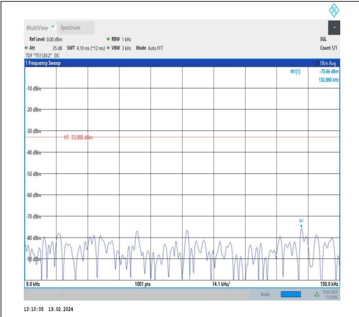
5-5-3MHz-5MHz-QPSK-QPSK-20501-20540-1RB#14-0RB#0-0. 009~0.15MHz-PASS
