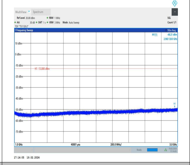
5-5-5MHz-3MHz-QPSK-QPSK-20510-20549-1RB#0-0RB#0-10 00~3000MHz-PASS
