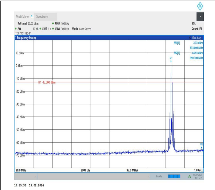
5-5-5MHz-3MHz-QPSK-QPSK-20510-20549-1RB#0-1RB#15-3 0~1000MHz-PASS
