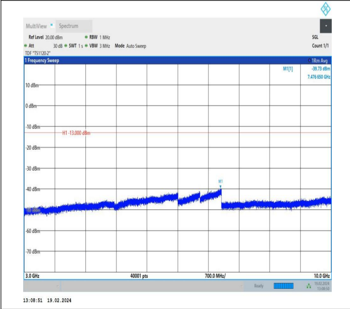
5-5-3MHz-5MHz-QPSK-QPSK-20416-20455-1RB#0-1RB#24-3 000~10000MHz-PASS
