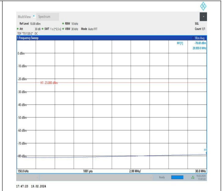
5-5-5MHz-10MHz-QPSK-QPSK-20428-20500-1RB#0-1RB#49- 0.15~30MHz-PASS
