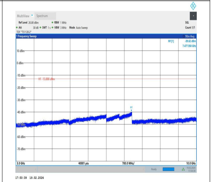
5-5-5MHz-10MHz-QPSK-QPSK-20478-20550-1RB#0-1RB#49- 3000~10000MHz-PASS
