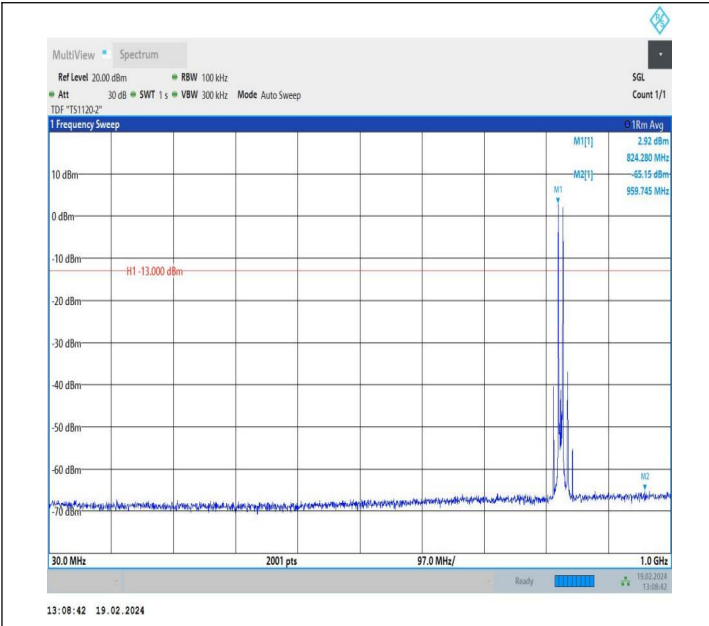
5-5-3MHz-5MHz-QPSK-QPSK-20416-20455-1RB#0-1RB#24-3 0~1000MHz-PASS
