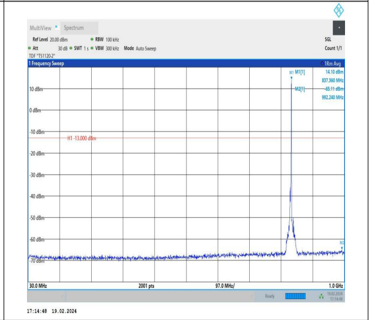
5-5-5MHz-3MHz-QPSK-QPSK-20510-20549-1RB#24-0RB#0-3 0~1000MHz-PASS
