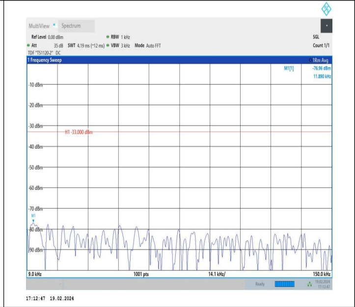
5-5-5MHz-3MHz-QPSK-QPSK-20425-20464-1RB#0-1RB#15-0. 009~0.15MHz-PASS
