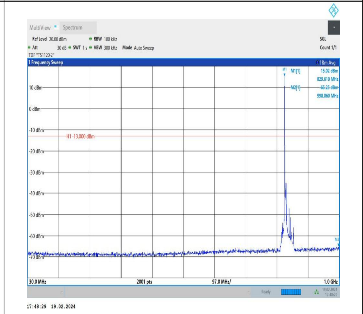
5-5-5MHz-10MHz-QPSK-QPSK-20478-20550-1RB#0-0RB#0-30.0~1000MHz-PASS
