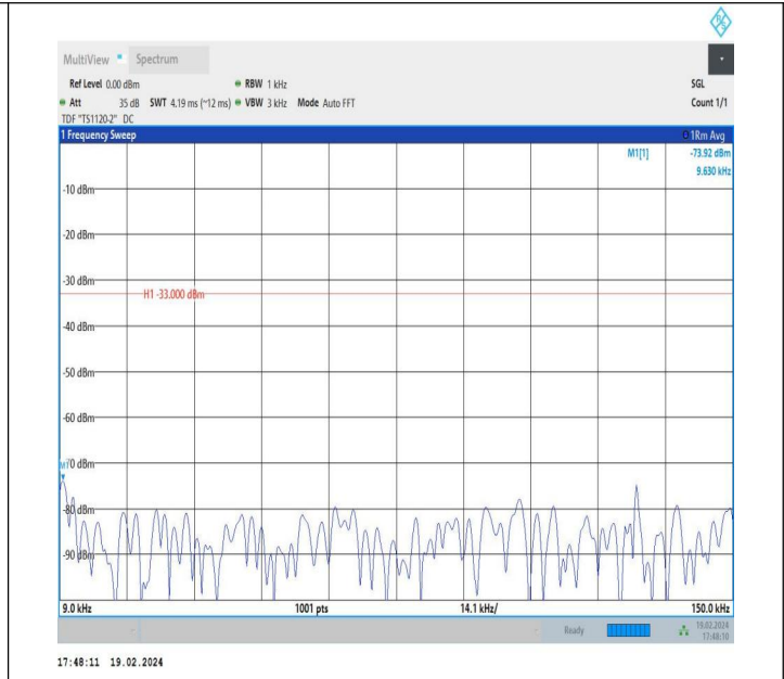
5-5-5MHz-10MHz-QPSK-QPSK-20478-20550-1RB#0-0RB#0-0.009~0.15MHz-PASS
