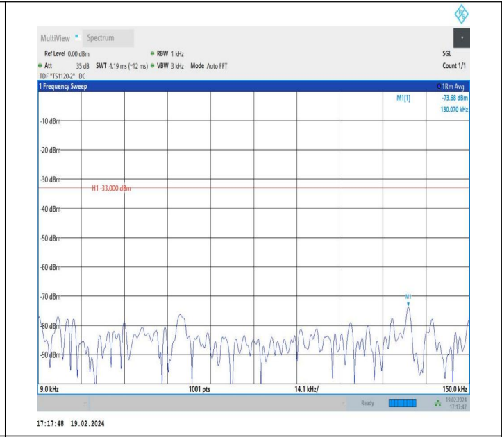
5-5-5MHz-3MHz-QPSK-QPSK-20595-20634-1RB#0-1RB#15-0. 009~0.15MHz-PASS
