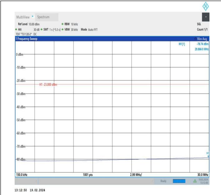
5-5-3MHz-5MHz-QPSK-QPSK-20586-20625-1RB#14-0RB#0-0. 15~30MHz-PASS
