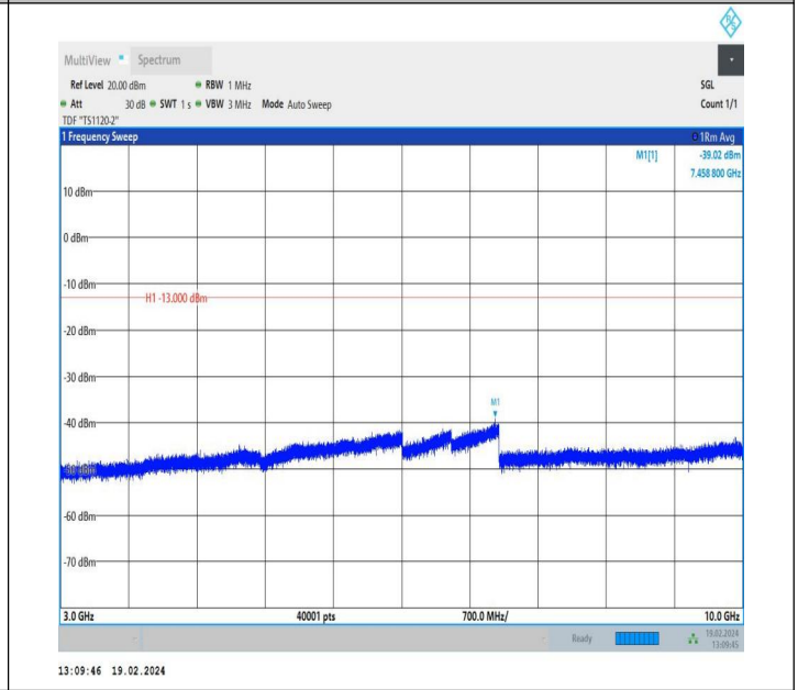
5-5-3MHz-5MHz-QPSK-QPSK-20501-20540-1RB#0-0RB#0-30 00~10000MHz-PASS
