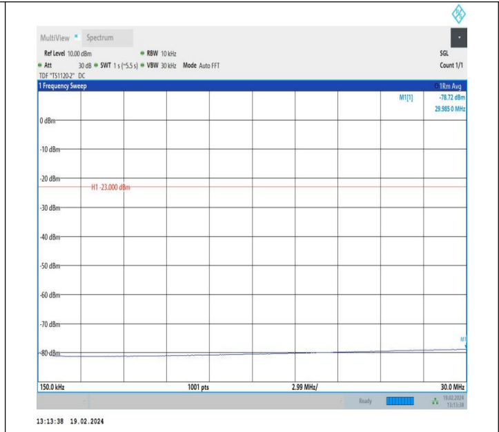
5-5-3MHz-5MHz-QPSK-QPSK-20586-20625-1RB#0-1RB#24-0. 15~30MHz-PASS
