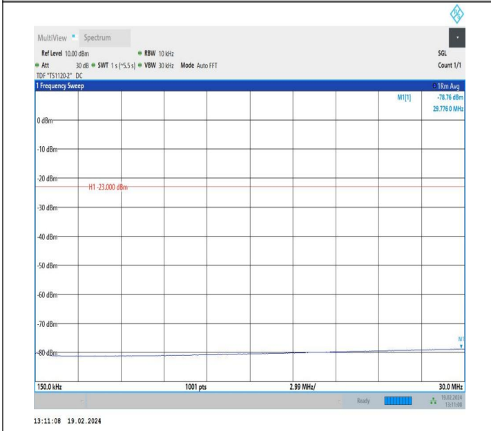
5-5-3MHz-5MHz-QPSK-QPSK-20501-20540-1RB#0-1RB#24-0. 15~30MHz-PASS
