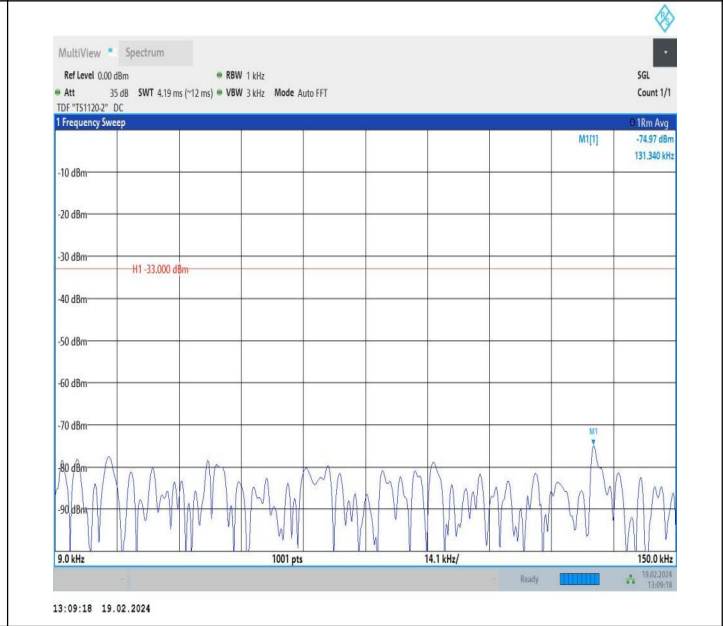
5-5-3MHz-5MHz-QPSK-QPSK-20501-20540-1RB#0-0RB#0-0.0 09~0.15MHz-PASS
