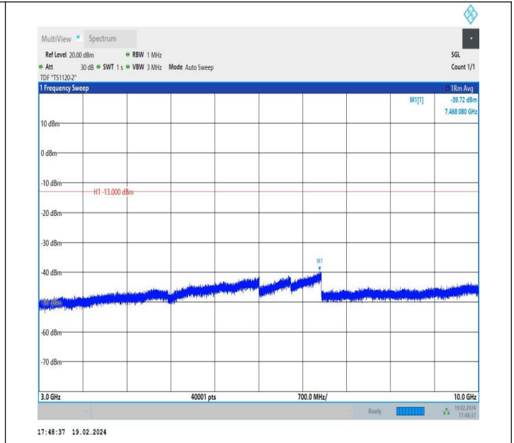
5-5-5MHz-10MHz-QPSK-QPSK-20478-20550-1RB#0-0RB#0-3 000~10000MHz-PASS
