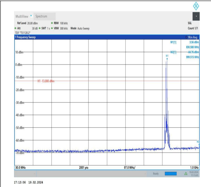
5-5-5MHz-3MHz-QPSK-QPSK-20425-20464-1RB#0-1RB#15-3 0~1000MHz-PASS
