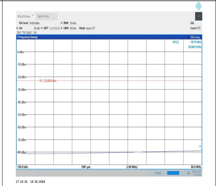
5-5-5MHz-3MHz-QPSK-QPSK-20510-20549-1RB#0-1RB#15-0. 15~30MHz-PASS
