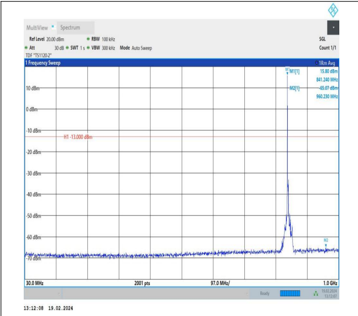
5-5-3MHz-5MHz-QPSK-QPSK-20586-20625-1RB#0-0RB#0-30 ~1000MHz-PASS
