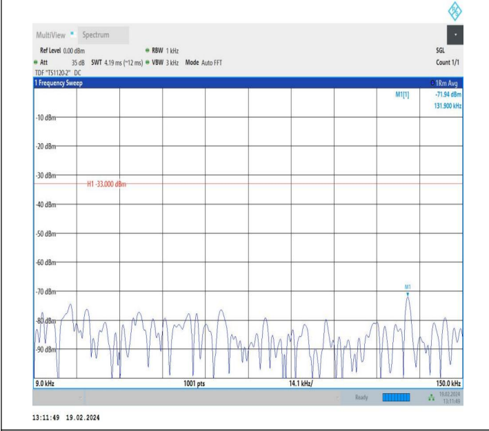
5-5-3MHz-5MHz-QPSK-QPSK-20586-20625-1RB#0-0RB#0-0.0 09~0.15MHz-PASS
