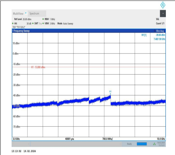
5-5-3MHz-5MHz-QPSK-QPSK-20586-20625-1RB#0-1RB#24-3 000~10000MHz-PASS
