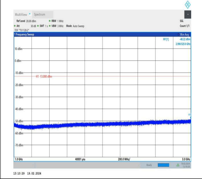
5-5-3MHz-5MHz-QPSK-QPSK-20501-20540-1RB#14-0RB#0-1 000~3000MHz-PASS
