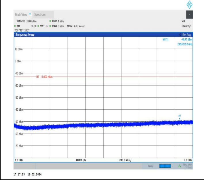
5-5-5MHz-3MHz-QPSK-QPSK-20595-20634-1RB#24-0RB#0-1 000~3000MHz-PASS
