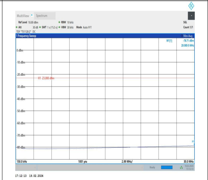
5-5-5MHz-3MHz-QPSK-QPSK-20425-20464-1RB#24-ORB#0-0. 15~30MHz-PASS
