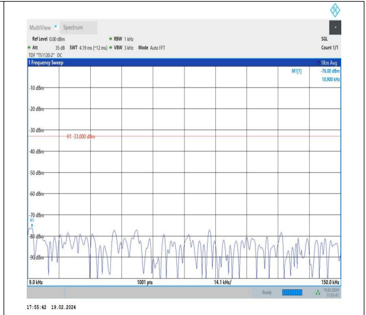
5-5-5MHz-10MHz-QPSK-QPSK-20528-20600-1RB#24-0RB#0- 0.009~0.15MHz-PASS
