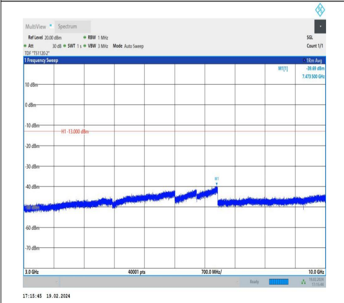
5-5-5MHz-3MHz-QPSK-QPSK-20510-20549-1RB#0-1RB#15-3 000~10000MHz-PASS
