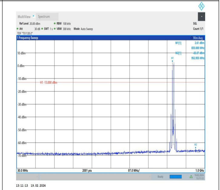
5-5-3MHz-5MHz-QPSK-QPSK-20501-20540-1RB#0-1RB#24-3 0~1000MHz-PASS
