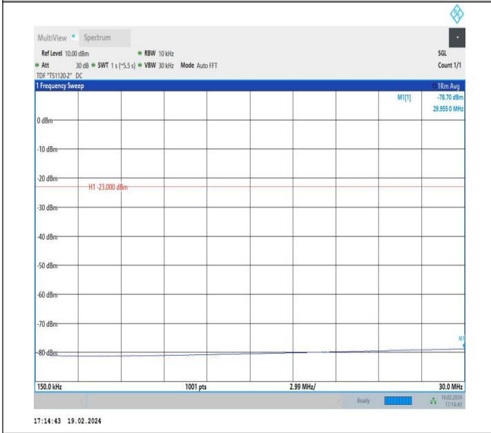
5-5-5MHz-3MHz-QPSK-QPSK-20510-20549-1RB#24-0RB#0-0. 15~30MHz-PASS
