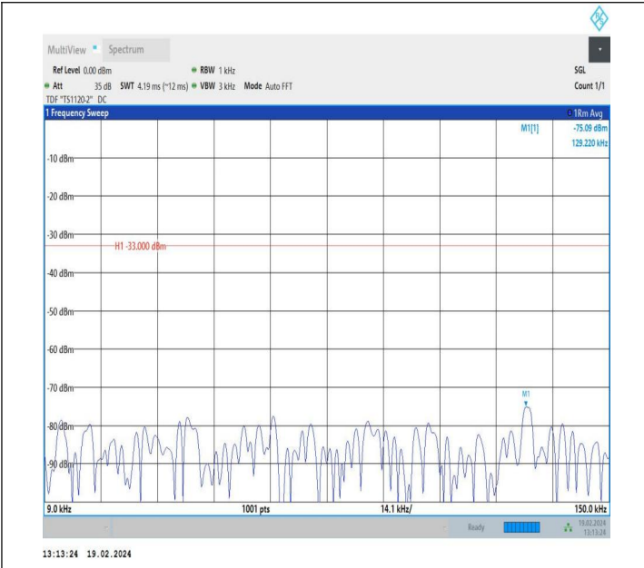
5-5-3MHz-5MHz-QPSK-QPSK-20586-20625-1RB#0-1RB#24-0. 009~0.15MHz-PASS
