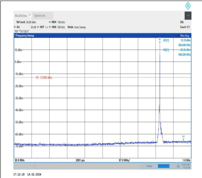
5-5-5MHz-3MHz-QPSK-QPSK-20425-20464-1RB#24-0RB#0-3 0~1000MHz-PASS
