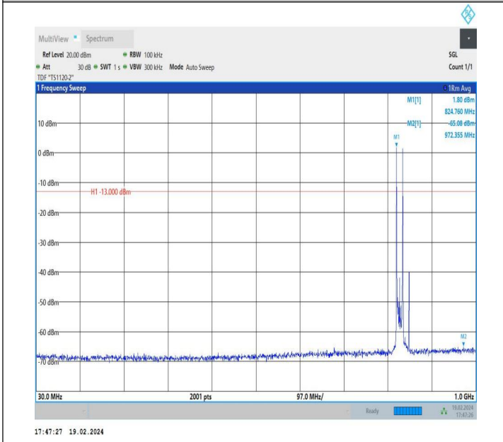
5-5-5MHz-10MHz-QPSK-QPSK-20428-20500-1RB#0-1RB#49- 30~1000MHz-PASS
