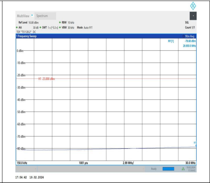
5-5-5MHz-10MHz-QPSK-QPSK-20528-20600-1RB#0-0RB#0-0.15~30MHz-PASS
