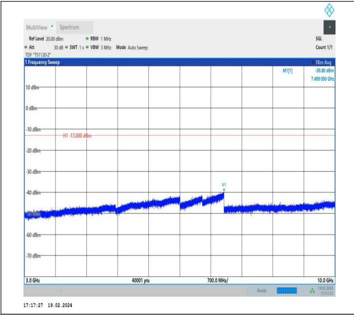
5-5-5MHz-3MHz-QPSK-QPSK-20595-20634-1RB#24-0RB#0-3 000~10000MHz-PASS
