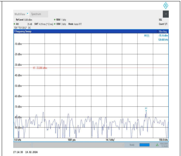
5-5-5MHz-3MHz-QPSK-QPSK-20510-20549-1RB#24-0RB#0-0. 009~0.15MHz-PASS
