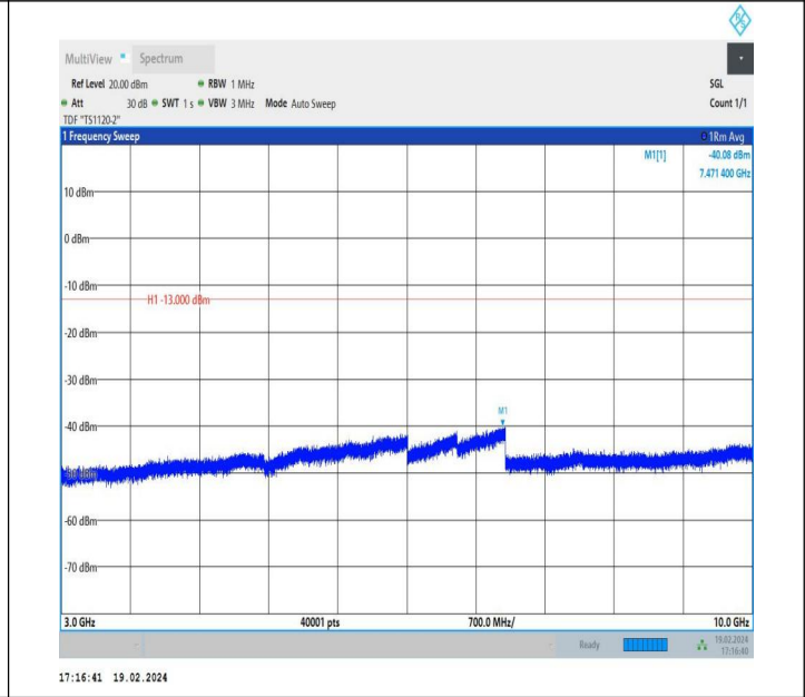
5-5-5MHz-3MHz-QPSK-QPSK-20595-20634-1RB#0-0RB#0-30 00~10000MHz-PASS
