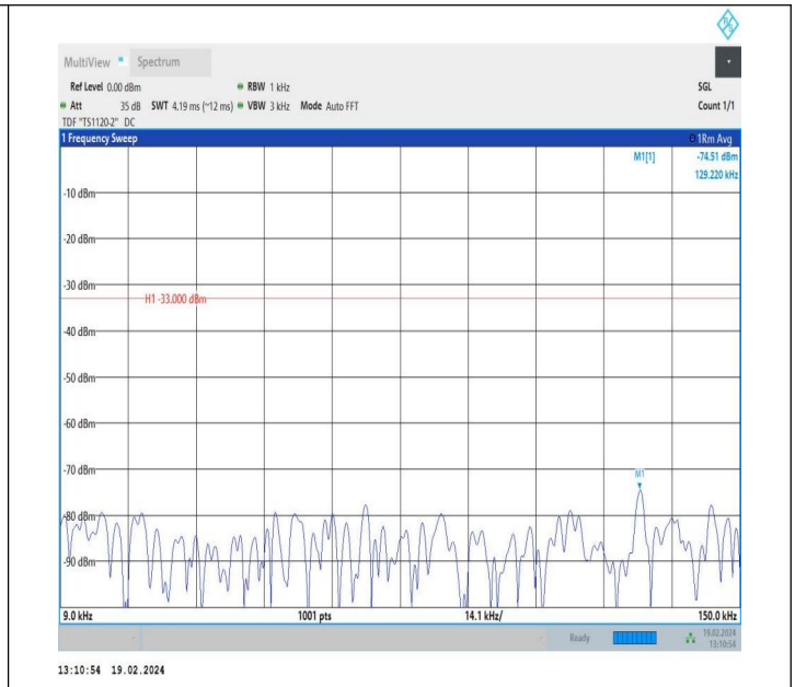
5-5-3MHz-5MHz-QPSK-QPSK-20501-20540-1RB#0-1RB#24-0. 009~0.15MHz-PASS
