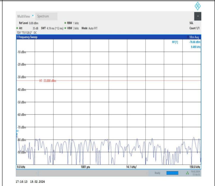
5-5-5MHz-3MHz-QPSK-QPSK-20595-20634-1RB#0-0RB#0-0.0 09~0.15MHz-PASS
