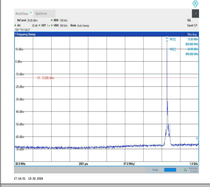
5-5-5MHz-3MHz-QPSK-QPSK-20510-20549-1RB#0-0RB#0-30 ~1000MHz-PASS
