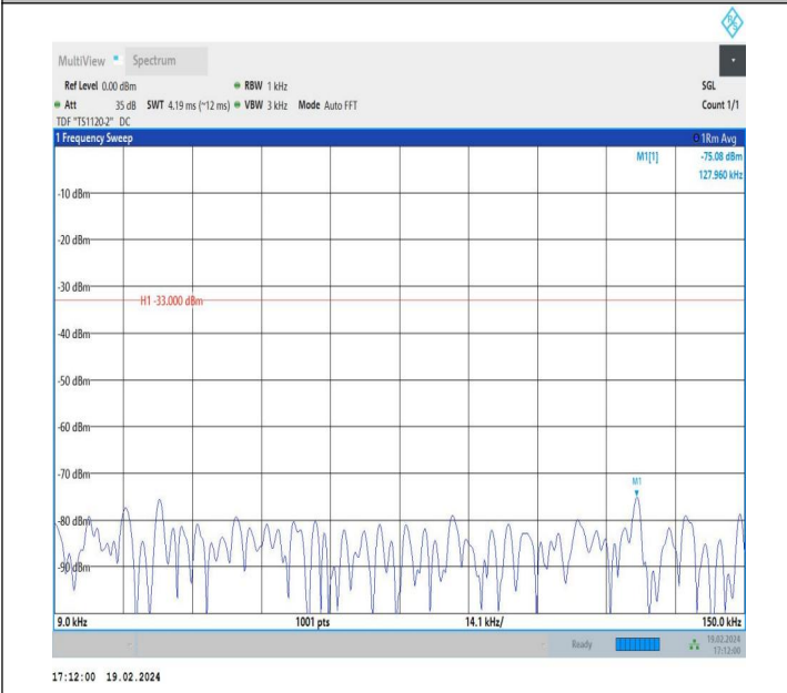
5-5-5MHz-3MHz-QPSK-QPSK-20425-20464-1RB#24-ORB#0-0. 009~0.15MHz-PASS
