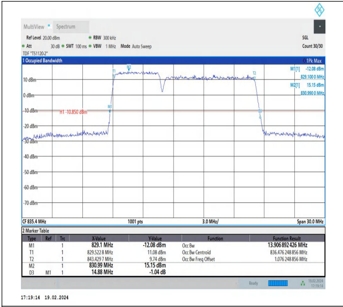
5-5-5MHz-10MHz-QPSK-QPSK-20478-20550-25RB#0-50RB#0-PASS
