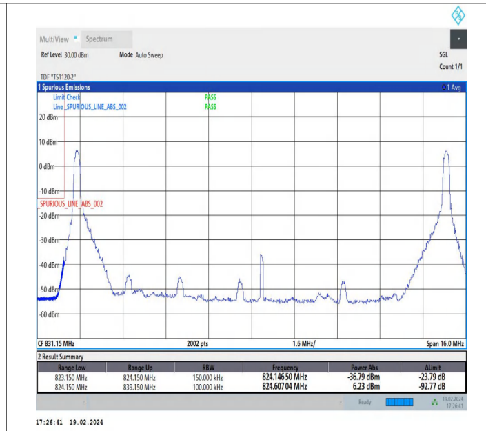
5MHz-10MHz_QPSK@QPSK-QPSK@QPSK_20428-20500_1 RB#0@25RB#0-1RB#49@50RB#0
