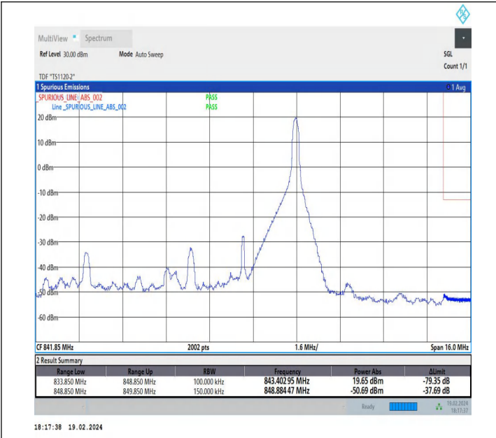
10MHz-5MHz_QPSK@QPSK-QPSK@QPSK_20550-20622_1R B#49@50RB#0-0RB#0@25RB#0
