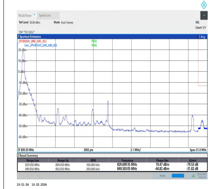
10MHz-10MHz_QPSK@QPSK-QPSK@QPSK_20501-20600_1 RB#0@50RB#0-0RB#0@50RB#0
