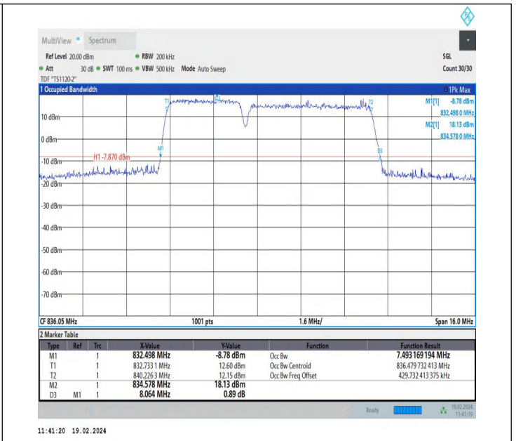
5-5-3MHz-5MHz-16QAM-16QAM-20501-20540-15RB#0-25RB#0- -PASS
