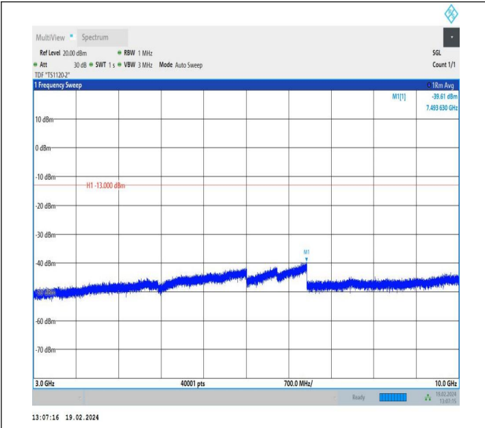
5-5-3MHz-5MHz-QPSK-QPSK-20416-20455-1RB#0-0RB#0-30 00~10000MHz-PASS
