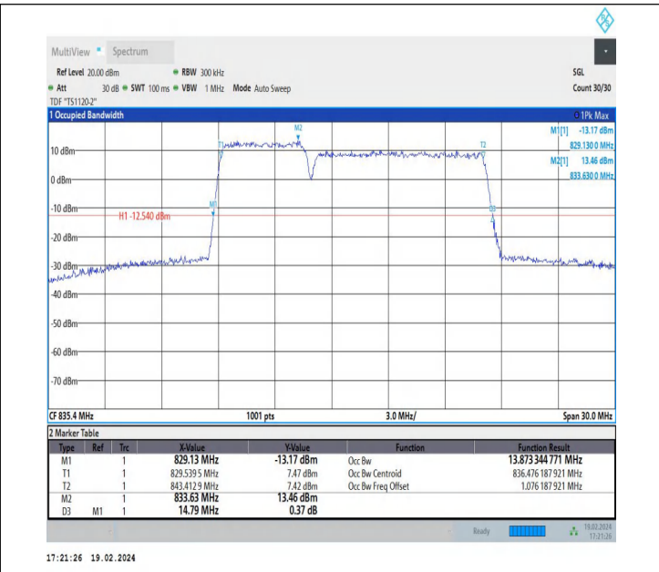
5-5-5MHz-10MHz-256QAM-256QAM-20478-20550-25RB#0-50R B#0-PASS
