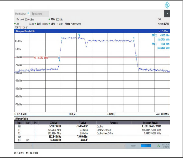
5-5-5MHz-10MHz-16QAM-16QAM-20478-20550-25RB#0-50RB#0-PASS
