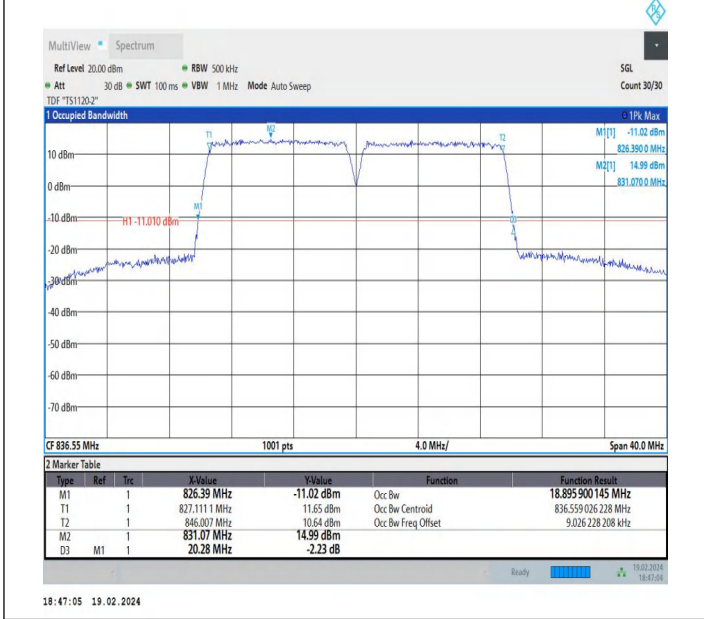
5-5-10MHz-10MHz-QPSK-QPSK-20476-20575-50RB#0-50RB #0-PASS
