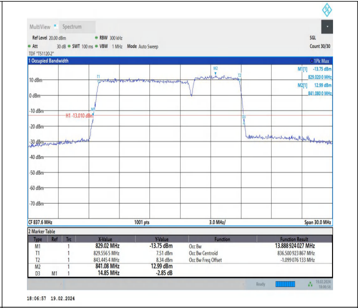
5-5-10MHz-5MHz-256QAM-256QAM-20500-20572-50RB#0-25R B#0-PASS
