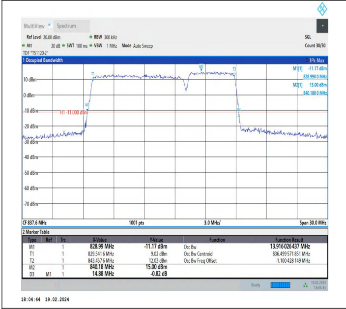
5-5-10MHz-5MHz-QPSK-QPSK-20500-20572-50RB#0-25RB# 0-PASS
