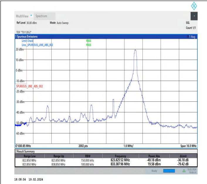
10MHz-5MHz_QPSK@QPSK-QPSK@QPSK_20450-20522_1R B#49@50RB#0-0RB#0@25RB#0
