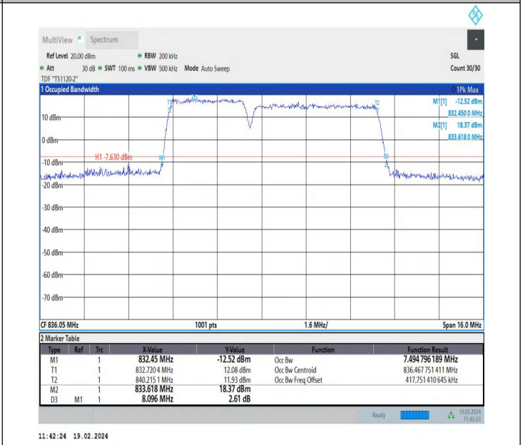
5-5-3MHz-5MHz-256QAM-256QAM-20501-20540-15RB#0-25RB#0- #0-PASS
