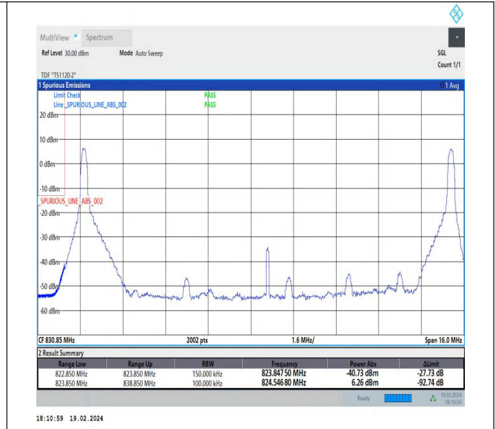
10MHz-5MHz_QPSK@QPSK-QPSK@QPSK_20450-20522_1 RB#0@50RB#0-1RB#24@25RB#0
