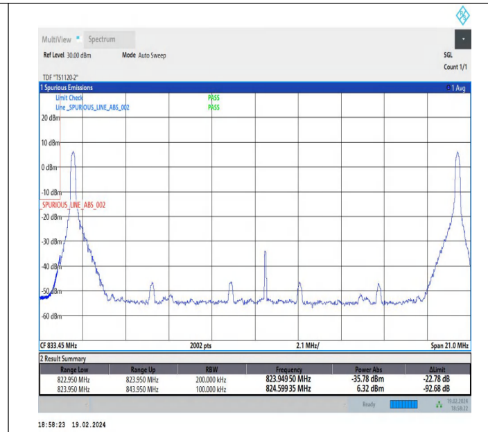
10MHz-10MHz_QPSK@QPSK-QPSK@QPSK_20450-20549_1 RB#0@50RB#0-1RB#49@50RB#0
