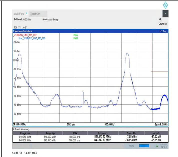
5MHz-3MHz_QPSK@QPSK-QPSK@QPSK_20595-20634_1RB #0@25RB#0-1RB#15@15RB#0
