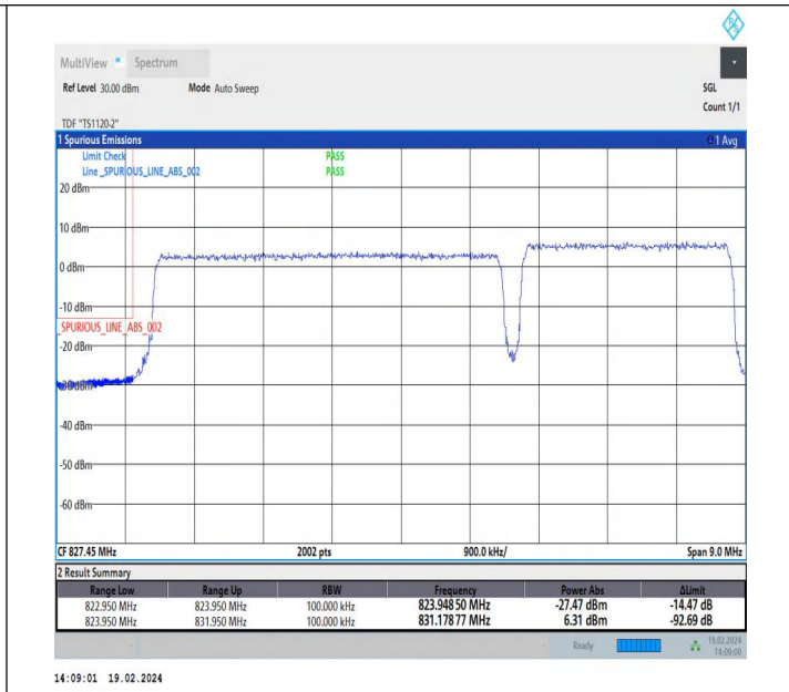
5MHz-3MHz_QPSK@QPSK-QPSK@QPSK_20425-20464_25RB#0@25RB#0-15RB#0@15RB#0
