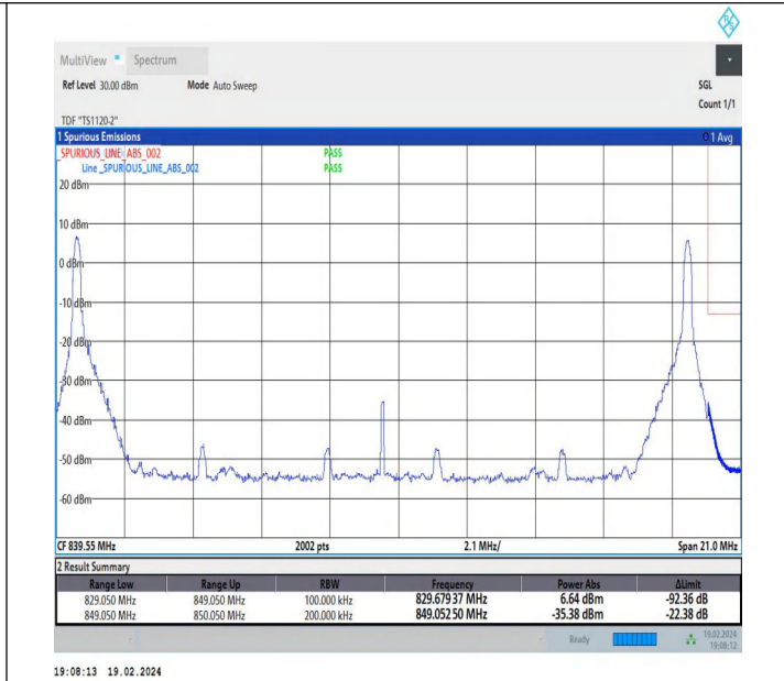
10MHz-10MHz_QPSK@QPSK-QPSK@QPSK_20501-20600_1 RB#0@50RB#0-1RB#49@50RB#0
