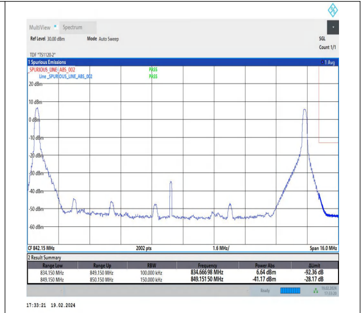
5MHz-10MHz_QPSK@QPSK-QPSK@QPSK_20528-20600_1 RB#0@25RB#0-1RB#49@50RB#0
