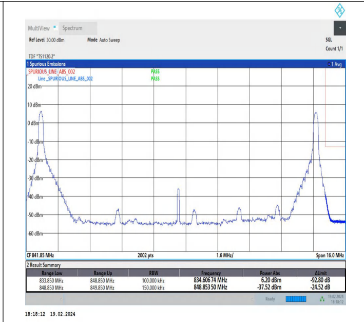
10MHz-5MHz_QPSK@QPSK-QPSK@QPSK_20550-20622_1 RB#0@50RB#0-1RB#24@25RB#0
