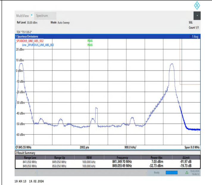
3MHz-5MHz_QPSK@QPSK-QPSK@QPSK_20586-20625_1RB#0@15RB#0-1RB#24@25RB#0
