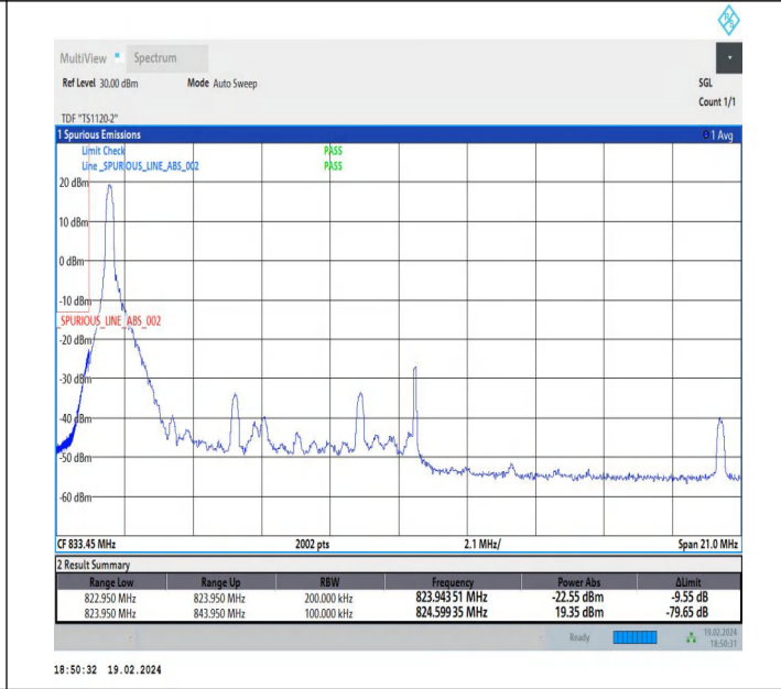
10MHz-10MHz_QPSK@QPSK-QPSK@QPSK_20450-20549_1 RB#0@50RB#0-0RB#0@50RB#0
