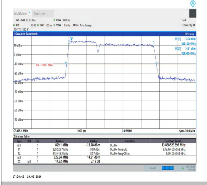
5-5-5MHz-10MHz-64QAM-64QAM-20478-20550-25RB#0-50RB#0-PASS
