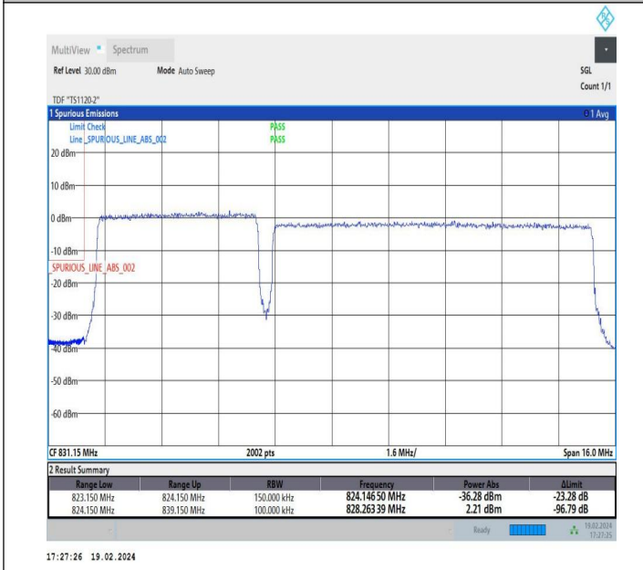
5MHz-10MHz_QPSK@QPSK-QPSK@QPSK_20428-20500_25 RB#0@25RB#0-50RB#0@50RB#0
