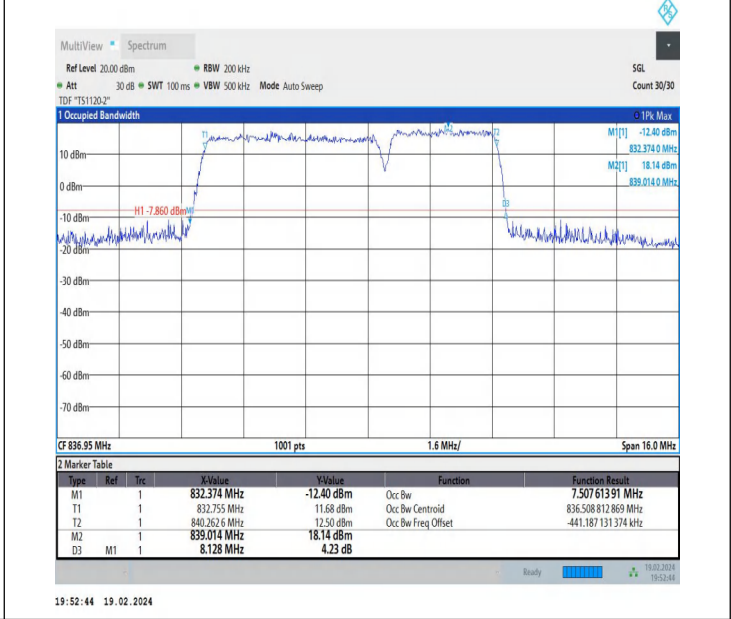
5-5-5MHz-3MHz-256QAM-256QAM-20510-20549-25RB#0-15RB #0-PASS
