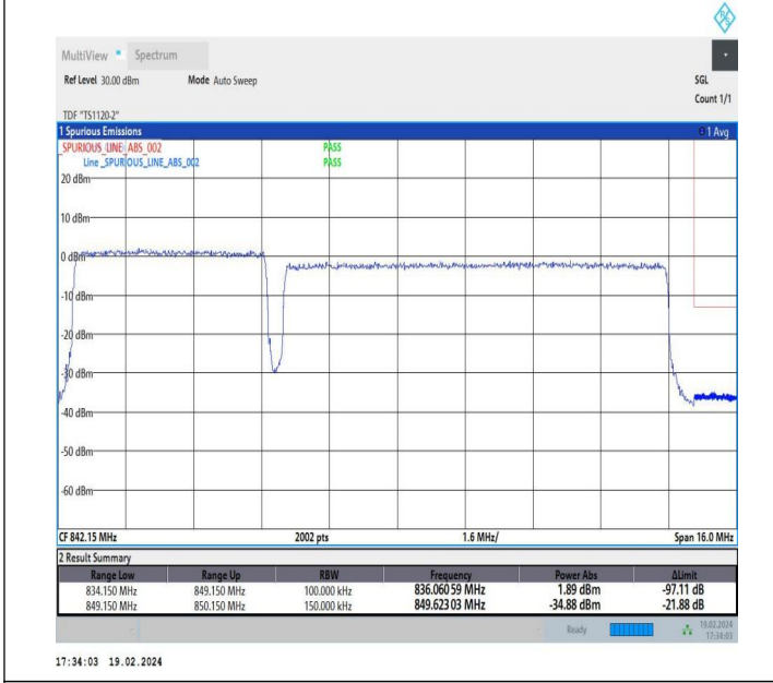
5MHz-10MHz_QPSK@QPSK-QPSK@QPSK_20528-20600_25 RB#0@25RB#0-50RB#0@50RB#0
