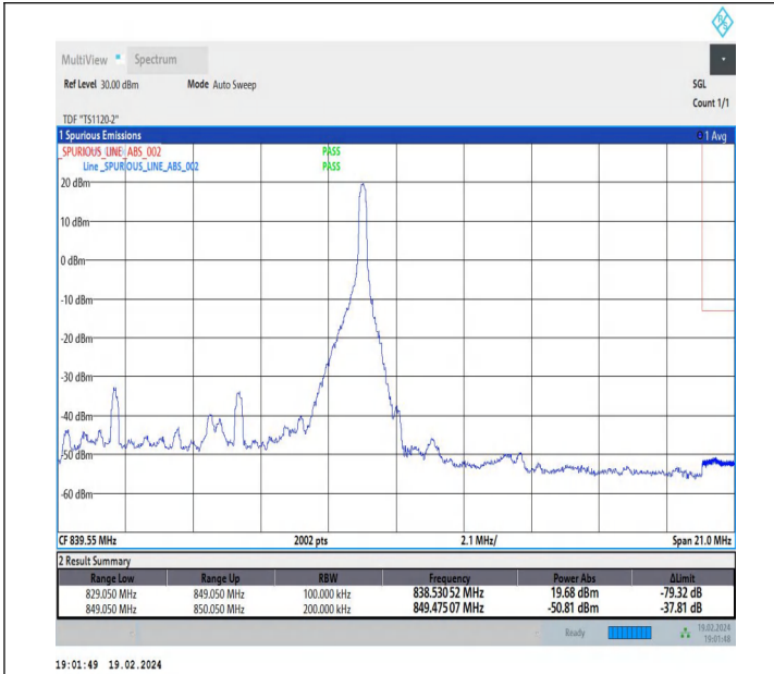
10MHz-10MHz_QPSK@QPSK-QPSK@QPSK_20501-20600_1 RB#49@50RB#0-0RB#0@50RB#0
