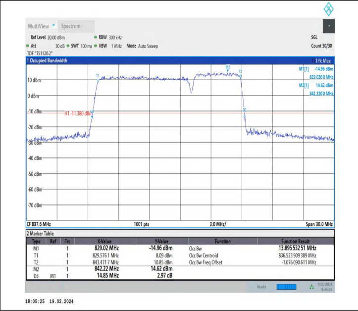
5-5-10MHz-5MHz-16QAM-16QAM-20500-20572-50RB#0-25RB# 0-PASS
