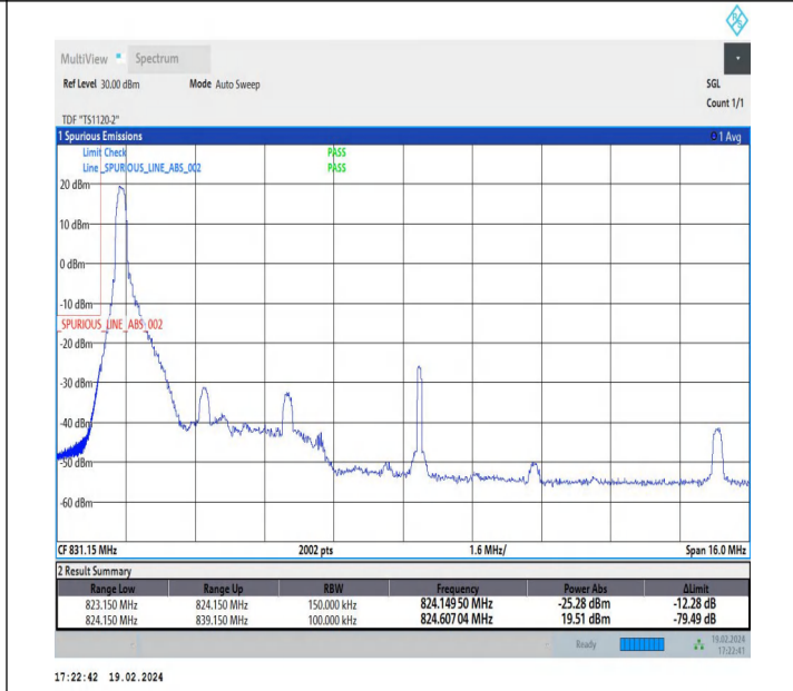
5MHz-10MHz_QPSK@QPSK-QPSK@QPSK_20428-20500_1RB#0@25RB#0-0RB#0@50RB#0
