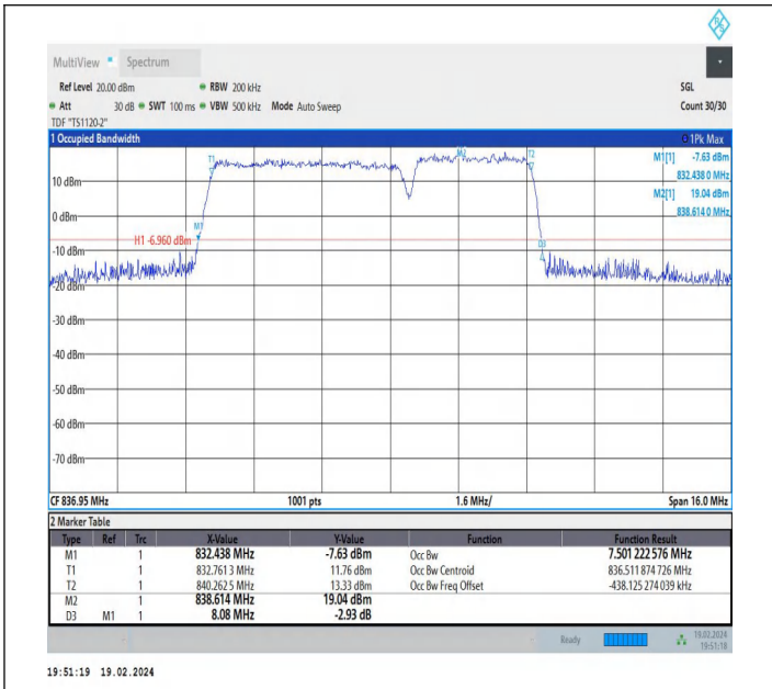
5-5-5MHz-3MHz-16QAM-16QAM-20510-20549-25RB#0-15RB #0-PASS
