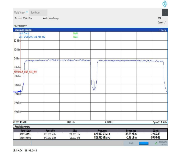
10MHz-10MHz_QPSK@QPSK-QPSK@QPSK_20450-20549_5 0RB#0@50RB#0-50RB#0@50RB#0
