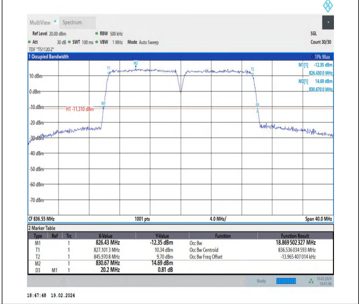
5-5-10MHz-10MHz-16QAM-16QAM-20476-20575-50RB#0-50RB #0-PASS
