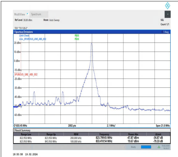
10MHz-10MHz_QPSK@QPSK-QPSK@QPSK_20450-20549_1 RB#49@50RB#0-0RB#0@50RB#0
