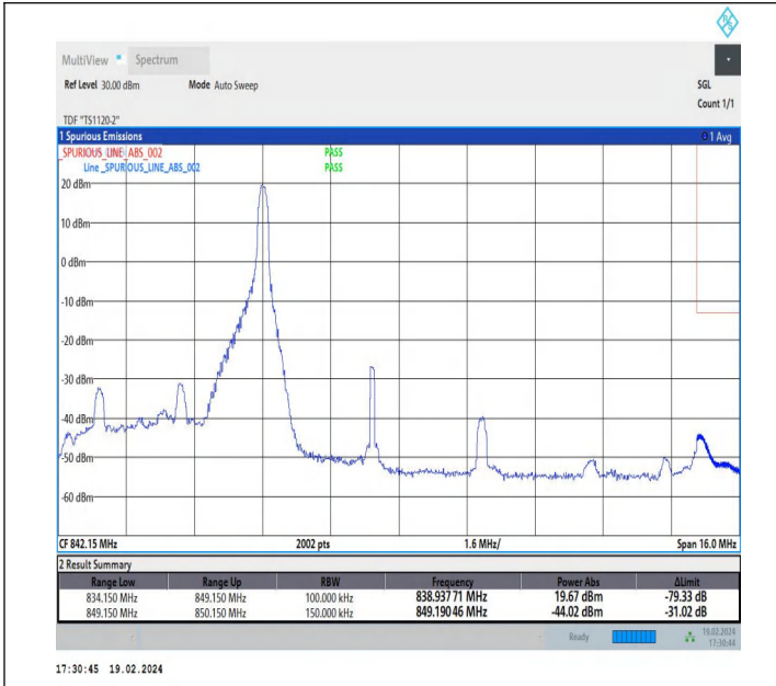
5MHz-10MHz_QPSK@QPSK-QPSK@QPSK_20528-20600_1R B#24@25RB#0-0RB#0@50RB#0
