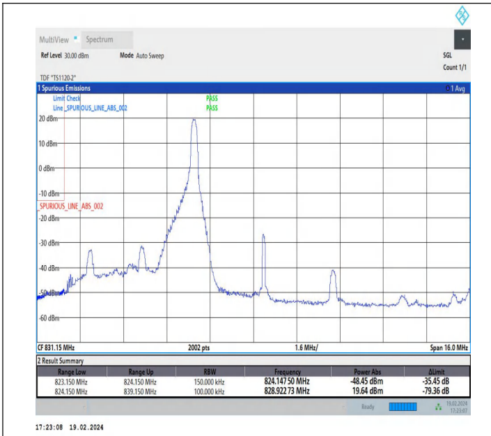
5MHz-10MHz_QPSK@QPSK-QPSK@QPSK_20428-20500_1R B#24@25RB#0-0RB#0@50RB#0
