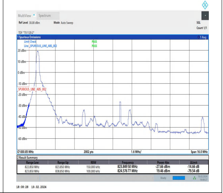
10MHz-5MHz_QPSK@QPSK-QPSK@QPSK_20450-20522_1 RB#0@50RB#0-0RB#0@25RB#0
