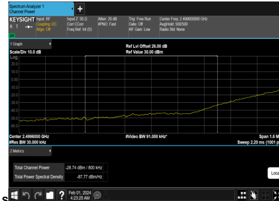
N7(40M)_DFT-s-OFDM_BPSK_Edge_1RB_Left_Low_CH_CHP_PAS
