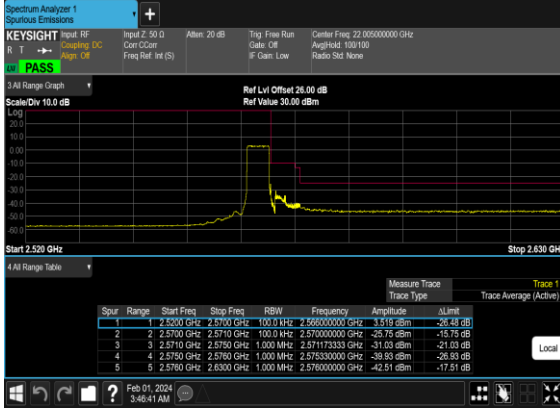
N7(5M)_DFT-s- OFDM_BPSK_Outer_Full_High_CH
