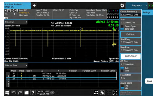
NTNV-11A-CDD-Ant1-5500
