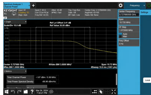
11AC20MIMO-Ant1-5745-PASS
