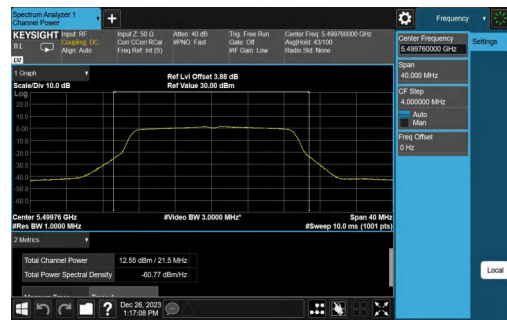
11AC20MIMO-Ant1-5500-TPC_L-PASS
