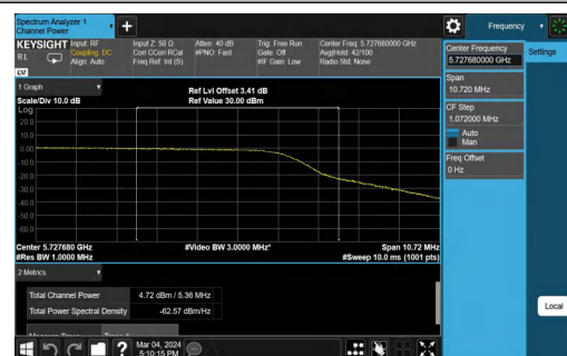
11AC20MIMO-Ant1-5720_UNII-3-TPC_L-PASS
