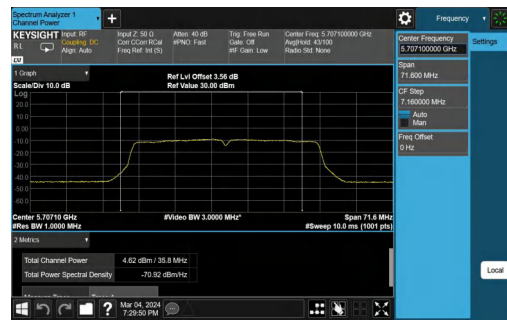
11N40MIMO-Ant1-5710_UNII-3-TPC_H-PASS
