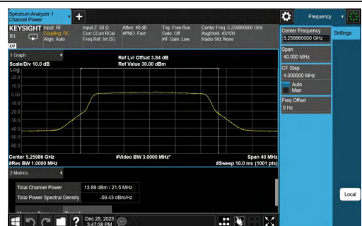
11AC20SISO-Ant1-5260-TPC_L-PASS
