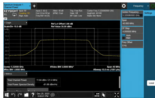
11AC20MIMO-Ant1-5320-TPC_L-PASS
