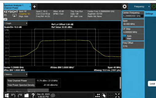
11AC20MIMO-Ant1-5300-TPC_L-PASS
