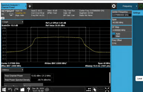
11AC20SISO-Ant0-5580-TPC_L-PASS
