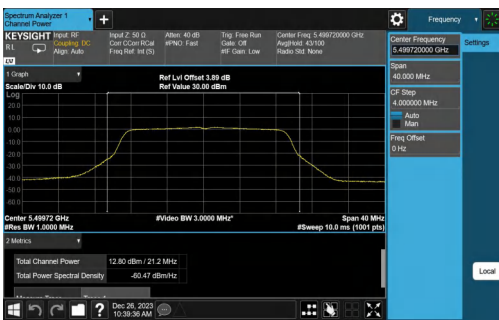
11AC20SISO-Ant0-5500-TPC_L-PASS
