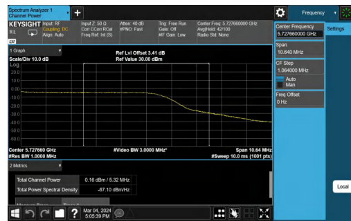
11N40MIMO-Ant1-5710_UNII-3-TPC_L-PASS
