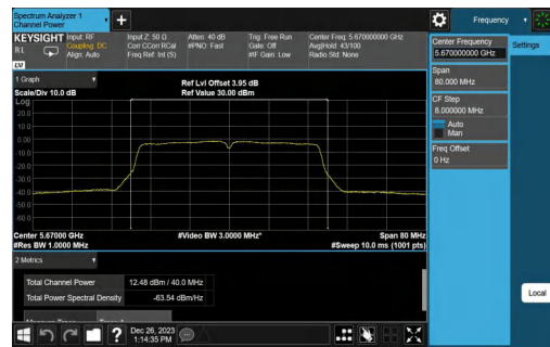
11N40MIMO-Ant1-5670-TPC_L-PASS
