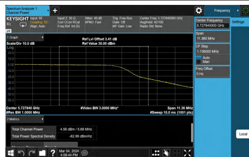
11N20MIMO-Ant1-5720_UNII-3-TPC_L-PASS
