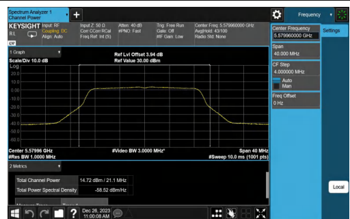
11N20SISO-Ant1-5580-TPC_L-PASS
