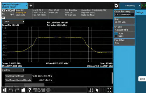
11N20SISO-Ant0-5500-TPC_L-PASS
