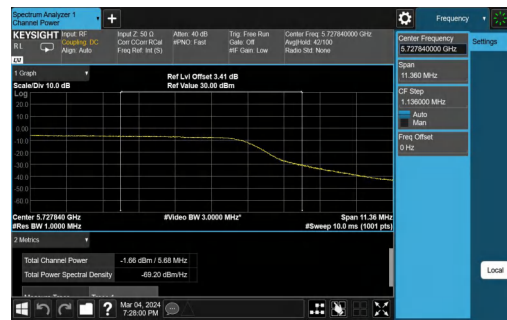
11N20MIMO-Ant1-5745-PASS
