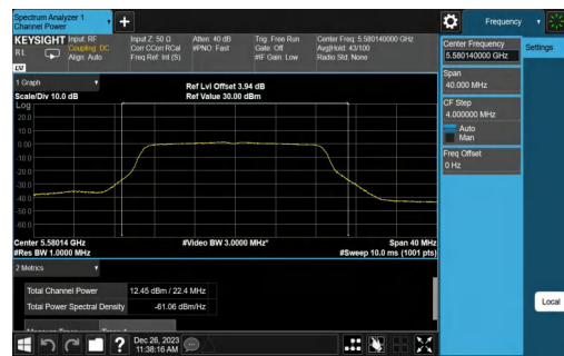
11N20MIMO-Ant1-5580-TPC_L-PASS
