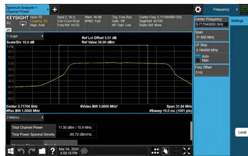
11N20MIMO-Ant1-5720_UNII-2C-TPC_L-PASS
