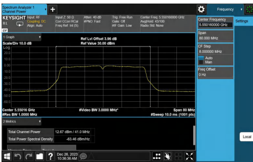
11N40SISO-Ant0-5550-TPC_L-PASS
