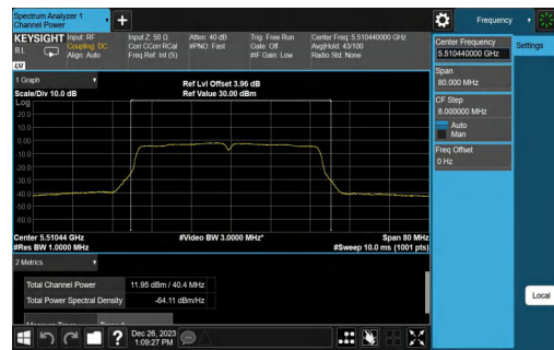
11N40MIMO-Ant1-5510-TPC_L-PASS
