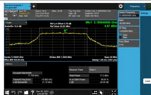
11AC20MIMO-Ant1-5180
