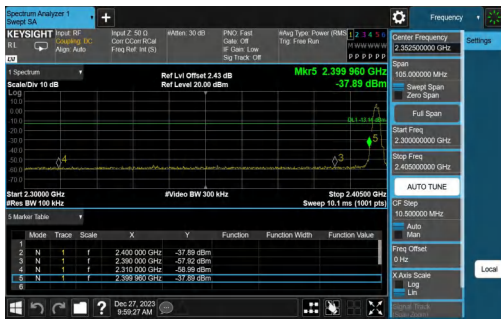
BLE_2M-Ant0-2402-PASS
