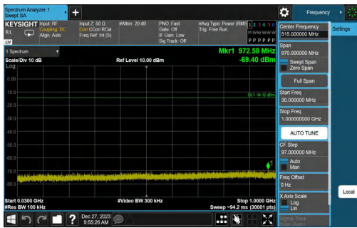
BLE_1M-Ant0-2480-30~1000-PASS
