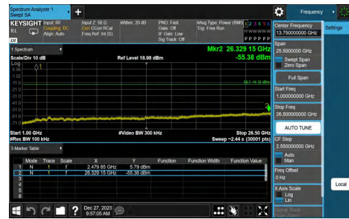
BLE_1M-Ant0-2480-1000~26500-PASS
