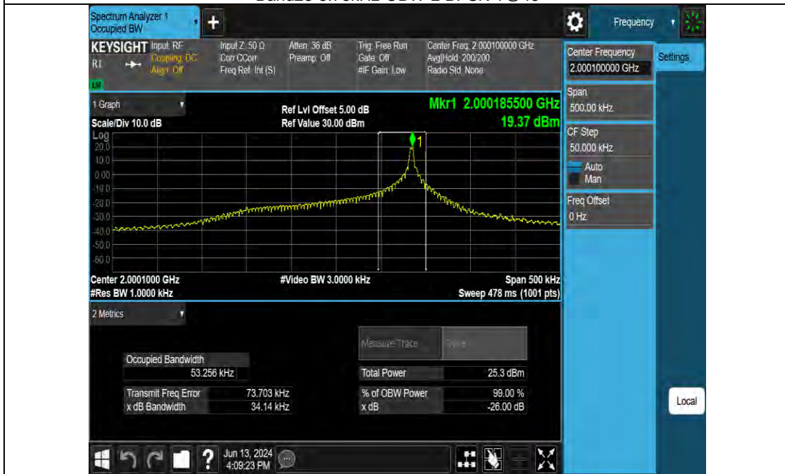
Band23-3.75kHz-OBW-M-QPSK-1 @ 1
