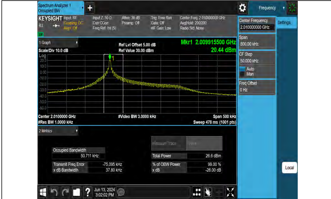
Band23-3.75kHz-OBW-M-QPSK-1 @46
