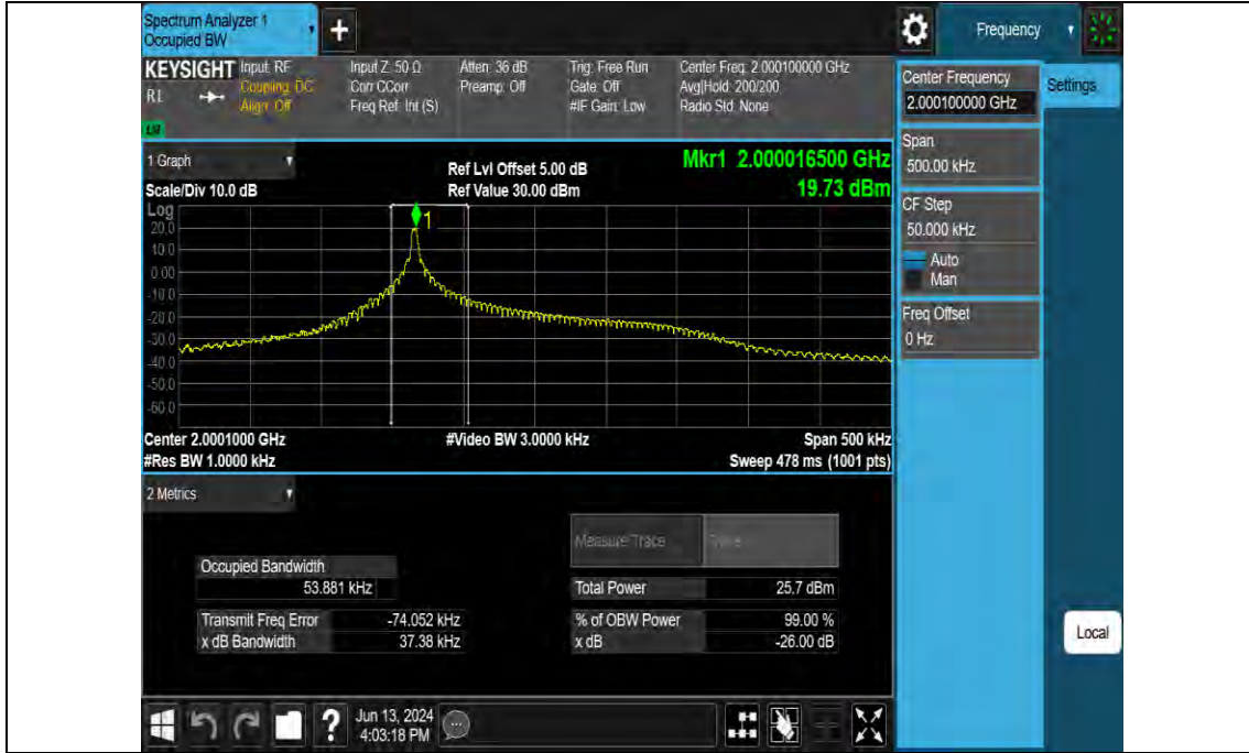
Band23-3.75kHz-OBW-L-BPSK-1 @ 46
