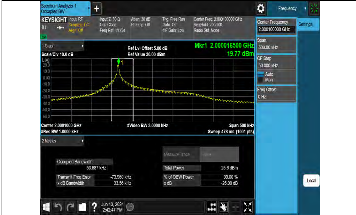
Band23-3.75kHz-OBW-L-QPSK-1 @ 46
