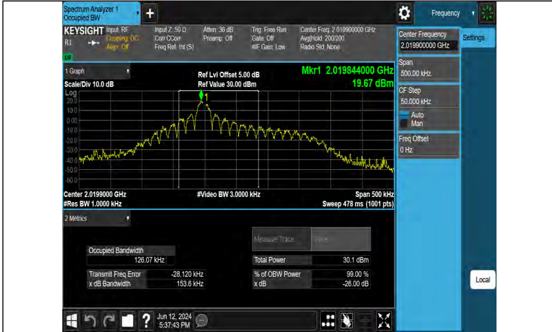
Band23-15kHz-OBW-H-QPSK-1@10
