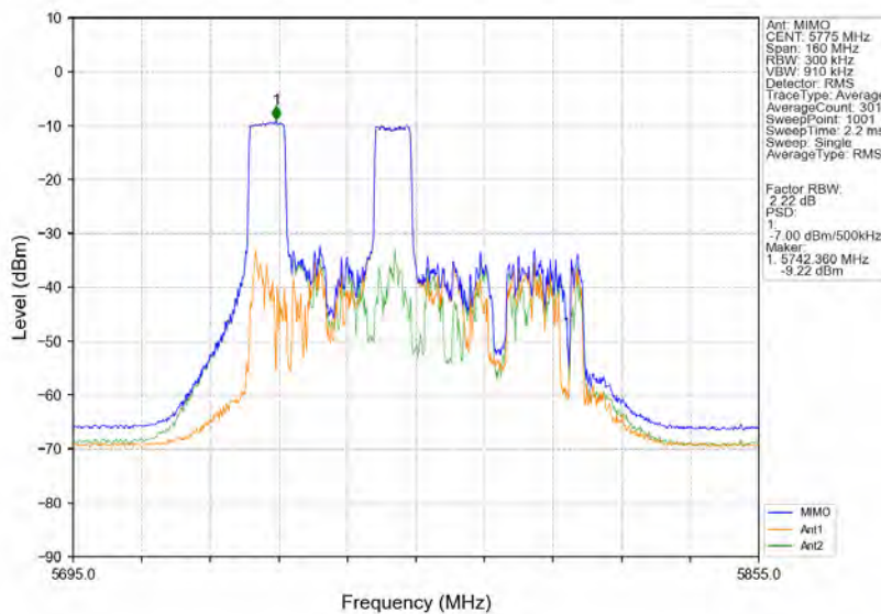
802.11ax(HE80) MCH 5775MHz RU106 Left MIMO NTN
