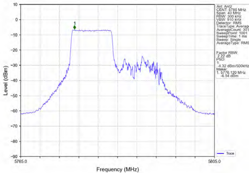
802.11ax(HE20)_MCH_5785MHz_RU106_Left_MIMO_NTNV
