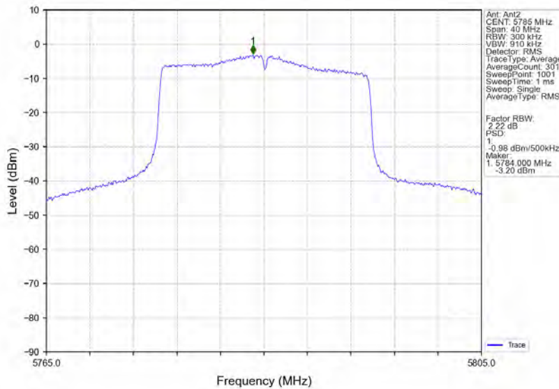
802.11ax(HE20)_MCH_5785MHz_RU242_Left_MIMO_NTNV
