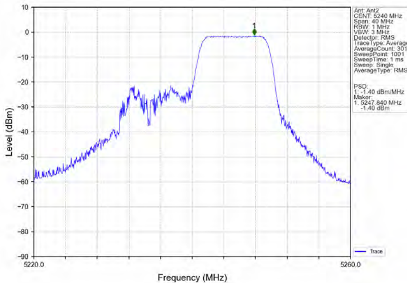
802.11ax(HE20) HCH 5240MHz RU106 Right Ant2 NTVN
