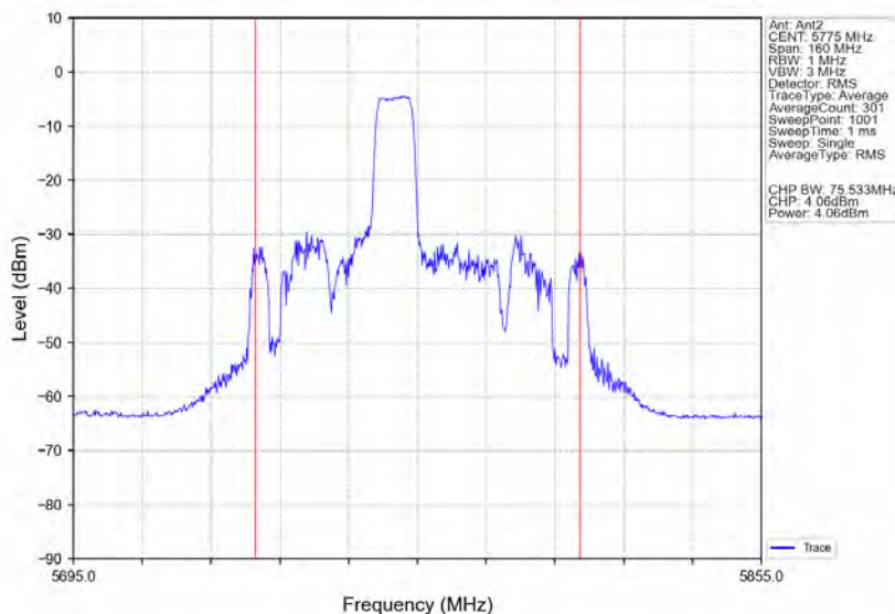
802.11ax(HE80) MCH 5775MHz RU106 Mid Ant2 NTN
