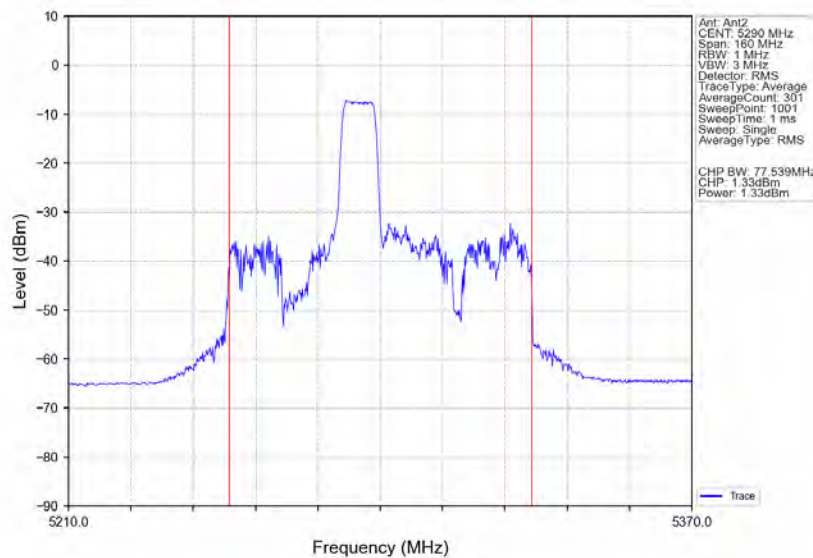
802.11ax(HE80) MCH 5290MHz RU106 Mid Ant2 NTN
