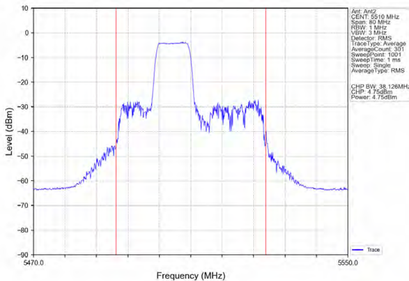
802.11ax(HE40) LCH 5510MHz RU106 Mid Ant2 NTN
