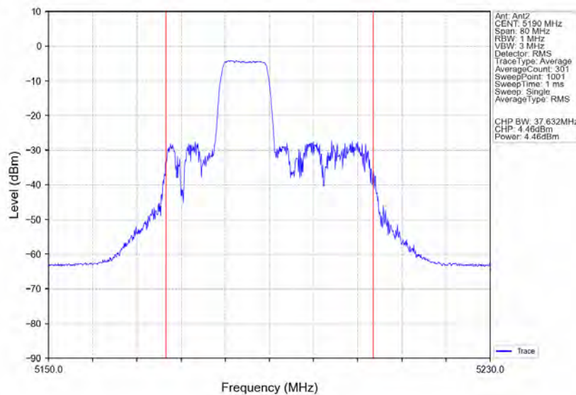
802.11ax(HE40) LCH 5190MHz RU106 Mid Ant2 NTN
