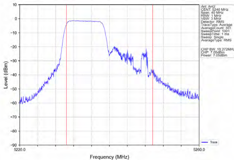
802.11ax(HE20) HCH 5240MHz RU106 Left Ant2 NTNv
