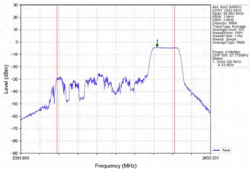
802.11ax(HE40) LCH 2422MHz RU106 Right Ant2 (MIMO) NTNW
