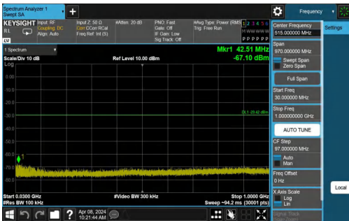
11N40SISO-Ant1-2452-30~1000-PASS
