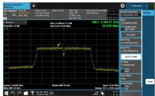
11N40SISO-Ant1-2452-PASS
