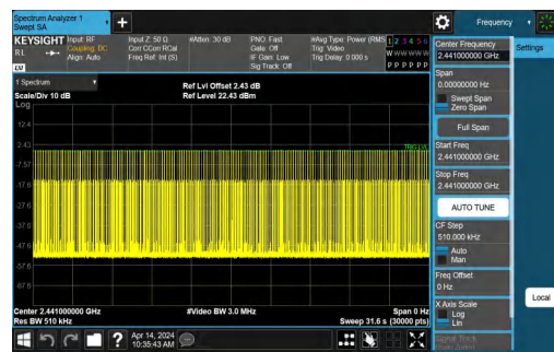
2DH3-Ant1-Hop-PASS
