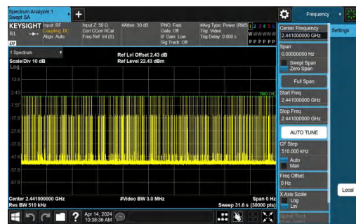
2DH5-Ant1-Hop-PASS
