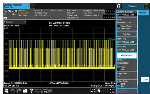
3DH3-Ant1-Hop-PASS
